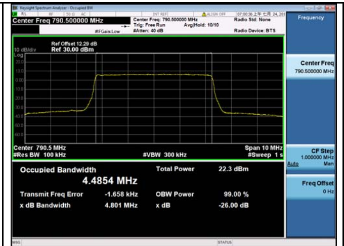
LTE band 14 - Low CH 16QAM-5
