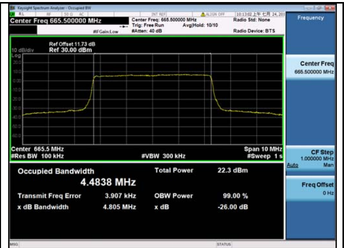
LTE band 71 - Low CH 16QAM-5
