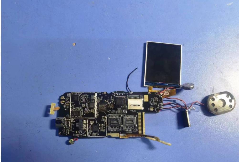
Photo 15 Appearance of PCB
