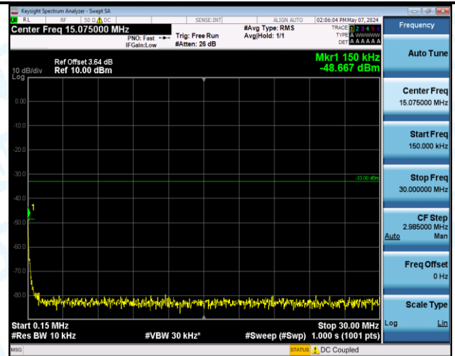
Band2_15MHz_16QAM_18675_1RB#0_1000~3000_1000~3000
