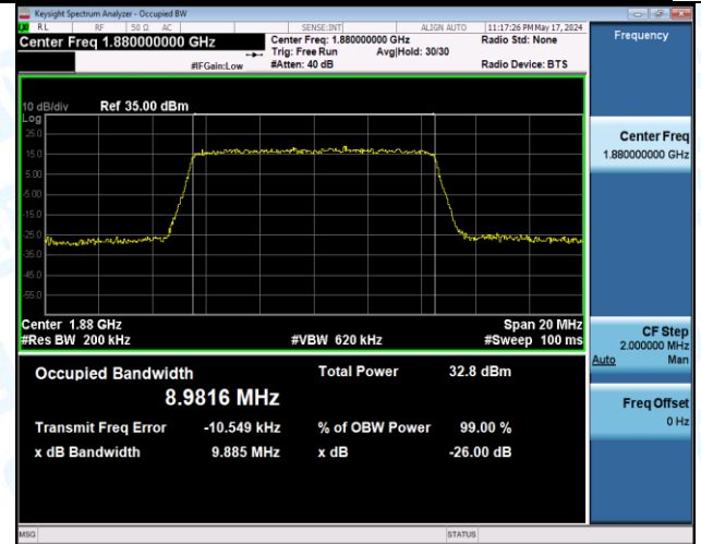
Band2-10MHz-16QAM-18650-27RB#0-PASS
