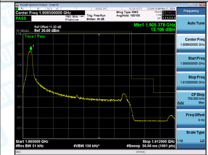
Band2_5MHz_16QAM_19175_25RB#0
