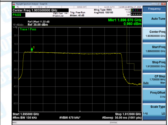
Band2_15MHz_QPSK_19125_75RB#4
