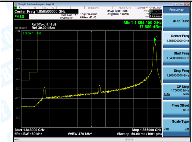
Band2_15MHz_16QAM_18675_1RB#74
