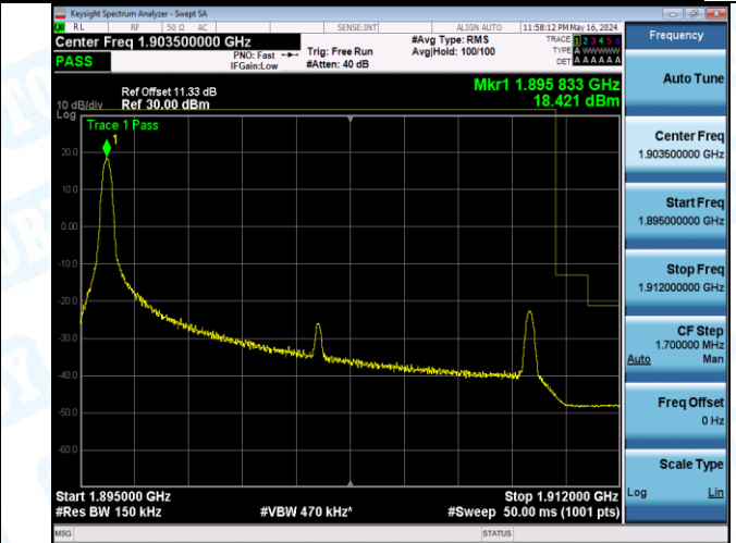
Band2_15MHz_QPSK_19125_75RB#0
