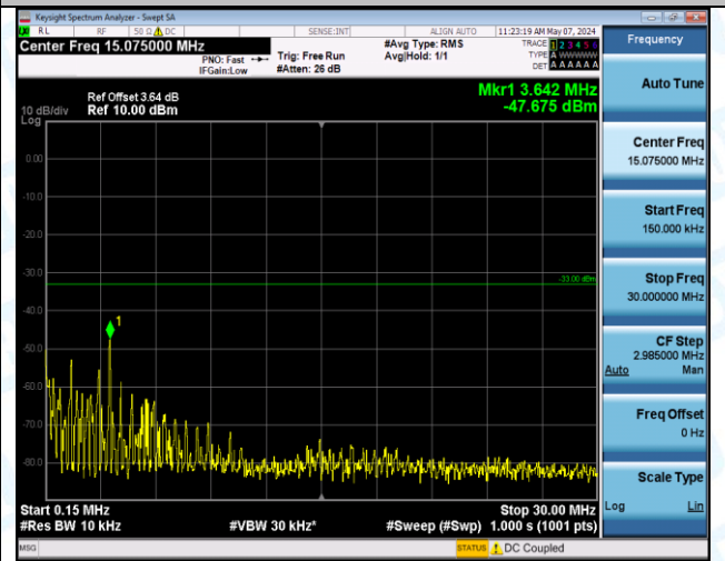
Band2_1.4MHz_16QAM_18607_1RB#5_1000~3000_1000~3000
