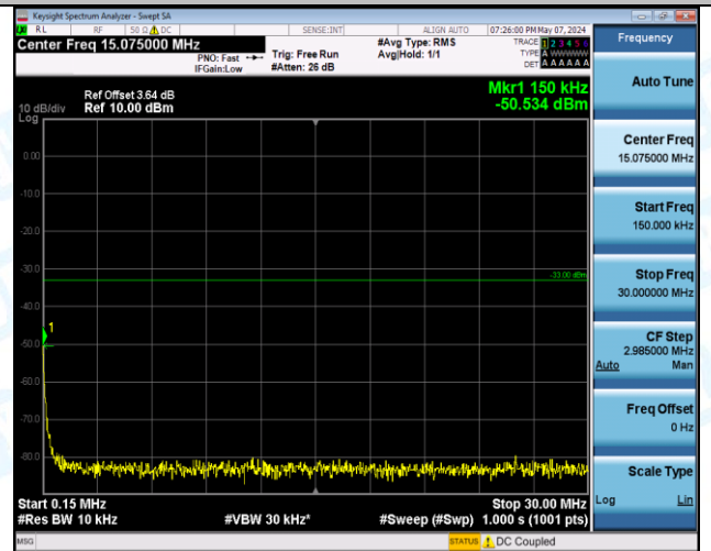
Band4_15MHz_QPSK_20175_75RB#0_1000~3000_1000~3000
