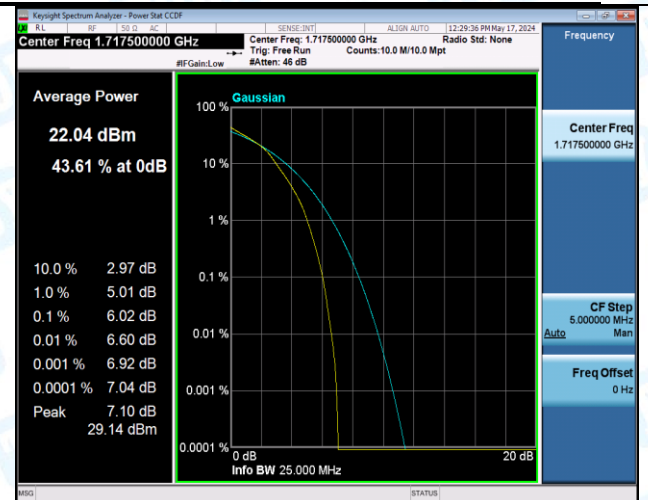
Band4-15MHz-16QAM-20175-27RB#0-PASS
