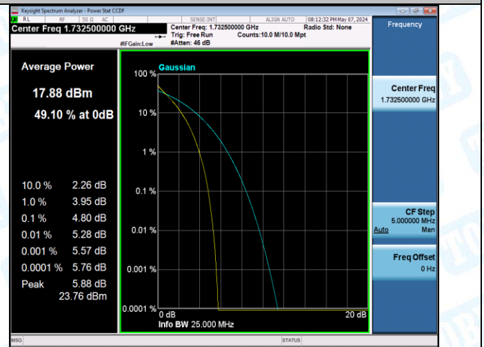
Band4-20MHz-QPSK-20300-100RB#0-PASS
