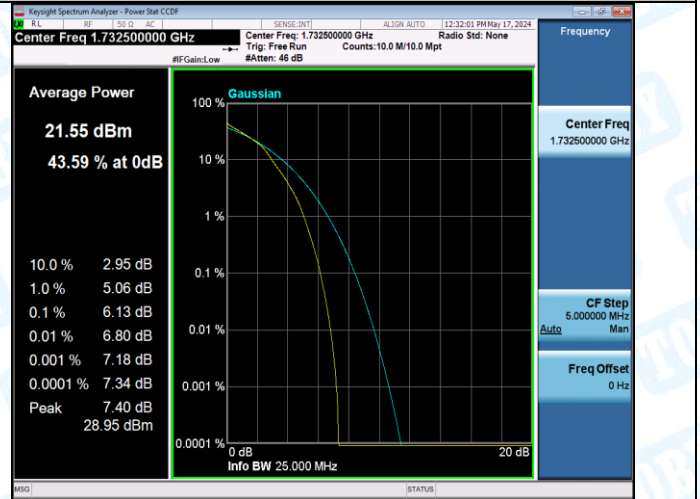
Band4-20MHz-16QAM-20300-27RB#0-PASS
