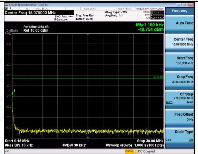
Band4_3MHz_16QAM_20175_1RB#0_1000~3000_1000~3000
