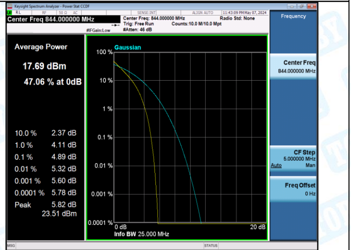
Band5-10MHz-16QAM-20450-27RB#0-PASS
