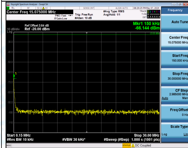
Band5_1.4MHz_QPSK_20525_1RB#0_1000~3000_1000~3000
