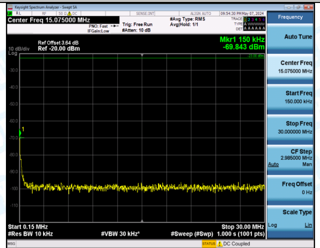
Band5_5MHz_QPSK_20425_25RB#0_1000~3000_1000~3000
