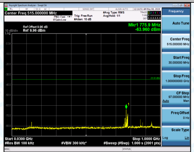
Band7_5MHz_16QAM_20775_25RB#0_20000~27000_20000~27000
