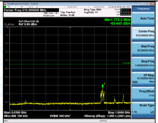
Band7_5MHz_QPSK_21425_1RB#24_20000-27000_20000-27000
