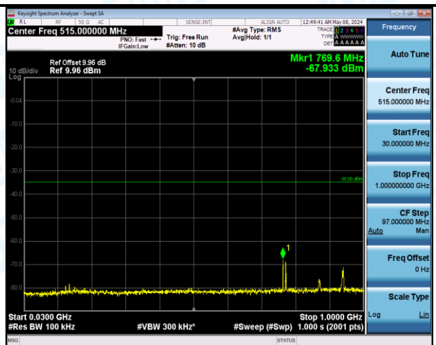
Band7_10MHz_QPSK_20800_1RB#49_20000~27000_20000~27000
