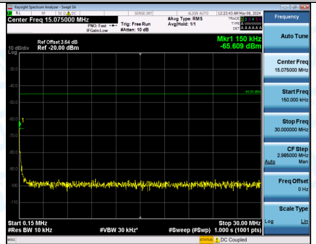
Band7_5MHz_16QAM_21100_25RB#0_1000~20000_1000~20000
