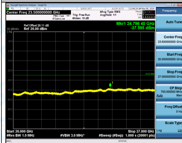
Band7_10MHz_QPSK_20800_1RB#49_0.15~30_0.15~30
