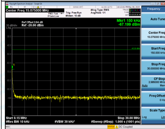
Band7_15MHz_QPSK_20825_1RB#0_1000~20000_1000~20000
