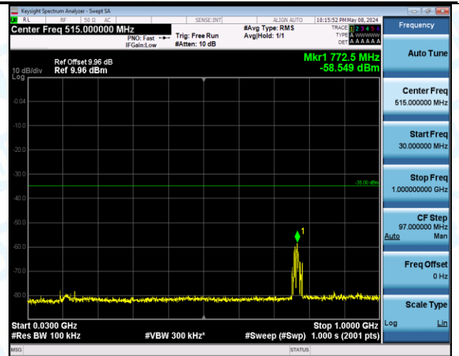
Band7_15MHz_16QAM_20825_1RB#74_20000~27000_20000~27000
