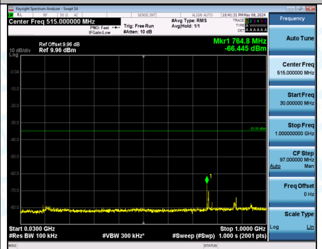
Band7_20MHz_QPSK_21100_1RB#0_20000~27000_20000~27000
