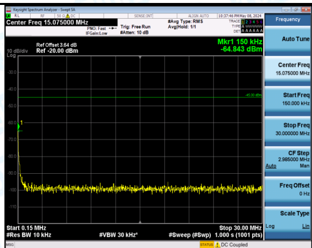
Band7_20MHz_QPSK_20850_1RB#0_1000~20000_1000~20000
