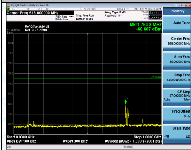
Band7_15MHz_16QAM_20825_1RB#0_20000~27000_20000~27000
