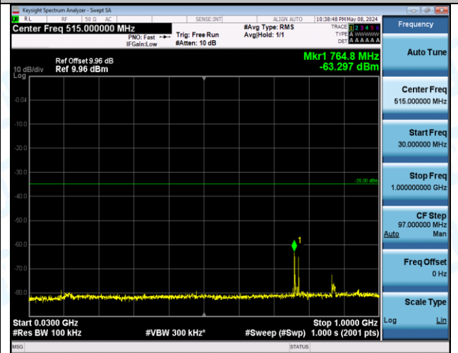
Band7_20MHz_16QAM_20850_1RB#0_20000~27000_20000~27000
