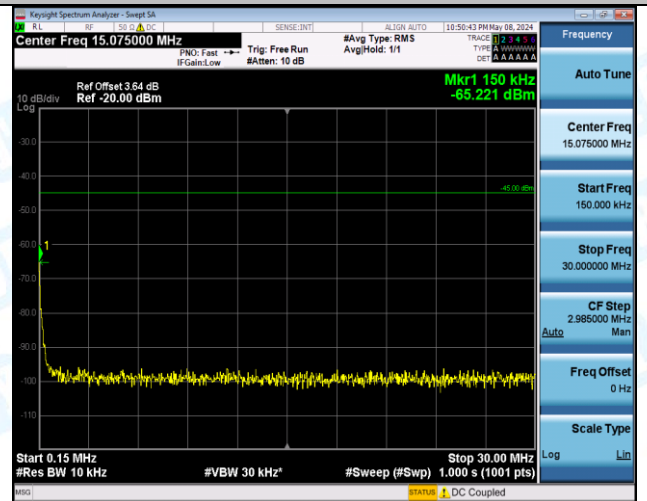
Band7_20MHz_QPSK_21350_100RB#0_1000~20000_1000~20000
