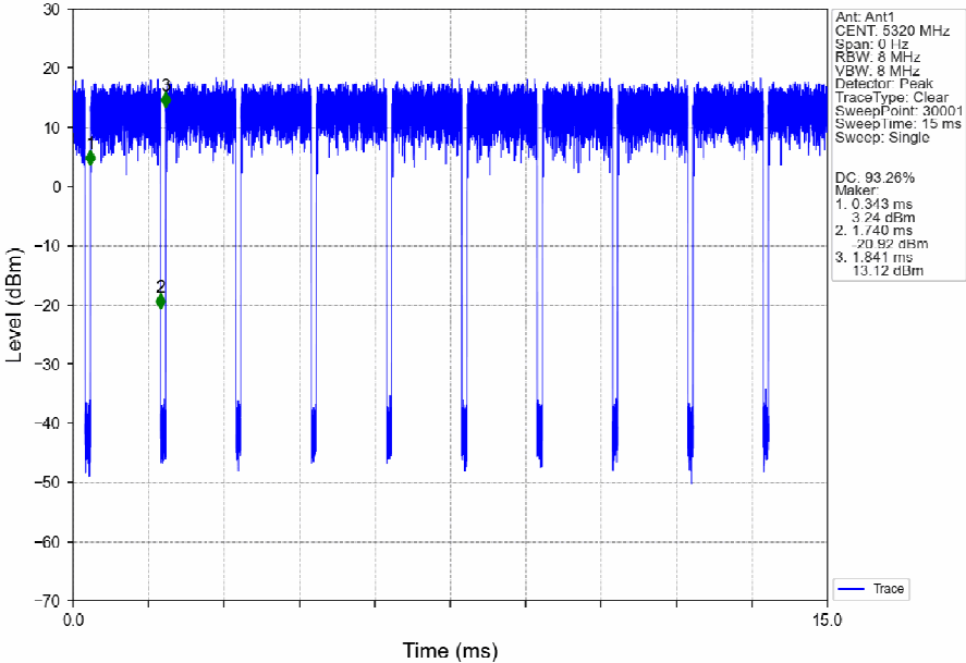
802.11a_HCH_5320MHz_Ant1_NTNV
