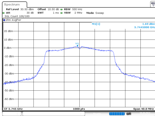
802.11n20_5745MHz
