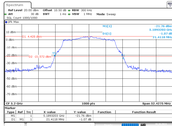
802.11a_5200MHz
