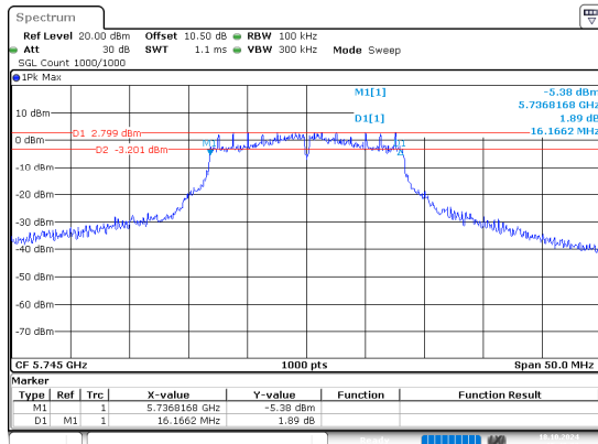
802.11a_5745MHz
