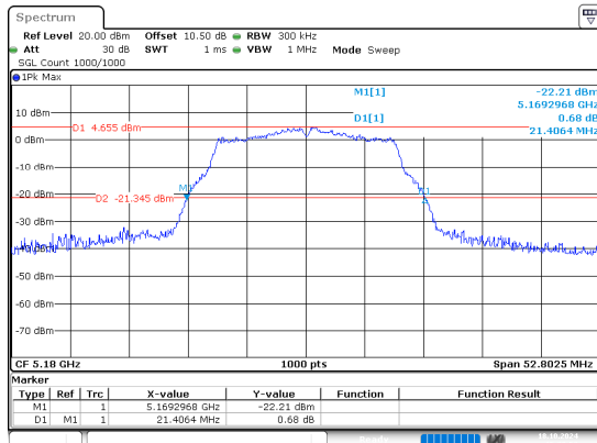
802.11a_5180MHz
