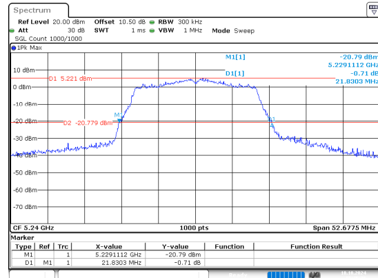
802.11n20_5240MHz
