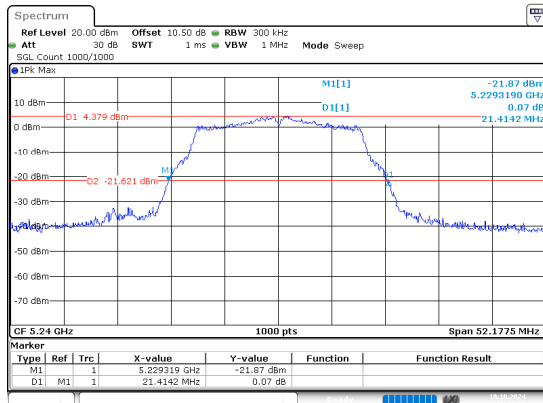
802.11a_5240MHz
