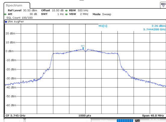
802.11a_5745MHz
