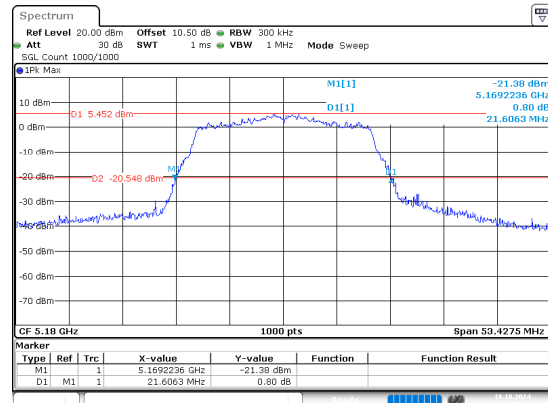
802.11n20_5180MHz
