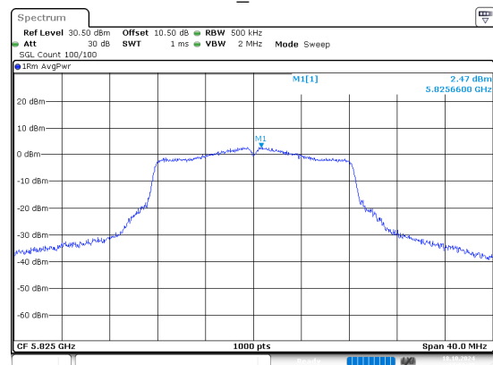
802.11a_5825MHz
