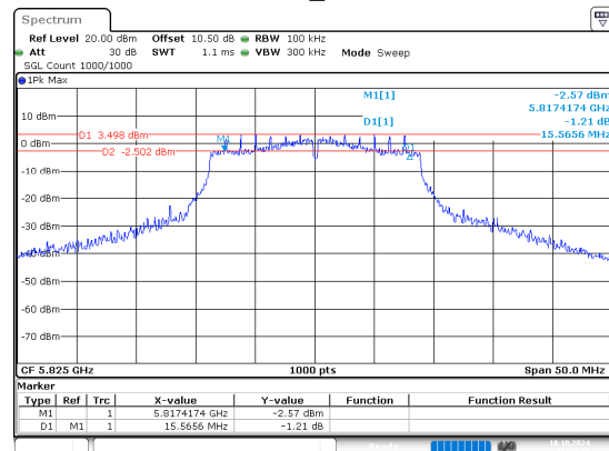
802.11n20_5825MHz
