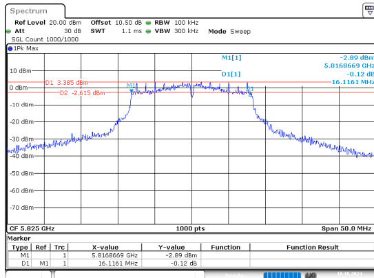
802.11a_5825MHz
