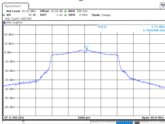
802.11a_5785MHz
