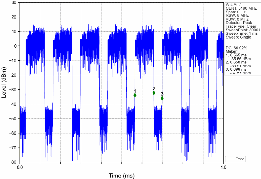
802.11ac(VHT40)_LCH_5190MHz_Ant1_NTNV
