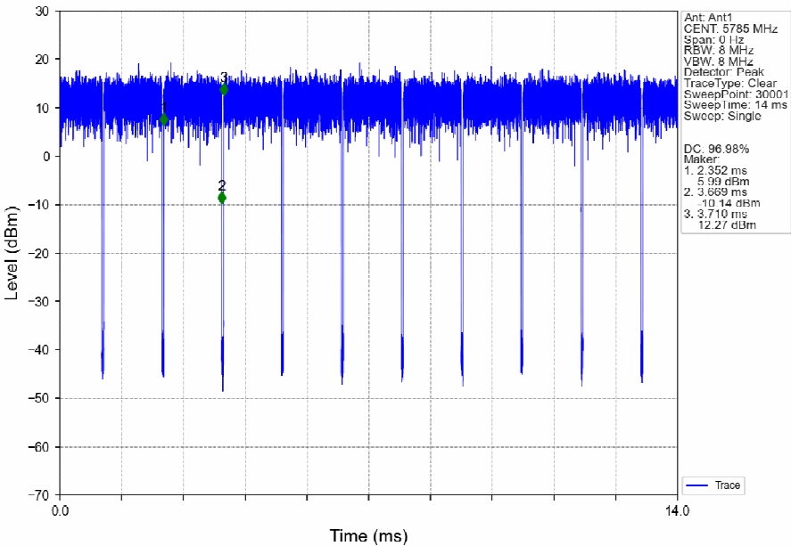
802.11ac(VHT20)_MCH_5785MHz_Ant1_NTNV
