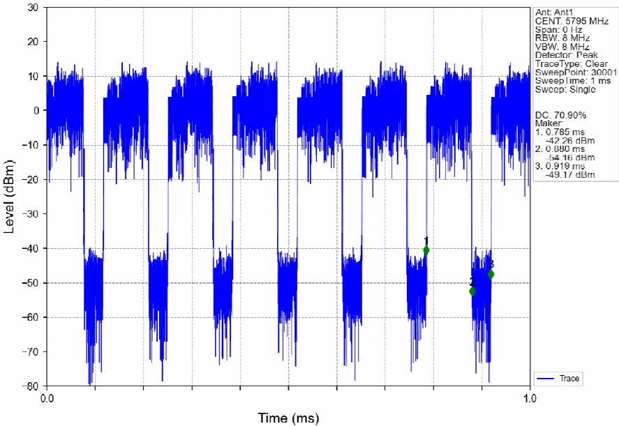
802.11ac(VHT40)_HCH_5795MHz_Ant1_NTNV
