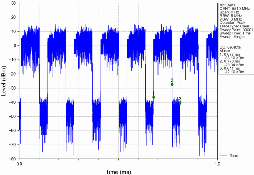
802.11ac(VHT40)_LCH_5510MHz_Ant1_NTNV
