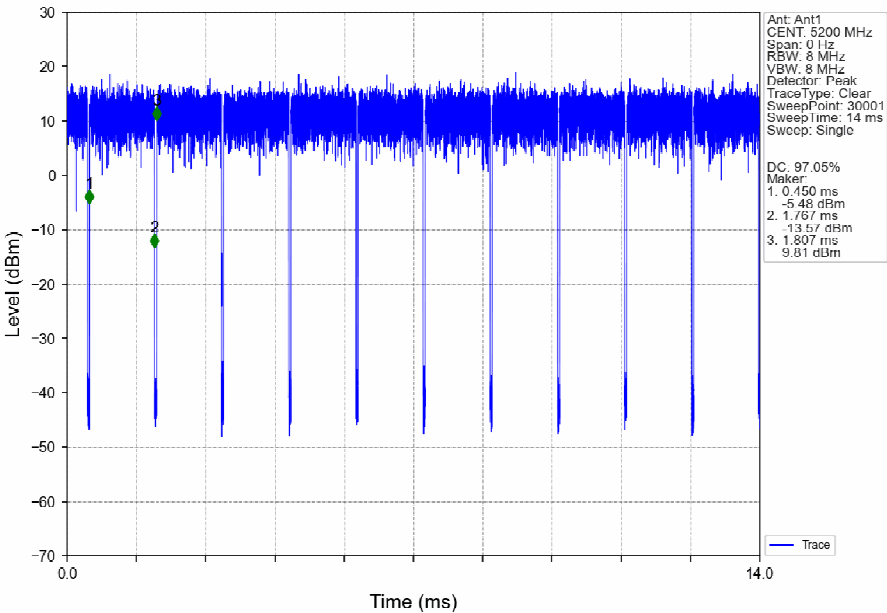
802.11ac(VHT20)_MCH_5200MHz_Ant1_NTNV
