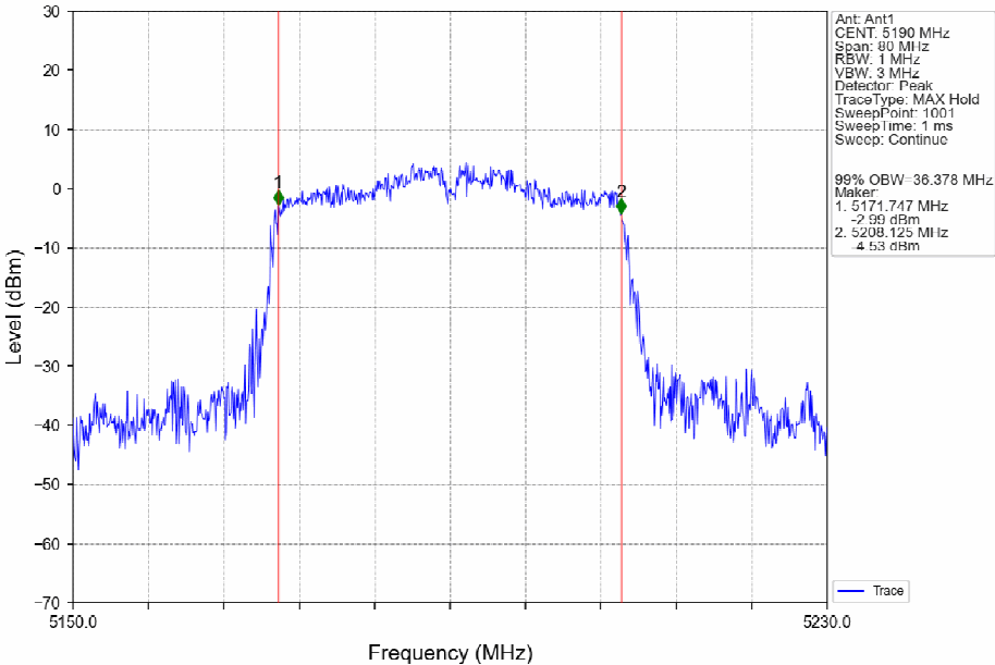
802.11ac(VHT40)_LCH_5190MHz_Ant1_NTNV
