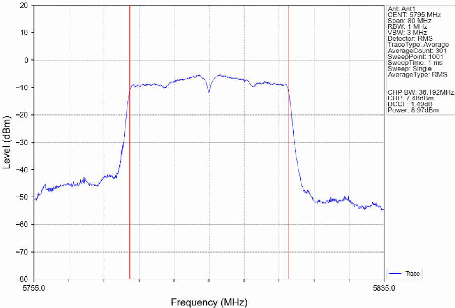
802.11ac(VHT40)_HCH_5795MHz_Ant1_NTNV
