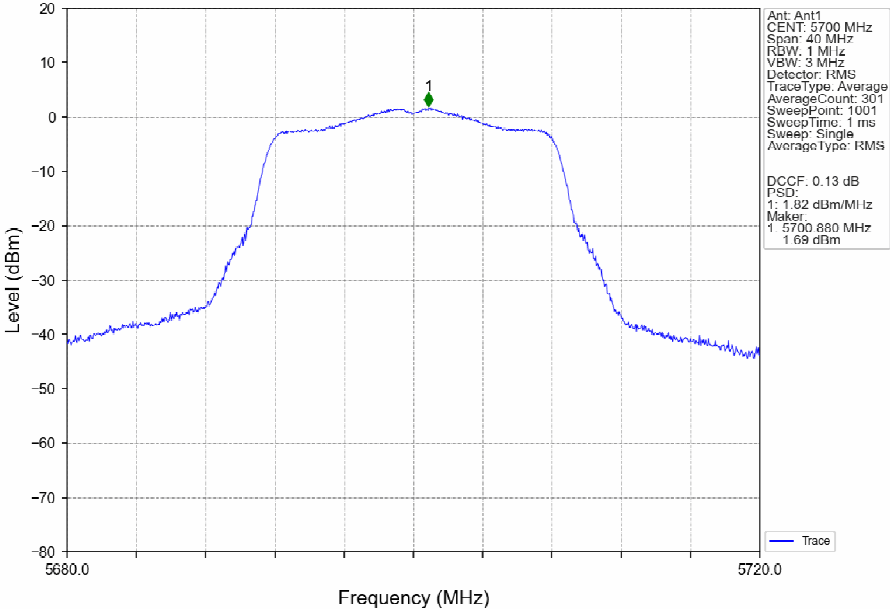
802.11a_HCH_5700MHz_Ant1_NTNV
