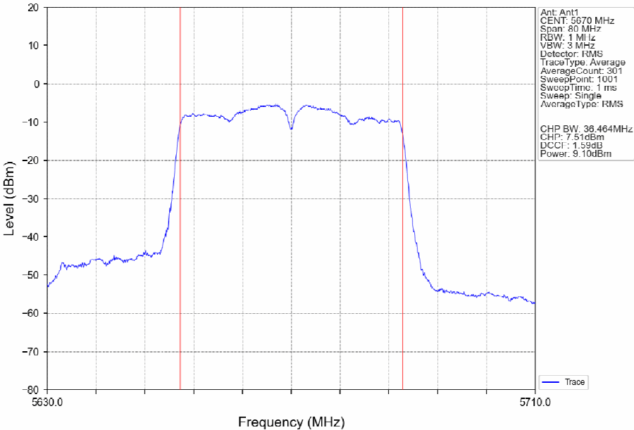
802.11ac(VHT40)_HCH_5670MHz_Ant1_NTNV
