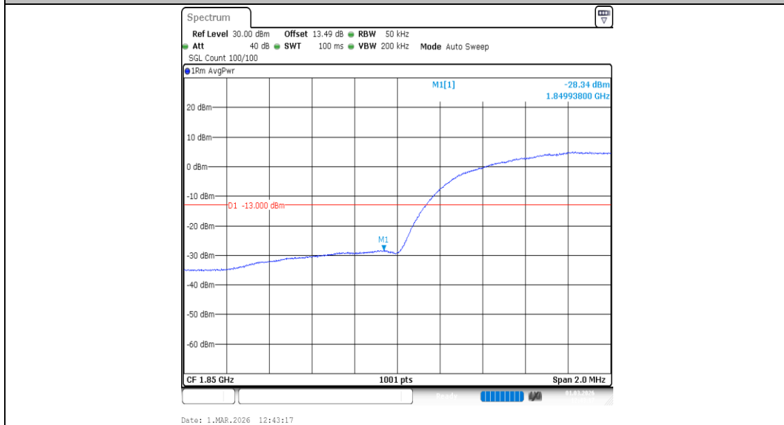
Band2-9262-2-PASS
