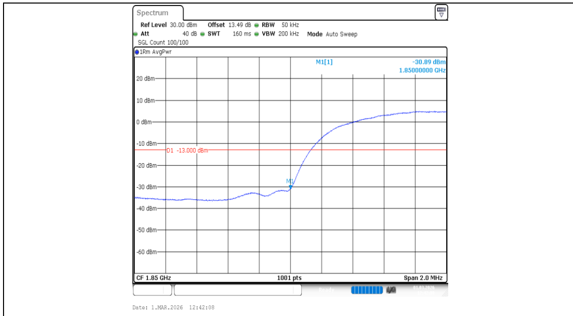
Band2-9262-1-PASS
