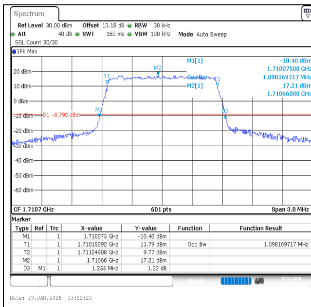
Band4-1.4MHz-QPSK-19957-6RB#0-PASS
