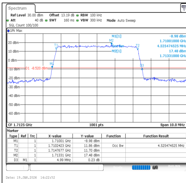
Band4-5MHz-QPSK-19975-25RB#0-PASS
