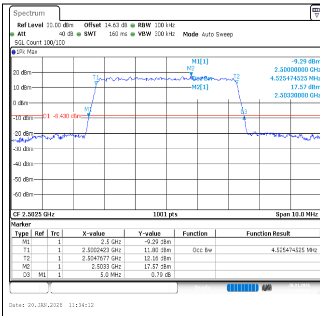
Band7-5MHz-QPSK-20775-25RB#0-PASS
