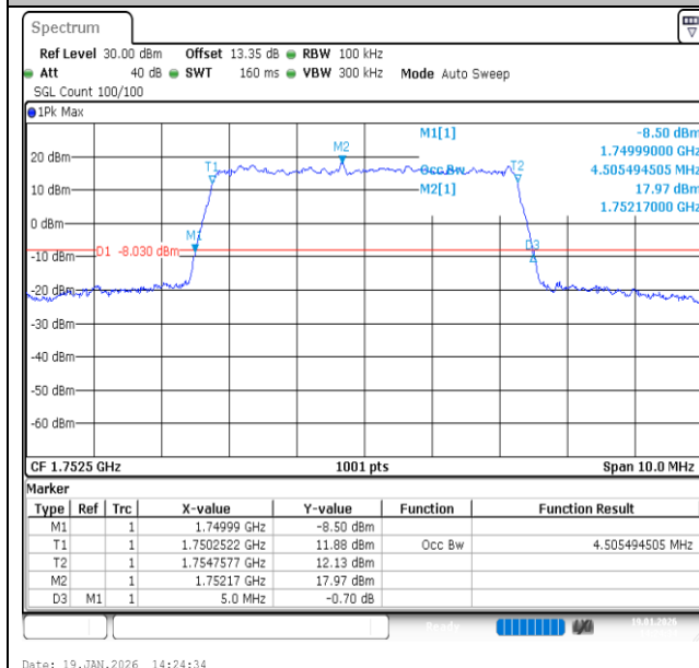
Band4-5MHz-QPSK-20375-25RB#0-PASS
