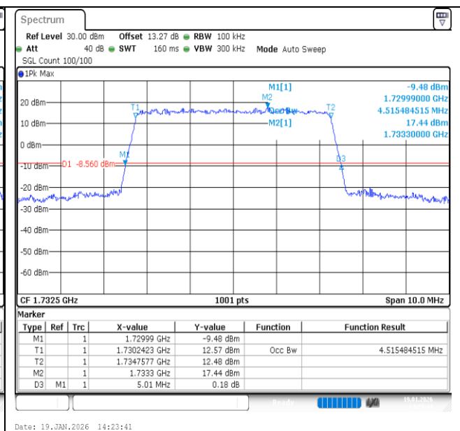
Band4-5MHz-QPSK-20175-25RB#0-PASS
