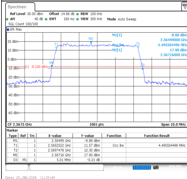
Band7-5MHz-QPSK-21425-25RB#0-PASS
