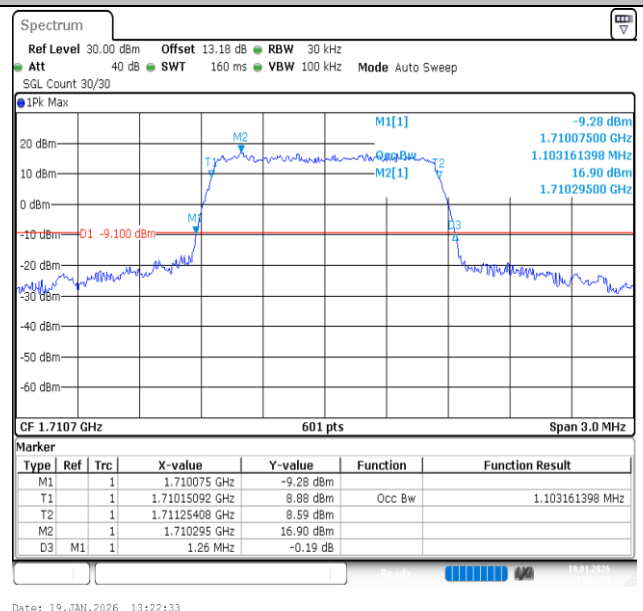
Band4-1.4MHz-16QAM-19957-6RB#0-PASS
