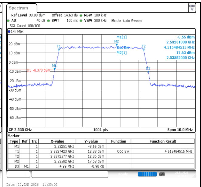
Band7-5MHz-QPSK-21100-25RB#0-PASS
