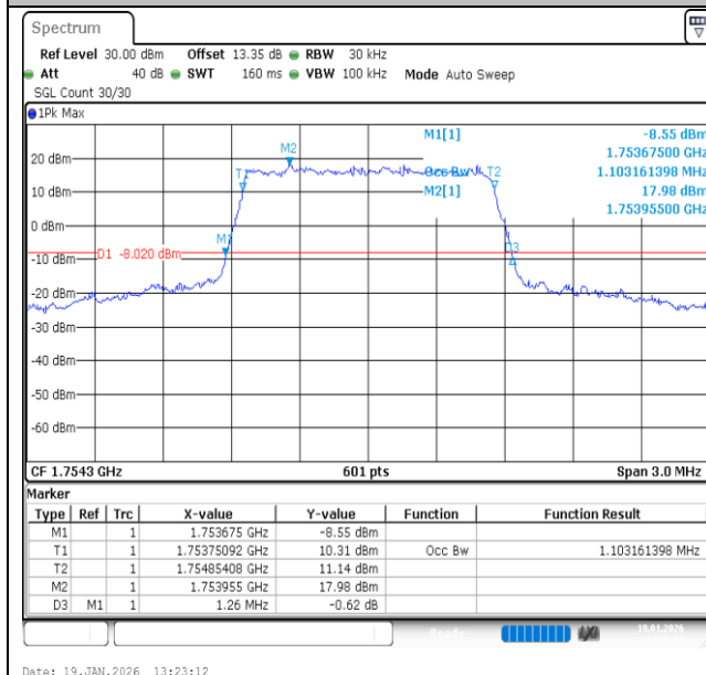
Band4-1.4MHz-QPSK-20393-6RB#0-PASS
