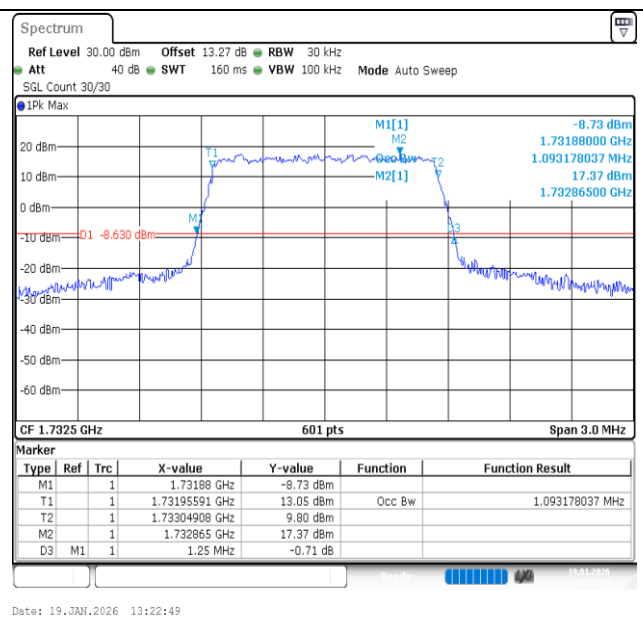
Band4-1.4MHz-QPSK-20175-6RB#0-PASS
