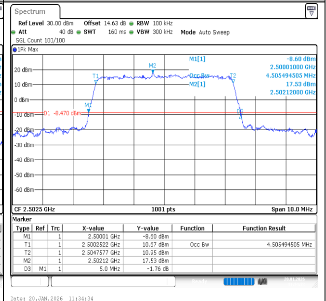
Band7-5MHz-16QAM-20775-25RB#0-PASS
