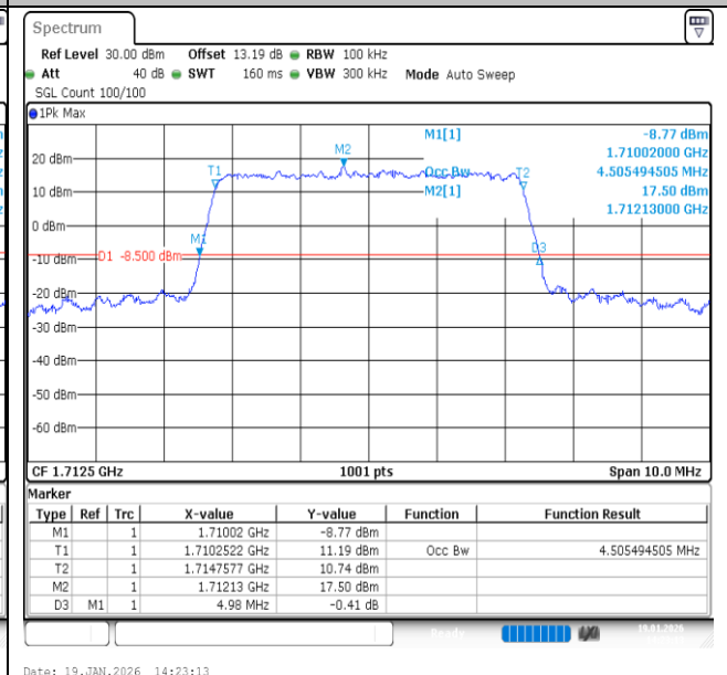
Band4-5MHz-16QAM-19975-25RB#0-PASS
