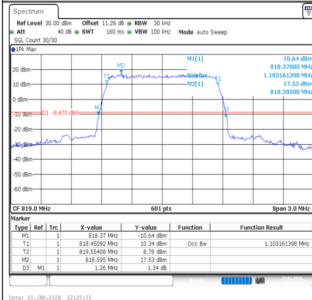
Band26(814-824)-1.4MHz-16QAM-26740-6RB#0-PASS
