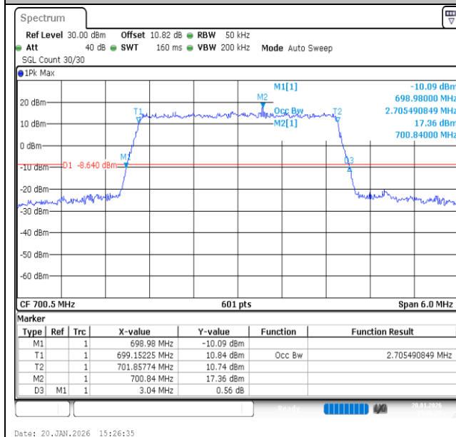
Band12-3MHz-QPSK-23025-15RB#0-PASS
