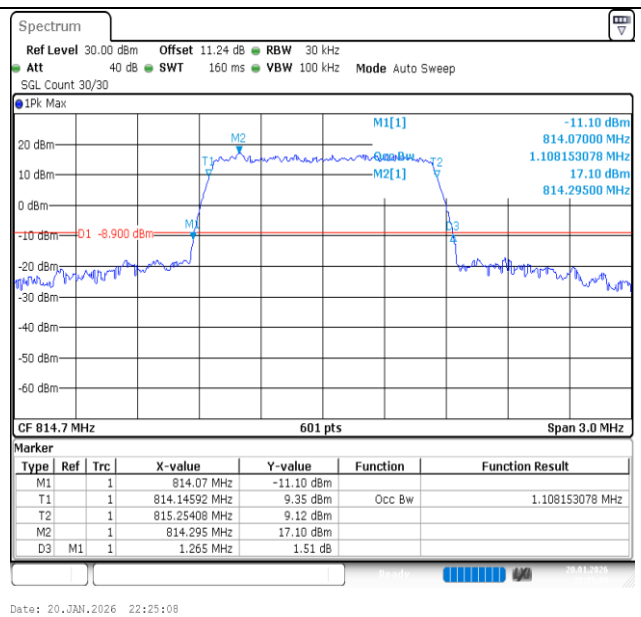
Band26(814-824)-1.4MHz-16QAM-26697-6RB#0-PASS
