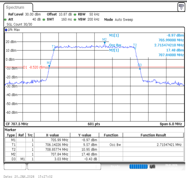
Band12-3MHz-QPSK-23095-15RB#0-PASS
