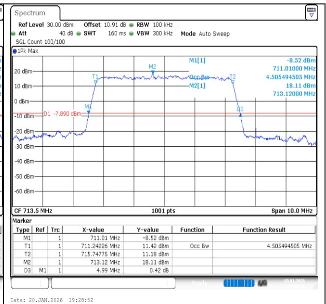
Band17-5MHz-16QAM-23825-25RB#0-PASS
