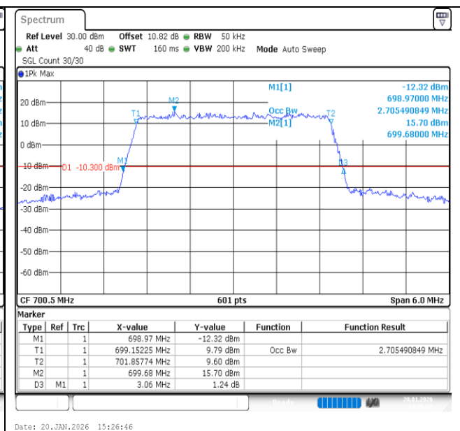
Band12-3MHz-16QAM-23025-15RB#0-PASS
