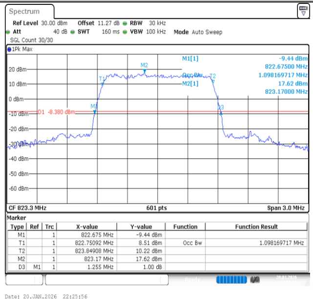
Band26(814-824)-1.4MHz-16QAM-26783-6RB#0-PASS
