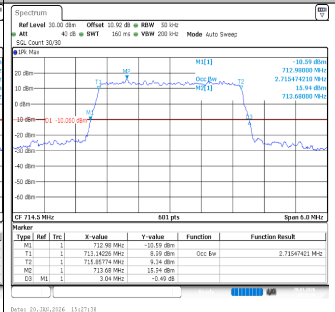
Band12-3MHz-16QAM-23165-15RB#0-PASS
