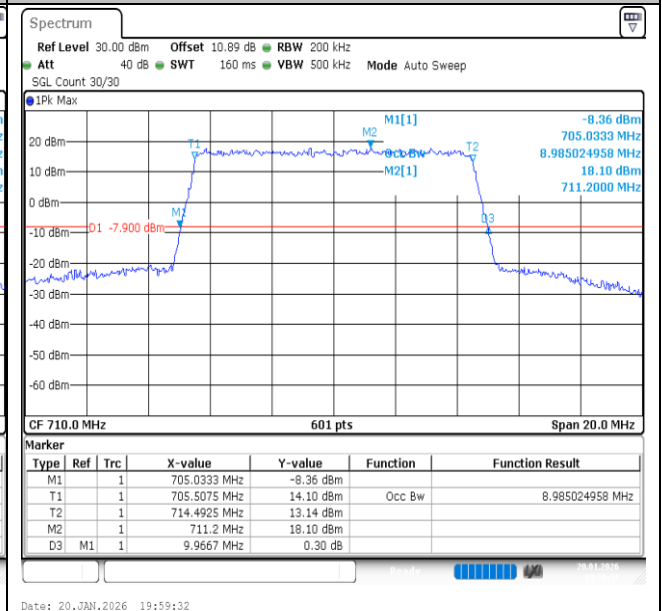
Band17-10MHz-QPSK-23790-50RB#0-PASS
