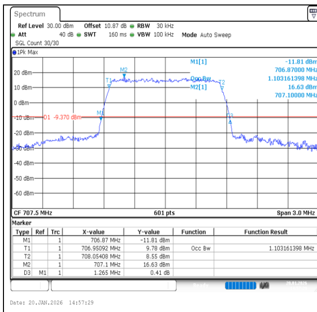
Band12-1.4MHz-16QAM-23095-6RB#0-PASS
