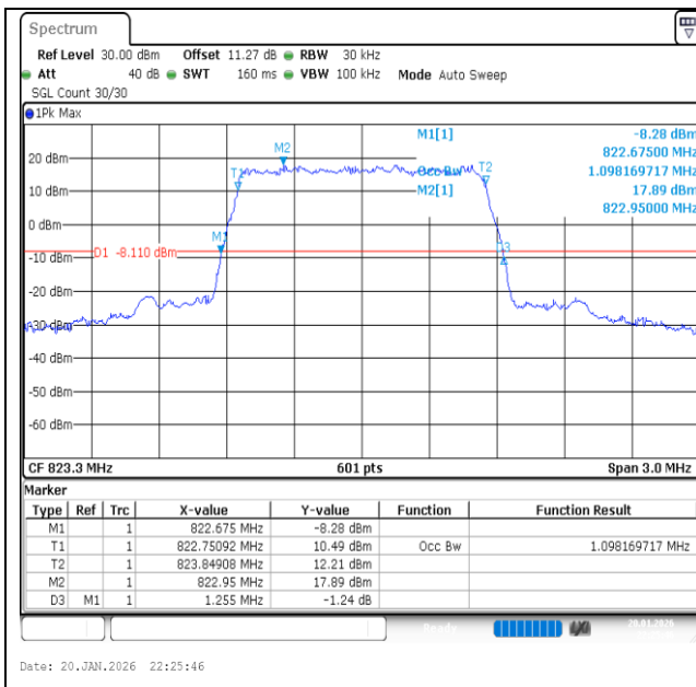
Band26(814-824)-1.4MHz-QPSK-26783-6RB#0-PASS
