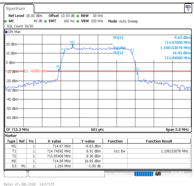
Band12-1.4MHz-16QAM-23173-6RB#0-PASS
