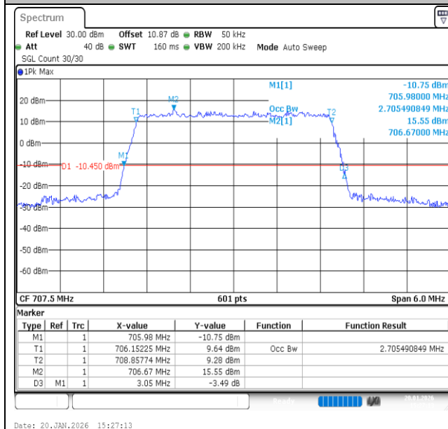
Band12-3MHz-16QAM-23095-15RB#0-PASS
