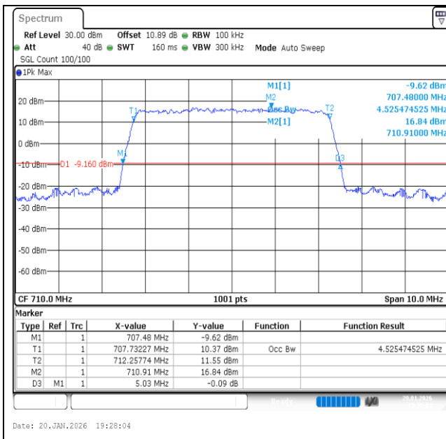
Band17-5MHz-16QAM-23790-25RB#0-PASS
