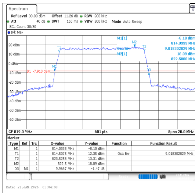
Band26(814-824)-10MHz-QPSK-26740-50RB#0-PASS
