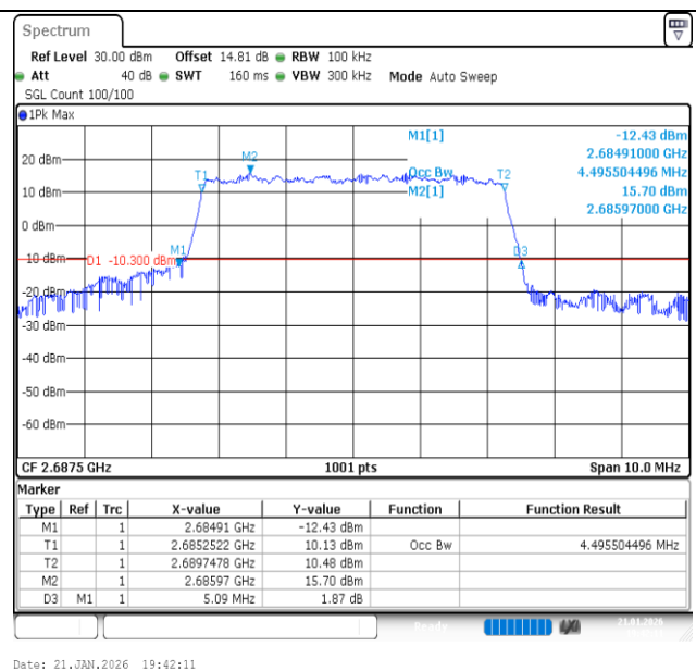
Band41-5MHz-16QAM-41565-25RB#0-PASS
