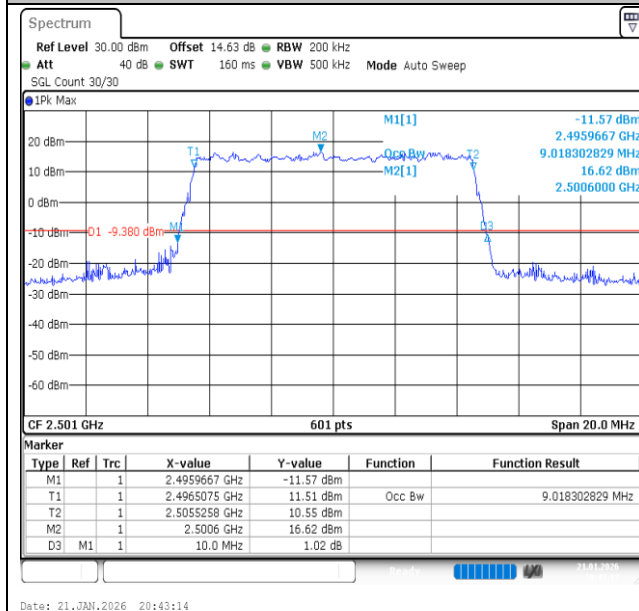
Band41-10MHz-QPSK-39700-50RB#0-PASS
