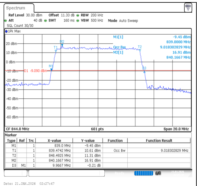
Band26(824-849)-10MHz-16QAM-26990-50RB#0-PASS
