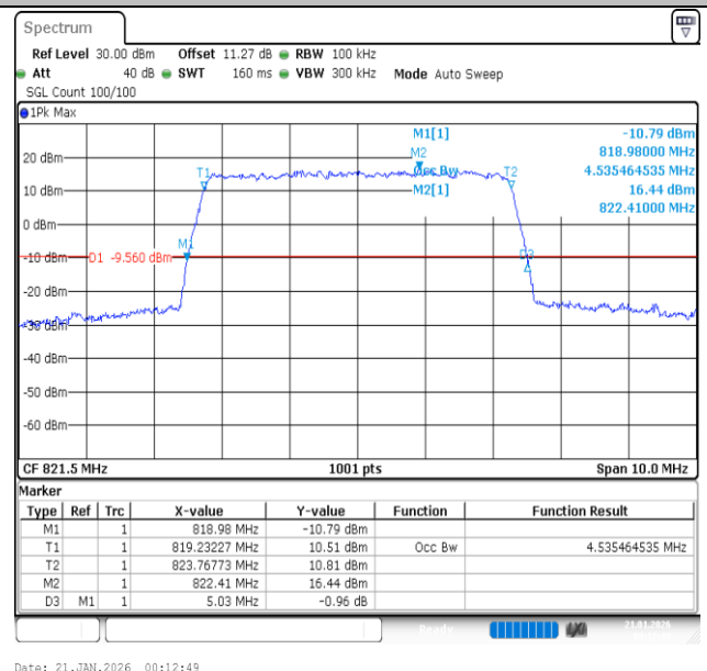
Band26(814-824)-5MHz-16QAM-26765-25RB#0-PASS
