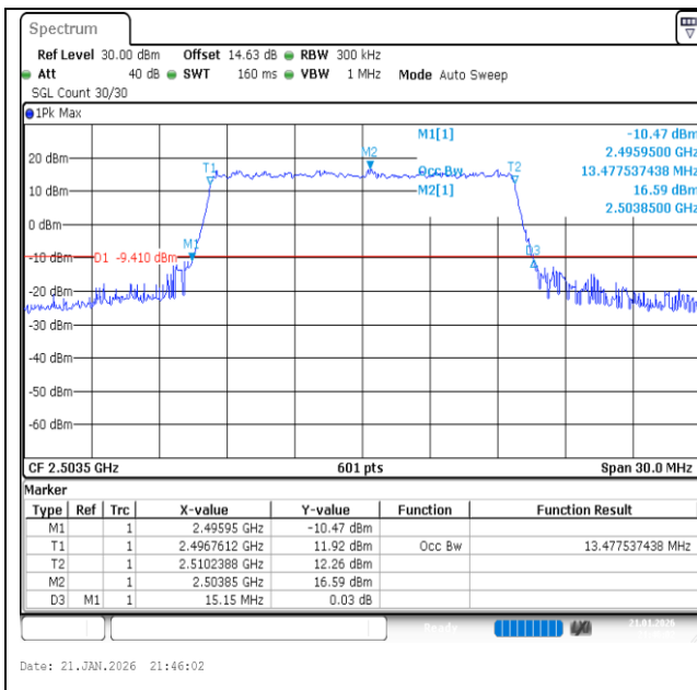
Band41-15MHz-QPSK-39725-75RB#0-PASS
