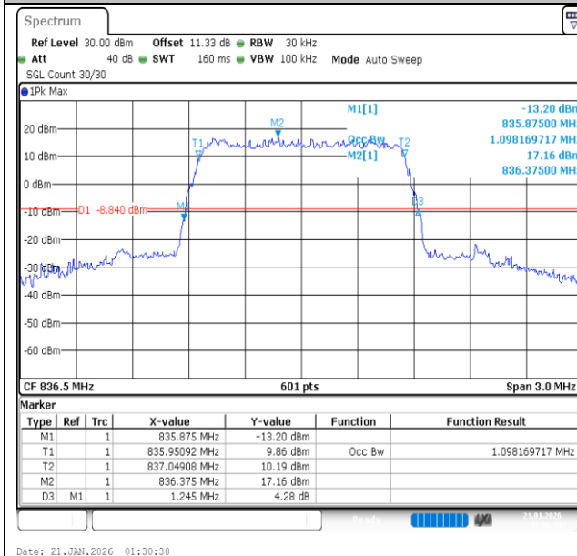
Band26(824-849)-1.4MHz-16QAM-26915-6RB#0-PASS
