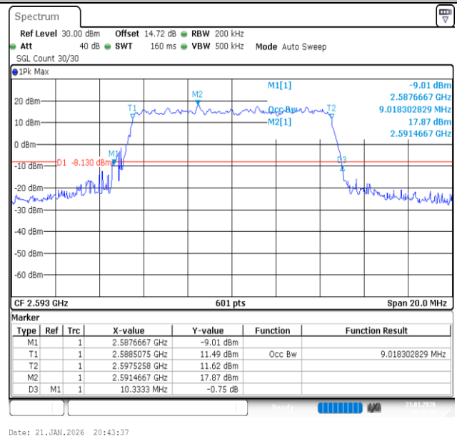
Band41-10MHz-QPSK-40620-50RB#0-PASS
