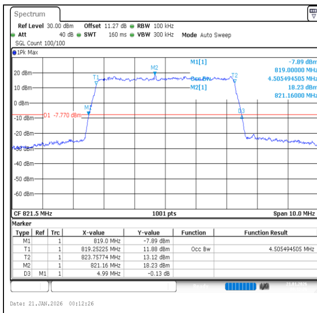
Band26(814-824)-5MHz-QPSK-26765-25RB#0-PASS
