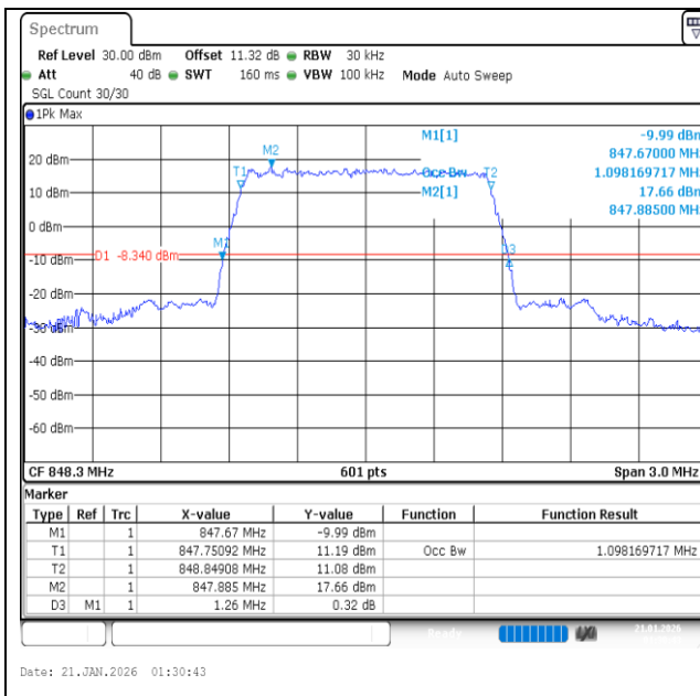
Band26(824-849)-1.4MHz-QPSK-27033-6RB#0-PASS
