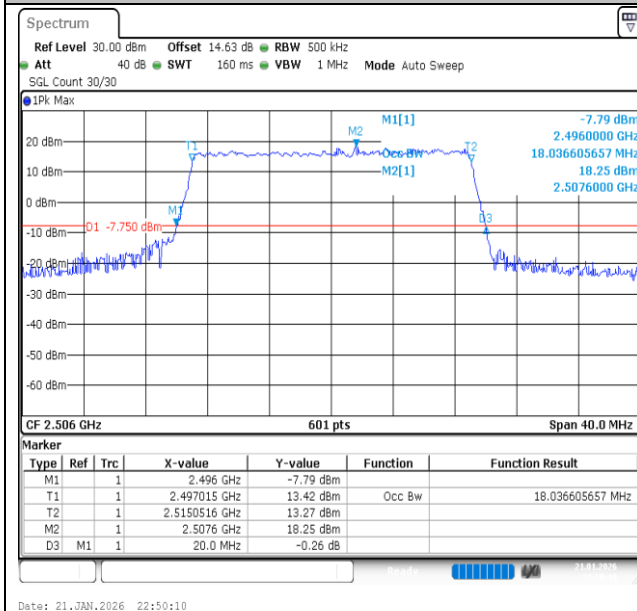
Band41-20MHz-QPSK-39750-100RB#0-PASS
