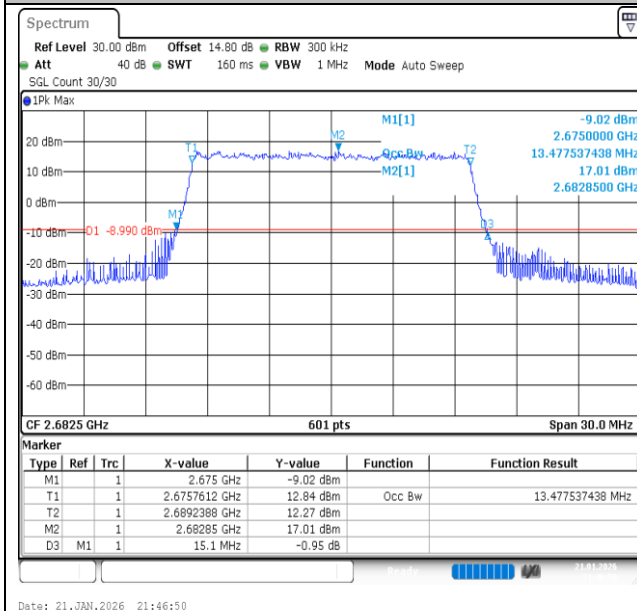
Band41-15MHz-QPSK-41515-75RB#0-PASS
