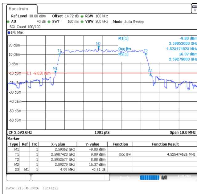
Band41-5MHz-16QAM-40620-25RB#0-PASS
