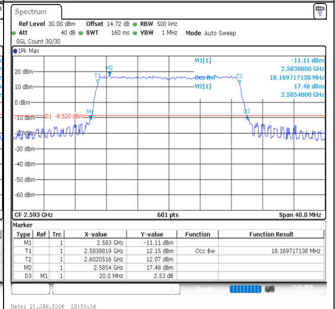
Band41-20MHz-QPSK-40620-100RB#0-PASS
