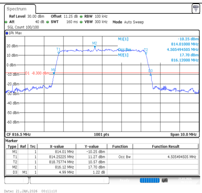
Band26(814-824)-5MHz-16QAM-26715-25RB#0-PASS
