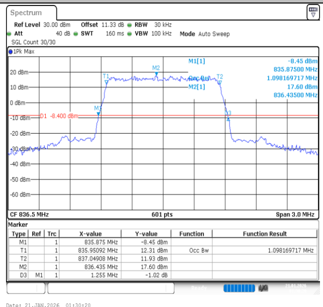
Band26(824-849)-1.4MHz-QPSK-26915-6RB#0-PASS
