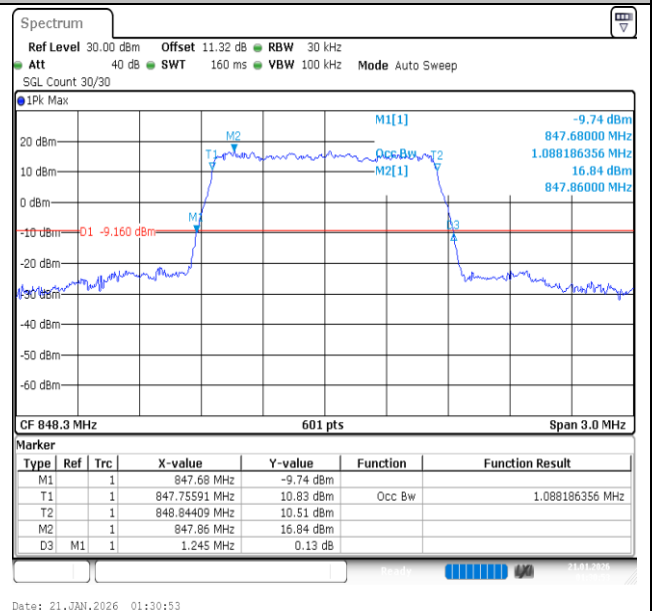
Band26(824-849)-1.4MHz-16QAM-27033-6RB#0-PASS
