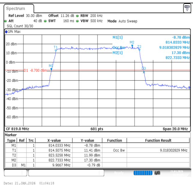
Band26(814-824)-10MHz-16QAM-26740-50RB#0-PASS
