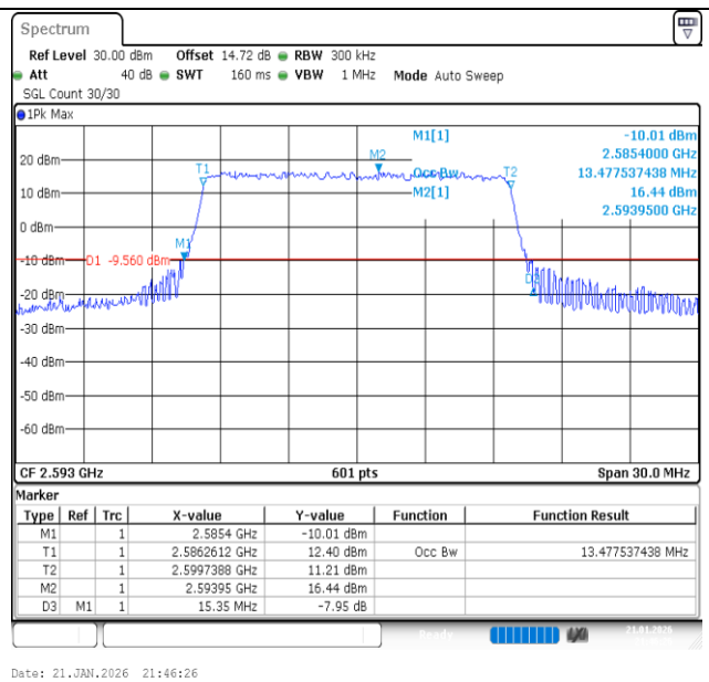
Band41-15MHz-QPSK-40620-75RB#0-PASS
