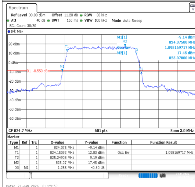
Band26(824-849)-1.4MHz-QPSK-26797-6RB#0-PASS
