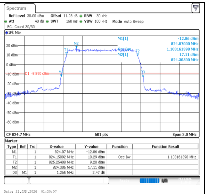
Band26(824-849)-1.4MHz-16QAM-26797-6RB#0-PASS
