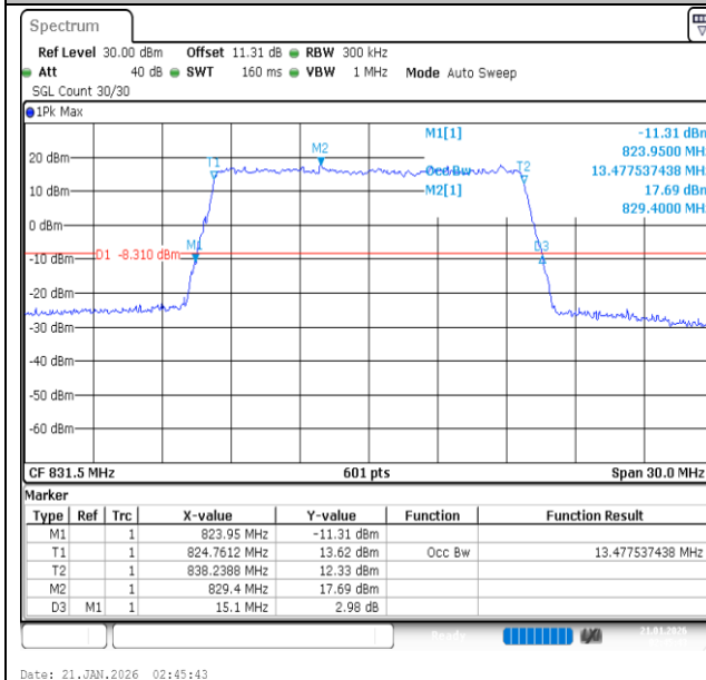
Band26(824-849)-15MHz-QPSK-26865-75RB#0-PASS
