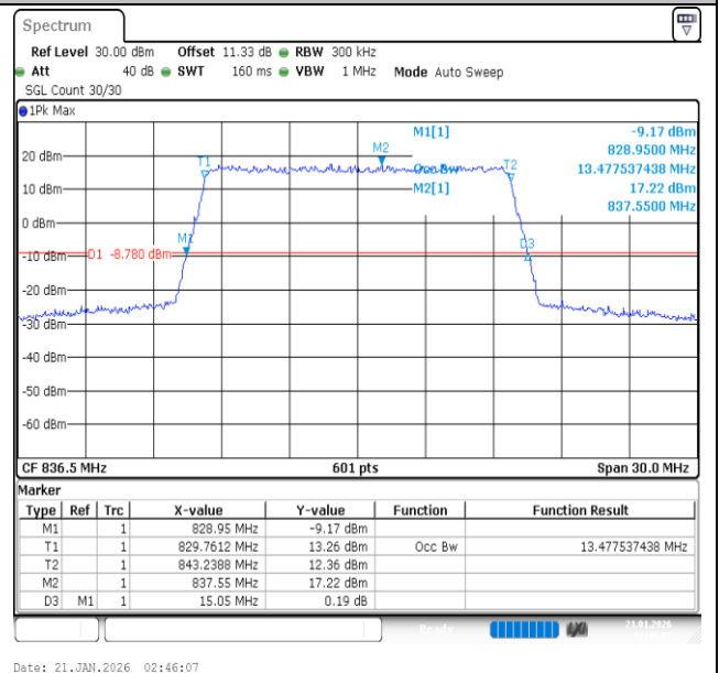
Band26(824-849)-15MHz-QPSK-26915-75RB#0-PASS
