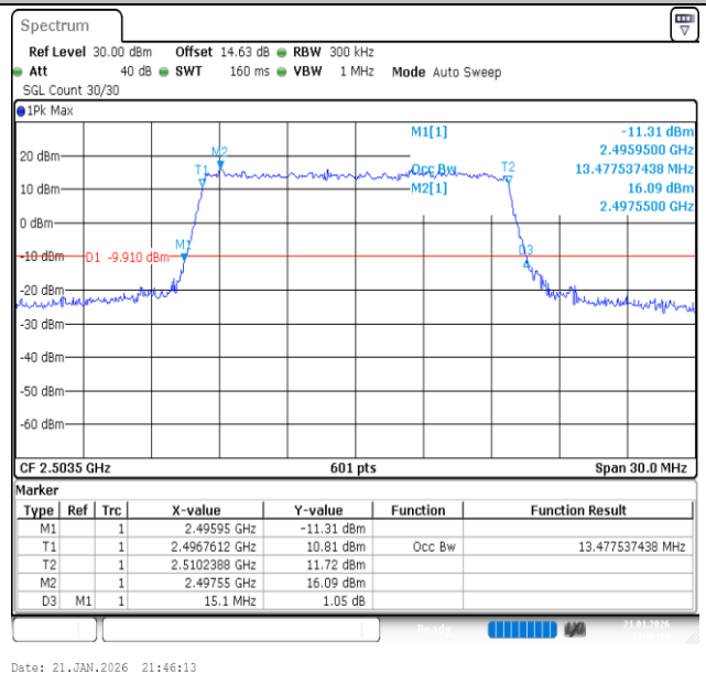
Band41-15MHz-16QAM-39725-75RB#0-PASS
