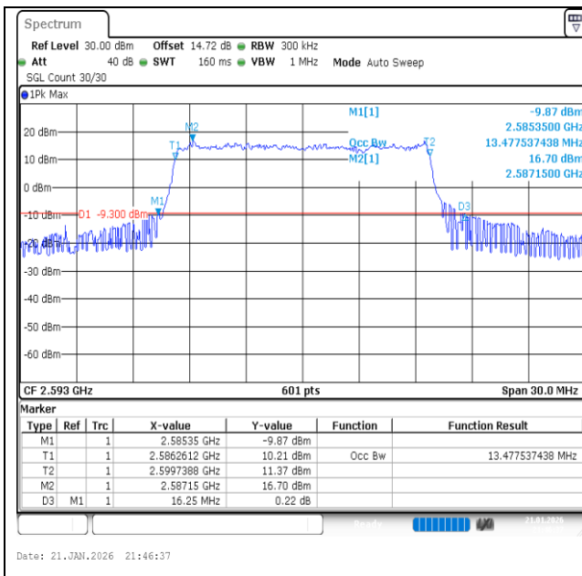
Band41-15MHz-16QAM-40620-75RB#0-PASS
