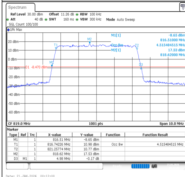
Band26(814-824)-5MHz-16QAM-26740-25RB#0-PASS
