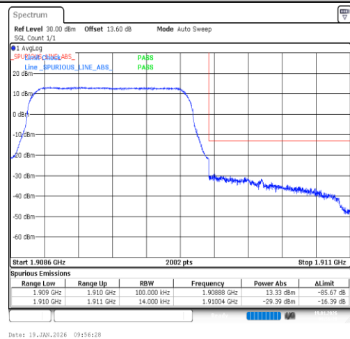
Band2-1.4MHz-QPSK-19193-6RB#0-PASS
