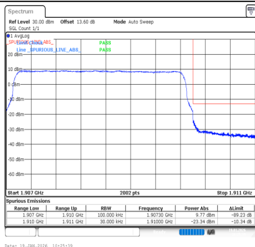
Band2-3MHz-QPSK-19185-15RB#0-PASS
