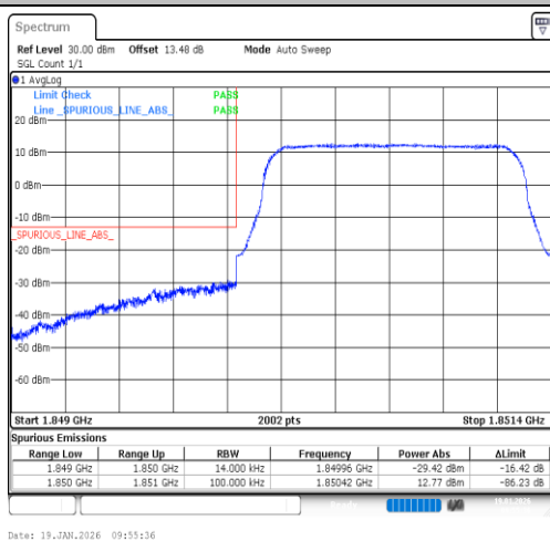
Band2-1.4MHz-16QAM-18607-6RB#0-PASS
