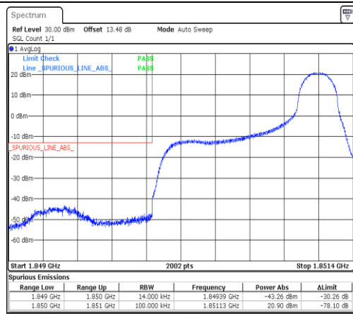
Band2-1.4MHz-16QAM-18607-1RB#5-PASS
