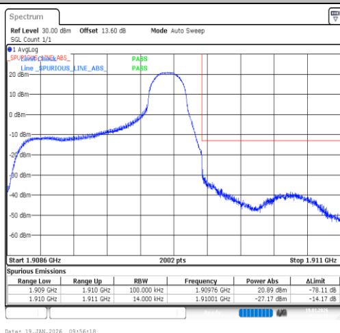
Band2-1.4MHz-16QAM-19193-1RB#5-PASS
