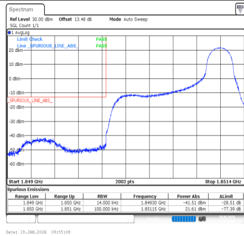
Band2-1.4MHz-QPSK-18607-1RB#5-PASS
