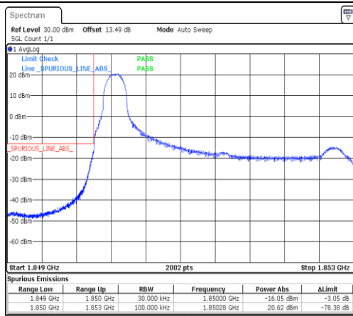
Band2-3MHz-16QAM-18615-1RB#0-PASS
