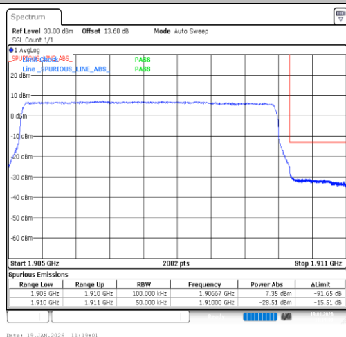
Band2-5MHz-QPSK-19175-25RB#0-PASS
