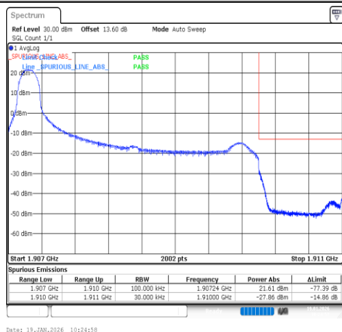
Band2-3MHz-QPSK-19185-1RB#0-PASS
