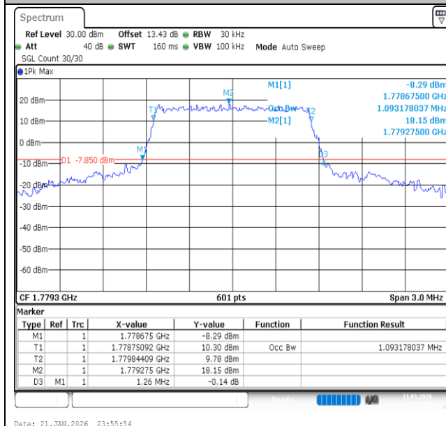
Band66-1.4MHz-QPSK-132665-6RB#0-PASS
