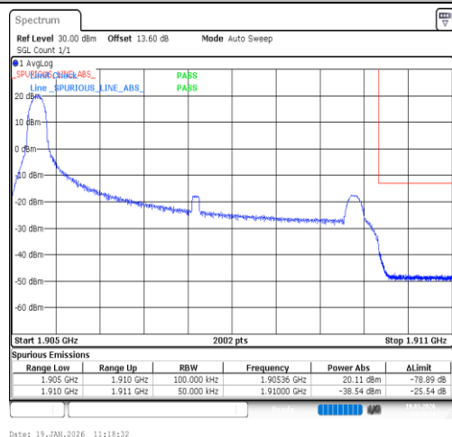
Band2-5MHz-16QAM-19175-1RB#0-PASS
