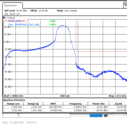
Band2-1.4MHz-QPSK-19193-1RB#5-PASS
