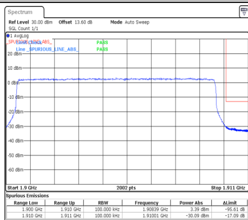
Band2-10MHz-16QAM-19150-1RB#0-PASS
