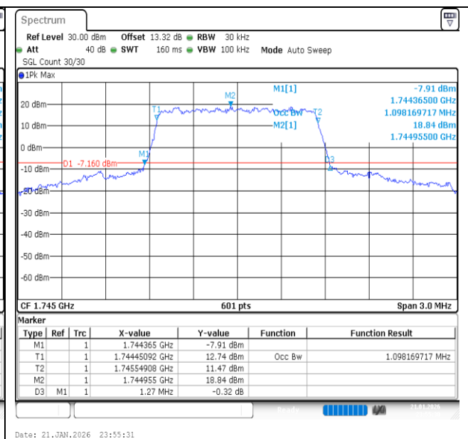
Band66-1.4MHz-QPSK-132322-6RB#0-PASS
