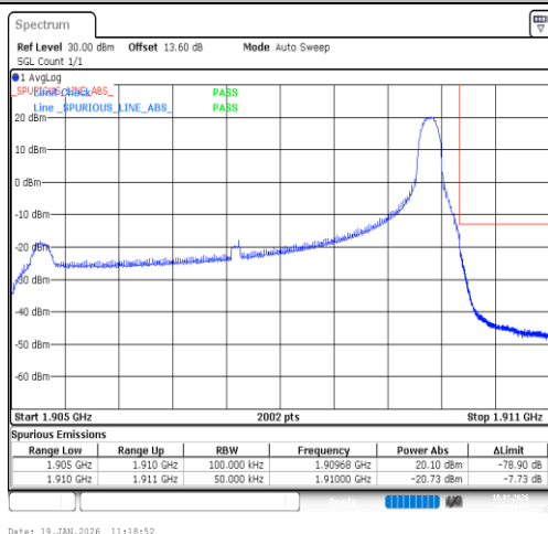
Band2-5MHz-16QAM-19175-1RB#24-PASS
