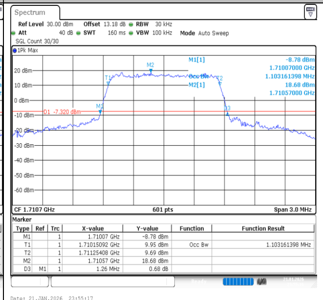
Band66-1.4MHz-16QAM-131979-6RB#0-PASS
