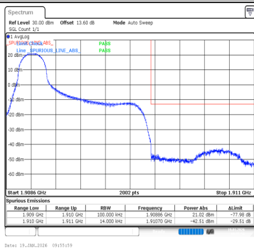
Band2-1.4MHz-16QAM-19193-1RB#0-PASS
