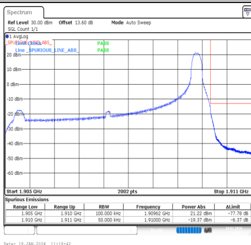
Band2-5MHz-QPSK-19175-1RB#24-PASS
