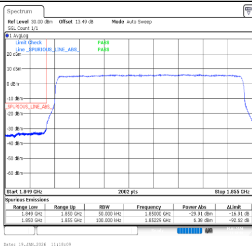
Band2-5MHz-16QAM-18625-25RB#0-PASS
