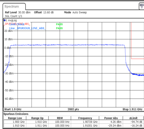
Band2-10MHz-QPSK-19150-1RB#0-PASS
