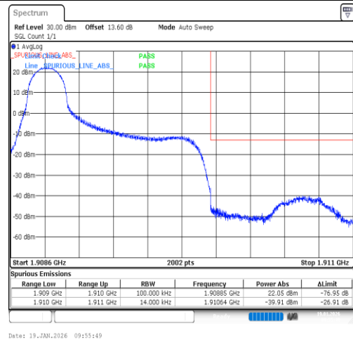
Band2-1.4MHz-QPSK-19193-1RB#0-PASS
