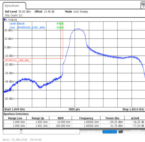
Band2-1.4MHz-QPSK-18607-1RB#0-PASS
