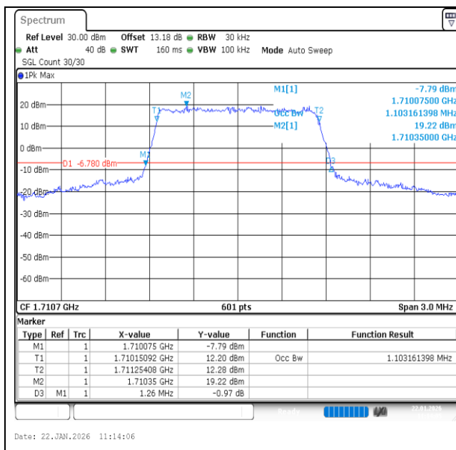
Band66-1.4MHz-QPSK-131979-6RB#0-PASS
