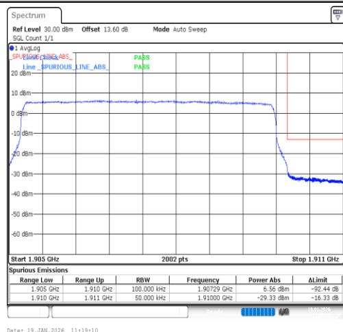
Band2-5MHz-16QAM-19175-25RB#0-PASS
