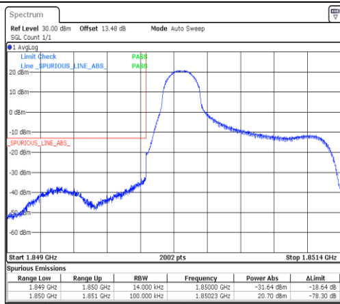
Band2-1.4MHz-16QAM-18607-1RB#0-PASS
