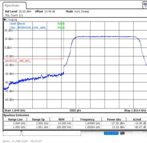
Band2-1.4MHz-QPSK-18607-6RB#0-PASS
