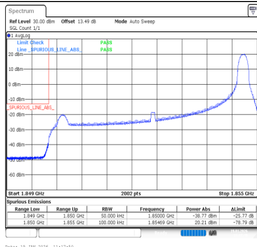
Band2-5MHz-16QAM-18625-1RB#24-PASS
