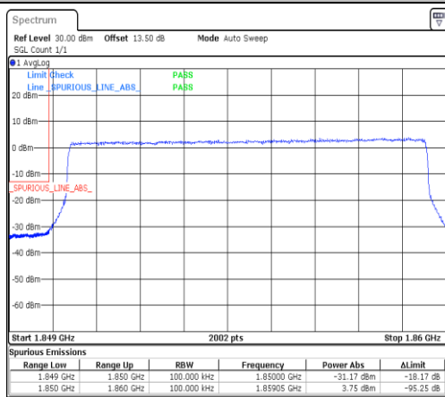
Band2-10MHz-16QAM-18650-1RB#0-PASS
