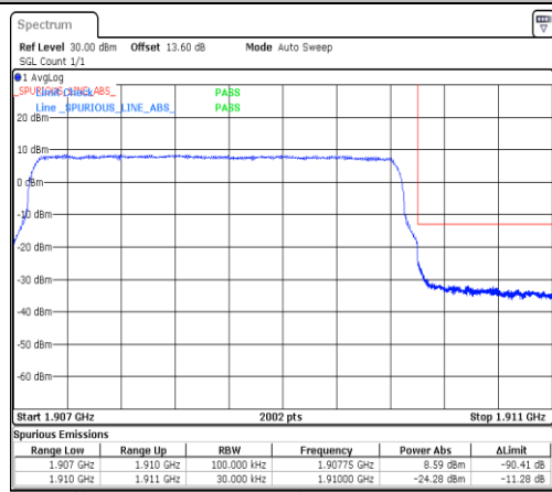
Band2-3MHz-16QAM-19185-1RB#0-PASS
