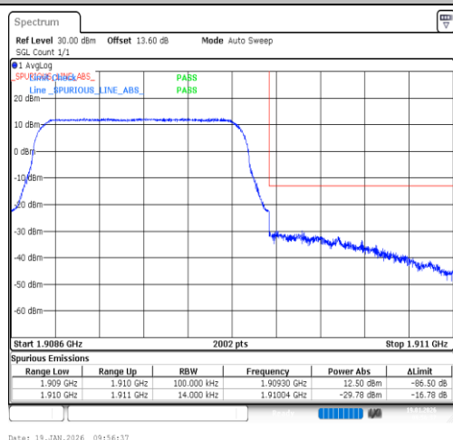
Band2-1.4MHz-16QAM-19193-6RB#0-PASS
