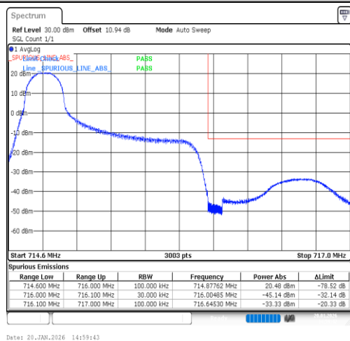
Band12-1.4MHz-16QAM-23173-1RB#0-PASS
