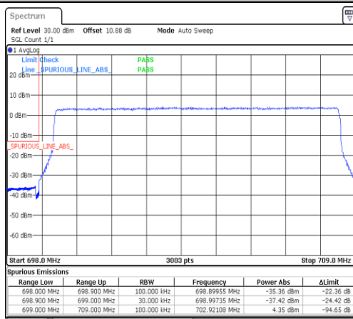
Band12-10MHz-QPSK-23060-1RB#0-PASS
