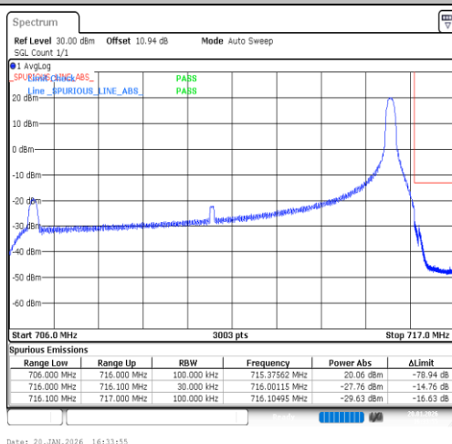
Band12-10MHz-16QAM-23130-1RB#49-PASS
