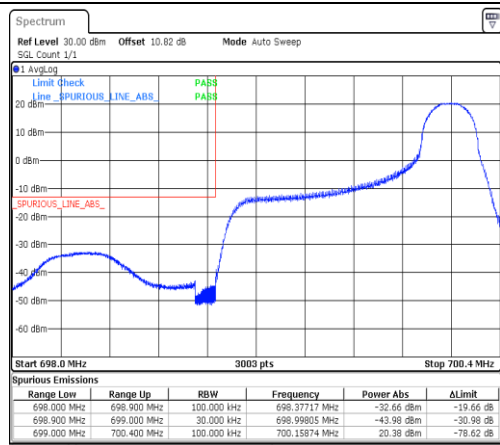
Band12-1.4MHz-16QAM-23017-1RB#5-PASS
