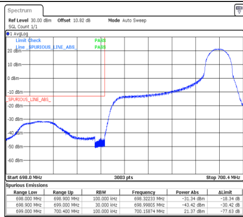
Band12-1.4MHz-QPSK-23017-1RB#5-PASS
