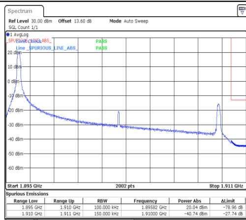
Band2-15MHz-16QAM-18675-1RB#74-PASS
