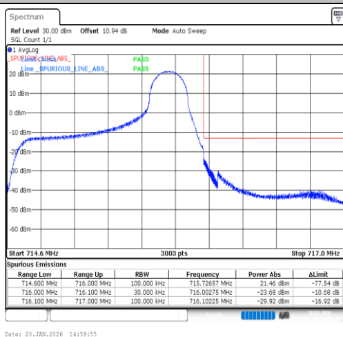
Band12-1.4MHz-QPSK-23173-1RB#5-PASS
