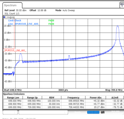
Band12-10MHz-16QAM-23060-1RB#49-PASS
