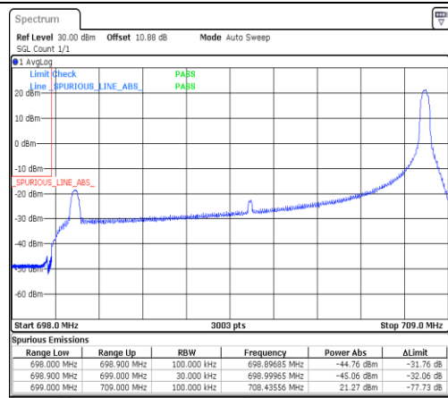
Band12-10MHz-QPSK-23060-1RB#49-PASS
