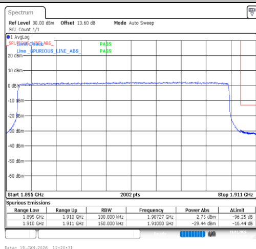
Band2-15MHz-QPSK-19125-75RB#0-PASS
