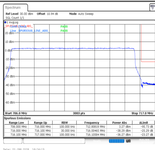
Band12-10MHz-16QAM-23130-50RB#0-PASS
