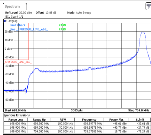
Band12-5MHz-16QAM-23035-1RB#24-PASS
