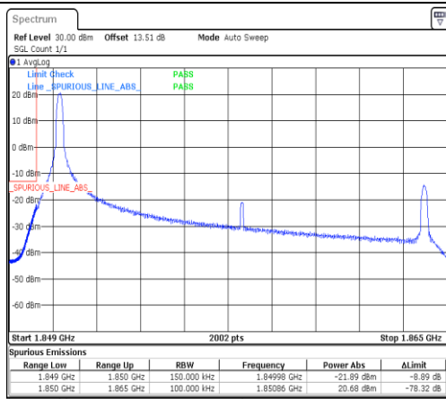
Band2-15MHz-16QAM-18675-1RB#0-PASS
