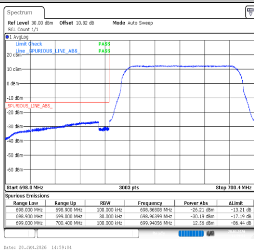
Band12-1.4MHz-QPSK-23017-6RB#0-PASS
