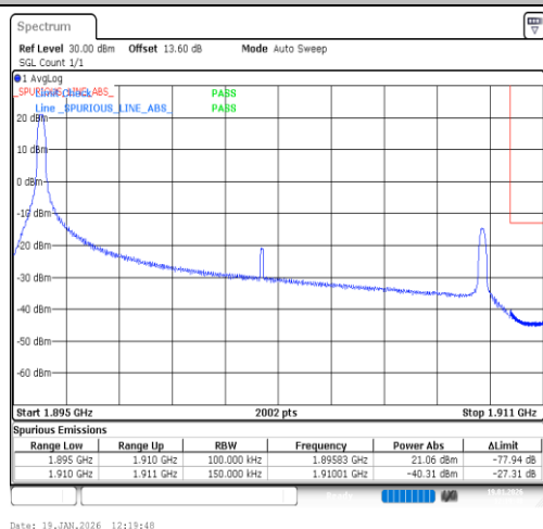
Band2-15MHz-QPSK-19125-1RB#0-PASS
