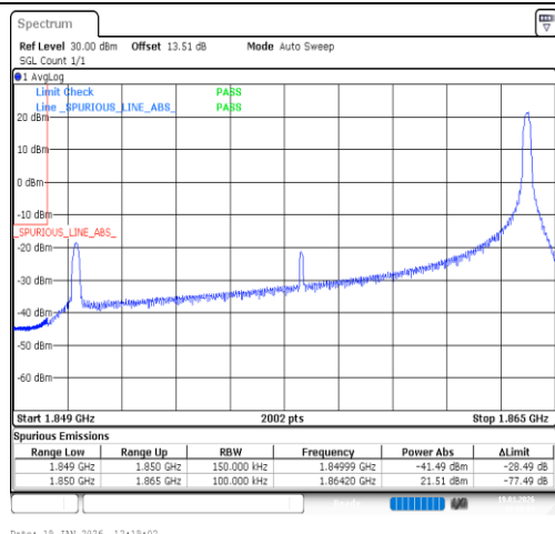
Band2-15MHz-QPSK-18675-1RB#74-PASS
