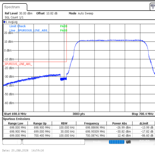
Band12-1.4MHz-16QAM-23017-6RB#0-PASS
