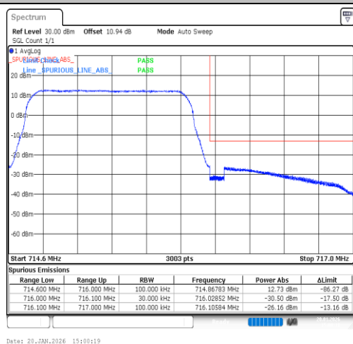
Band12-1.4MHz-QPSK-23173-6RB#0-PASS
