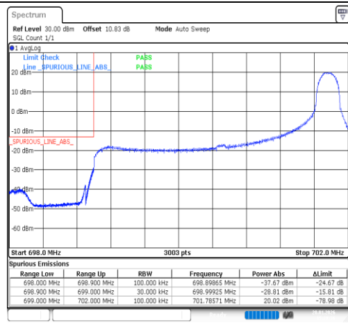
Band12-3MHz-16QAM-23025-1RB#14-PASS
