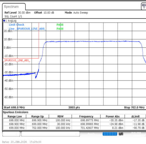
Band12-3MHz-16QAM-23025-15RB#0-PASS
