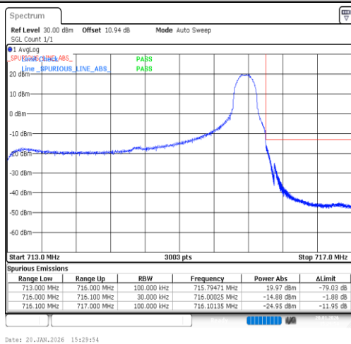
Band12-3MHz-16QAM-23165-1RB#14-PASS
