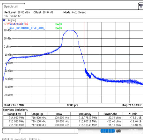
Band12-1.4MHz-16QAM-23173-1RB#5-PASS
