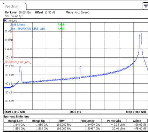
Band2-15MHz-16QAM-18675-1RB#74-PASS
