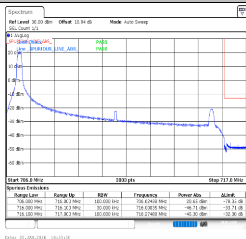
Band12-10MHz-16QAM-23130-1RB#0-PASS
