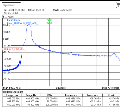
Band12-5MHz-QPSK-23035-1RB#0-PASS
