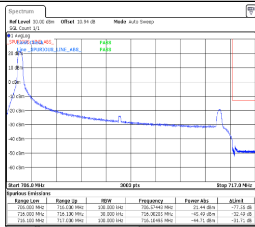
Band12-10MHz-QPSK-23060-1RB#49-PASS
