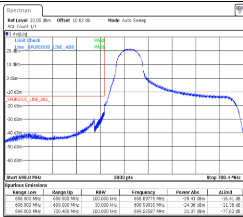
Band12-1.4MHz-QPSK-23017-1RB#0-PASS
