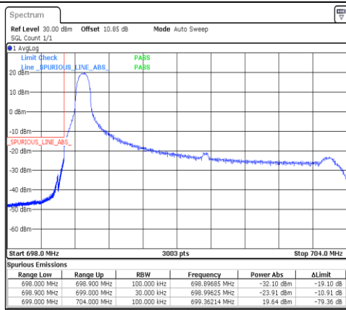
Band12-5MHz-16QAM-23035-1RB#0-PASS
