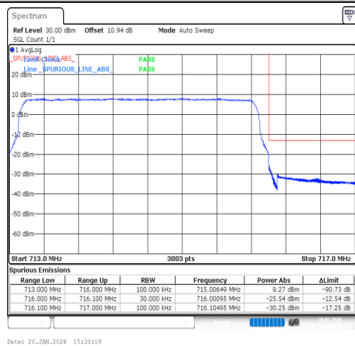
Band12-3MHz-16QAM-23165-15RB#0-PASS
