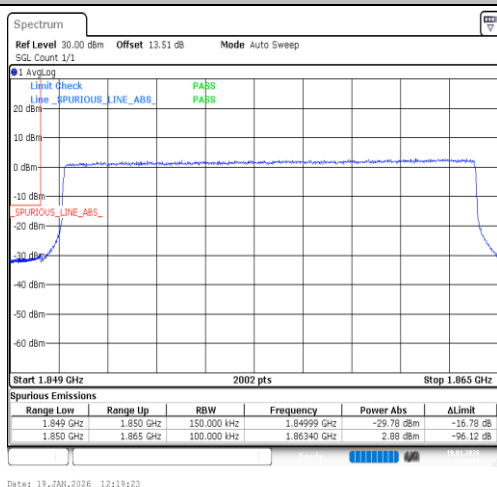
Band2-15MHz-QPSK-18675-75RB#0-PASS
