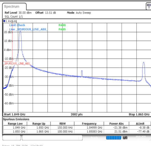
Band2-15MHz-QPSK-18675-1RB#0-PASS
