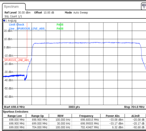
Band12-5MHz-16QAM-23035-1RB#0-PASS
