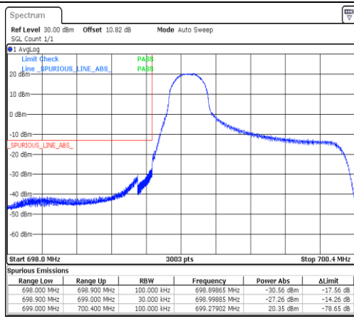
Band12-1.4MHz-16QAM-23017-1RB#0-PASS
