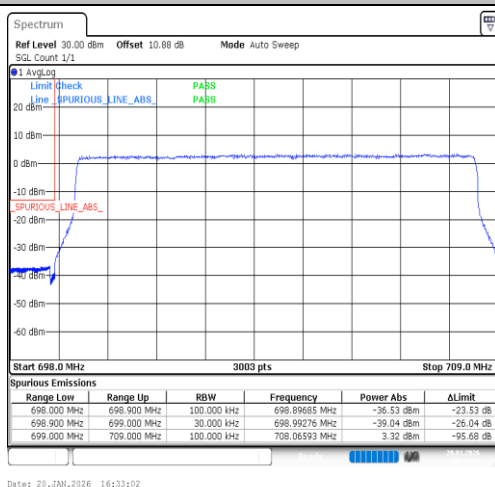
Band12-10MHz-16QAM-23060-50RB#0-PASS
