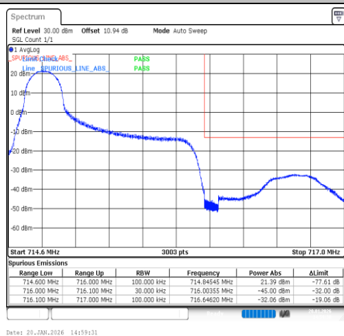
Band12-1.4MHz-QPSK-23173-1RB#0-PASS
