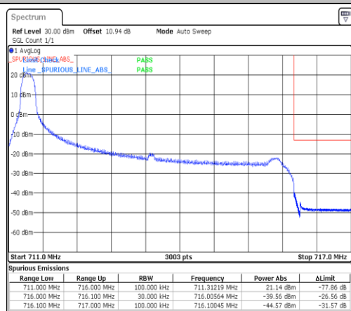
Band12-5MHz-QPSK-23035-1RB#24-PASS
