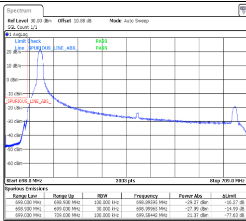
Band12-10MHz-QPSK-23060-1RB#0-PASS
