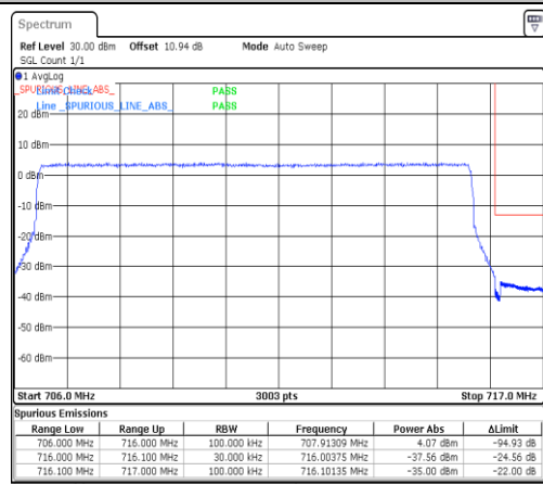
Band12-10MHz-QPSK-23130-1RB#0-PASS
