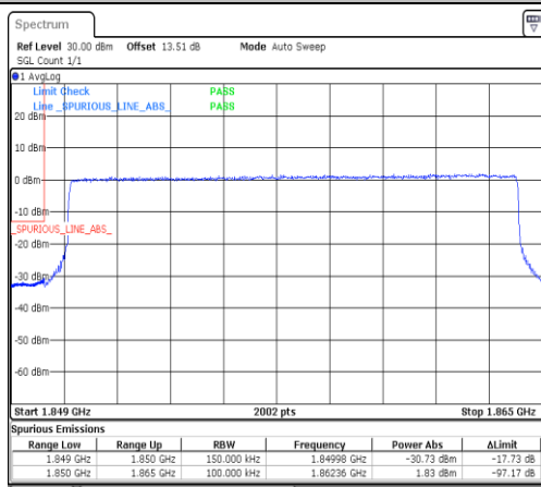
Band2-15MHz-16QAM-18675-1RB#0-PASS
