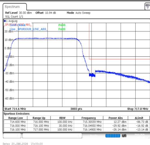
Band12-1.4MHz-16QAM-23173-6RB#0-PASS
