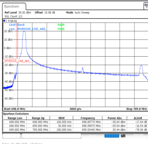
Band12-10MHz-16QAM-23060-1RB#0-PASS
