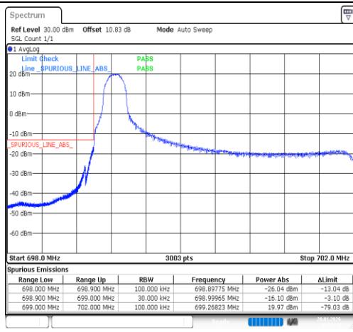
Band12-3MHz-16QAM-23025-1RB#0-PASS
