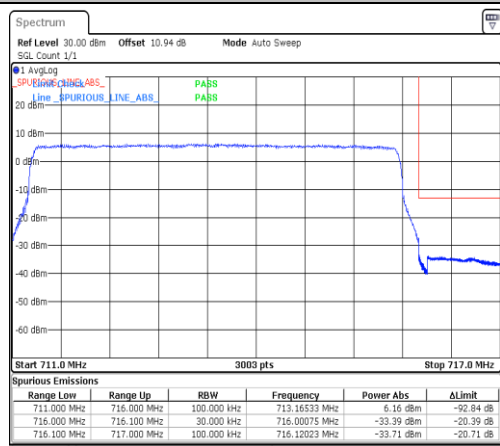
Band12-5MHz-16QAM-23155-1RB#0-PASS
