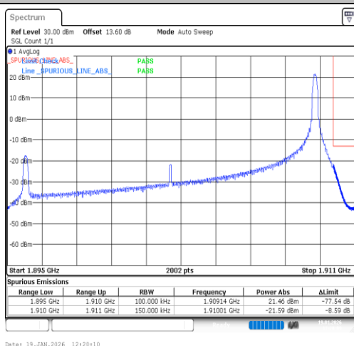
Band2-15MHz-QPSK-19125-1RB#74-PASS
