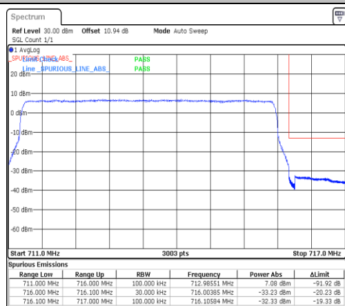
Band12-5MHz-QPSK-23155-1RB#0-PASS
