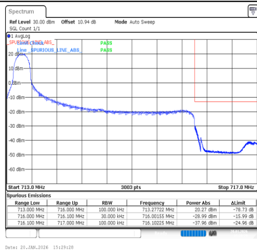
Band12-3MHz-16QAM-23165-1RB#0-PASS
