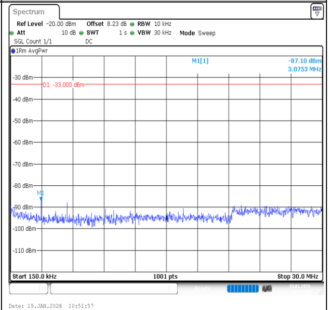
Band2-3MHz-16QAM-18900-1RB#0-0.15~30-PASS
