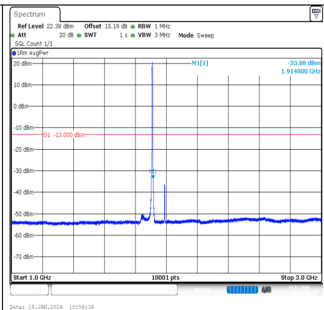
Band2-3MHz-QPSK-19185-15RB#0-1000~3000-PASS
