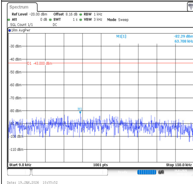
Band2-3MHz-16QAM-19185-1RB#14-0.009~0.15-PASS
