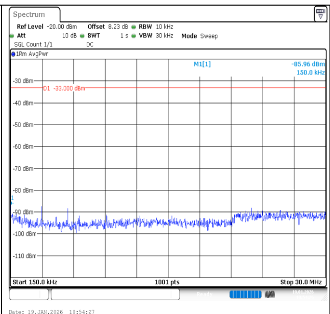
Band2-3MHz-QPSK-19185-1RB#0-0.15~30-PASS
