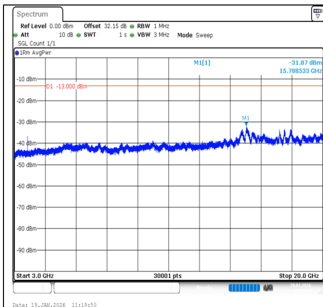
Band2-5MHz-QPSK-18625-1RB#0-3000~20000-PASS
