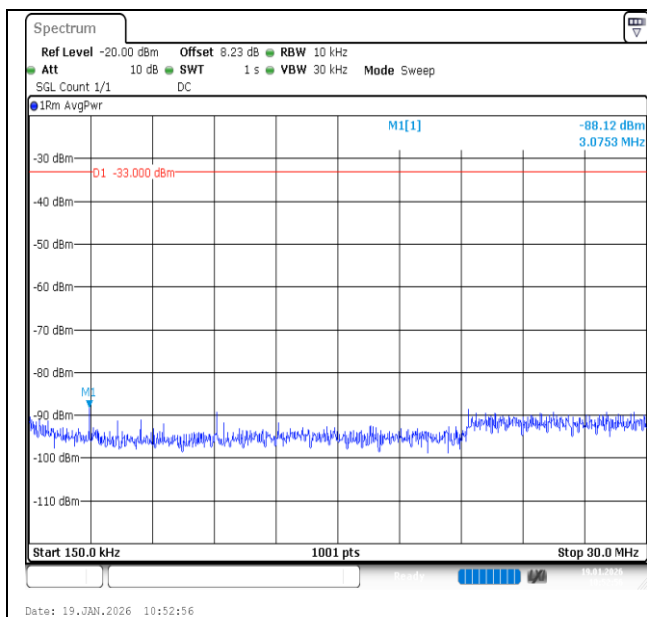
Band2-3MHz-16QAM-18900-1RB#14-0.15~30-PASS
