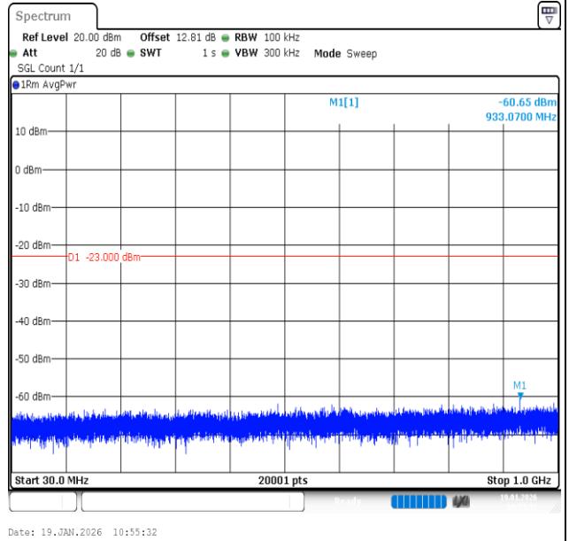
Band2-3MHz-QPSK-19185-1RB#14-30~1000-PASS
