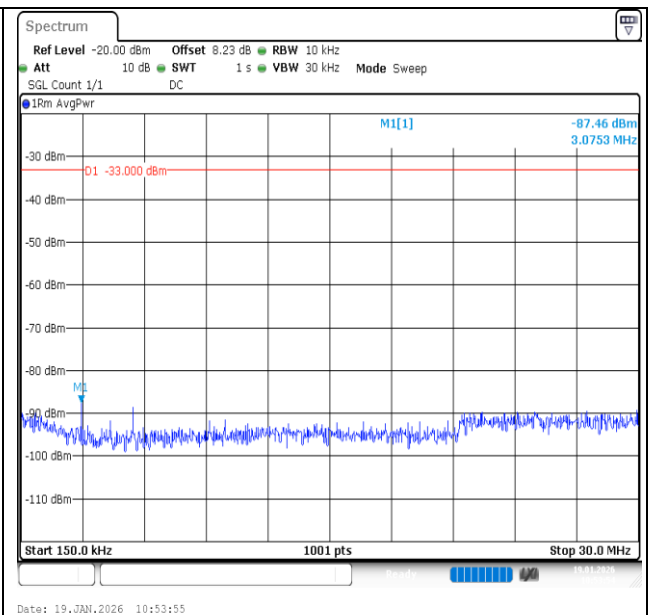
Band2-3MHz-16QAM-18900-15RB#0-0.15~30-PASS
