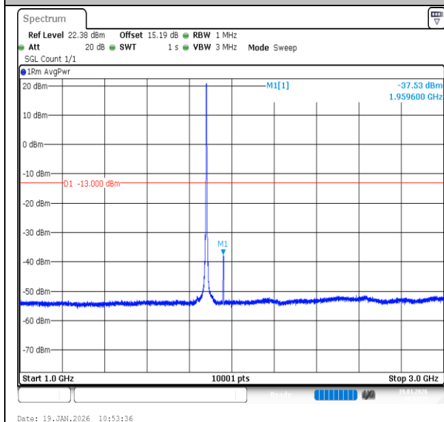
Band2-3MHz-QPSK-18900-15RB#0-1000~3000-PASS
