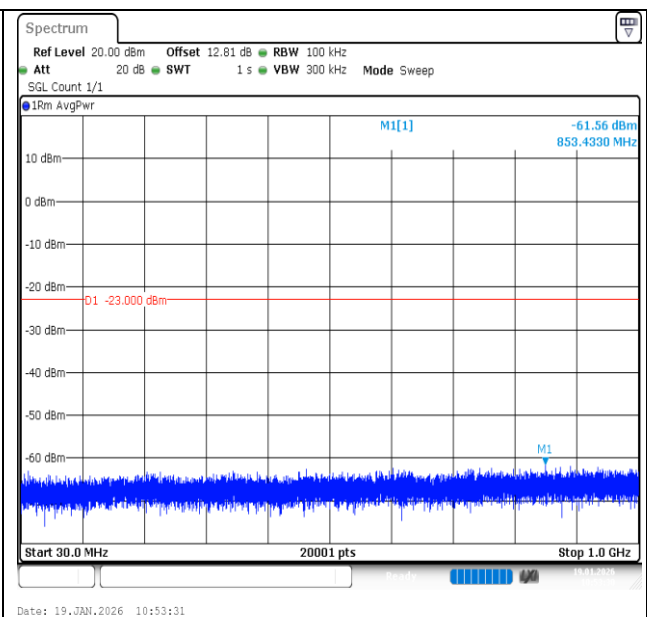
Band2-3MHz-QPSK-18900-15RB#0-30~1000-PASS
