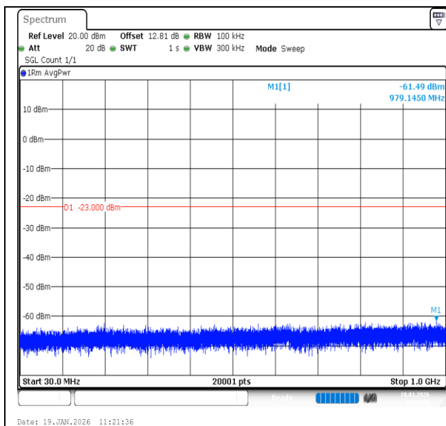
Band2-5MHz-QPSK-18625-25RB#0-30~1000-PASS
