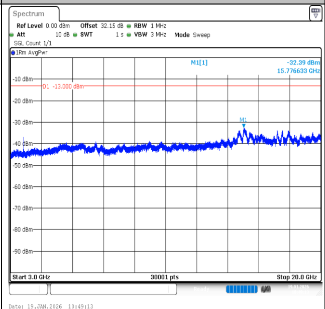
Band2-3MHz-16QAM-18615-1RB#0-3000~20000-PASS
