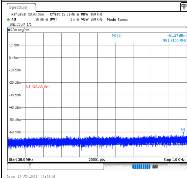
Band2-3MHz-16QAM-18900-15RB#0-30~1000-PASS
