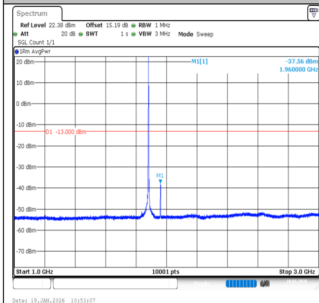
Band2-3MHz-16QAM-18900-1RB#14-1000~3000-PASS
