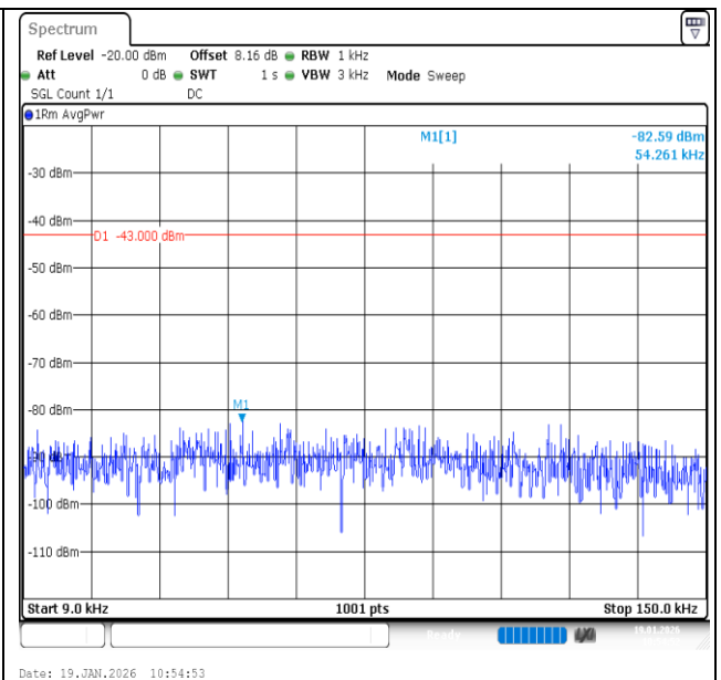
Band2-3MHz-16QAM-19185-1RB#0-0.009~0.15-PASS
