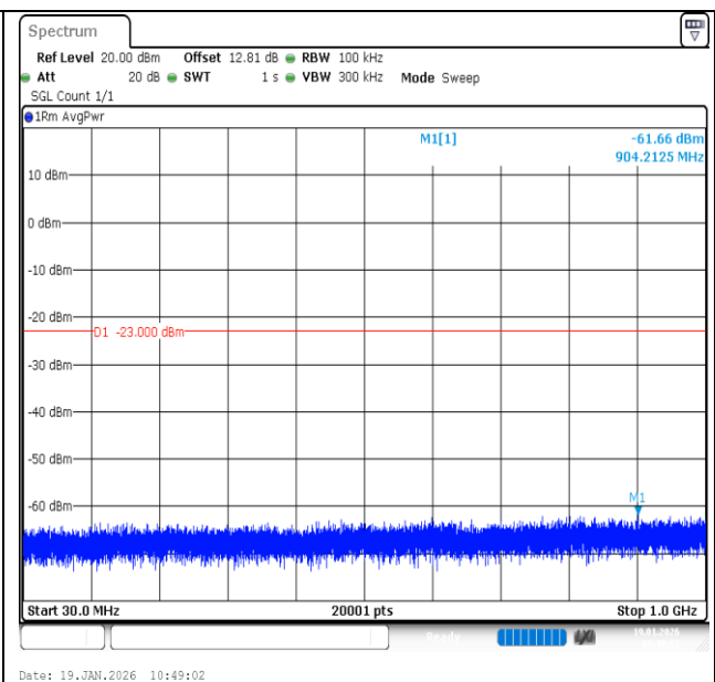
Band2-3MHz-16QAM-18615-1RB#0-30~1000-PASS
