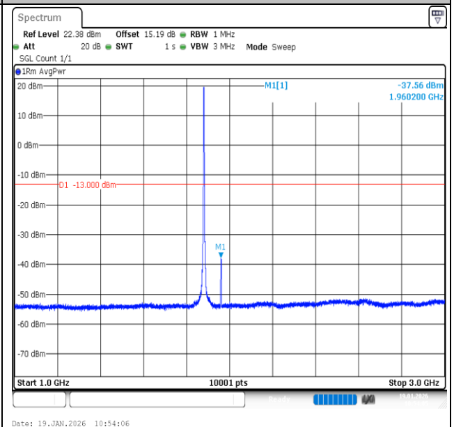
Band2-3MHz-16QAM-18900-15RB#0-1000~3000-PASS
