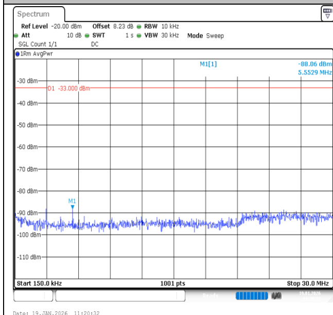
Band2-5MHz-QPSK-18625-1RB#24-0.15~30-PASS
