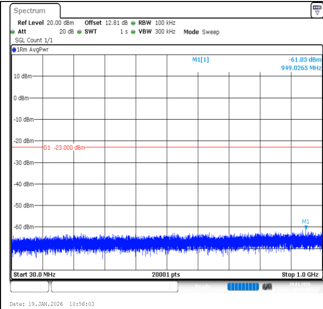
Band2-3MHz-16QAM-19185-1RB#14-30~1000-PASS
