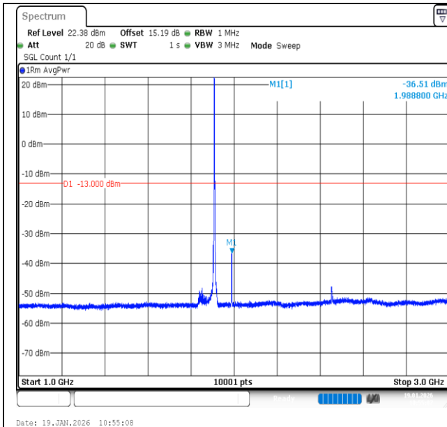
Band2-3MHz-16QAM-19185-1RB#0-1000~3000-PASS
