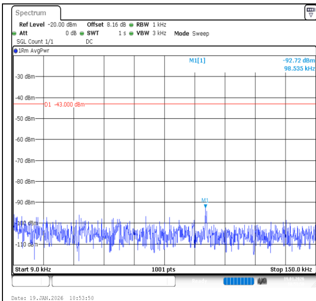
Band2-3MHz-16QAM-18900-15RB#0-0.009~0.15-PASS
