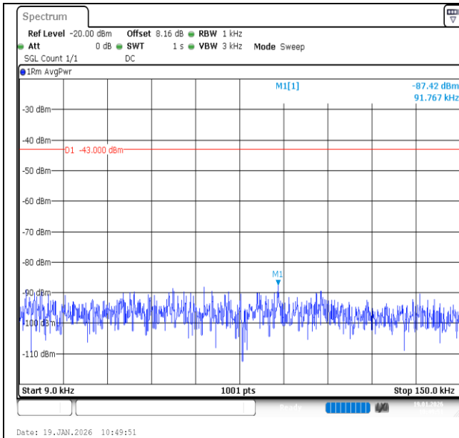
Band2-3MHz-16QAM-18615-1RB#14-0.009~0.15-PASS
