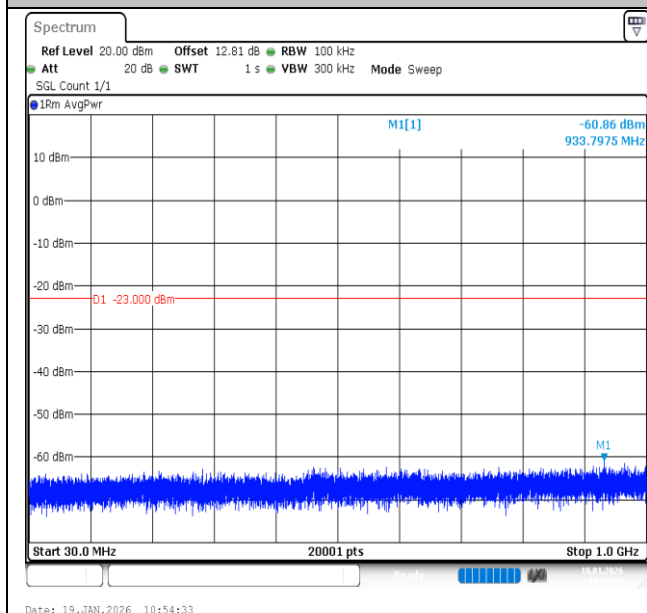
Band2-3MHz-QPSK-19185-1RB#0-30~1000-PASS
