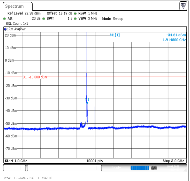
Band2-3MHz-16QAM-19185-1RB#14-1000~3000-PASS
