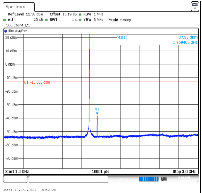
Band2-3MHz-16QAM-18900-1RB#0-1000~3000-PASS
