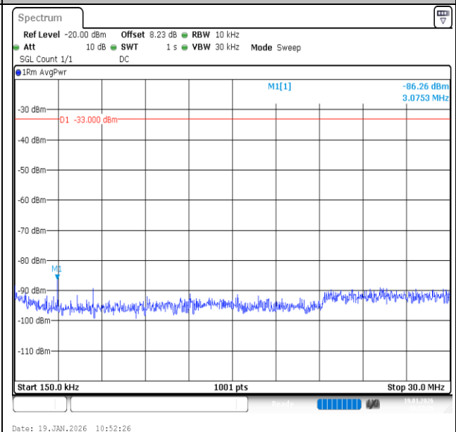
Band2-3MHz-QPSK-18900-1RB#14-0.15~30-PASS
