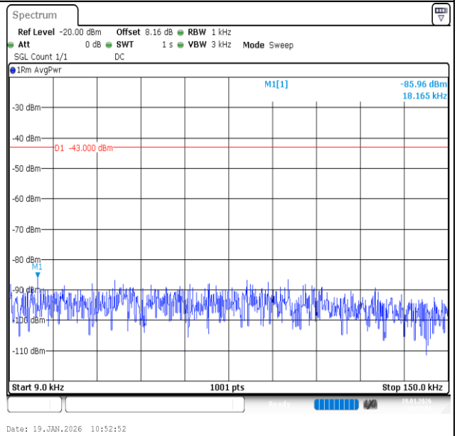
Band2-3MHz-16QAM-18900-1RB#14-0.009~0.15-PASS
