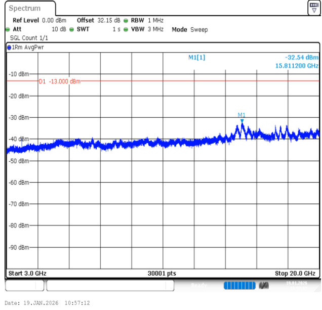
Band2-3MHz-16QAM-19185-15RB#0-3000~20000-PASS
