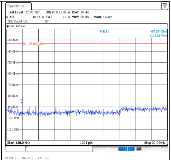
Band2-5MHz-QPSK-18625-1RB#0-0.15~30-PASS
