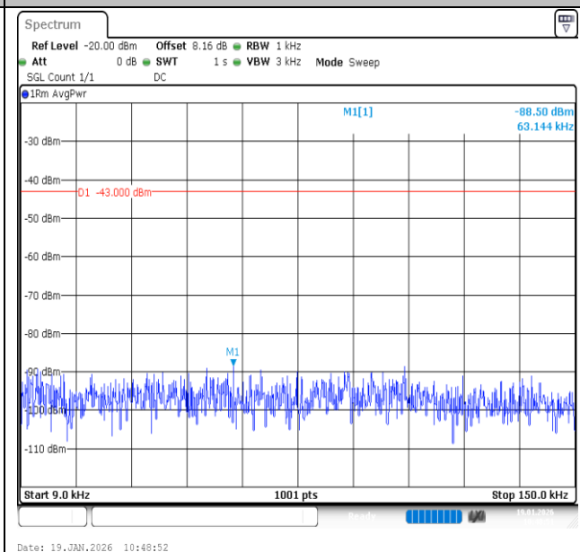
Band2-3MHz-16QAM-18615-1RB#0-0.009~0.15-PASS
