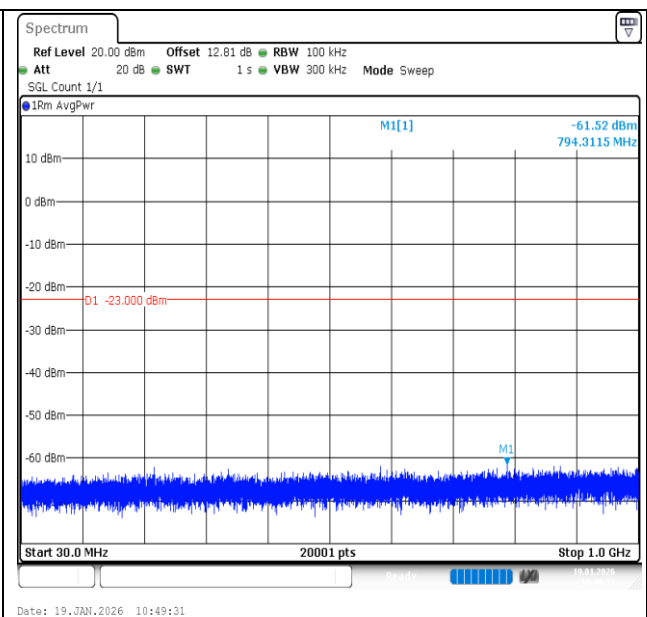
Band2-3MHz-QPSK-18615-1RB#14-30~1000-PASS
