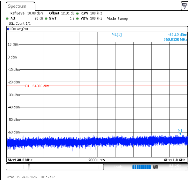
Band2-3MHz-16QAM-18900-1RB#0-30~1000-PASS
