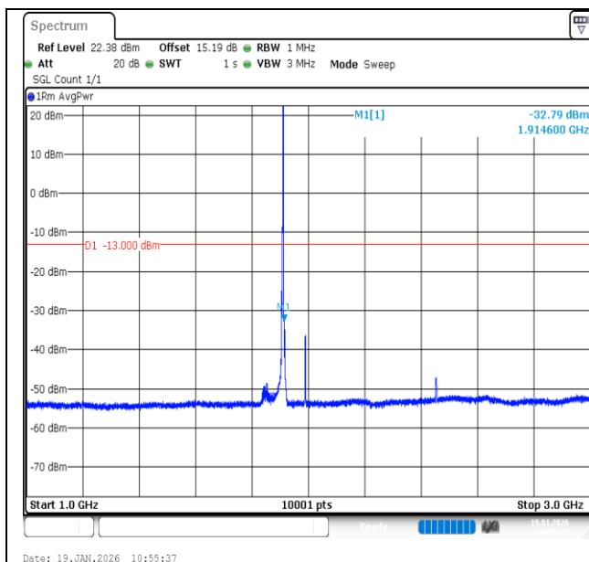
Band2-3MHz-QPSK-19185-1RB#14-1000~3000-PASS
