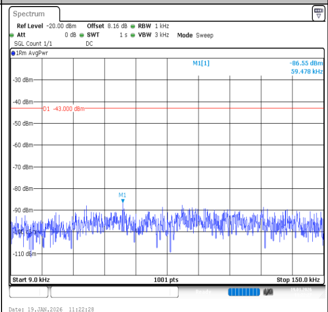
Band2-5MHz-QPSK-18900-1RB#0-0.009~0.15-PASS
