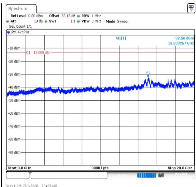
Band2-1.4MHz-16QAM-19193-6RB#0-3000~20000-PASS
