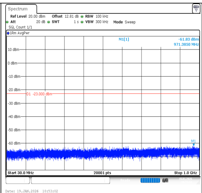
Band2-3MHz-16QAM-18900-1RB#14-30~1000-PASS
