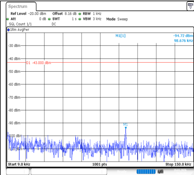
Band2-3MHz-QPSK-18615-15RB#0-0.009~0.15-PASS
