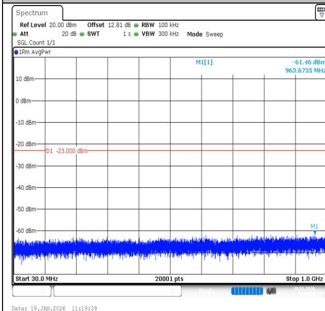
Band2-5MHz-QPSK-18625-1RB#0-30~1000-PASS
