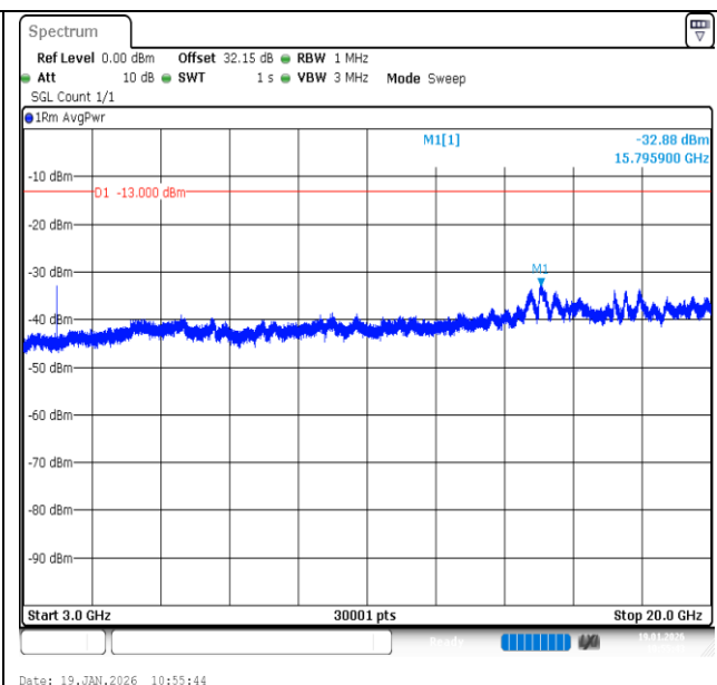
Band2-3MHz-QPSK-19185-1RB#14-3000~20000-PASS
