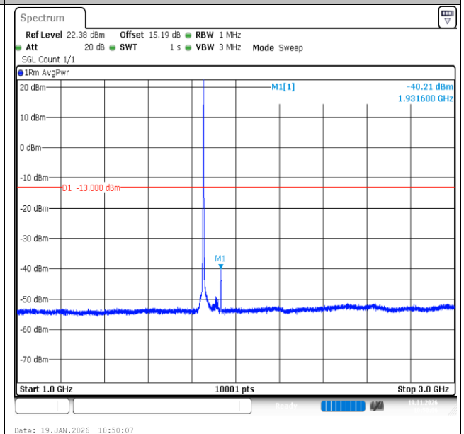
Band2-3MHz-16QAM-18615-1RB#14-1000~3000-PASS
