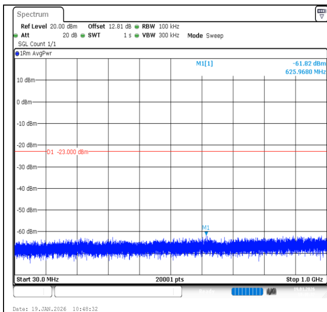
Band2-3MHz-QPSK-18615-1RB#0-30~1000-PASS
