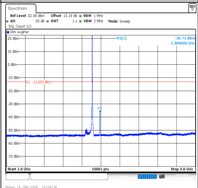
Band2-3MHz-QPSK-19185-1RB#0-1000~3000-PASS
