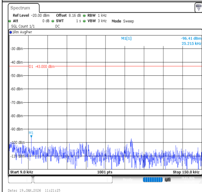
Band2-5MHz-QPSK-18625-25RB#0-0.009~0.15-PASS
