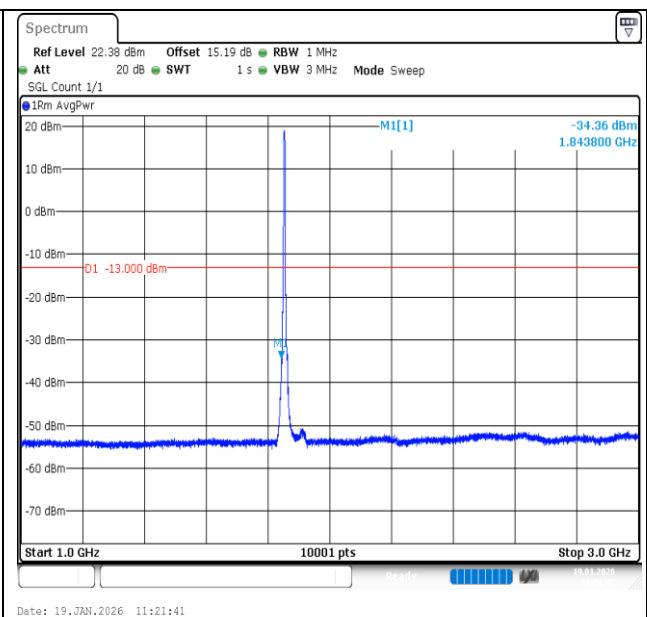
Band2-5MHz-QPSK-18625-25RB#0-1000~3000-PASS
