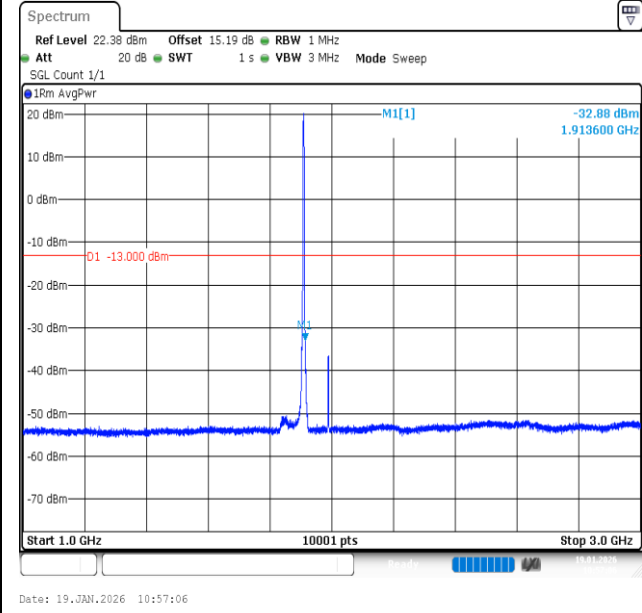
Band2-3MHz-16QAM-19185-15RB#0-1000~3000-PASS
