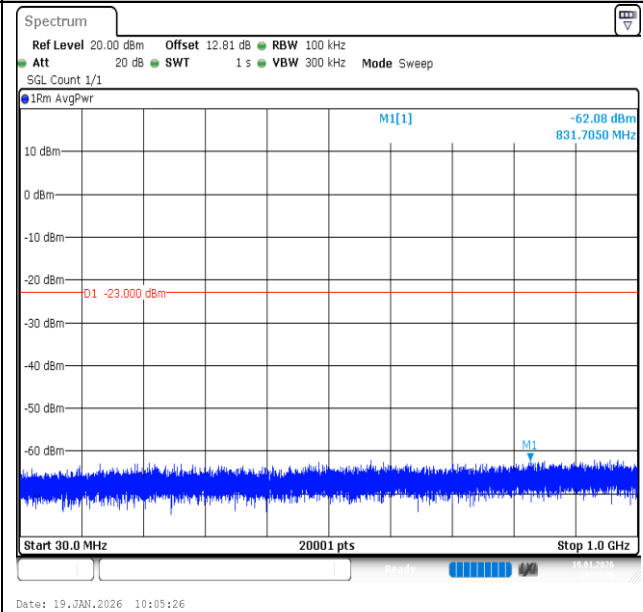
Band2-1.4MHz-16QAM-19193-6RB#0-30~1000-PASS
