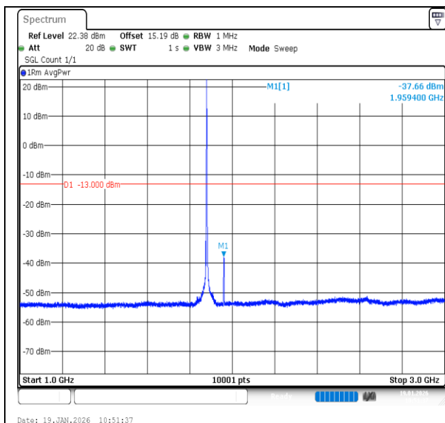
Band2-3MHz-QPSK-18900-1RB#0-1000~3000-PASS
