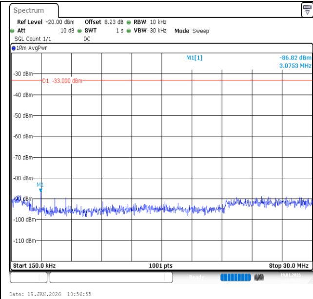
Band2-3MHz-16QAM-19185-15RB#0-0.15~30-PASS
