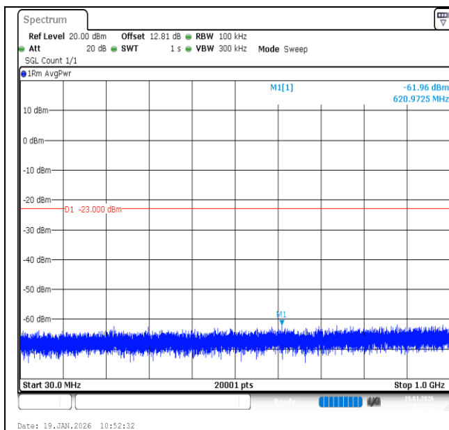
Band2-3MHz-QPSK-18900-1RB#14-30~1000-PASS
