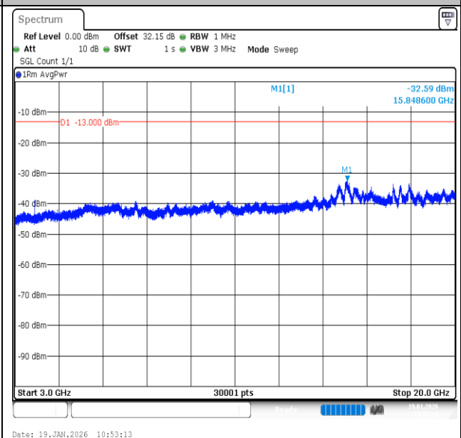
Band2-3MHz-16QAM-18900-1RB#14-3000~20000-PASS
