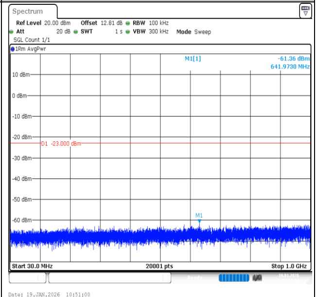
Band2-3MHz-16QAM-18615-15RB#0-30~1000-PASS
