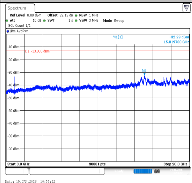
Band2-3MHz-QPSK-18900-15RB#0-3000~20000-PASS
