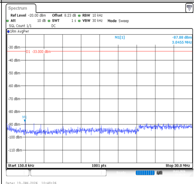
Band2-3MHz-QPSK-18615-1RB#0-0.15~30-PASS
