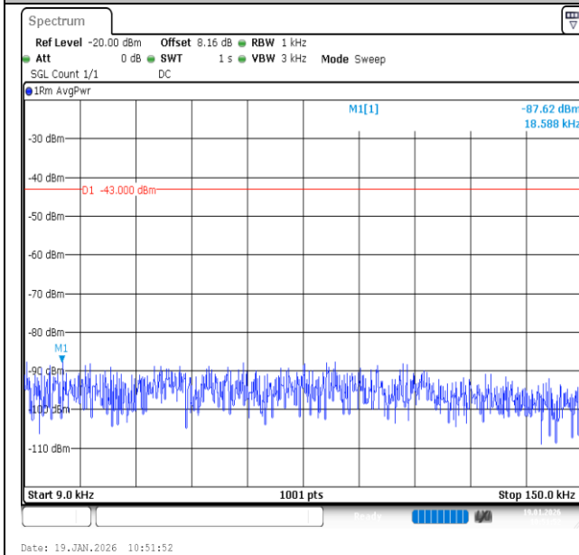
Band2-3MHz-16QAM-18900-1RB#0-0.009~0.15-PASS
