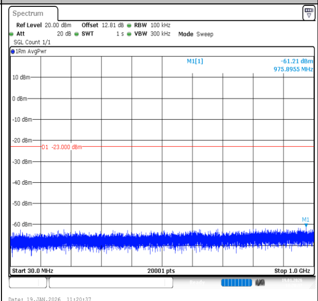
Band2-5MHz-QPSK-18625-1RB#24-30~1000-PASS
