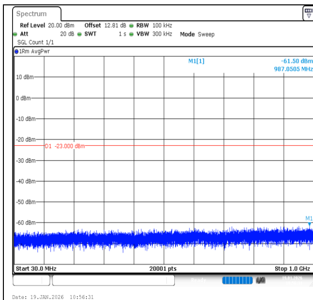
Band2-3MHz-QPSK-19185-15RB#0-30~1000-PASS
