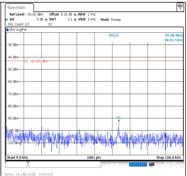
Band2-3MHz-16QAM-18615-15RB#0-0.009~0.15-PASS
