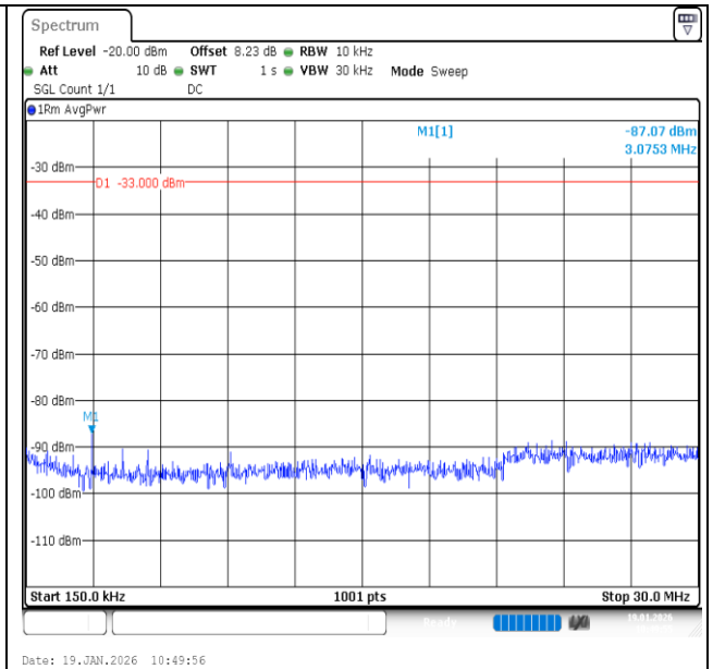
Band2-3MHz-16QAM-18615-1RB#14-0.15~30-PASS
