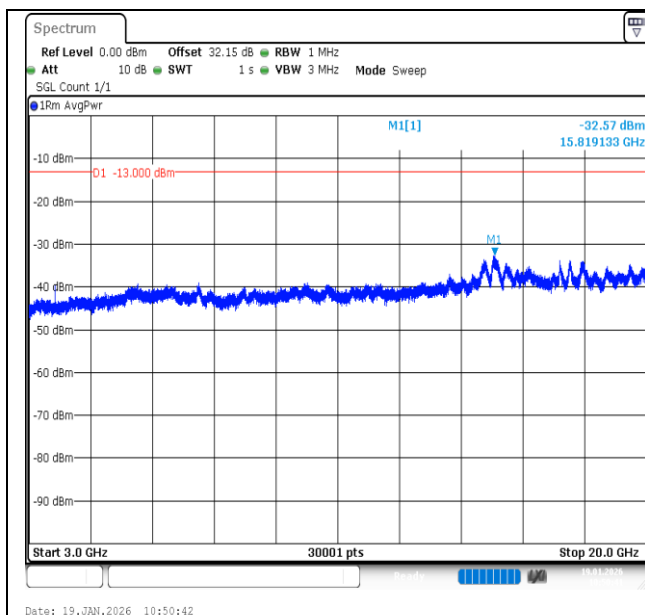
Band2-3MHz-QPSK-18615-15RB#0-3000~20000-PASS
