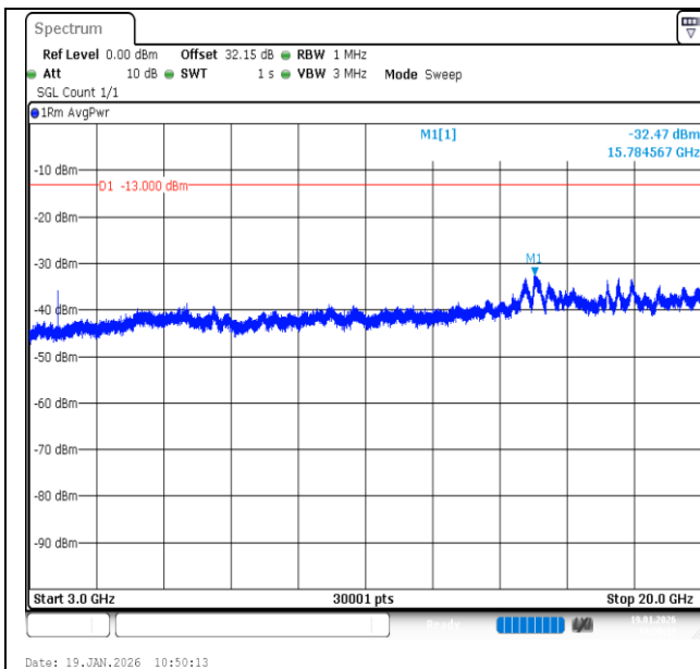
Band2-3MHz-16QAM-18615-1RB#14-3000~20000-PASS
