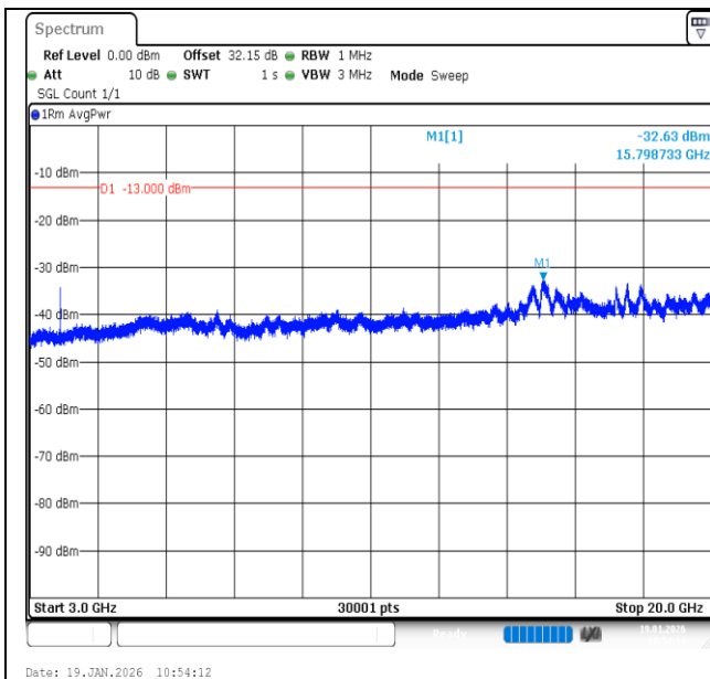
Band2-3MHz-16QAM-18900-15RB#0-3000~20000-PASS
