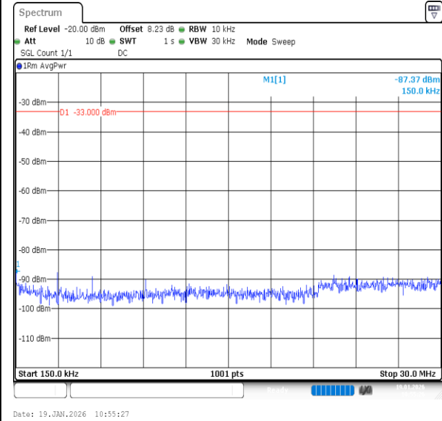
Band2-3MHz-QPSK-19185-1RB#14-0.15~30-PASS
