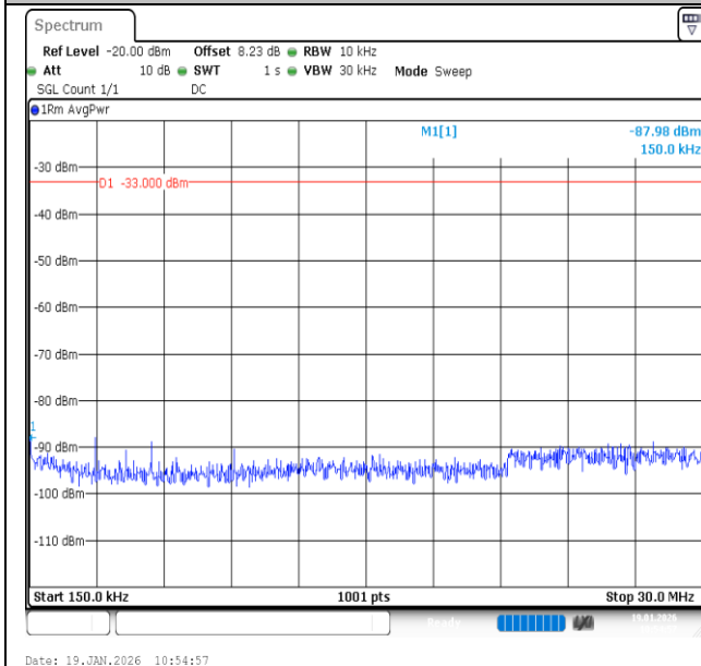
Band2-3MHz-16QAM-19185-1RB#0-0.15~30-PASS
