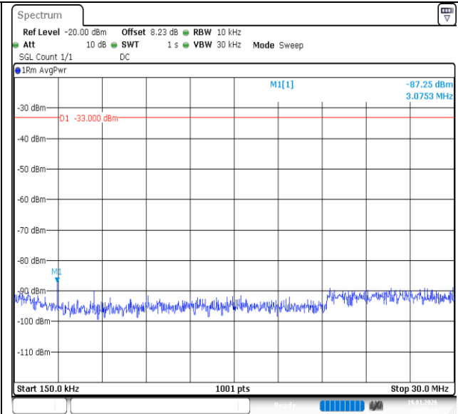
Band2-3MHz-QPSK-18615-15RB#0-0.15~30-PASS
