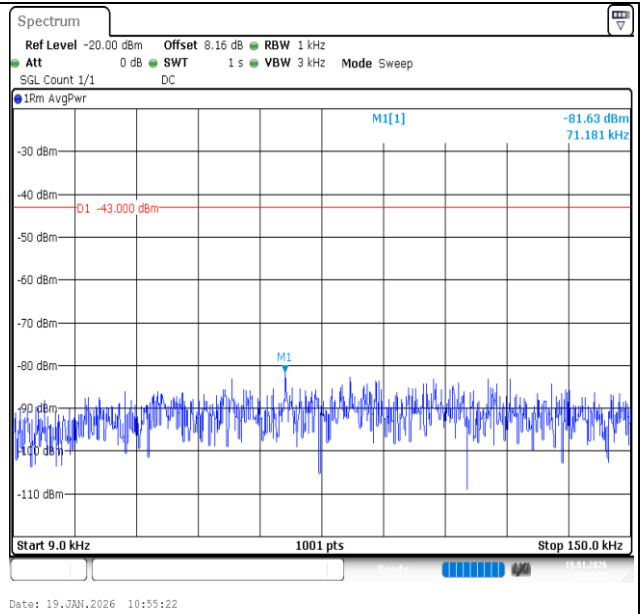
Band2-3MHz-QPSK-19185-1RB#14-0.009~0.15-PASS
