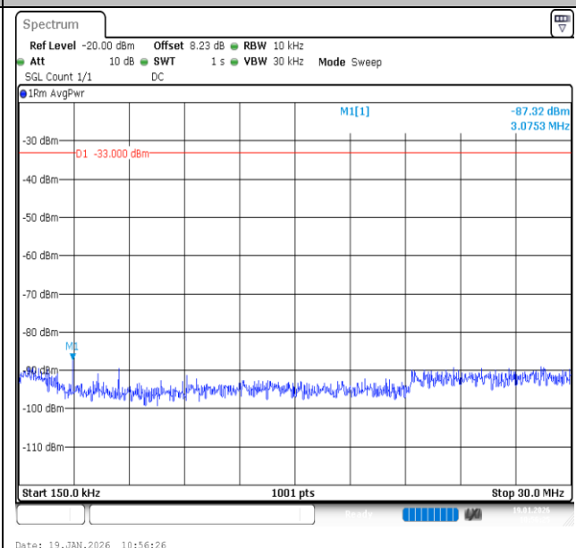
Band2-3MHz-QPSK-19185-15RB#0-0.15~30-PASS
