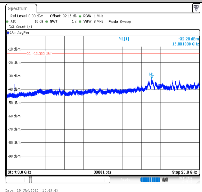
Band2-3MHz-QPSK-18615-1RB#14-3000~20000-PASS
