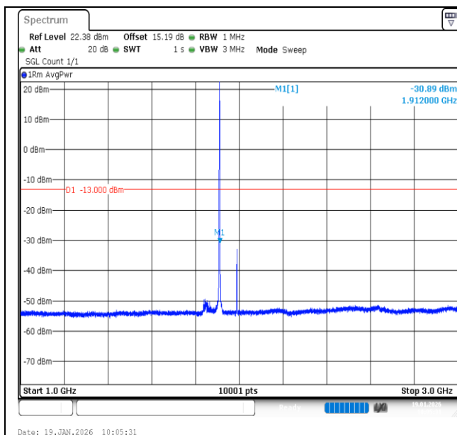
Band2-1.4MHz-16QAM-19193-6RB#0-1000~3000-PASS
