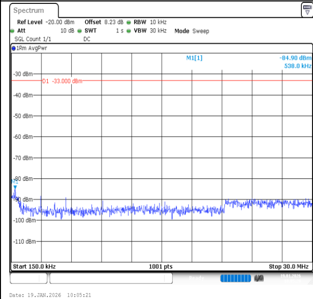
Band2-1.4MHz-16QAM-19193-6RB#0-0.15~30-PASS
