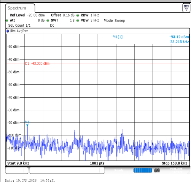
Band2-3MHz-QPSK-18900-15RB#0-0.009~0.15-PASS
