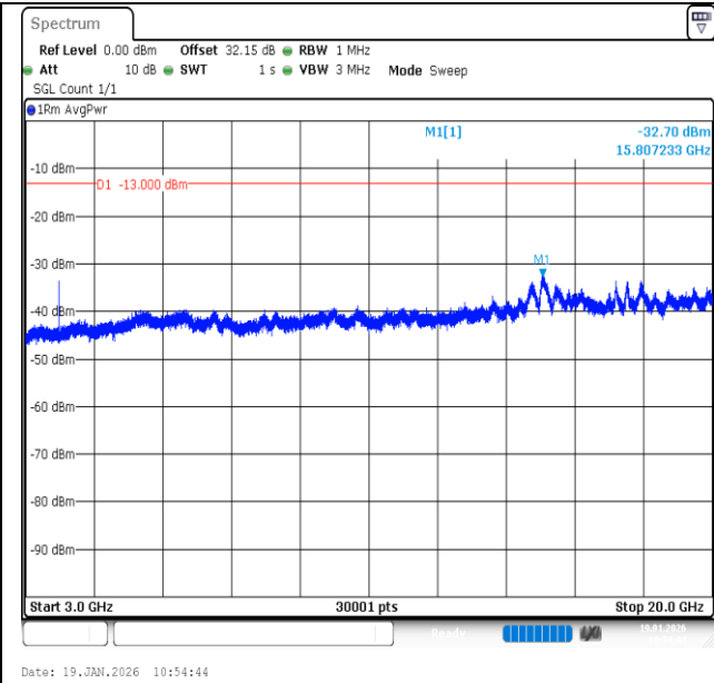
Band2-3MHz-QPSK-19185-1RB#0-3000~20000-PASS
