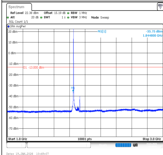
Band2-3MHz-16QAM-18615-1RB#0-1000~3000-PASS
