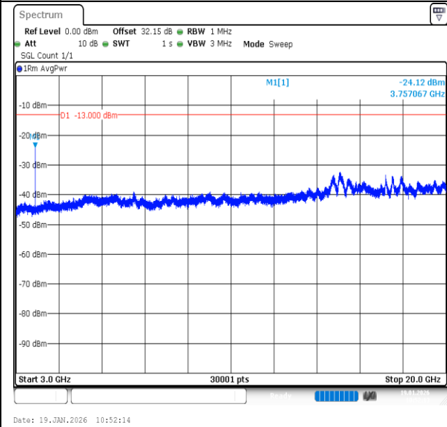
Band2-3MHz-16QAM-18900-1RB#0-3000~20000-PASS
