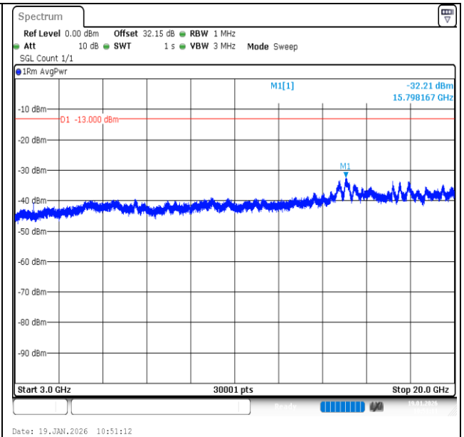
Band2-3MHz-16QAM-18615-15RB#0-3000~20000-PASS
