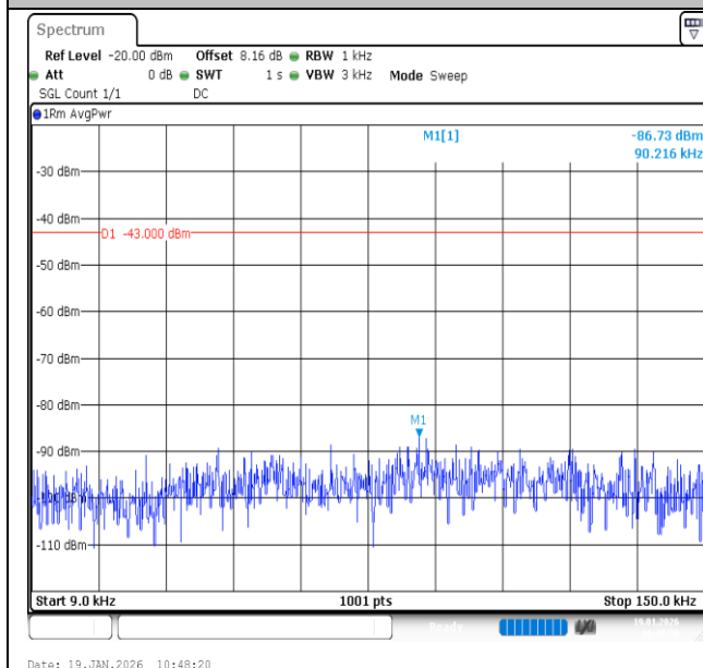
Band2-3MHz-QPSK-18615-1RB#0-0.009~0.15-PASS
