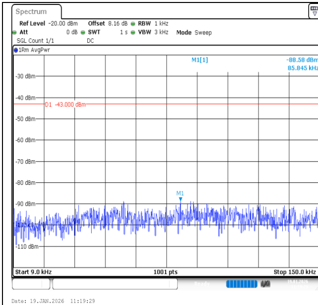
Band2-5MHz-QPSK-18625-1RB#0-0.009~0.15-PASS
