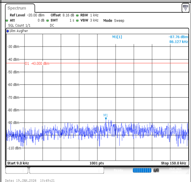
Band2-3MHz-QPSK-18615-1RB#14-0.009~0.15-PASS
