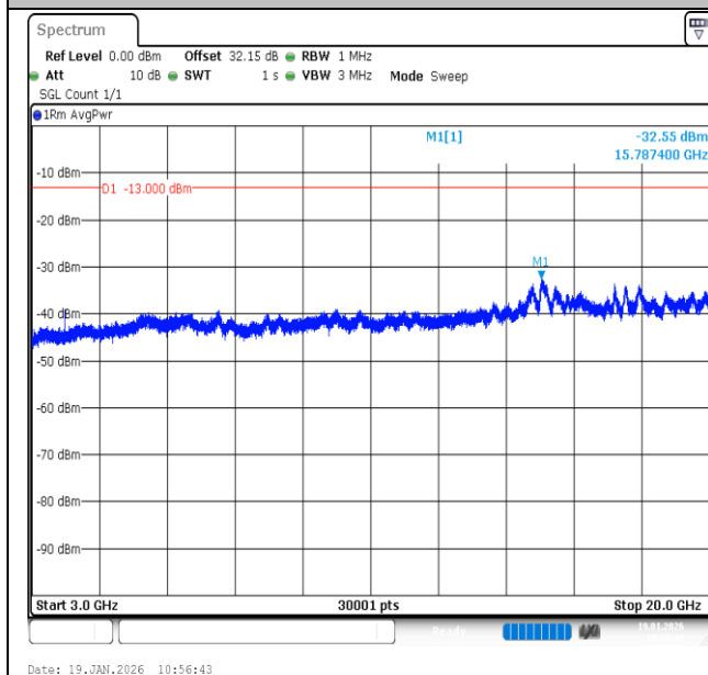
Band2-3MHz-QPSK-19185-15RB#0-3000~20000-PASS
