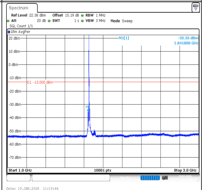
Band2-5MHz-QPSK-18625-1RB#0-1000~3000-PASS
