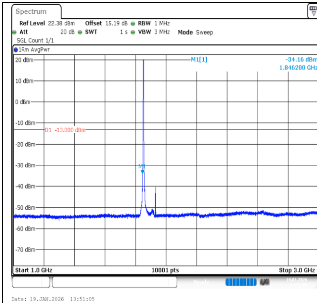
Band2-3MHz-16QAM-18615-15RB#0-1000~3000-PASS
