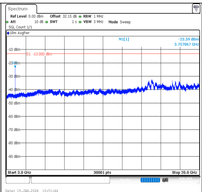
Band2-3MHz-QPSK-18900-1RB#0-3000~20000-PASS
