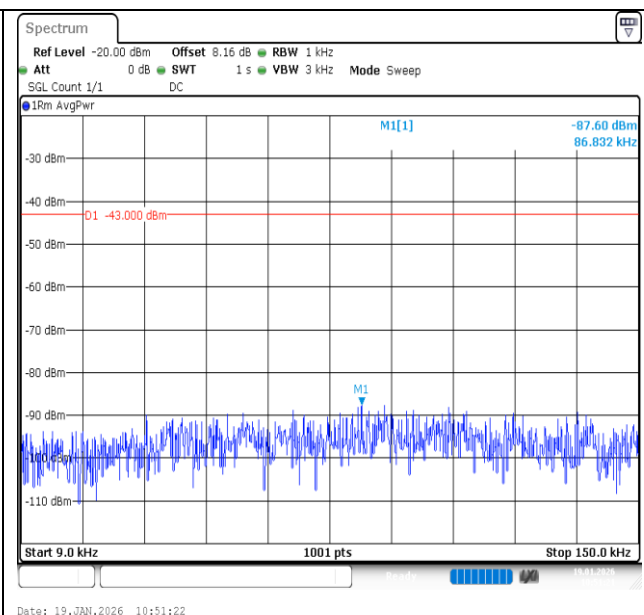
Band2-3MHz-QPSK-18900-1RB#0-0.009~0.15-PASS
