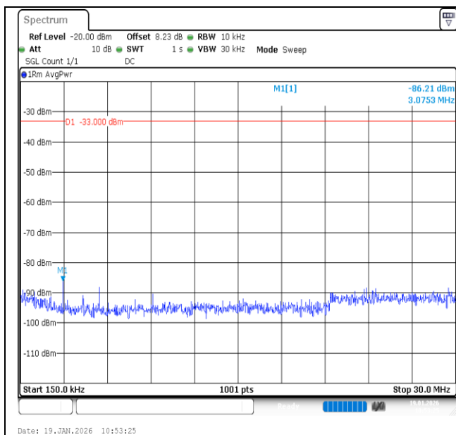
Band2-3MHz-QPSK-18900-15RB#0-0.15~30-PASS
