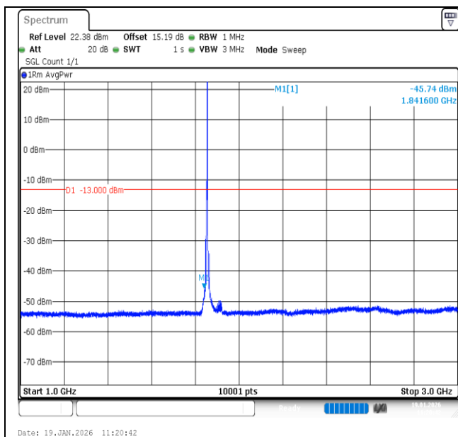
Band2-5MHz-QPSK-18625-1RB#24-1000~3000-PASS
