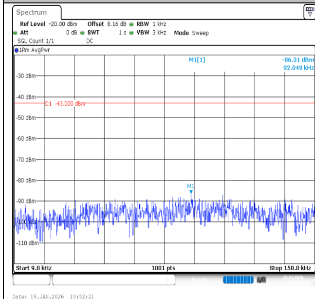
Band2-3MHz-QPSK-18900-1RB#14-0.009~0.15-PASS
