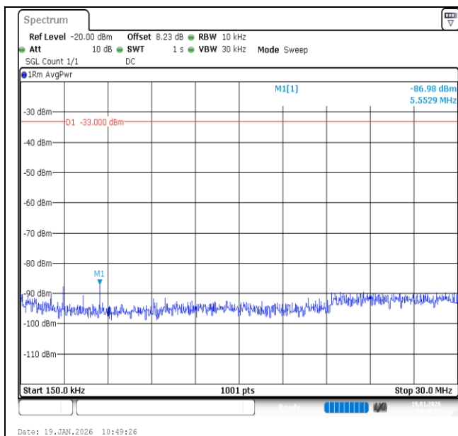
Band2-3MHz-QPSK-18615-1RB#14-0.15~30-PASS
