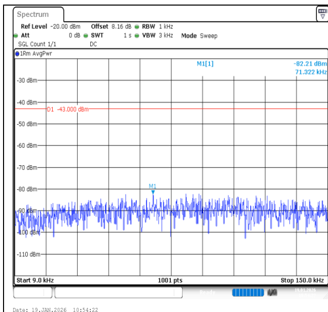
Band2-3MHz-QPSK-19185-1RB#0-0.009~0.15-PASS
