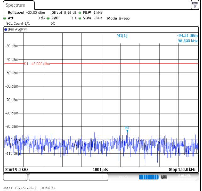
Band2-3MHz-16QAM-19185-15RB#0-0.009~0.15-PASS
