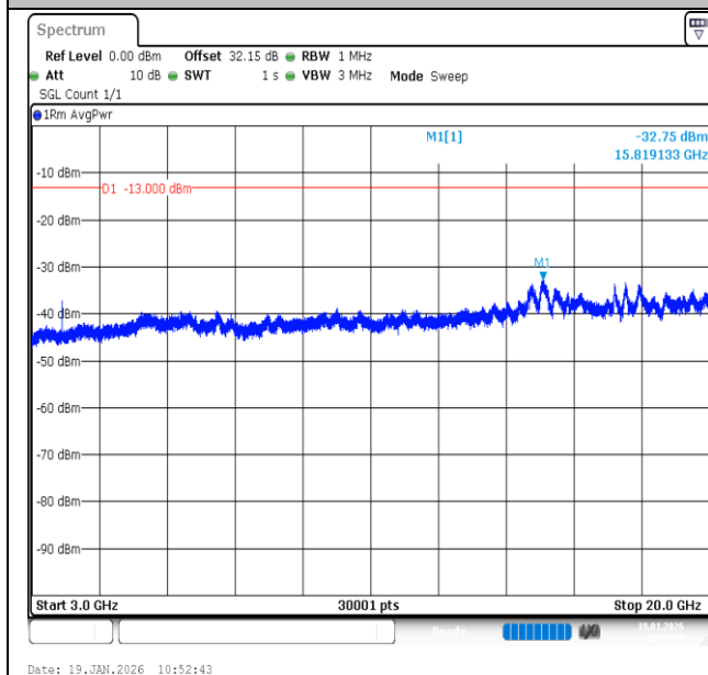
Band2-3MHz-QPSK-18900-1RB#14-3000~20000-PASS
