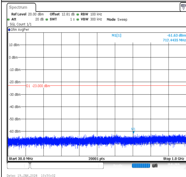
Band2-3MHz-16QAM-18615-1RB#14-30~1000-PASS
