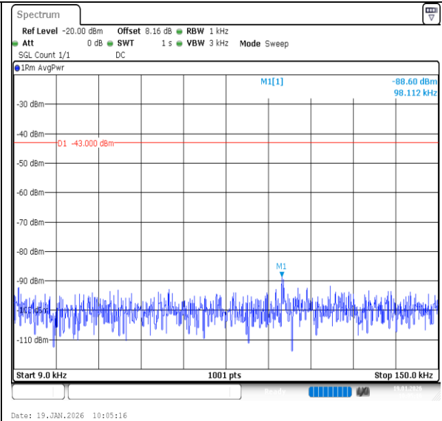
Band2-1.4MHz-16QAM-19193-6RB#0-0.009~0.15-PASS
