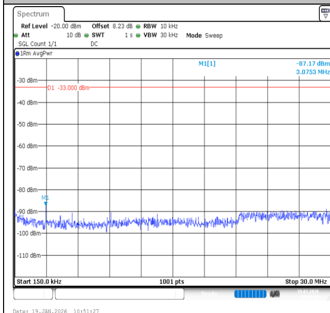
Band2-3MHz-QPSK-18900-1RB#0-0.15~30-PASS
