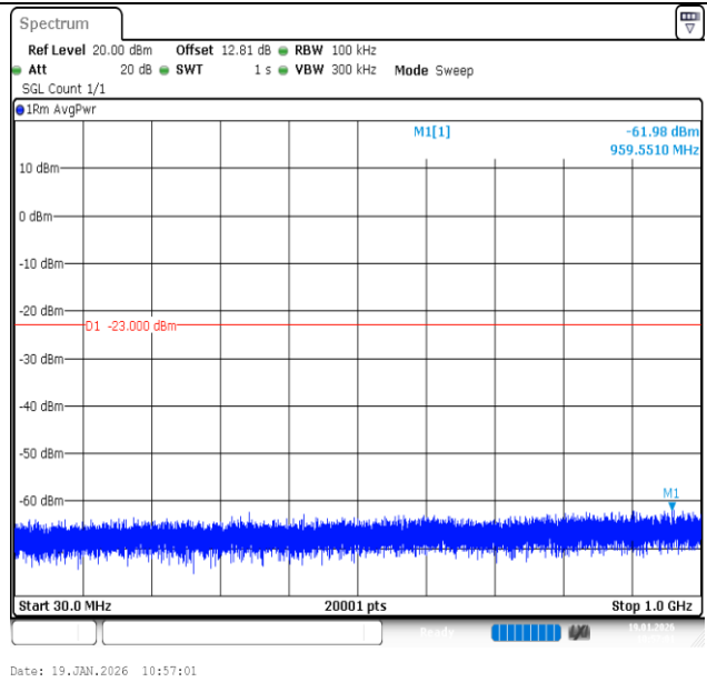
Band2-3MHz-16QAM-19185-15RB#0-30~1000-PASS
