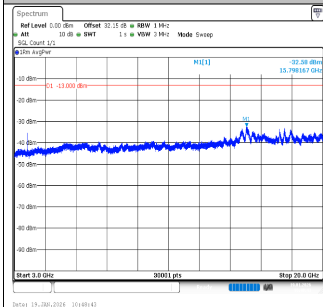
Band2-3MHz-QPSK-18615-1RB#0-3000~20000-PASS
