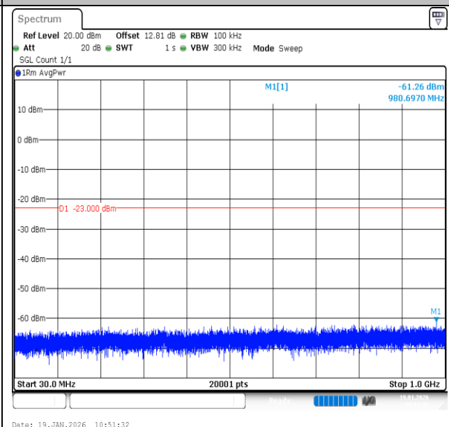
Band2-3MHz-QPSK-18900-1RB#0-30~1000-PASS
