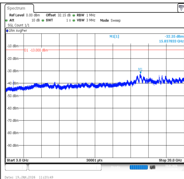
Band2-5MHz-QPSK-18625-1RB#24-3000~20000-PASS
