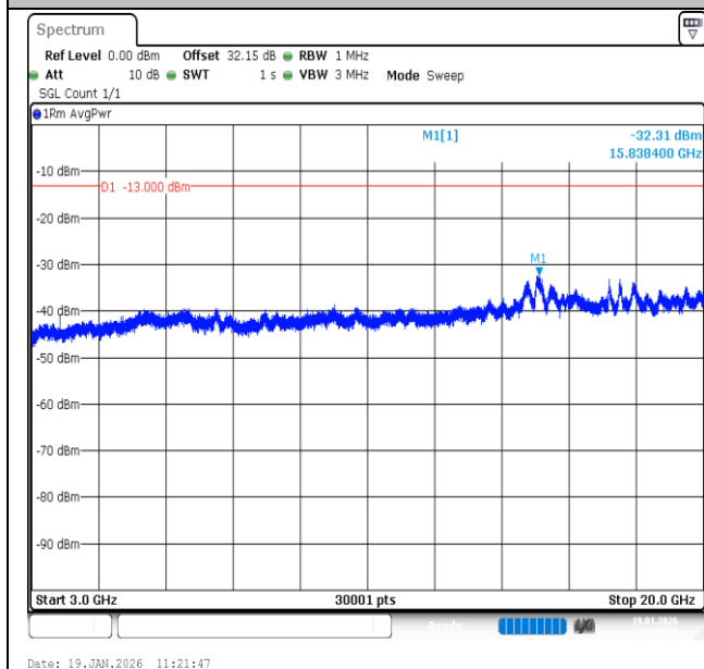
Band2-5MHz-QPSK-18625-25RB#0-3000~20000-PASS
