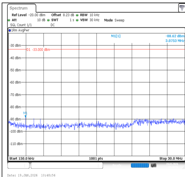
Band2-3MHz-16QAM-18615-1RB#0-0.15~30-PASS
