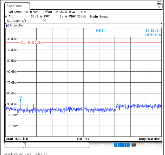
Band2-3MHz-16QAM-19185-1RB#14-0.15~30-PASS
