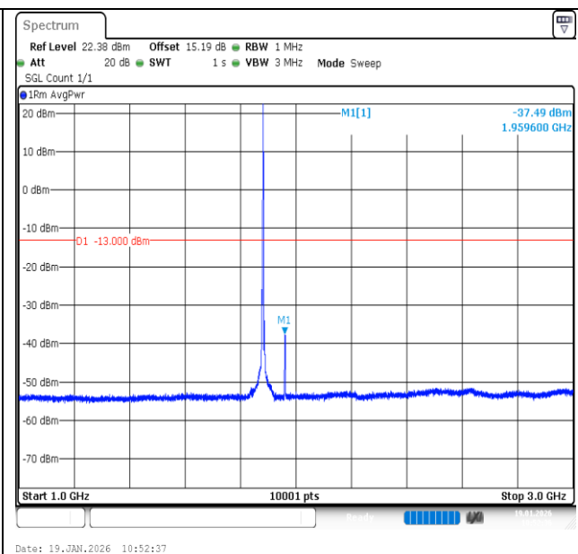
Band2-3MHz-QPSK-18900-1RB#14-1000~3000-PASS
