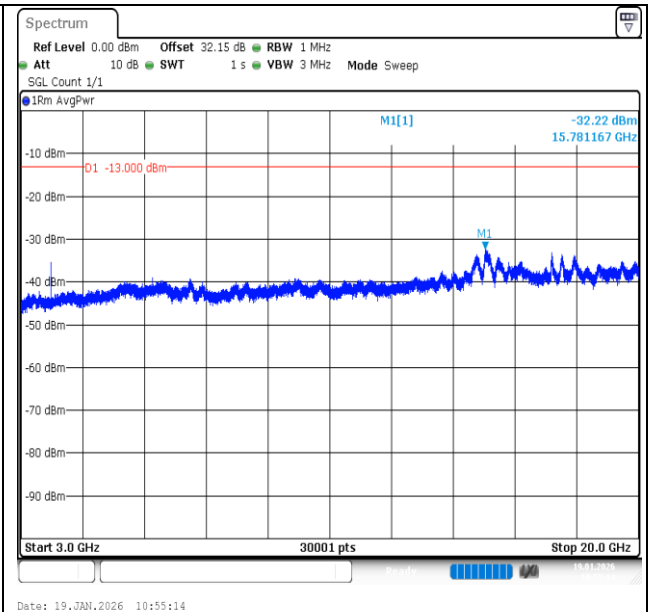
Band2-3MHz-16QAM-19185-1RB#0-3000~20000-PASS
