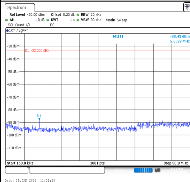
Band2-5MHz-QPSK-18625-25RB#0-0.15~30-PASS
