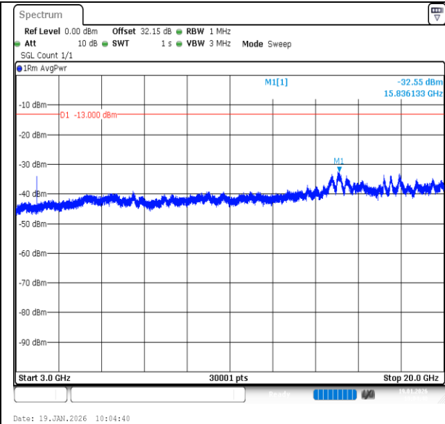
Band2-1.4MHz-16QAM-19193-1RB#5-3000~20000-PASS
