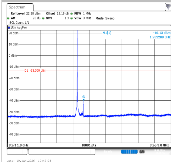
Band2-3MHz-QPSK-18615-1RB#14-1000~3000-PASS
