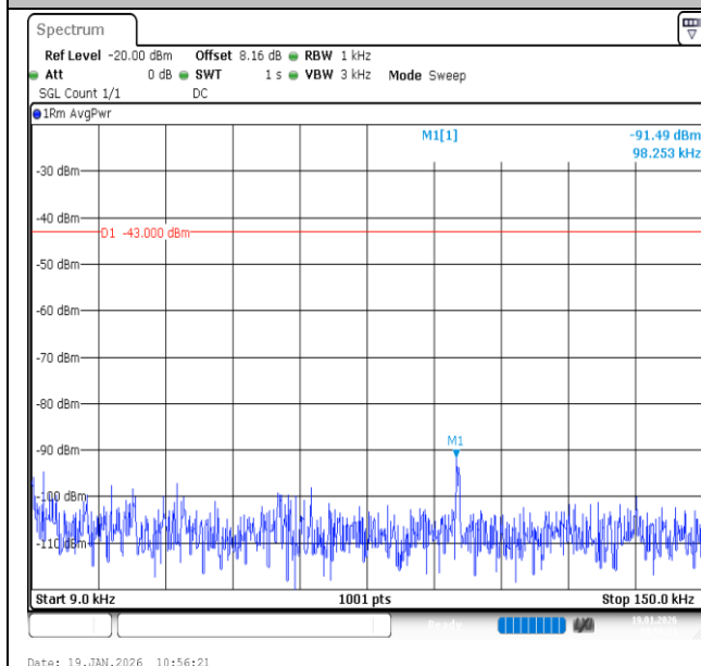
Band2-3MHz-QPSK-19185-15RB#0-0.009~0.15-PASS
