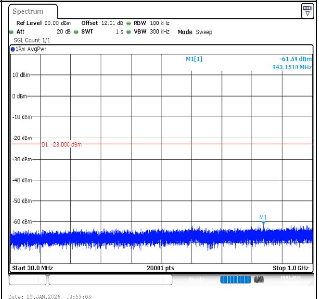
Band2-3MHz-16QAM-19185-1RB#0-30~1000-PASS
