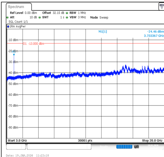
Band2-5MHz-16QAM-18900-1RB#0-3000~20000-PASS
