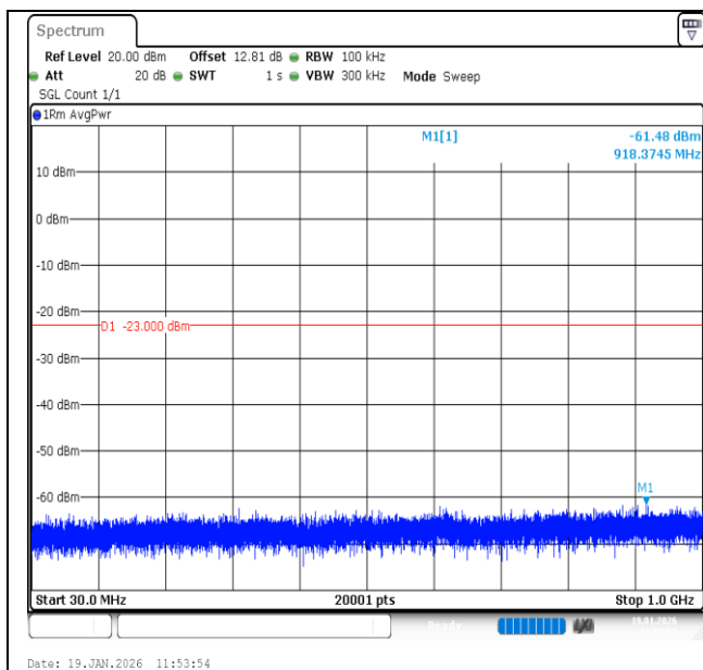
Band2-10MHz-QPSK-18900-1RB#49-30~1000-PASS
