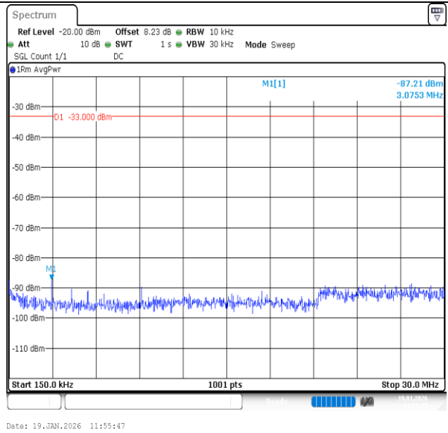
Band2-10MHz-QPSK-19150-1RB#0-0.15~30-PASS
