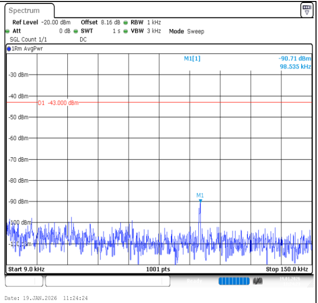
Band2-5MHz-QPSK-18900-25RB#0-0.009~0.15-PASS
