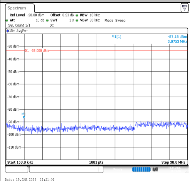
Band2-5MHz-16QAM-18625-1RB#24-0.15~30-PASS
