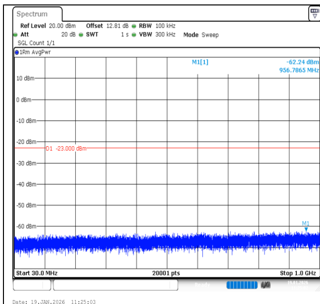
Band2-5MHz-16QAM-18900-25RB#0-30~1000-PASS
