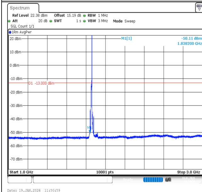
Band2-10MHz-QPSK-18650-1RB#49-1000~3000-PASS
