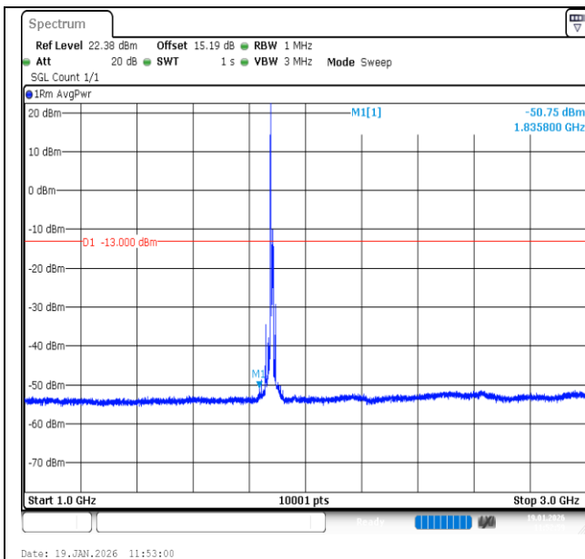
Band2-10MHz-QPSK-18900-1RB#0-1000~3000-PASS
