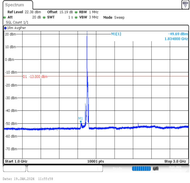
Band2-10MHz-QPSK-19150-1RB#0-1000~3000-PASS
