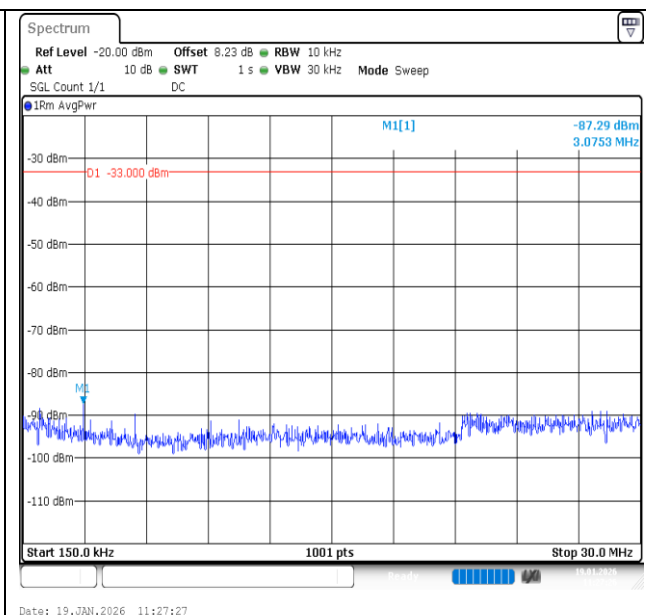
Band2-5MHz-QPSK-19175-25RB#0-0.15~30-PASS
