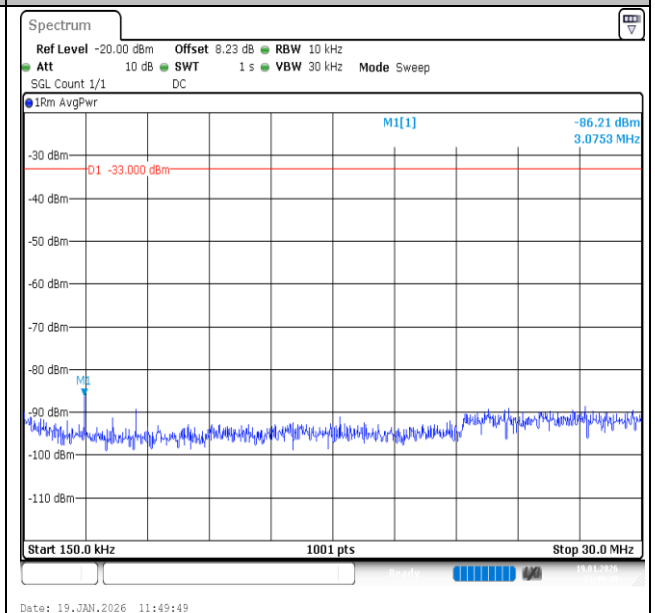
Band2-10MHz-QPSK-18650-1RB#0-0.15~30-PASS
