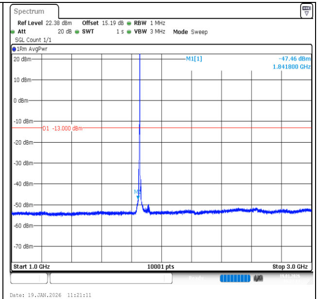
Band2-5MHz-16QAM-18625-1RB#24-1000~3000-PASS
