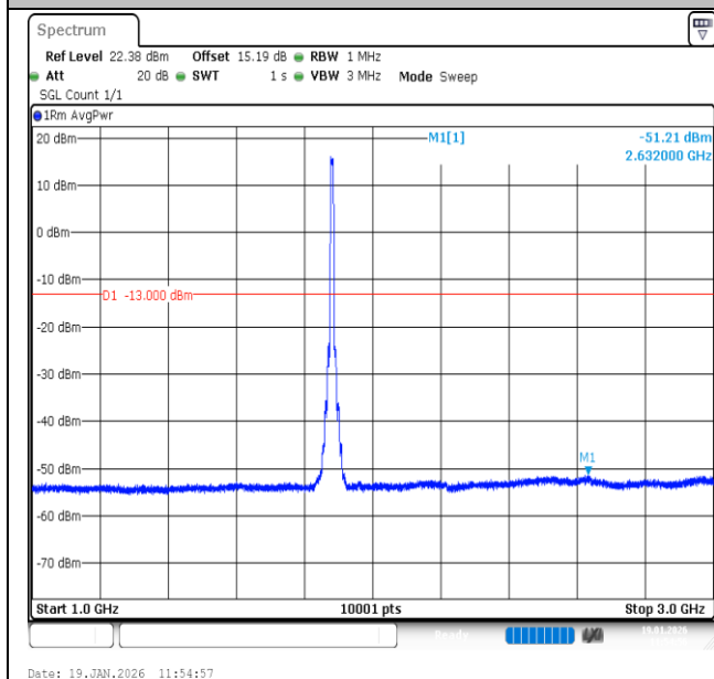
Band2-10MHz-QPSK-18900-50RB#0-1000~3000-PASS
