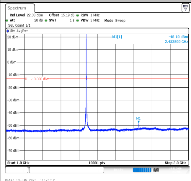
Band2-5MHz-16QAM-18900-1RB#0-1000~3000-PASS
