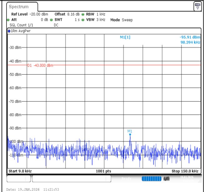
Band2-5MHz-16QAM-18625-25RB#0-0.009~0.15-PASS
