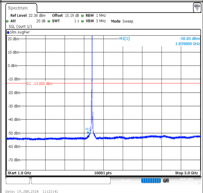
Band2-5MHz-QPSK-18900-1RB#24-1000~3000-PASS
