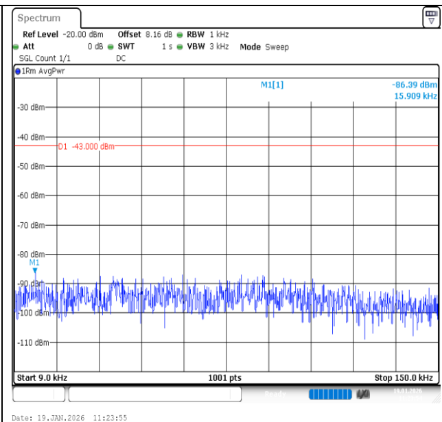
Band2-5MHz-16QAM-18900-1RB#24-0.009~0.15-PASS
