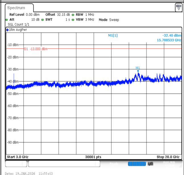
Band2-10MHz-QPSK-18900-50RB#0-3000~20000-PASS
