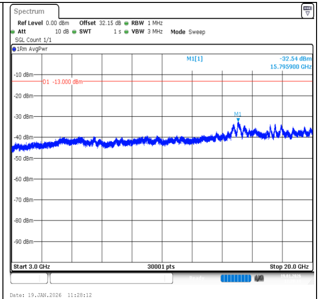
Band2-5MHz-16QAM-19175-25RB#0-3000~20000-PASS
