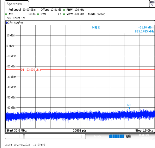
Band2-10MHz-QPSK-19150-1RB#0-30~1000-PASS
