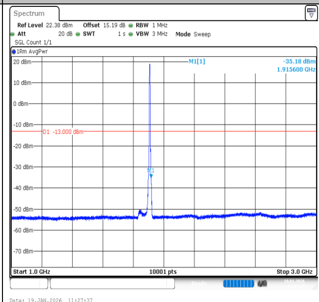
Band2-5MHz-QPSK-19175-25RB#0-1000~3000-PASS
