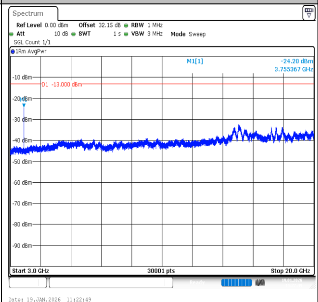
Band2-5MHz-QPSK-18900-1RB#0-3000~20000-PASS
