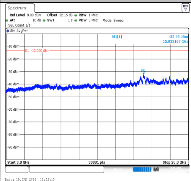
Band2-5MHz-16QAM-18625-25RB#0-3000~20000-PASS
