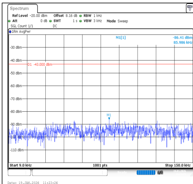
Band2-5MHz-QPSK-18900-1RB#24-0.009~0.15-PASS
