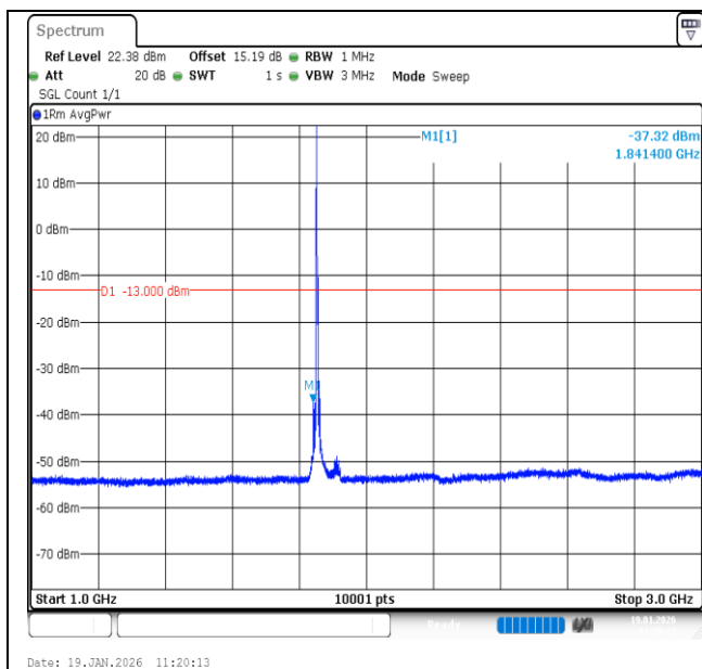
Band2-5MHz-16QAM-18625-1RB#0-1000~3000-PASS
