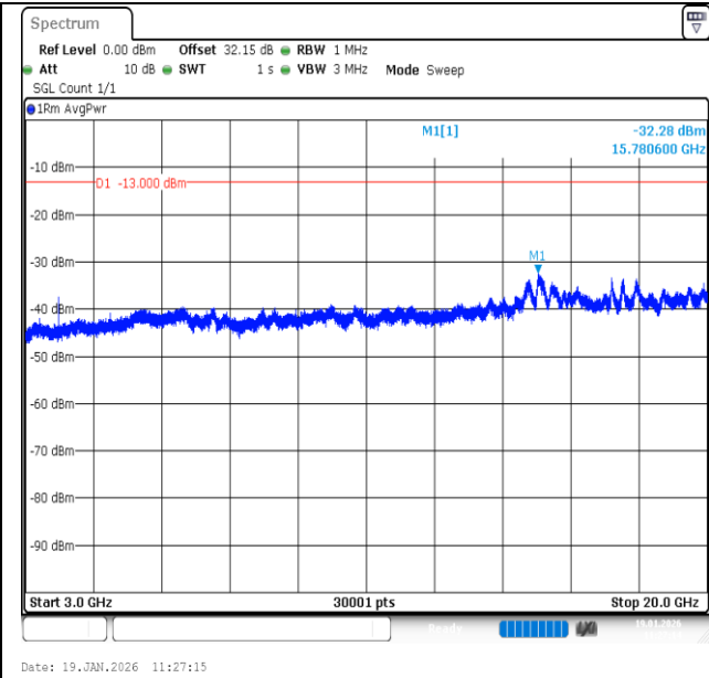
Band2-5MHz-16QAM-19175-1RB#24-3000~20000-PASS
