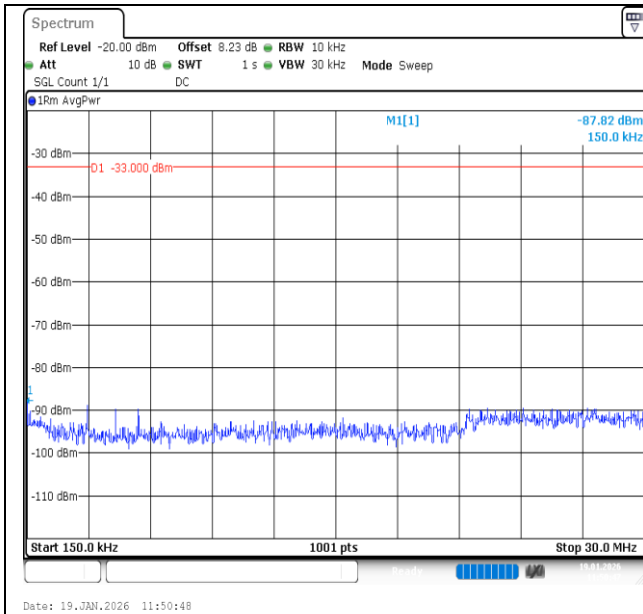
Band2-10MHz-QPSK-18650-1RB#49-0.15~30-PASS
