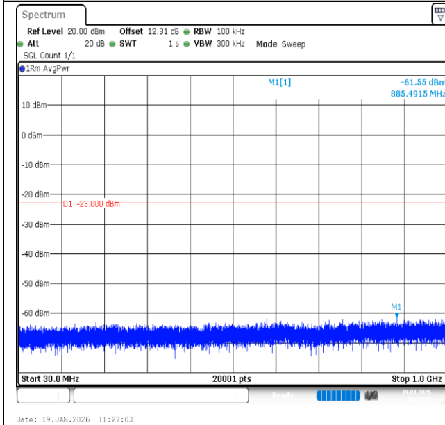
Band2-5MHz-16QAM-19175-1RB#24-30~1000-PASS
