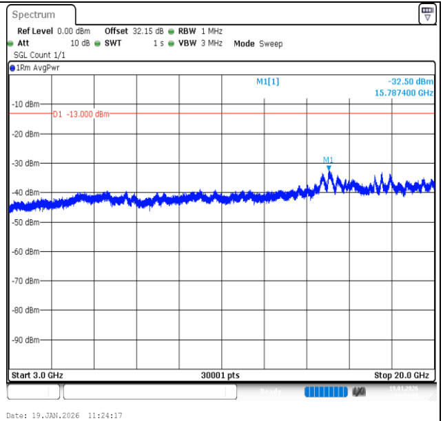
Band2-5MHz-16QAM-18900-1RB#24-3000~20000-PASS
