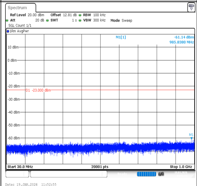
Band2-10MHz-QPSK-18900-1RB#0-30~1000-PASS
