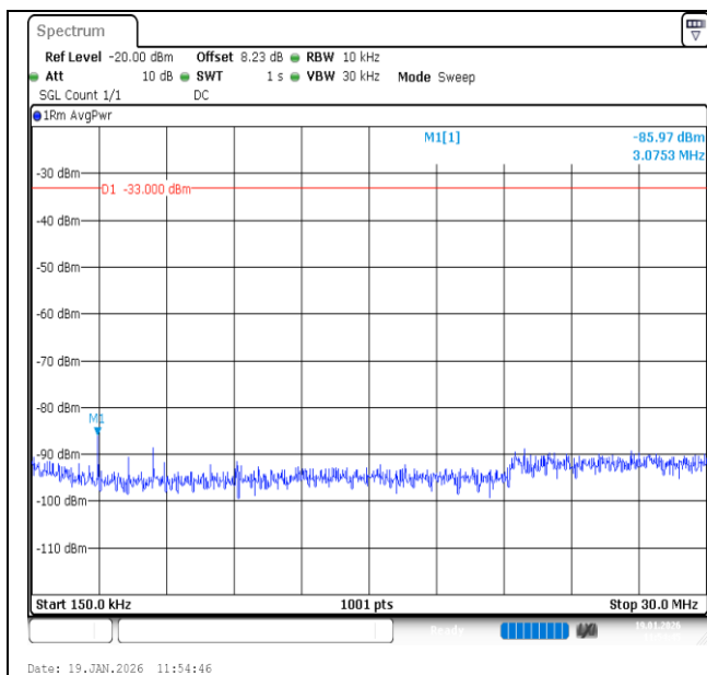
Band2-10MHz-QPSK-18900-50RB#0-0.15~30-PASS
