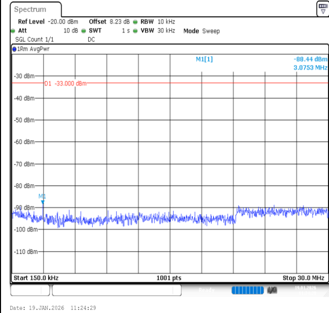
Band2-5MHz-QPSK-18900-25RB#0-0.15~30-PASS
