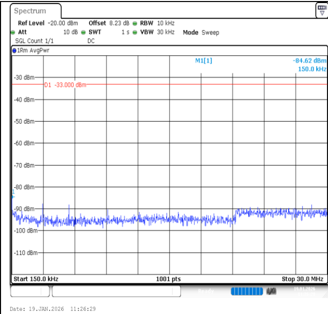
Band2-5MHz-QPSK-19175-1RB#24-0.15~30-PASS
