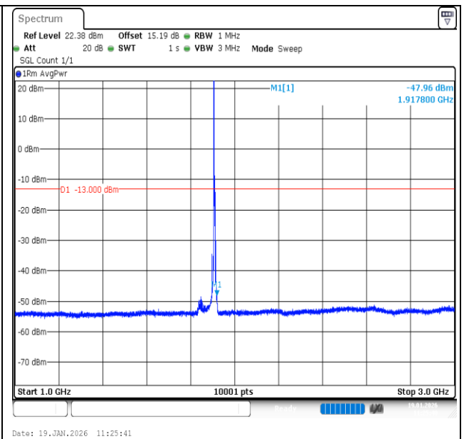
Band2-5MHz-QPSK-19175-1RB#0-1000~3000-PASS
