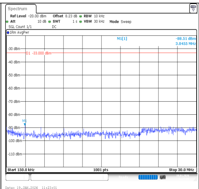
Band2-5MHz-16QAM-18900-1RB#0-0.15~30-PASS
