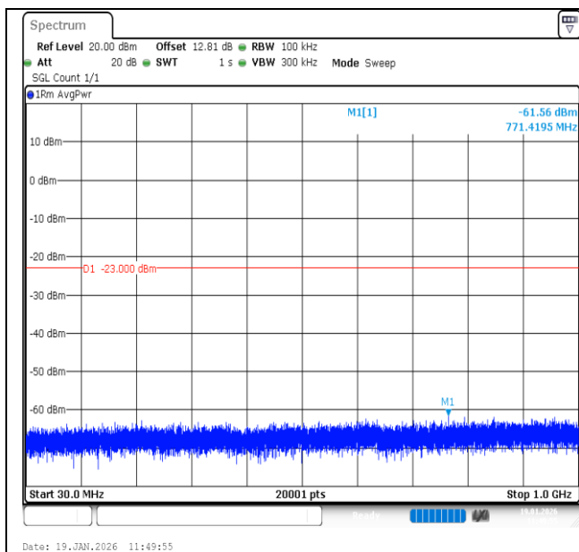
Band2-10MHz-QPSK-18650-1RB#0-30~1000-PASS
