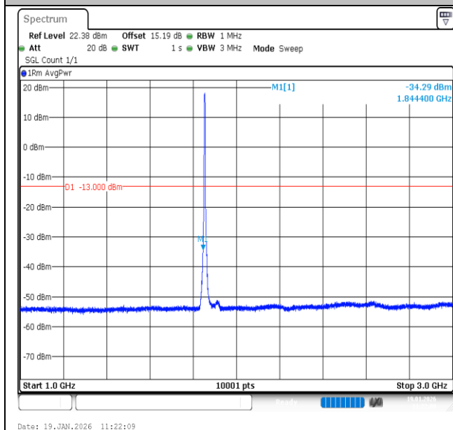
Band2-5MHz-16QAM-18625-25RB#0-1000~3000-PASS
