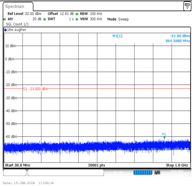
Band2-5MHz-QPSK-19175-1RB#24-30~1000-PASS
