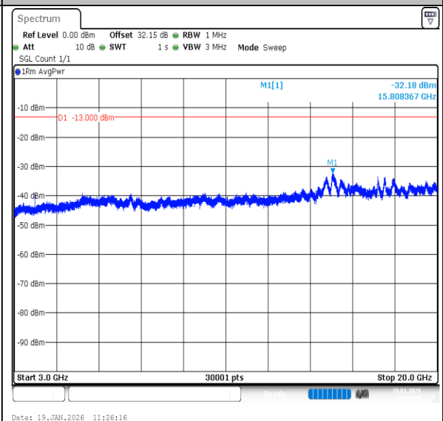
Band2-5MHz-16QAM-19175-1RB#0-3000~20000-PASS
