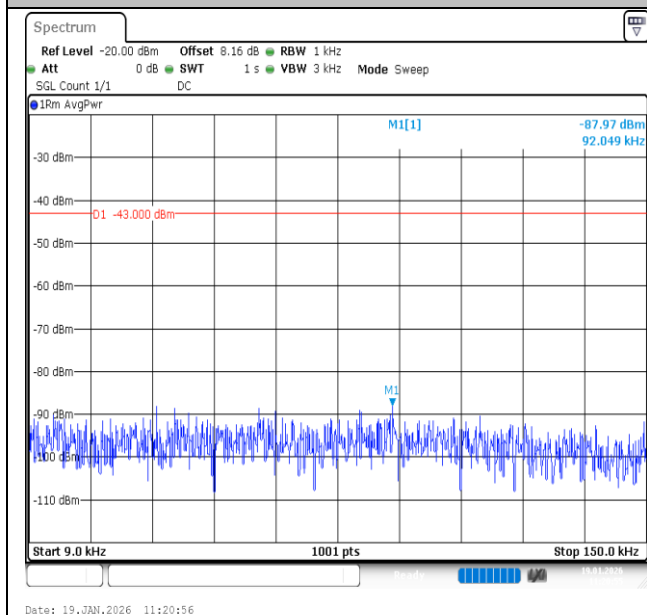
Band2-5MHz-16QAM-18625-1RB#24-0.009~0.15-PASS
