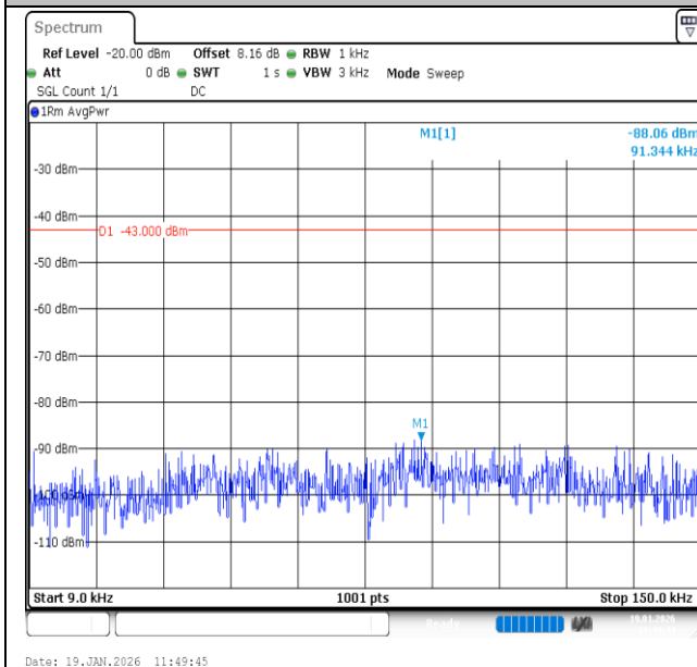
Band2-10MHz-QPSK-18650-1RB#0-0.009~0.15-PASS
