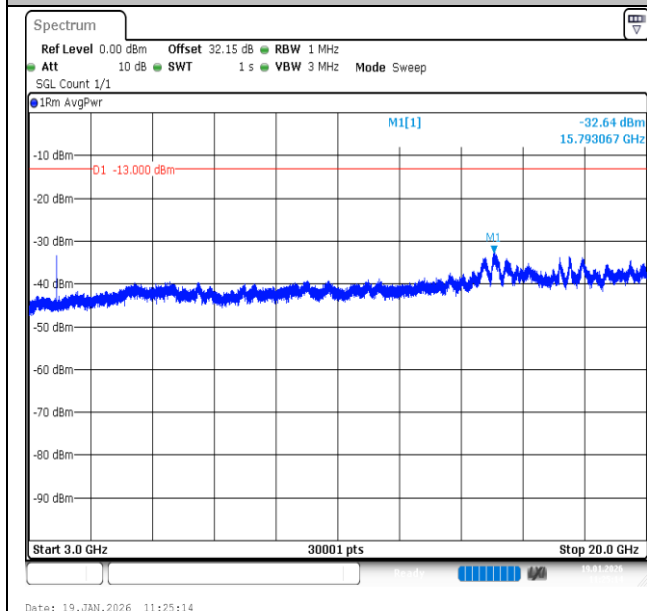
Band2-5MHz-16QAM-18900-25RB#0-3000~20000-PASS
