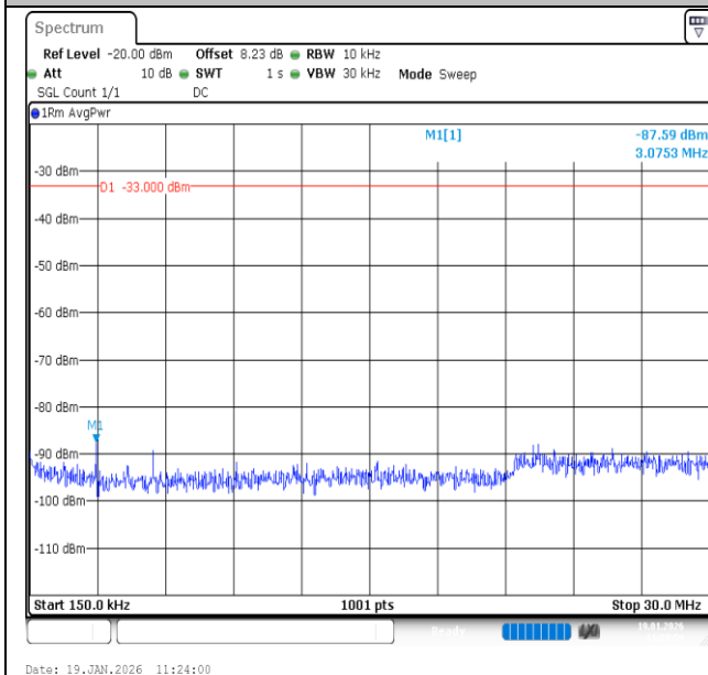
Band2-5MHz-16QAM-18900-1RB#24-0.15~30-PASS
