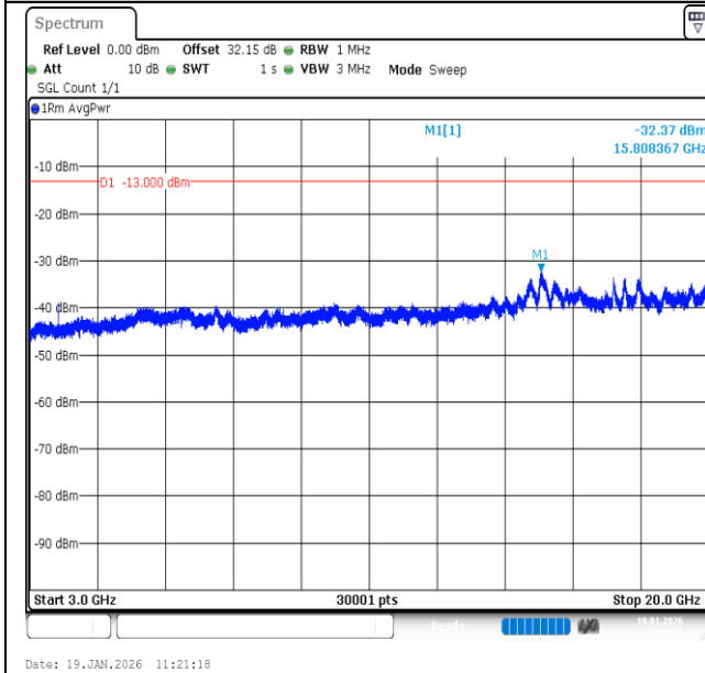
Band2-5MHz-16QAM-18625-1RB#24-3000~20000-PASS
