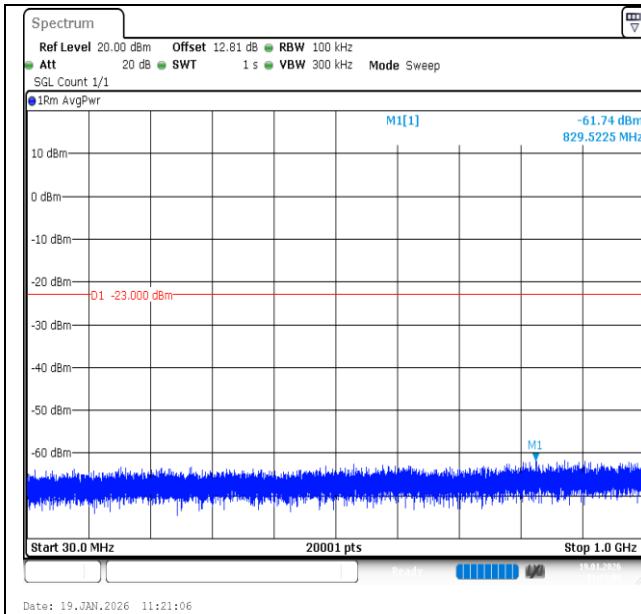
Band2-5MHz-16QAM-18625-1RB#24-30~1000-PASS
