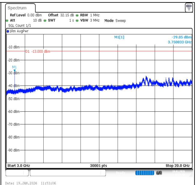
Band2-10MHz-QPSK-18900-1RB#0-3000~20000-PASS
