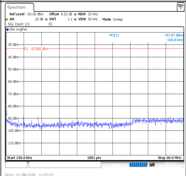
Band2-5MHz-QPSK-19175-1RB#0-0.15~30-PASS
