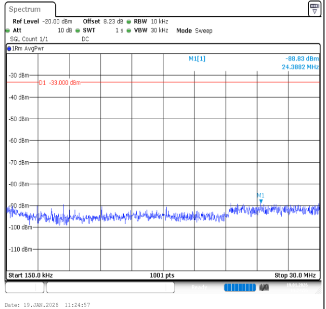
Band2-5MHz-16QAM-18900-25RB#0-0.15~30-PASS
