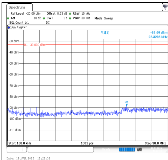
Band2-5MHz-QPSK-18900-1RB#0-0.15~30-PASS
