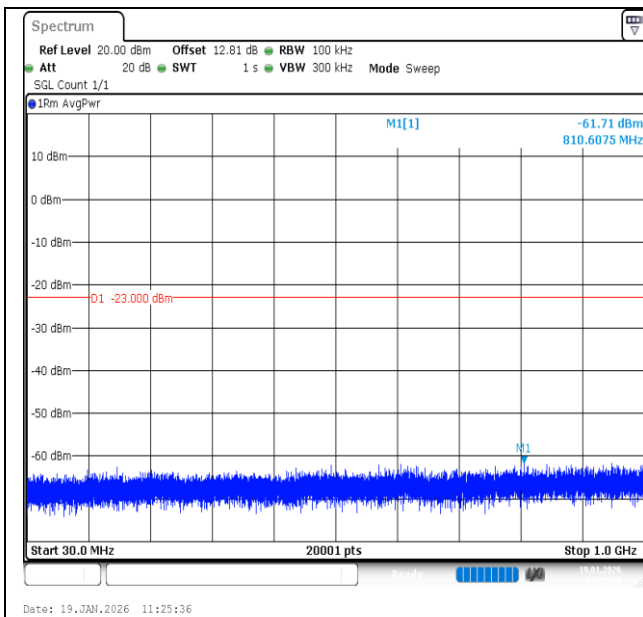
Band2-5MHz-QPSK-19175-1RB#0-30~1000-PASS
