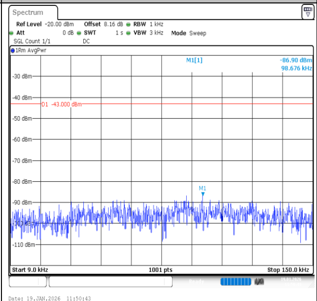
Band2-10MHz-QPSK-18650-1RB#49-0.009~0.15-PASS
