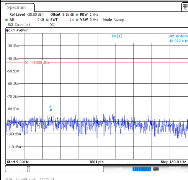
Band2-5MHz-16QAM-19175-1RB#0-0.009~0.15-PASS
