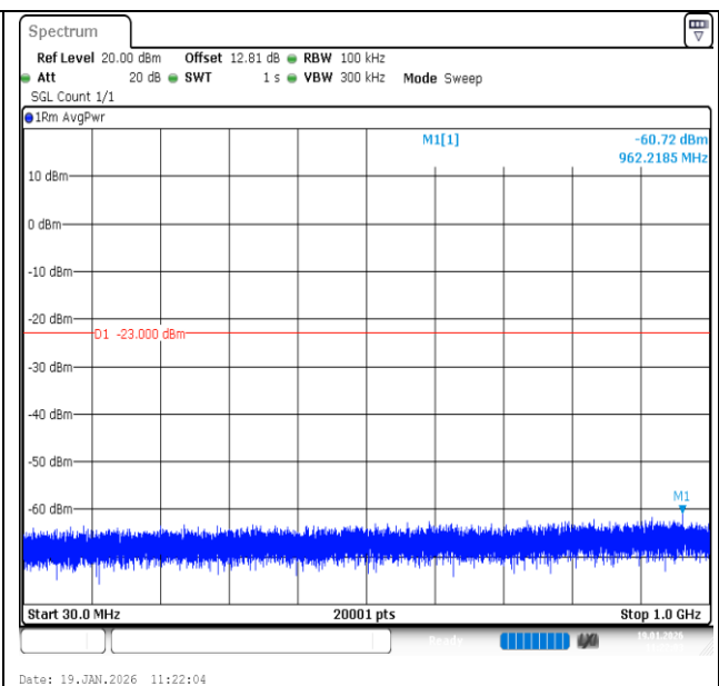
Band2-5MHz-16QAM-18625-25RB#0-30~1000-PASS
