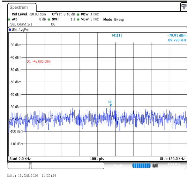
Band2-5MHz-QPSK-19175-1RB#0-0.009~0.15-PASS
