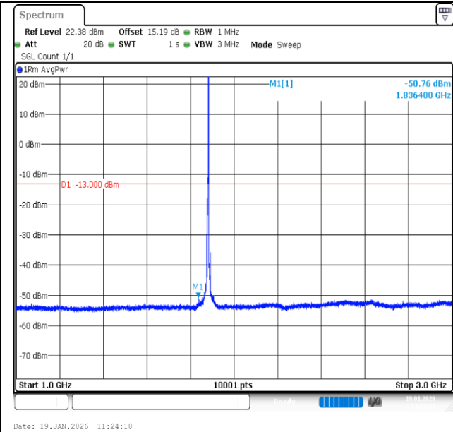
Band2-5MHz-16QAM-18900-1RB#24-1000~3000-PASS
