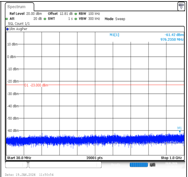
Band2-10MHz-QPSK-18650-1RB#49-30~1000-PASS
