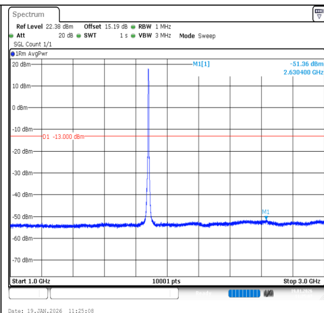
Band2-5MHz-16QAM-18900-25RB#0-1000~3000-PASS
