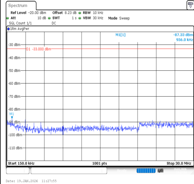
Band2-5MHz-16QAM-19175-25RB#0-0.15~30-PASS
