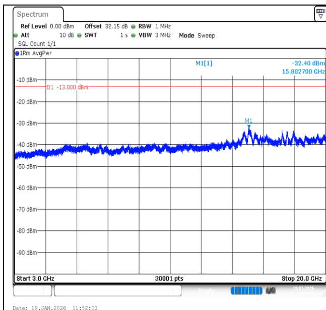
Band2-10MHz-QPSK-18650-50RB#0-3000~20000-PASS
