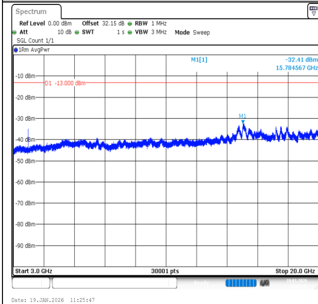
Band2-5MHz-QPSK-19175-1RB#0-3000~20000-PASS
