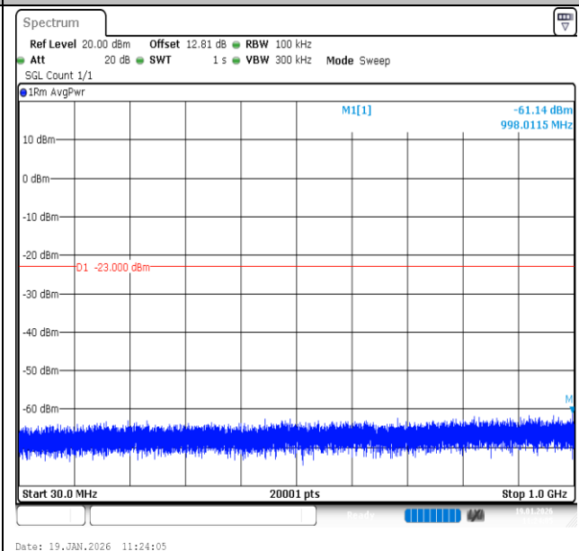
Band2-5MHz-16QAM-18900-1RB#24-30~1000-PASS
