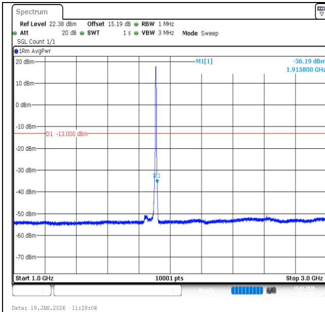
Band2-5MHz-16QAM-19175-25RB#0-1000~3000-PASS
