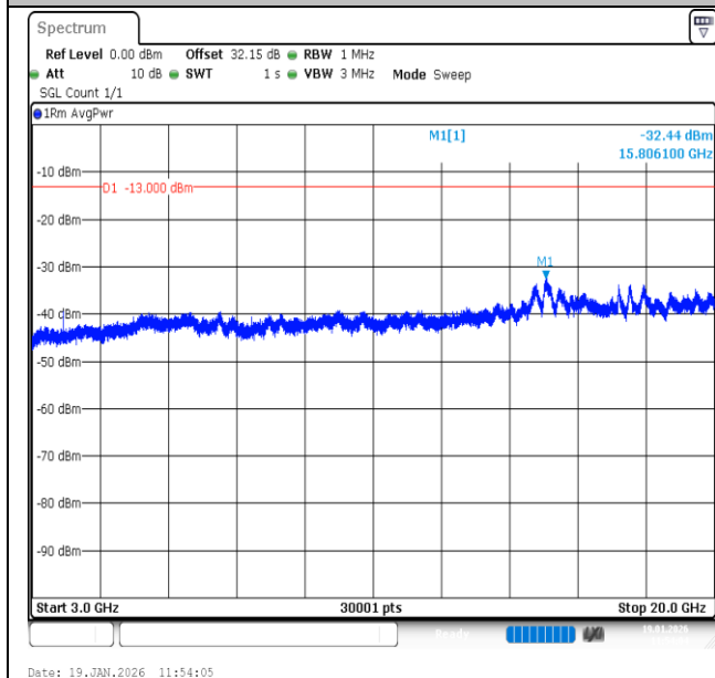
Band2-10MHz-QPSK-18900-1RB#49-3000~20000-PASS
