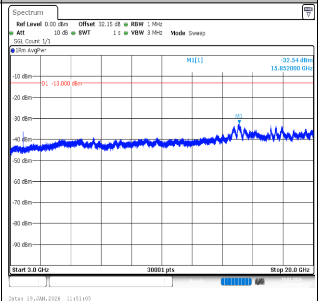
Band2-10MHz-QPSK-18650-1RB#49-3000~20000-PASS
