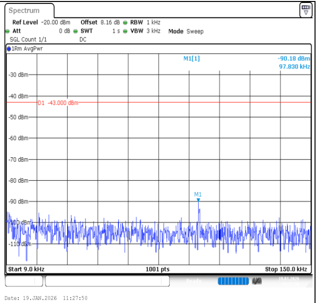
Band2-5MHz-16QAM-19175-25RB#0-0.009~0.15-PASS
