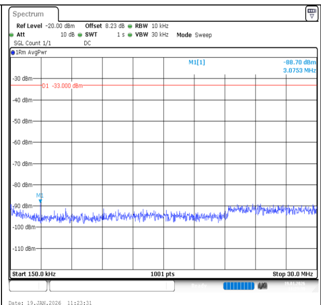
Band2-5MHz-QPSK-18900-1RB#24-0.15~30-PASS
