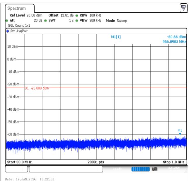
Band2-5MHz-QPSK-18900-1RB#0-30~1000-PASS
