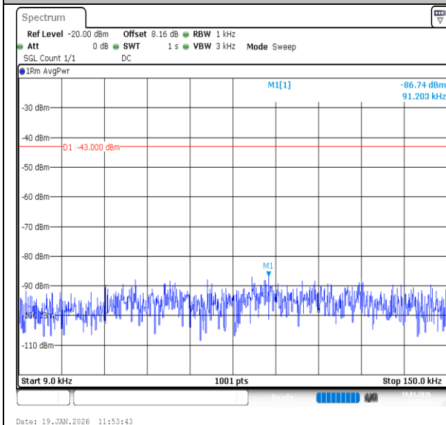
Band2-10MHz-QPSK-18900-1RB#49-0.009~0.15-PASS
