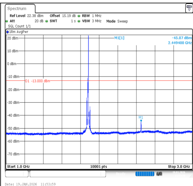
Band2-10MHz-QPSK-18900-1RB#49-1000~3000-PASS
