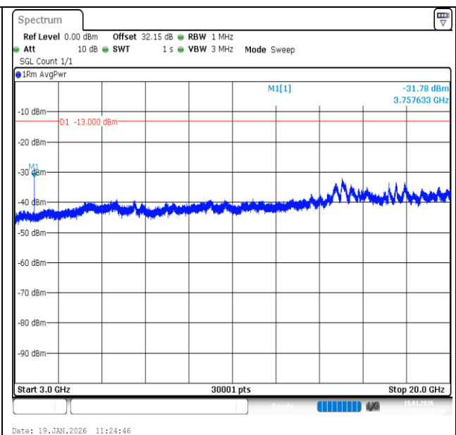
Band2-5MHz-QPSK-18900-25RB#0-3000~20000-PASS
