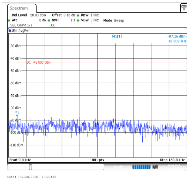
Band2-5MHz-16QAM-18900-1RB#0-0.009~0.15-PASS
