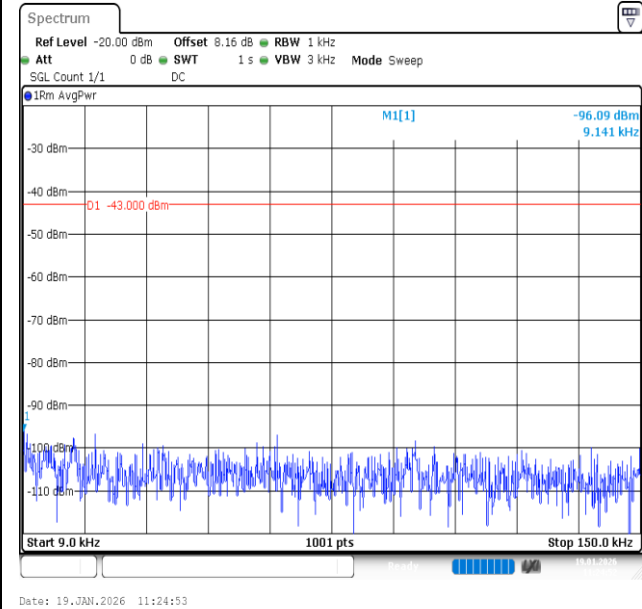
Band2-5MHz-16QAM-18900-25RB#0-0.009~0.15-PASS
