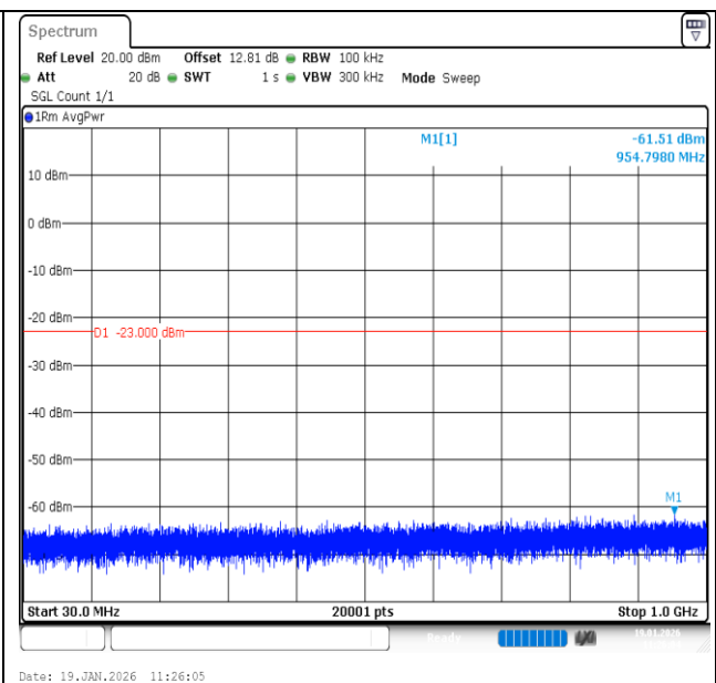
Band2-5MHz-16QAM-19175-1RB#0-30~1000-PASS
