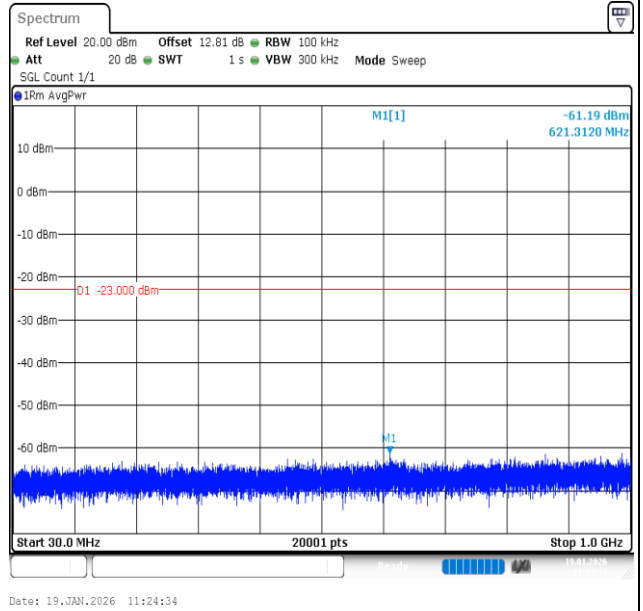
Band2-5MHz-QPSK-18900-25RB#0-30~1000-PASS
