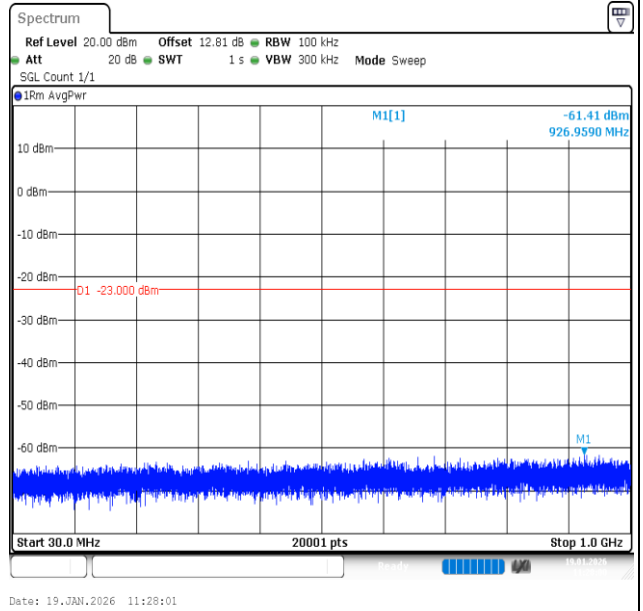
Band2-5MHz-16QAM-19175-25RB#0-30~1000-PASS
