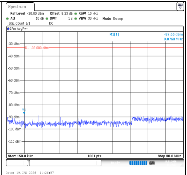
Band2-5MHz-16QAM-19175-1RB#24-0.15~30-PASS
