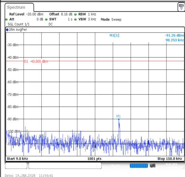
Band2-10MHz-QPSK-18900-50RB#0-0.009~0.15-PASS
