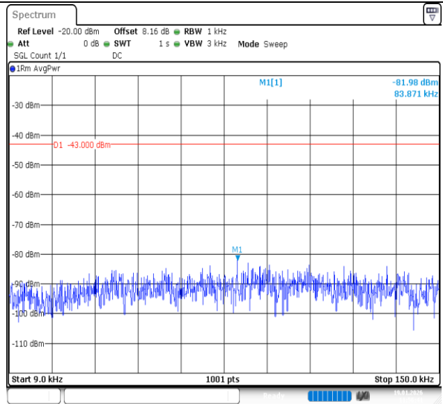
Band2-10MHz-QPSK-19150-1RB#49-0.009~0.15-PASS
