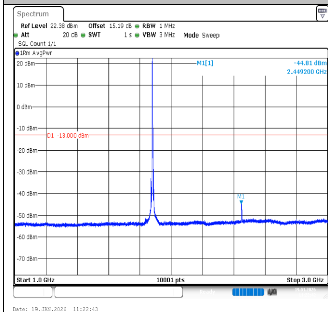
Band2-5MHz-QPSK-18900-1RB#0-1000~3000-PASS
