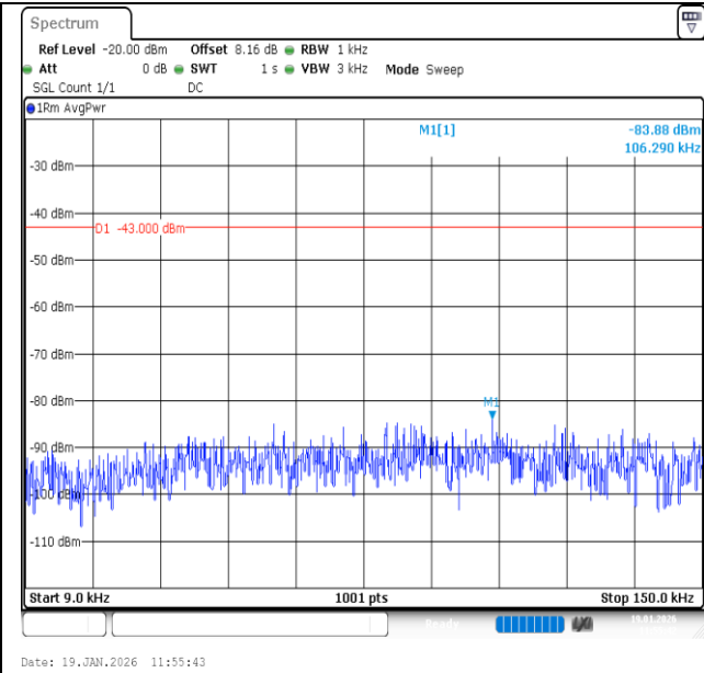
Band2-10MHz-QPSK-19150-1RB#0-0.009~0.15-PASS
