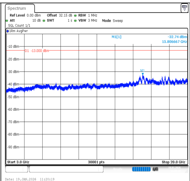
Band2-5MHz-16QAM-18625-1RB#0-3000~20000-PASS
