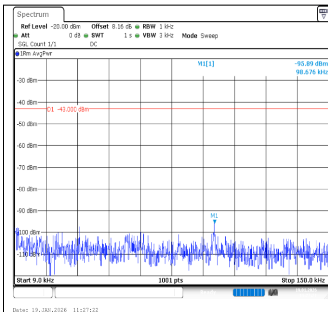
Band2-5MHz-QPSK-19175-25RB#0-0.009~0.15-PASS
