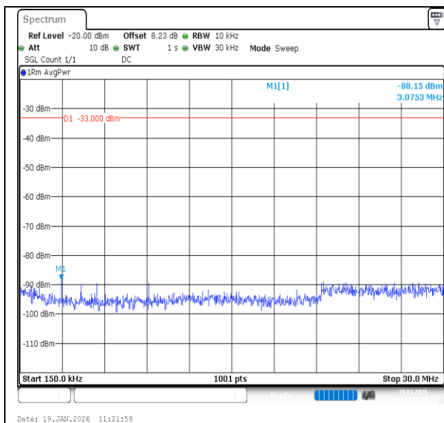
Band2-5MHz-16QAM-18625-25RB#0-0.15~30-PASS
