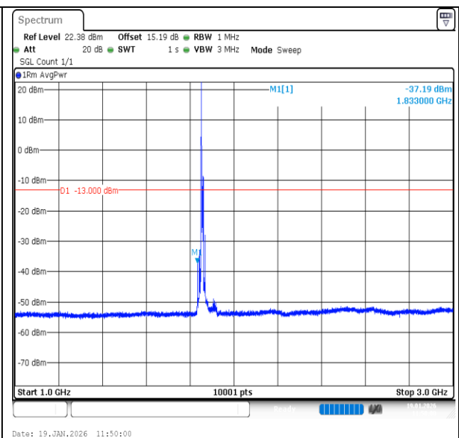
Band2-10MHz-QPSK-18650-1RB#0-1000~3000-PASS
