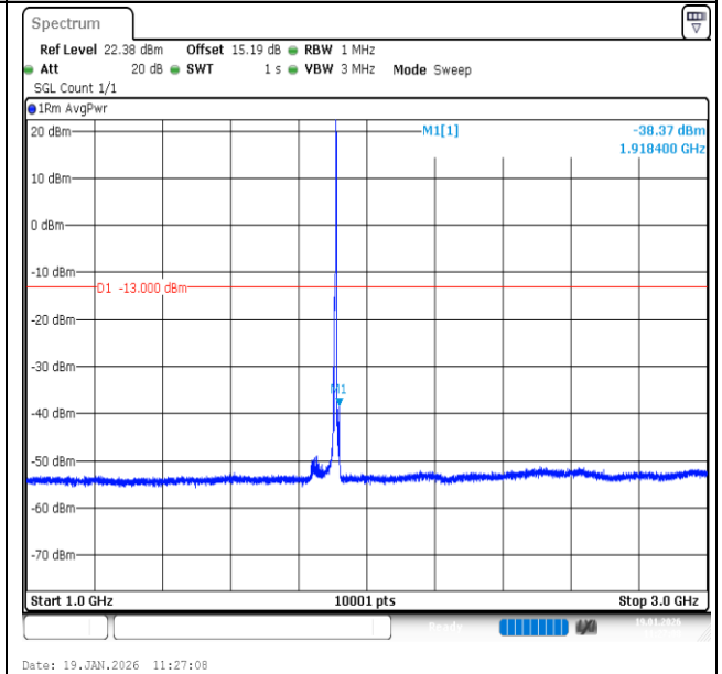
Band2-5MHz-16QAM-19175-1RB#24-1000~3000-PASS
