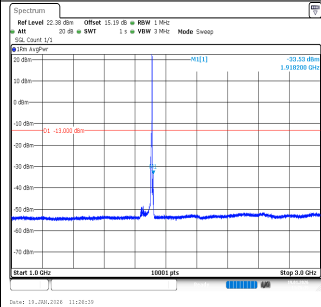
Band2-5MHz-QPSK-19175-1RB#24-1000~3000-PASS
