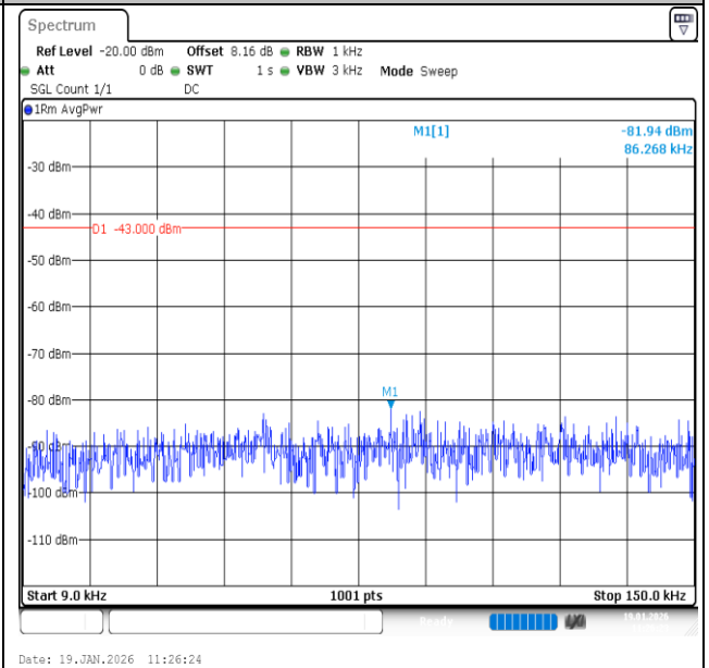
Band2-5MHz-QPSK-19175-1RB#24-0.009~0.15-PASS
