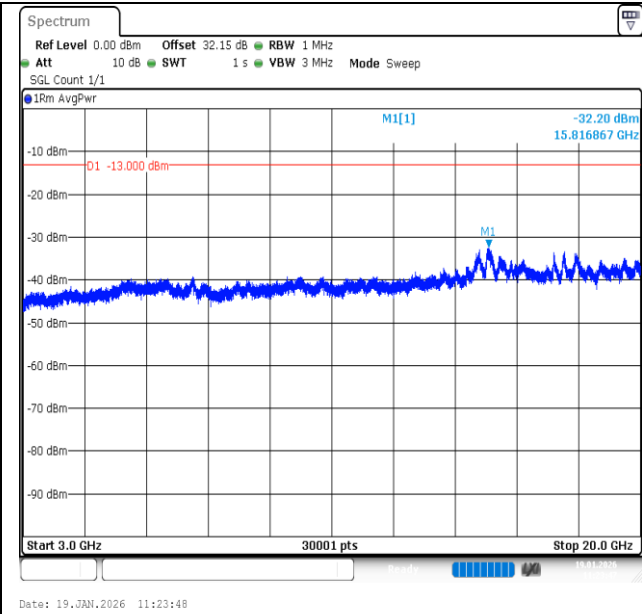
Band2-5MHz-QPSK-18900-1RB#24-3000~20000-PASS
