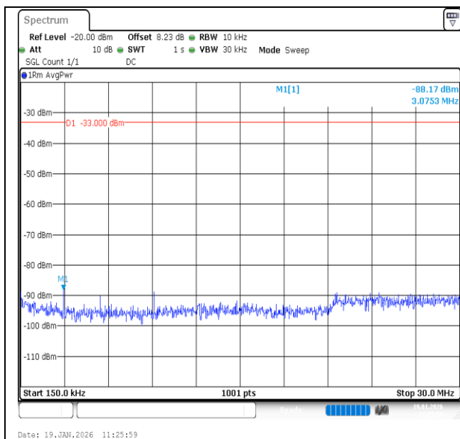
Band2-5MHz-16QAM-19175-1RB#0-0.15~30-PASS
