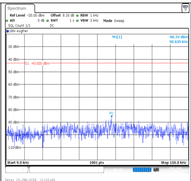
Band2-10MHz-QPSK-18900-1RB#0-0.009~0.15-PASS
