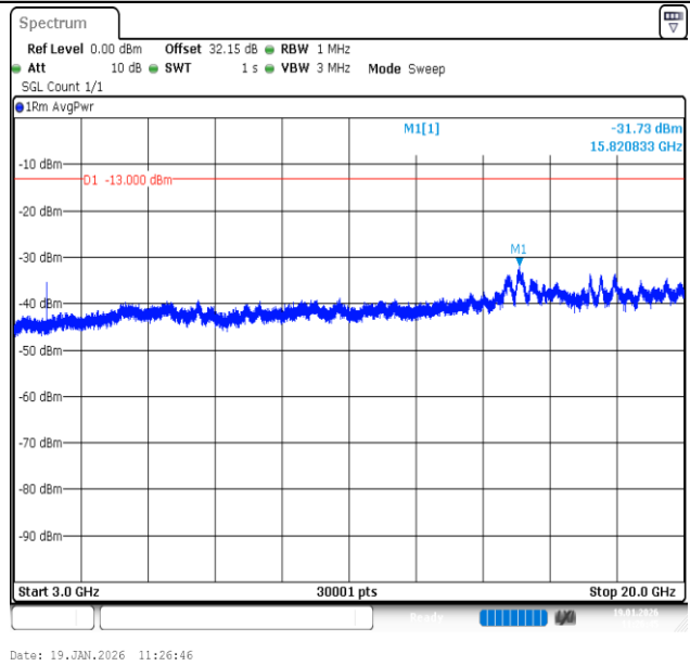
Band2-5MHz-QPSK-19175-1RB#24-3000~20000-PASS
