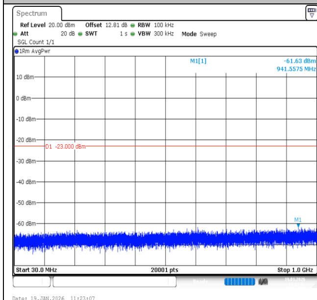
Band2-5MHz-16QAM-18900-1RB#0-30~1000-PASS
