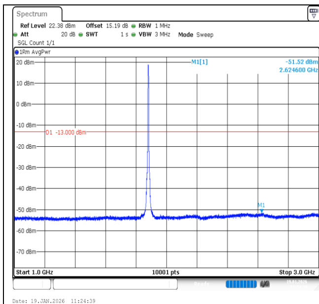
Band2-5MHz-QPSK-18900-25RB#0-1000~3000-PASS
