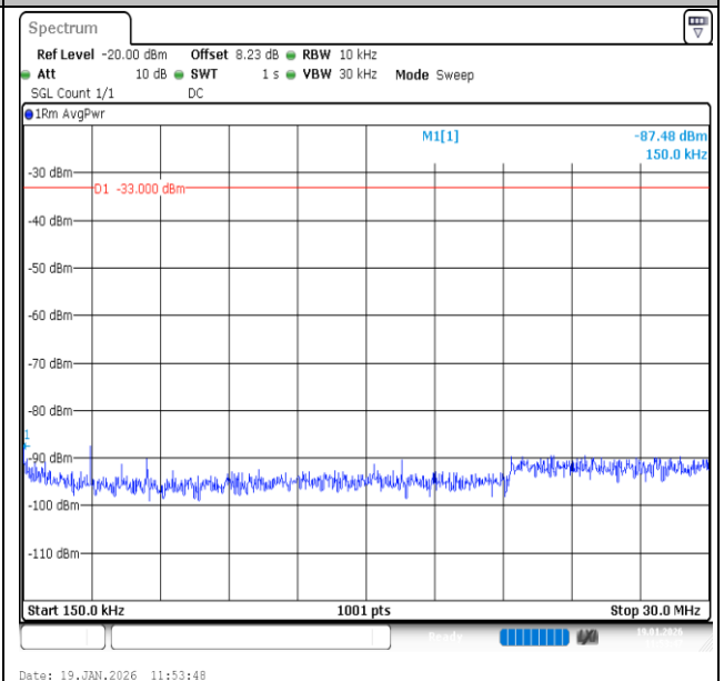
Band2-10MHz-QPSK-18900-1RB#49-0.15~30-PASS
