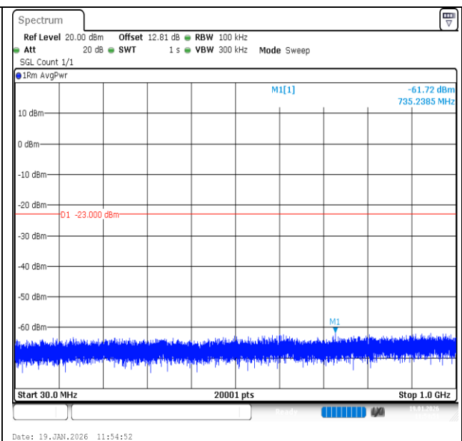
Band2-10MHz-QPSK-18900-50RB#0-30~1000-PASS
