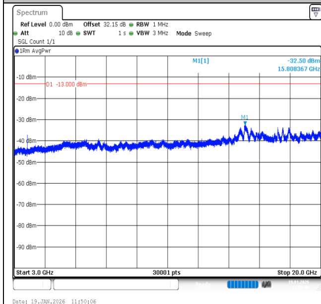
Band2-10MHz-QPSK-18650-1RB#0-3000~20000-PASS
