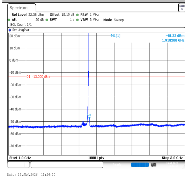
Band2-5MHz-16QAM-19175-1RB#0-1000~3000-PASS
