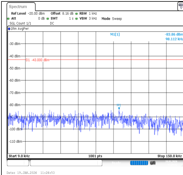
Band2-5MHz-16QAM-19175-1RB#24-0.009~0.15-PASS
