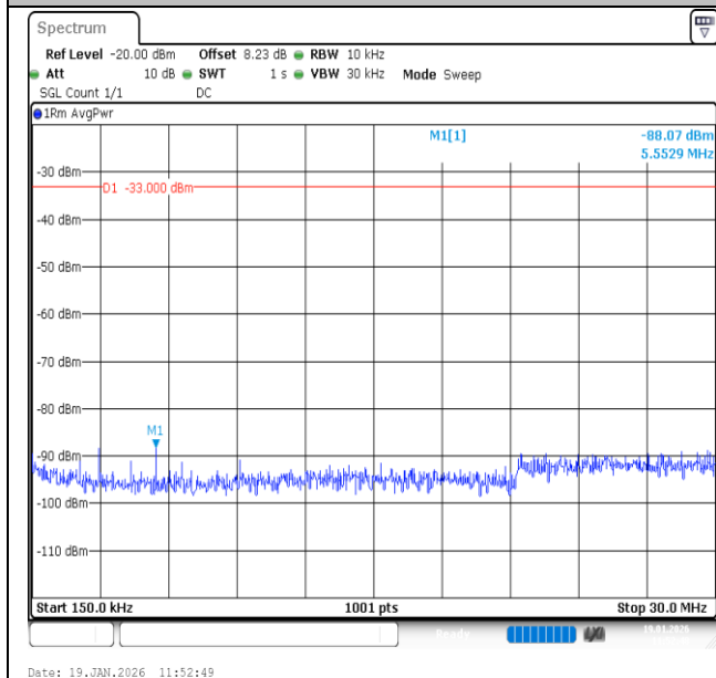
Band2-10MHz-QPSK-18900-1RB#0-0.15~30-PASS
