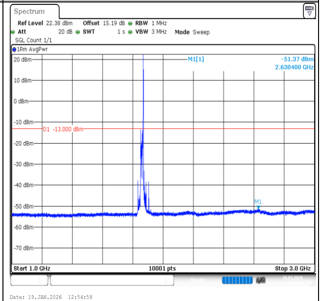
Band2-20MHz-16QAM-18700-1RB#99-1000~3000-PASS
