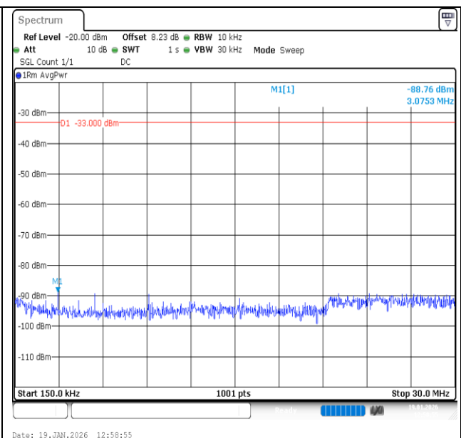
Band2-20MHz-16QAM-18900-100RB#0-0.15~30-PASS
