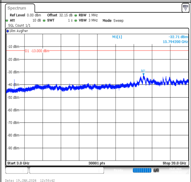
Band2-20MHz-QPSK-18900-100RB#0-3000~20000-PASS
