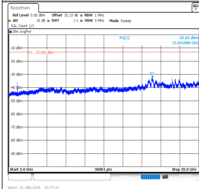
Band2-20MHz-16QAM-18900-1RB#0-3000~20000-PASS
