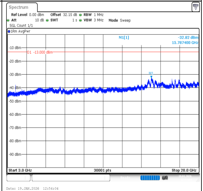
Band2-20MHz-16QAM-18700-1RB#0-3000~20000-PASS
