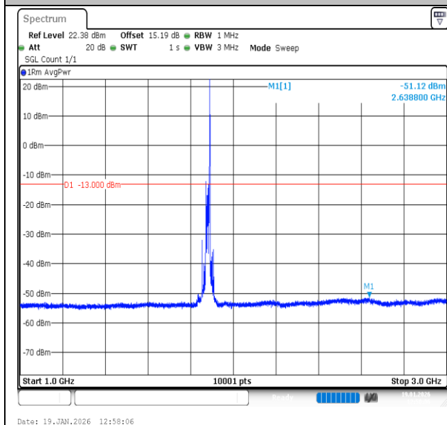
Band2-20MHz-16QAM-18900-1RB#99-1000~3000-PASS
