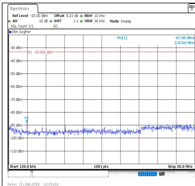
Band2-20MHz-QPSK-18900-100RB#0-0.15~30-PASS
