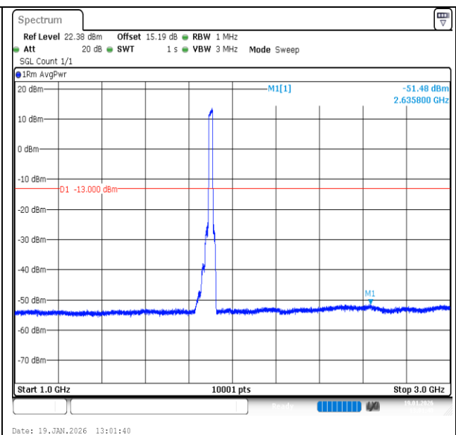
Band2-20MHz-QPSK-19100-100RB#0-1000~3000-PASS
