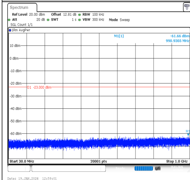
Band2-20MHz-16QAM-18900-100RB#0-30~1000-PASS
