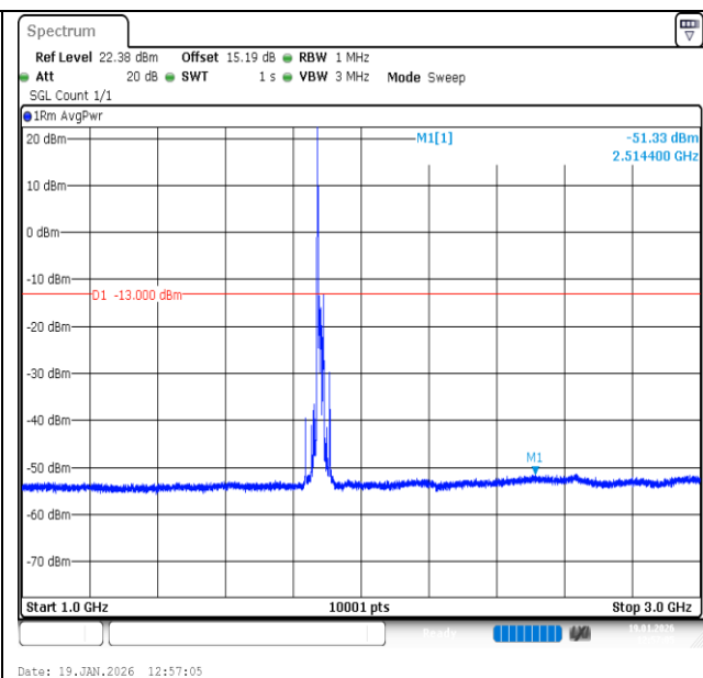
Band2-20MHz-16QAM-18900-1RB#0-1000~3000-PASS
