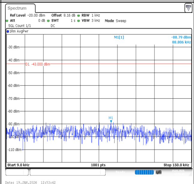
Band2-20MHz-16QAM-18700-1RB#0-0.009~0.15-PASS
