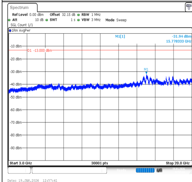
Band2-20MHz-QPSK-18900-1RB#99-3000~20000-PASS
