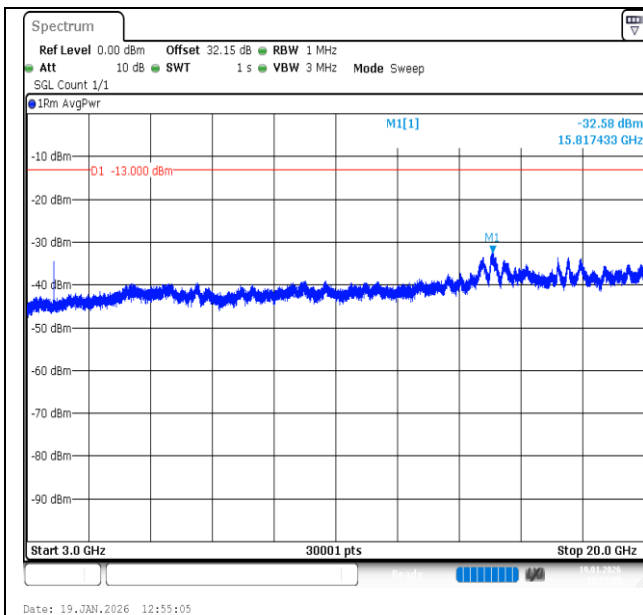
Band2-20MHz-16QAM-18700-1RB#99-3000~20000-PASS
