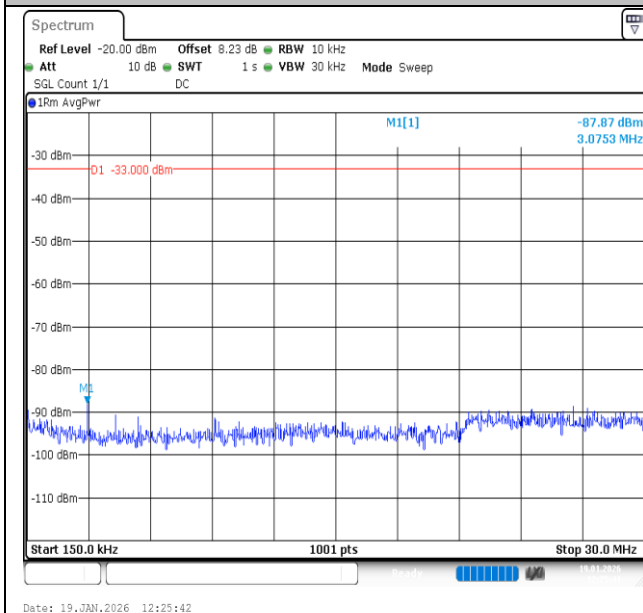
Band2-15MHz-16QAM-18900-1RB#74-0.15~30-PASS
