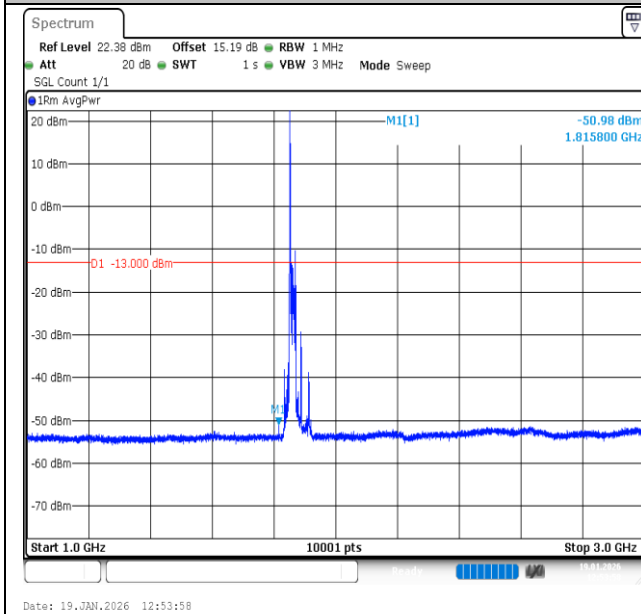
Band2-20MHz-16QAM-18700-1RB#0-1000~3000-PASS
