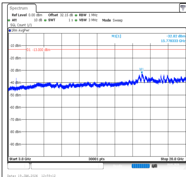
Band2-20MHz-16QAM-18900-100RB#0-3000~20000-PASS
