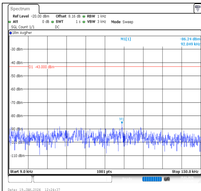
Band2-15MHz-16QAM-18900-1RB#0-0.009~0.15-PASS
