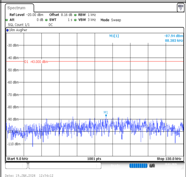
Band2-20MHz-QPSK-18700-1RB#99-0.009~0.15-PASS
