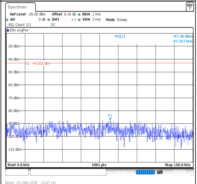
Band2-15MHz-16QAM-19125-1RB#0-0.009~0.15-PASS
