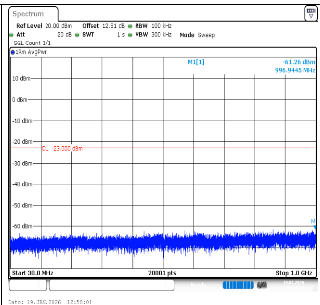
Band2-20MHz-16QAM-18900-1RB#99-30~1000-PASS
