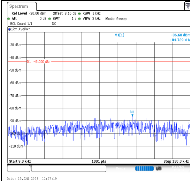
Band2-20MHz-QPSK-18900-1RB#99-0.009~0.15-PASS
