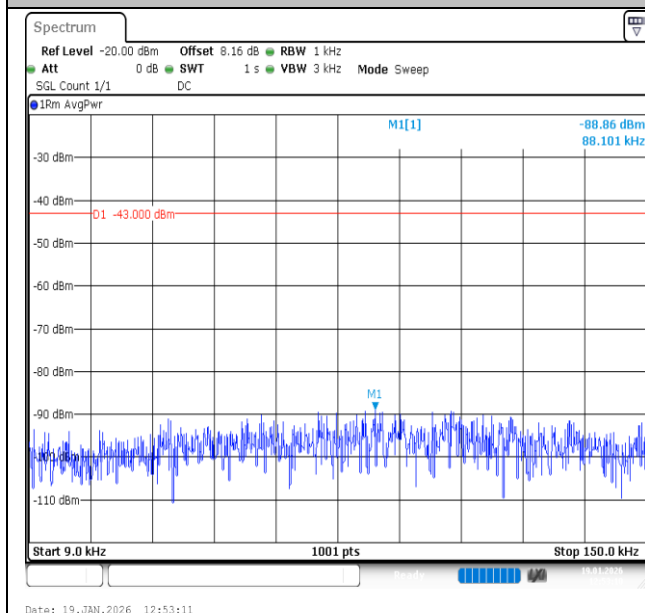
Band2-20MHz-QPSK-18700-1RB#0-0.009~0.15-PASS
