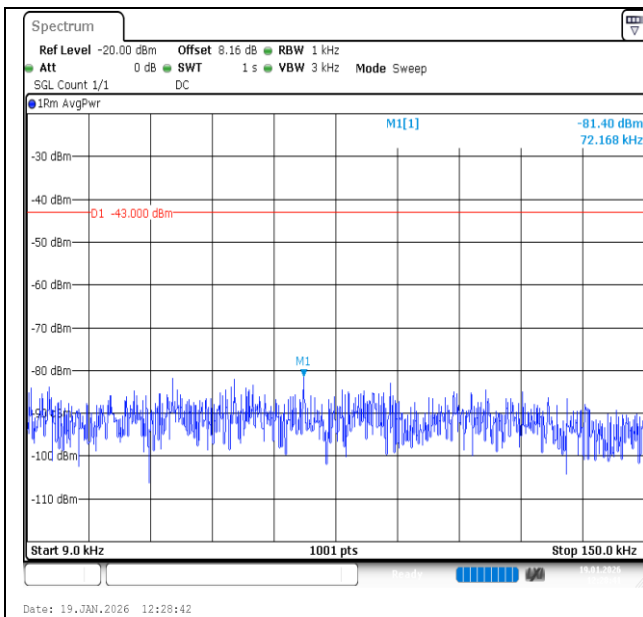
Band2-15MHz-16QAM-19125-1RB#74-0.009~0.15-PASS
