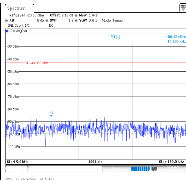
Band2-20MHz-16QAM-19100-1RB#0-0.009~0.15-PASS
