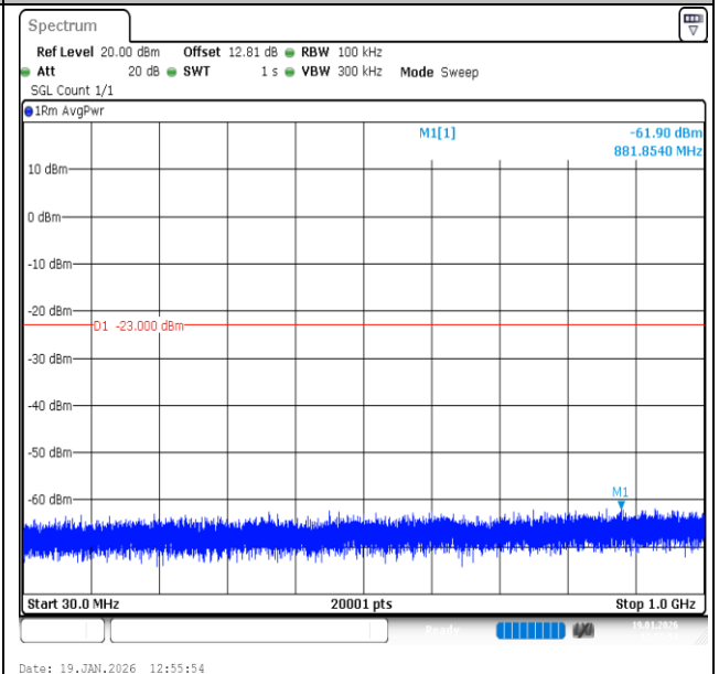
Band2-20MHz-16QAM-18700-100RB#0-30~1000-PASS
