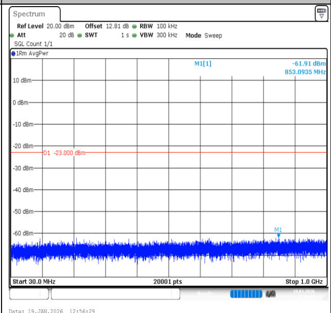
Band2-20MHz-QPSK-18900-1RB#0-30~1000-PASS
