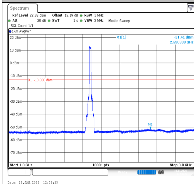
Band2-20MHz-QPSK-18900-100RB#0-1000~3000-PASS
