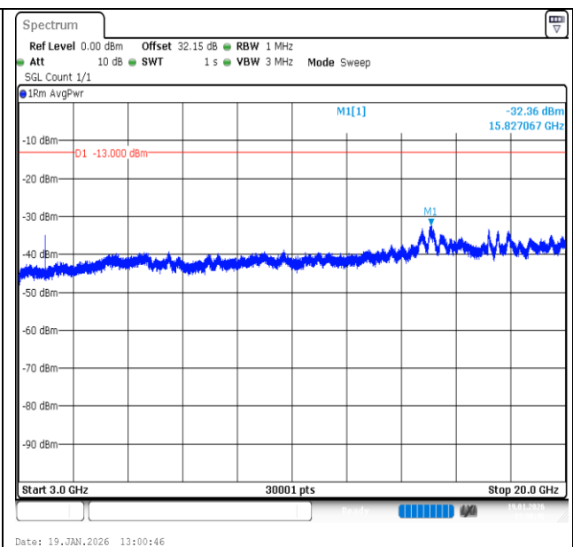
Band2-20MHz-QPSK-19100-1RB#99-3000~20000-PASS
