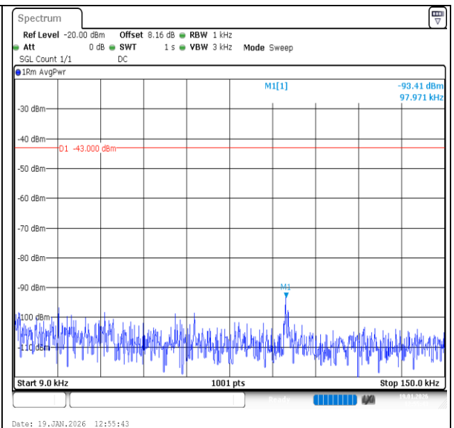
Band2-20MHz-16QAM-18700-100RB#0-0.009~0.15-PASS
