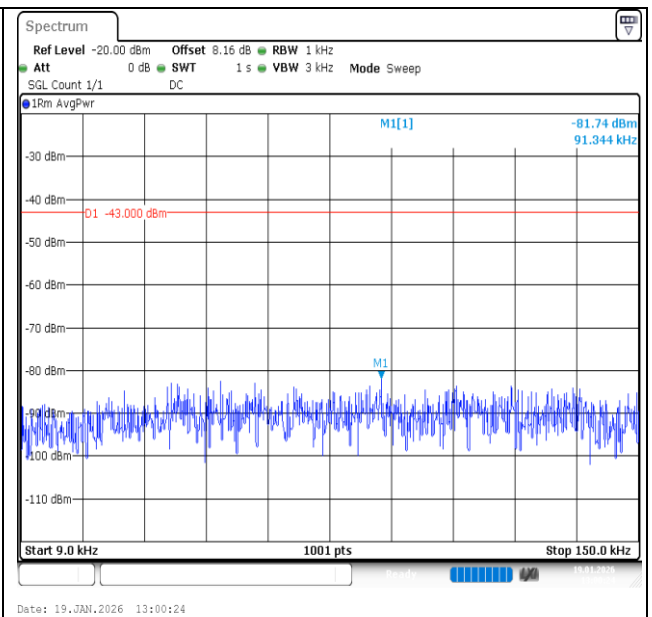
Band2-20MHz-QPSK-19100-1RB#99-0.009~0.15-PASS
