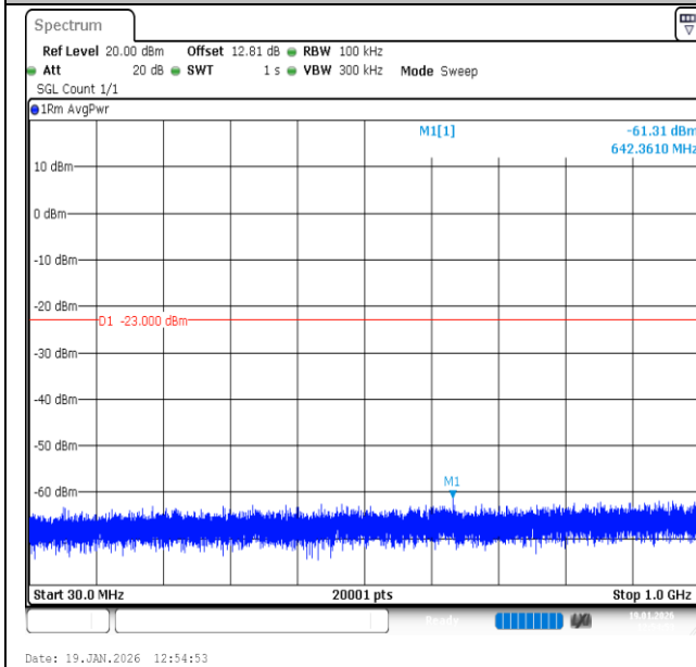
Band2-20MHz-16QAM-18700-1RB#99-30~1000-PASS
