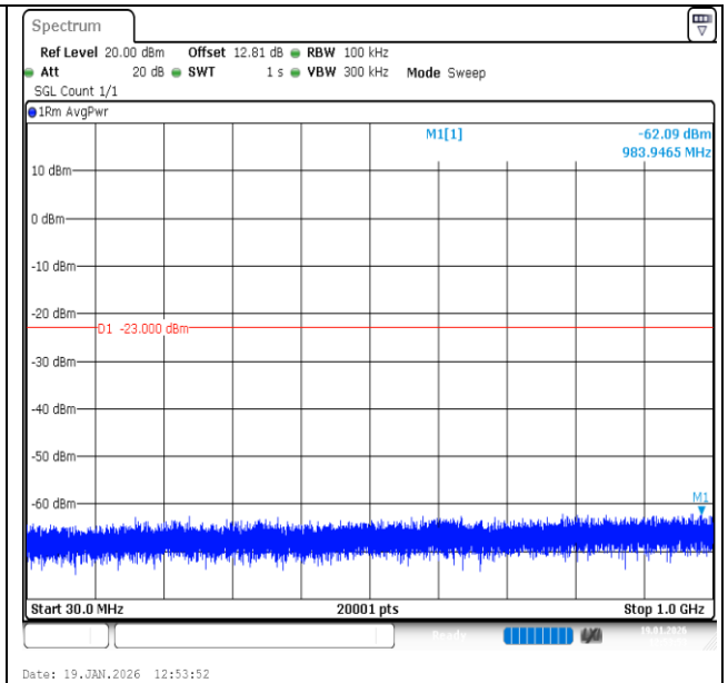
Band2-20MHz-16QAM-18700-1RB#0-30~1000-PASS
