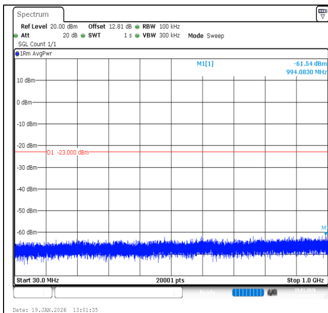
Band2-20MHz-QPSK-19100-100RB#0-30~1000-PASS
