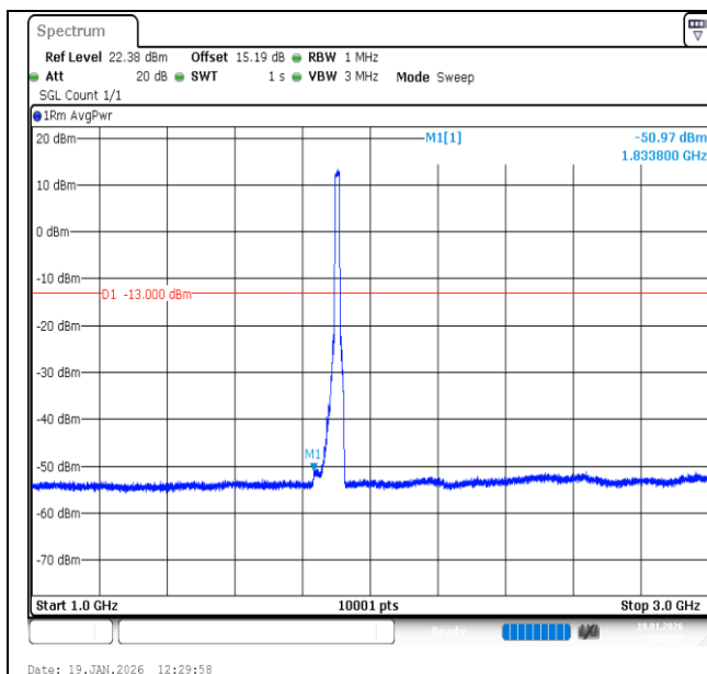
Band2-15MHz-16QAM-19125-75RB#0-1000~3000-PASS
