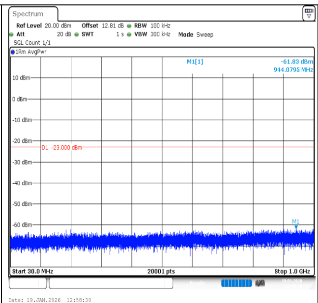
Band2-20MHz-QPSK-18900-100RB#0-30~1000-PASS
