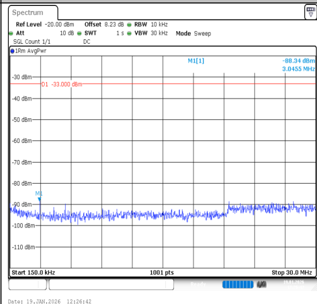
Band2-15MHz-16QAM-18900-75RB#0-0.15~30-PASS
