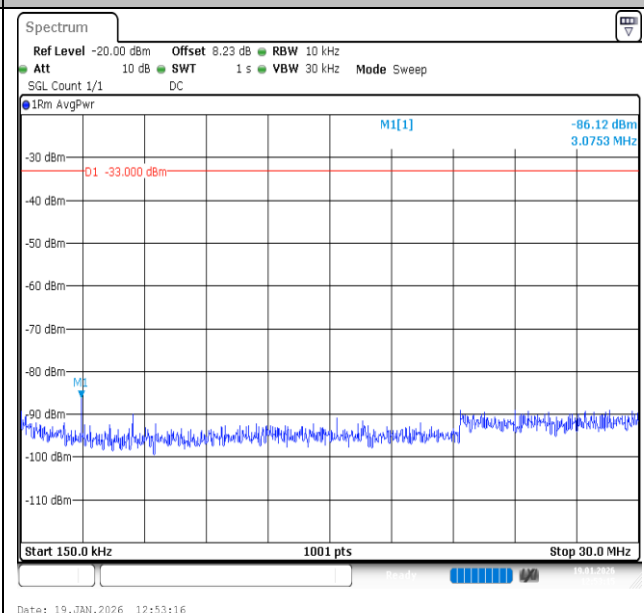
Band2-20MHz-QPSK-18700-1RB#0-0.15~30-PASS
