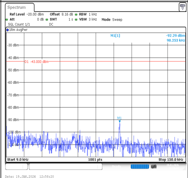
Band2-20MHz-QPSK-18900-100RB#0-0.009~0.15-PASS
