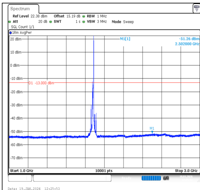
Band2-15MHz-16QAM-18900-1RB#74-1000~3000-PASS
