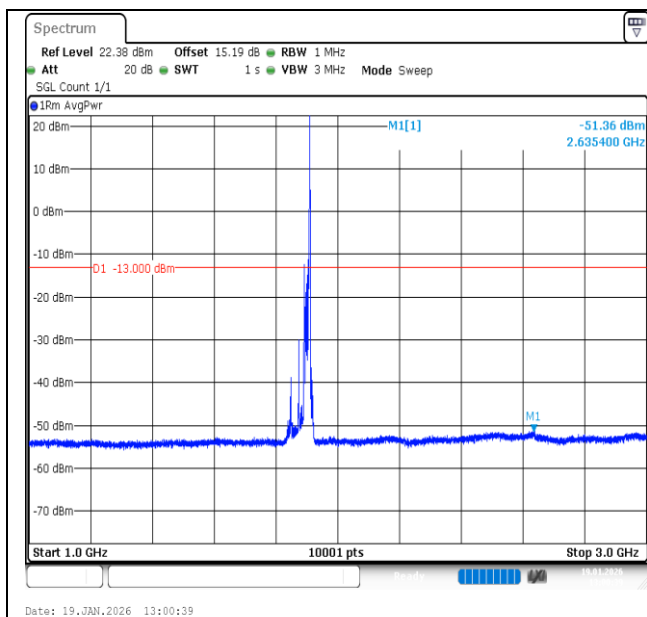
Band2-20MHz-QPSK-19100-1RB#99-1000~3000-PASS
