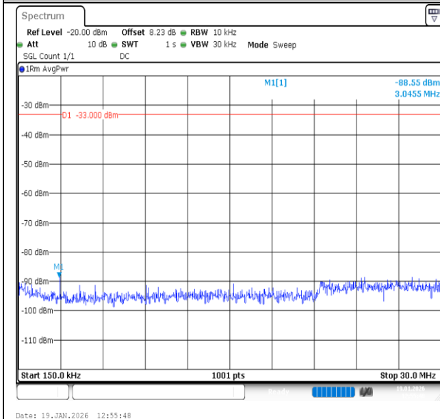
Band2-20MHz-16QAM-18700-100RB#0-0.15~30-PASS
