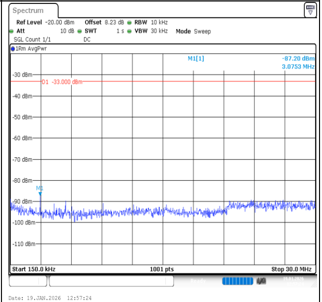
Band2-20MHz-QPSK-18900-1RB#99-0.15~30-PASS
