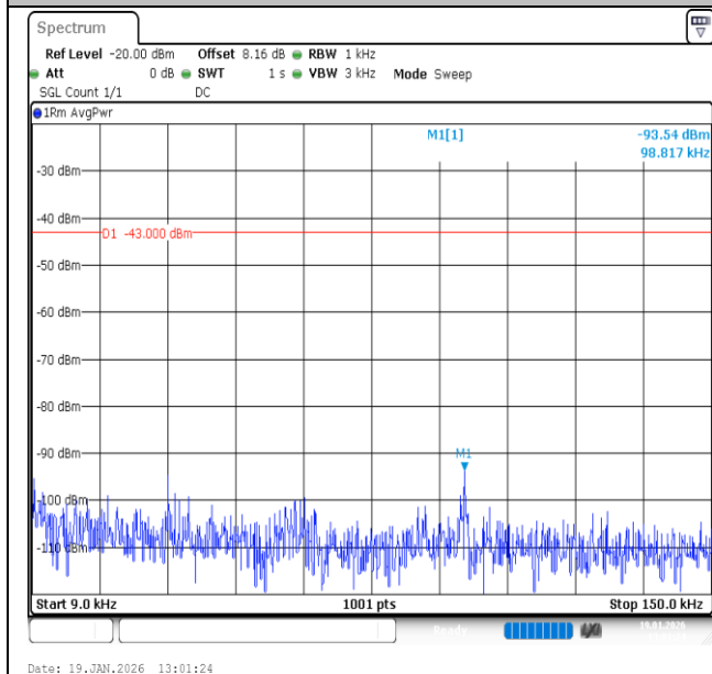
Band2-20MHz-QPSK-19100-100RB#0-0.009~0.15-PASS
