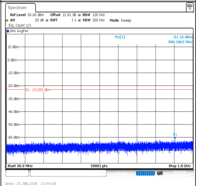
Band2-20MHz-QPSK-19100-1RB#99-30~1000-PASS
