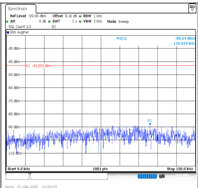
Band2-20MHz-QPSK-18900-1RB#0-0.009~0.15-PASS
