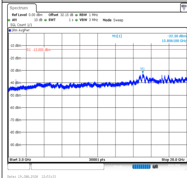
Band2-20MHz-QPSK-18700-1RB#0-3000~20000-PASS
