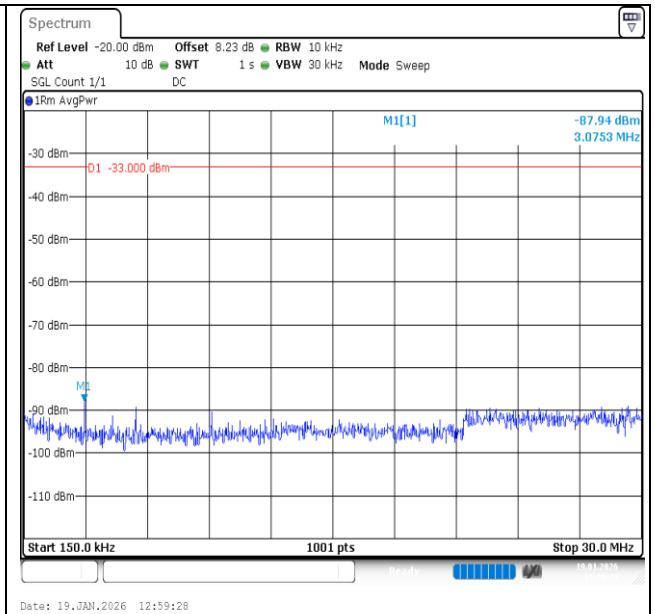
Band2-20MHz-QPSK-19100-1RB#0-0.15~30-PASS
