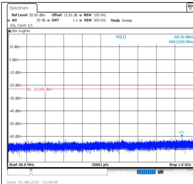
Band2-15MHz-16QAM-18900-75RB#0-30~1000-PASS
