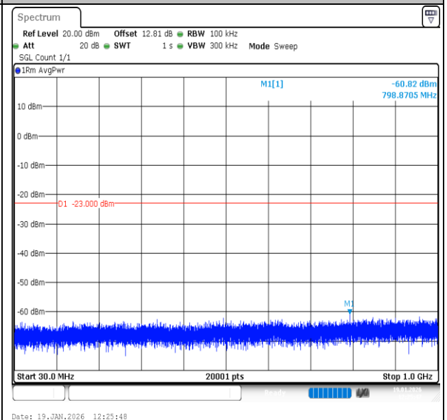
Band2-15MHz-16QAM-18900-1RB#74-30~1000-PASS
