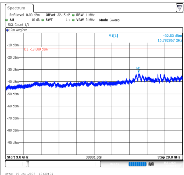
Band2-15MHz-16QAM-19125-75RB#0-3000~20000-PASS
