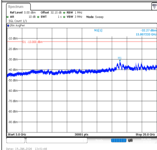
Band2-20MHz-QPSK-19100-100RB#0-3000~20000-PASS
