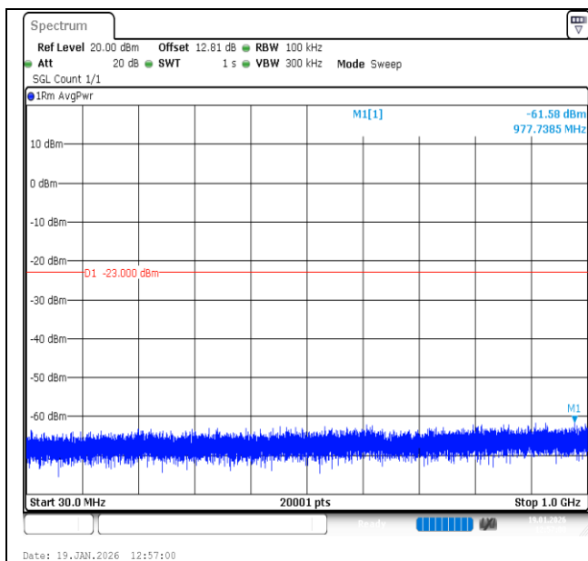
Band2-20MHz-16QAM-18900-1RB#0-30~1000-PASS
