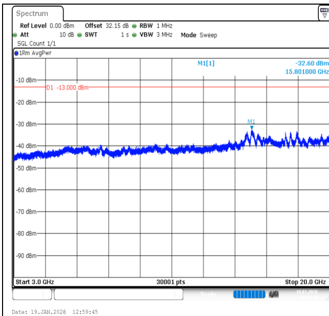
Band2-20MHz-QPSK-19100-1RB#0-3000~20000-PASS
