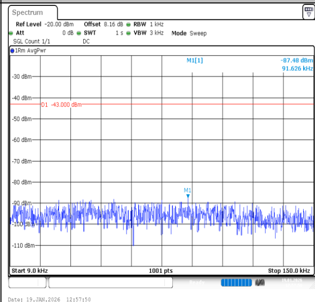
Band2-20MHz-16QAM-18900-1RB#99-0.009~0.15-PASS
