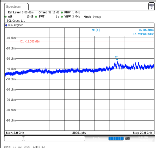
Band2-20MHz-16QAM-18900-1RB#99-3000~20000-PASS
