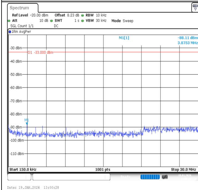
Band2-20MHz-QPSK-19100-1RB#99-0.15~30-PASS
