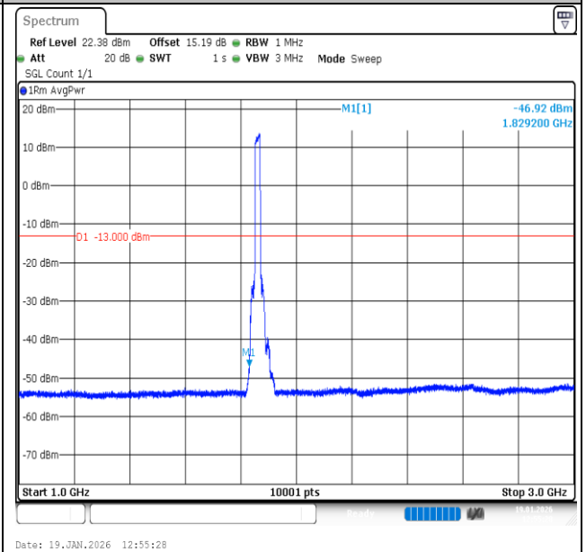
Band2-20MHz-QPSK-18700-100RB#0-1000~3000-PASS
