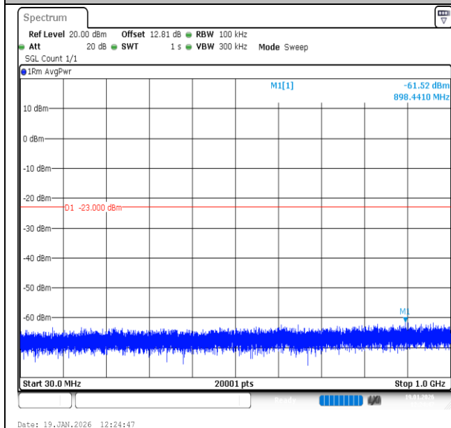
Band2-15MHz-16QAM-18900-1RB#0-30~1000-PASS
