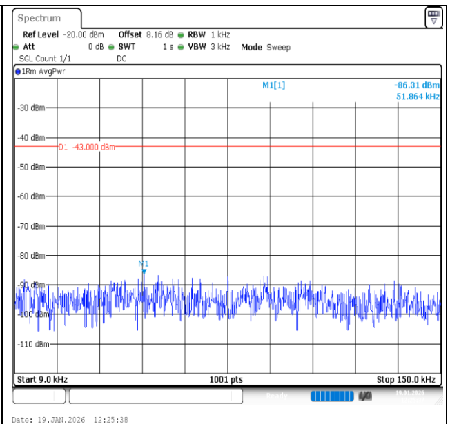
Band2-15MHz-16QAM-18900-1RB#74-0.009~0.15-PASS
