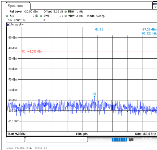
Band2-20MHz-16QAM-18700-1RB#99-0.009~0.15-PASS
