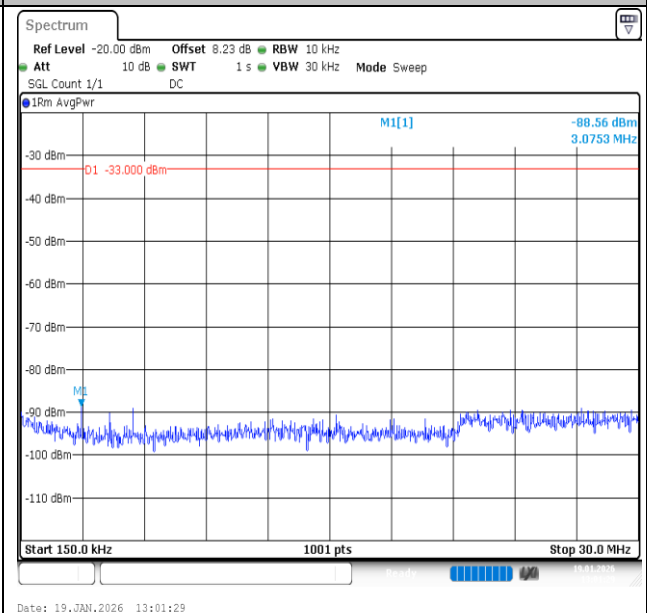
Band2-20MHz-QPSK-19100-100RB#0-0.15~30-PASS
