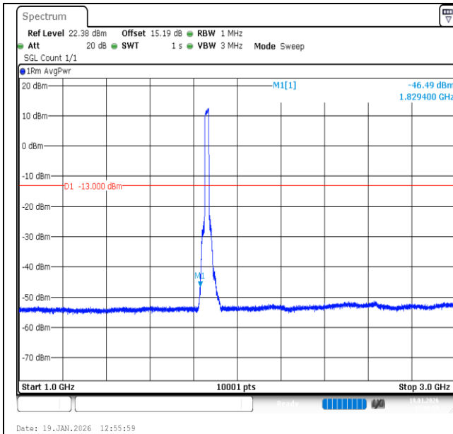
Band2-20MHz-16QAM-18700-100RB#0-1000~3000-PASS
