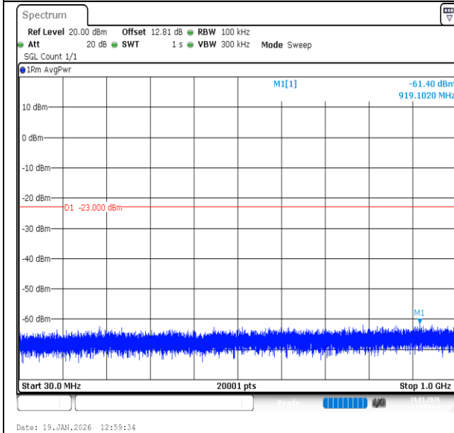
Band2-20MHz-QPSK-19100-1RB#0-30~1000-PASS
