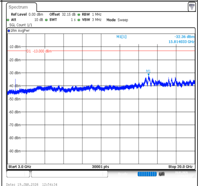
Band2-20MHz-QPSK-18700-1RB#99-3000~20000-PASS
