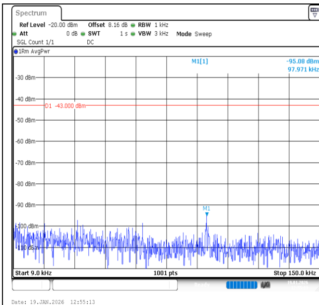
Band2-20MHz-QPSK-18700-100RB#0-0.009~0.15-PASS
