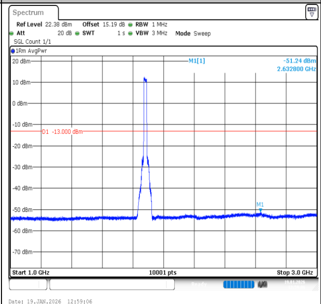
Band2-20MHz-16QAM-18900-100RB#0-1000~3000-PASS
