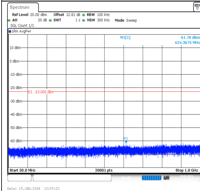
Band2-20MHz-QPSK-18700-100RB#0-30~1000-PASS
