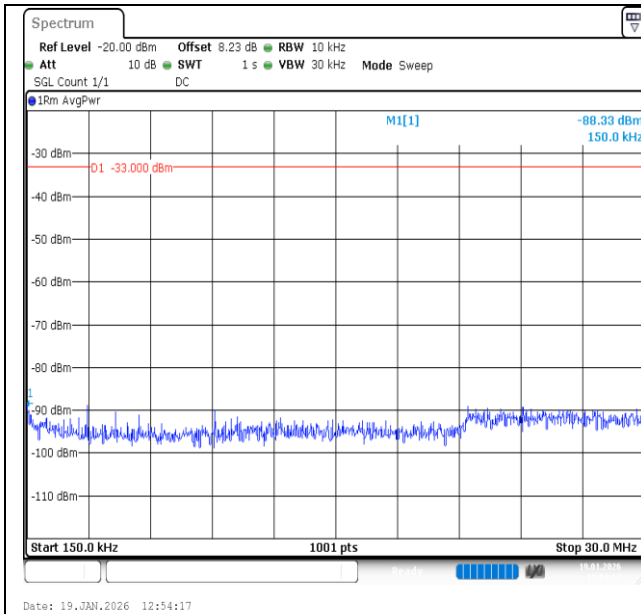
Band2-20MHz-QPSK-18700-1RB#99-0.15~30-PASS
