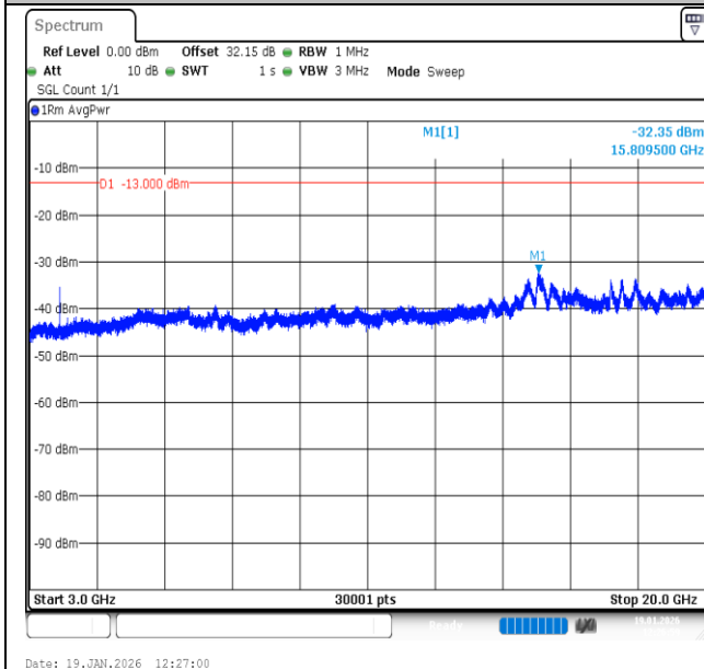
Band2-15MHz-16QAM-18900-75RB#0-3000~20000-PASS
