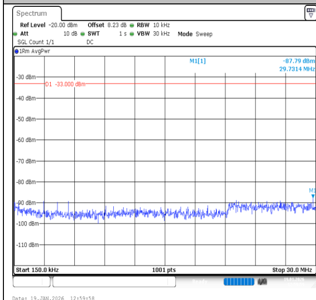
Band2-20MHz-16QAM-19100-1RB#0-0.15~30-PASS
