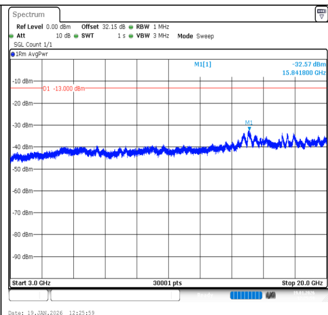
Band2-15MHz-16QAM-18900-1RB#74-3000~20000-PASS
