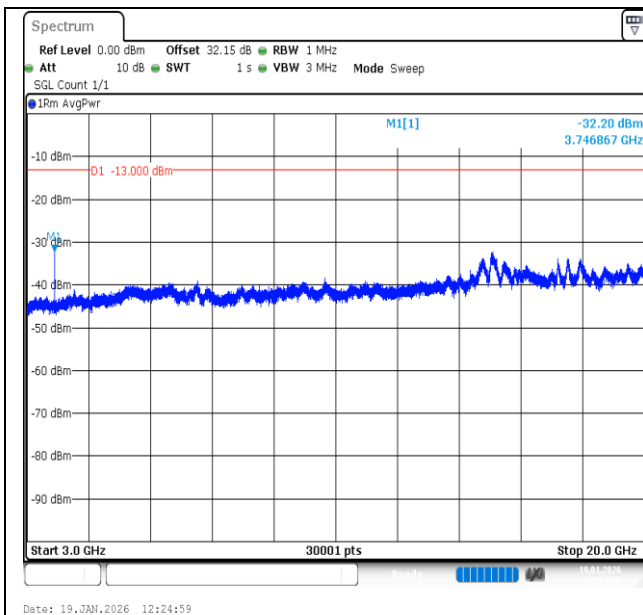
Band2-15MHz-16QAM-18900-1RB#0-3000~20000-PASS
