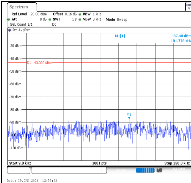
Band2-20MHz-QPSK-19100-1RB#0-0.009~0.15-PASS
