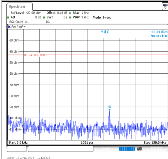
Band2-15MHz-16QAM-18900-75RB#0-0.009~0.15-PASS
