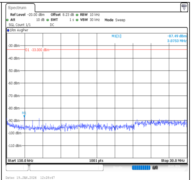
Band2-15MHz-16QAM-19125-1RB#74-0.15~30-PASS
