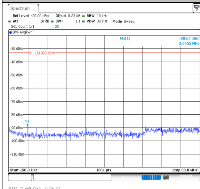
Band2-20MHz-QPSK-18900-1RB#0-0.15~30-PASS
