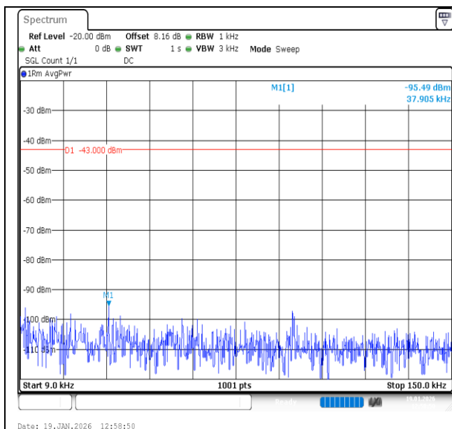
Band2-20MHz-16QAM-18900-100RB#0-0.009~0.15-PASS
