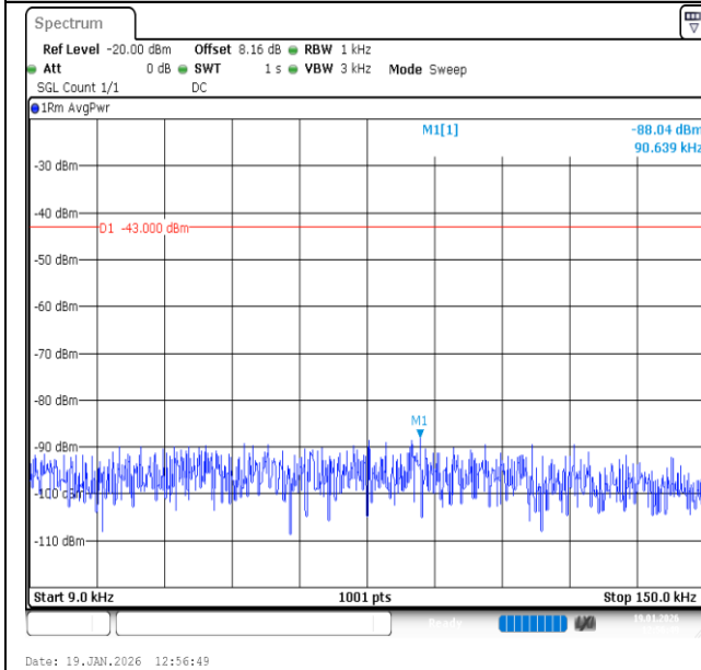
Band2-20MHz-16QAM-18900-1RB#0-0.009~0.15-PASS
