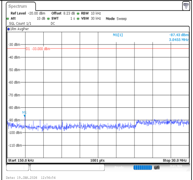
Band2-20MHz-16QAM-18900-1RB#0-0.15~30-PASS
