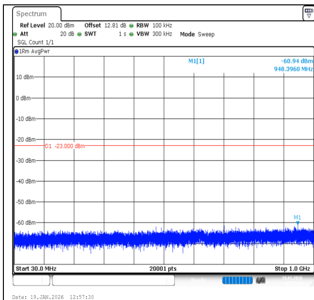
Band2-20MHz-QPSK-18900-1RB#99-30~1000-PASS
