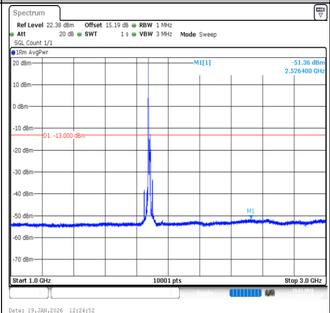
Band2-15MHz-16QAM-18900-1RB#0-1000~3000-PASS
