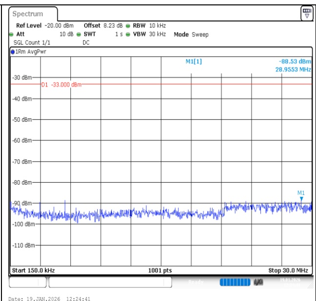
Band2-15MHz-16QAM-18900-1RB#0-0.15~30-PASS
