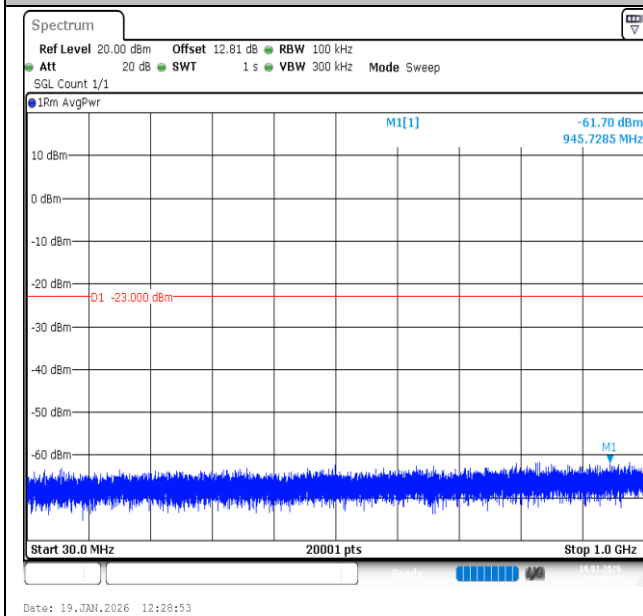
Band2-15MHz-16QAM-19125-1RB#74-30~1000-PASS
