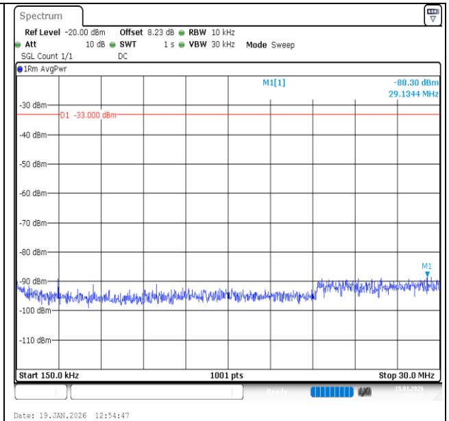
Band2-20MHz-16QAM-18700-1RB#99-0.15~30-PASS
