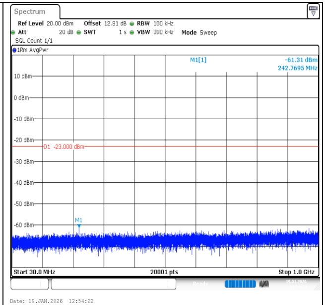
Band2-20MHz-QPSK-18700-1RB#99-30~1000-PASS
