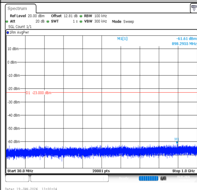
Band2-20MHz-16QAM-19100-1RB#0-30~1000-PASS
