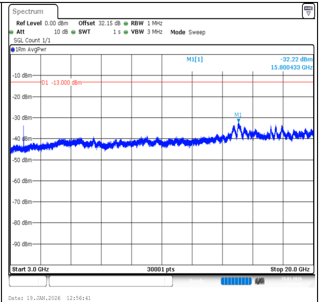
Band2-20MHz-QPSK-18900-1RB#0-3000~20000-PASS
