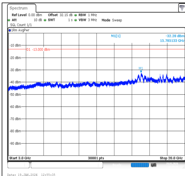
Band2-20MHz-QPSK-18700-100RB#0-3000~20000-PASS
