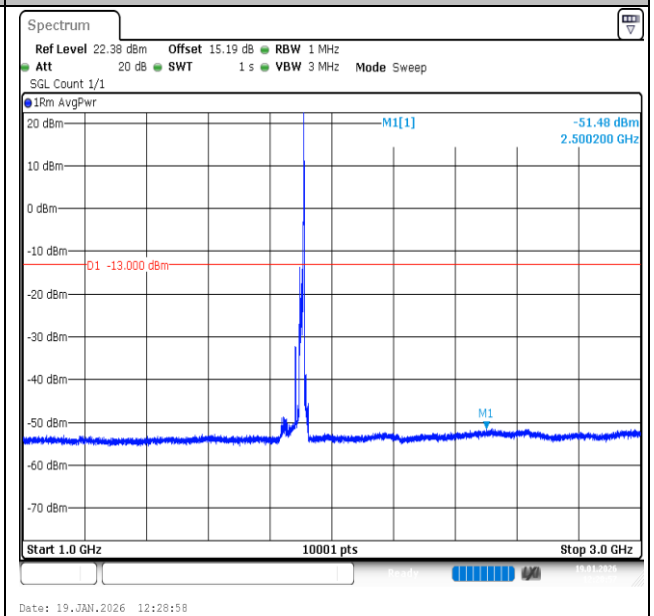
Band2-15MHz-16QAM-19125-1RB#74-1000~3000-PASS
