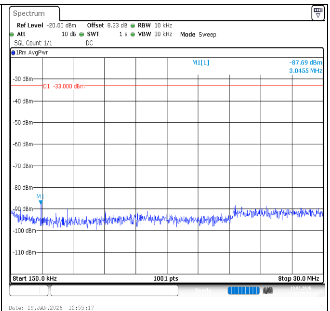
Band2-20MHz-QPSK-18700-100RB#0-0.15~30-PASS
