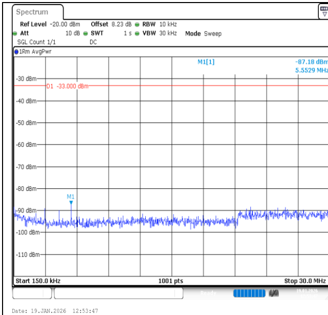
Band2-20MHz-16QAM-18700-1RB#0-0.15~30-PASS
