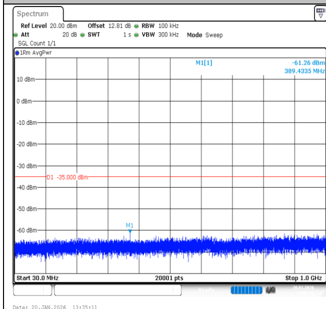
Band7-15MHz-QPSK-21375-1RB#0-30~1000-PASS
