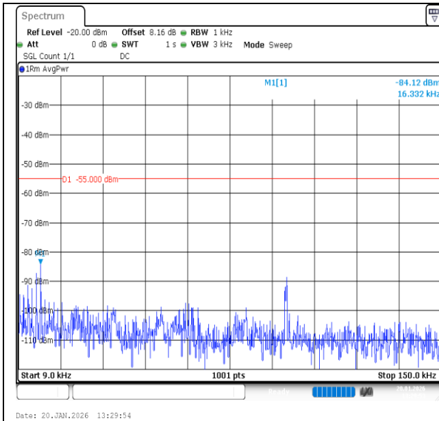
Band7-15MHz-QPSK-20825-75RB#0-0.009~0.15-PASS
