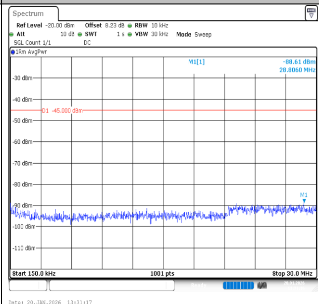
Band7-15MHz-QPSK-21100-1RB#0-0.15~30-PASS
