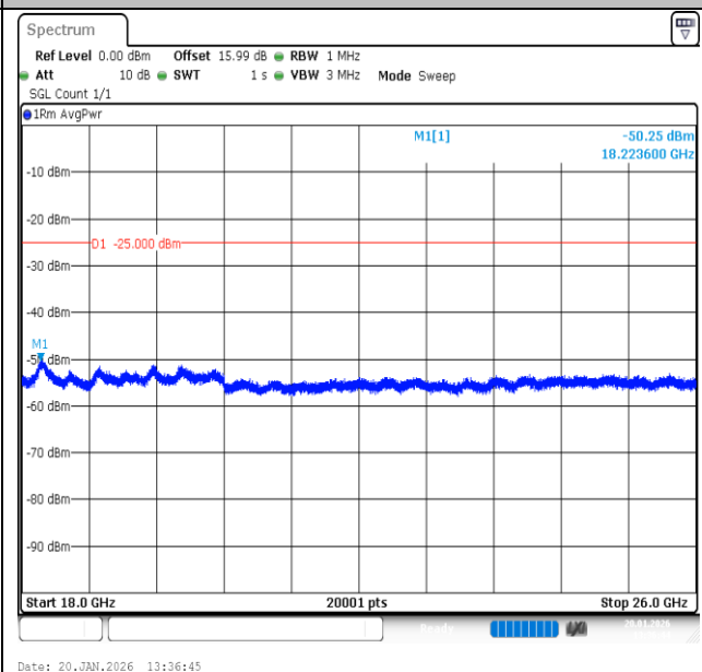
Band7-15MHz-QPSK-21375-1RB#74-18000~26000-PASS
