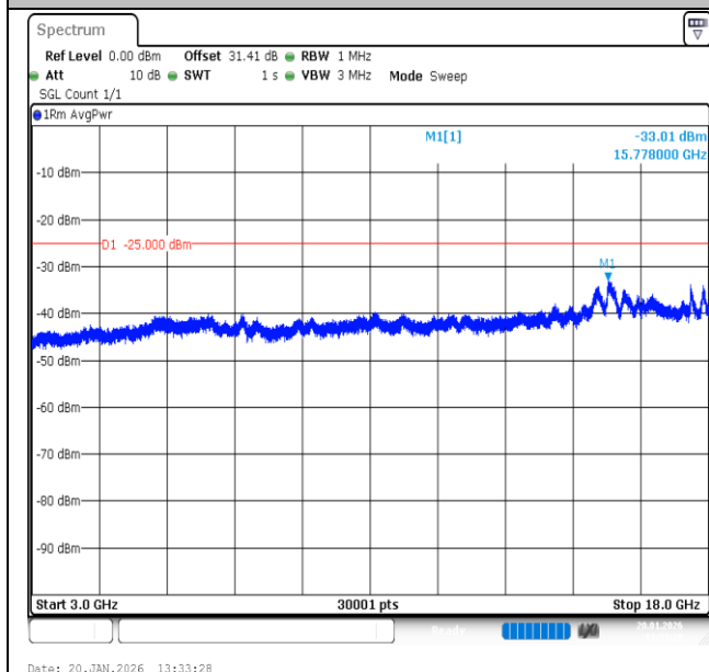
Band7-15MHz-16QAM-21100-1RB#74-3000~18000-PASS
