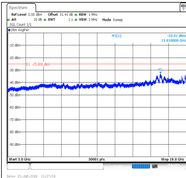
Band7-15MHz-QPSK-21375-75RB#0-3000~18000-PASS
