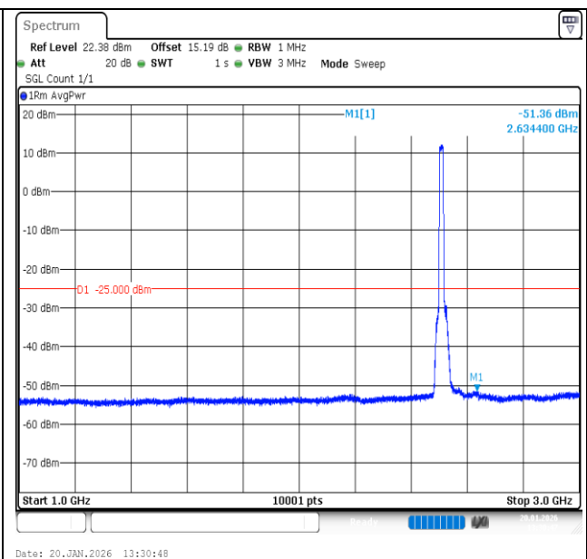
Band7-15MHz-16QAM-20825-75RB#0-1000~3000-PASS
