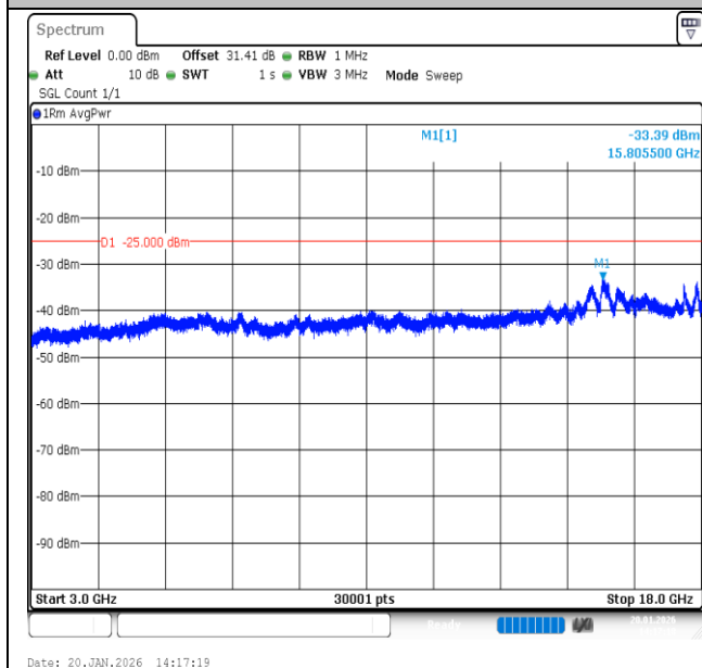
Band7-20MHz-QPSK-20850-1RB#99-3000~18000-PASS
