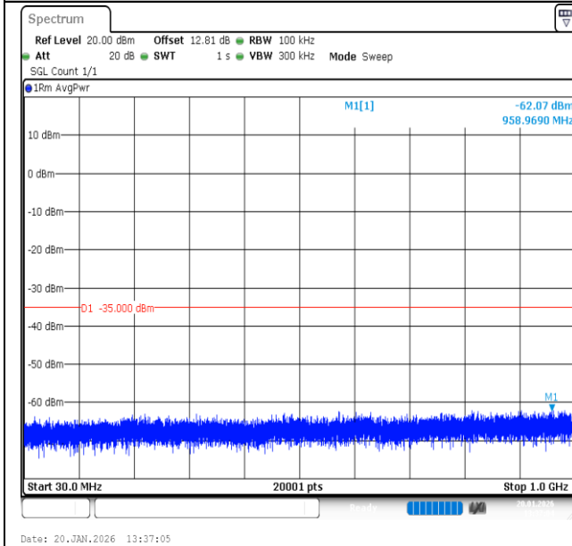
Band7-15MHz-16QAM-21375-1RB#74-30~1000-PASS
