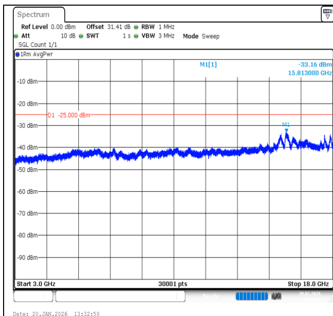
Band7-15MHz-QPSK-21100-1RB#74-3000~18000-PASS
