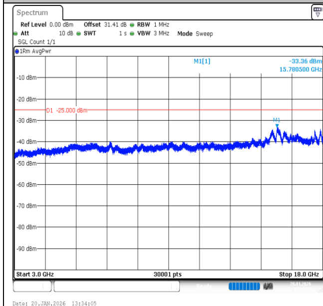
Band7-15MHz-QPSK-21100-75RB#0-3000~18000-PASS
