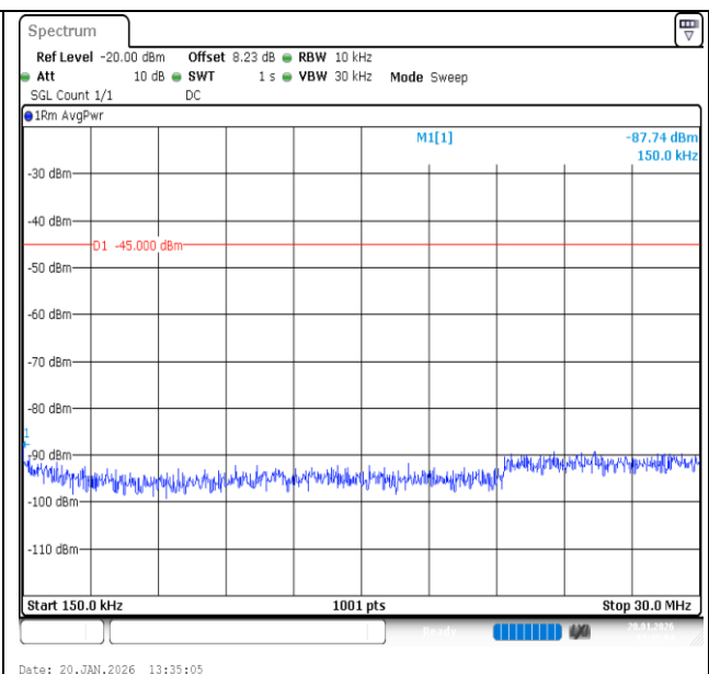
Band7-15MHz-QPSK-21375-1RB#0-0.15~30-PASS
