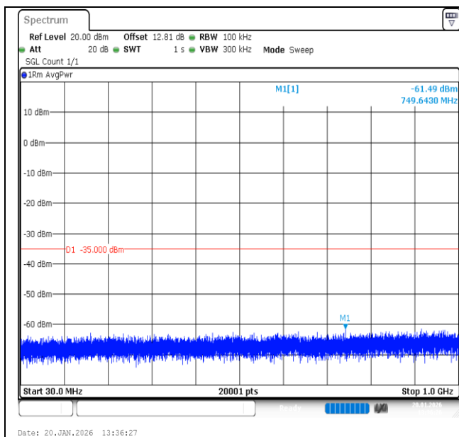
Band7-15MHz-QPSK-21375-1RB#74-30~1000-PASS
