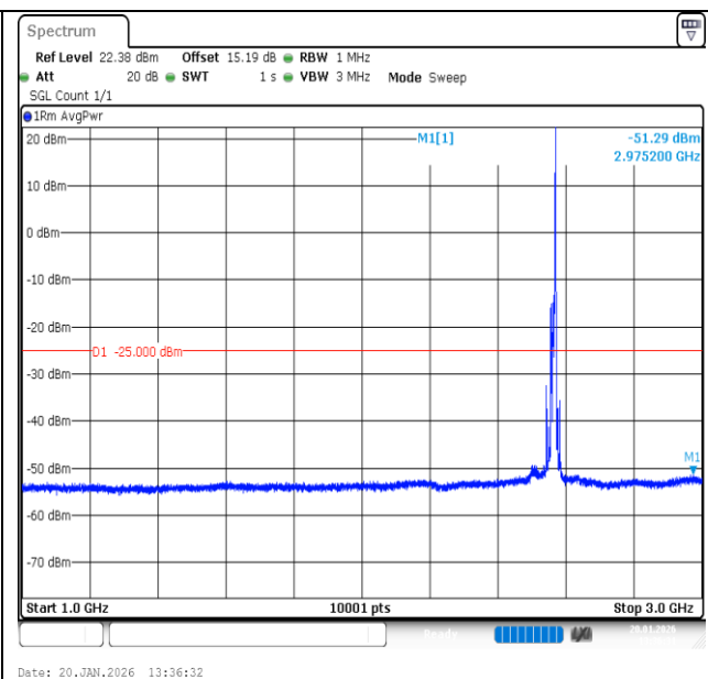
Band7-15MHz-QPSK-21375-1RB#74-1000~3000-PASS
