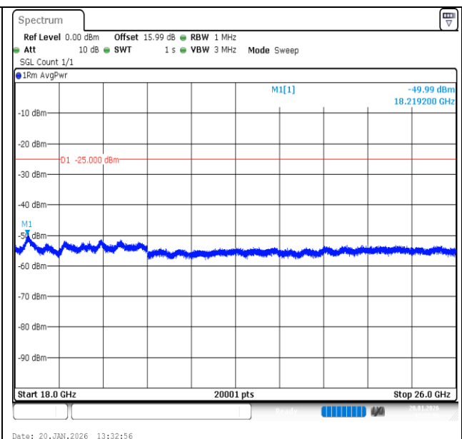
Band7-15MHz-QPSK-21100-1RB#74-18000~26000-PASS
