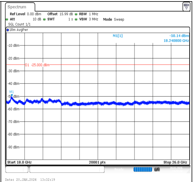
Band7-15MHz-16QAM-21100-1RB#0-18000~26000-PASS
