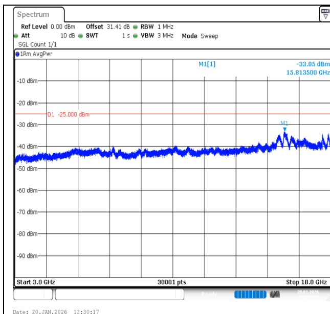
Band7-15MHz-QPSK-20825-75RB#0-3000~18000-PASS
