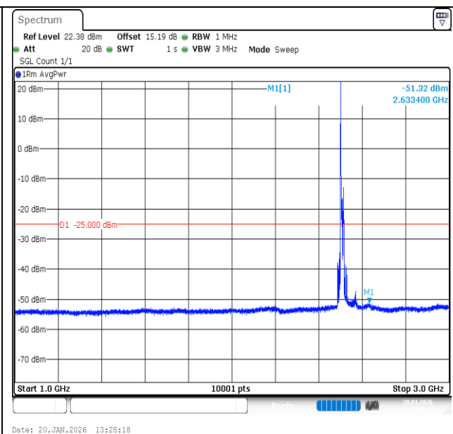
Band7-15MHz-16QAM-20825-1RB#0-1000~3000-PASS
