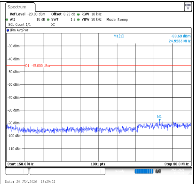
Band7-15MHz-16QAM-20825-1RB#74-0.15~30-PASS
