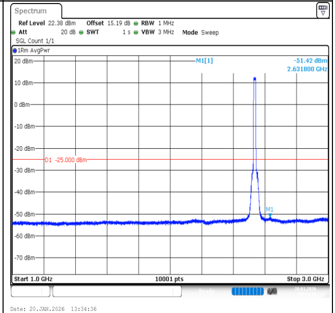
Band7-15MHz-16QAM-21100-75RB#0-1000~3000-PASS
