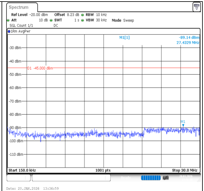
Band7-15MHz-16QAM-21375-1RB#74-0.15~30-PASS
