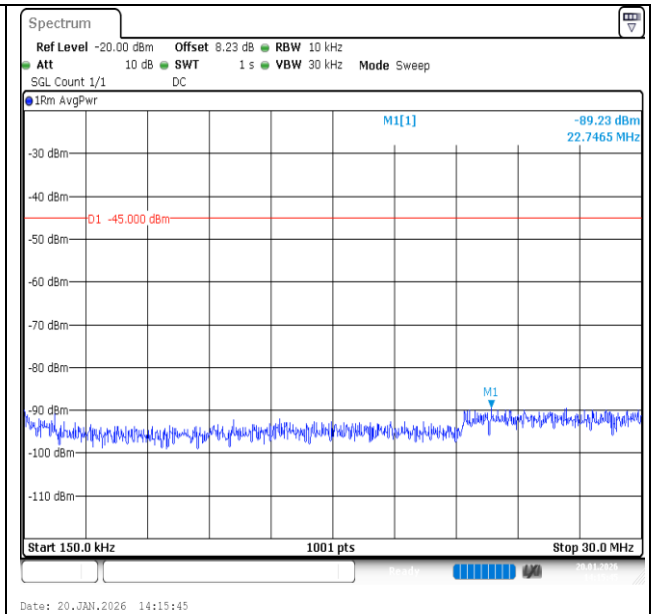
Band7-20MHz-QPSK-20850-1RB#0-0.15~30-PASS
