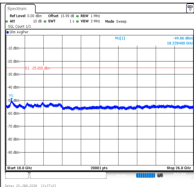
Band7-15MHz-16QAM-21375-1RB#74-18000~26000-PASS
