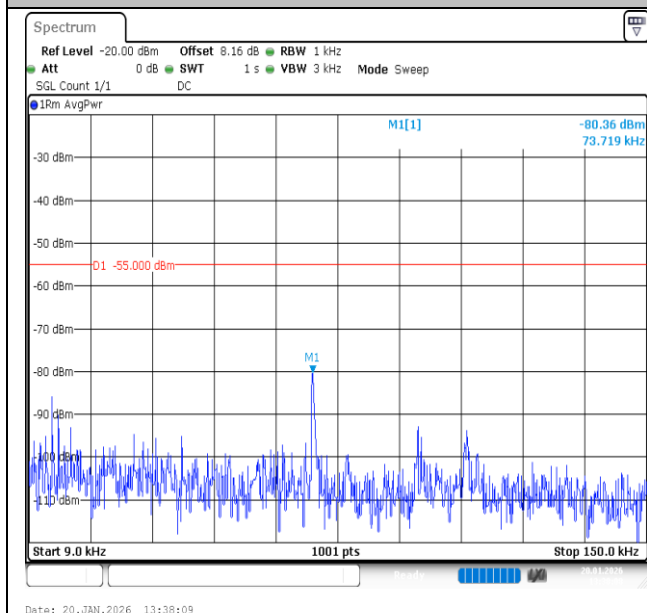
Band7-15MHz-16QAM-21375-75RB#0-0.009~0.15-PASS
