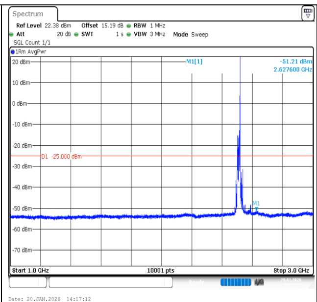
Band7-20MHz-QPSK-20850-1RB#99-1000~3000-PASS
