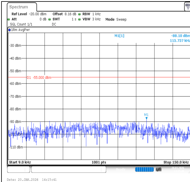
Band7-20MHz-QPSK-20850-1RB#0-0.009~0.15-PASS
