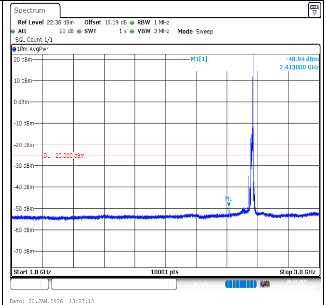
Band7-15MHz-16QAM-21375-1RB#74-1000~3000-PASS
