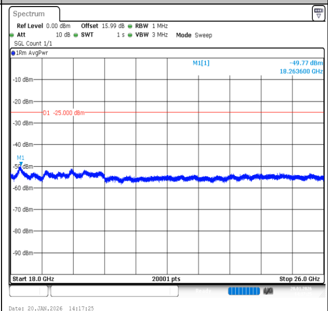
Band7-20MHz-QPSK-20850-1RB#99-18000~26000-PASS
