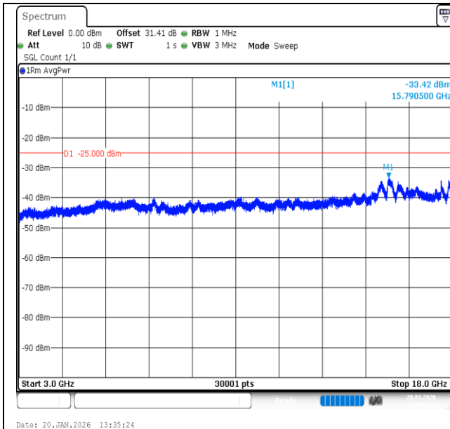
Band7-15MHz-QPSK-21375-1RB#0-3000~18000-PASS
