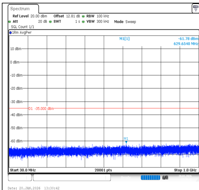
Band7-15MHz-16QAM-20825-75RB#0-30~1000-PASS
