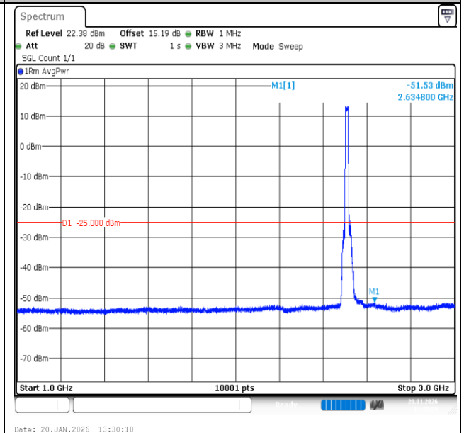
Band7-15MHz-QPSK-20825-75RB#0-1000~3000-PASS
