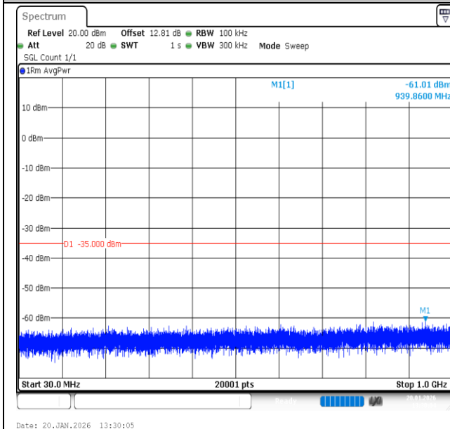
Band7-15MHz-QPSK-20825-75RB#0-30~1000-PASS
