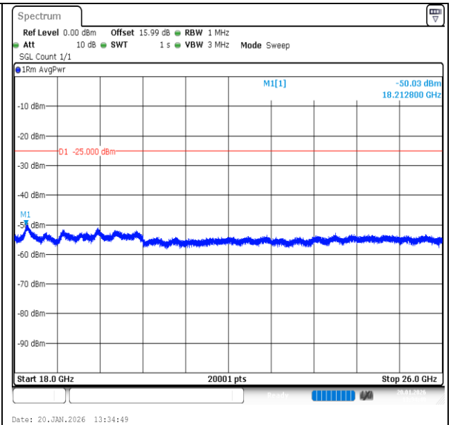
Band7-15MHz-16QAM-21100-75RB#0-18000~26000-PASS
