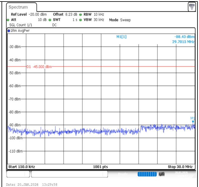
Band7-15MHz-QPSK-20825-75RB#0-0.15~30-PASS
