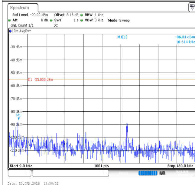
Band7-15MHz-16QAM-20825-75RB#0-0.009~0.15-PASS
