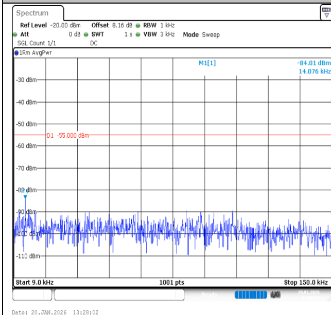
Band7-15MHz-16QAM-20825-1RB#0-0.009~0.15-PASS
