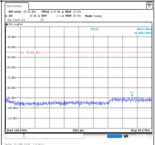
Band7-15MHz-QPSK-21375-1RB#74-0.15~30-PASS
