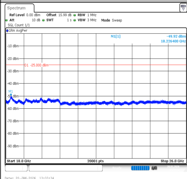
Band7-15MHz-16QAM-21100-1RB#74-18000~26000-PASS
