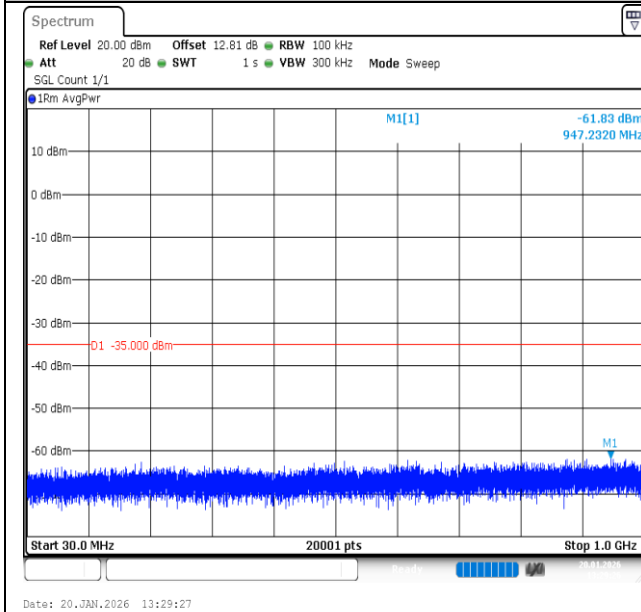
Band7-15MHz-16QAM-20825-1RB#74-30~1000-PASS
