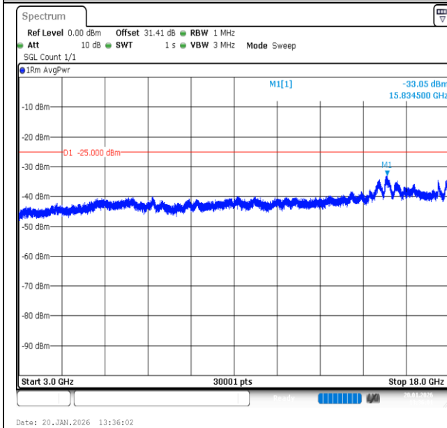
Band7-15MHz-16QAM-21375-1RB#0-3000~18000-PASS
