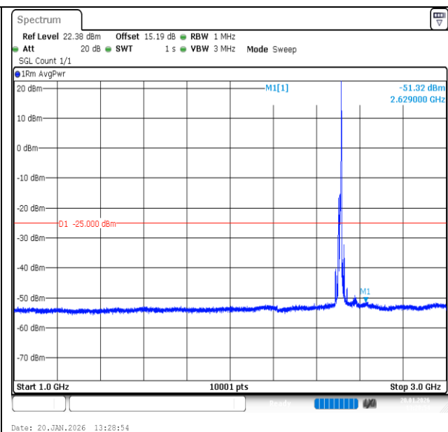
Band7-15MHz-QPSK-20825-1RB#74-1000~3000-PASS
