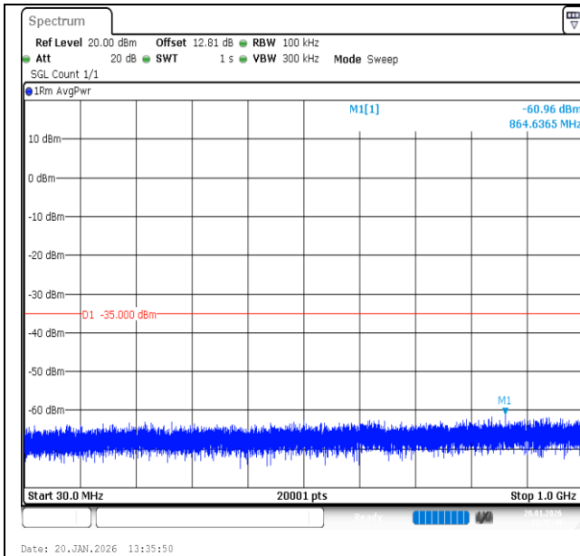
Band7-15MHz-16QAM-21375-1RB#0-30~1000-PASS
