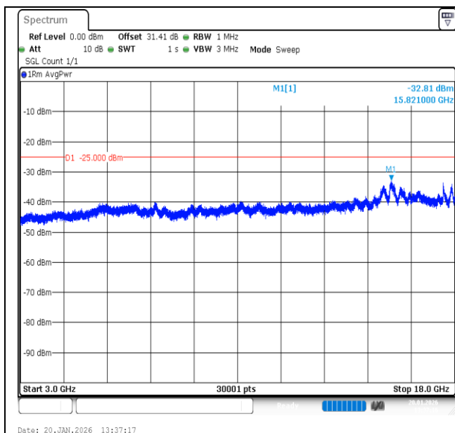
Band7-15MHz-16QAM-21375-1RB#74-3000~18000-PASS
