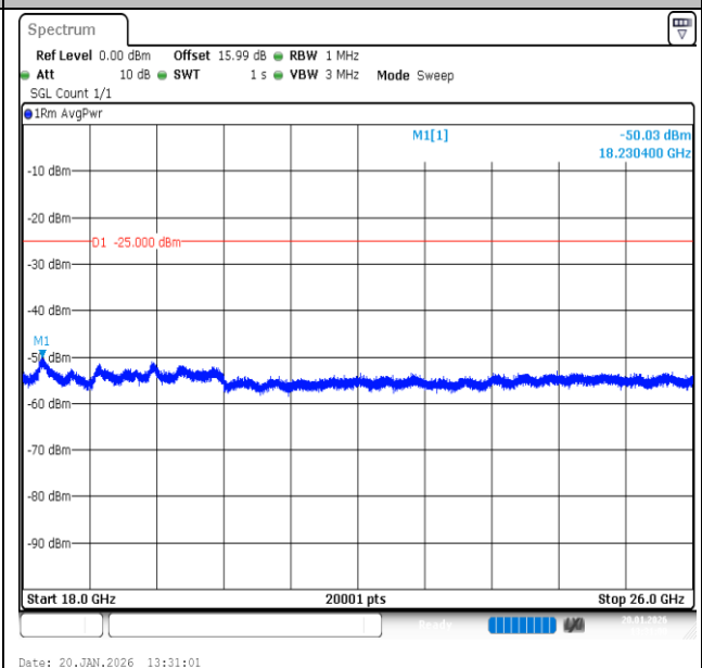
Band7-15MHz-16QAM-20825-75RB#0-18000~26000-PASS
