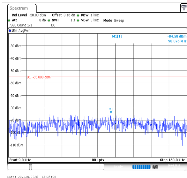
Band7-15MHz-QPSK-21375-1RB#0-0.009~0.15-PASS
