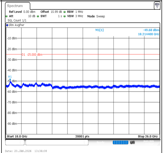
Band7-15MHz-16QAM-21375-1RB#0-18000~26000-PASS
