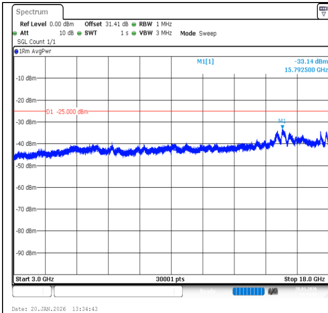
Band7-15MHz-16QAM-21100-75RB#0-3000~18000-PASS
