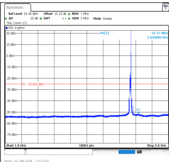
Band7-15MHz-16QAM-21100-1RB#74-1000~3000-PASS
