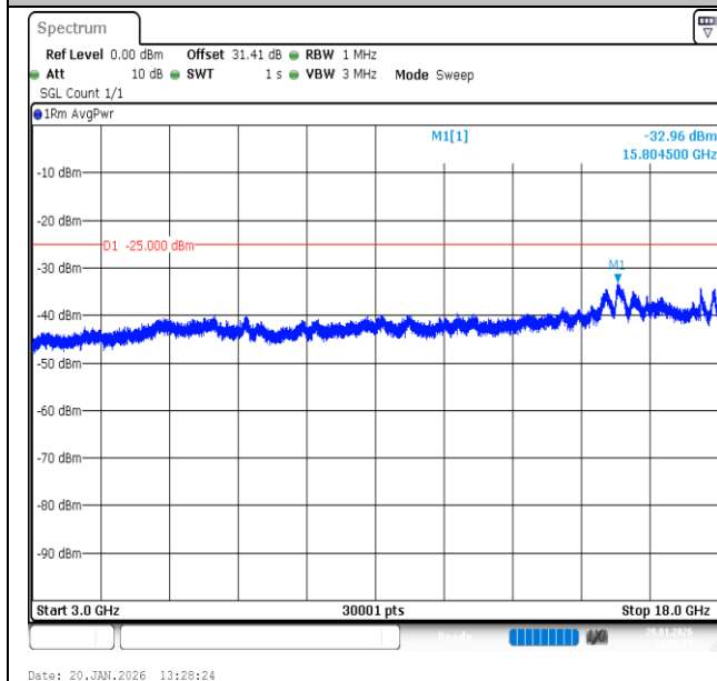
Band7-15MHz-16QAM-20825-1RB#0-3000~18000-PASS
