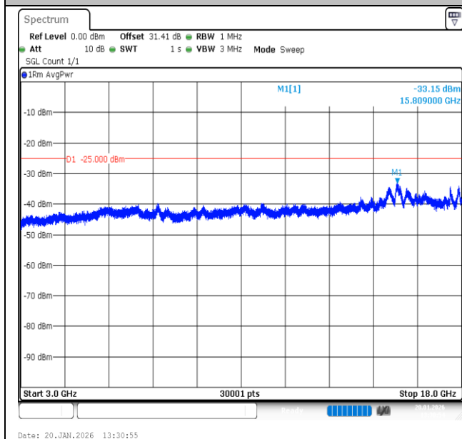
Band7-15MHz-16QAM-20825-75RB#0-3000~18000-PASS
