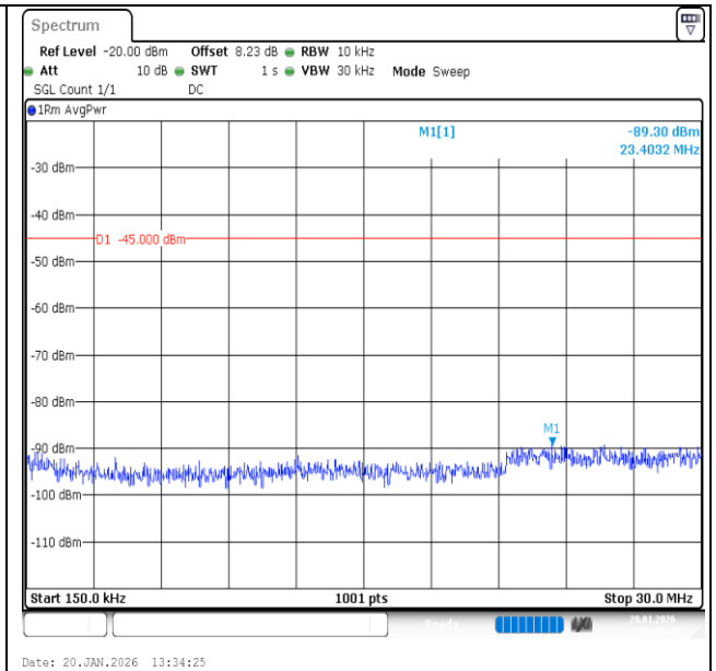
Band7-15MHz-16QAM-21100-75RB#0-0.15~30-PASS
