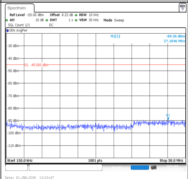
Band7-15MHz-QPSK-21100-75RB#0-0.15~30-PASS
