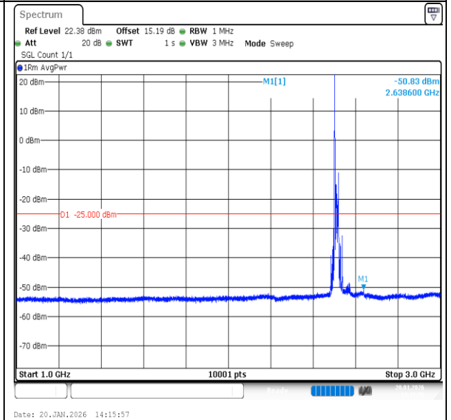
Band7-20MHz-QPSK-20850-1RB#0-1000~3000-PASS
