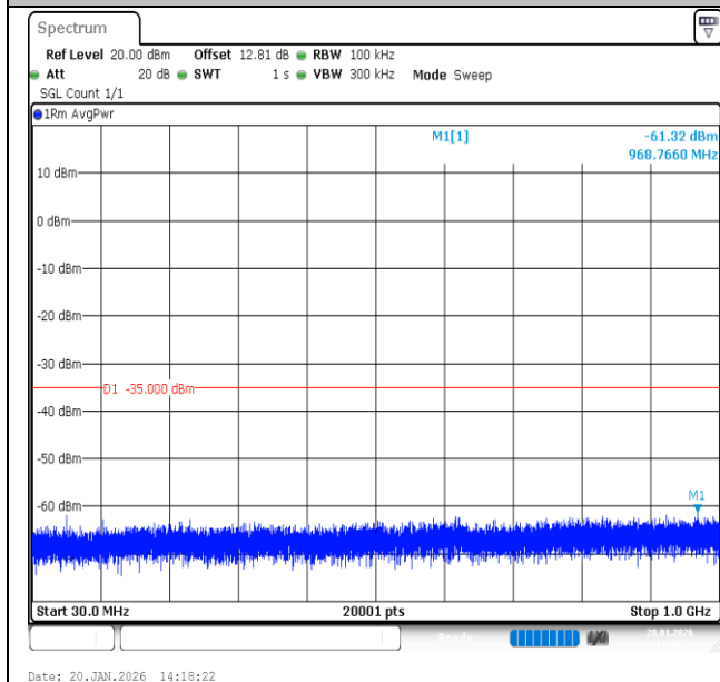
Band7-20MHz-QPSK-20850-100RB#0-30~1000-PASS
