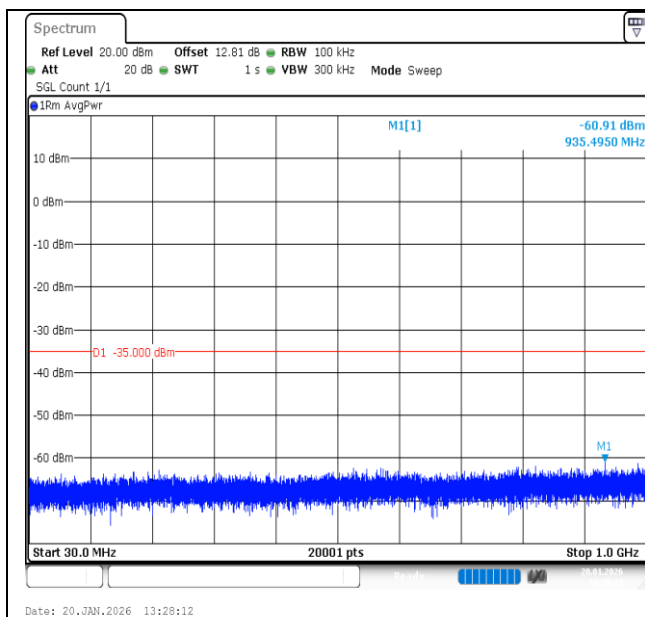
Band7-15MHz-16QAM-20825-1RB#0-30~1000-PASS
