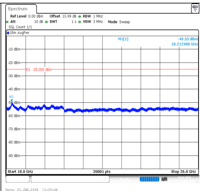
Band7-15MHz-16QAM-20825-1RB#74-18000~26000-PASS
