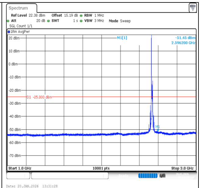
Band7-15MHz-QPSK-21100-1RB#0-1000~3000-PASS
