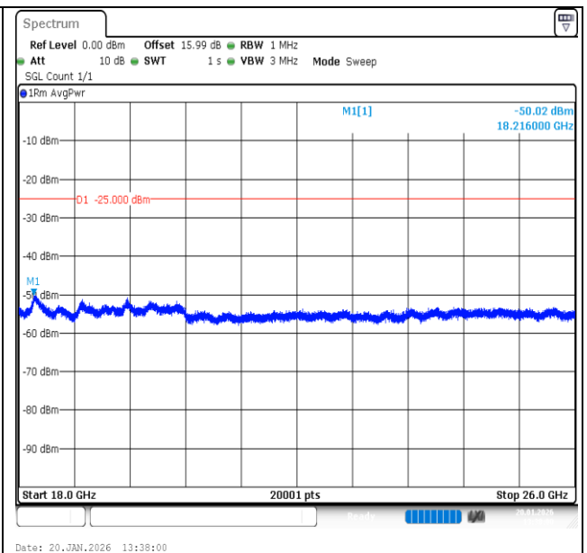
Band7-15MHz-QPSK-21375-75RB#0-18000~26000-PASS
