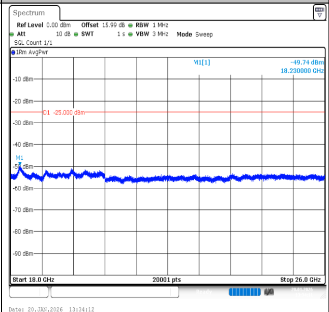
Band7-15MHz-QPSK-21100-75RB#0-18000~26000-PASS
