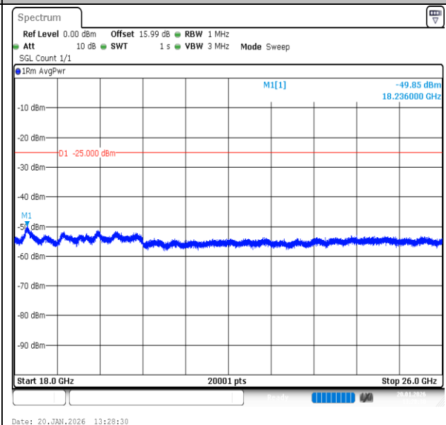
Band7-15MHz-16QAM-20825-1RB#0-18000~26000-PASS
