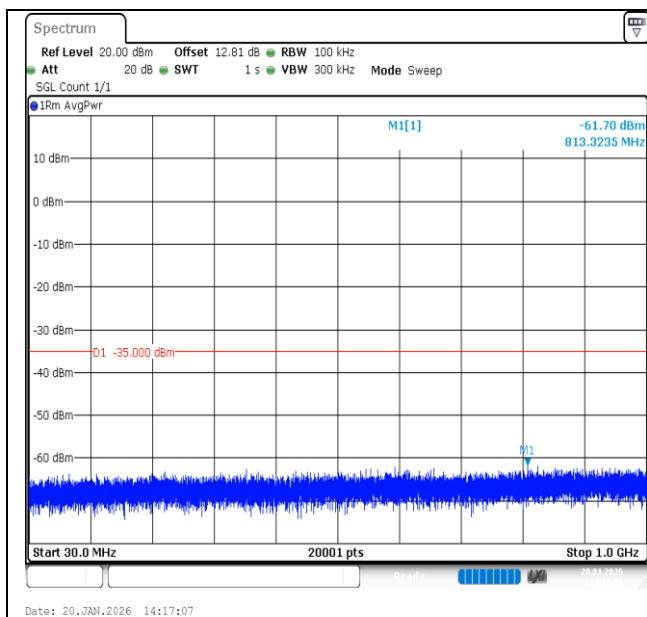
Band7-20MHz-QPSK-20850-1RB#99-30~1000-PASS
