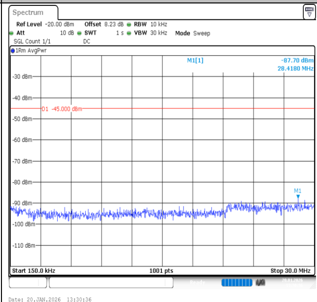
Band7-15MHz-16QAM-20825-75RB#0-0.15~30-PASS
