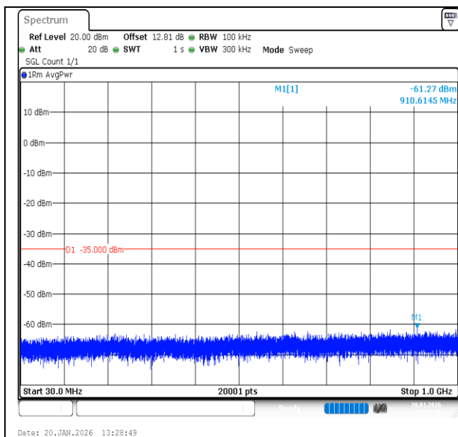
Band7-15MHz-QPSK-20825-1RB#74-30~1000-PASS
