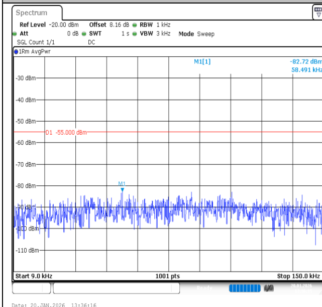
Band7-15MHz-QPSK-21375-1RB#74-0.009~0.15-PASS
