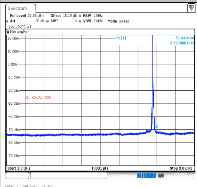
Band7-15MHz-QPSK-21375-1RB#0-1000~3000-PASS
