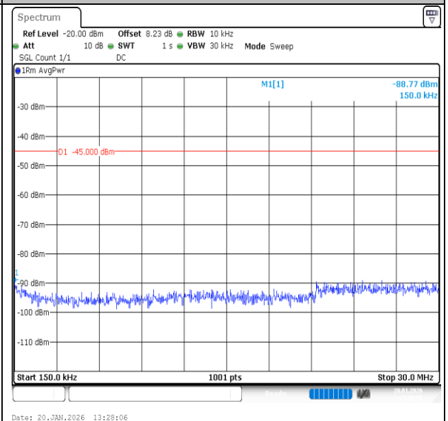
Band7-15MHz-16QAM-20825-1RB#0-0.15~30-PASS
