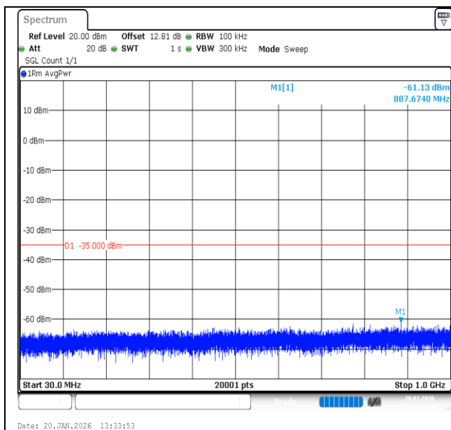
Band7-15MHz-QPSK-21100-75RB#0-30~1000-PASS
