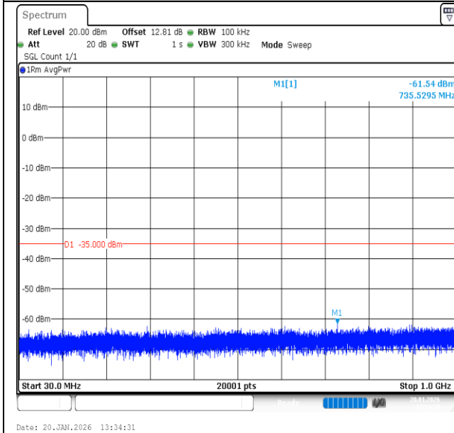
Band7-15MHz-16QAM-21100-75RB#0-30~1000-PASS
