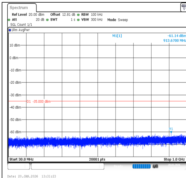
Band7-15MHz-QPSK-21100-1RB#0-30~1000-PASS
