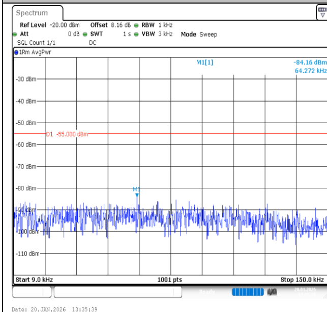
Band7-15MHz-16QAM-21375-1RB#0-0.009~0.15-PASS
