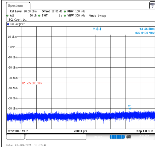
Band7-15MHz-QPSK-21375-75RB#0-30~1000-PASS
