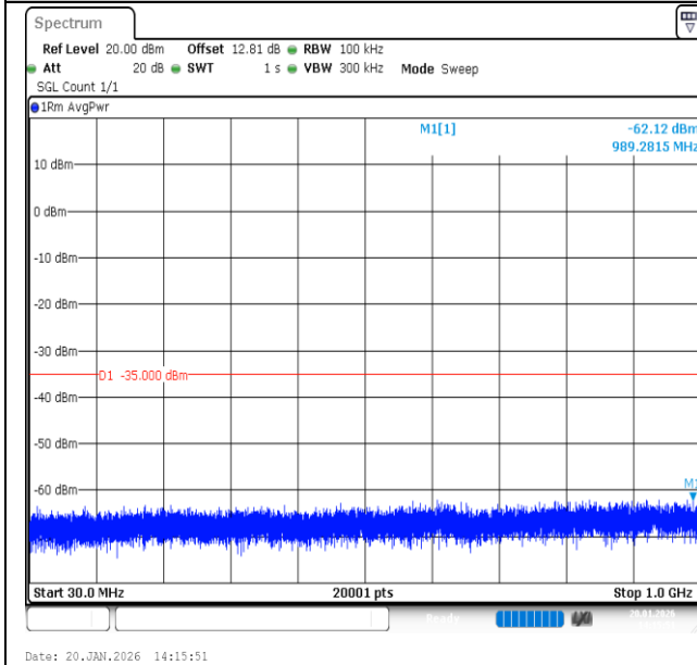
Band7-20MHz-QPSK-20850-1RB#0-30~1000-PASS
