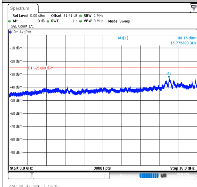
Band7-15MHz-QPSK-20825-1RB#74-3000~18000-PASS
