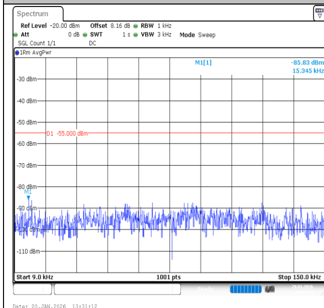
Band7-15MHz-QPSK-21100-1RB#0-0.009~0.15-PASS
