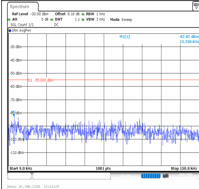
Band7-15MHz-16QAM-21100-1RB#74-0.009~0.15-PASS
