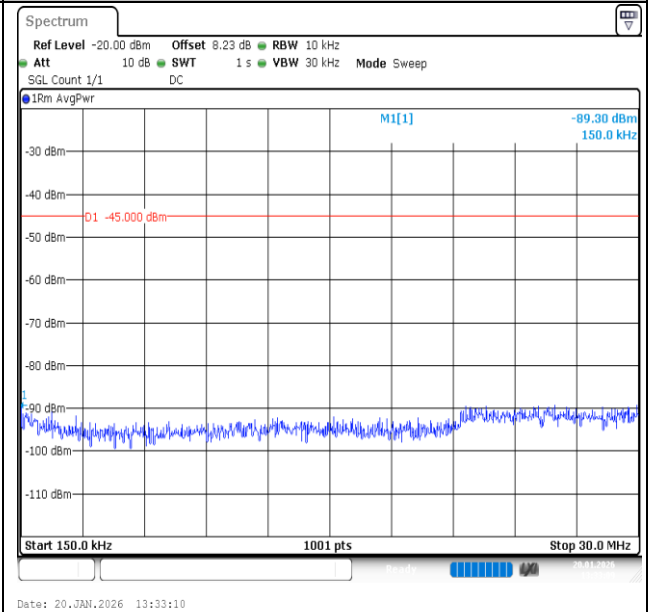
Band7-15MHz-16QAM-21100-1RB#74-0.15~30-PASS
