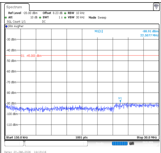
Band7-20MHz-QPSK-20850-100RB#0-0.15~30-PASS
