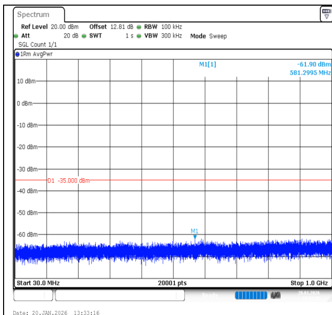
Band7-15MHz-16QAM-21100-1RB#74-30~1000-PASS
