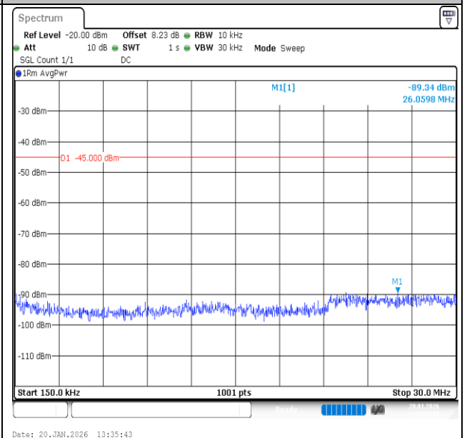
Band7-15MHz-16QAM-21375-1RB#0-0.15~30-PASS
