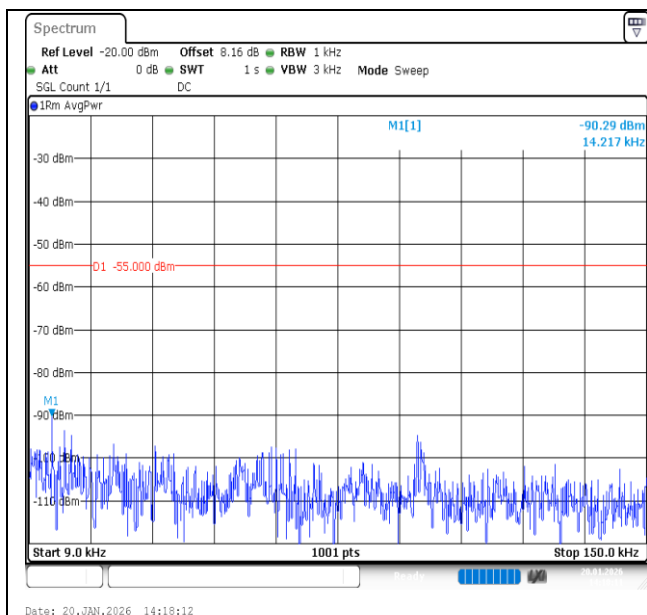
Band7-20MHz-QPSK-20850-100RB#0-0.009~0.15-PASS
