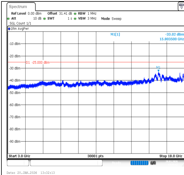
Band7-15MHz-16QAM-21100-1RB#0-3000~18000-PASS
