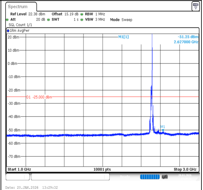
Band7-15MHz-16QAM-20825-1RB#74-1000~3000-PASS
