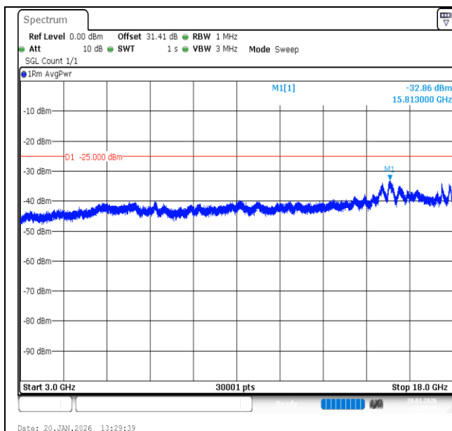
Band7-15MHz-16QAM-20825-1RB#74-3000~18000-PASS
