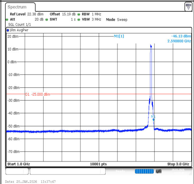
Band7-15MHz-QPSK-21375-75RB#0-1000~3000-PASS
