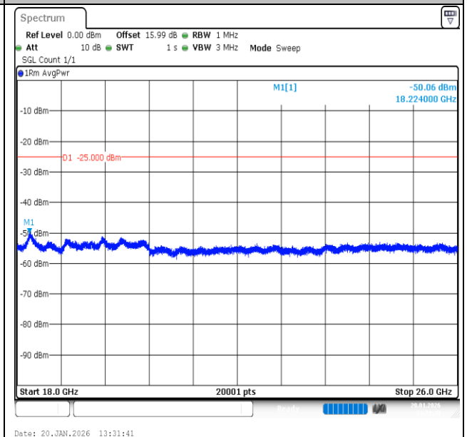
Band7-15MHz-QPSK-21100-1RB#0-18000~26000-PASS
