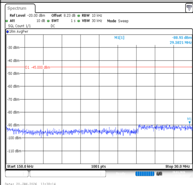
Band7-15MHz-16QAM-21375-75RB#0-0.15~30-PASS
