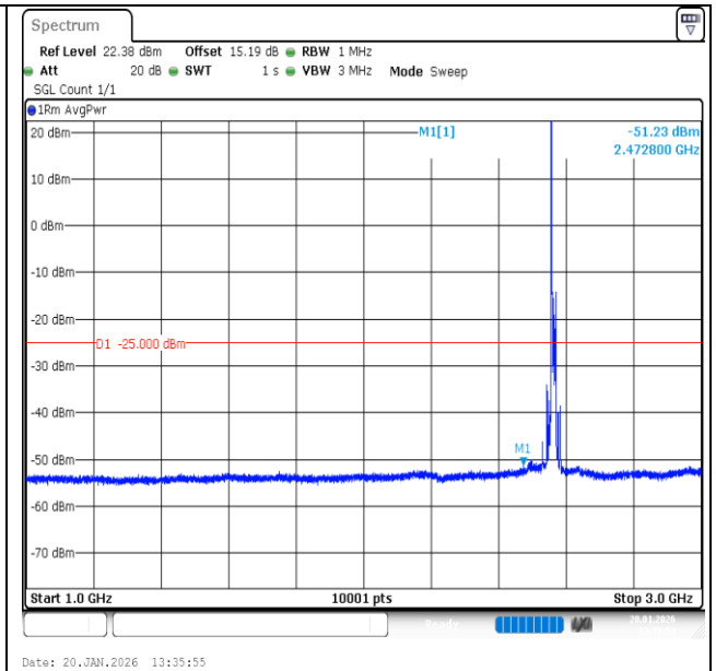
Band7-15MHz-16QAM-21375-1RB#0-1000~3000-PASS
