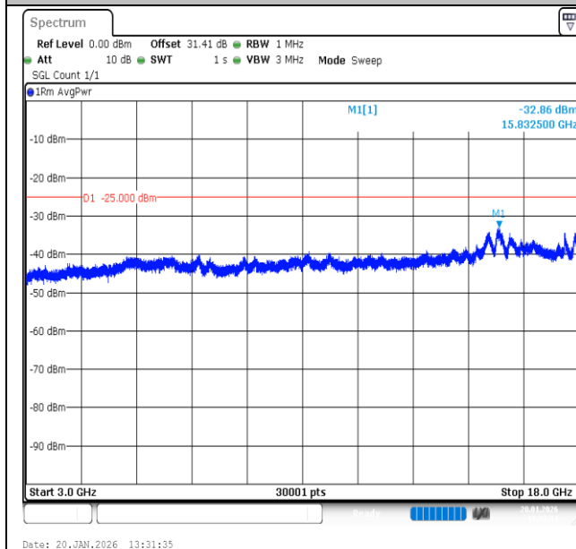
Band7-15MHz-QPSK-21100-1RB#0-3000~18000-PASS
