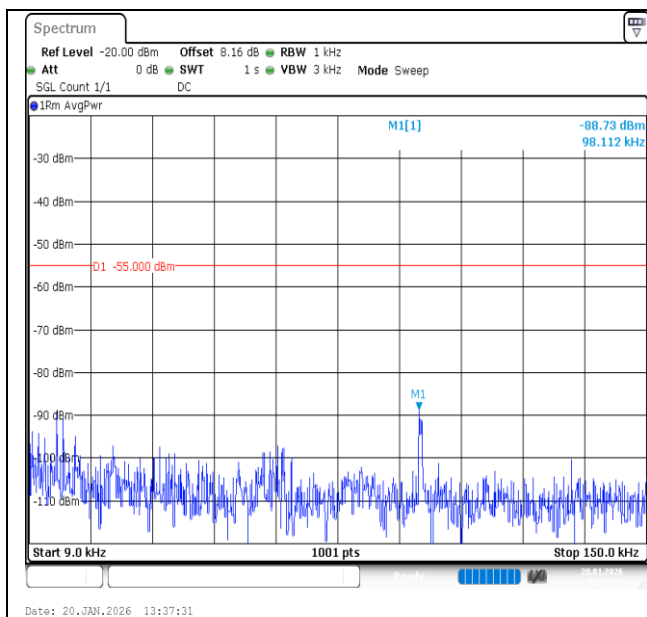
Band7-15MHz-QPSK-21375-75RB#0-0.009~0.15-PASS
