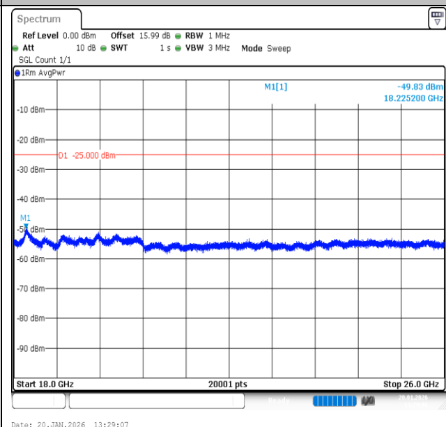
Band7-15MHz-QPSK-20825-1RB#74-18000~26000-PASS
