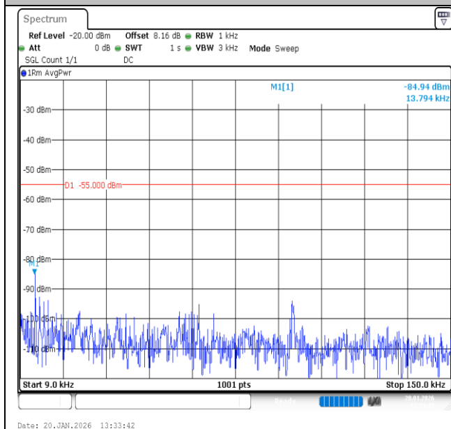
Band7-15MHz-QPSK-21100-75RB#0-0.009~0.15-PASS
