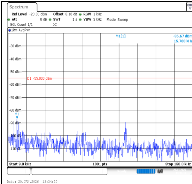
Band7-15MHz-16QAM-21100-75RB#0-0.009~0.15-PASS
