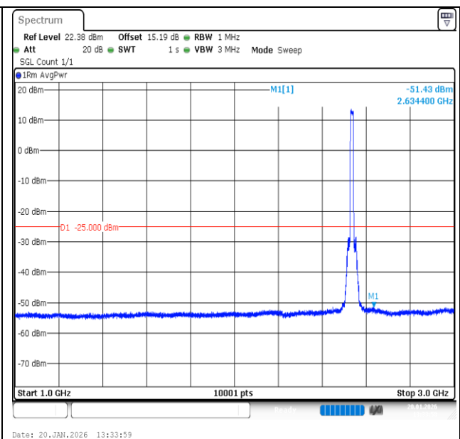
Band7-15MHz-QPSK-21100-75RB#0-1000~3000-PASS
