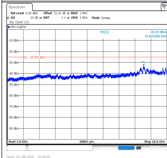
Band7-15MHz-QPSK-21375-1RB#74-3000~18000-PASS
