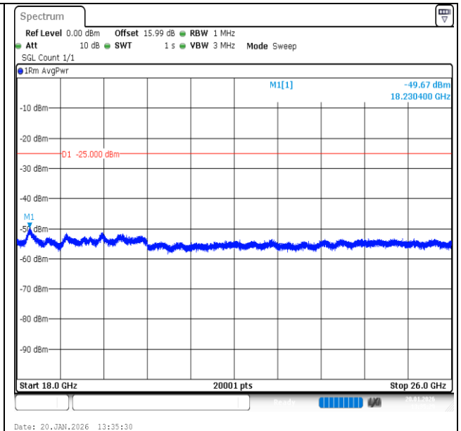
Band7-15MHz-QPSK-21375-1RB#0-18000~26000-PASS
