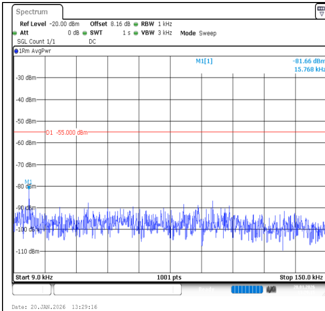
Band7-15MHz-16QAM-20825-1RB#74-0.009~0.15-PASS
