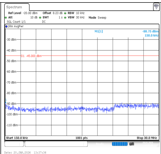
Band7-15MHz-QPSK-21375-75RB#0-0.15~30-PASS
