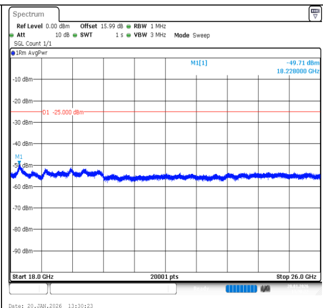
Band7-15MHz-QPSK-20825-75RB#0-18000~26000-PASS
