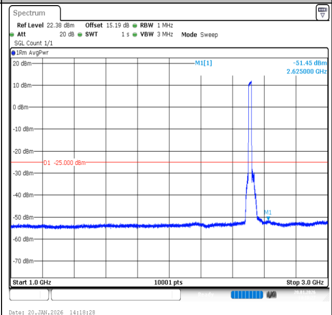
Band7-20MHz-QPSK-20850-100RB#0-1000~3000-PASS
