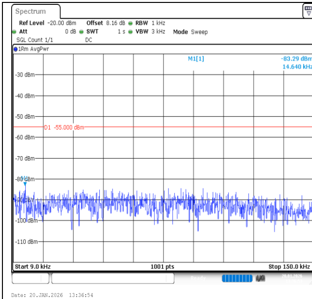
Band7-15MHz-16QAM-21375-1RB#74-0.009~0.15-PASS
