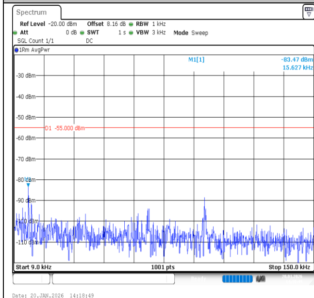
Band7-20MHz-16QAM-20850-100RB#0-0.009~0.15-PASS
