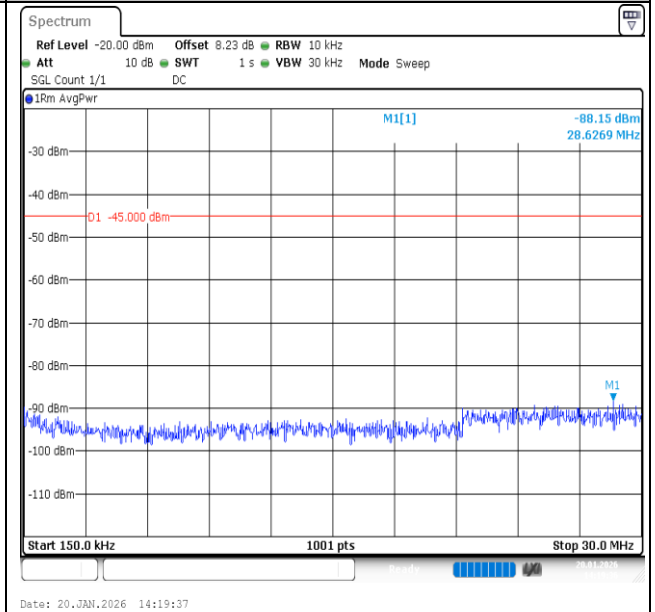
Band7-20MHz-QPSK-21100-1RB#0-0.15~30-PASS
