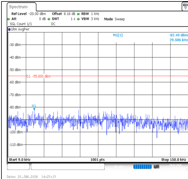
Band7-20MHz-16QAM-21350-1RB#99-0.009~0.15-PASS
