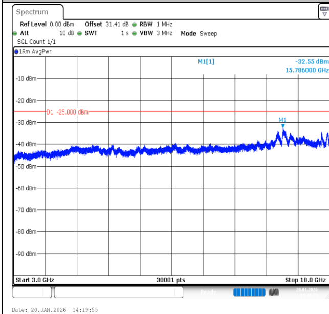
Band7-20MHz-QPSK-21100-1RB#0-3000~18000-PASS
