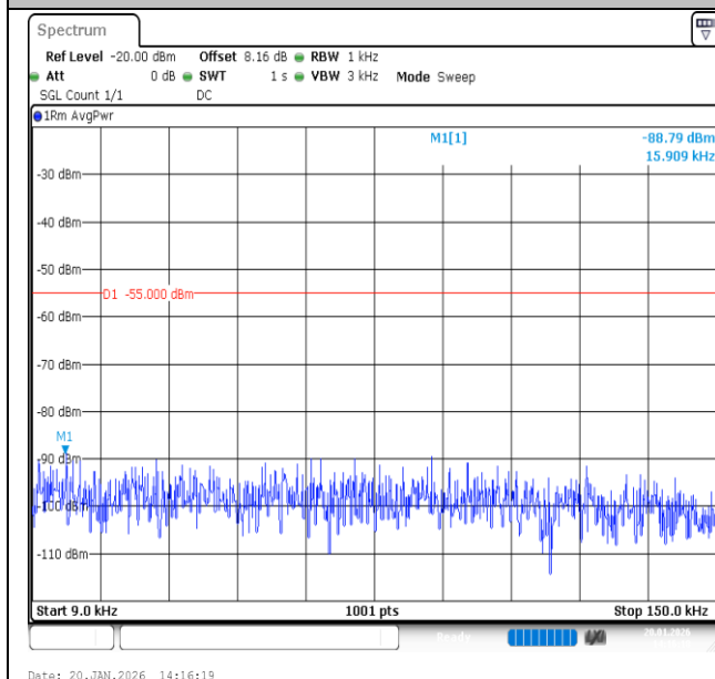
Band7-20MHz-16QAM-20850-1RB#0-0.009~0.15-PASS
