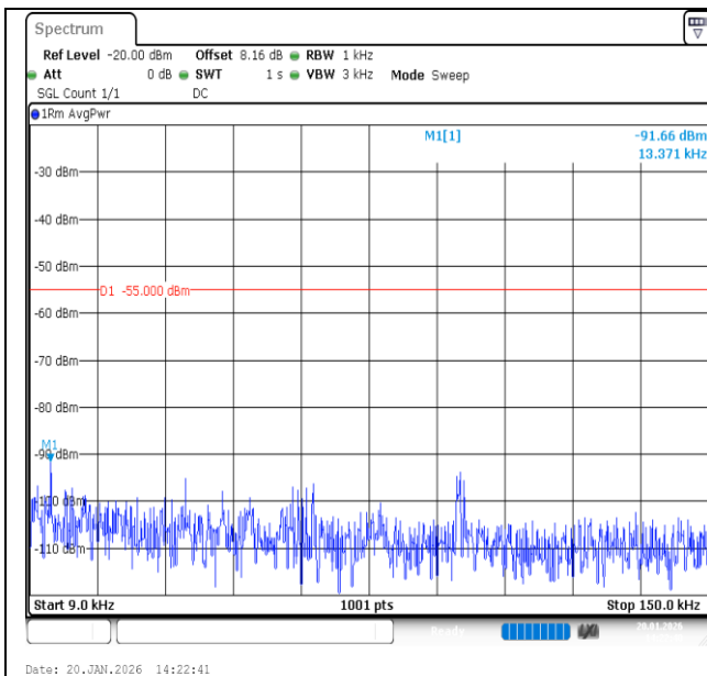
Band7-20MHz-16QAM-21100-100RB#0-0.009~0.15-PASS
