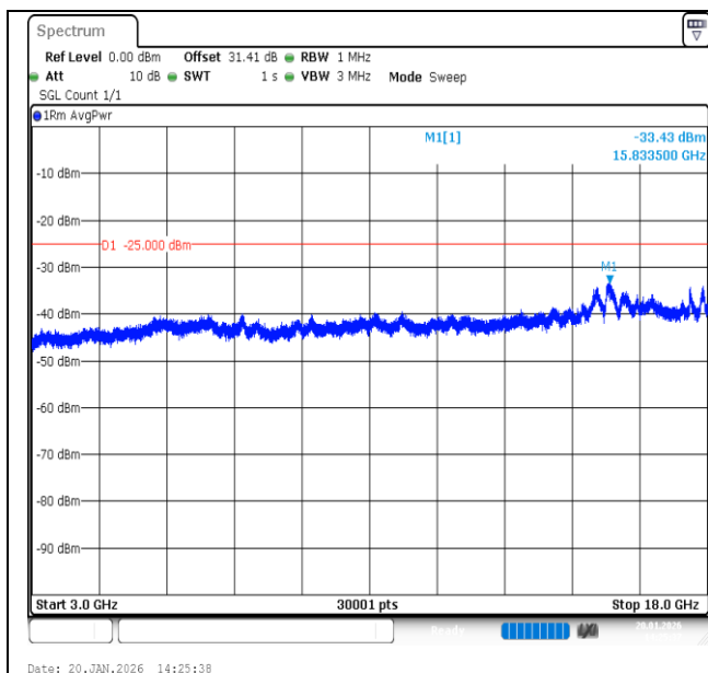
Band7-20MHz-16QAM-21350-1RB#99-3000~18000-PASS
