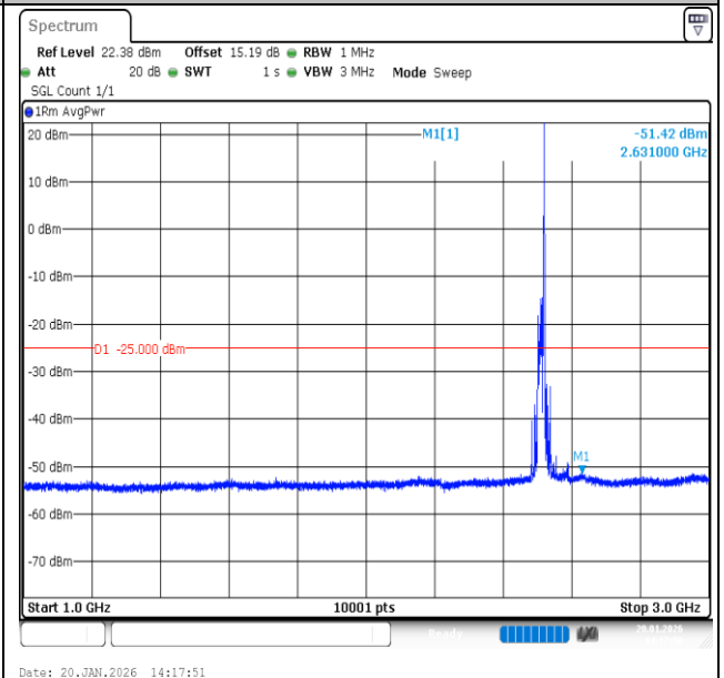
Band7-20MHz-16QAM-20850-1RB#99-1000~3000-PASS
