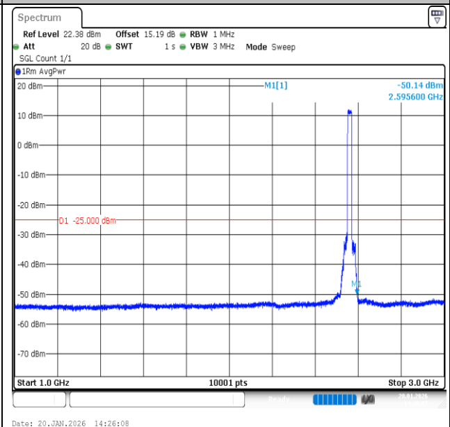
Band7-20MHz-QPSK-21350-100RB#0-1000~3000-PASS
