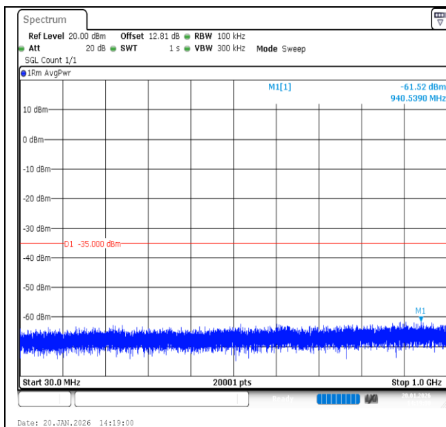
Band7-20MHz-16QAM-20850-100RB#0-30~1000-PASS
