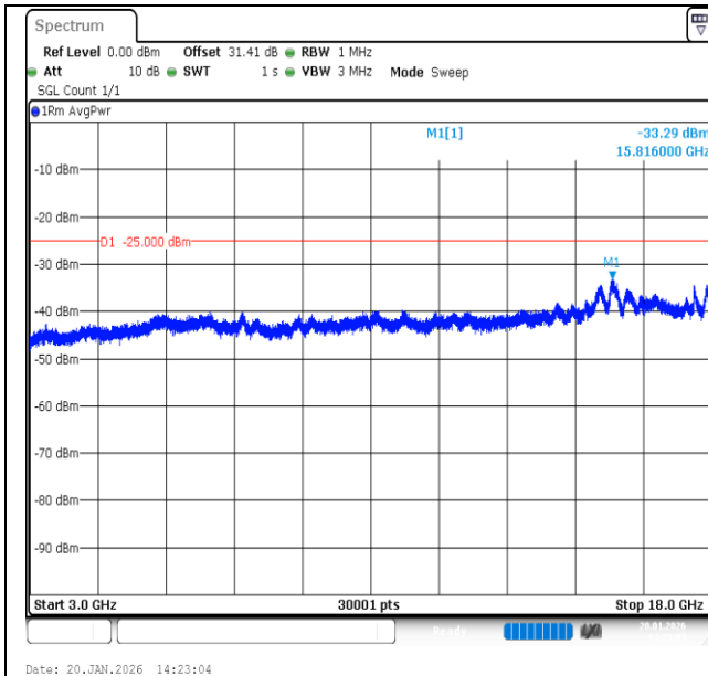
Band7-20MHz-16QAM-21100-100RB#0-3000~18000-PASS
