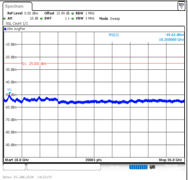
Band7-20MHz-QPSK-21350-1RB#0-18000~26000-PASS
