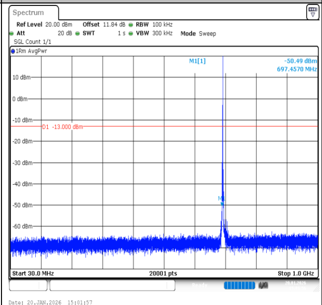
Band12-1.4MHz-QPSK-23017-1RB#5-30~1000-PASS
