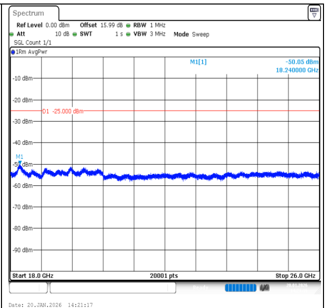
Band7-20MHz-QPSK-21100-1RB#99-18000~26000-PASS
