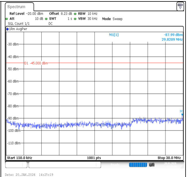
Band7-20MHz-16QAM-21350-1RB#99-0.15~30-PASS
