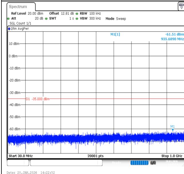
Band7-20MHz-16QAM-21100-100RB#0-30~1000-PASS
