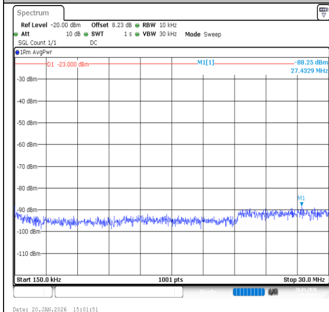
Band12-1.4MHz-QPSK-23017-1RB#5-0.15~30-PASS
