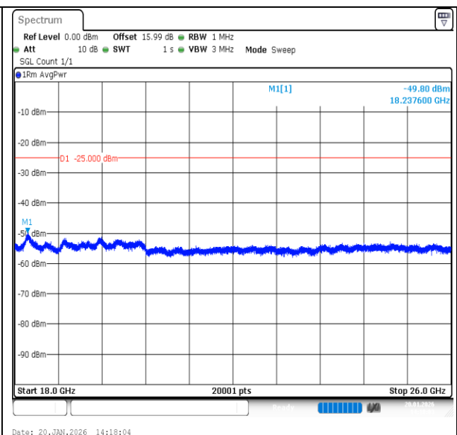
Band7-20MHz-16QAM-20850-1RB#99-18000~26000-PASS
