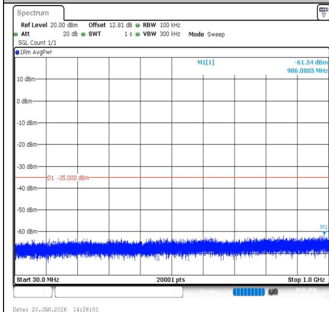
Band7-20MHz-QPSK-21350-100RB#0-30~1000-PASS
