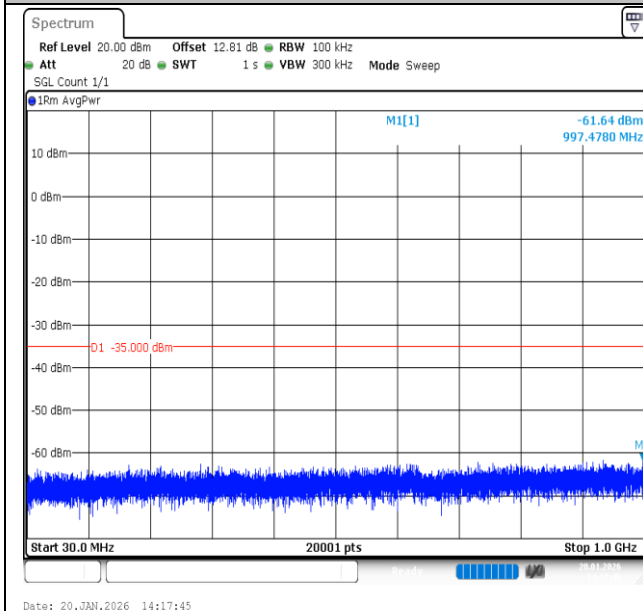
Band7-20MHz-16QAM-20850-1RB#99-30~1000-PASS
