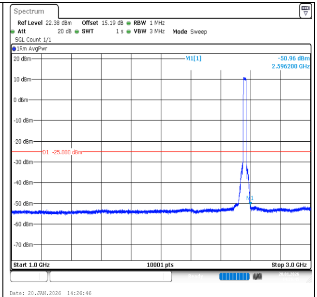
Band7-20MHz-16QAM-21350-100RB#0-1000~3000-PASS
