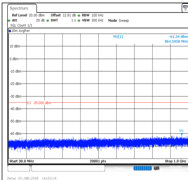
Band7-20MHz-QPSK-21100-100RB#0-30~1000-PASS
