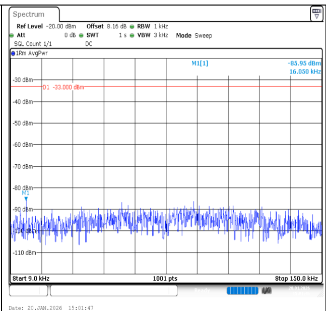
Band12-1.4MHz-QPSK-23017-1RB#5-0.009~0.15-PASS
