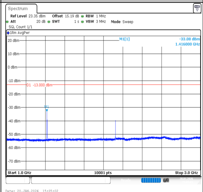
Band12-1.4MHz-QPSK-23095-1RB#5-1000~3000-PASS
