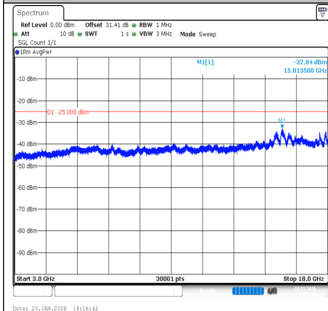
Band7-20MHz-16QAM-20850-1RB#0-3000~18000-PASS
