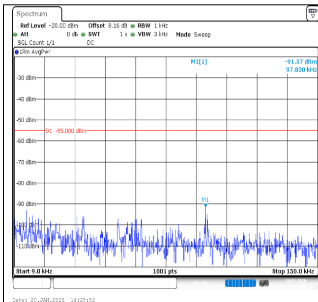
Band7-20MHz-QPSK-21350-100RB#0-0.009~0.15-PASS
