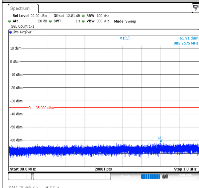
Band7-20MHz-QPSK-21350-1RB#0-30~1000-PASS
