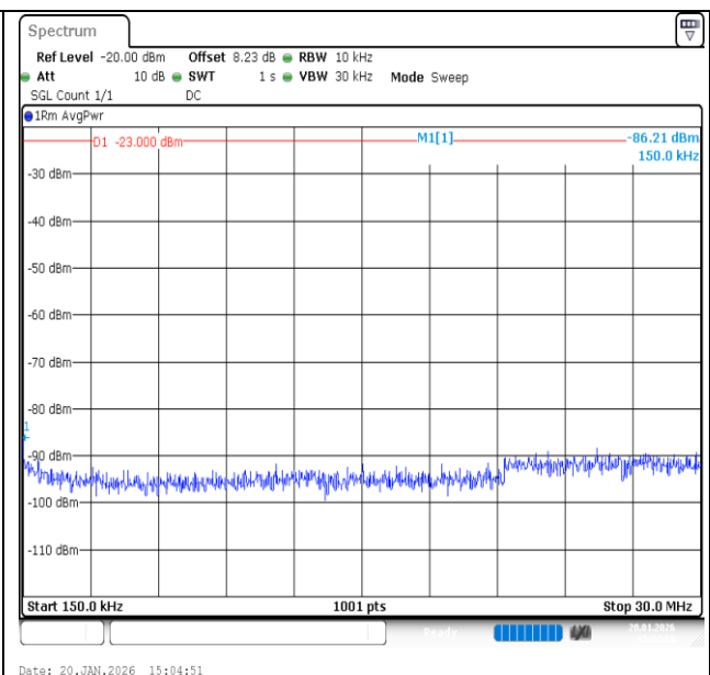
Band12-1.4MHz-QPSK-23095-1RB#5-0.15~30-PASS
