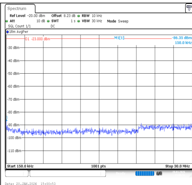
Band12-1.4MHz-QPSK-23017-1RB#0-0.15~30-PASS
