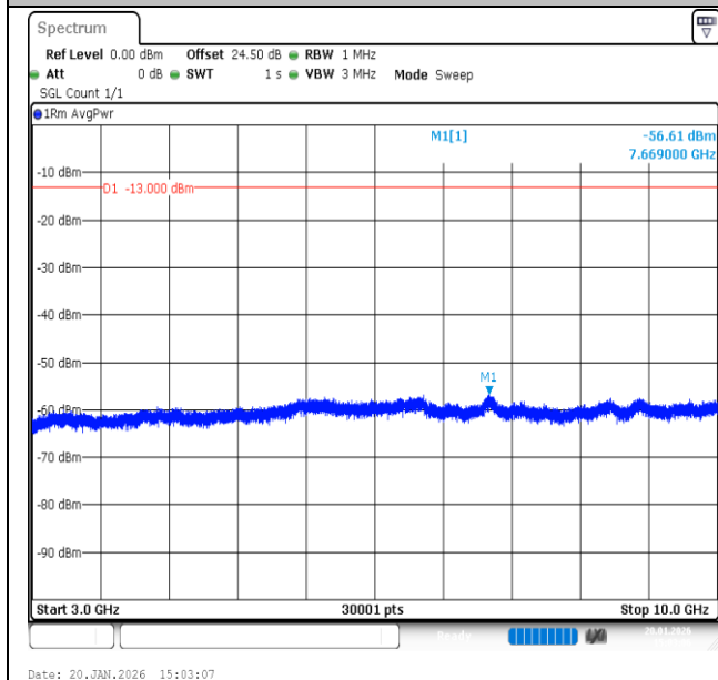
Band12-1.4MHz-QPSK-23017-6RB#0-3000~10000-PASS
