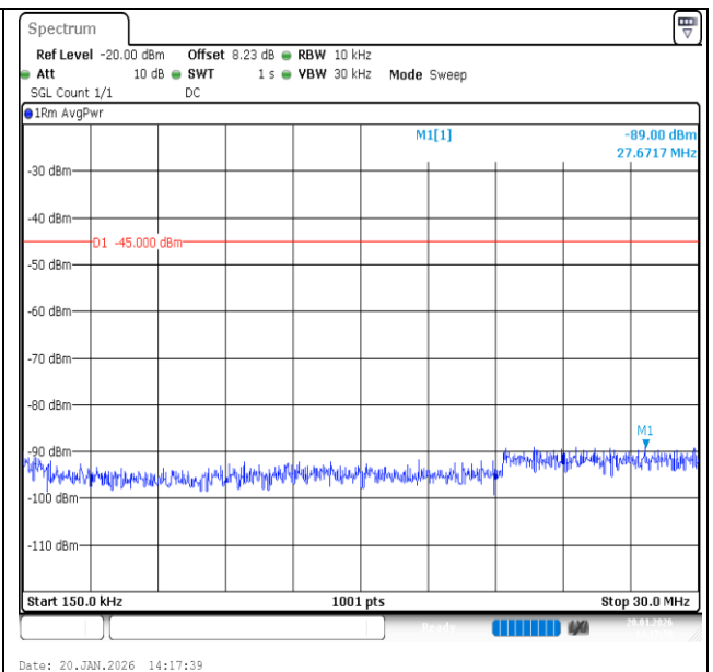
Band7-20MHz-16QAM-20850-1RB#99-0.15~30-PASS
