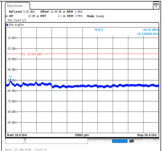
Band7-20MHz-16QAM-21100-100RB#0-18000~26000-PASS
