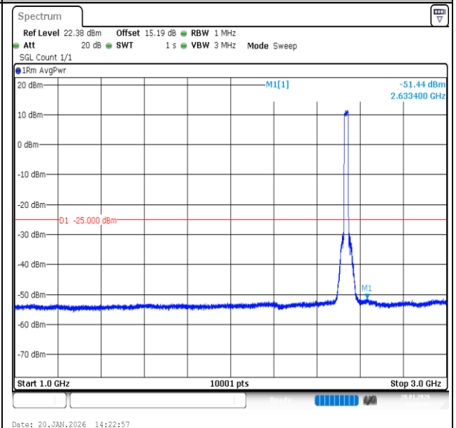
Band7-20MHz-16QAM-21100-100RB#0-1000~3000-PASS
