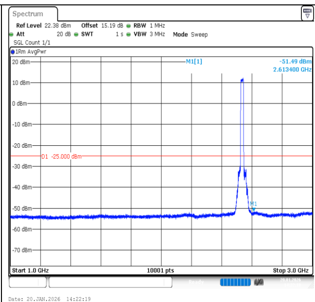
Band7-20MHz-QPSK-21100-100RB#0-1000~3000-PASS
