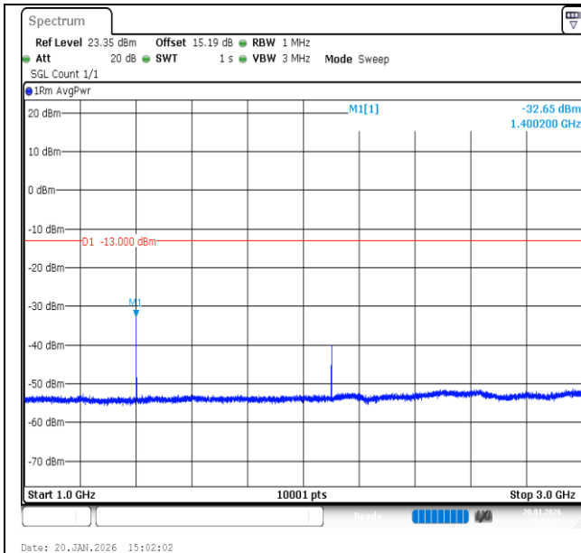
Band12-1.4MHz-QPSK-23017-1RB#5-1000~3000-PASS
