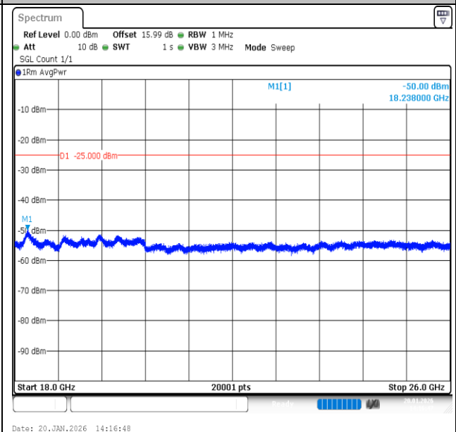
Band7-20MHz-16QAM-20850-1RB#0-18000~26000-PASS
