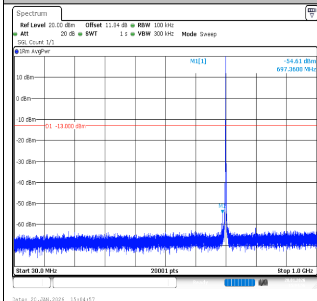
Band12-1.4MHz-QPSK-23095-1RB#5-30~1000-PASS
