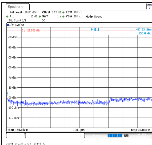
Band12-1.4MHz-QPSK-23095-1RB#0-0.15~30-PASS
