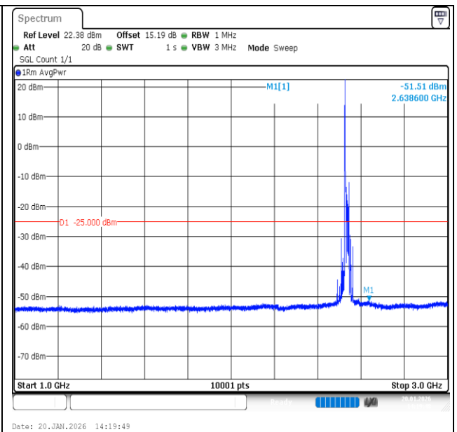
Band7-20MHz-QPSK-21100-1RB#0-1000~3000-PASS
