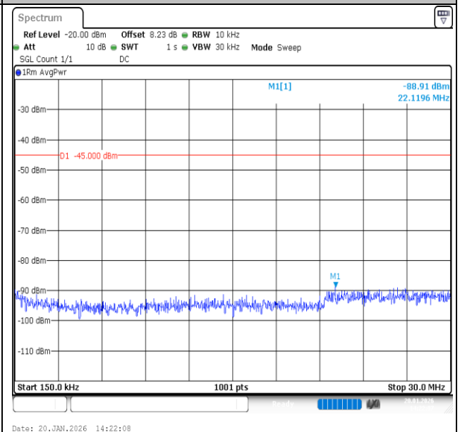
Band7-20MHz-QPSK-21100-100RB#0-0.15~30-PASS
