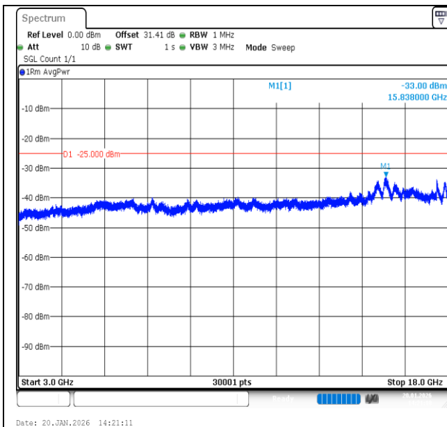
Band7-20MHz-QPSK-21100-1RB#99-3000~18000-PASS
