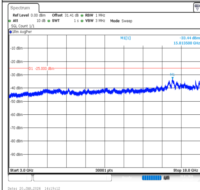
Band7-20MHz-16QAM-20850-100RB#0-3000~18000-PASS
