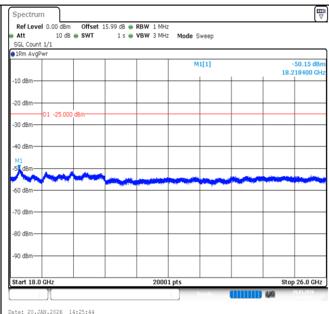
Band7-20MHz-16QAM-21350-1RB#99-18000~26000-PASS
