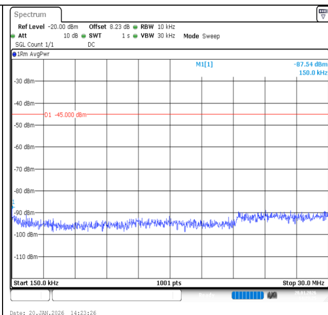
Band7-20MHz-QPSK-21350-1RB#0-0.15~30-PASS
