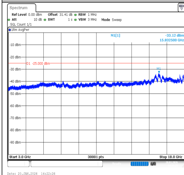
Band7-20MHz-QPSK-21100-100RB#0-3000~18000-PASS
