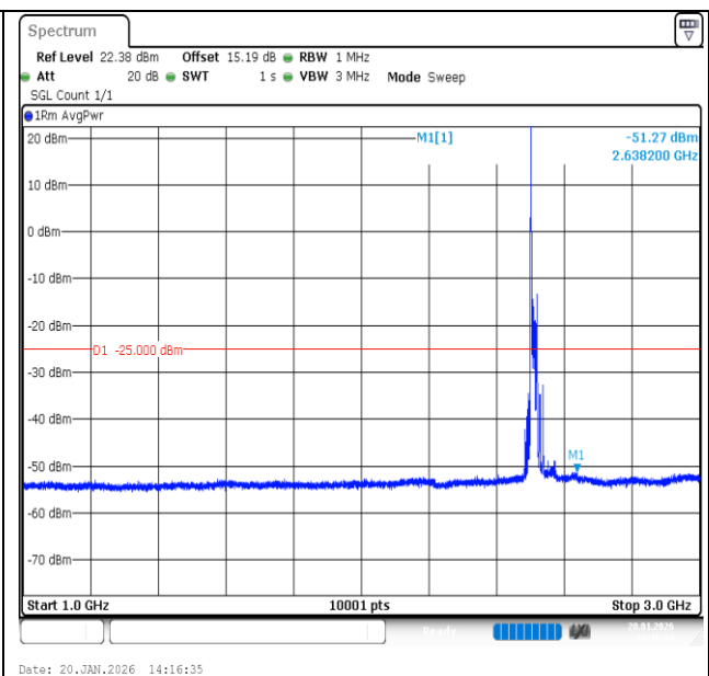
Band7-20MHz-16QAM-20850-1RB#0-1000~3000-PASS
