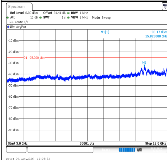
Band7-20MHz-16QAM-21350-100RB#0-3000~18000-PASS
