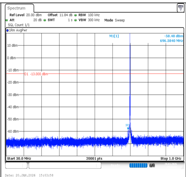
Band12-1.4MHz-QPSK-23095-1RB#0-30~1000-PASS
