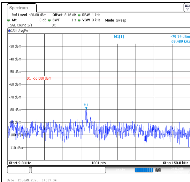
Band7-20MHz-16QAM-20850-1RB#99-0.009~0.15-PASS
