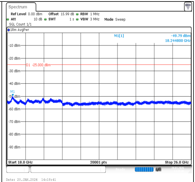
Band7-20MHz-QPSK-20850-100RB#0-18000~26000-PASS
