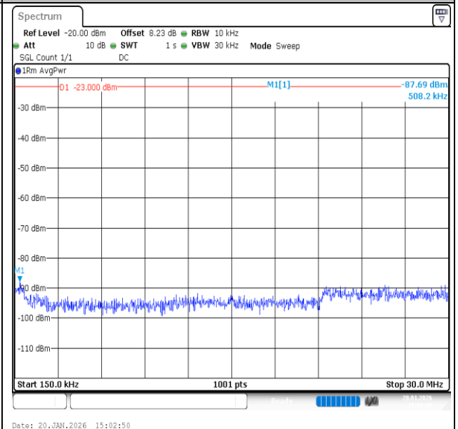
Band12-1.4MHz-QPSK-23017-6RB#0-0.15~30-PASS
