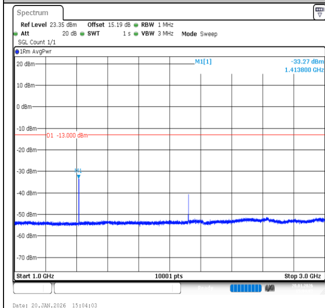
Band12-1.4MHz-QPSK-23095-1RB#0-1000~3000-PASS
