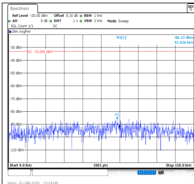
Band12-1.4MHz-QPSK-23095-1RB#5-0.009~0.15-PASS
