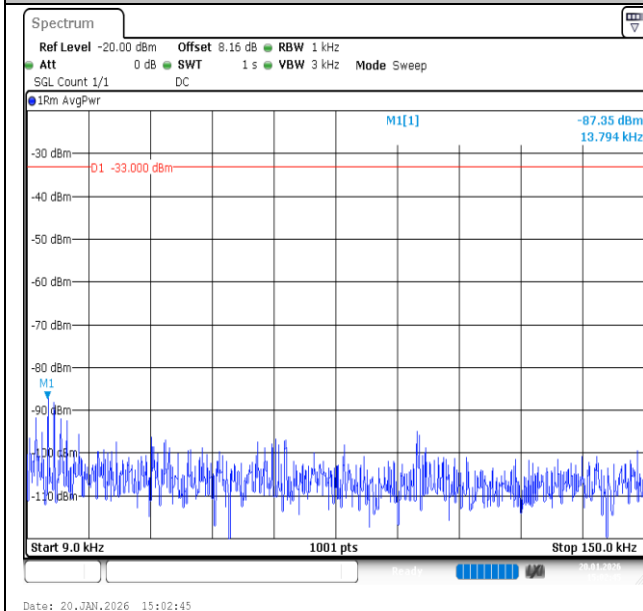
Band12-1.4MHz-QPSK-23017-6RB#0-0.009~0.15-PASS
