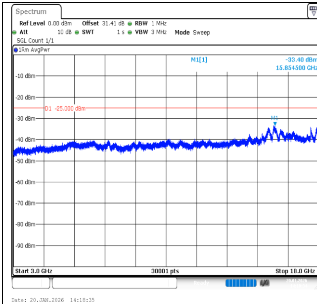
Band7-20MHz-QPSK-20850-100RB#0-3000~18000-PASS
