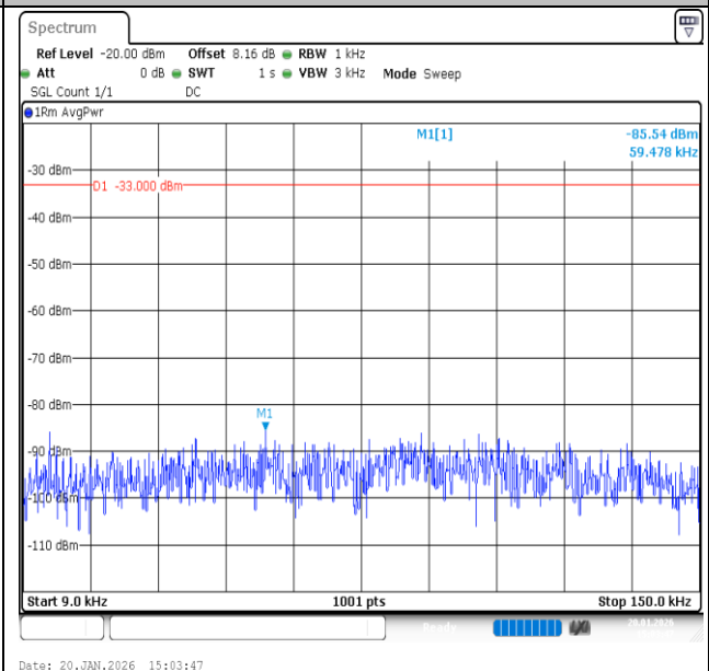
Band12-1.4MHz-QPSK-23095-1RB#0-0.009~0.15-PASS
