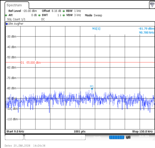
Band7-20MHz-QPSK-21350-1RB#99-0.009~0.15-PASS
