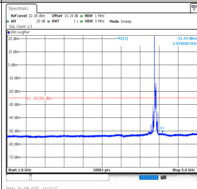
Band7-20MHz-QPSK-21350-1RB#0-1000~3000-PASS
