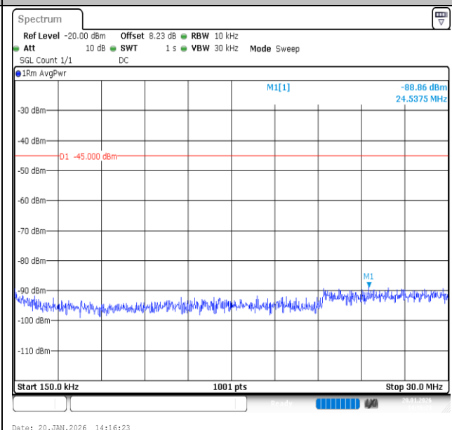
Band7-20MHz-16QAM-20850-1RB#0-0.15~30-PASS
