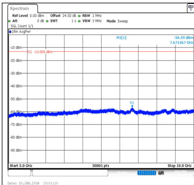
Band12-1.4MHz-QPSK-23017-1RB#0-3000~10000-PASS
