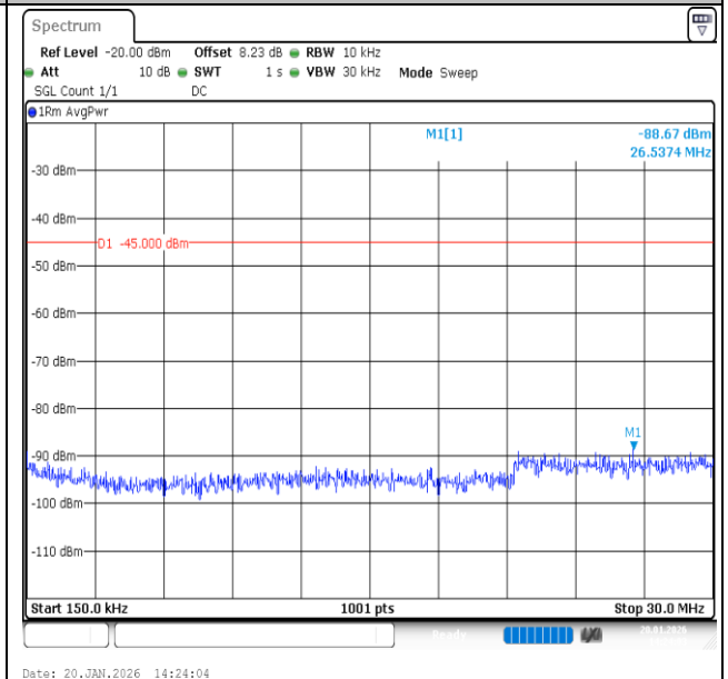
Band7-20MHz-16QAM-21350-1RB#0-0.15~30-PASS
