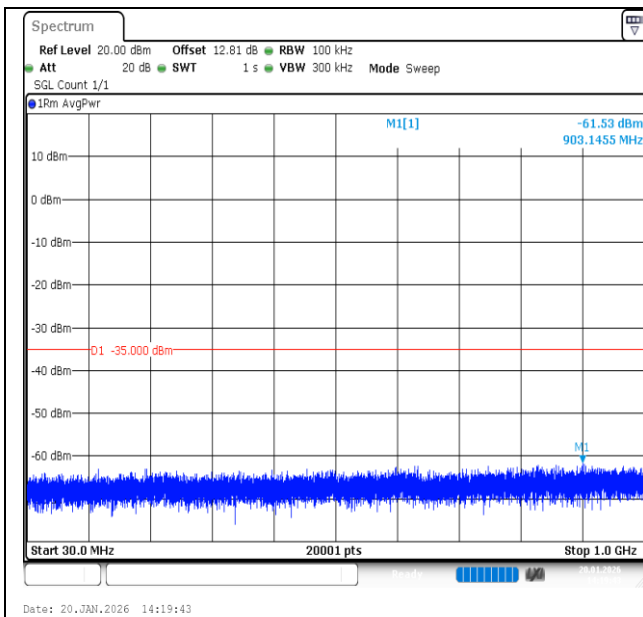
Band7-20MHz-QPSK-21100-1RB#0-30~1000-PASS
