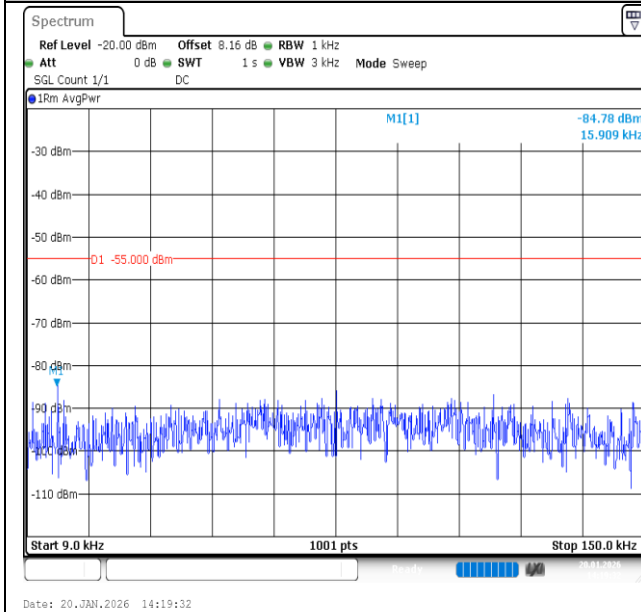
Band7-20MHz-QPSK-21100-1RB#0-0.009~0.15-PASS
