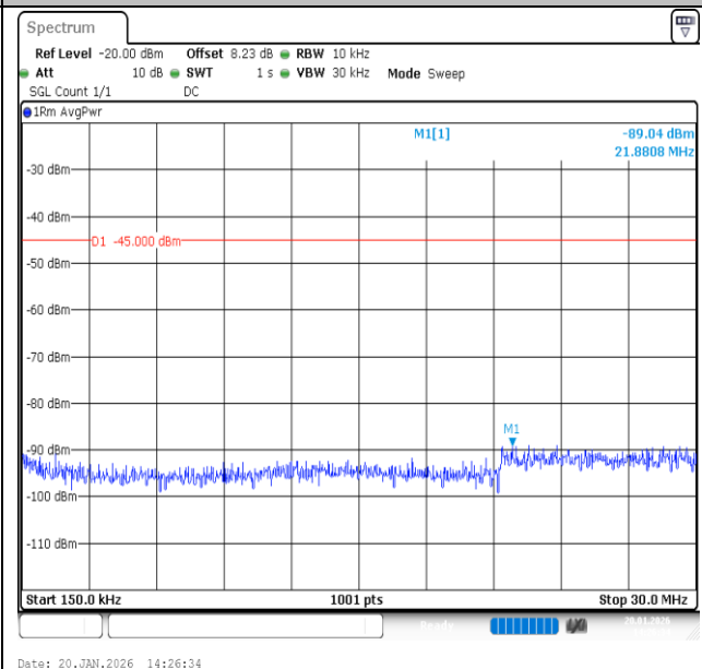
Band7-20MHz-16QAM-21350-100RB#0-0.15~30-PASS
