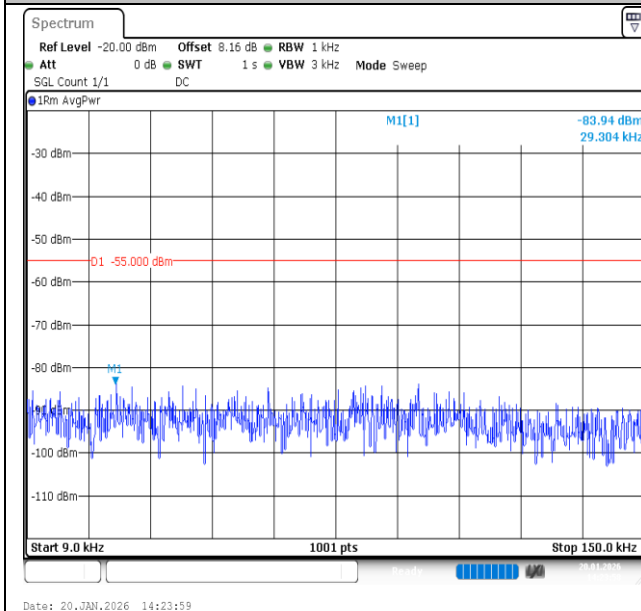
Band7-20MHz-16QAM-21350-1RB#0-0.009~0.15-PASS
