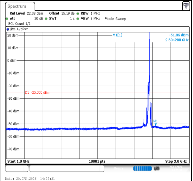
Band7-20MHz-16QAM-21350-1RB#99-1000~3000-PASS
