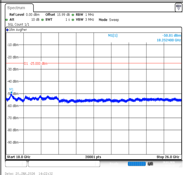
Band7-20MHz-QPSK-21100-100RB#0-18000~26000-PASS
