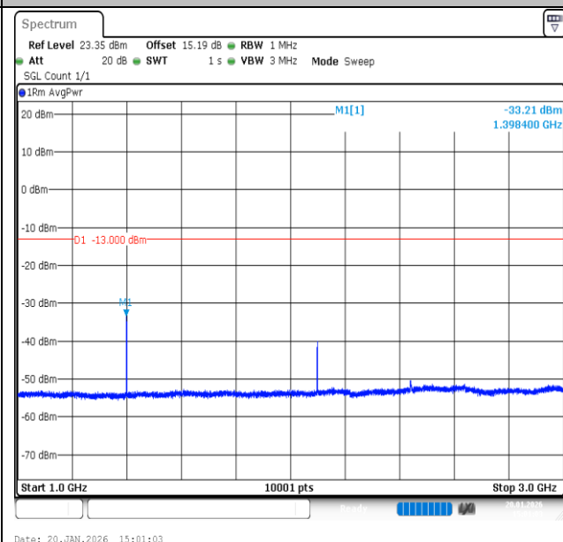
Band12-1.4MHz-QPSK-23017-1RB#0-1000~3000-PASS
