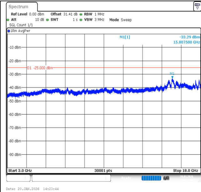
Band7-20MHz-QPSK-21350-1RB#0-3000~18000-PASS
