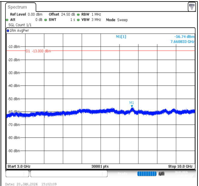
Band12-1.4MHz-QPSK-23017-1RB#5-3000~10000-PASS
