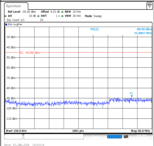
Band7-20MHz-16QAM-20850-100RB#0-0.15~30-PASS
