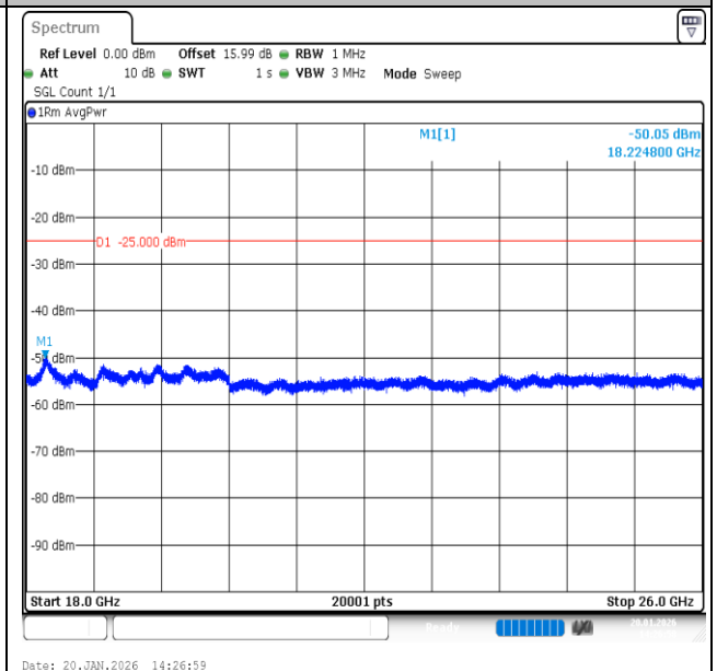
Band7-20MHz-16QAM-21350-100RB#0-18000~26000-PASS
