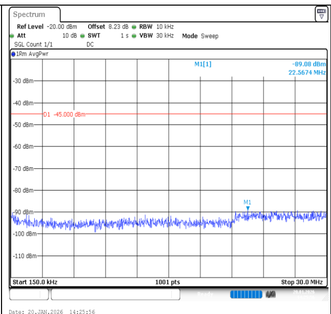
Band7-20MHz-QPSK-21350-100RB#0-0.15~30-PASS
