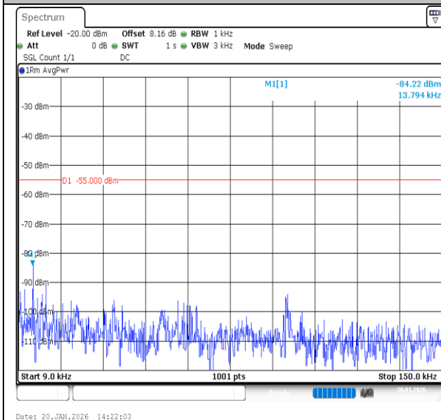
Band7-20MHz-QPSK-21100-100RB#0-0.009~0.15-PASS
