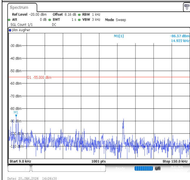
Band7-20MHz-16QAM-21350-100RB#0-0.009~0.15-PASS
