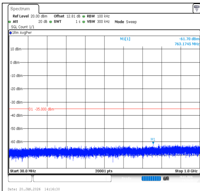
Band7-20MHz-16QAM-20850-1RB#0-30~1000-PASS
