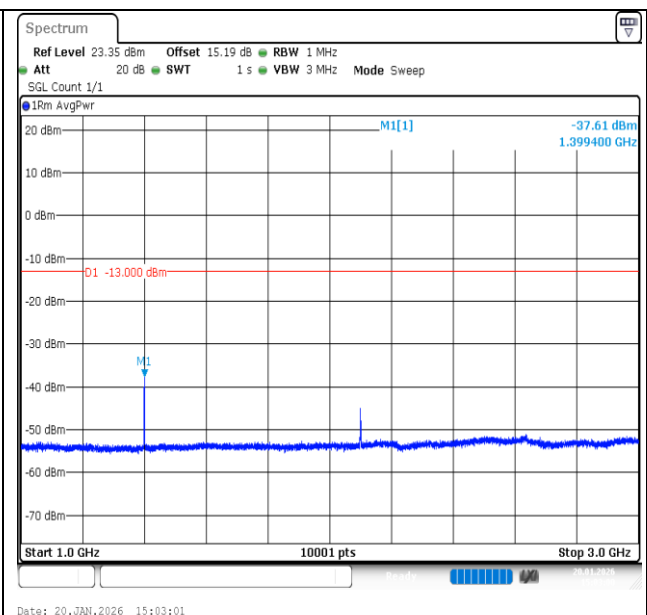
Band12-1.4MHz-QPSK-23017-6RB#0-1000~3000-PASS
