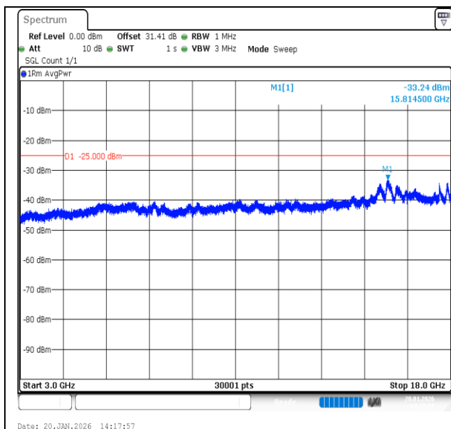
Band7-20MHz-16QAM-20850-1RB#99-3000~18000-PASS
