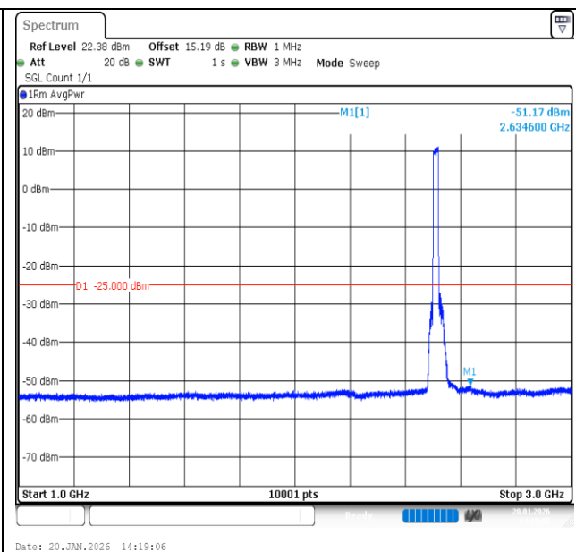
Band7-20MHz-16QAM-20850-100RB#0-1000~3000-PASS
