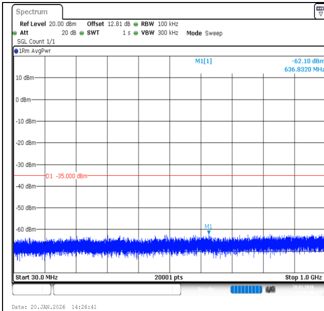
Band7-20MHz-16QAM-21350-100RB#0-30~1000-PASS
