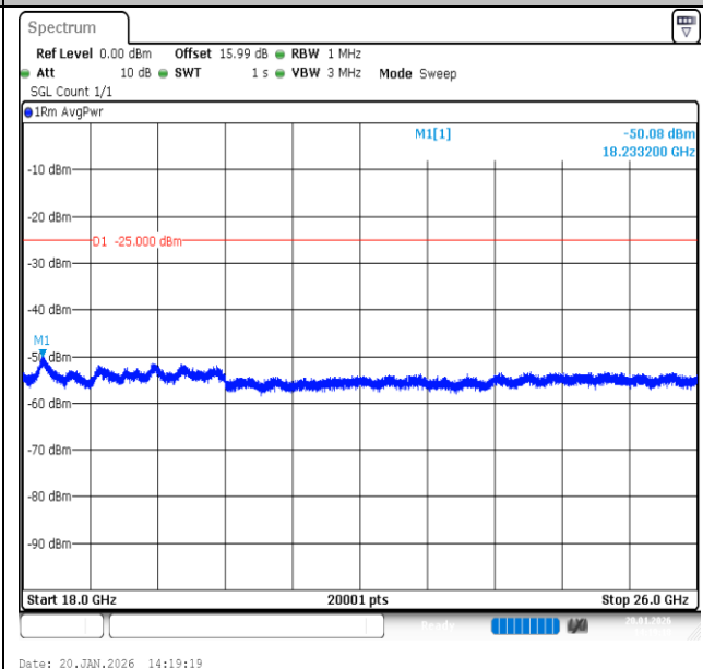
Band7-20MHz-16QAM-20850-100RB#0-18000~26000-PASS
