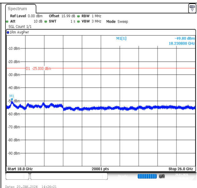
Band7-20MHz-QPSK-21350-100RB#0-18000~26000-PASS
