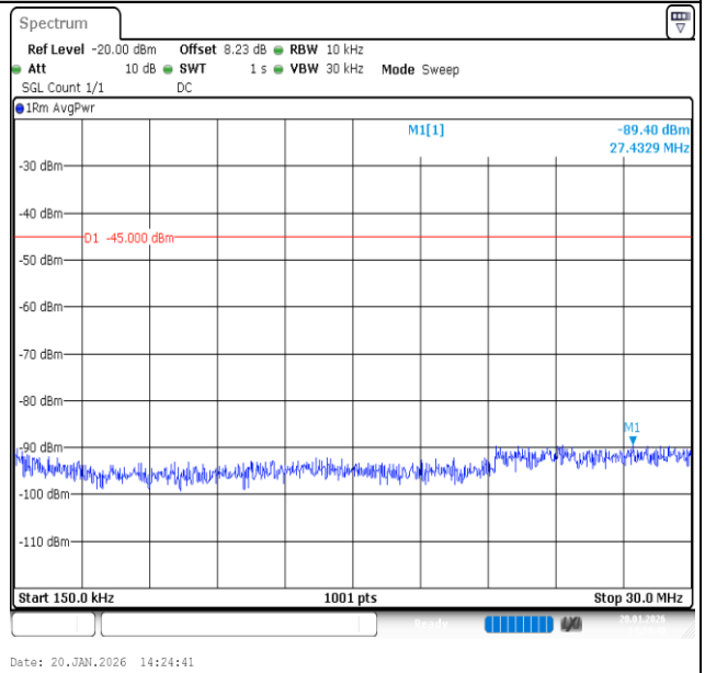
Band7-20MHz-QPSK-21350-1RB#99-0.15~30-PASS
