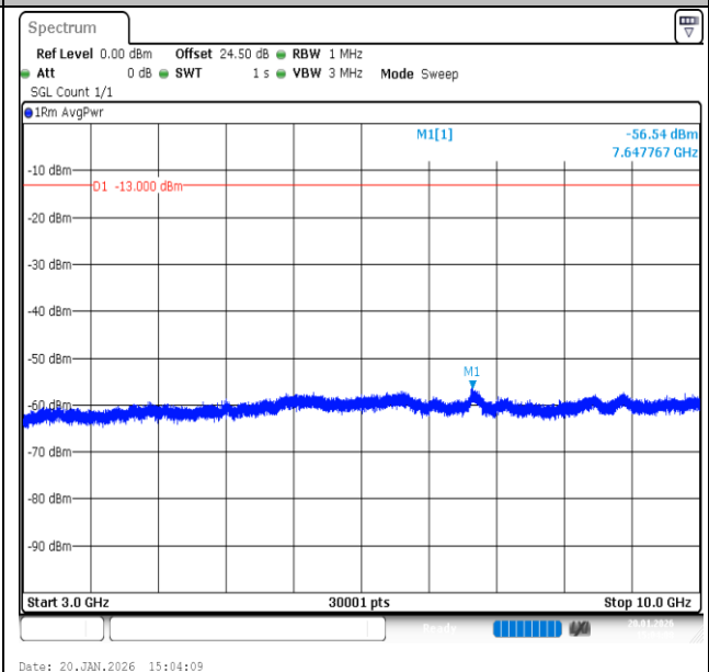
Band12-1.4MHz-QPSK-23095-1RB#0-3000~10000-PASS
