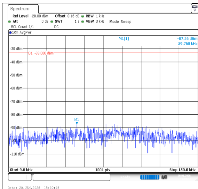
Band12-1.4MHz-QPSK-23017-1RB#0-0.009~0.15-PASS
