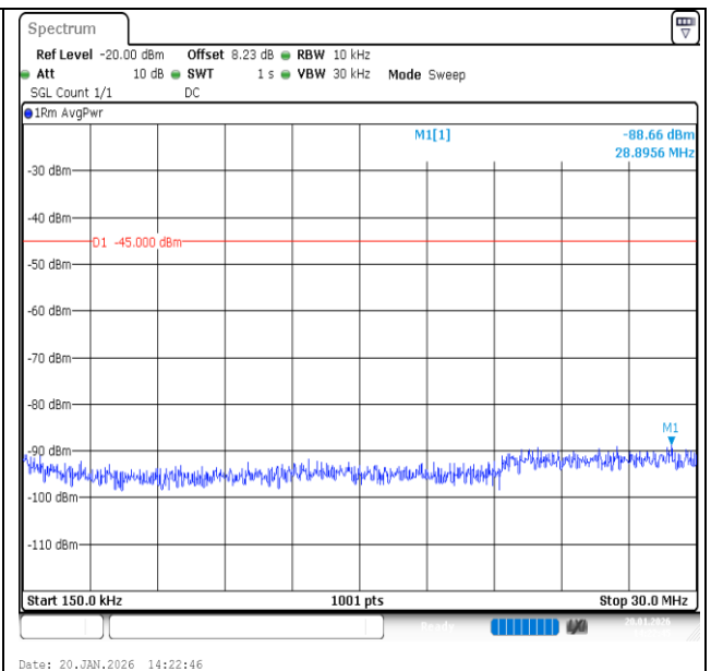
Band7-20MHz-16QAM-21100-100RB#0-0.15~30-PASS
