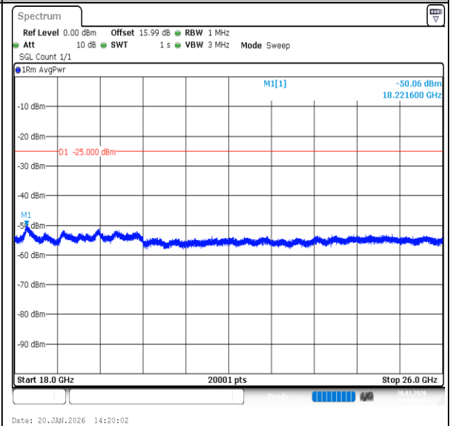
Band7-20MHz-QPSK-21100-1RB#0-18000~26000-PASS
