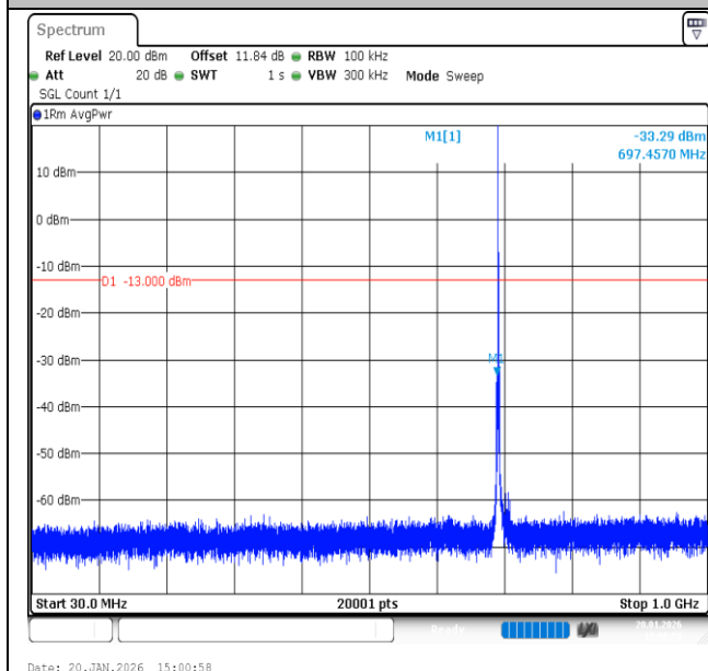
Band12-1.4MHz-QPSK-23017-1RB#0-30~1000-PASS
