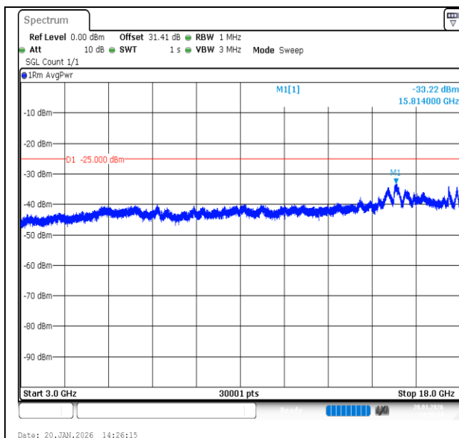
Band7-20MHz-QPSK-21350-100RB#0-3000~18000-PASS
