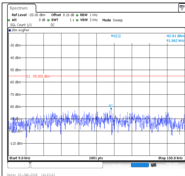
Band7-20MHz-QPSK-21350-1RB#0-0.009~0.15-PASS
