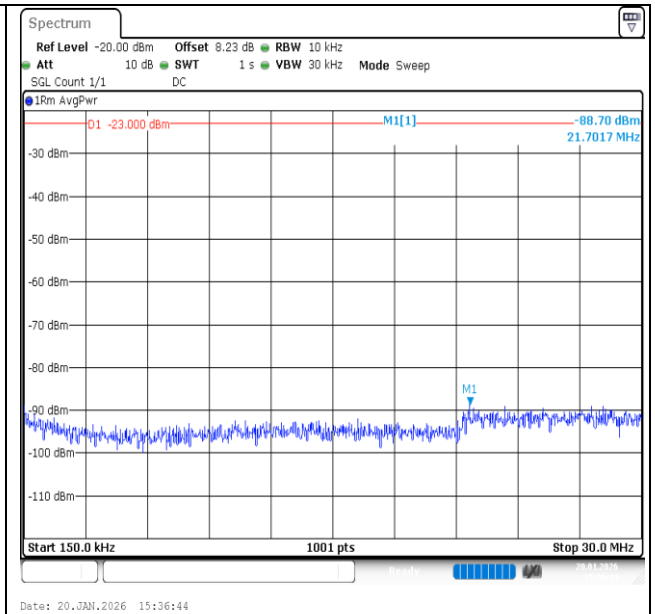
Band12-3MHz-QPSK-23165-1RB#0-0.15~30-PASS
