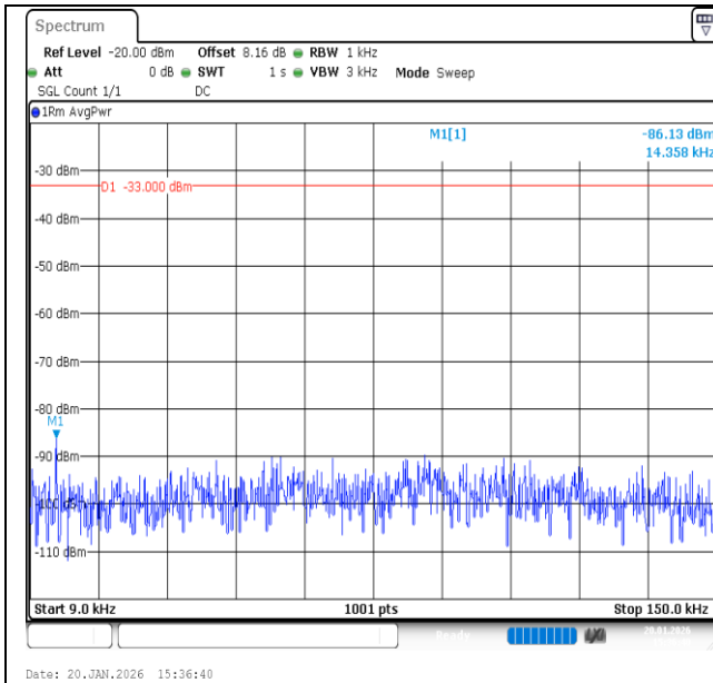
Band12-3MHz-QPSK-23165-1RB#0-0.009~0.15-PASS
