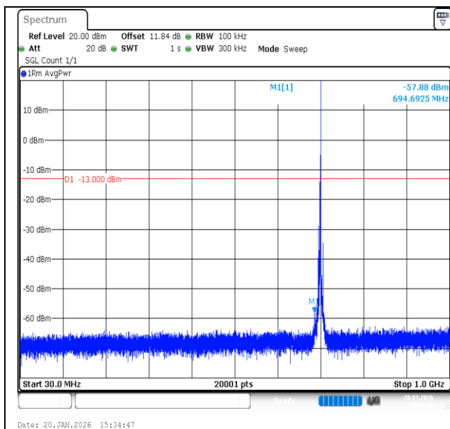
Band12-3MHz-QPSK-23095-1RB#14-30~1000-PASS
