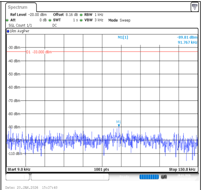
Band12-3MHz-QPSK-23165-1RB#14-0.009~0.15-PASS
