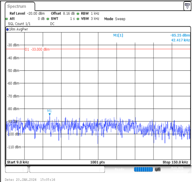
Band12-1.4MHz-16QAM-23095-1RB#5-0.009~0.15-PASS
