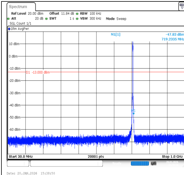
Band12-3MHz-QPSK-23165-15RB#0-30~1000-PASS
