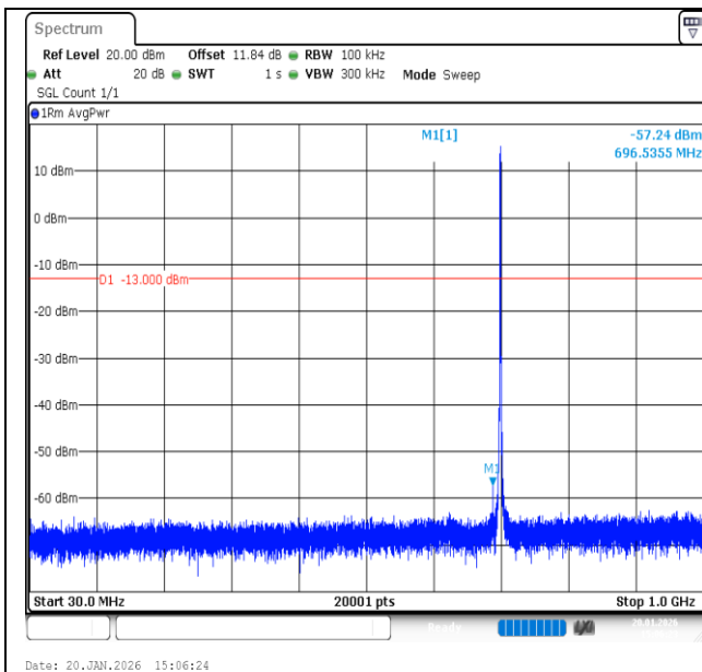
Band12-1.4MHz-16QAM-23095-6RB#0-30~1000-PASS
