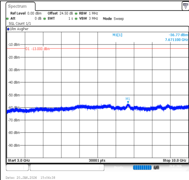
Band12-1.4MHz-16QAM-23095-1RB#0-3000~10000-PASS
