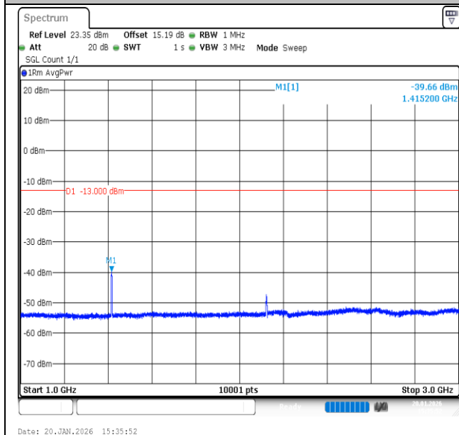
Band12-3MHz-QPSK-23095-15RB#0-1000~3000-PASS
