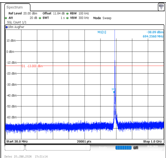
Band12-3MHz-16QAM-23025-1RB#0-30~1000-PASS
