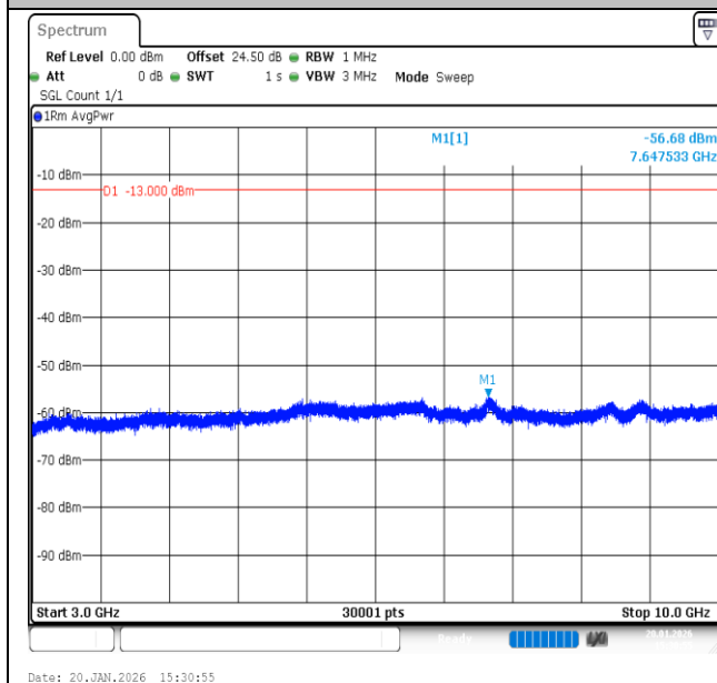
Band12-3MHz-QPSK-23025-1RB#0-3000~10000-PASS
