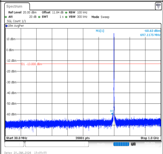
Band12-1.4MHz-QPSK-23095-6RB#0-30~1000-PASS
