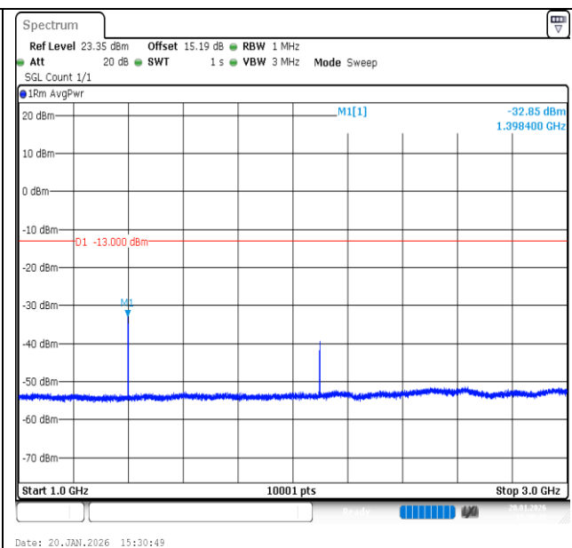
Band12-3MHz-QPSK-23025-1RB#0-1000~3000-PASS
