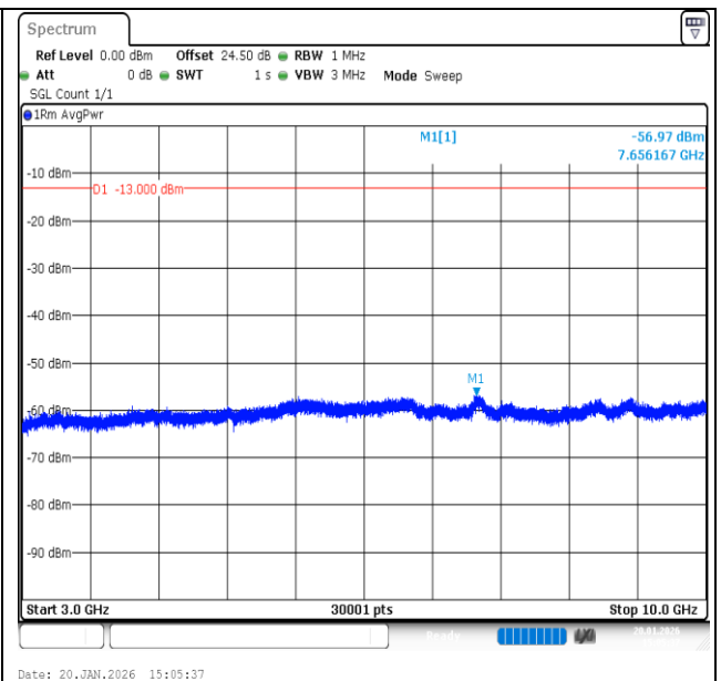
Band12-1.4MHz-16QAM-23095-1RB#5-3000~10000-PASS
