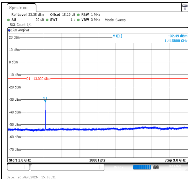
Band12-1.4MHz-16QAM-23095-1RB#5-1000~3000-PASS
