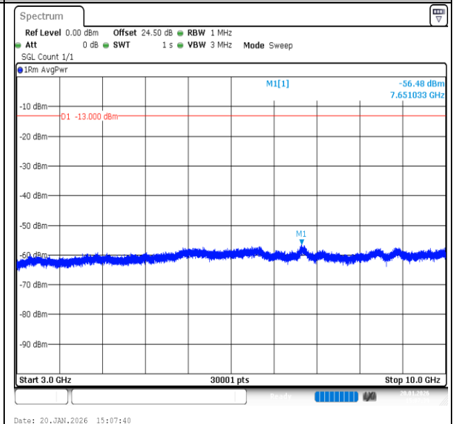
Band12-1.4MHz-16QAM-23173-1RB#0-3000~10000-PASS
