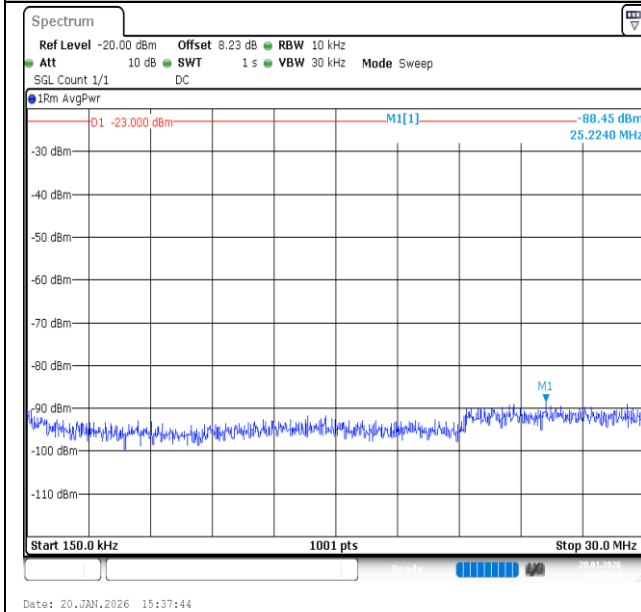
Band12-3MHz-QPSK-23165-1RB#14-0.15~30-PASS
