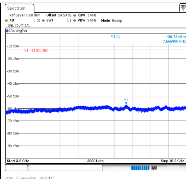
Band12-1.4MHz-16QAM-23173-6RB#0-3000~10000-PASS
