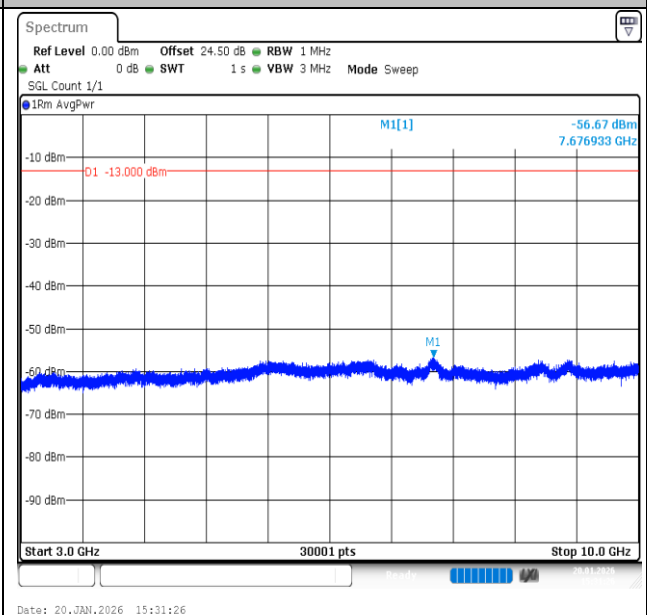
Band12-3MHz-16QAM-23025-1RB#0-3000~10000-PASS
