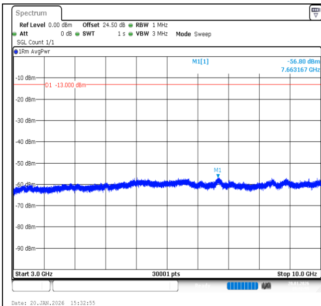
Band12-3MHz-QPSK-23025-15RB#0-3000~10000-PASS
