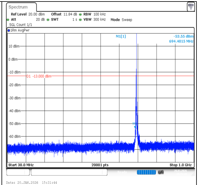
Band12-3MHz-QPSK-23025-1RB#14-30~1000-PASS
