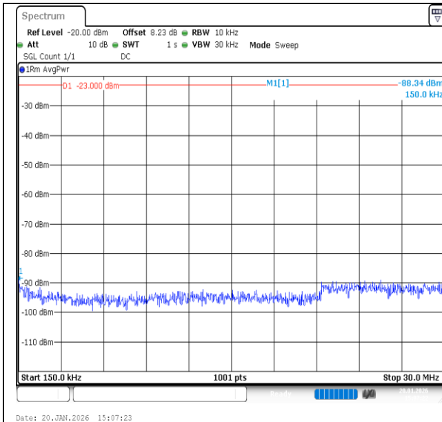
Band12-1.4MHz-16QAM-23173-1RB#0-0.15~30-PASS
