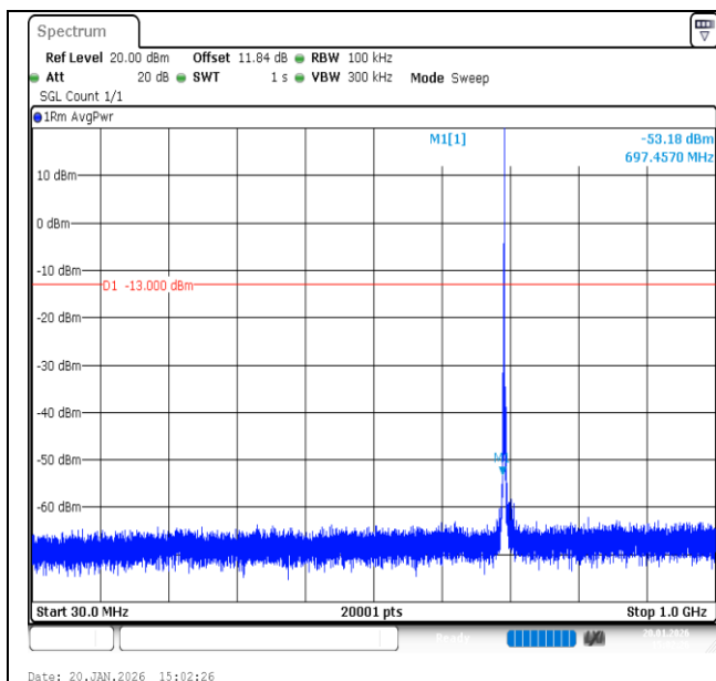
Band12-1.4MHz-16QAM-23017-1RB#5-30~1000-PASS
