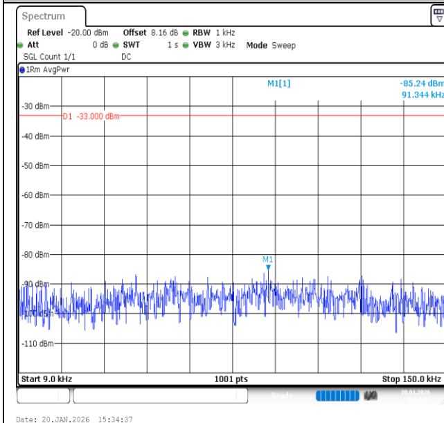
Band12-3MHz-QPSK-23095-1RB#14-0.009~0.15-PASS
