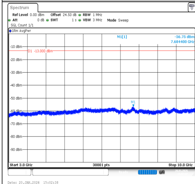
Band12-1.4MHz-16QAM-23017-1RB#5-3000~10000-PASS
