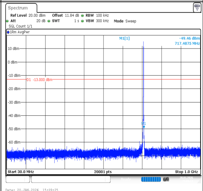
Band12-1.4MHz-16QAM-23173-6RB#0-30~1000-PASS
