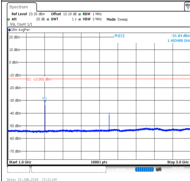
Band12-3MHz-QPSK-23025-1RB#14-1000~3000-PASS
