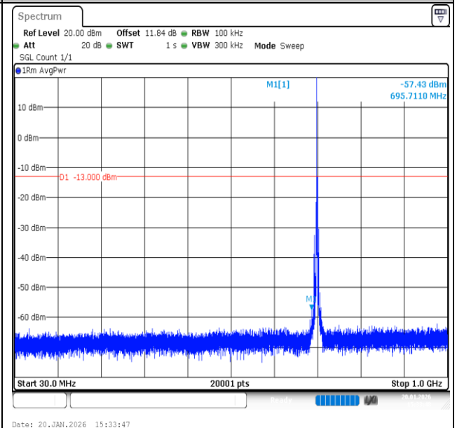
Band12-3MHz-QPSK-23095-1RB#0-30~1000-PASS
