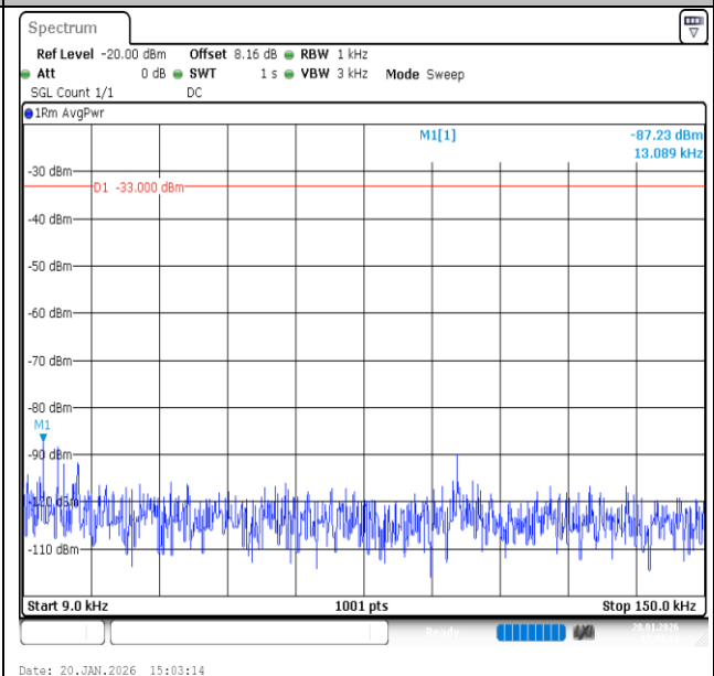
Band12-1.4MHz-16QAM-23017-6RB#0-0.009~0.15-PASS
