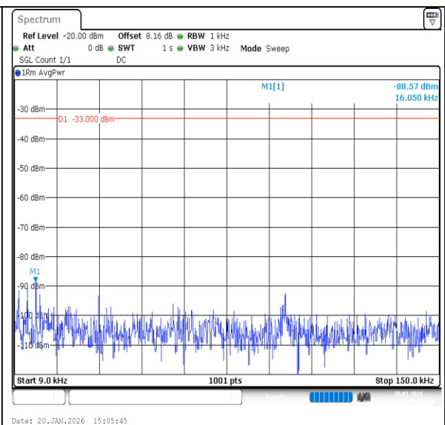
Band12-1.4MHz-QPSK-23095-6RB#0-0.009~0.15-PASS
