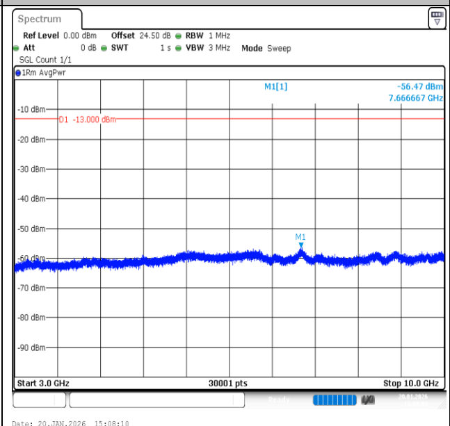
Band12-1.4MHz-QPSK-23173-1RB#5-3000~10000-PASS
