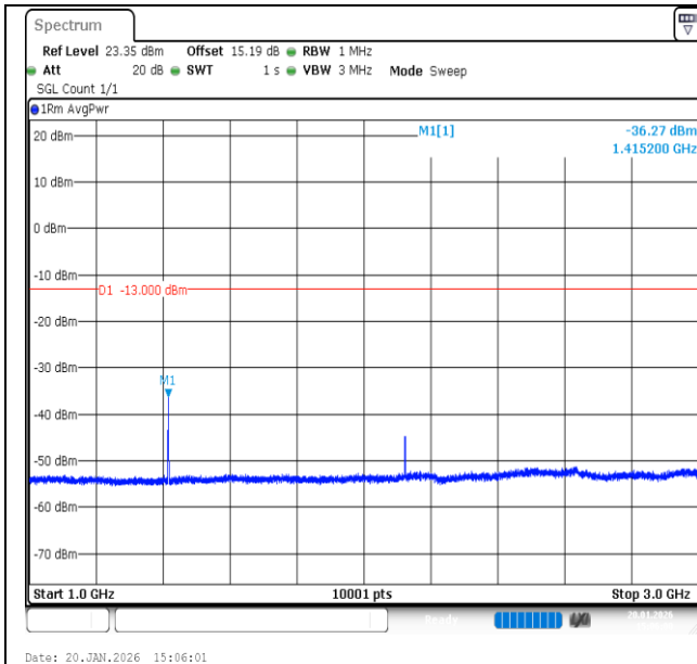
Band12-1.4MHz-QPSK-23095-6RB#0-1000~3000-PASS
