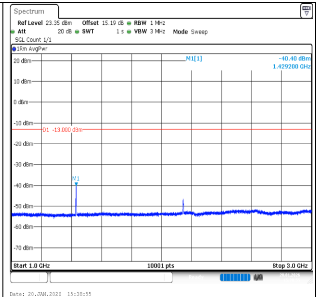
Band12-3MHz-QPSK-23165-15RB#0-1000~3000-PASS
