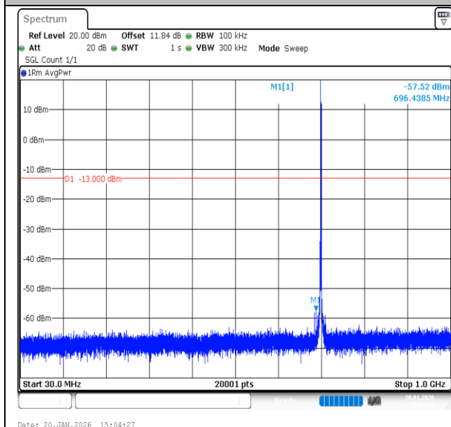
Band12-1.4MHz-16QAM-23095-1RB#0-30~1000-PASS
