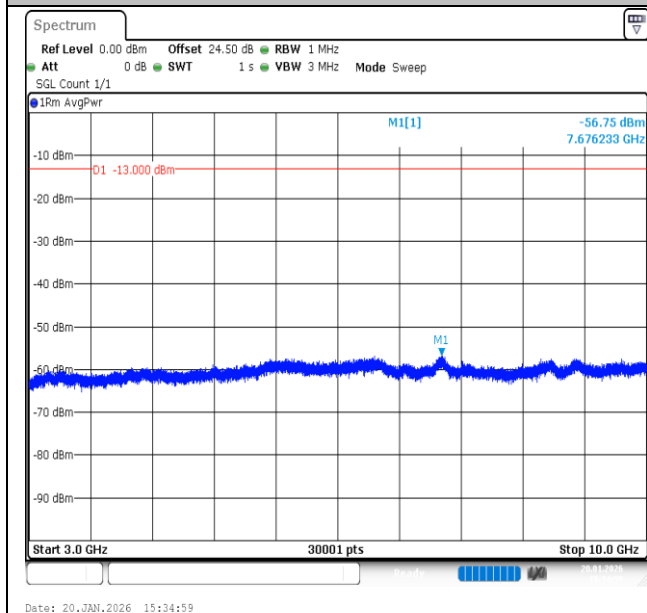
Band12-3MHz-QPSK-23095-1RB#14-3000~10000-PASS
