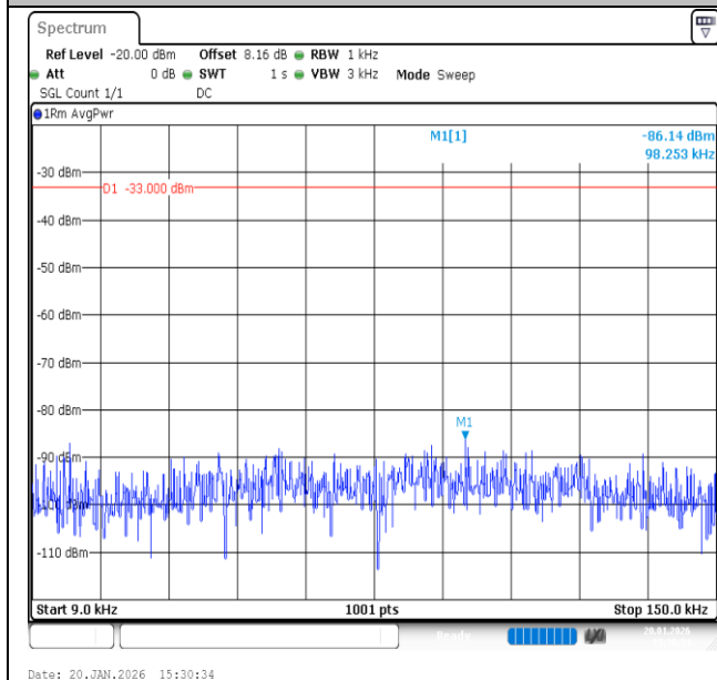
Band12-3MHz-QPSK-23025-1RB#0-0.009~0.15-PASS
