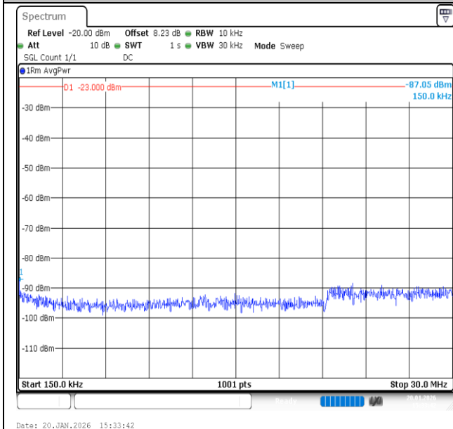
Band12-3MHz-QPSK-23095-1RB#0-0.15~30-PASS
