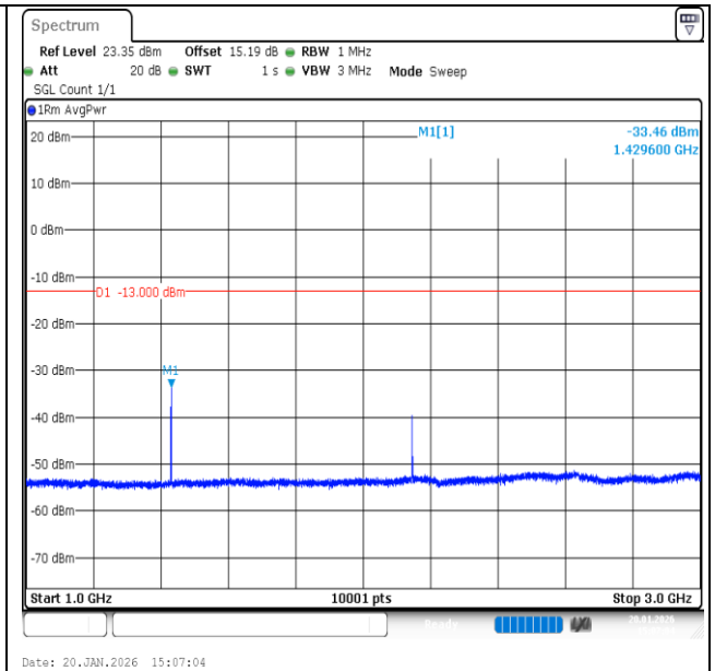
Band12-1.4MHz-QPSK-23173-1RB#0-1000~3000-PASS
