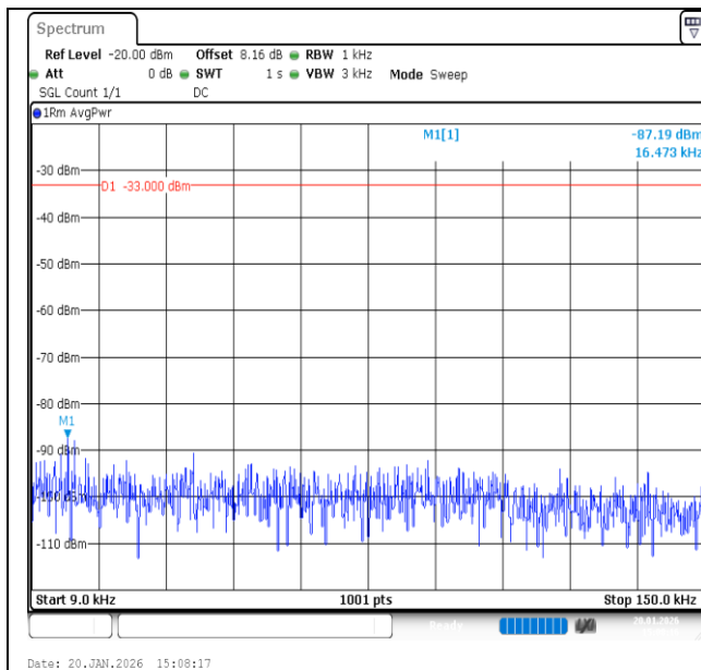
Band12-1.4MHz-16QAM-23173-1RB#5-0.009~0.15-PASS
