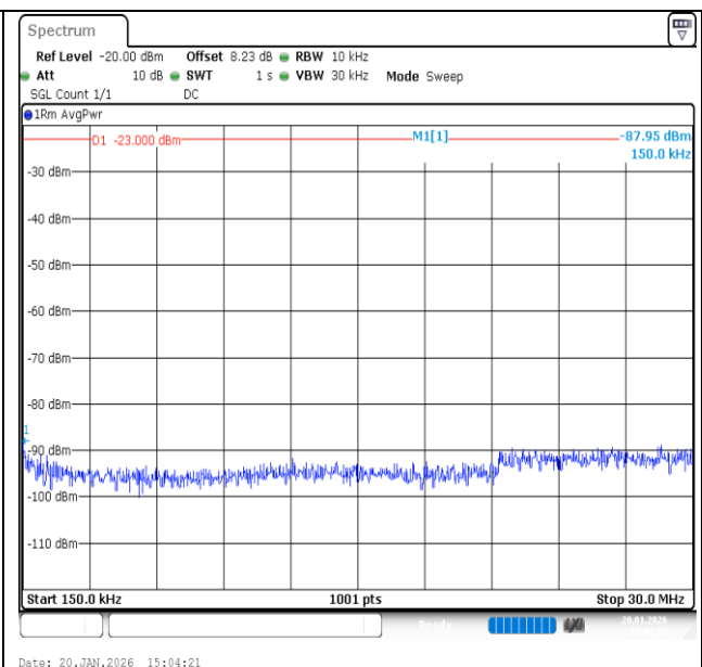
Band12-1.4MHz-16QAM-23095-1RB#0-0.15~30-PASS
