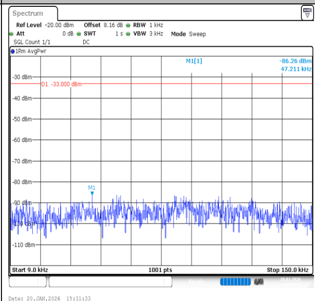
Band12-3MHz-QPSK-23025-1RB#14-0.009~0.15-PASS
