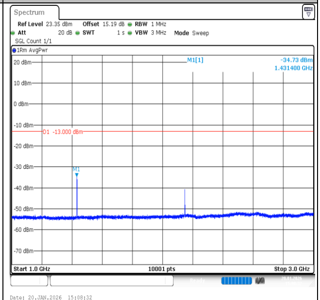
Band12-1.4MHz-16QAM-23173-1RB#5-1000~3000-PASS
