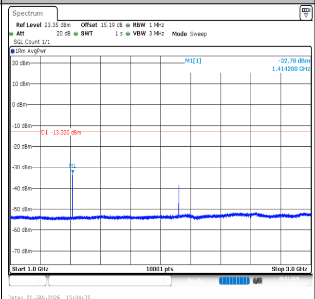
Band12-1.4MHz-16QAM-23095-1RB#0-1000~3000-PASS
