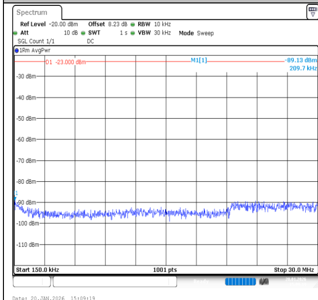
Band12-1.4MHz-16QAM-23173-6RB#0-0.15~30-PASS
