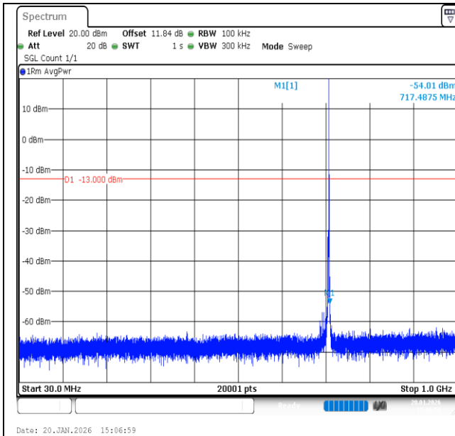
Band12-1.4MHz-QPSK-23173-1RB#0-30~1000-PASS
