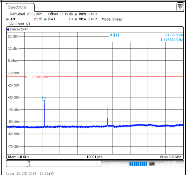
Band12-3MHz-QPSK-23165-1RB#0-1000~3000-PASS
