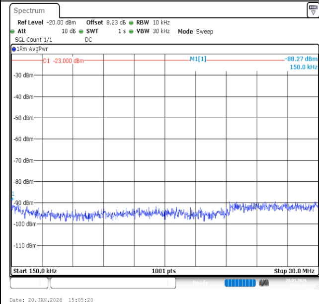
Band12-1.4MHz-16QAM-23095-1RB#5-0.15~30-PASS
