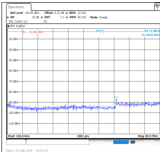
Band12-3MHz-16QAM-23025-1RB#0-0.15~30-PASS
