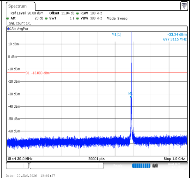
Band12-1.4MHz-16QAM-23017-1RB#0-30~1000-PASS
