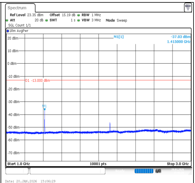
Band12-1.4MHz-16QAM-23095-6RB#0-1000~3000-PASS
