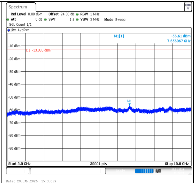
Band12-3MHz-QPSK-23095-1RB#0-3000~10000-PASS
