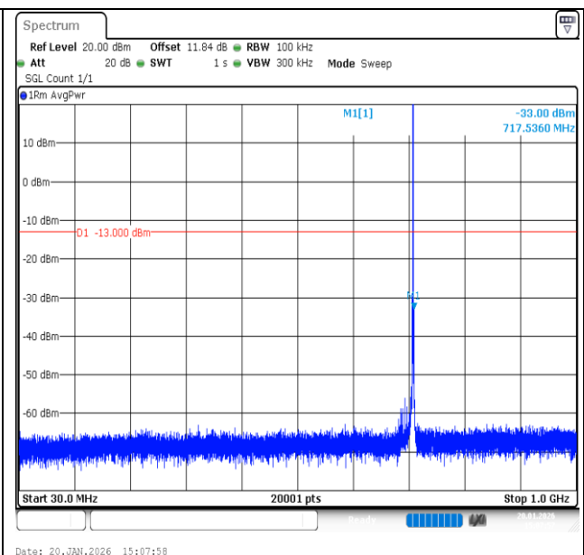
Band12-1.4MHz-QPSK-23173-1RB#5-30~1000-PASS
