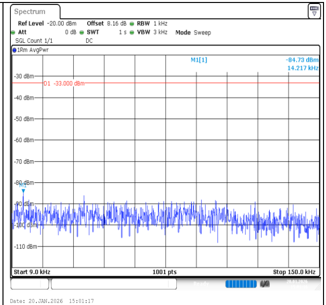
Band12-1.4MHz-16QAM-23017-1RB#0-0.009~0.15-PASS
