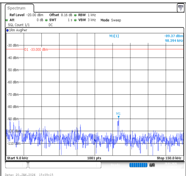
Band12-1.4MHz-16QAM-23173-6RB#0-0.009~0.15-PASS
