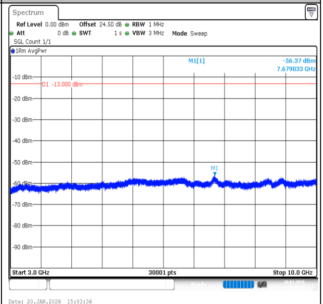
Band12-1.4MHz-16QAM-23017-6RB#0-3000~10000-PASS
