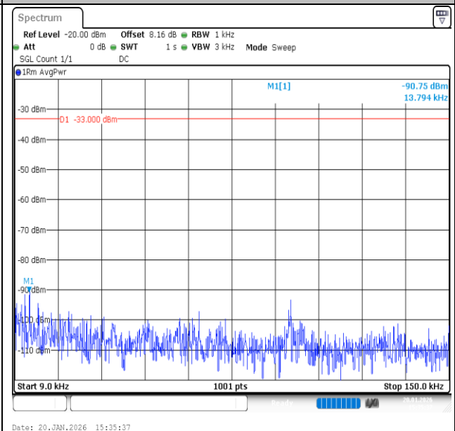
Band12-3MHz-QPSK-23095-15RB#0-0.009~0.15-PASS
