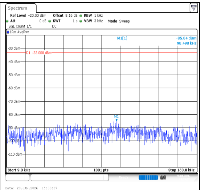
Band12-3MHz-QPSK-23095-1RB#0-0.009~0.15-PASS
