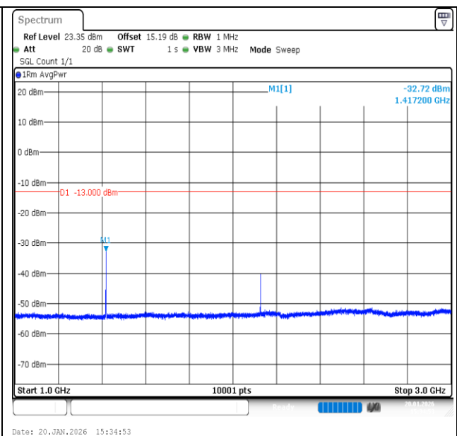
Band12-3MHz-QPSK-23095-1RB#14-1000~3000-PASS
