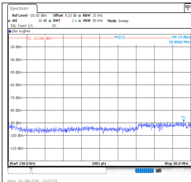
Band12-1.4MHz-QPSK-23173-1RB#5-0.15~30-PASS
