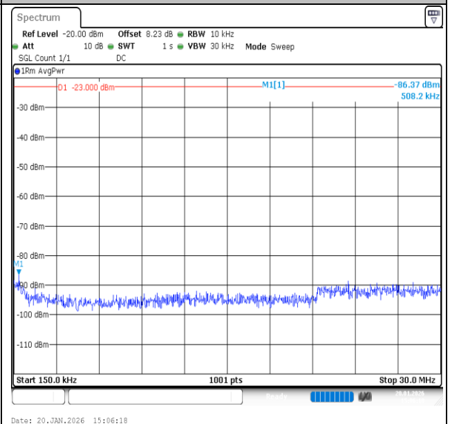
Band12-1.4MHz-16QAM-23095-6RB#0-0.15~30-PASS
