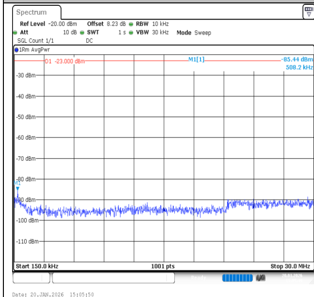
Band12-1.4MHz-QPSK-23095-6RB#0-0.15~30-PASS
