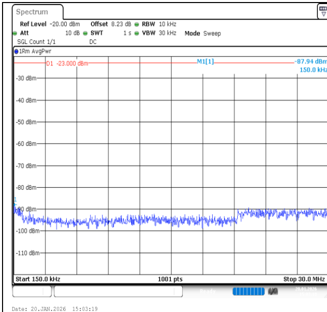
Band12-1.4MHz-16QAM-23017-6RB#0-0.15~30-PASS
