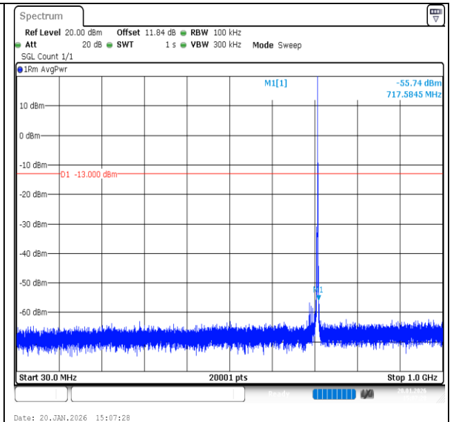
Band12-1.4MHz-16QAM-23173-1RB#0-30~1000-PASS
