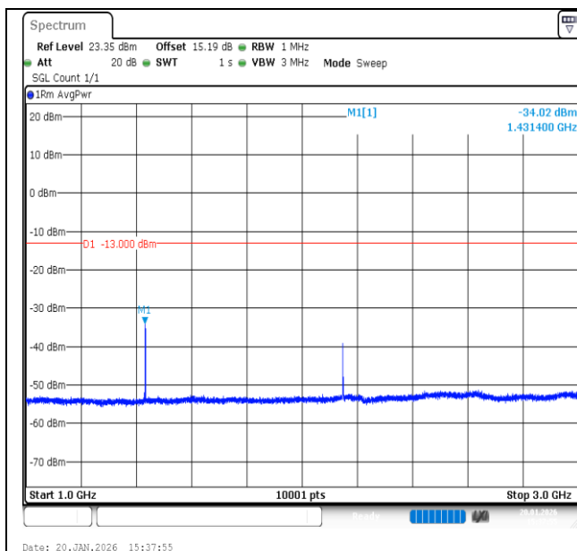
Band12-3MHz-QPSK-23165-1RB#14-1000~3000-PASS
