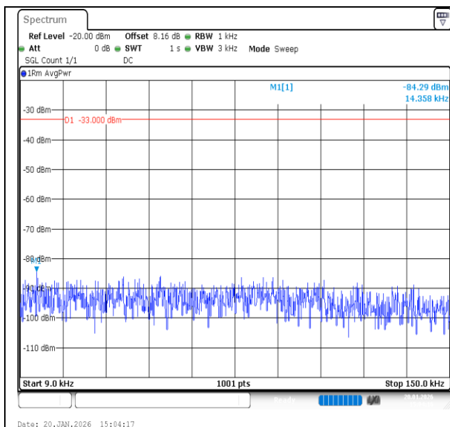
Band12-1.4MHz-16QAM-23095-1RB#0-0.009~0.15-PASS
