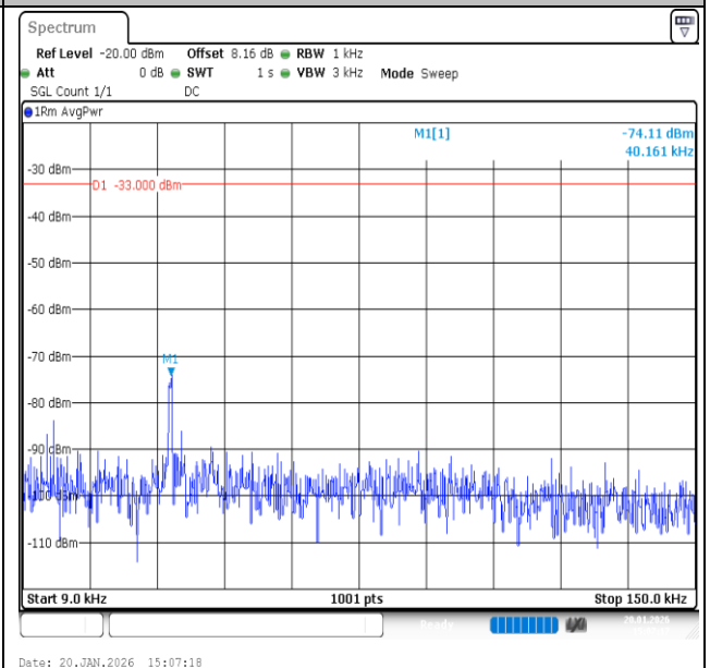
Band12-1.4MHz-16QAM-23173-1RB#0-0.009~0.15-PASS
