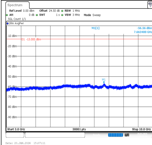
Band12-1.4MHz-QPSK-23173-1RB#0-3000~10000-PASS
