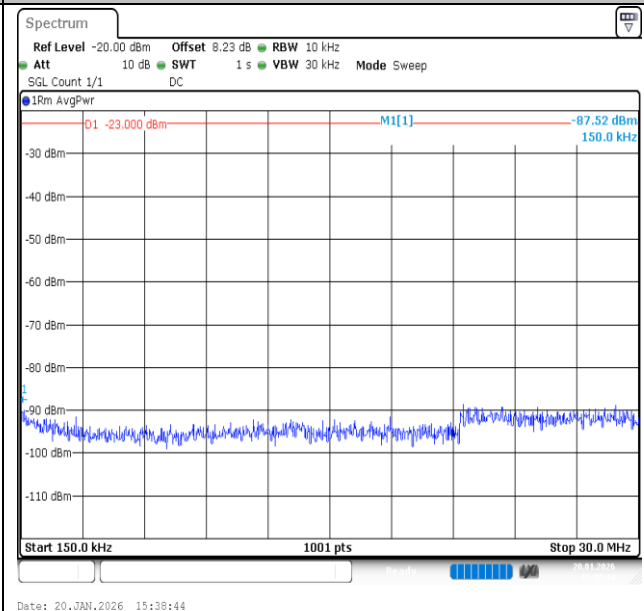
Band12-3MHz-QPSK-23165-15RB#0-0.15~30-PASS
