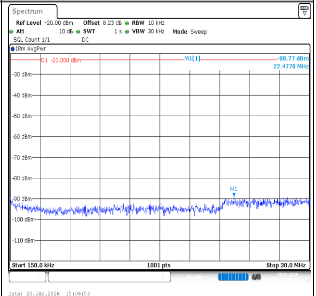
Band12-1.4MHz-QPSK-23173-1RB#0-0.15~30-PASS
