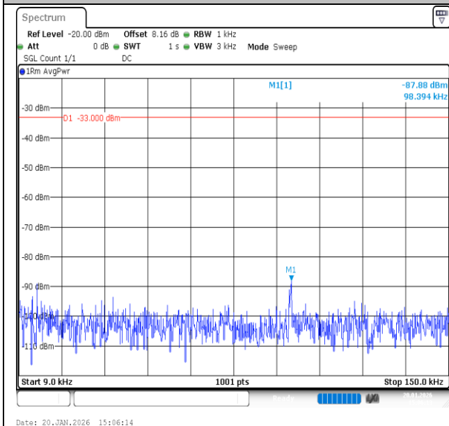
Band12-1.4MHz-16QAM-23095-6RB#0-0.009~0.15-PASS
