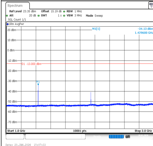
Band12-1.4MHz-16QAM-23173-1RB#0-1000~3000-PASS
