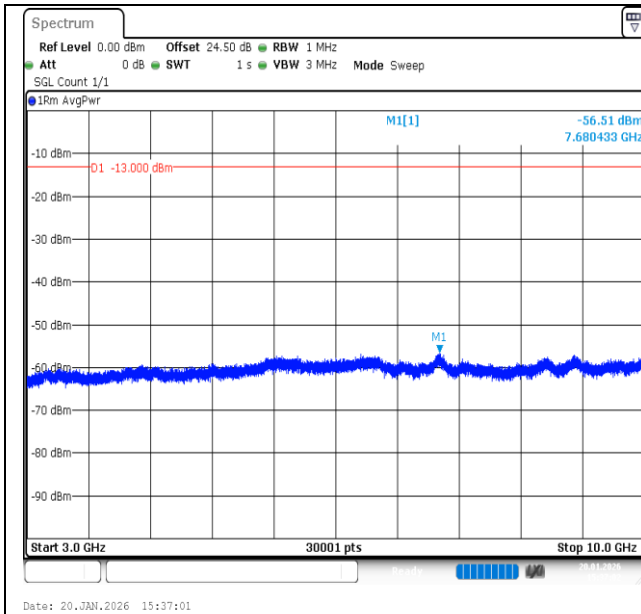
Band12-3MHz-QPSK-23165-1RB#0-3000~10000-PASS
