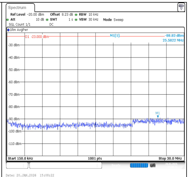
Band12-1.4MHz-16QAM-23173-1RB#5-0.15~30-PASS
