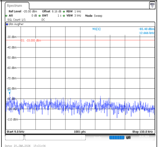
Band12-3MHz-16QAM-23025-1RB#0-0.009~0.15-PASS
