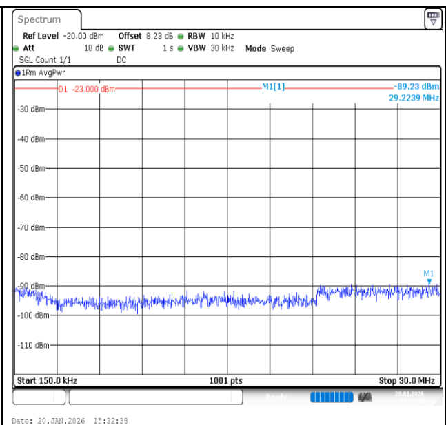
Band12-3MHz-QPSK-23025-15RB#0-0.15~30-PASS
