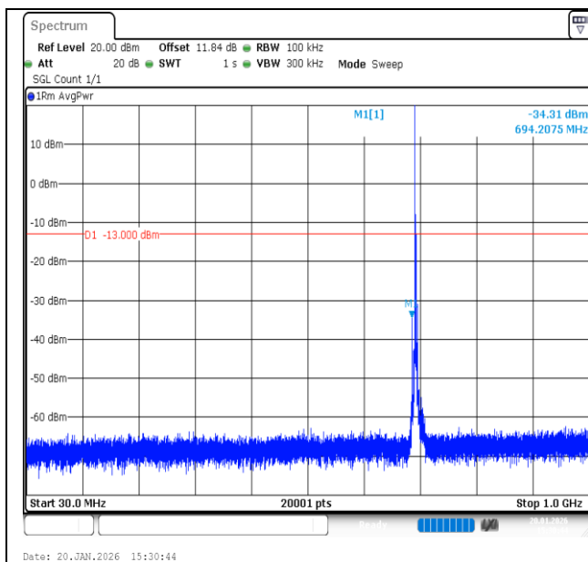
Band12-3MHz-QPSK-23025-1RB#0-30~1000-PASS
