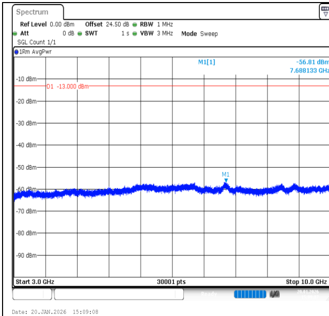
Band12-1.4MHz-QPSK-23173-6RB#0-3000~10000-PASS
