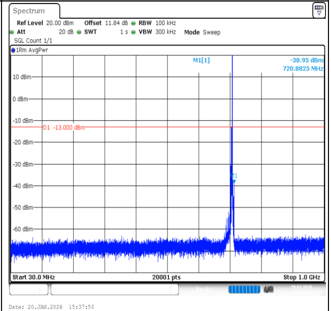
Band12-3MHz-QPSK-23165-1RB#14-30~1000-PASS
