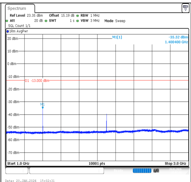
Band12-1.4MHz-16QAM-23017-1RB#5-1000~3000-PASS
