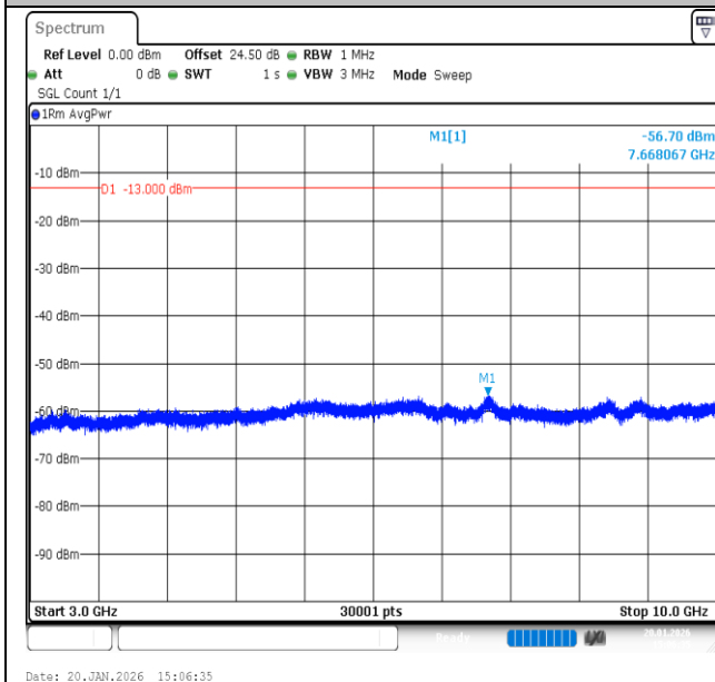
Band12-1.4MHz-16QAM-23095-6RB#0-3000~10000-PASS
