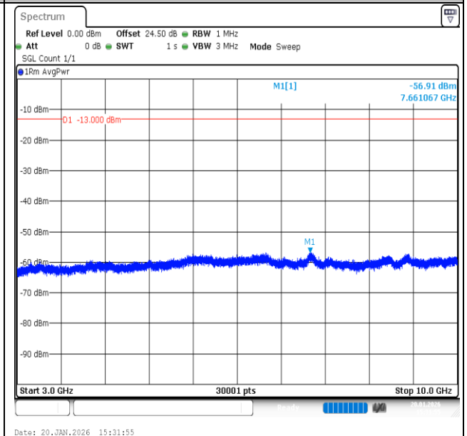
Band12-3MHz-QPSK-23025-1RB#14-3000~10000-PASS
