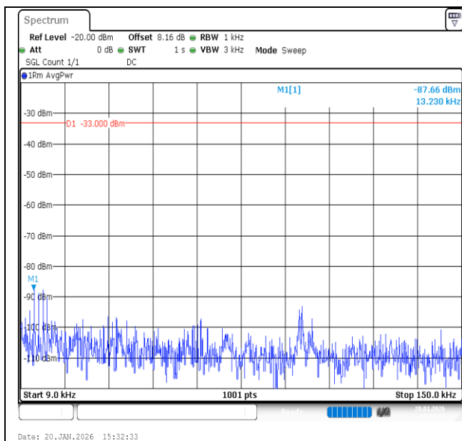
Band12-3MHz-QPSK-23025-15RB#0-0.009~0.15-PASS
