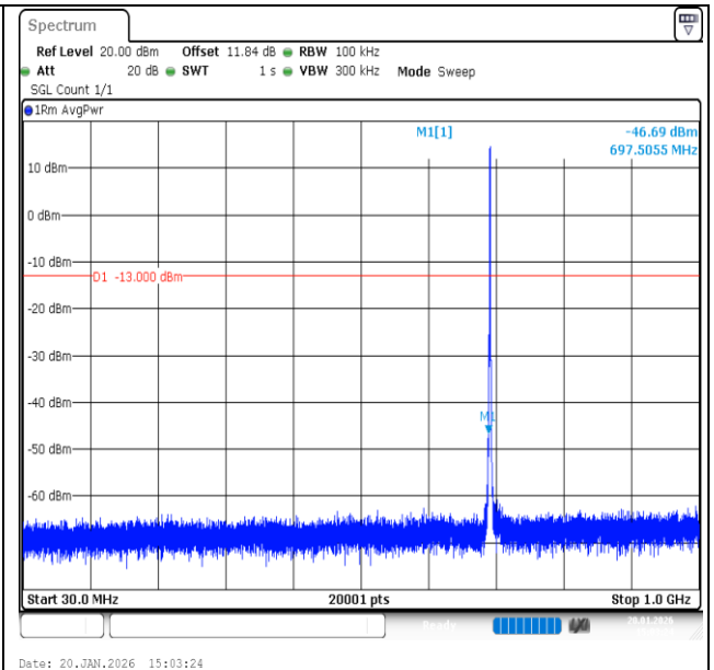
Band12-1.4MHz-16QAM-23017-6RB#0-30~1000-PASS
