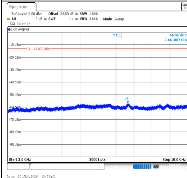
Band12-3MHz-QPSK-23165-15RB#0-3000~10000-PASS
