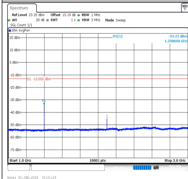
Band12-3MHz-16QAM-23025-1RB#0-1000~3000-PASS
