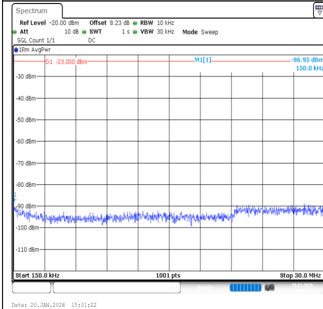
Band12-1.4MHz-16QAM-23017-1RB#0-0.15~30-PASS
