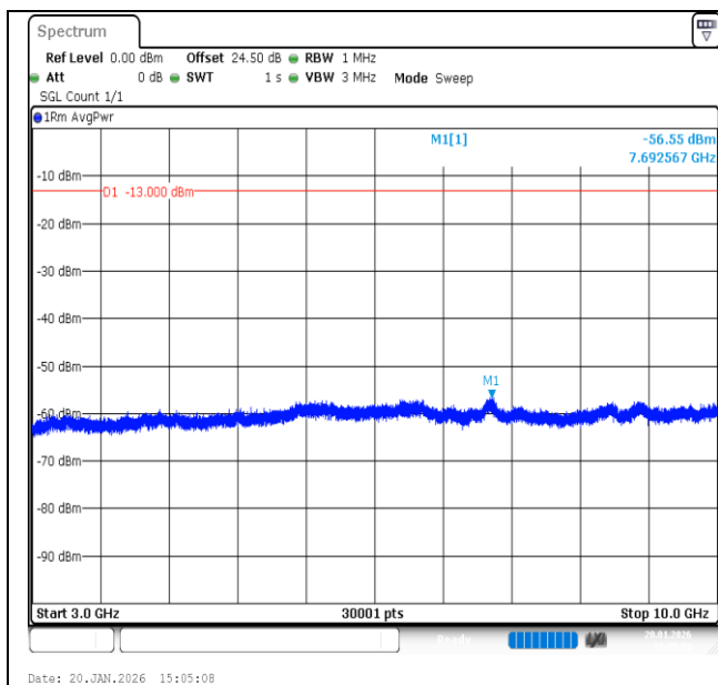
Band12-1.4MHz-QPSK-23095-1RB#5-3000~10000-PASS
