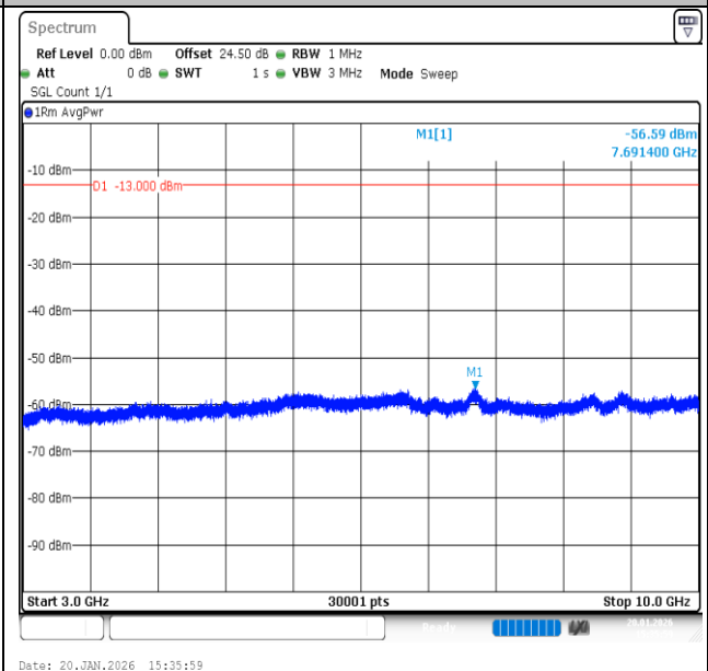
Band12-3MHz-QPSK-23095-15RB#0-3000~10000-PASS
