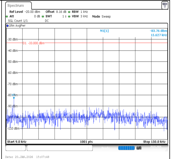
Band12-1.4MHz-QPSK-23173-1RB#5-0.009~0.15-PASS
