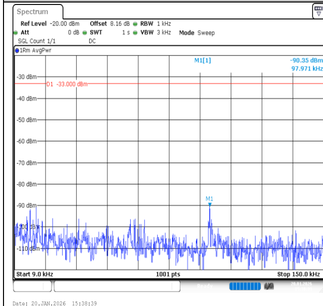
Band12-3MHz-QPSK-23165-15RB#0-0.009~0.15-PASS
