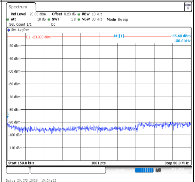
Band12-3MHz-QPSK-23095-1RB#14-0.15~30-PASS
