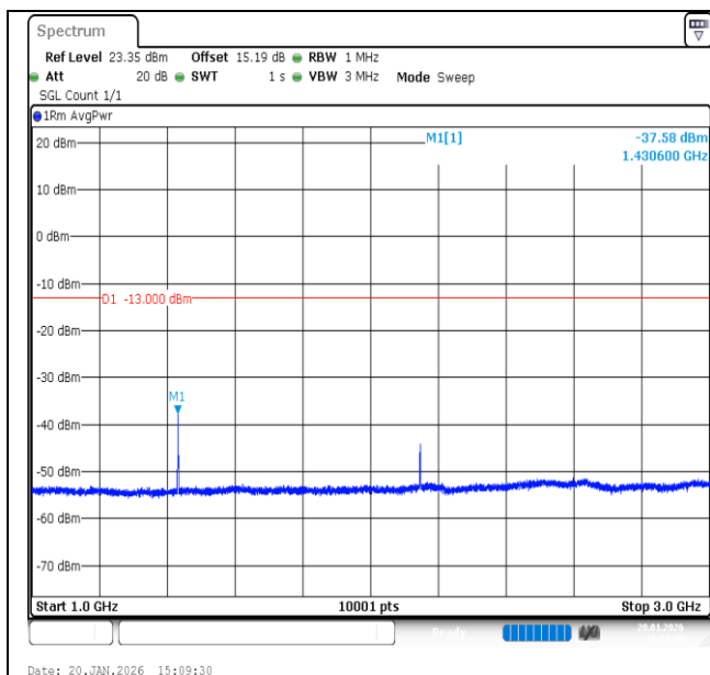
Band12-1.4MHz-16QAM-23173-6RB#0-1000~3000-PASS
