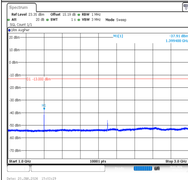
Band12-1.4MHz-16QAM-23017-6RB#0-1000~3000-PASS
