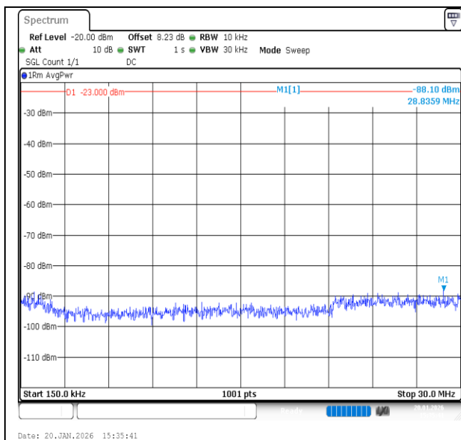
Band12-3MHz-QPSK-23095-15RB#0-0.15~30-PASS
