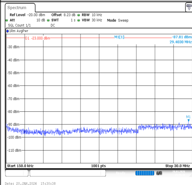
Band12-3MHz-QPSK-23025-1RB#0-0.15~30-PASS
