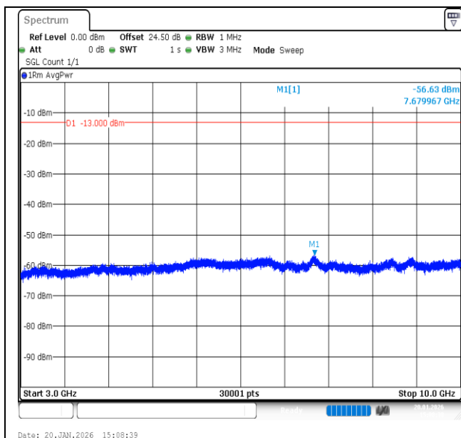
Band12-1.4MHz-16QAM-23173-1RB#5-3000~10000-PASS
