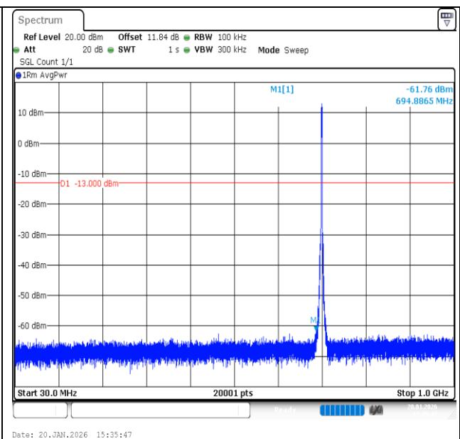
Band12-3MHz-QPSK-23095-15RB#0-30~1000-PASS
