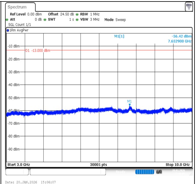
Band12-1.4MHz-QPSK-23095-6RB#0-3000~10000-PASS
