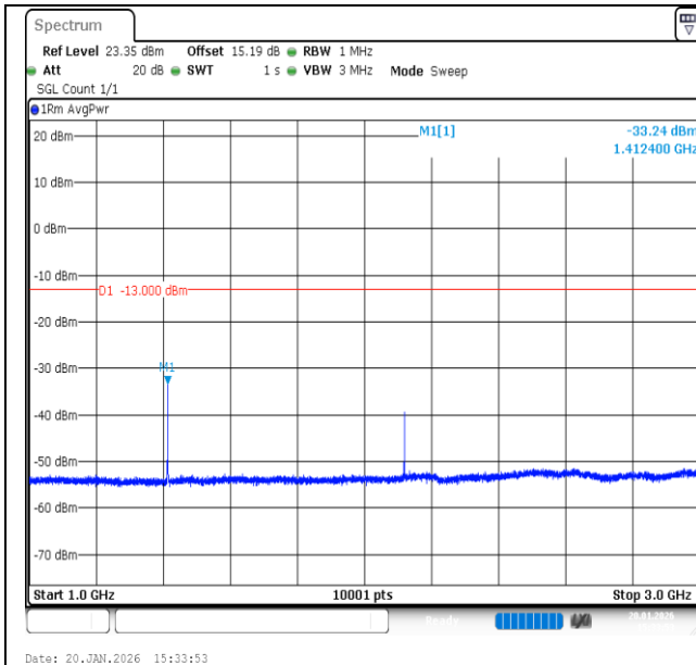
Band12-3MHz-QPSK-23095-1RB#0-1000~3000-PASS
