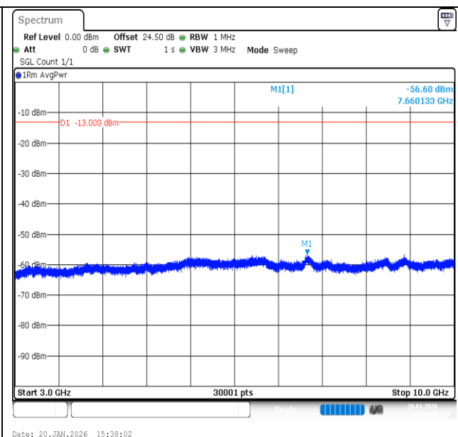
Band12-3MHz-QPSK-23165-1RB#14-3000~10000-PASS
