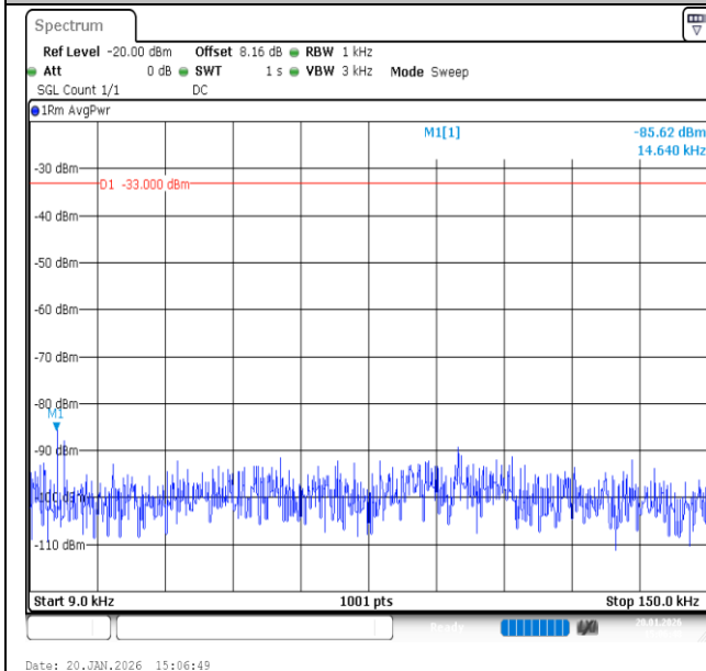
Band12-1.4MHz-QPSK-23173-1RB#0-0.009~0.15-PASS
