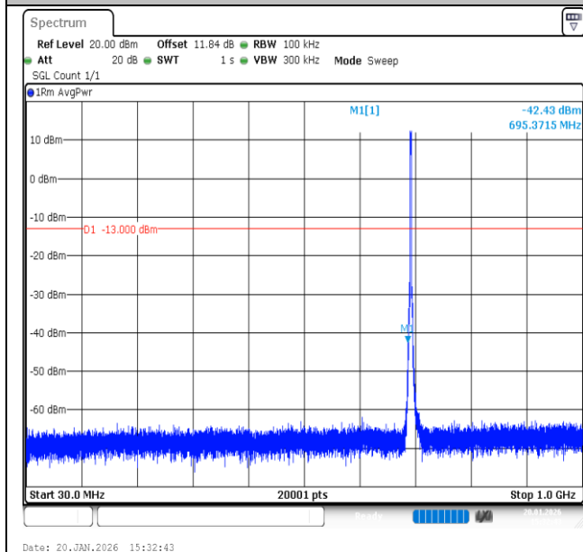
Band12-3MHz-QPSK-23025-15RB#0-30~1000-PASS
