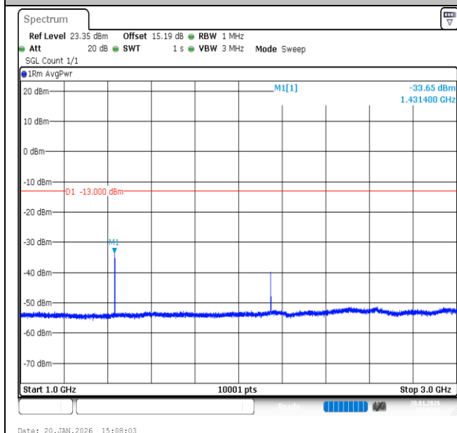
Band12-1.4MHz-QPSK-23173-1RB#5-1000~3000-PASS
