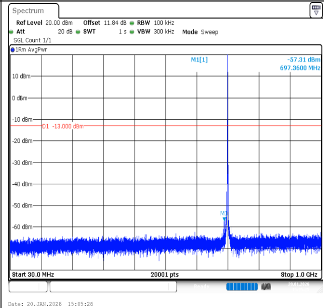
Band12-1.4MHz-16QAM-23095-1RB#5-30~1000-PASS
