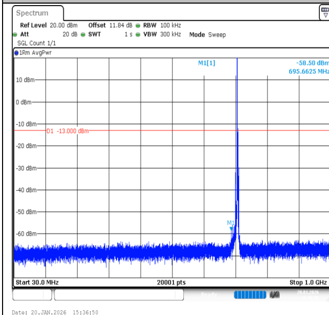
Band12-3MHz-QPSK-23165-1RB#0-30~1000-PASS
