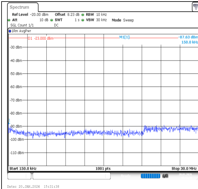
Band12-3MHz-QPSK-23025-1RB#14-0.15~30-PASS
