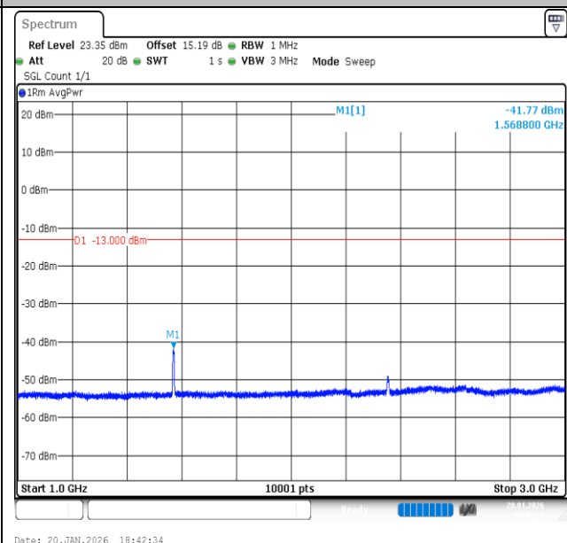
Band13-5MHz-QPSK-23255-25RB#0-1000~3000-PASS
