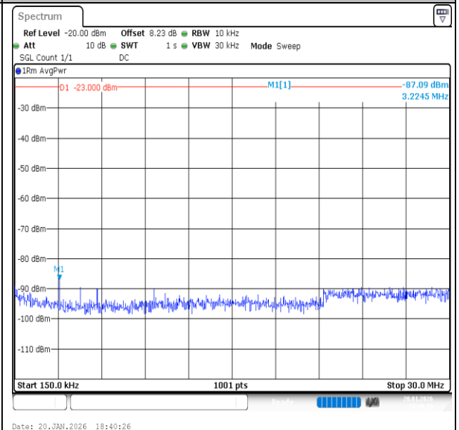
Band13-5MHz-QPSK-23255-1RB#0-0.15~30-PASS
