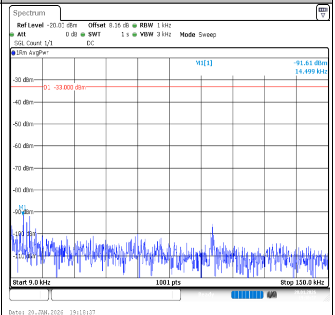
Band13-10MHz-16QAM-23230-50RB#0-0.009~0.15-PASS
