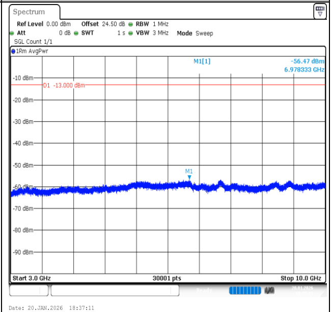
Band13-5MHz-16QAM-23205-25RB#0-3000~10000-PASS
