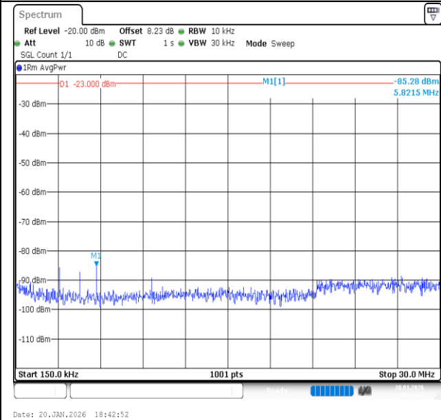
Band13-5MHz-16QAM-23255-25RB#0-0.15~30-PASS
