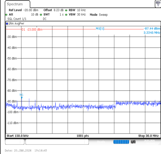
Band13-10MHz-16QAM-23230-1RB#0-0.15~30-PASS
