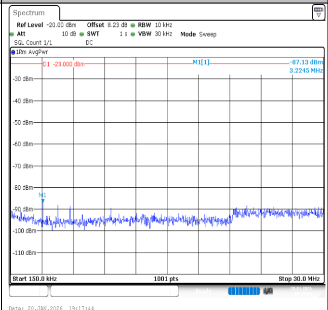
Band13-10MHz-16QAM-23230-1RB#49-0.15~30-PASS
