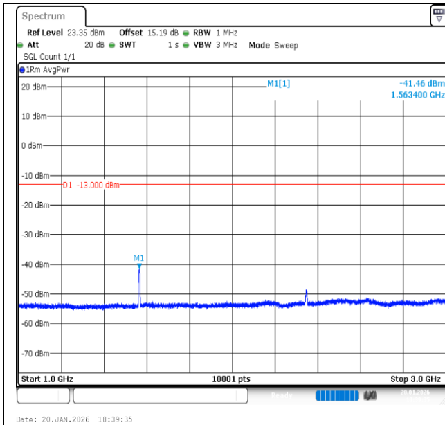
Band13-5MHz-QPSK-23230-25RB#0-1000~3000-PASS
