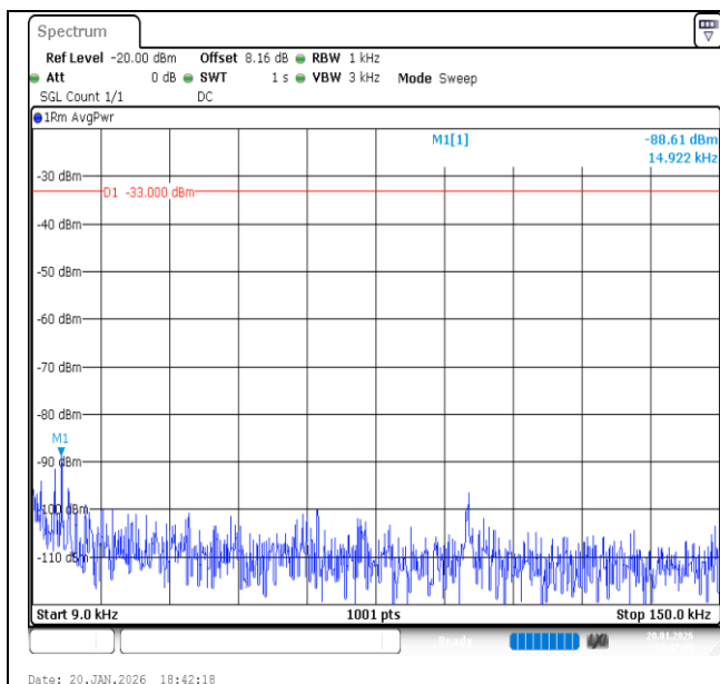
Band13-5MHz-QPSK-23255-25RB#0-0.009~0.15-PASS
