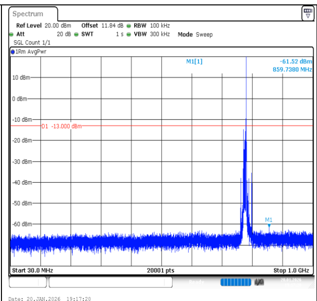
Band13-10MHz-QPSK-23230-1RB#49-30~1000-PASS
