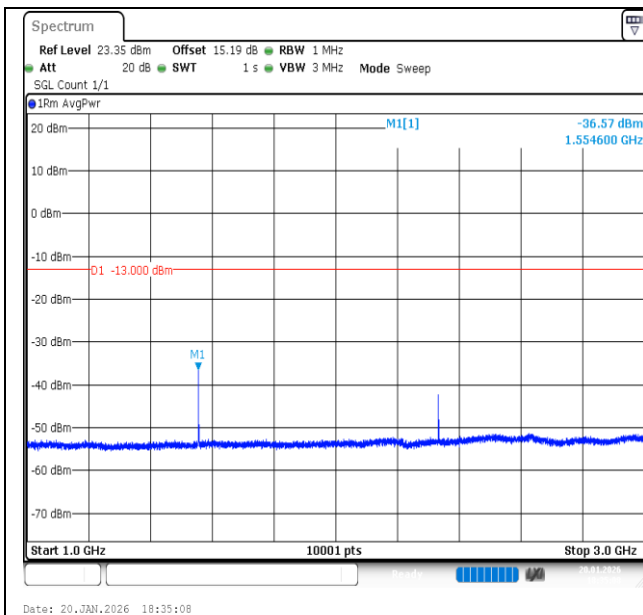
Band13-5MHz-16QAM-23205-1RB#0-1000~3000-PASS
