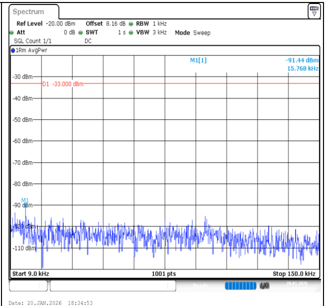
Band13-5MHz-16QAM-23205-1RB#0-0.009~0.15-PASS
