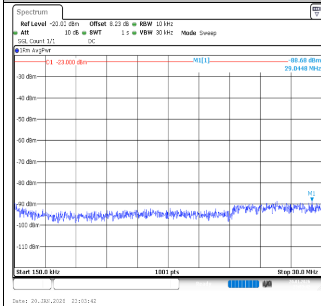
Band26 (814-824)-1.4MHz-QPSK-26697-1RB#5-0.15~30-PASS
