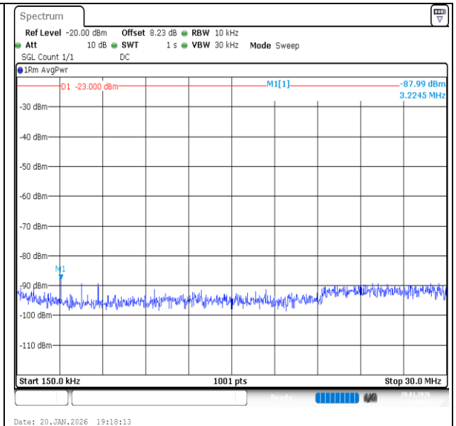
Band13-10MHz-QPSK-23230-50RB#0-0.15~30-PASS
