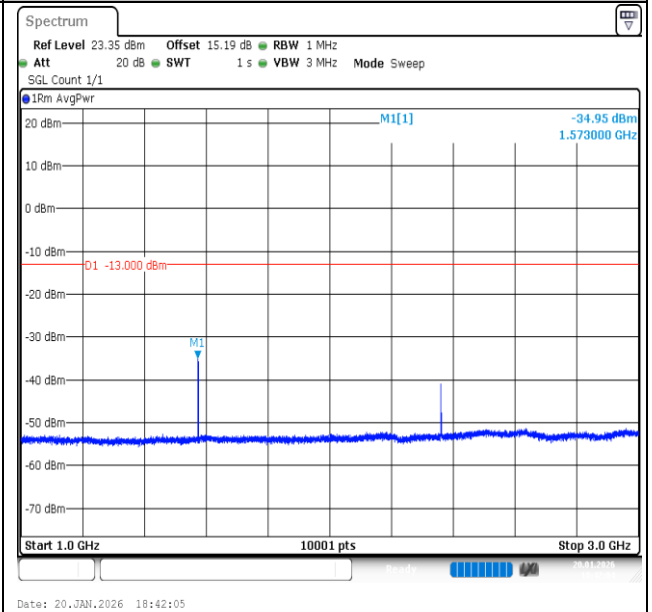
Band13-5MHz-16QAM-23255-1RB#24-1000~3000-PASS
