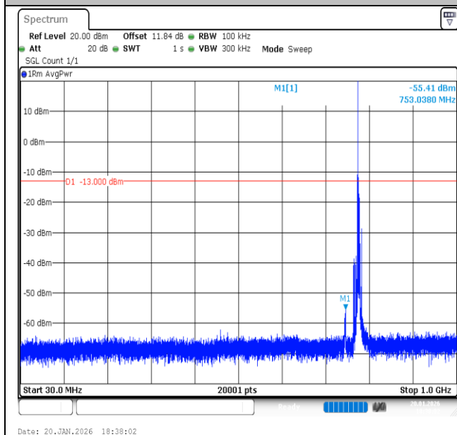
Band13-5MHz-16QAM-23230-1RB#0-30~1000-PASS
