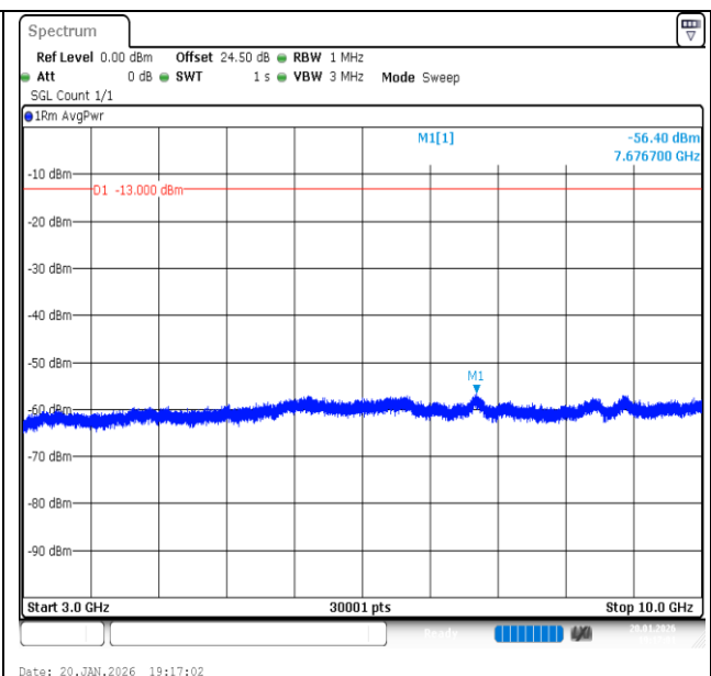
Band13-10MHz-16QAM-23230-1RB#0-3000~10000-PASS
