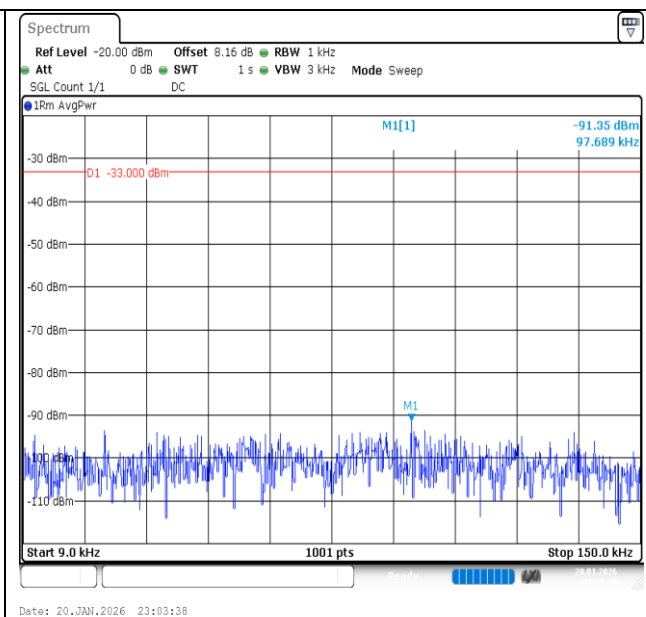
Band26 (814-824)-1.4MHz-QPSK-26697-1RB#5-0.009~0.15-PASS
