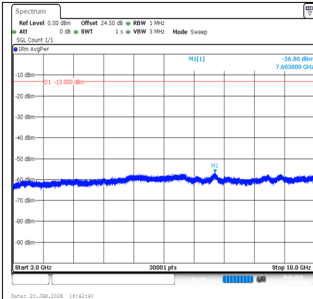
Band13-5MHz-QPSK-23255-25RB#0-3000~10000-PASS
