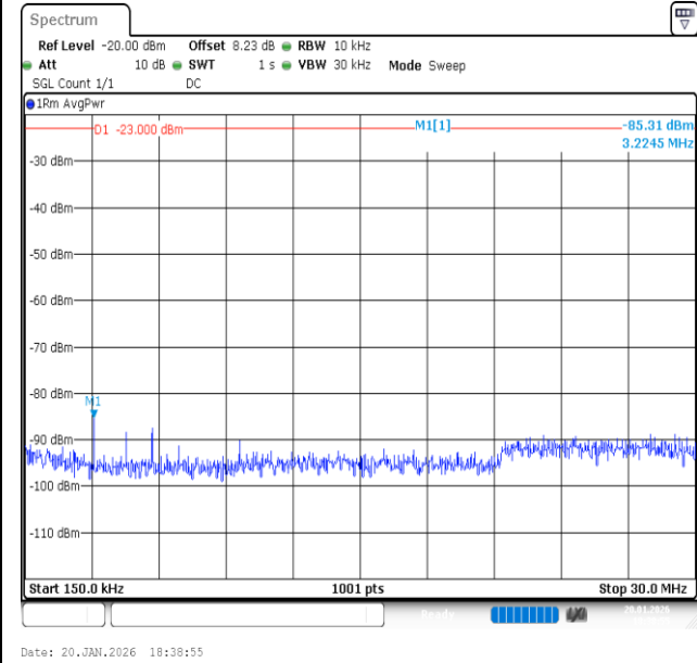
Band13-5MHz-16QAM-23230-1RB#24-0.15~30-PASS
