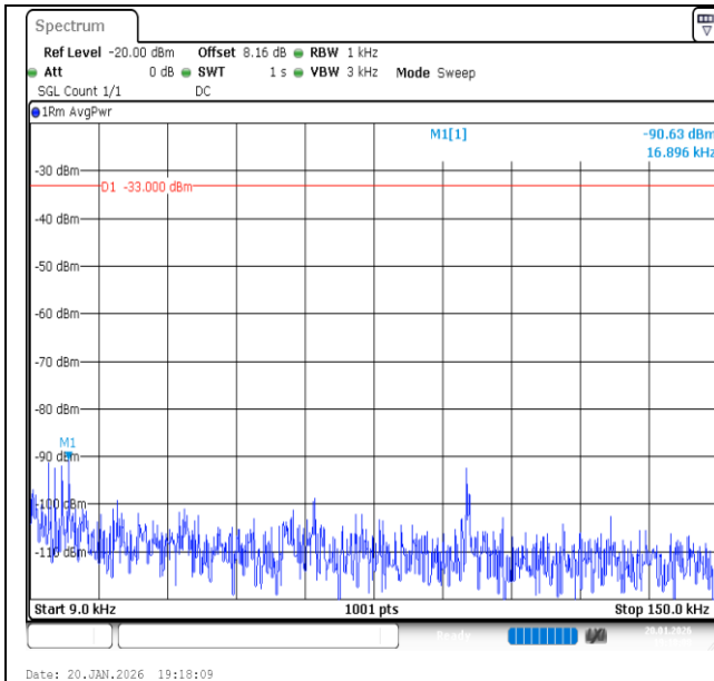
Band13-10MHz-QPSK-23230-50RB#0-0.009~0.15-PASS
