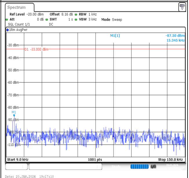
Band13-10MHz-QPSK-23230-1RB#49-0.009~0.15-PASS
