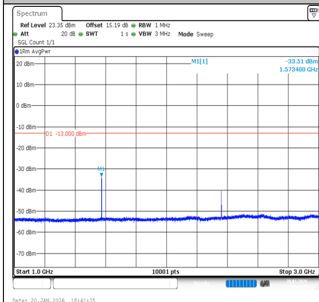
Band13-5MHz-QPSK-23255-1RB#24-1000~3000-PASS
