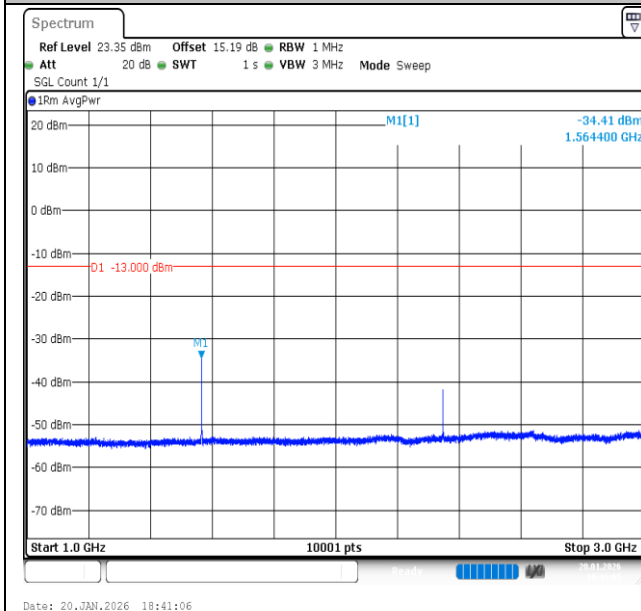
Band13-5MHz-16QAM-23255-1RB#0-1000~3000-PASS
