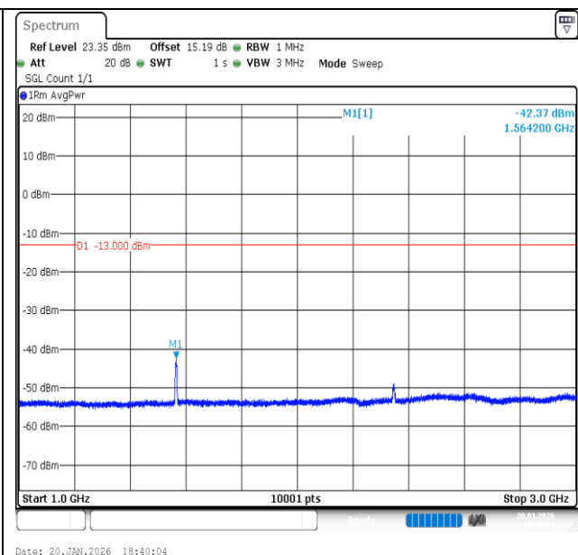
Band13-5MHz-16QAM-23230-25RB#0-1000~3000-PASS
