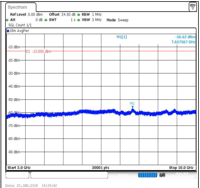
Band13-5MHz-QPSK-23230-25RB#0-3000~10000-PASS
