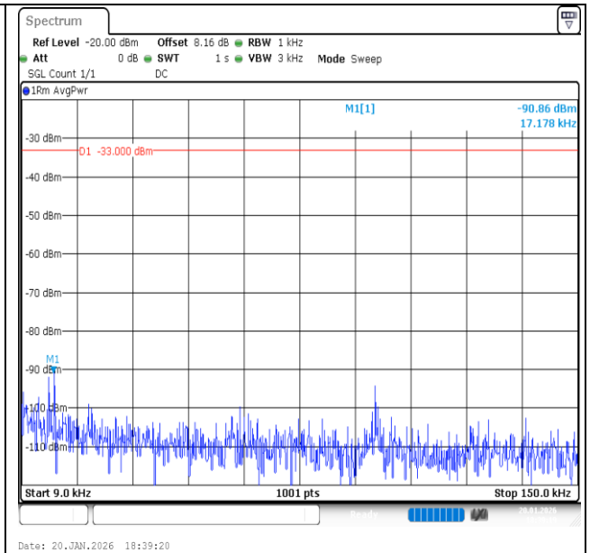
Band13-5MHz-QPSK-23230-25RB#0-0.009~0.15-PASS
