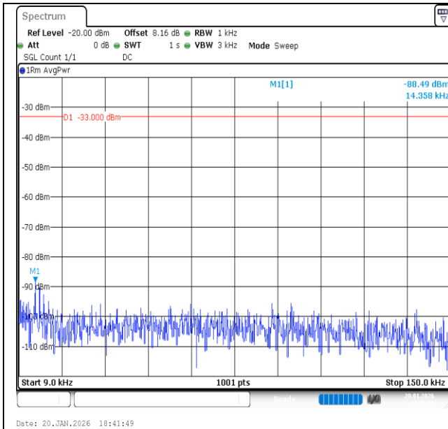
Band13-5MHz-16QAM-23255-1RB#24-0.009~0.15-PASS
