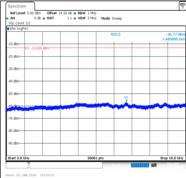
Band13-10MHz-QPSK-23230-50RB#0-3000~10000-PASS
