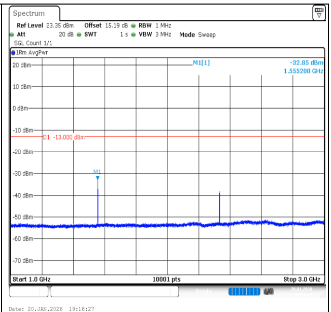
Band13-10MHz-QPSK-23230-1RB#0-1000~3000-PASS
