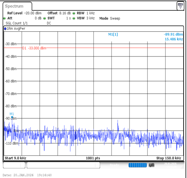
Band13-10MHz-16QAM-23230-1RB#0-0.009~0.15-PASS
