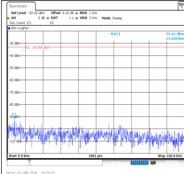
Band13-5MHz-16QAM-23205-1RB#24-0.009~0.15-PASS
