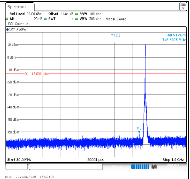
Band13-5MHz-16QAM-23205-25RB#0-30~1000-PASS
