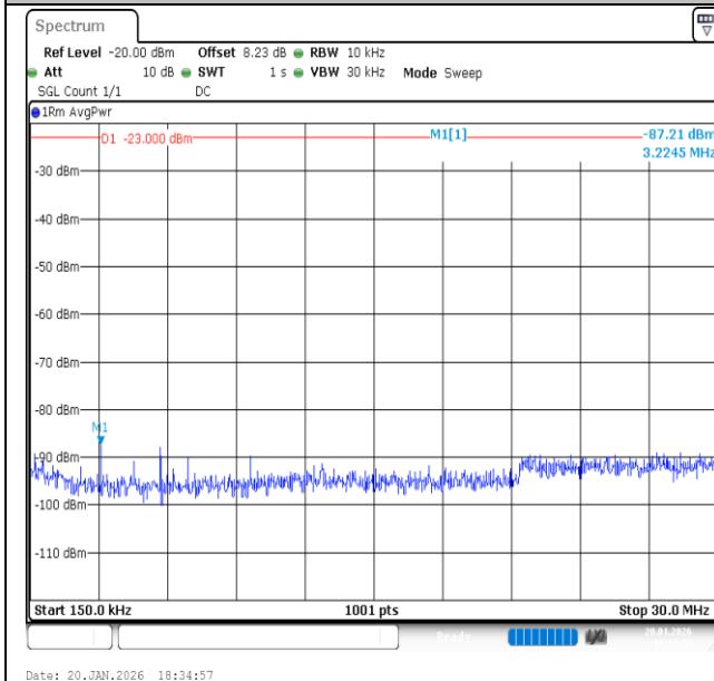
Band13-5MHz-16QAM-23205-1RB#0-0.15~30-PASS
