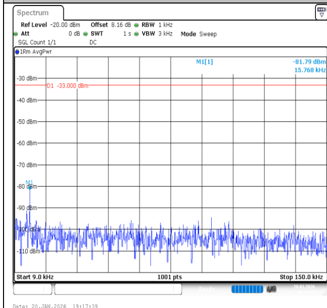
Band13-10MHz-16QAM-23230-1RB#49-0.009~0.15-PASS
