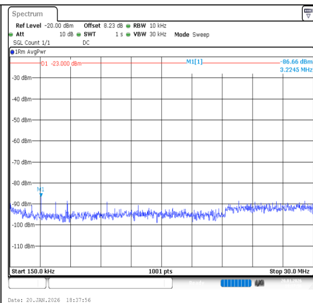
Band13-5MHz-16QAM-23230-1RB#0-0.15~30-PASS
