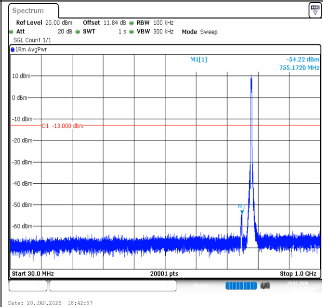
Band13-5MHz-16QAM-23255-25RB#0-30~1000-PASS
