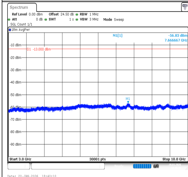
Band13-5MHz-16QAM-23230-25RB#0-3000~10000-PASS
