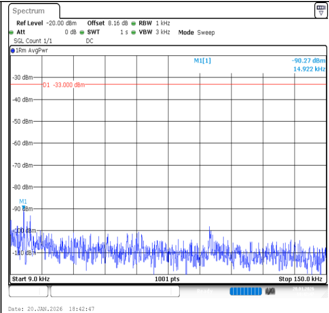
Band13-5MHz-16QAM-23255-25RB#0-0.009~0.15-PASS
