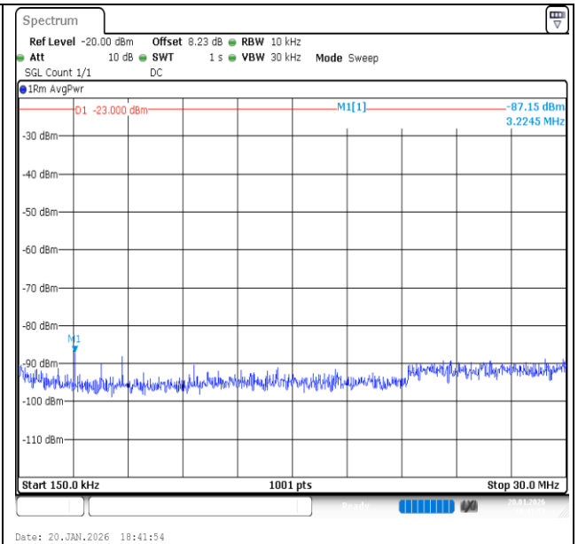
Band13-5MHz-16QAM-23255-1RB#24-0.15~30-PASS
