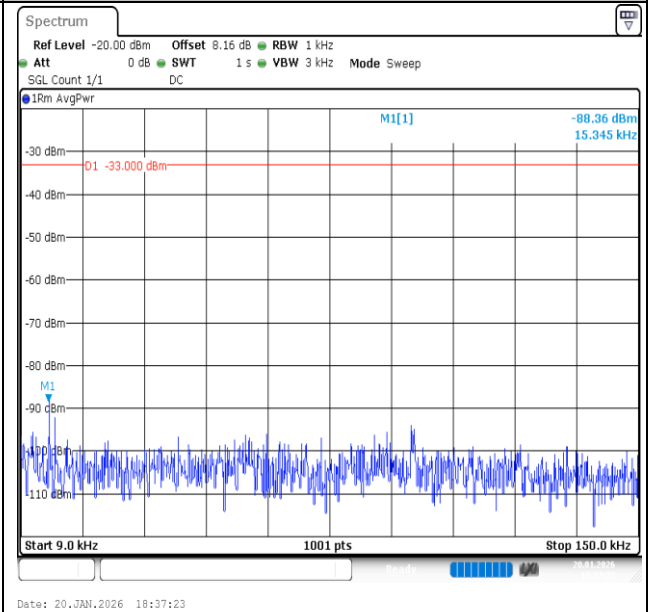
Band13-5MHz-QPSK-23230-1RB#0-0.009~0.15-PASS
