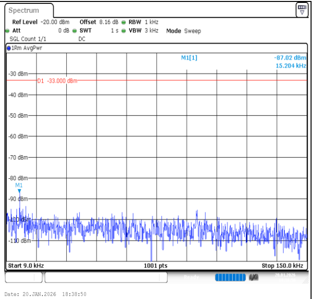
Band13-5MHz-16QAM-23230-1RB#24-0.009~0.15-PASS
