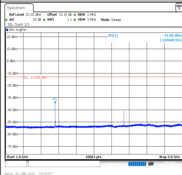
Band13-5MHz-16QAM-23230-1RB#0-1000~3000-PASS
