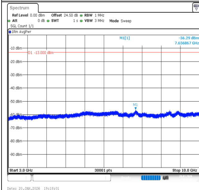
Band13-10MHz-16QAM-23230-1RB#49-3000~10000-PASS
