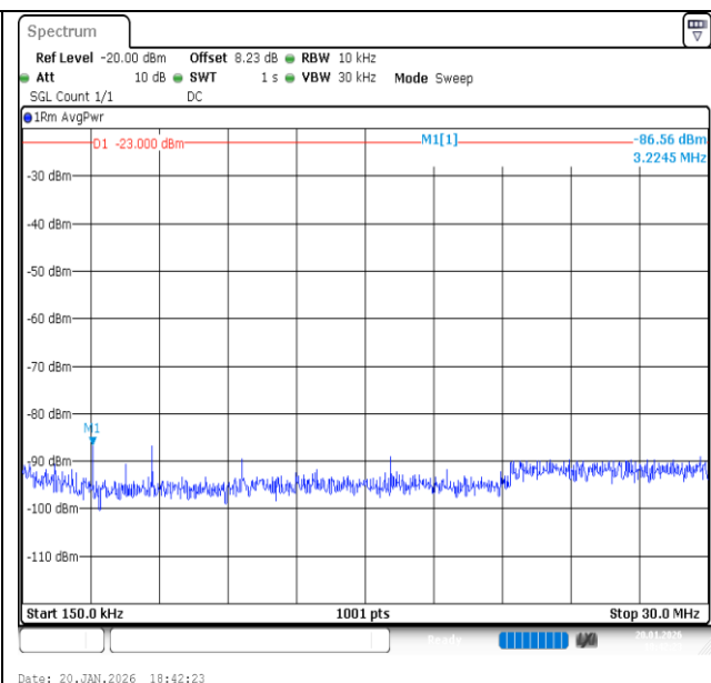
Band13-5MHz-QPSK-23255-25RB#0-0.15~30-PASS
