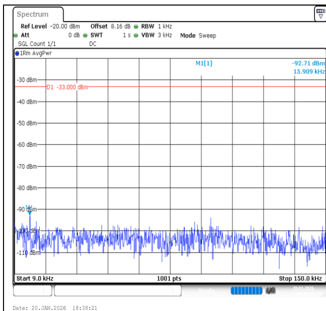
Band13-5MHz-QPSK-23230-1RB#24-0.009~0.15-PASS
