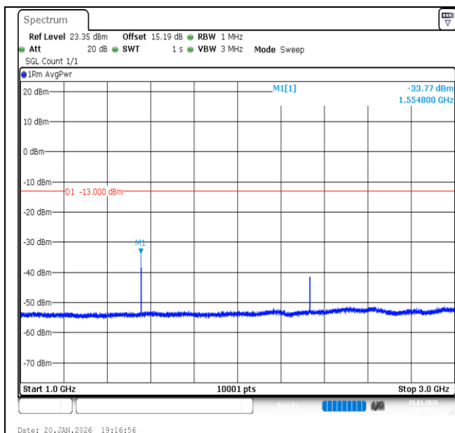
Band13-10MHz-16QAM-23230-1RB#0-1000~3000-PASS
