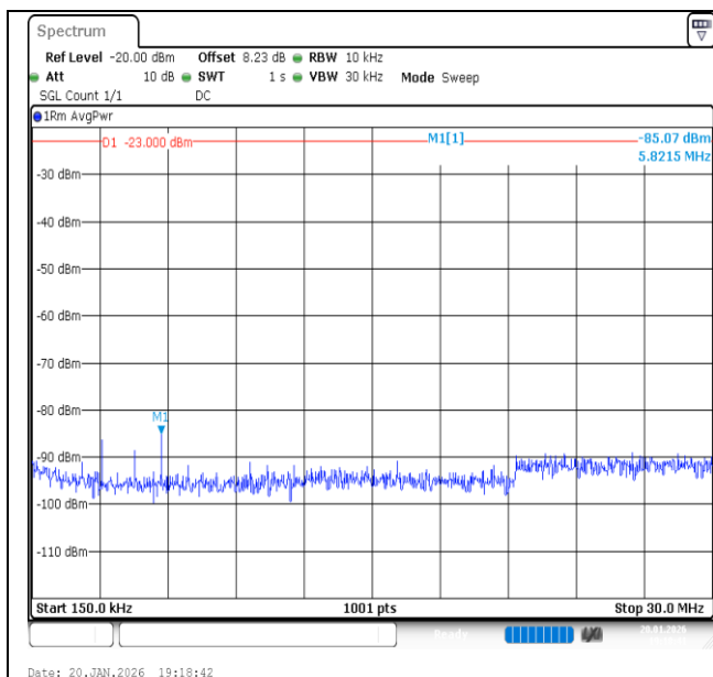
Band13-10MHz-16QAM-23230-50RB#0-0.15~30-PASS
