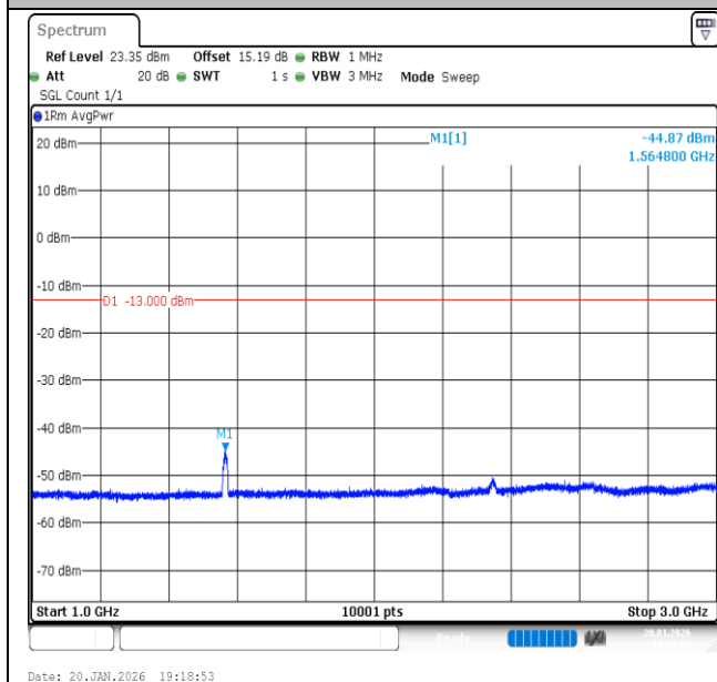
Band13-10MHz-16QAM-23230-50RB#0-1000~3000-PASS
