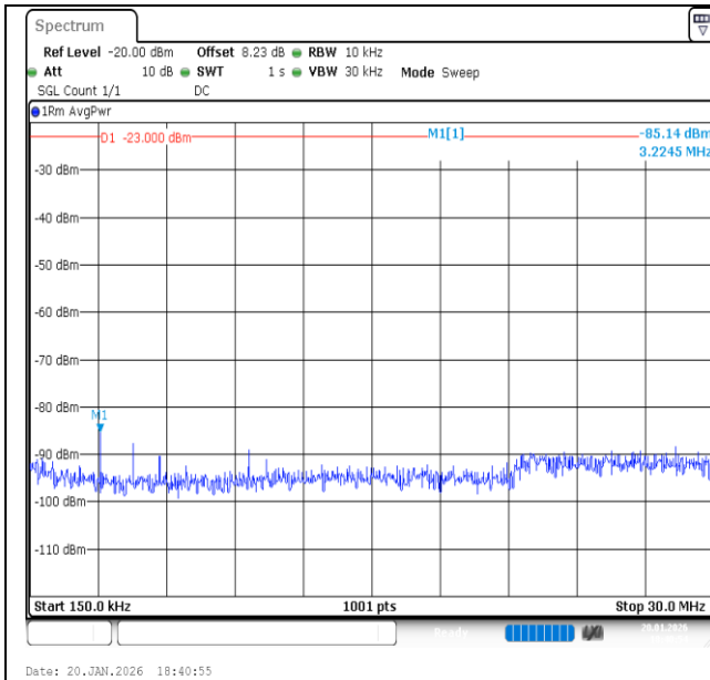
Band13-5MHz-16QAM-23255-1RB#0-0.15~30-PASS
