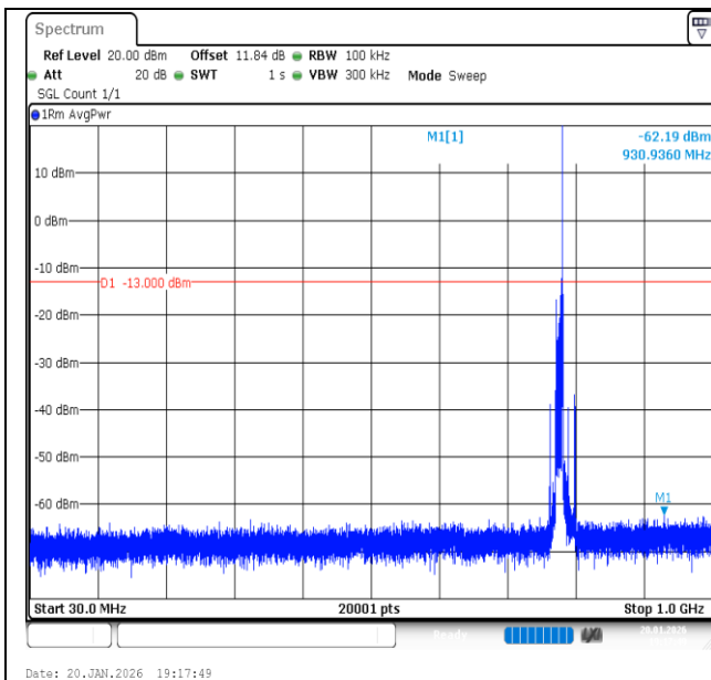
Band13-10MHz-16QAM-23230-1RB#49-30~1000-PASS
