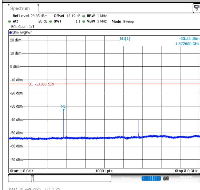
Band13-10MHz-QPSK-23230-1RB#49-1000~3000-PASS
