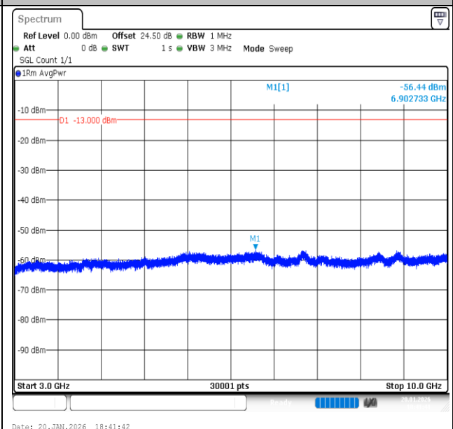
Band13-5MHz-QPSK-23255-1RB#24-3000~10000-PASS
