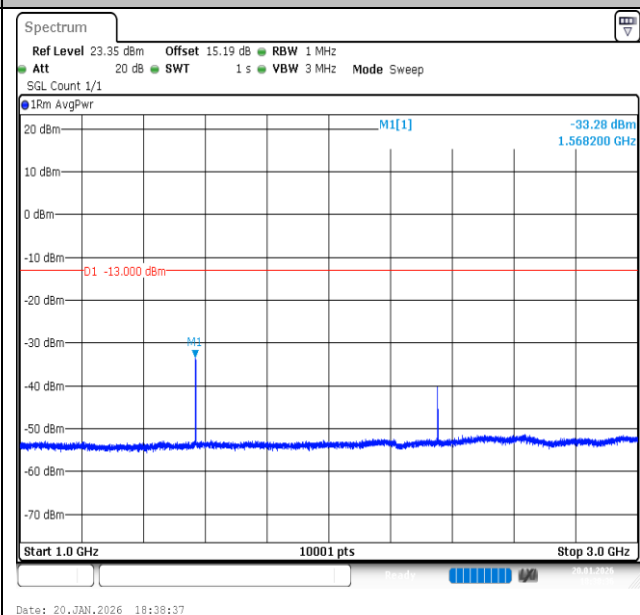
Band13-5MHz-QPSK-23230-1RB#24-1000~3000-PASS
