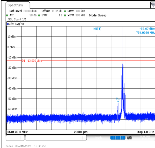
Band13-5MHz-16QAM-23255-1RB#24-30~1000-PASS
