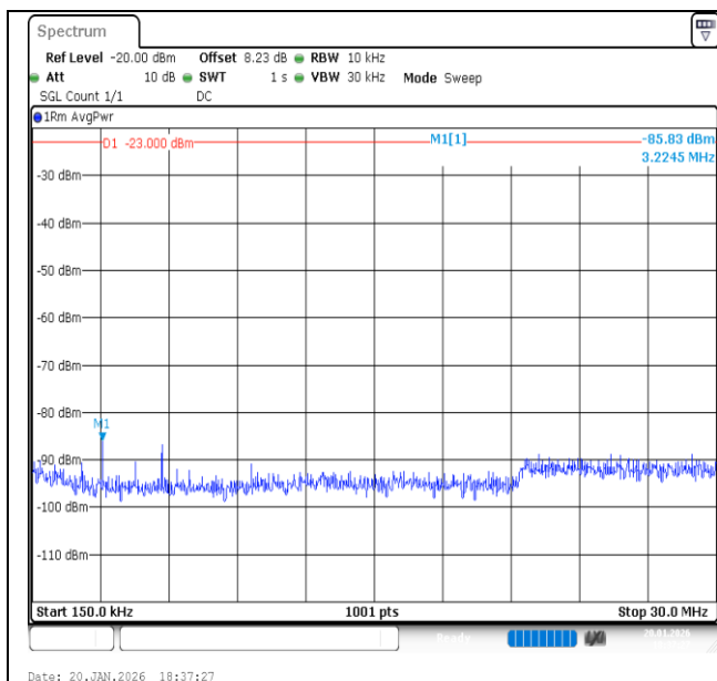
Band13-5MHz-QPSK-23230-1RB#0-0.15~30-PASS
