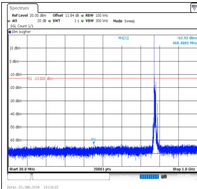
Band13-10MHz-QPSK-23230-1RB#0-30~1000-PASS
