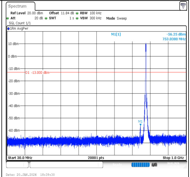
Band13-5MHz-QPSK-23230-25RB#0-30~1000-PASS
