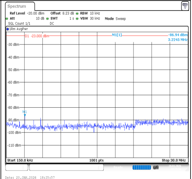
Band13-5MHz-16QAM-23205-1RB#24-0.15~30-PASS
