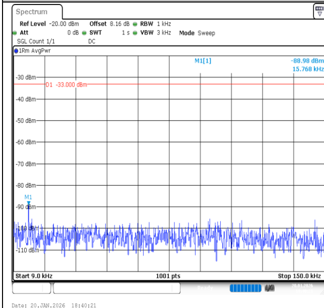
Band13-5MHz-QPSK-23255-1RB#0-0.009~0.15-PASS
