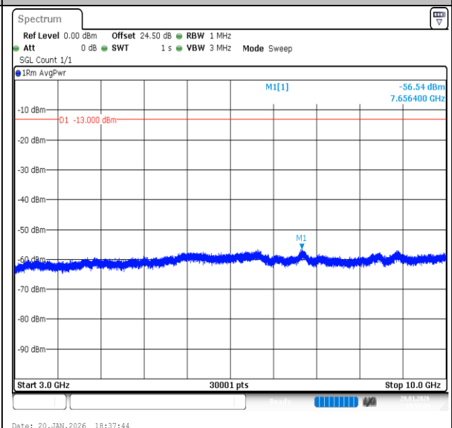
Band13-5MHz-QPSK-23230-1RB#0-3000~10000-PASS
