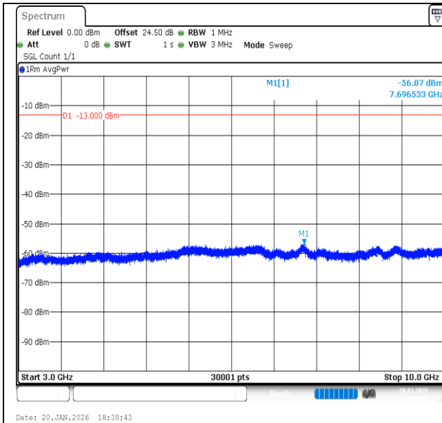
Band13-5MHz-QPSK-23230-1RB#24-3000~10000-PASS
