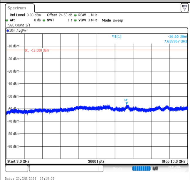
Band13-10MHz-16QAM-23230-50RB#0-3000~10000-PASS
