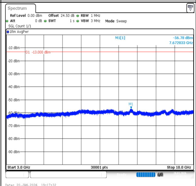
Band13-10MHz-QPSK-23230-1RB#49-3000~10000-PASS
