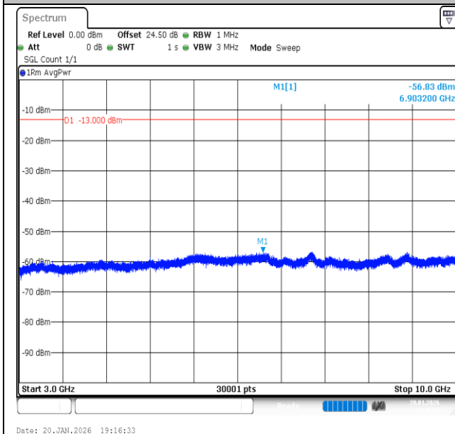
Band13-10MHz-QPSK-23230-1RB#0-3000~10000-PASS
