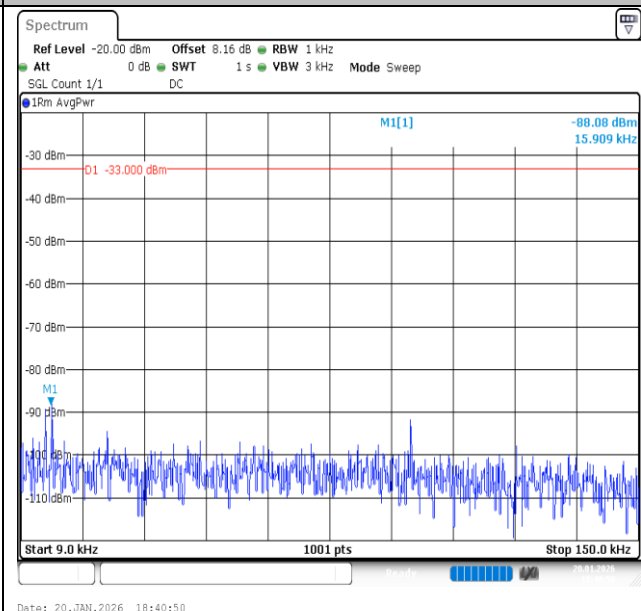
Band13-5MHz-16QAM-23255-1RB#0-0.009~0.15-PASS
