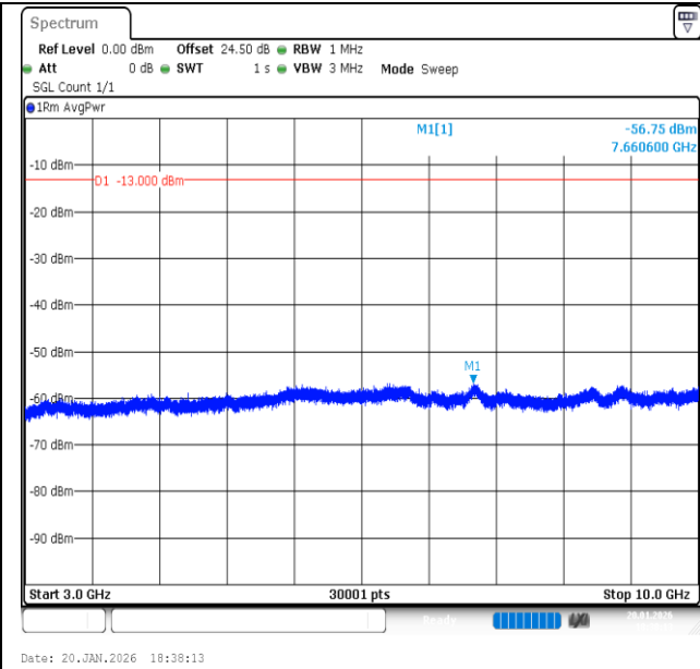
Band13-5MHz-16QAM-23230-1RB#0-3000~10000-PASS
