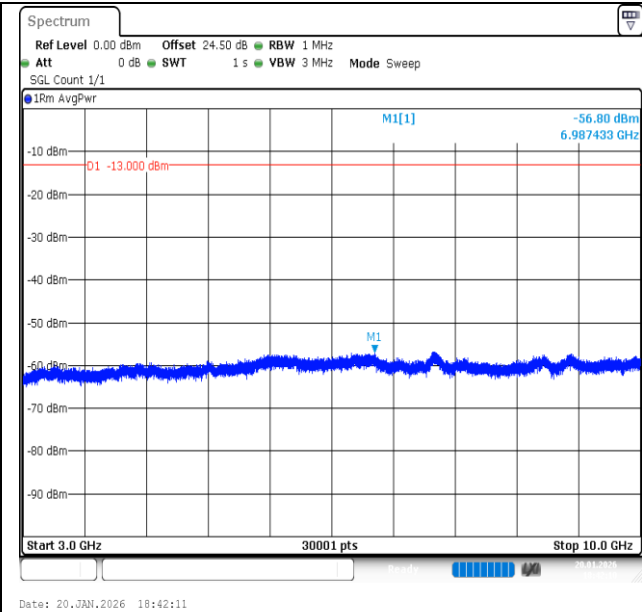
Band13-5MHz-16QAM-23255-1RB#24-3000~10000-PASS
