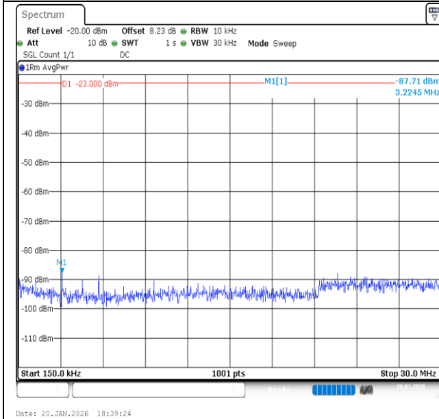
Band13-5MHz-QPSK-23230-25RB#0-0.15~30-PASS
