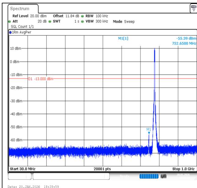
Band13-5MHz-16QAM-23230-25RB#0-30~1000-PASS
