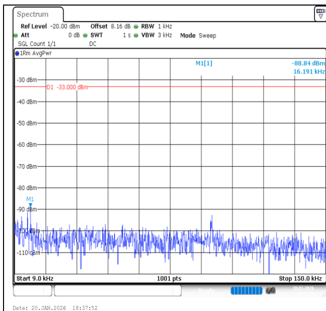
Band13-5MHz-16QAM-23230-1RB#0-0.009~0.15-PASS
