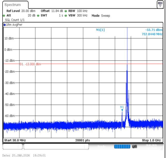
Band13-5MHz-16QAM-23230-1RB#24-30~1000-PASS
