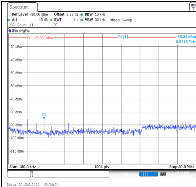
Band13-5MHz-16QAM-23205-25RB#0-0.15~30-PASS
