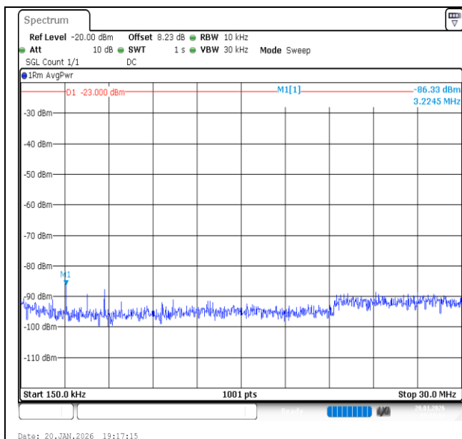
Band13-10MHz-QPSK-23230-1RB#49-0.15~30-PASS
