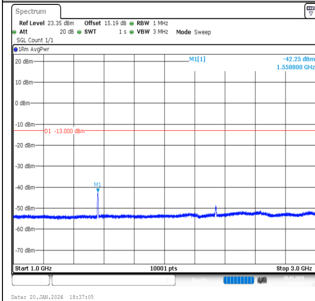
Band13-5MHz-16QAM-23205-25RB#0-1000~3000-PASS
