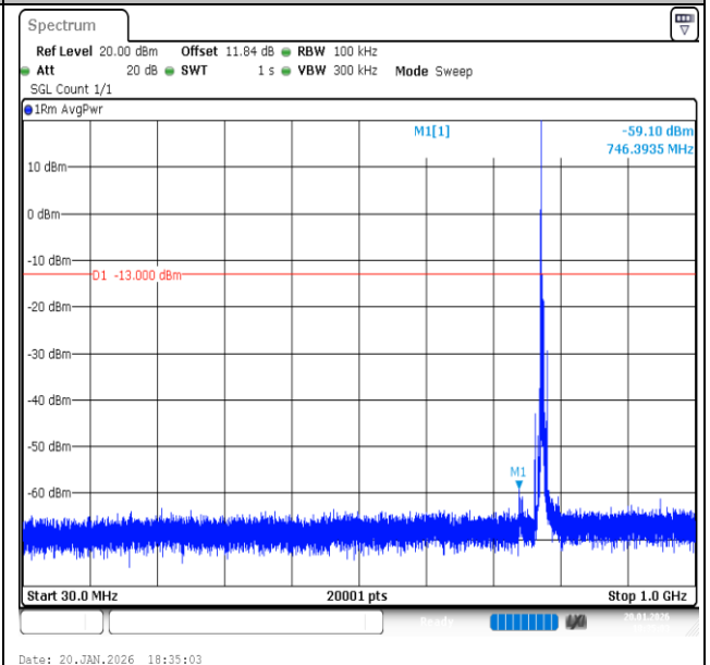
Band13-5MHz-16QAM-23205-1RB#0-30~1000-PASS
