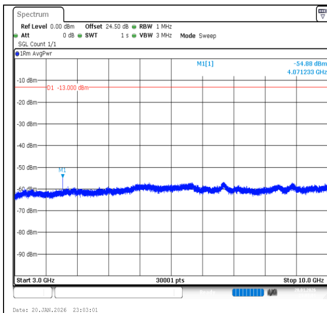
Band26 (814-824)-1.4MHz-QPSK-26697-1RB#0-3000~10000-PASS
