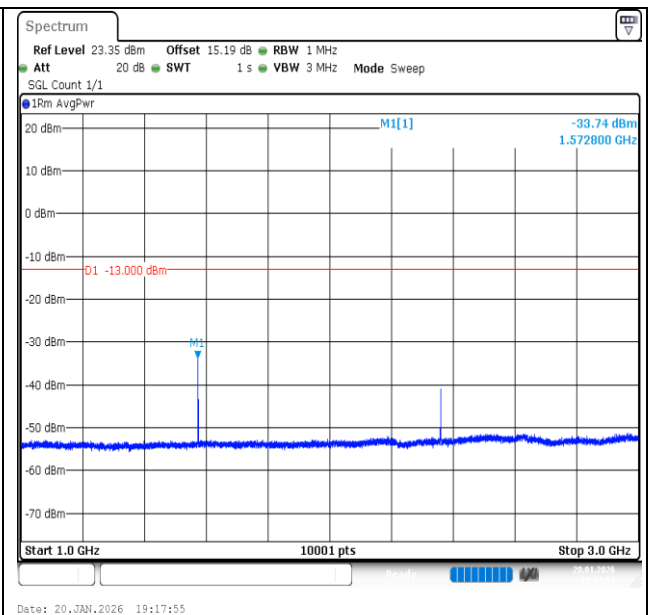
Band13-10MHz-16QAM-23230-1RB#49-1000~3000-PASS
