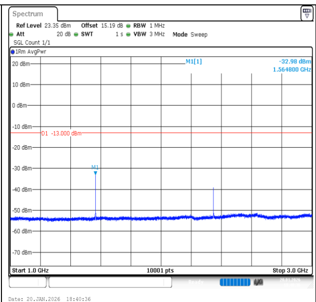
Band13-5MHz-QPSK-23255-1RB#0-1000~3000-PASS
