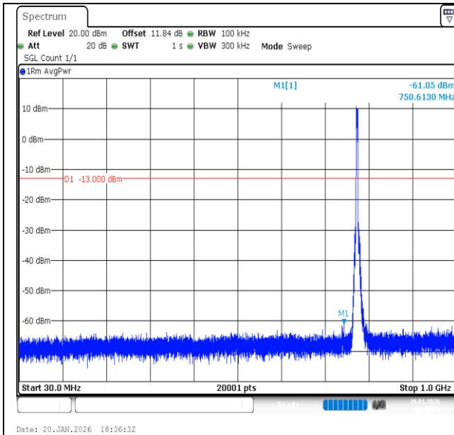
Band13-5MHz-QPSK-23205-25RB#0-30~1000-PASS
