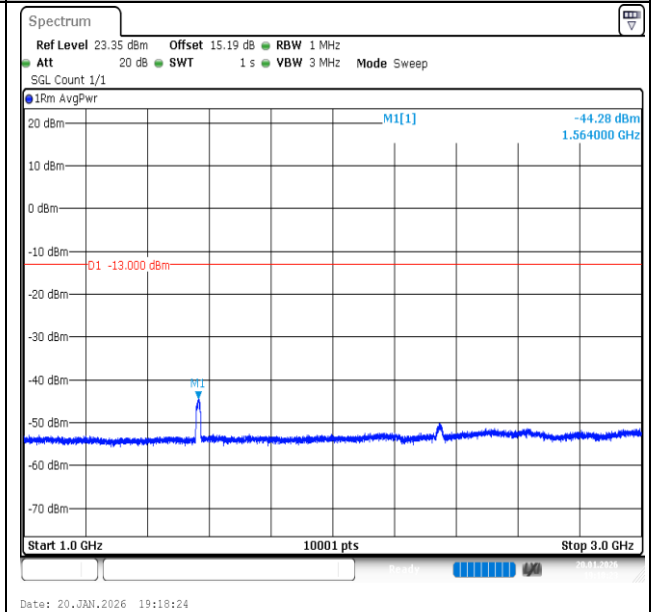
Band13-10MHz-QPSK-23230-50RB#0-1000~3000-PASS
