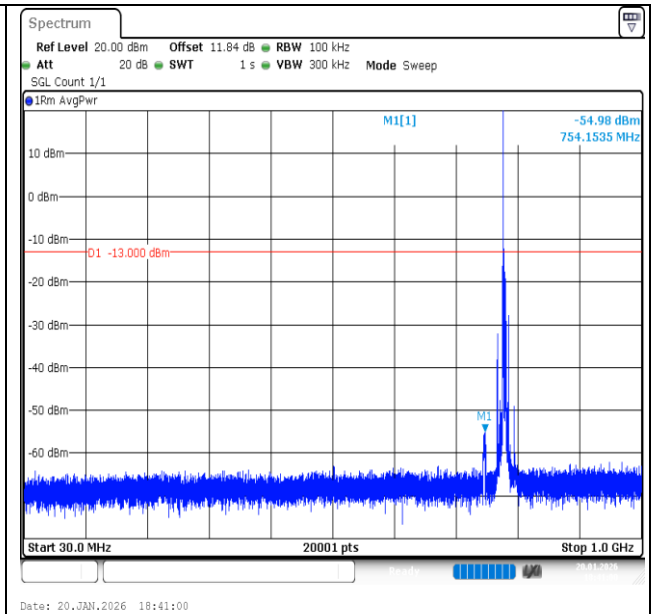
Band13-5MHz-16QAM-23255-1RB#0-30~1000-PASS
