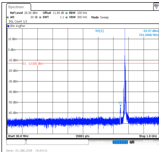
Band13-5MHz-QPSK-23255-1RB#0-30~1000-PASS
