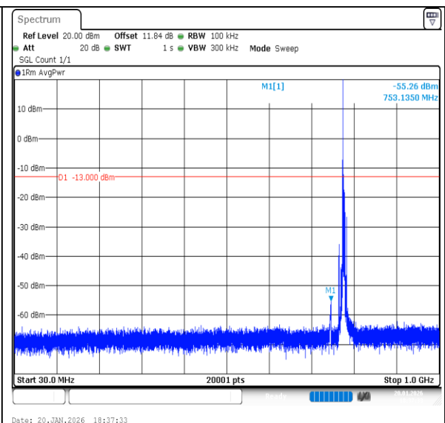
Band13-5MHz-QPSK-23230-1RB#0-30~1000-PASS
