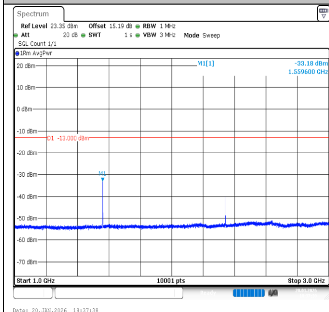
Band13-5MHz-QPSK-23230-1RB#0-1000~3000-PASS
