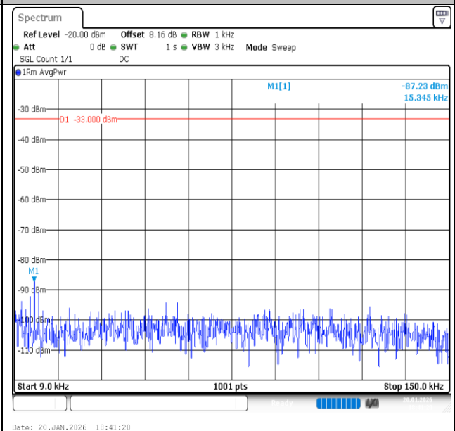
Band13-5MHz-QPSK-23255-1RB#24-0.009~0.15-PASS
