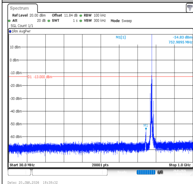
Band13-5MHz-QPSK-23230-1RB#24-30~1000-PASS
