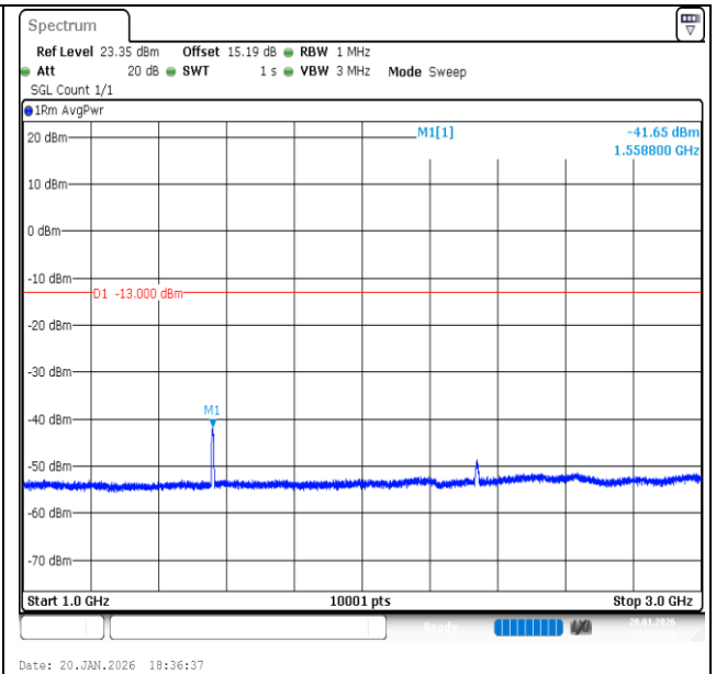
Band13-5MHz-QPSK-23205-25RB#0-1000~3000-PASS
