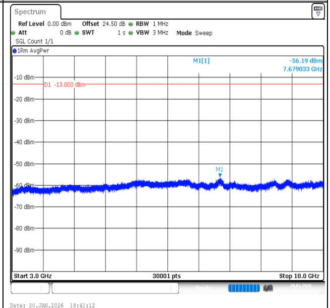
Band13-5MHz-16QAM-23255-1RB#0-3000~10000-PASS
