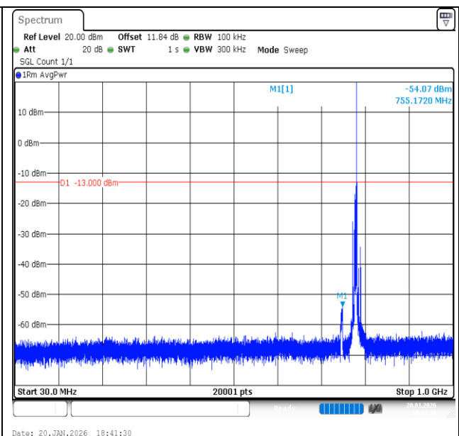
Band13-5MHz-QPSK-23255-1RB#24-30~1000-PASS
