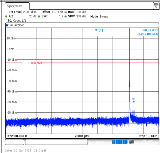
Band26 (814-824)-1.4MHz-QPSK-26697-1RB#5-30~1000-PASS
