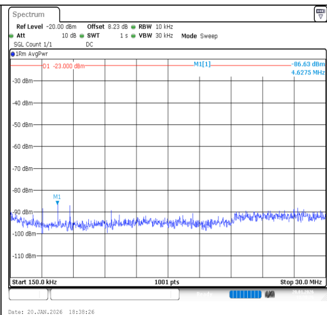
Band13-5MHz-QPSK-23230-1RB#24-0.15~30-PASS
