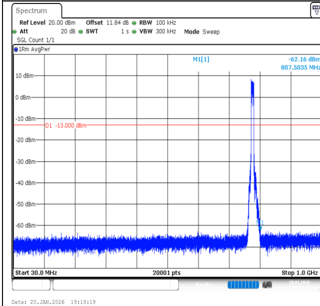
Band13-10MHz-QPSK-23230-50RB#0-30~1000-PASS
