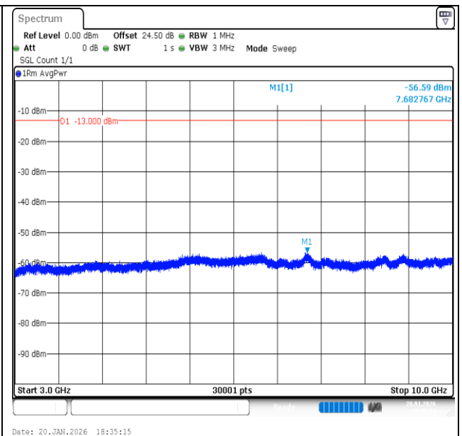
Band13-5MHz-16QAM-23205-1RB#0-3000~10000-PASS
