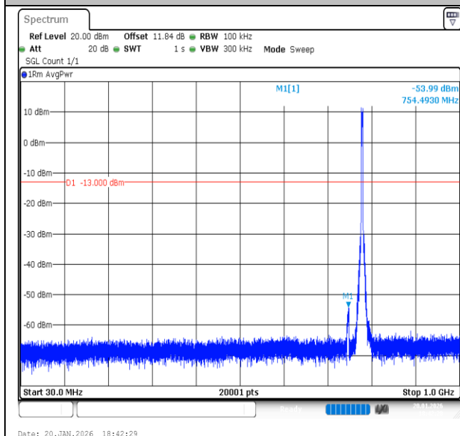
Band13-5MHz-QPSK-23255-25RB#0-30~1000-PASS
