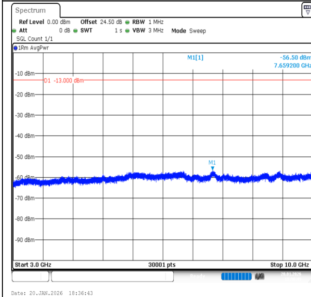
Band13-5MHz-QPSK-23205-25RB#0-3000~10000-PASS
