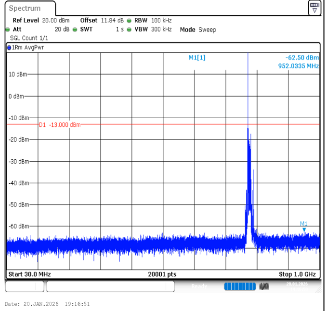
Band13-10MHz-16QAM-23230-1RB#0-30~1000-PASS
