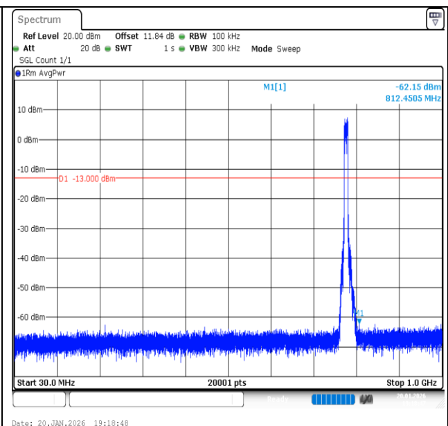
Band13-10MHz-16QAM-23230-50RB#0-30~1000-PASS
