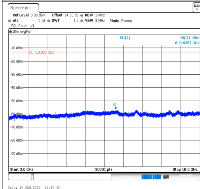
Band13-5MHz-QPSK-23255-1RB#0-3000~10000-PASS
