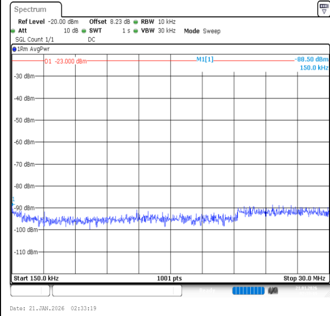
Band26 (824-849)-10MHz-QPSK-26915-1RB#0-0.15~30-PASS
