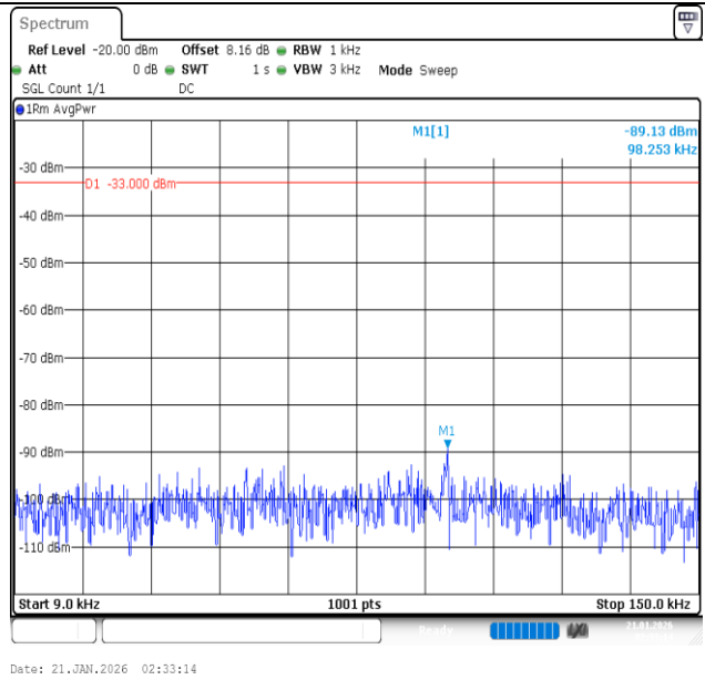
Band26 (824-849)-10MHz-QPSK-26915-1RB#0-0.009~0.15-PASS
