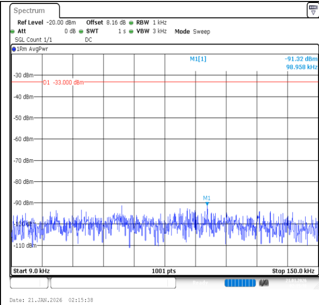
Band26 (824-849)-5MHz-QPSK-26915-1RB#24-0.009~0.15-PASS
