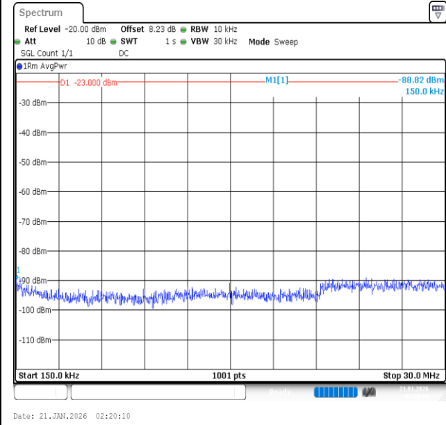
Band26 (824-849)-5MHz-16QAM-27015-25RB#0-0.15~30-PASS
