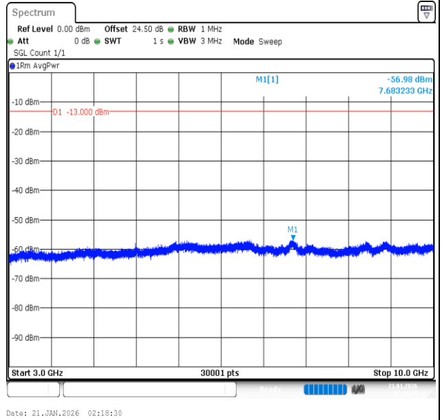
Band26 (824-849)-5MHz-16QAM-27015-1RB#0-3000~10000-PASS
