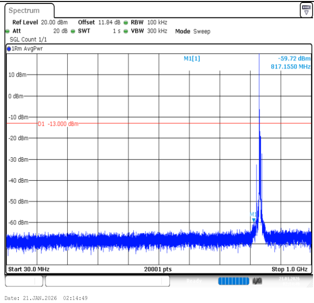
Band26 (824-849)-5MHz-QPSK-26915-1RB#0-30~1000-PASS
