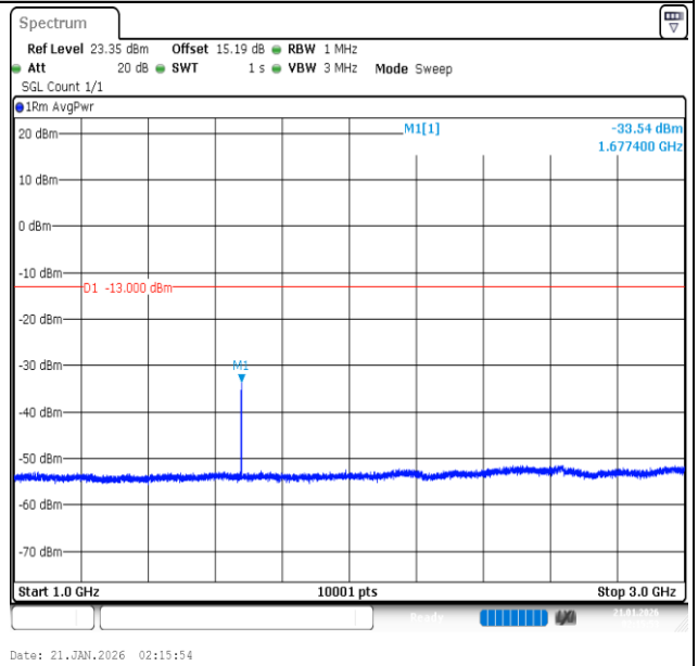
Band26 (824-849)-5MHz-QPSK-26915-1RB#24-1000~3000-PASS
