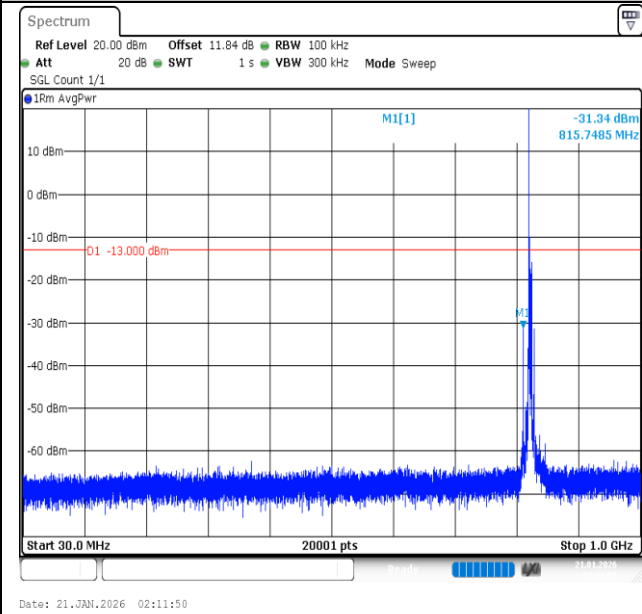
Band26 (824-849)-5MHz-QPSK-26815-1RB#0-30~1000-PASS
