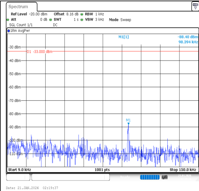
Band26 (824-849)-5MHz-QPSK-27015-25RB#0-0.009~0.15-PASS
