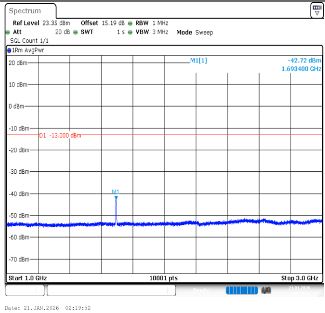
Band26 (824-849)-5MHz-QPSK-27015-25RB#0-1000~3000-PASS
