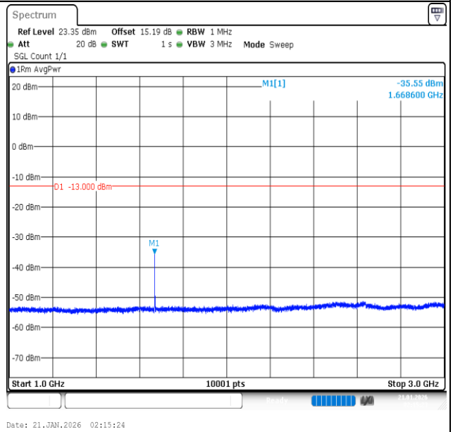
Band26 (824-849)-5MHz-16QAM-26915-1RB#0-1000~3000-PASS
