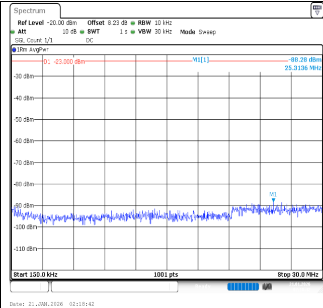
Band26 (824-849)-5MHz-QPSK-27015-1RB#24-0.15~30-PASS
