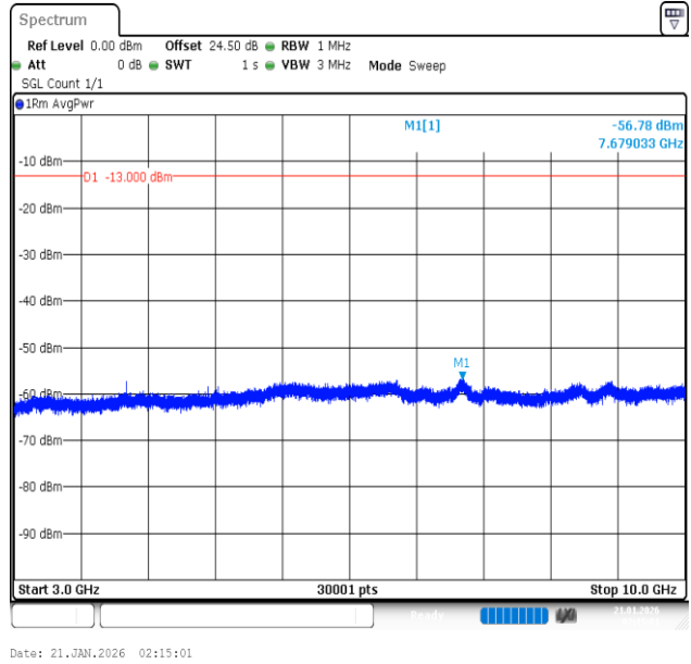
Band26 (824-849)-5MHz-QPSK-26915-1RB#0-3000~10000-PASS
