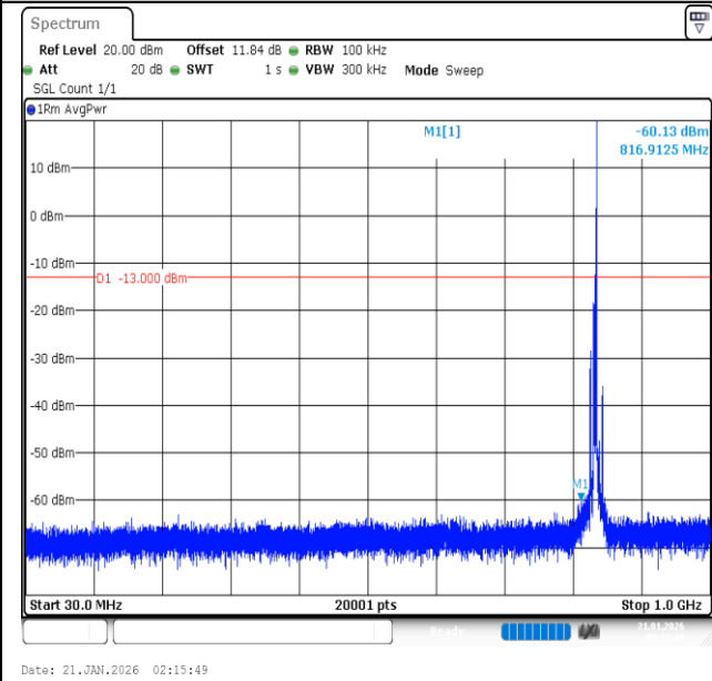
Band26 (824-849)-5MHz-QPSK-26915-1RB#24-30~1000-PASS
