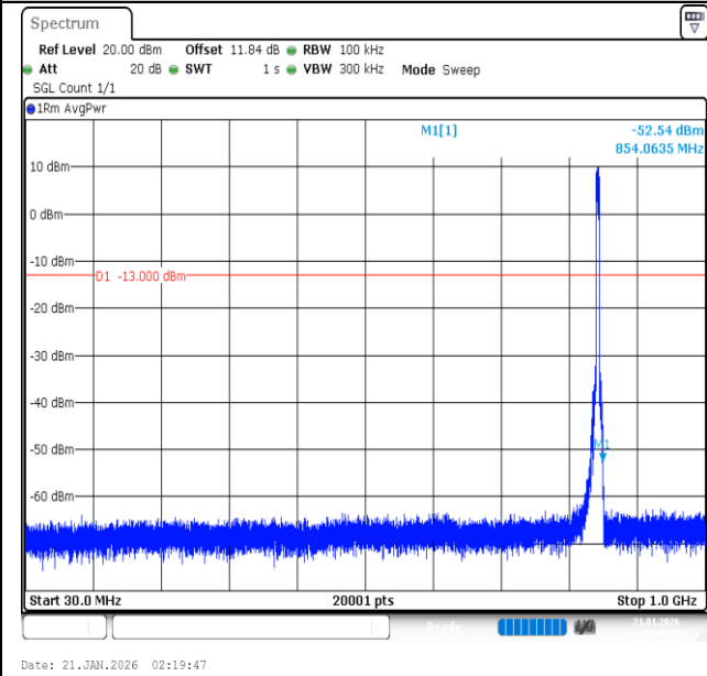
Band26 (824-849)-5MHz-QPSK-27015-25RB#0-30~1000-PASS
