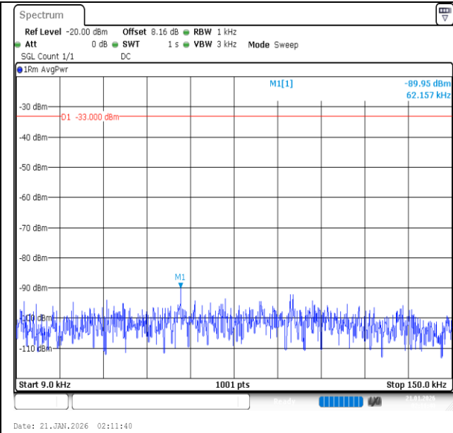
Band26 (824-849)-5MHz-QPSK-26815-1RB#0-0.009~0.15-PASS
