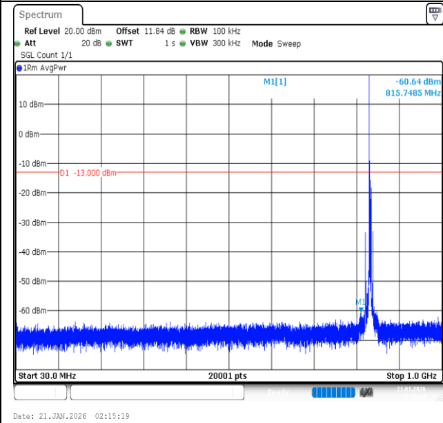
Band26 (824-849)-5MHz-16QAM-26915-1RB#0-30~1000-PASS
