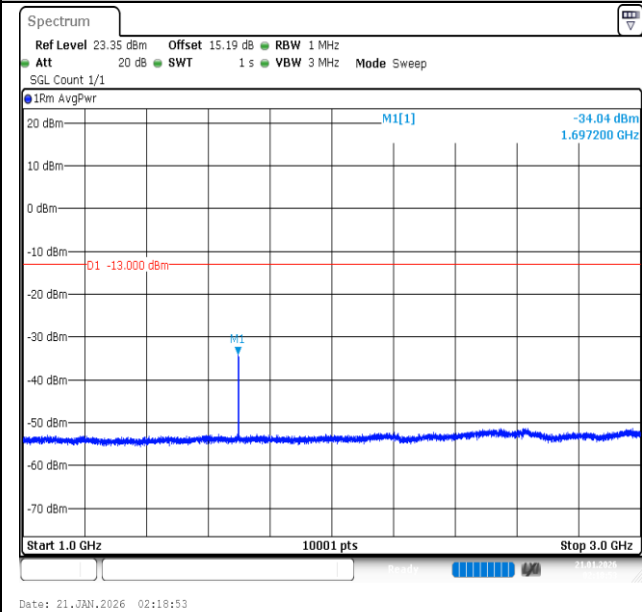
Band26 (824-849)-5MHz-QPSK-27015-1RB#24-1000~3000-PASS
