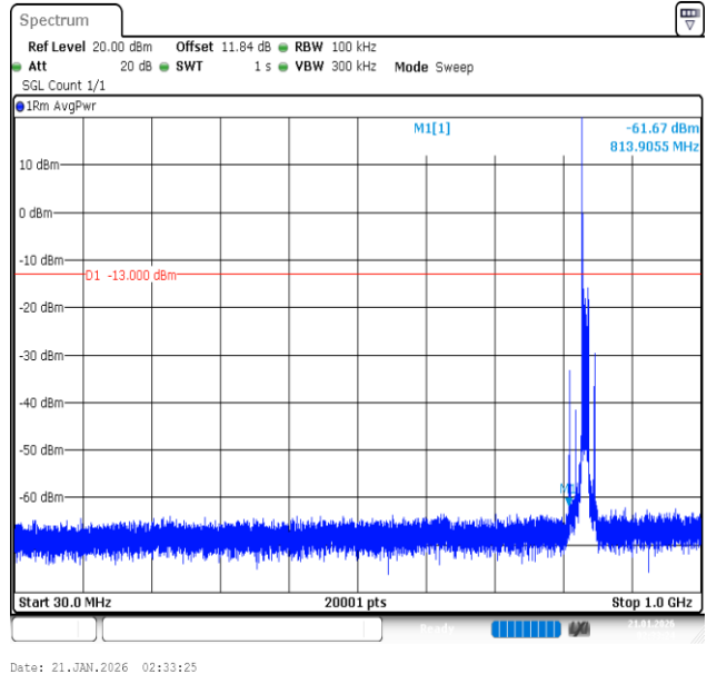
Band26 (824-849)-10MHz-QPSK-26915-1RB#0-30~1000-PASS
