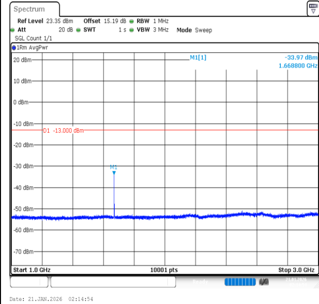
Band26 (824-849)-5MHz-QPSK-26915-1RB#0-1000~3000-PASS
