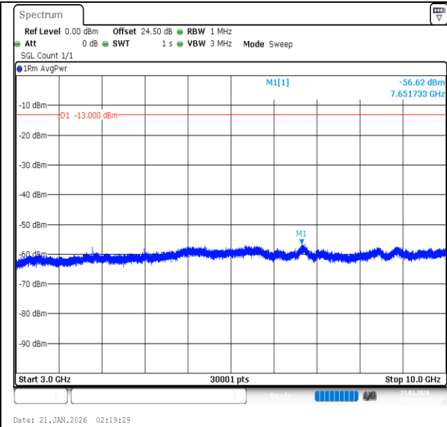
Band26 (824-849)-5MHz-16QAM-27015-1RB#24-3000~10000-PASS
