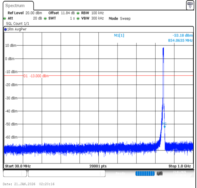
Band26 (824-849)-5MHz-16QAM-27015-25RB#0-30~1000-PASS
