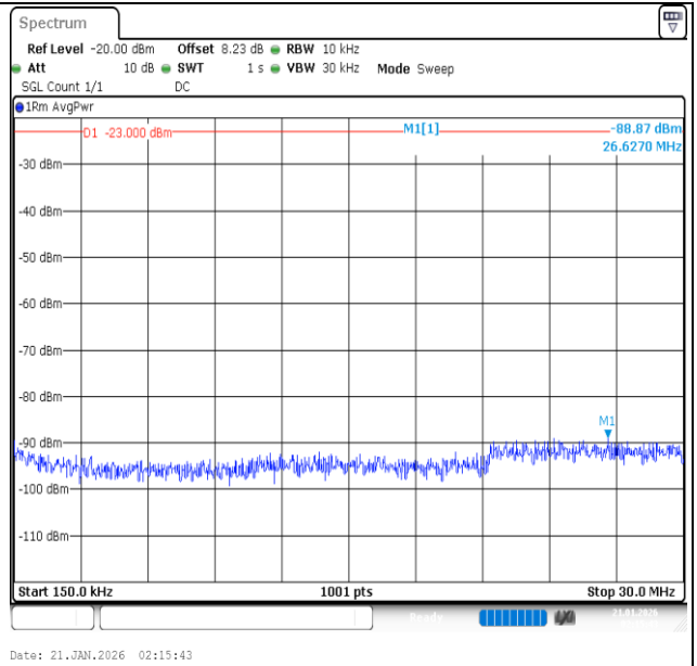
Band26 (824-849)-5MHz-QPSK-26915-1RB#24-0.15~30-PASS
