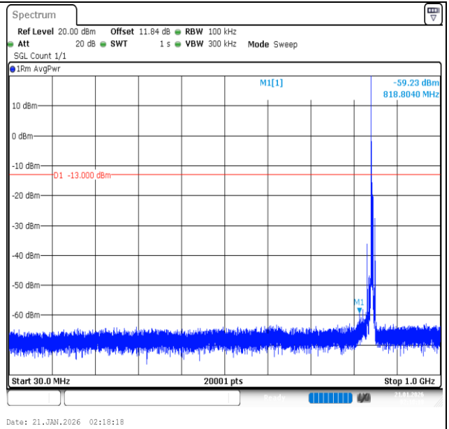
Band26 (824-849)-5MHz-16QAM-27015-1RB#0-30~1000-PASS
