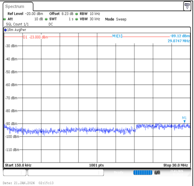
Band26 (824-849)-5MHz-16QAM-26915-1RB#0-0.15~30-PASS
