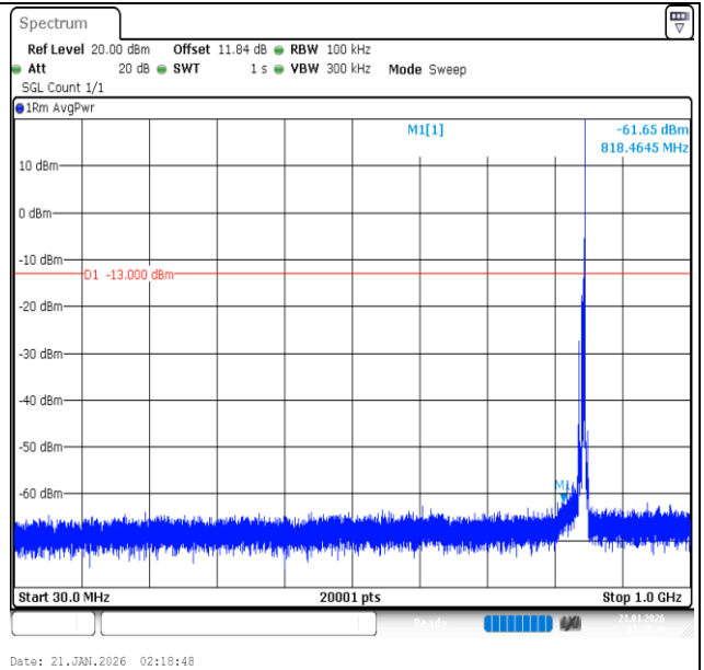
Band26 (824-849)-5MHz-QPSK-27015-1RB#24-30~1000-PASS
