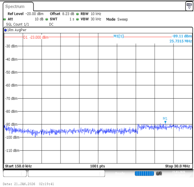
Band26 (824-849)-5MHz-QPSK-27015-25RB#0-0.15~30-PASS
