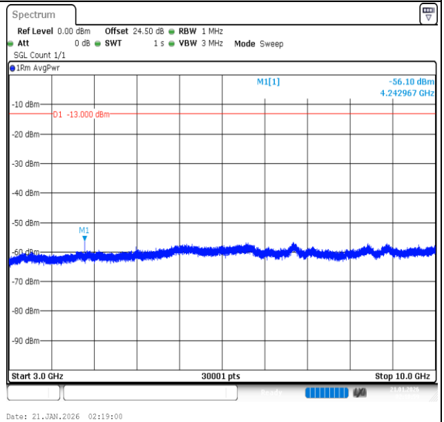
Band26 (824-849)-5MHz-QPSK-27015-1RB#24-3000~10000-PASS
