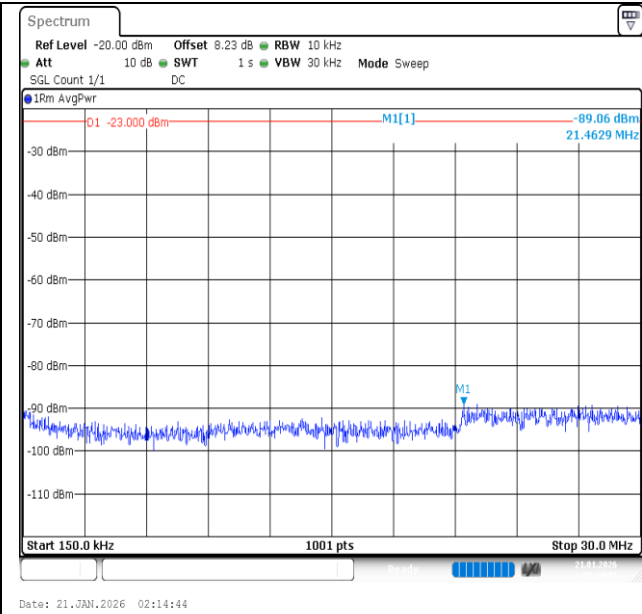
Band26 (824-849)-5MHz-QPSK-26915-1RB#0-0.15~30-PASS
