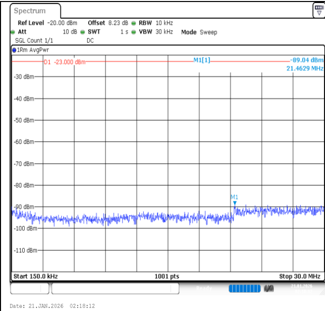
Band26 (824-849)-5MHz-16QAM-27015-1RB#0-0.15~30-PASS
