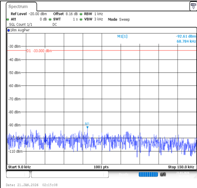
Band26 (824-849)-5MHz-16QAM-26915-1RB#0-0.009~0.15-PASS
