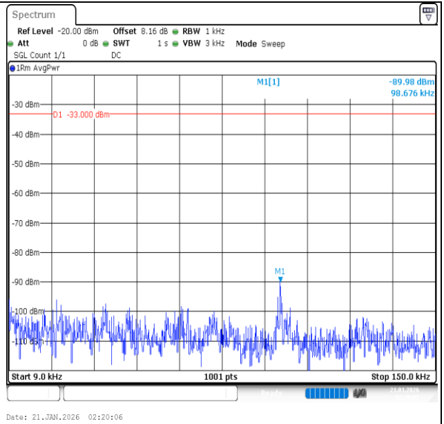
Band26 (824-849)-5MHz-16QAM-27015-25RB#0-0.009~0.15-PASS
