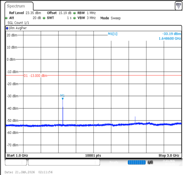
Band26 (824-849)-5MHz-QPSK-26815-1RB#0-1000~3000-PASS
