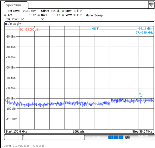
Band26 (824-849)-5MHz-QPSK-26815-1RB#0-0.15~30-PASS
