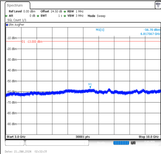
Band26 (824-849)-10MHz-QPSK-26840-50RB#0-3000~10000-PASS
