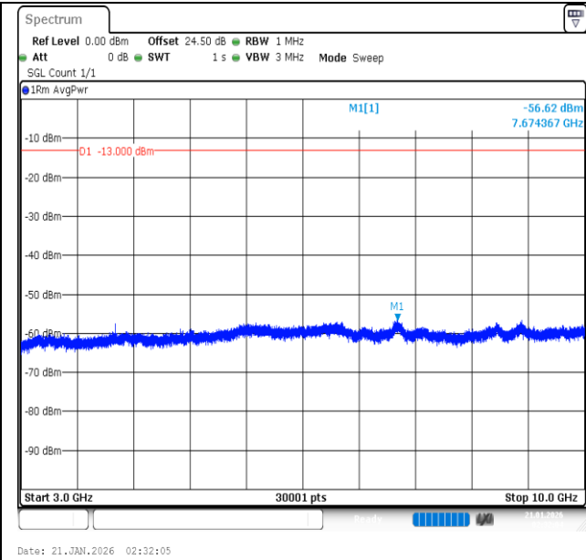
Band26 (824-849)-10MHz-16QAM-26840-1RB#49-3000~10000-PASS
