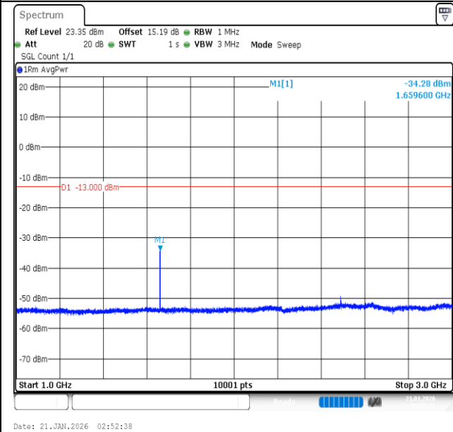
Band26 (824-849)-15MHz-QPSK-26915-1RB#0-1000~3000-PASS
