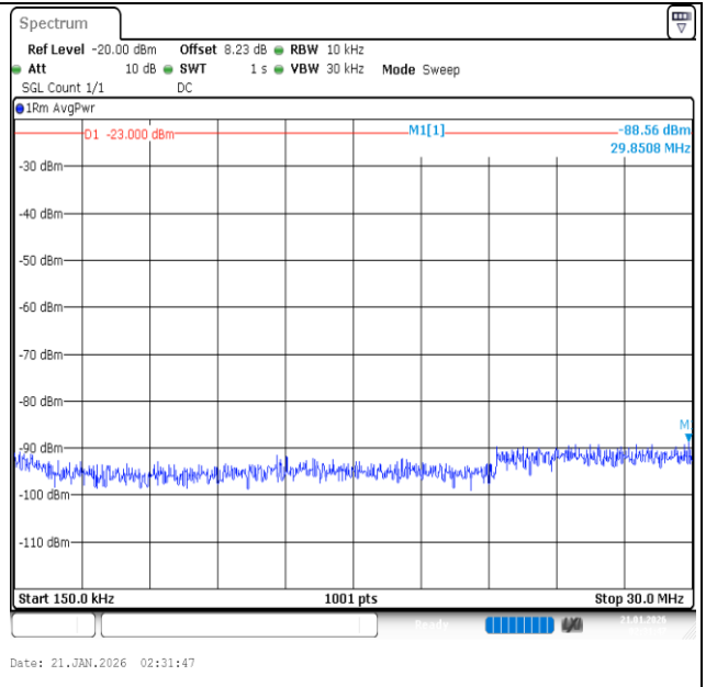
Band26 (824-849)-10MHz-16QAM-26840-1RB#49-0.15~30-PASS
