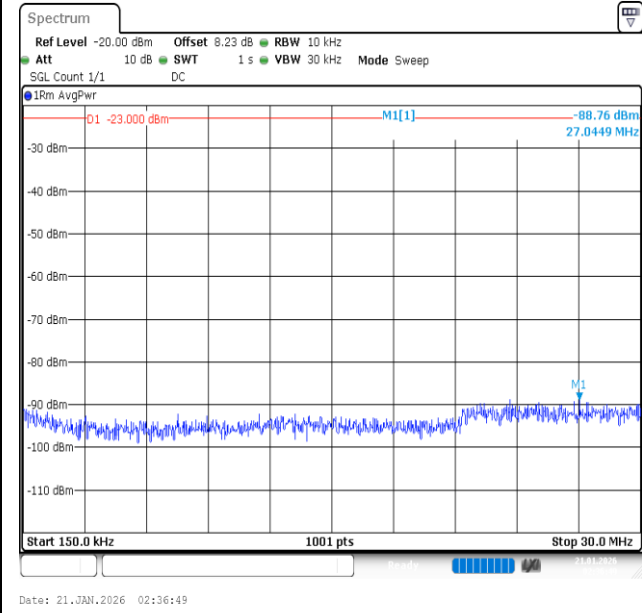
Band26 (824-849)-10MHz-16QAM-26990-1RB#0-0.15~30-PASS
