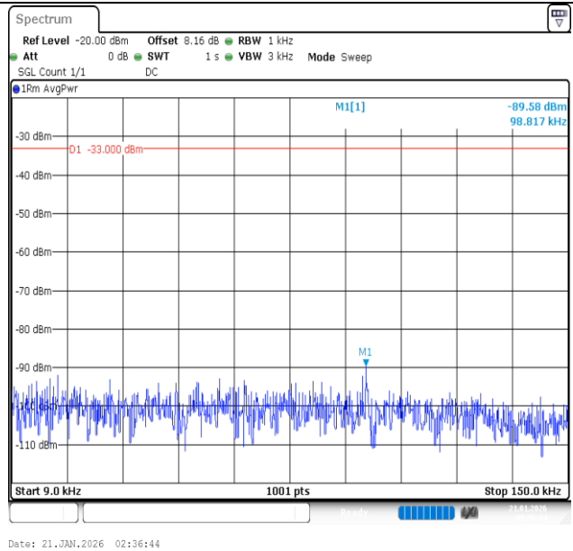
Band26 (824-849)-10MHz-16QAM-26990-1RB#0-0.009~0.15-PASS
