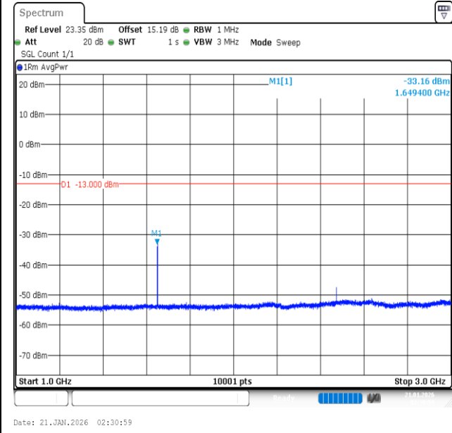
Band26 (824-849)-10MHz-16QAM-26840-1RB#0-1000~3000-PASS
