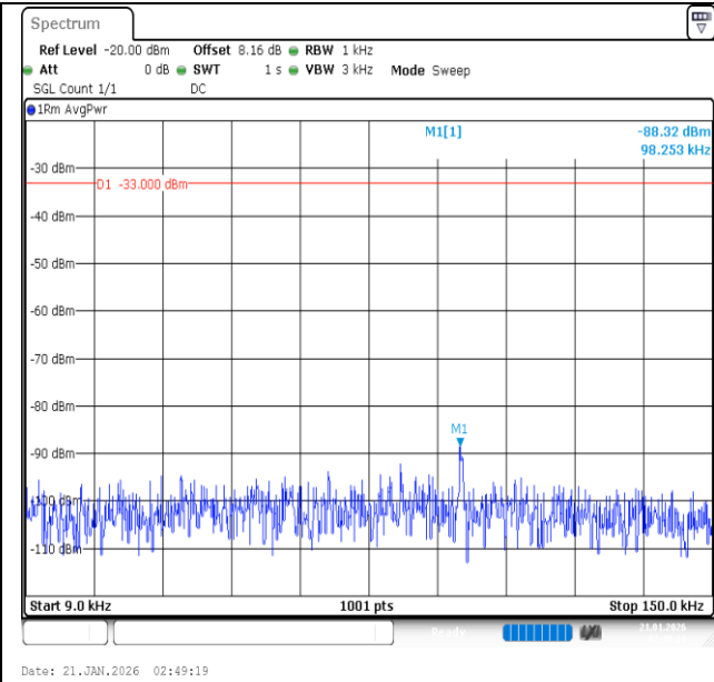
Band26 (824-849)-15MHz-QPSK-26865-1RB#0-0.009~0.15-PASS
