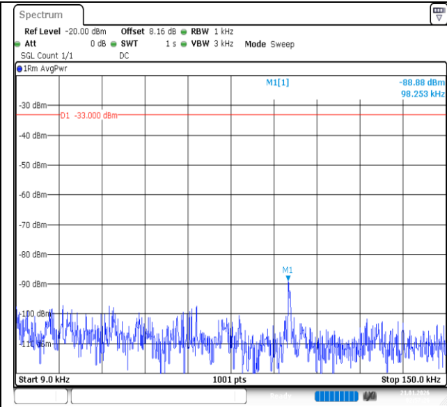
Band26 (824-849)-15MHz-QPSK-26965-75RB#0-0.009~0.15-PASS
