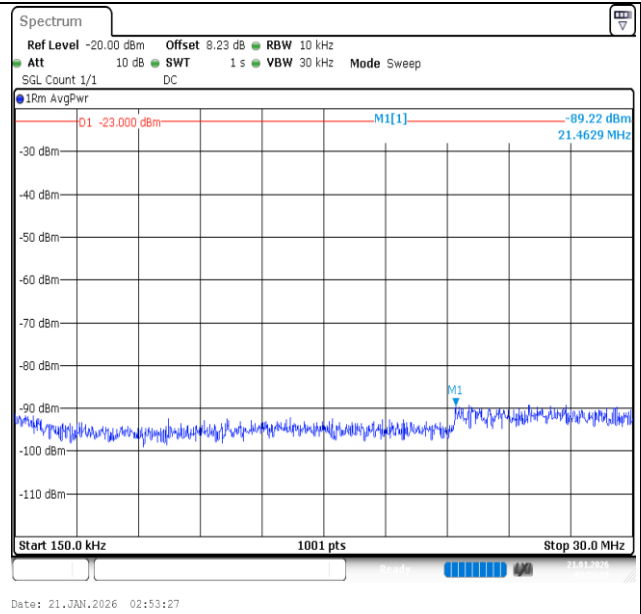
Band26 (824-849)-15MHz-QPSK-26915-1RB#74-0.15~30-PASS
