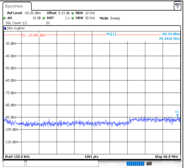
Band26 (824-849)-15MHz-QPSK-26965-75RB#0-0.15~30-PASS
