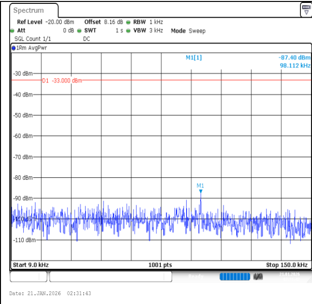
Band26 (824-849)-10MHz-16QAM-26840-1RB#49-0.009~0.15-PASS
