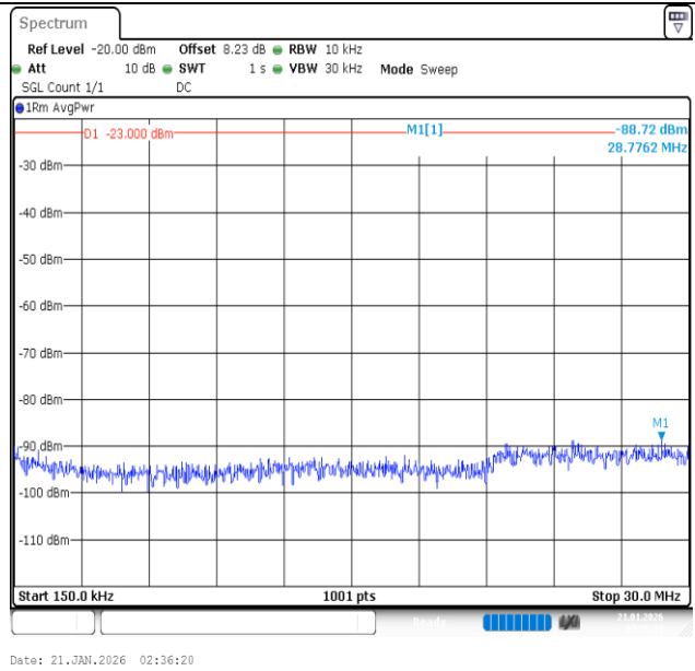
Band26 (824-849)-10MHz-QPSK-26990-1RB#0-0.15~30-PASS
