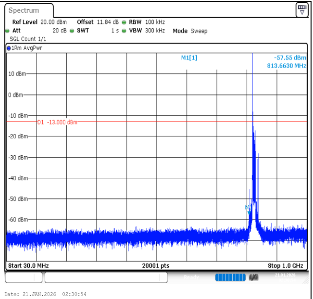
Band26 (824-849)-10MHz-16QAM-26840-1RB#0-30~1000-PASS
