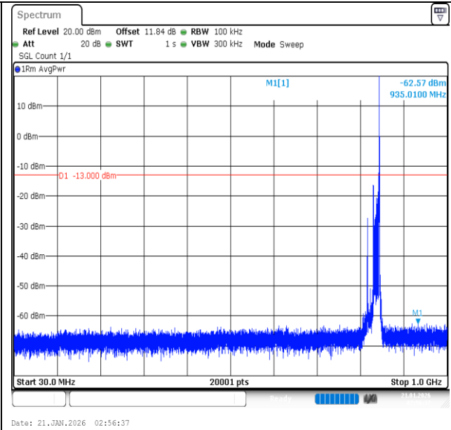
Band26 (824-849)-15MHz-QPSK-26965-1RB#74-30~1000-PASS
