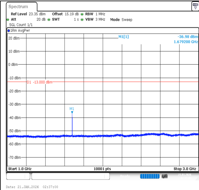
Band26 (824-849)-10MHz-16QAM-26990-1RB#0-1000~3000-PASS
