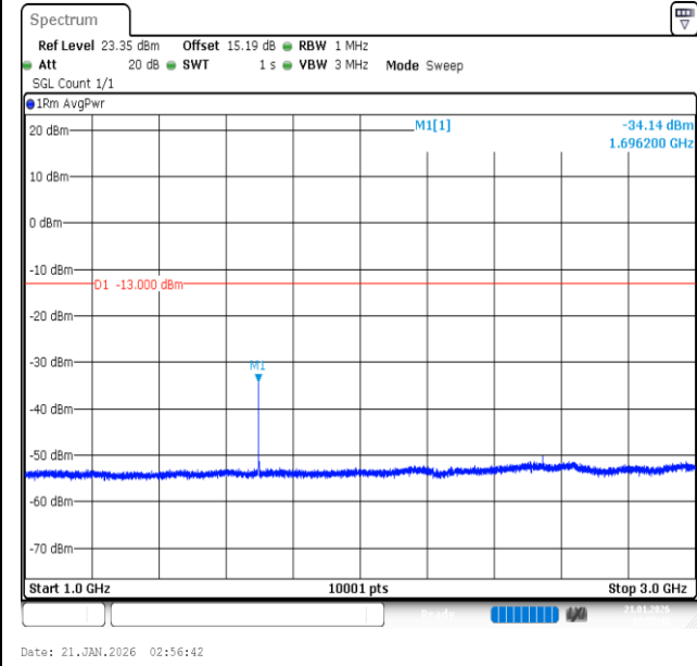
Band26 (824-849)-15MHz-QPSK-26965-1RB#74-1000~3000-PASS
