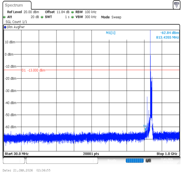
Band26 (824-849)-10MHz-16QAM-26990-1RB#0-30~1000-PASS
