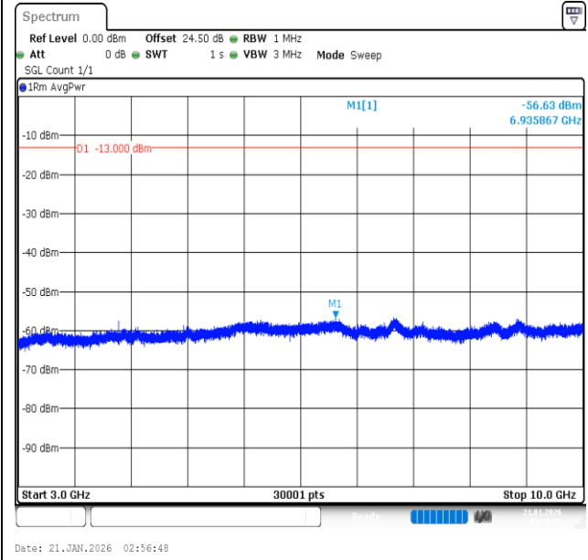
Band26 (824-849)-15MHz-QPSK-26965-1RB#74-3000~10000-PASS
