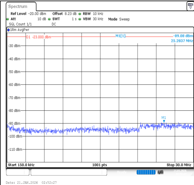
Band26 (824-849)-15MHz-QPSK-26915-1RB#0-0.15~30-PASS
