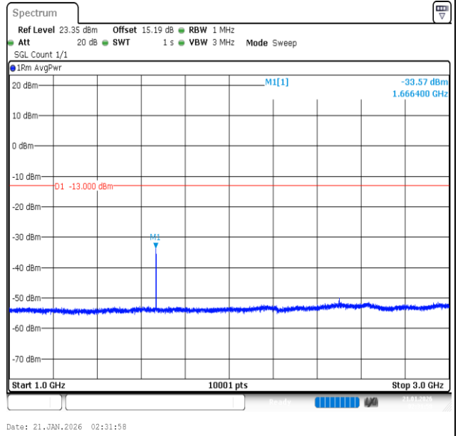
Band26 (824-849)-10MHz-16QAM-26840-1RB#49-1000~3000-PASS
