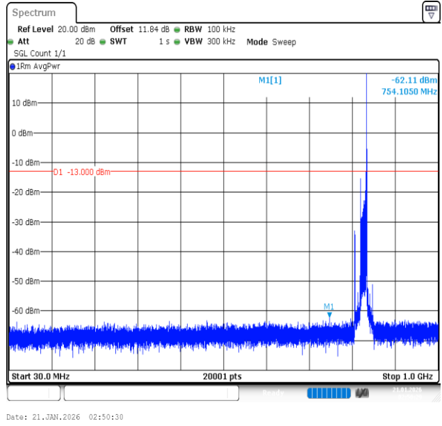
Band26 (824-849)-15MHz-QPSK-26865-1RB#74-30-1000-PASS
