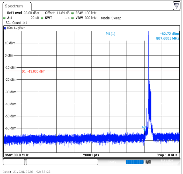
Band26 (824-849)-15MHz-QPSK-26915-1RB#0-30~1000-PASS
