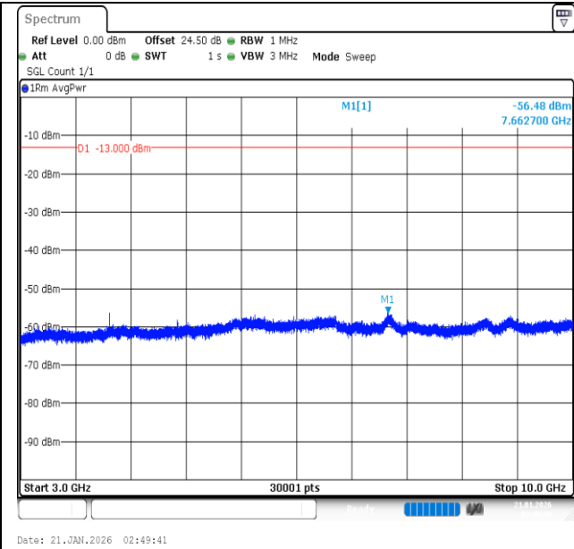
Band26 (824-849)-15MHz-QPSK-26865-1RB#0-3000-10000-PASS
