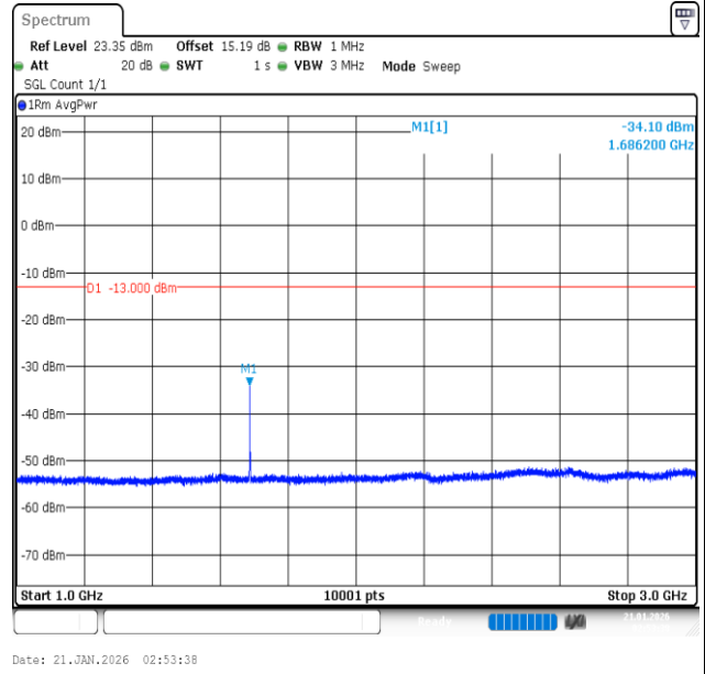
Band26 (824-849)-15MHz-QPSK-26915-1RB#74-1000~3000-PASS
