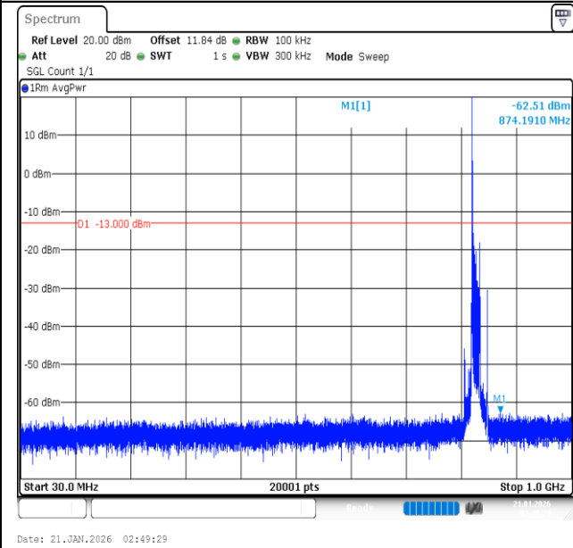
Band26 (824-849)-15MHz-QPSK-26865-1RB#0-30~1000-PASS
