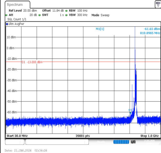
Band26 (824-849)-10MHz-QPSK-26990-1RB#0-30~1000-PASS
