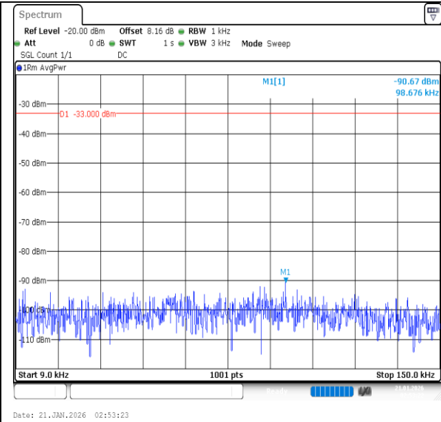
Band26 (824-849)-15MHz-QPSK-26915-1RB#74-0.009~0.15-PASS
