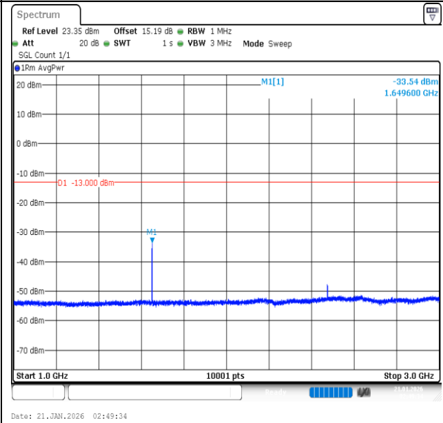
Band26 (824-849)-15MHz-QPSK-26865-1RB#0-1000~3000-PASS
