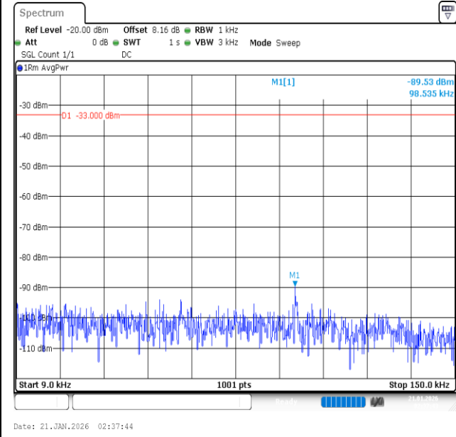
Band26 (824-849)-10MHz-16QAM-26990-1RB#49-0.009~0.15-PASS
