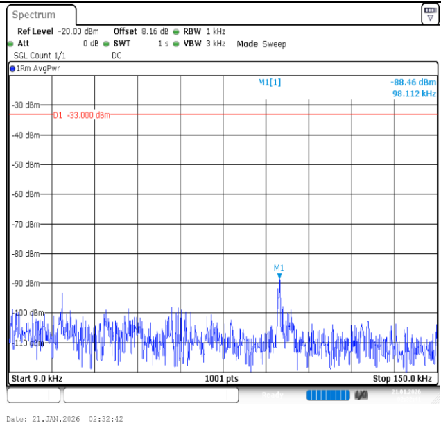
Band26 (824-849)-10MHz-16QAM-26840-50RB#0-0.009~0.15-PASS
