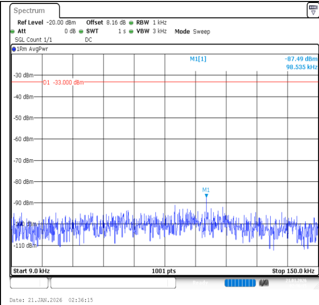
Band26 (824-849)-10MHz-QPSK-26990-1RB#0-0.009~0.15-PASS
