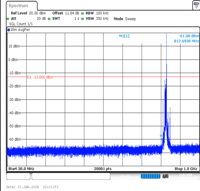
Band26 (824-849)-10MHz-16QAM-26840-1RB#49-30~1000-PASS
