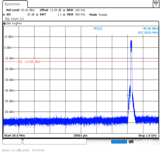
Band26 (824-849)-10MHz-16QAM-26840-50RB#0-30~1000-PASS
