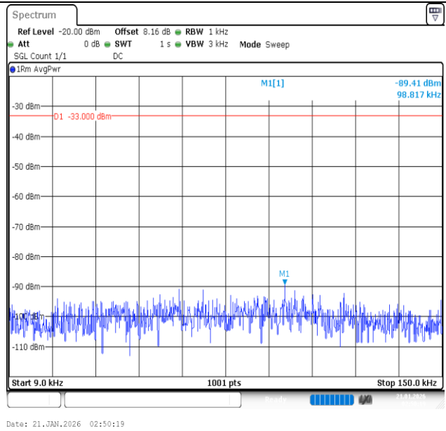
Band26 (824-849)-15MHz-QPSK-26865-1RB#74-0.009-0.15-PASS
