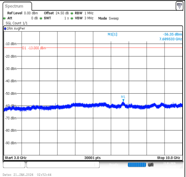
Band26 (824-849)-15MHz-QPSK-26915-1RB#0-3000~10000-PASS
