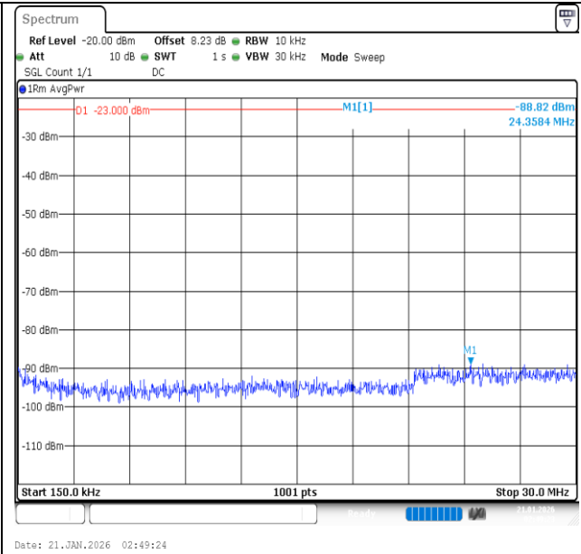
Band26 (824-849)-15MHz-QPSK-26865-1RB#0-0.15~30-PASS
