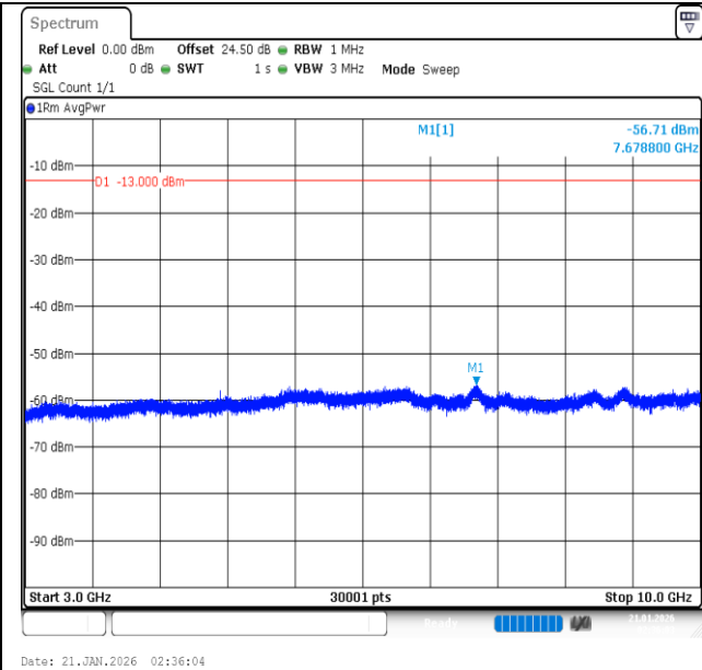
Band26 (824-849)-10MHz-16QAM-26915-50RB#0-3000~10000-PASS
