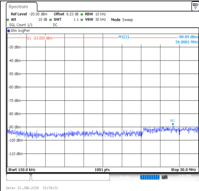
Band26 (824-849)-15MHz-QPSK-26965-1RB#74-0.15~30-PASS
