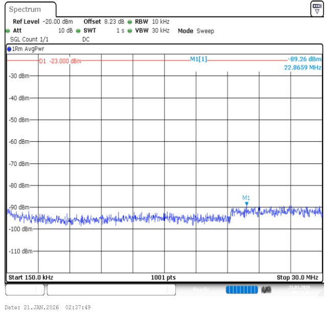
Band26 (824-849)-10MHz-16QAM-26990-1RB#49-0.15~30-PASS
