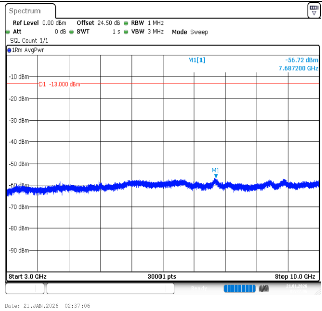
Band26 (824-849)-10MHz-16QAM-26990-1RB#0-3000~10000-PASS
