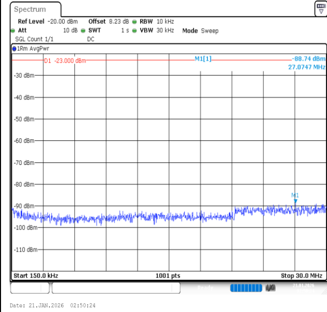
Band26 (824-849)-15MHz-QPSK-26865-1RB#74-0.15-30-PASS
