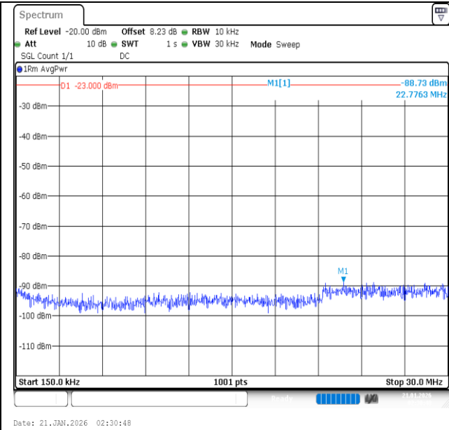
Band26 (824-849)-10MHz-16QAM-26840-1RB#0-0.15~30-PASS
