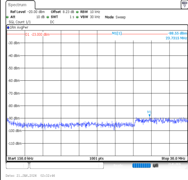
Band26 (824-849)-10MHz-16QAM-26840-50RB#0-0.15~30-PASS
