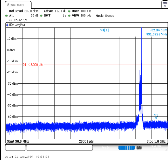
Band26 (824-849)-15MHz-QPSK-26915-1RB#74-30~1000-PASS
