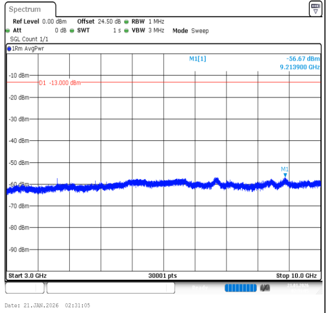
Band26 (824-849)-10MHz-16QAM-26840-1RB#0-3000~10000-PASS
