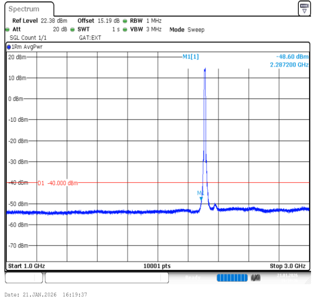
Band40 (2305-2315)-10MHz-16QAM-38750-50RB#0-1000~3000-PASS
