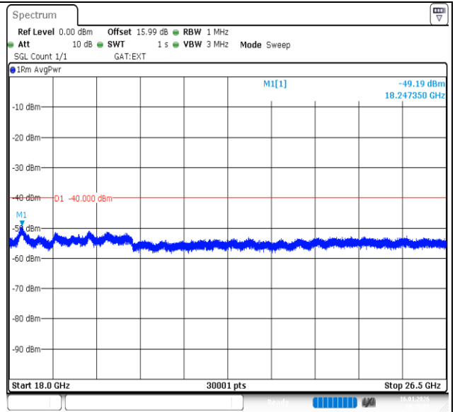
Band40 (2305-2315)-5MHz-16QAM-38775-1RB#0-18000~26500-PASS
