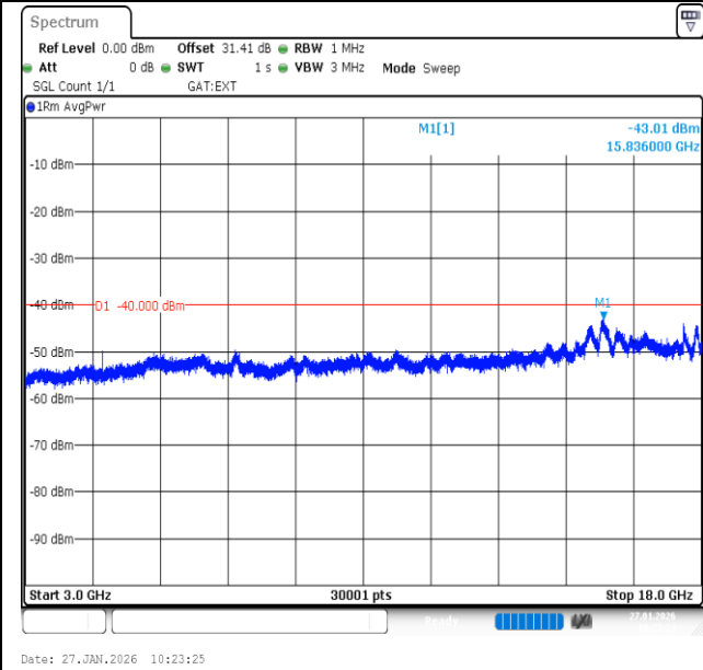
Band40 (2350-2360)-5MHz-QPSK-39200-1RB#24-3000~18000-PASS
