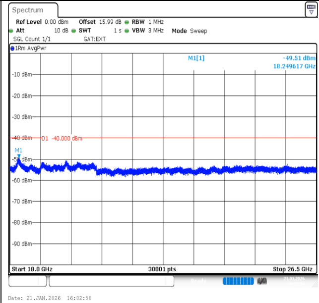
Band40 (2305-2315)-10MHz-QPSK-38750-1RB#0-18000~26500-PASS
