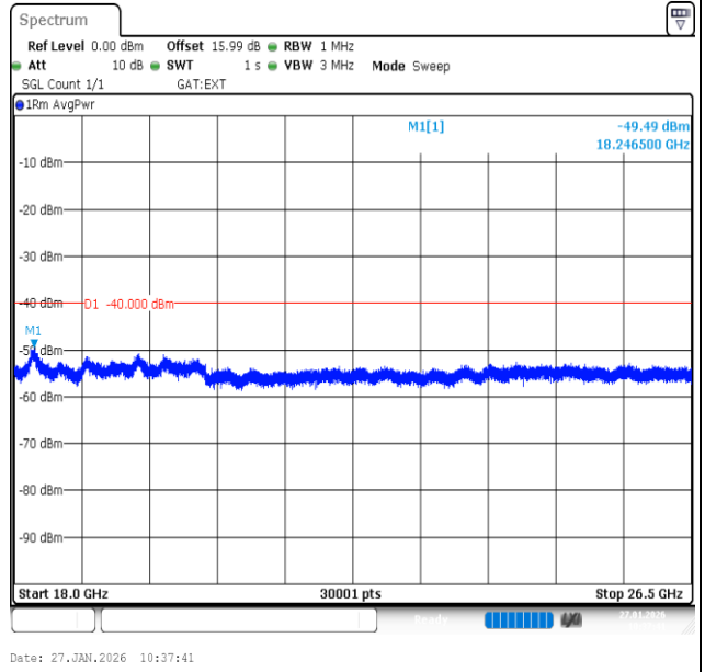
Band40 (2350-2360)-5MHz-QPSK-39225-1RB#0-18000~26500-PASS
