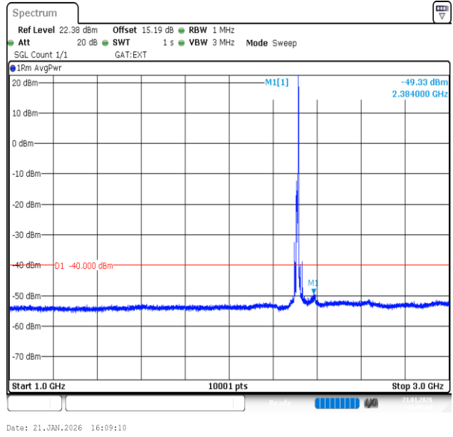
Band40 (2305-2315)-10MHz-QPSK-38750-1RB#49-1000~3000-PASS
