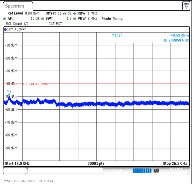
Band40 (2350-2360)-5MHz-QPSK-39200-1RB#24-18000~26500-PASS
