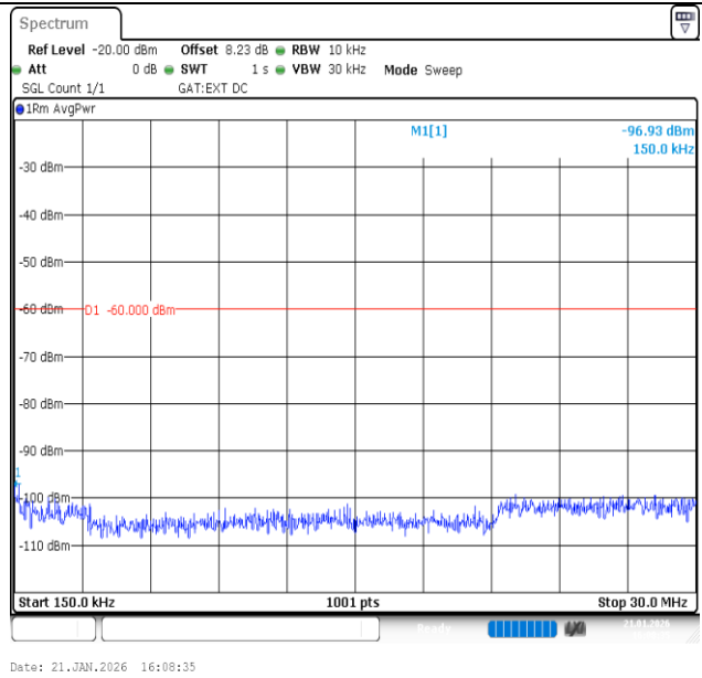
Band40 (2305-2315)-10MHz-QPSK-38750-1RB#49-0.15~30-PASS
