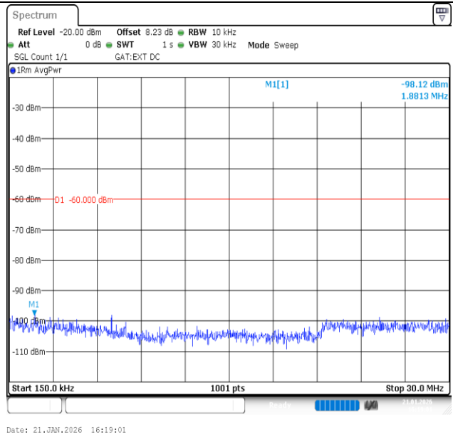
Band40 (2305-2315)-10MHz-16QAM-38750-50RB#0-0.15~30-PASS
