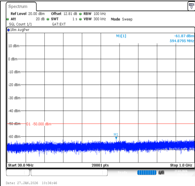
Band40 (2350-2360)-5MHz-QPSK-39225-1RB#0-30~1000-PASS
