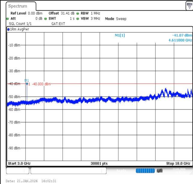
Band40 (2305-2315)-10MHz-QPSK-38750-1RB#0-3000~18000-PASS
