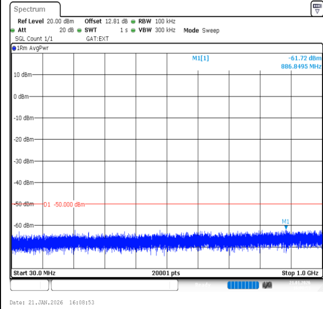
Band40 (2305-2315)-10MHz-QPSK-38750-1RB#49-30~1000-PASS
