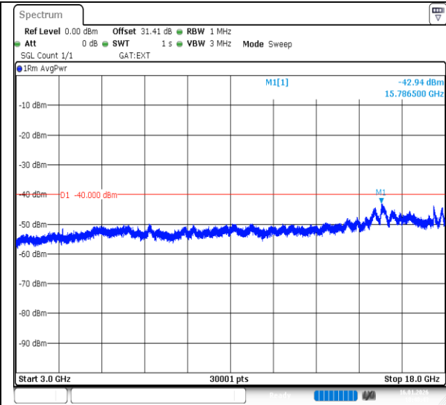
Band40 (2305-2315)-5MHz-16QAM-38775-25RB#0-3000~18000-PASS
