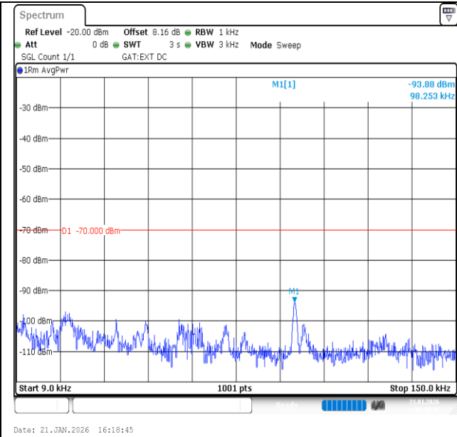
Band40 (2305-2315)-10MHz-16QAM-38750-50RB#0-0.009~0.15-PASS
