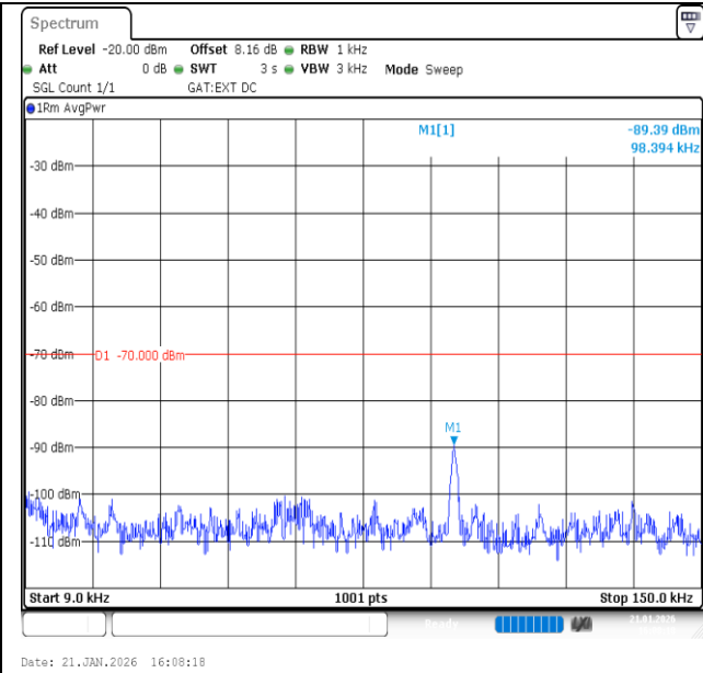
Band40 (2305-2315)-10MHz-QPSK-38750-1RB#49-0.009~0.15-PASS
