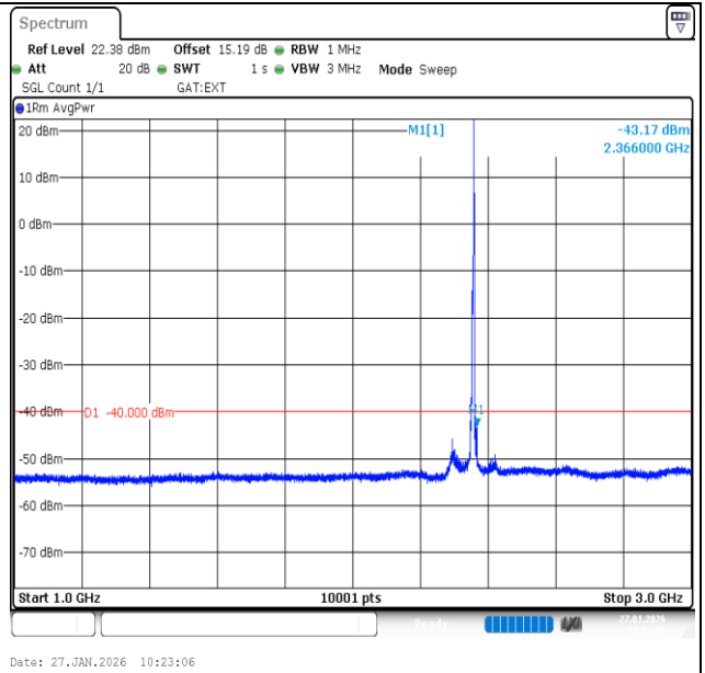
Band40 (2350-2360)-5MHz-QPSK-39200-1RB#24-1000~3000-PASS
