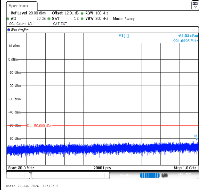
Band40 (2305-2315)-10MHz-16QAM-38750-50RB#0-30~1000-PASS
