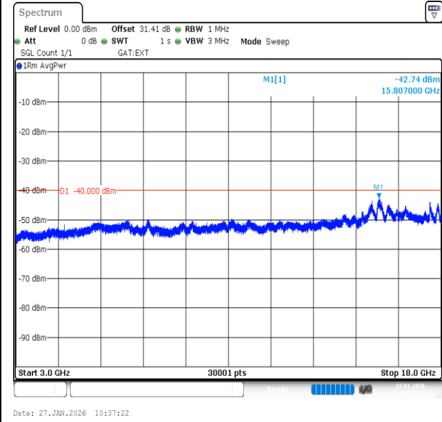
Band40 (2350-2360)-5MHz-QPSK-39225-1RB#0-3000~18000-PASS
