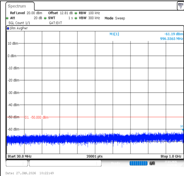
Band40 (2350-2360)-5MHz-QPSK-39200-1RB#24-30~1000-PASS
