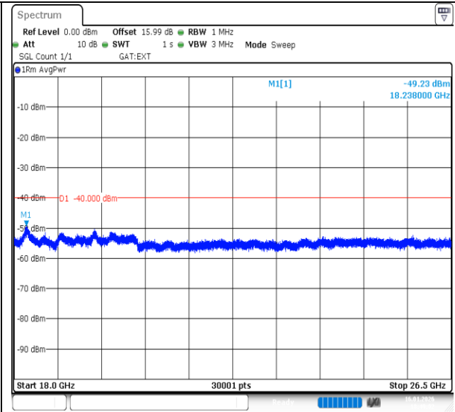
Band40 (2305-2315)-5MHz-16QAM-38775-25RB#0-18000~26500-PASS
