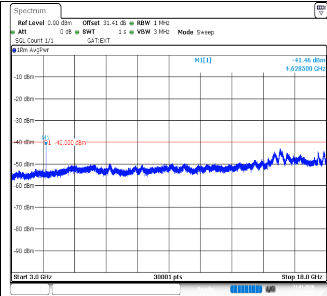
Band40 (2305-2315)-10MHz-QPSK-38750-1RB#49-3000~18000-PASS
