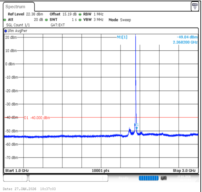
Band40 (2350-2360)-5MHz-QPSK-39225-1RB#0-1000~3000-PASS
