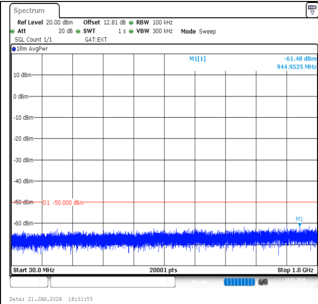
Band40 (2305-2315)-10MHz-QPSK-38750-1RB#0-30~1000-PASS
