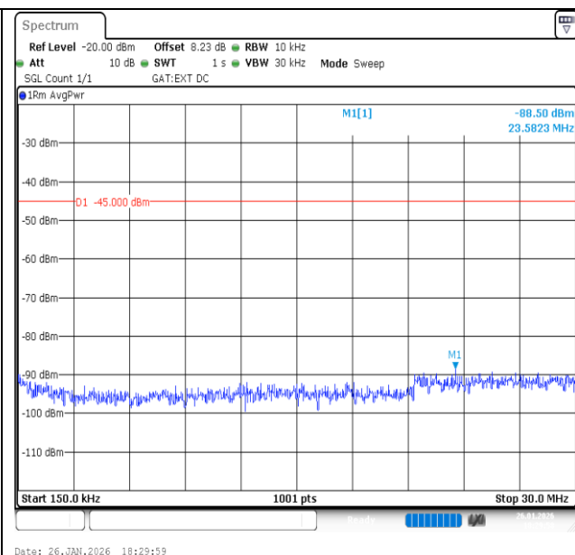
Band41-15MHz-QPSK-40620-1RB#0-0.15~30-PASS
