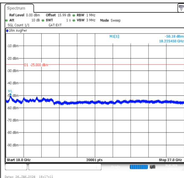
Band41-15MHz-QPSK-39725-1RB#74-18000~27000-PASS
