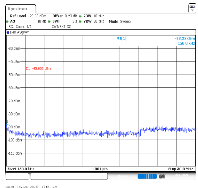
Band41-10MHz-16QAM-41540-1RB#0-0.15~30-PASS
