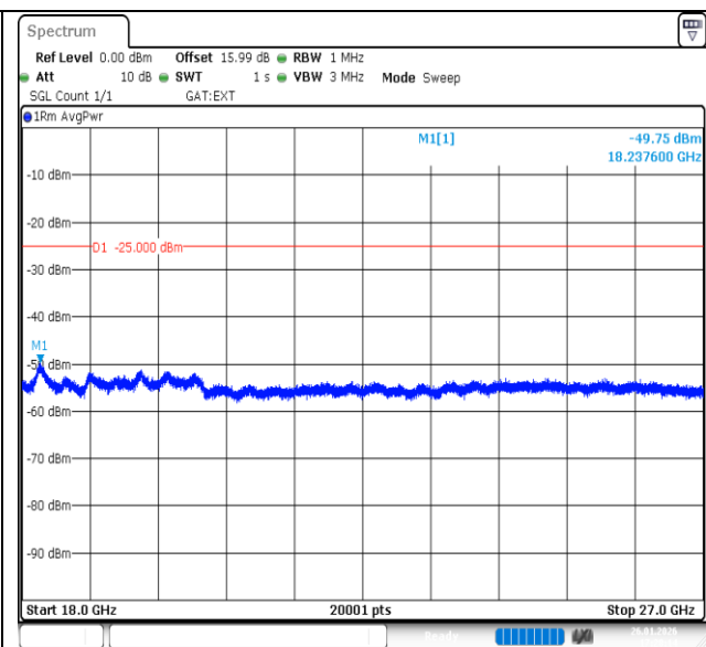
Band41-10MHz-QPSK-40620-1RB#0-18000~27000-PASS
