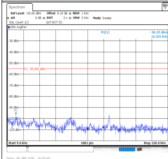
Band41-15MHz-QPSK-39725-75RB#0-0.009~0.15-PASS
