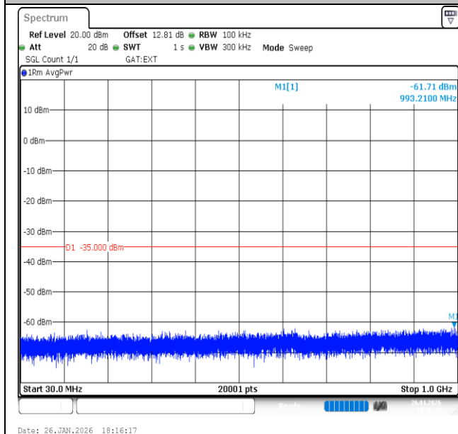
Band41-15MHz-QPSK-39725-1RB#74-30~1000-PASS
