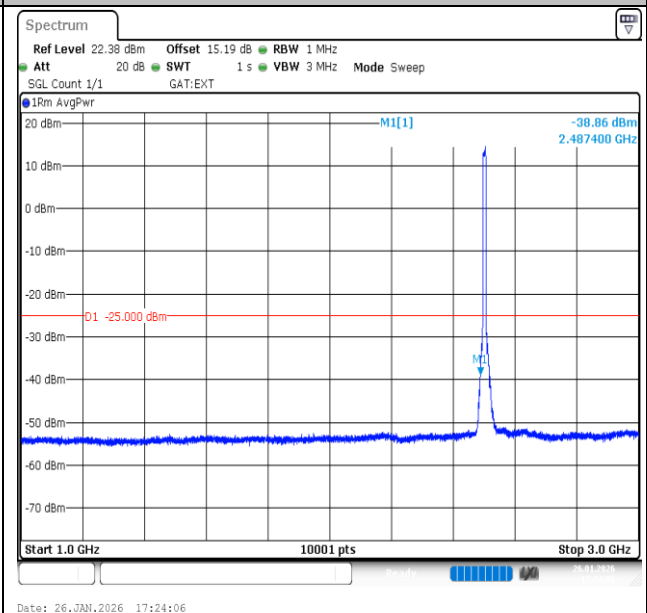
Band41-10MHz-16QAM-39700-50RB#0-1000~3000-PASS
