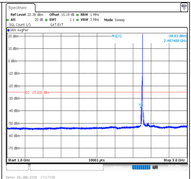
Band41-10MHz-16QAM-39700-1RB#49-1000~3000-PASS
