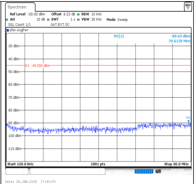
Band41-10MHz-QPSK-40620-50RB#0-0.15~30-PASS
