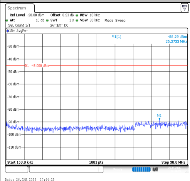
Band41-10MHz-16QAM-40620-50RB#0-0.15~30-PASS
