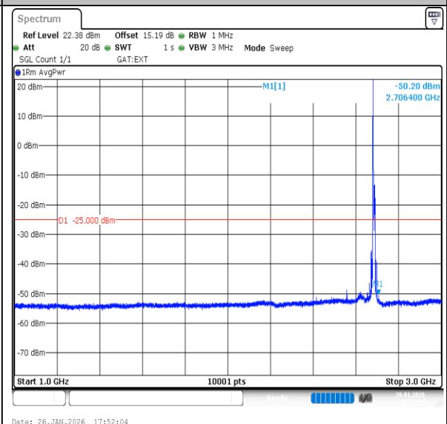
Band41-10MHz-16QAM-41540-1RB#0-1000~3000-PASS
