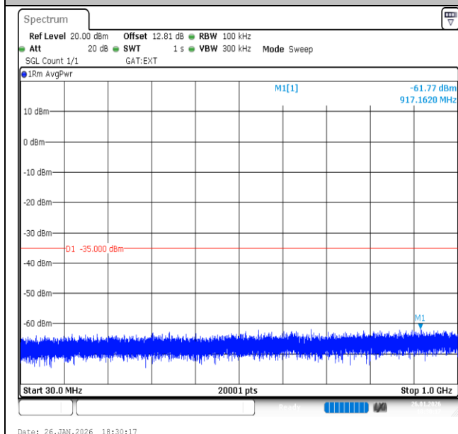
Band41-15MHz-QPSK-40620-1RB#0-30~1000-PASS
