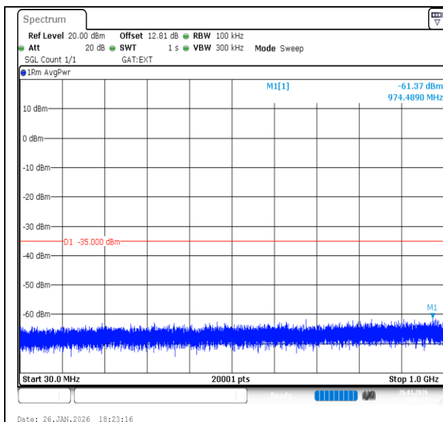
Band41-15MHz-QPSK-39725-75RB#0-30~1000-PASS
