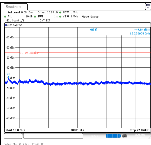
Band41-10MHz-QPSK-40620-50RB#0-18000~27000-PASS
