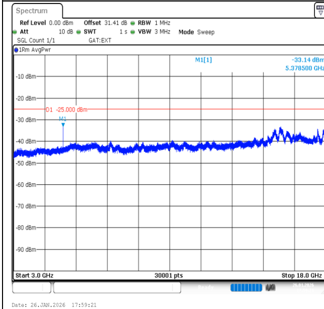
Band41-10MHz-16QAM-41540-1RB#49-3000~18000-PASS
