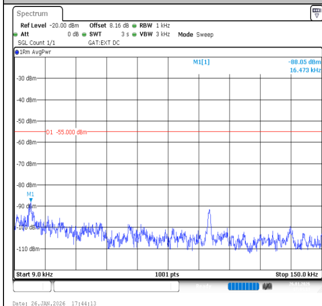
Band41-10MHz-16QAM-40620-50RB#0-0.009~0.15-PASS
