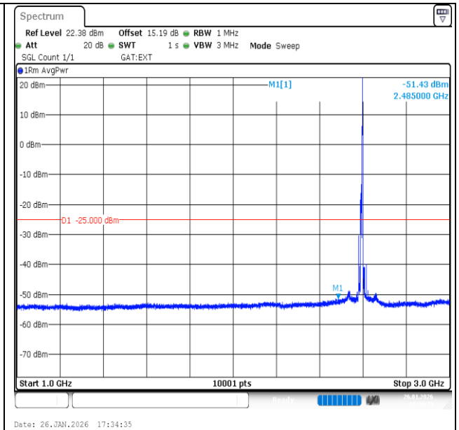
Band41-10MHz-QPSK-40620-1RB#49-1000~3000-PASS
