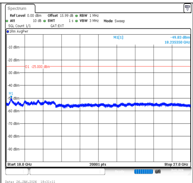
Band41-15MHz-QPSK-40620-1RB#0-18000~27000-PASS
