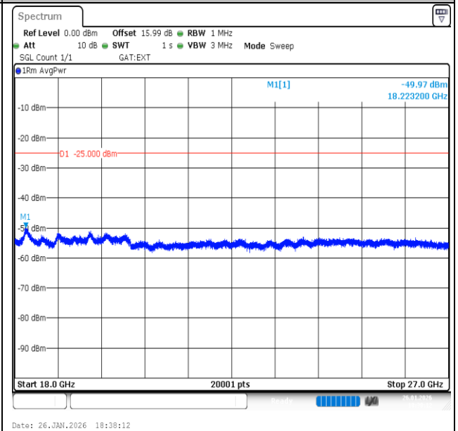
Band41-15MHz-QPSK-40620-1RB#74-18000~27000-PASS
