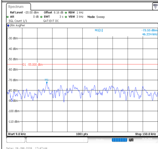
Band41-10MHz-QPSK-41540-1RB#0-0.009~0.15-PASS
