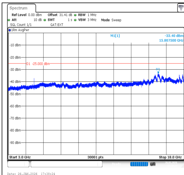
Band41-10MHz-16QAM-40620-1RB#49-3000~18000-PASS
