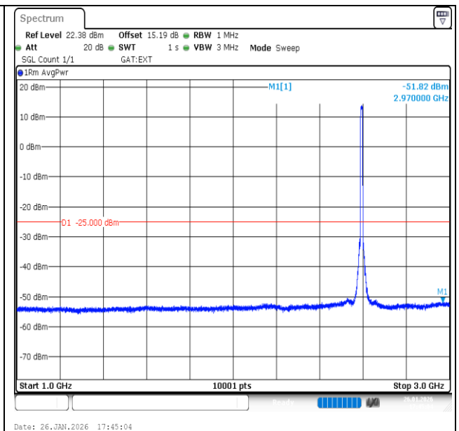
Band41-10MHz-16QAM-40620-50RB#0-1000~3000-PASS
