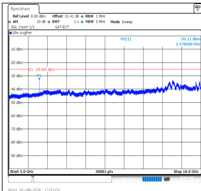
Band41-10MHz-QPSK-41540-1RB#49-3000~18000-PASS
