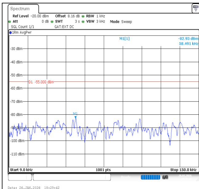
Band41-15MHz-QPSK-40620-1RB#0-0.009~0.15-PASS
