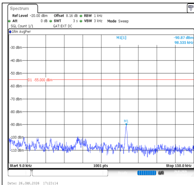
Band41-10MHz-16QAM-39700-50RB#0-0.009~0.15-PASS
