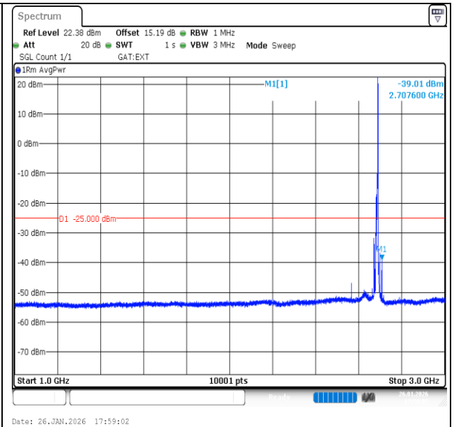
Band41-10MHz-16QAM-41540-1RB#49-1000~3000-PASS
