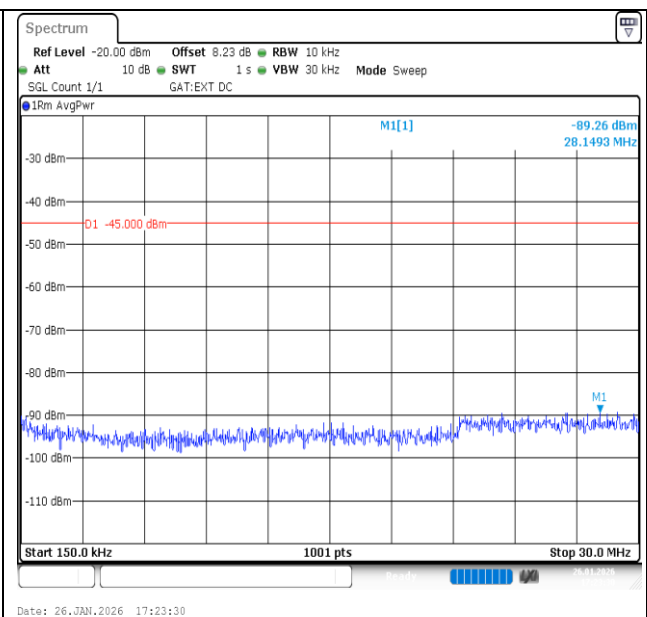
Band41-10MHz-16QAM-39700-50RB#0-0.15~30-PASS
