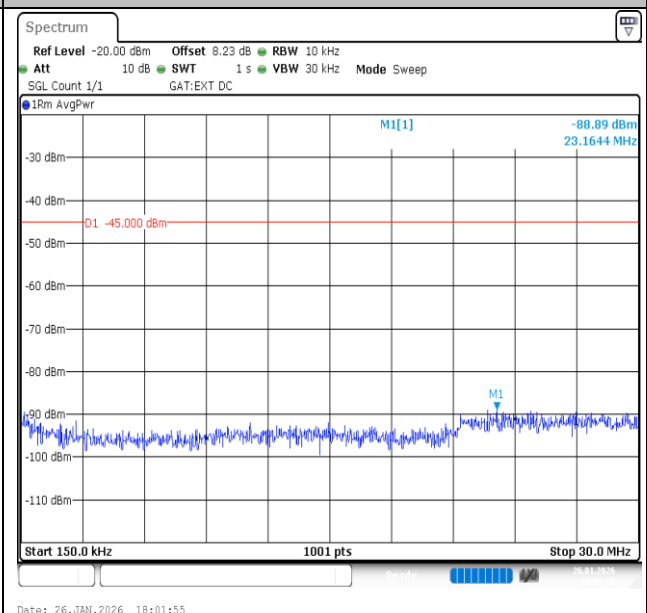
Band41-10MHz-QPSK-41540-50RB#0-0.15~30-PASS
