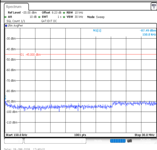
Band41-10MHz-QPSK-41540-1RB#0-0.15~30-PASS
