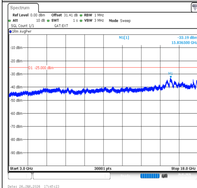
Band41-10MHz-16QAM-40620-50RB#0-3000~18000-PASS
