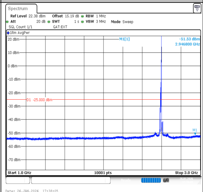
Band41-10MHz-16QAM-40620-1RB#49-1000~3000-PASS
