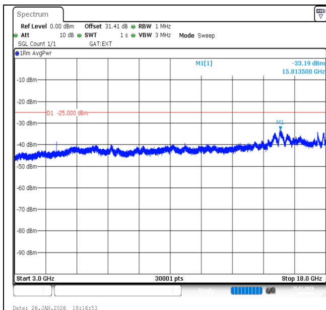
Band41-15MHz-QPSK-39725-1RB#74-3000~18000-PASS
