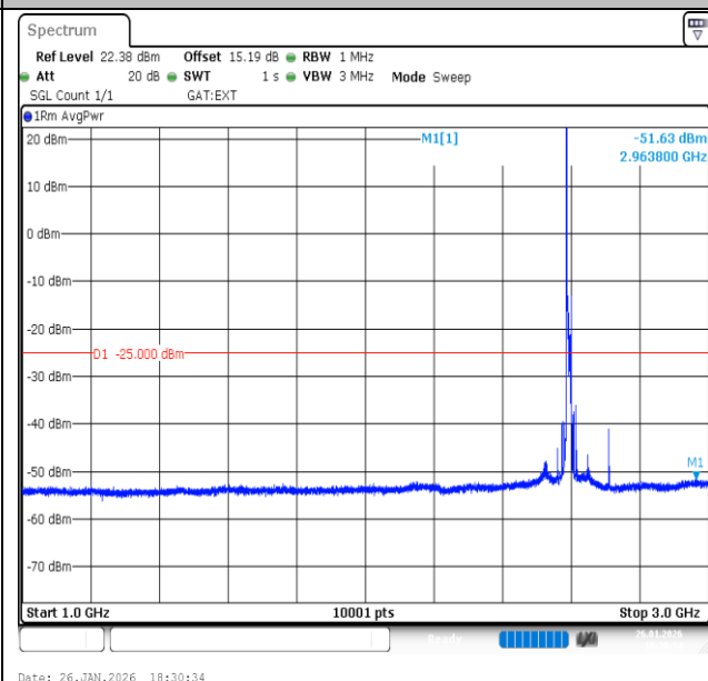
Band41-15MHz-QPSK-40620-1RB#0-1000~3000-PASS
