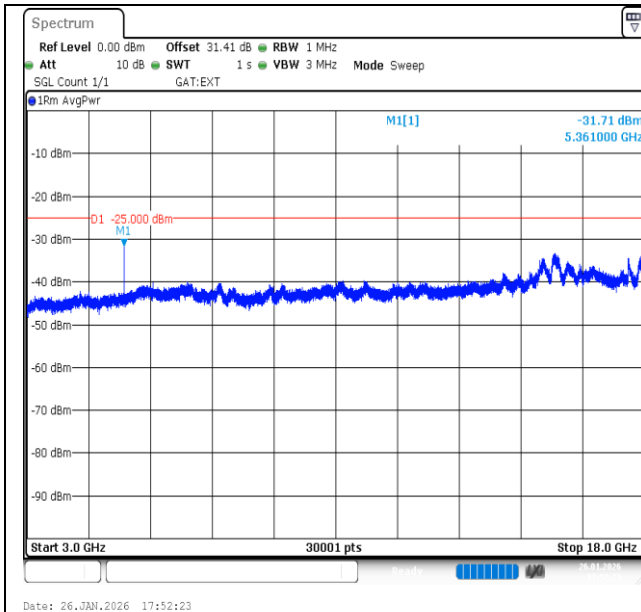
Band41-10MHz-16QAM-41540-1RB#0-3000~18000-PASS
