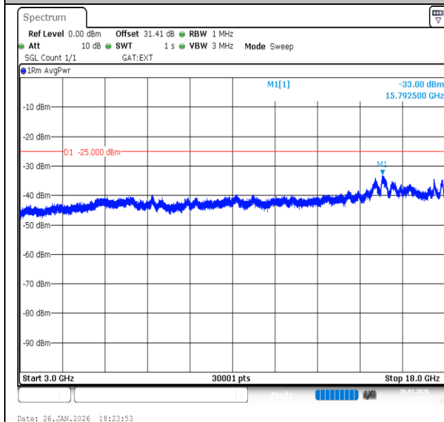
Band41-15MHz-QPSK-39725-75RB#0-3000~18000-PASS
