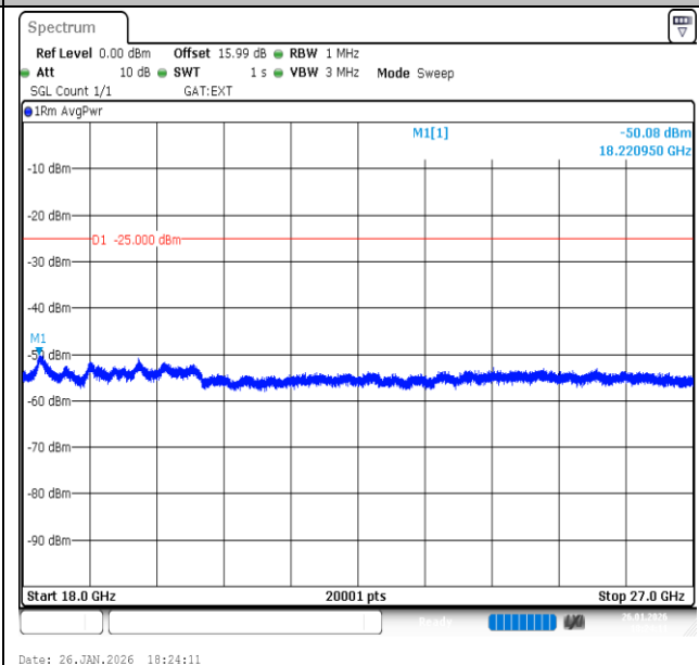
Band41-15MHz-QPSK-39725-75RB#0-18000~27000-PASS
