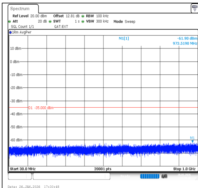
Band41-10MHz-16QAM-40620-1RB#0-30~1000-PASS
