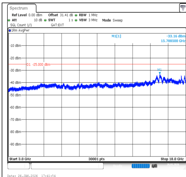
Band41-10MHz-QPSK-40620-50RB#0-3000~18000-PASS
