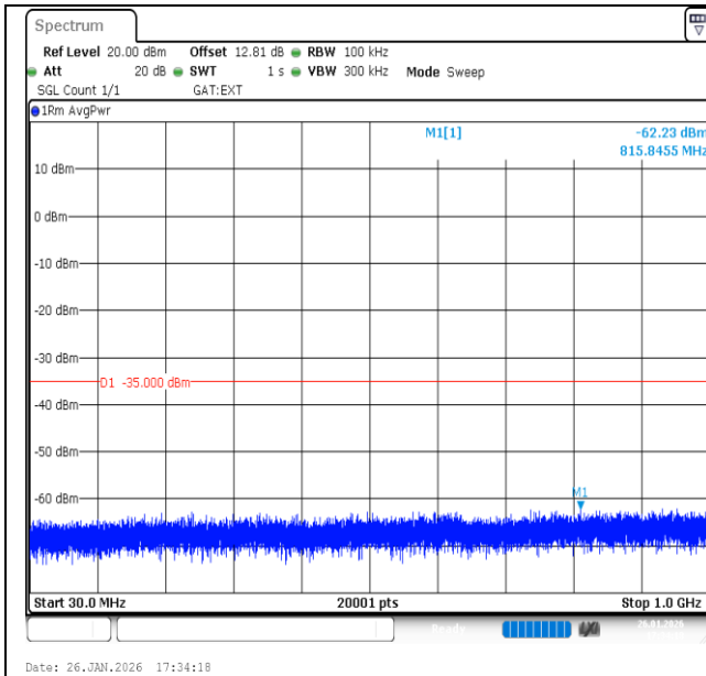
Band41-10MHz-QPSK-40620-1RB#49-30~1000-PASS
