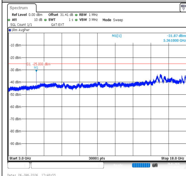
Band41-10MHz-QPSK-41540-1RB#0-3000~18000-PASS
