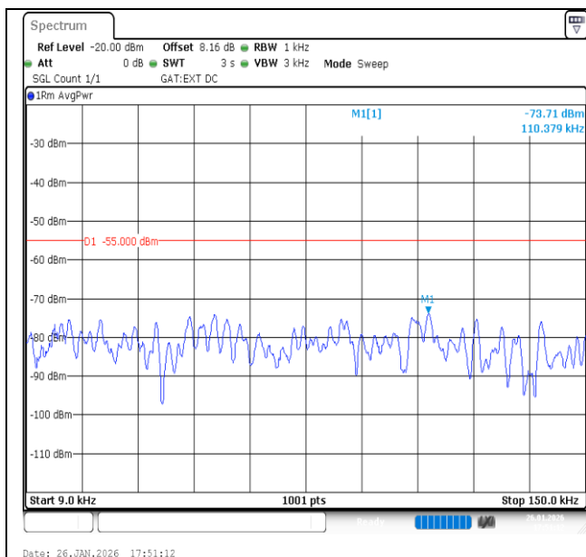
Band41-10MHz-16QAM-41540-1RB#0-0.009~0.15-PASS
