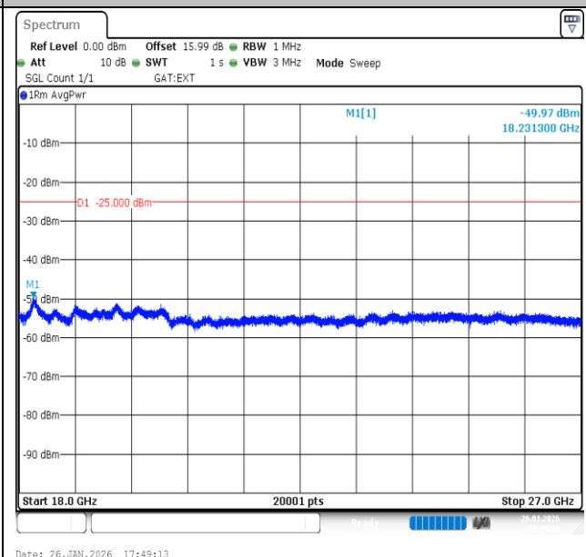
Band41-10MHz-QPSK-41540-1RB#0-18000~27000-PASS
