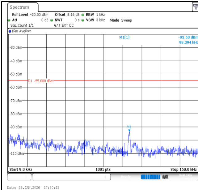
Band41-10MHz-QPSK-40620-50RB#0-0.009~0.15-PASS
