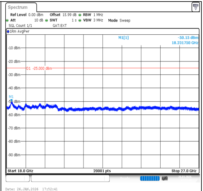
Band41-10MHz-16QAM-41540-1RB#0-18000~27000-PASS
