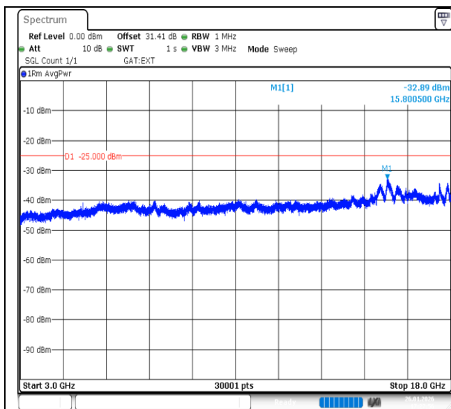
Band41-10MHz-QPSK-40620-1RB#0-3000~18000-PASS
