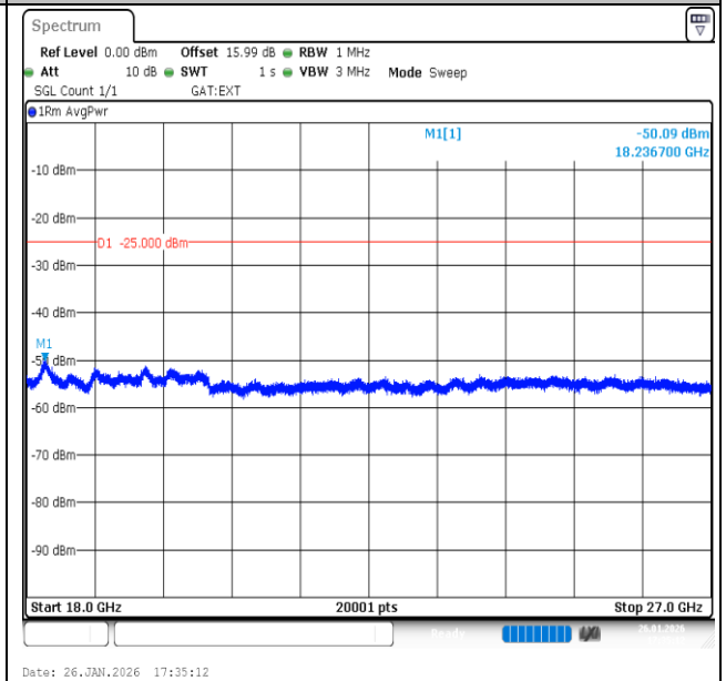
Band41-10MHz-QPSK-40620-1RB#49-18000~27000-PASS
