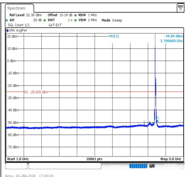
Band41-10MHz-QPSK-41540-1RB#0-1000~3000-PASS
