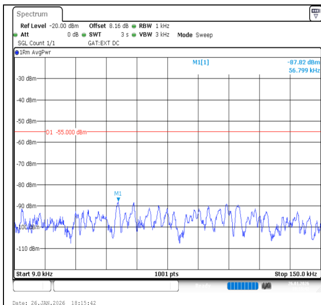
Band41-15MHz-QPSK-39725-1RB#74-0.009~0.15-PASS
