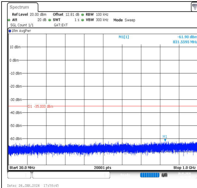
Band41-10MHz-16QAM-41540-1RB#49-30~1000-PASS
