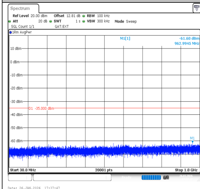
Band41-10MHz-16QAM-40620-1RB#49-30~1000-PASS
