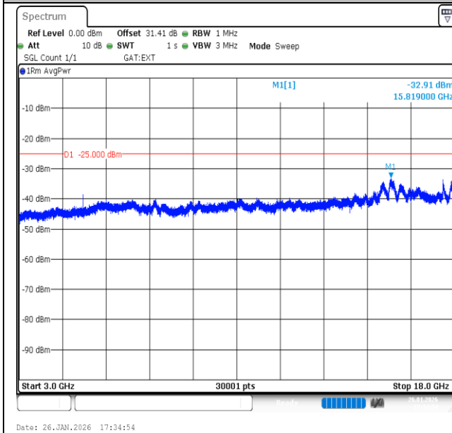
Band41-10MHz-QPSK-40620-1RB#49-3000~18000-PASS
