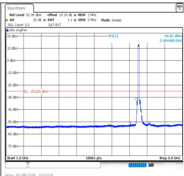
Band41-15MHz-QPSK-39725-75RB#0-1000~3000-PASS
