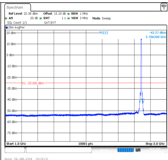
Band41-10MHz-QPSK-41540-50RB#0-1000~3000-PASS
