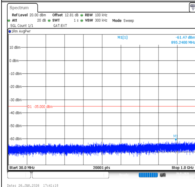
Band41-10MHz-QPSK-40620-50RB#0-30~1000-PASS
