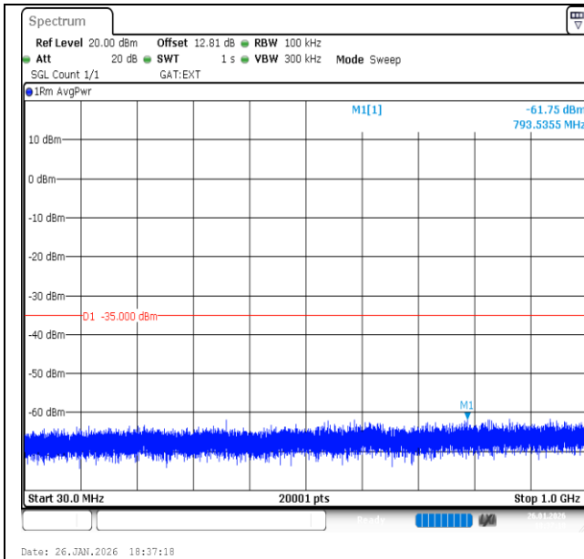
Band41-15MHz-QPSK-40620-1RB#74-30~1000-PASS
