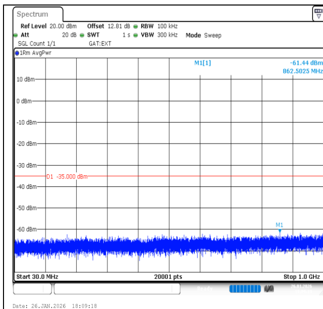
Band41-15MHz-QPSK-39725-1RB#0-30~1000-PASS
