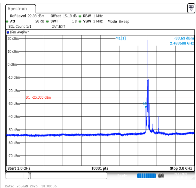
Band41-15MHz-QPSK-39725-1RB#0-1000~3000-PASS
