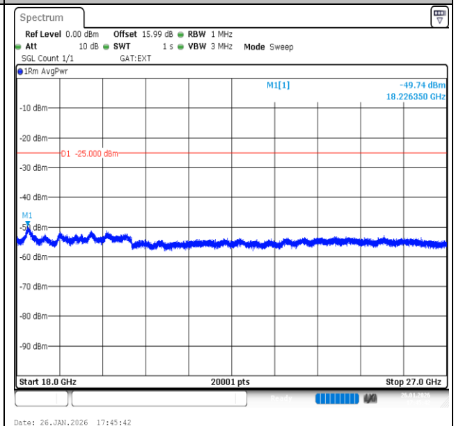
Band41-10MHz-16QAM-40620-50RB#0-18000~27000-PASS
