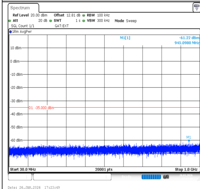
Band41-10MHz-16QAM-39700-50RB#0-30~1000-PASS
