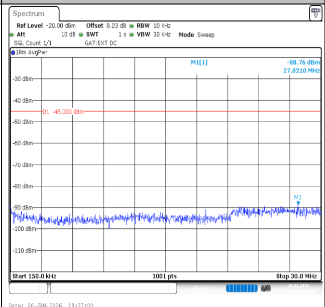
Band41-15MHz-QPSK-40620-1RB#74-0.15~30-PASS
