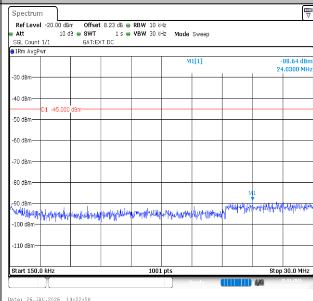
Band41-15MHz-QPSK-39725-75RB#0-0.15~30-PASS
