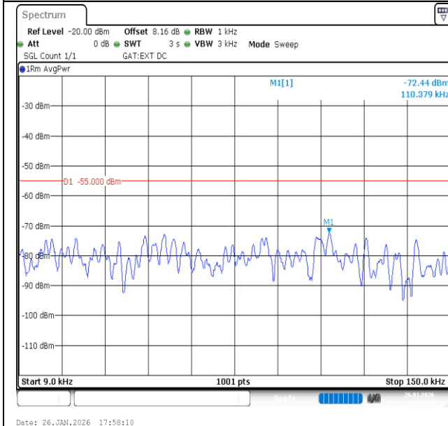
Band41-10MHz-16QAM-41540-1RB#49-0.009~0.15-PASS
