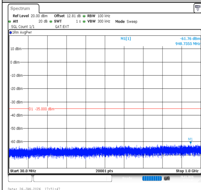
Band41-10MHz-16QAM-41540-1RB#0-30~1000-PASS
