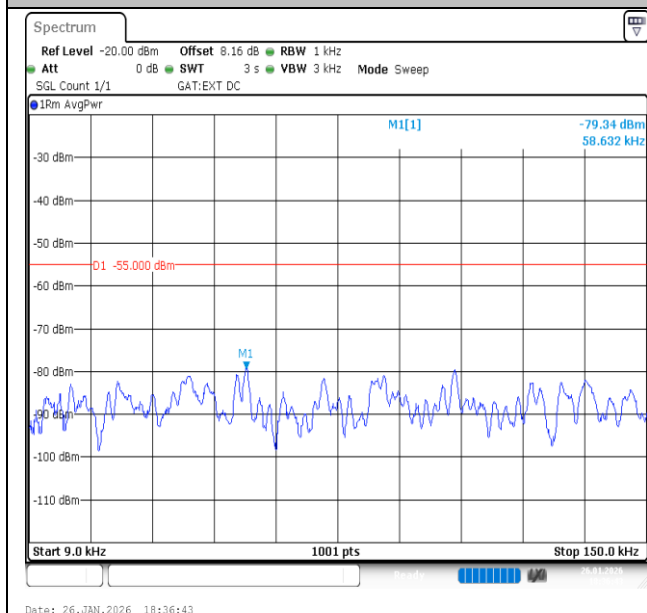
Band41-15MHz-QPSK-40620-1RB#74-0.009~0.15-PASS
