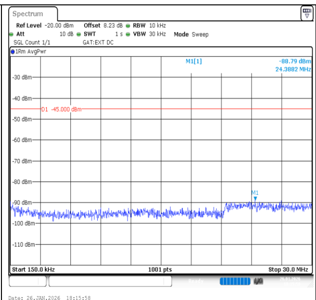
Band41-15MHz-QPSK-39725-1RB#74-0.15~30-PASS
