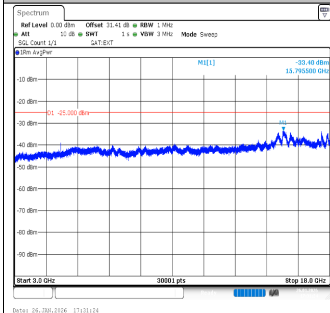
Band41-10MHz-16QAM-40620-1RB#0-3000~18000-PASS
