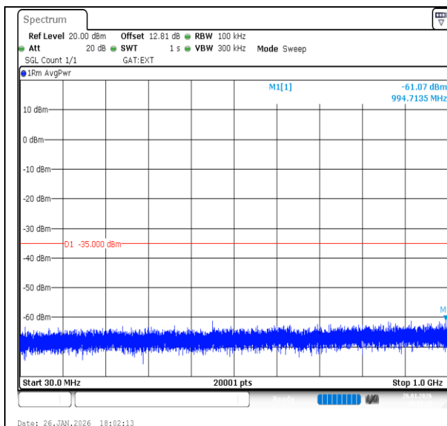
Band41-10MHz-QPSK-41540-50RB#0-30~1000-PASS
