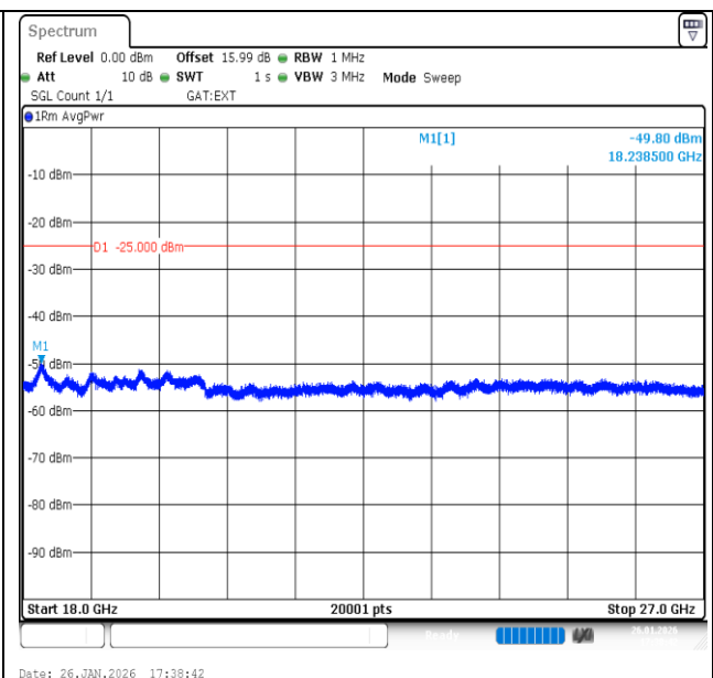
Band41-10MHz-16QAM-40620-1RB#49-18000~27000-PASS
