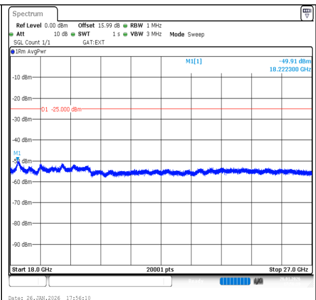
Band41-10MHz-QPSK-41540-1RB#49-18000~27000-PASS
