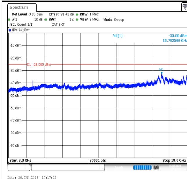
Band41-10MHz-16QAM-39700-1RB#49-3000~18000-PASS
