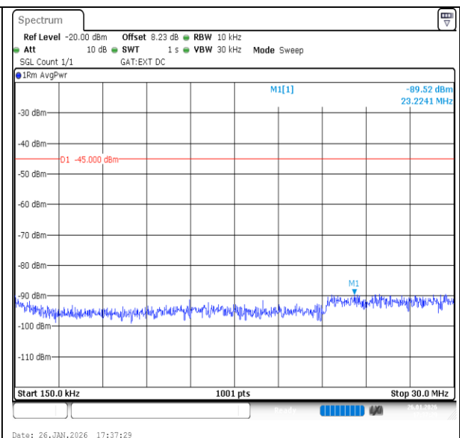
Band41-10MHz-16QAM-40620-1RB#49-0.15~30-PASS
