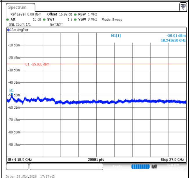
Band41-10MHz-16QAM-39700-1RB#49-18000~27000-PASS
