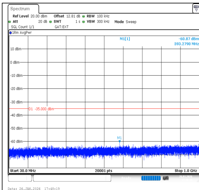
Band41-10MHz-QPSK-41540-1RB#0-30~1000-PASS
