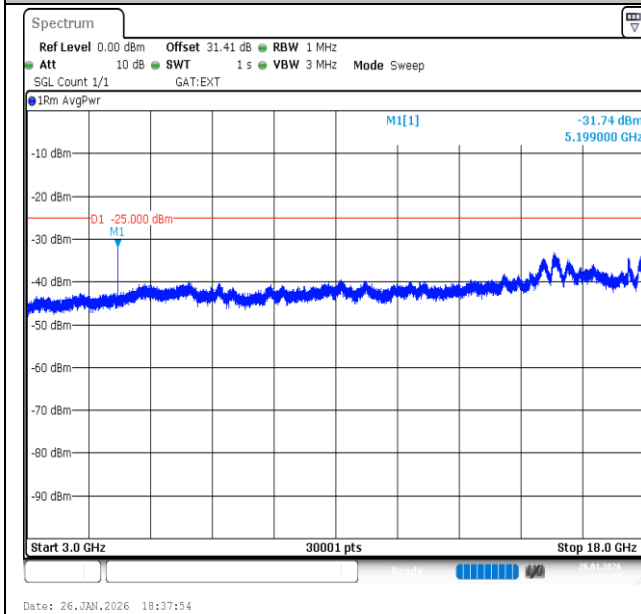
Band41-15MHz-QPSK-40620-1RB#74-3000~18000-PASS
