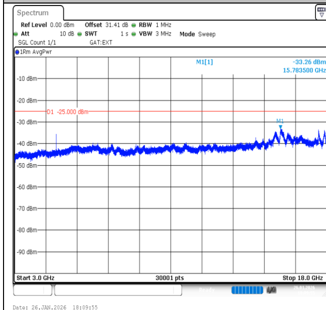
Band41-15MHz-QPSK-39725-1RB#0-3000~18000-PASS
