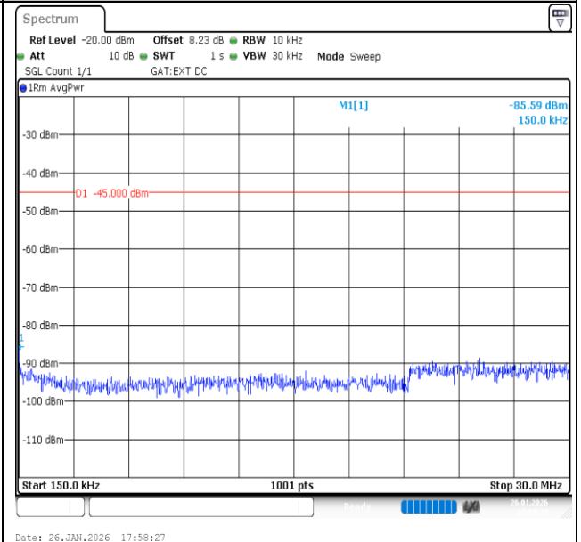
Band41-10MHz-16QAM-41540-1RB#49-0.15~30-PASS
