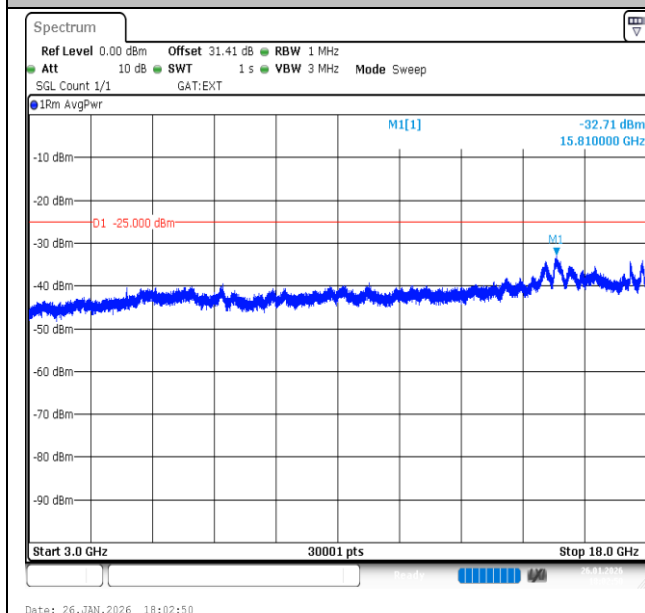
Band41-10MHz-QPSK-41540-50RB#0-3000~18000-PASS
