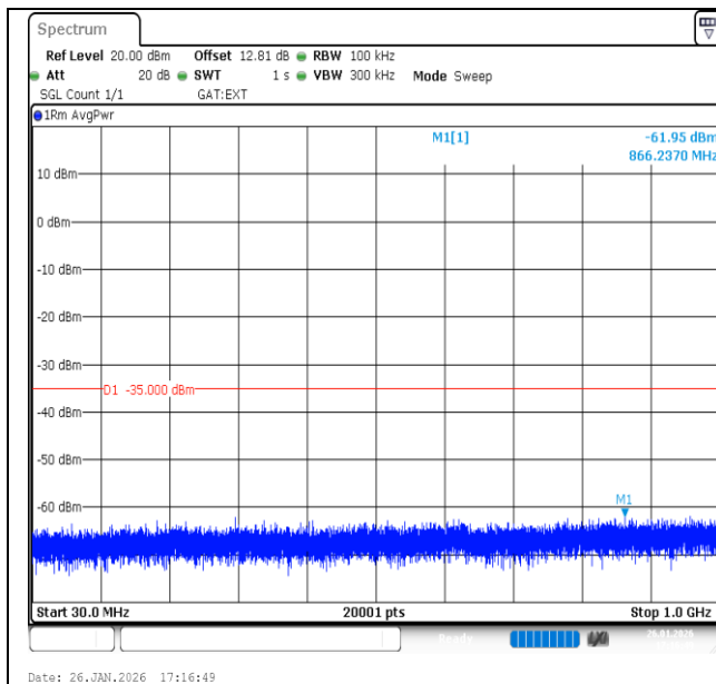
Band41-10MHz-16QAM-39700-1RB#49-30~1000-PASS
