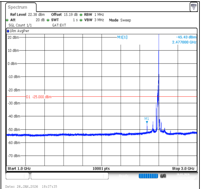
Band41-15MHz-QPSK-40620-1RB#74-1000~3000-PASS
