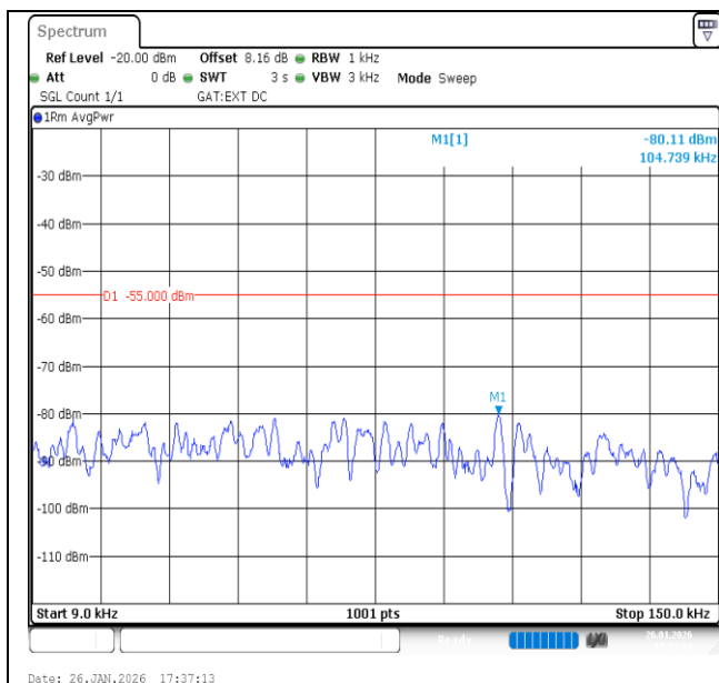
Band41-10MHz-16QAM-40620-1RB#49-0.009~0.15-PASS
