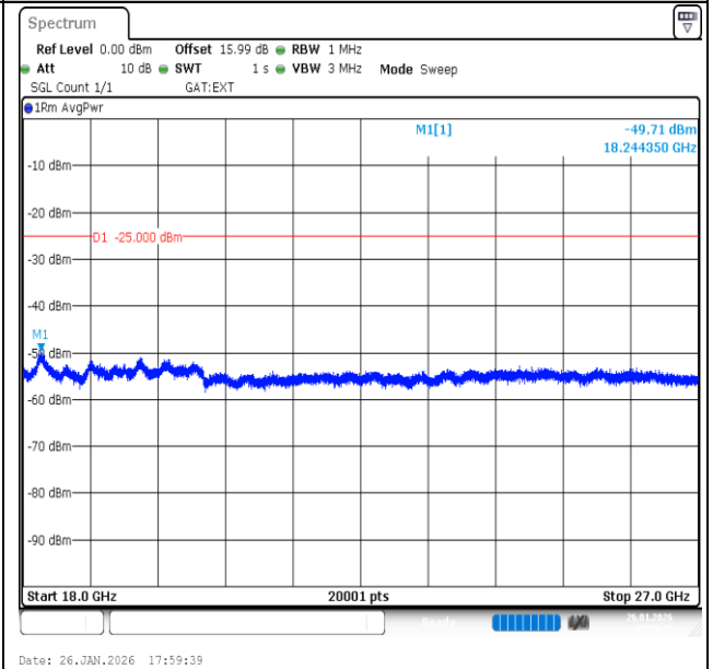
Band41-10MHz-16QAM-41540-1RB#49-18000~27000-PASS
