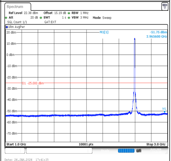
Band41-10MHz-QPSK-40620-50RB#0-1000~3000-PASS
