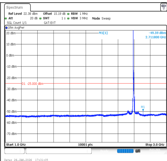
Band41-10MHz-16QAM-40620-1RB#0-1000~3000-PASS
