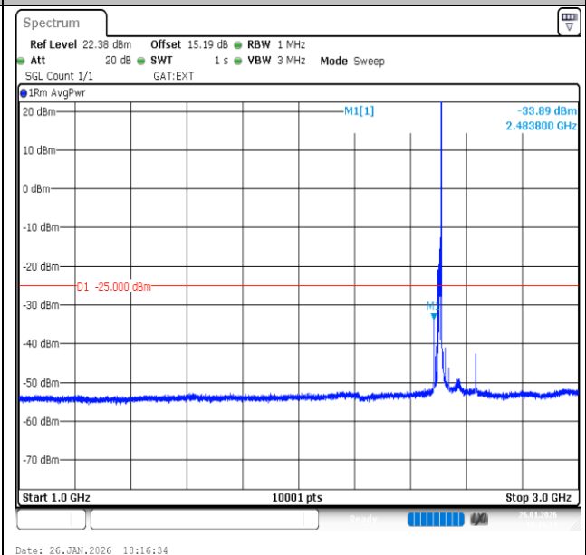
Band41-15MHz-QPSK-39725-1RB#74-1000~3000-PASS
