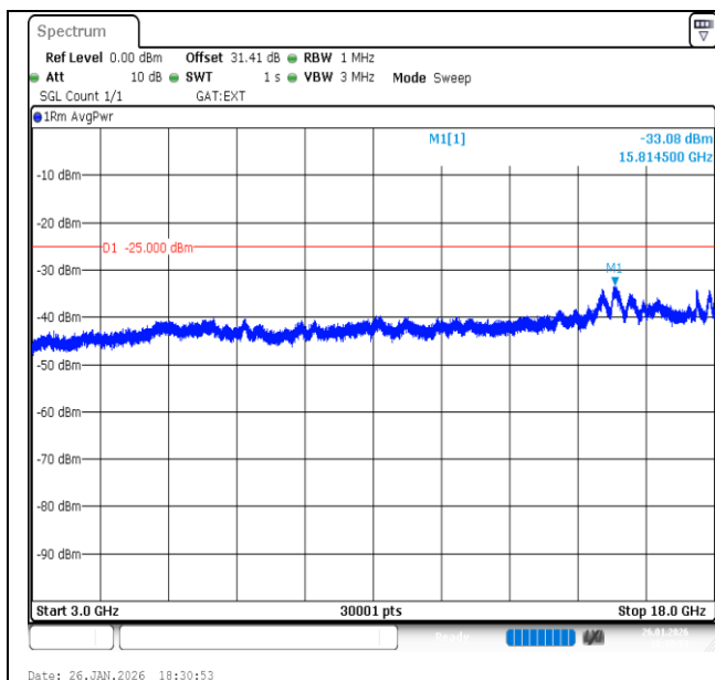
Band41-15MHz-QPSK-40620-1RB#0-3000~18000-PASS
