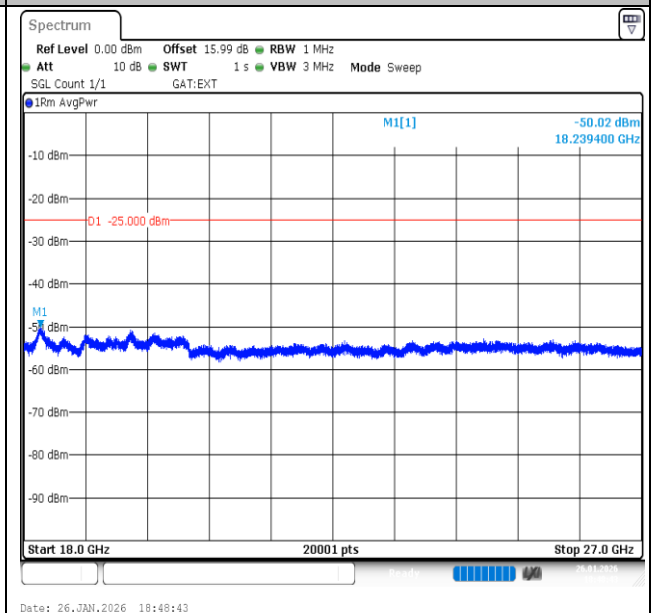
Band41-15MHz-16QAM-40620-75RB#0-18000~27000-PASS
