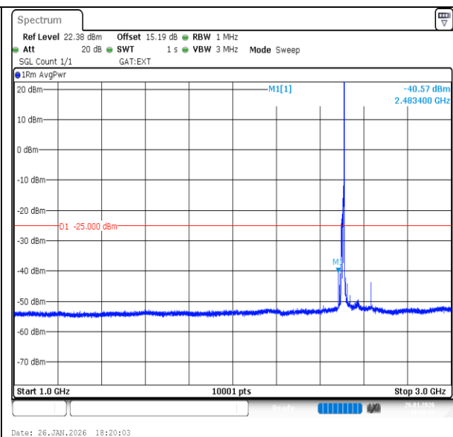
Band41-15MHz-16QAM-39725-1RB#74-1000~3000-PASS
