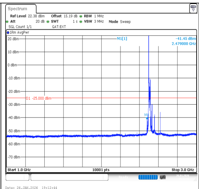
Band41-20MHz-QPSK-39750-1RB#0-1000~3000-PASS
