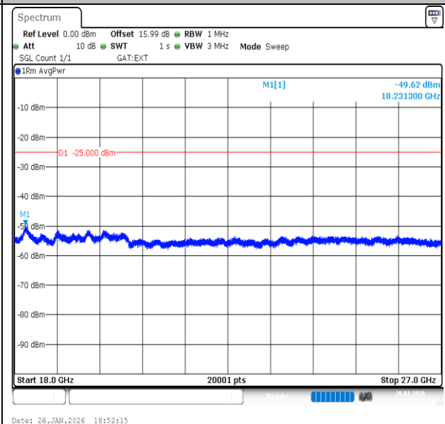
Band41-15MHz-QPSK-41515-1RB#0-18000~27000-PASS
