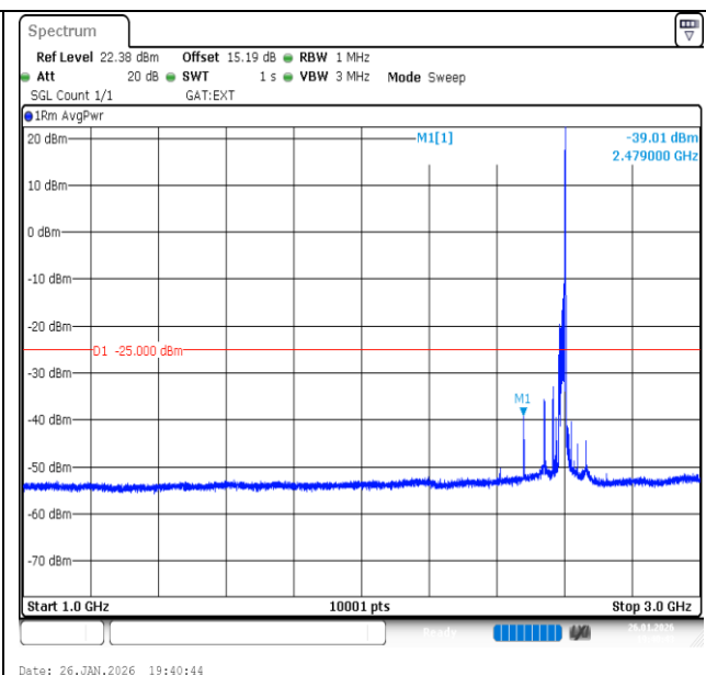
Band41-20MHz-QPSK-40620-1RB#99-1000~3000-PASS
