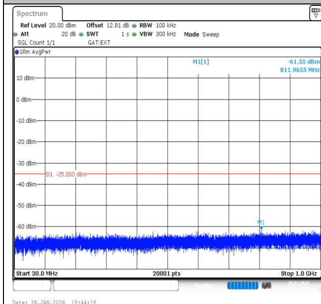
Band41-15MHz-QPSK-40620-75RB#0-30~1000-PASS
