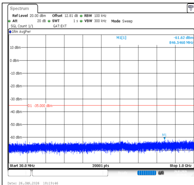
Band41-15MHz-16QAM-39725-1RB#74-30~1000-PASS
