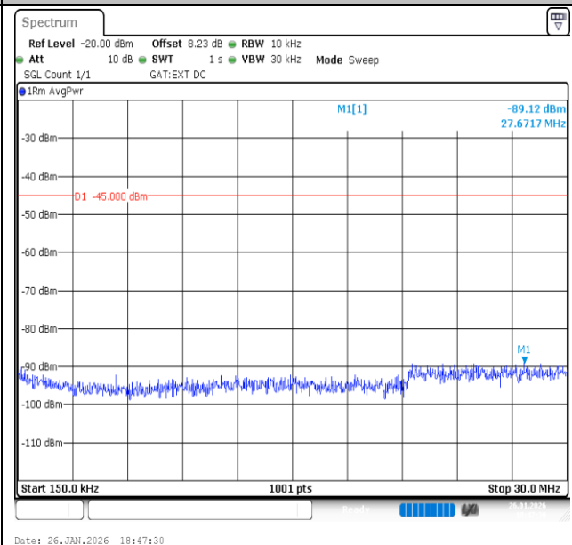
Band41-15MHz-16QAM-40620-75RB#0-0.15~30-PASS
