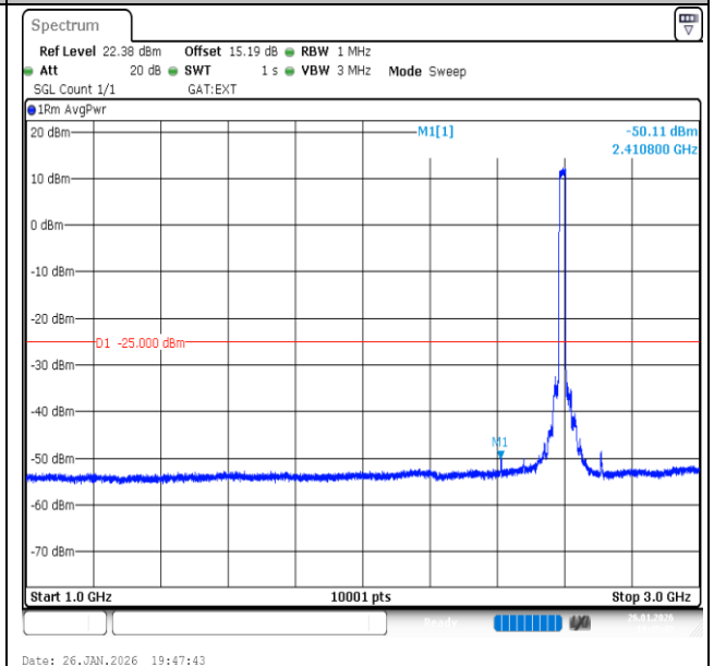
Band41-20MHz-QPSK-40620-100RB#0-1000~3000-PASS
