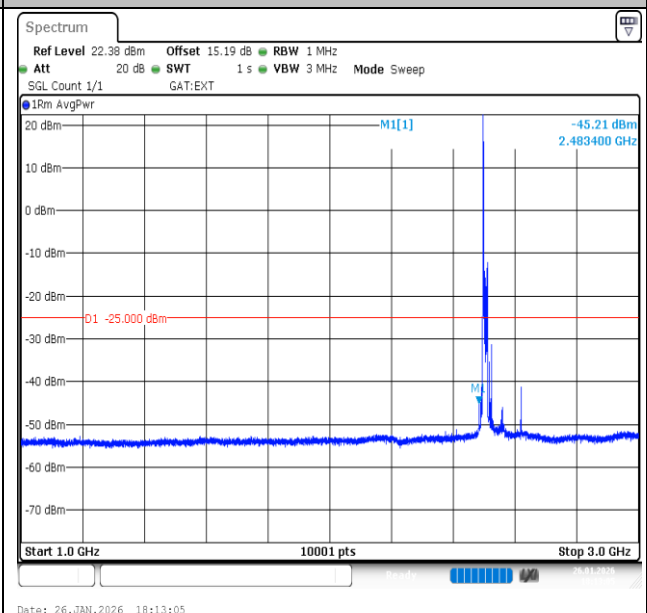
Band41-15MHz-16QAM-39725-1RB#0-1000~3000-PASS
