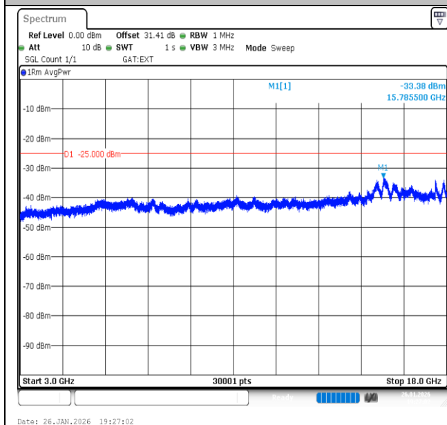
Band41-20MHz-QPSK-39750-100RB#0-3000~18000-PASS
