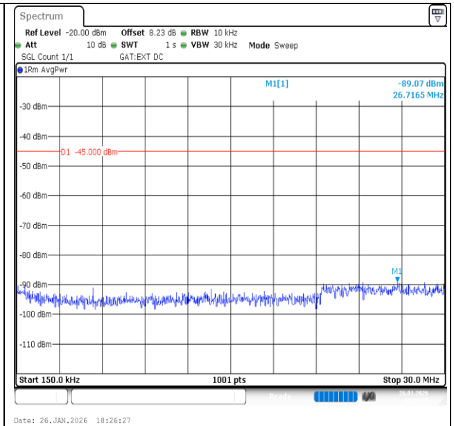
Band41-15MHz-16QAM-39725-75RB#0-0.15~30-PASS
