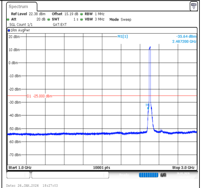
Band41-15MHz-16QAM-39725-75RB#0-1000~3000-PASS
