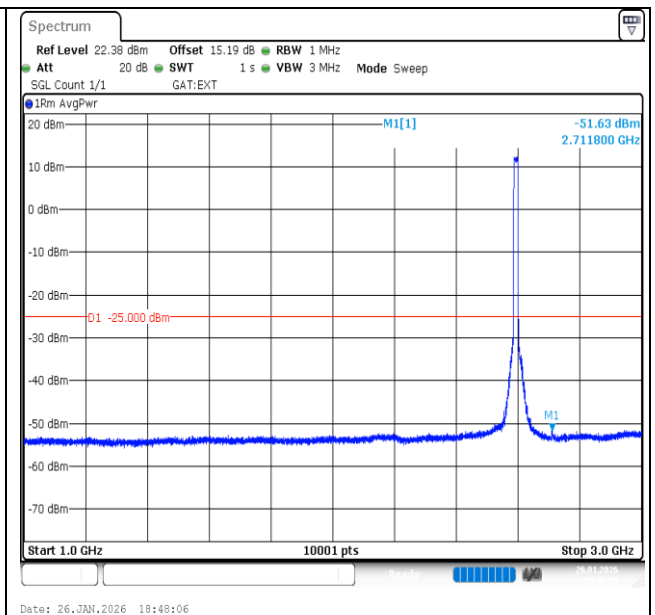
Band41-15MHz-16QAM-40620-75RB#0-1000~3000-PASS
