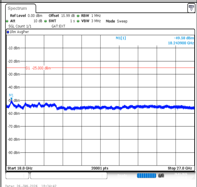
Band41-15MHz-16QAM-40620-1RB#0-18000~27000-PASS
