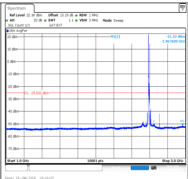
Band41-15MHz-16QAM-40620-1RB#0-1000~3000-PASS
