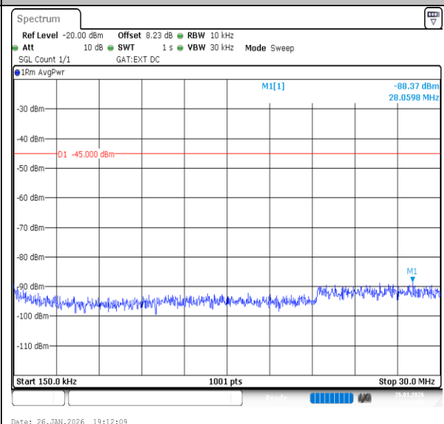
Band41-20MHz-QPSK-39750-1RB#0-0.15~30-PASS
