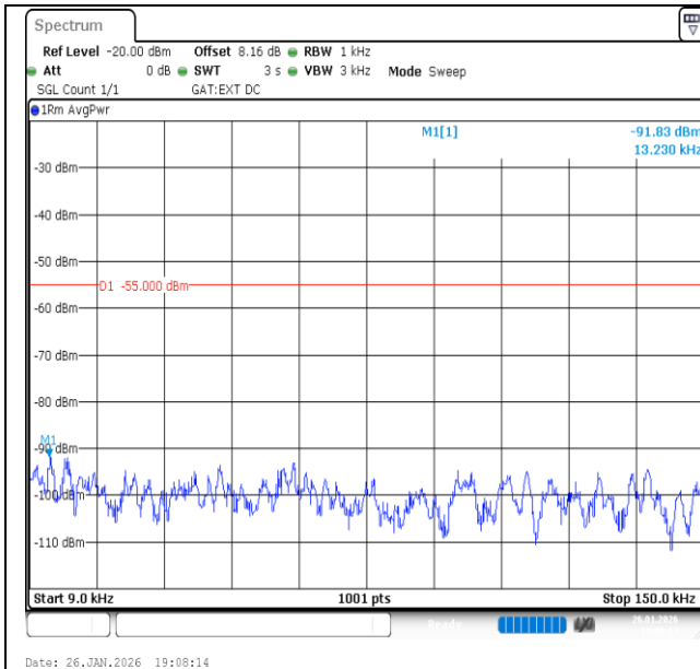
Band41-15MHz-16QAM-41515-75RB#0-0.009~0.15-PASS
