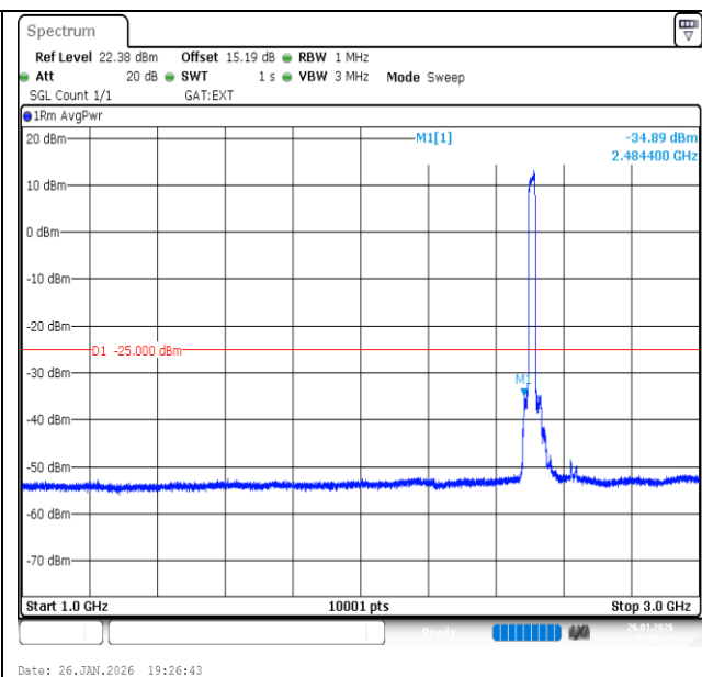
Band41-20MHz-QPSK-39750-100RB#0-1000~3000-PASS
