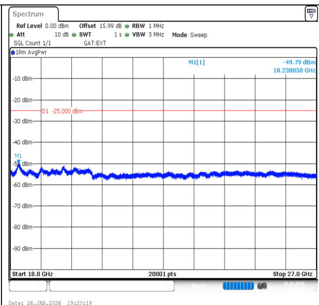
Band41-20MHz-QPSK-39750-1RB#99-18000~27000-PASS
