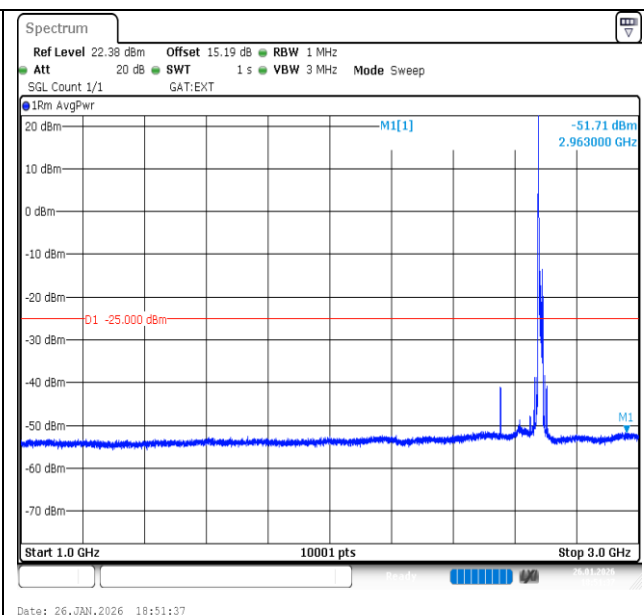
Band41-15MHz-QPSK-41515-1RB#0-1000~3000-PASS
