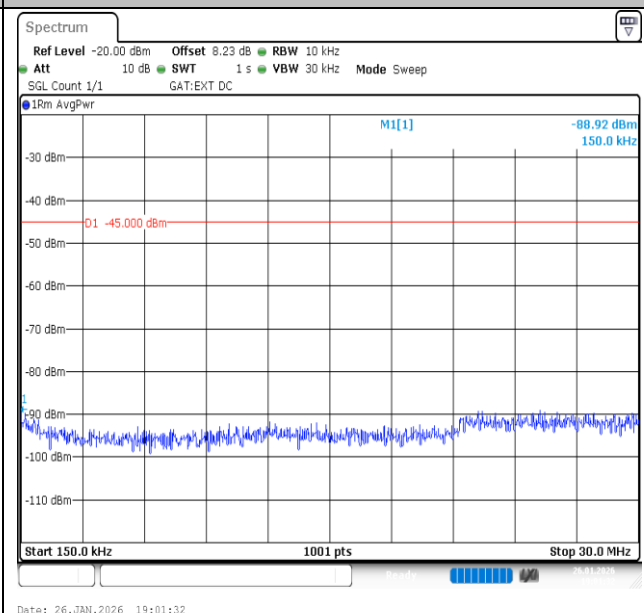
Band41-15MHz-16QAM-41515-1RB#74-0.15~30-PASS
