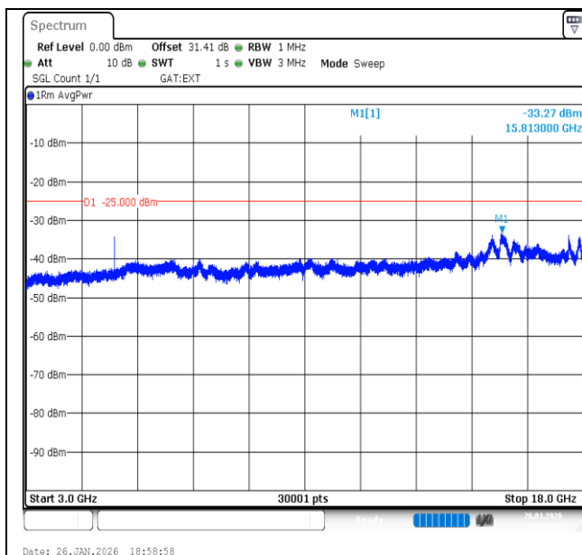
Band41-15MHz-QPSK-41515-1RB#74-3000~18000-PASS
