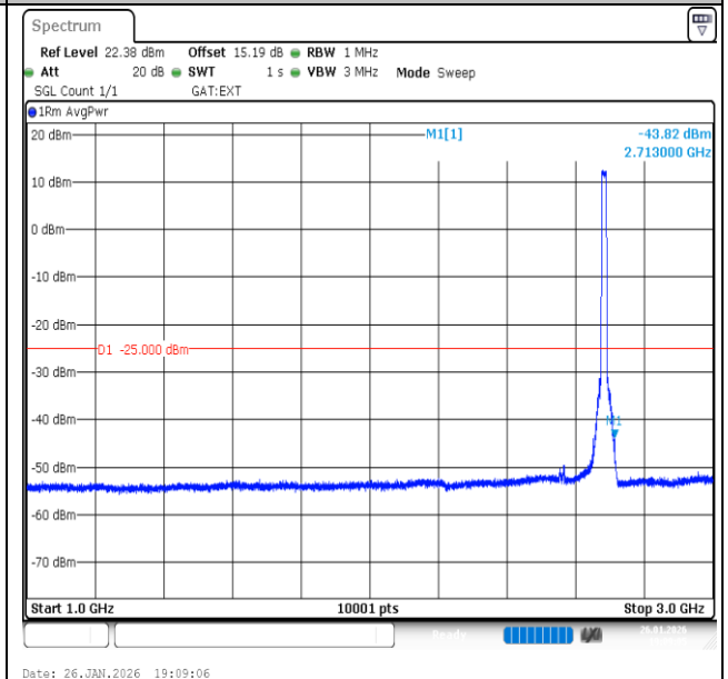
Band41-15MHz-16QAM-41515-75RB#0-1000~3000-PASS
