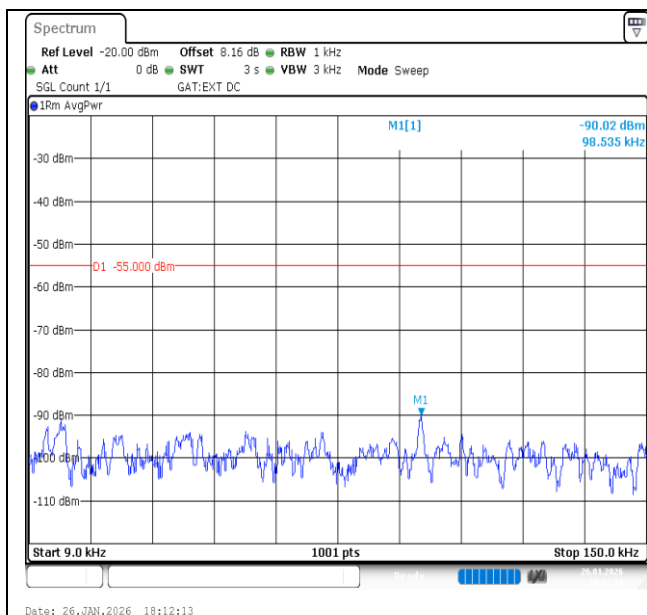
Band41-15MHz-16QAM-39725-1RB#0-0.009~0.15-PASS
