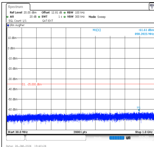
Band41-20MHz-QPSK-40620-1RB#99-30~1000-PASS
