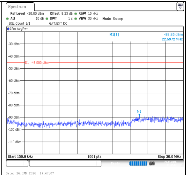
Band41-20MHz-QPSK-40620-100RB#0-0.15~30-PASS
