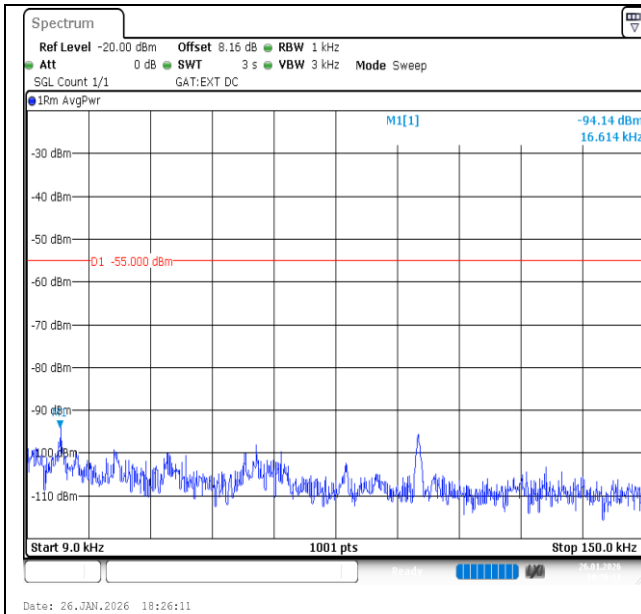
Band41-15MHz-16QAM-39725-75RB#0-0.009~0.15-PASS
