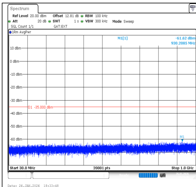
Band41-15MHz-16QAM-40620-1RB#0-30~1000-PASS
