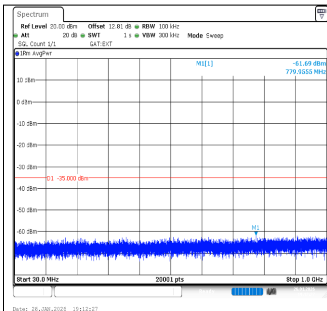
Band41-20MHz-QPSK-39750-1RB#0-30~1000-PASS
