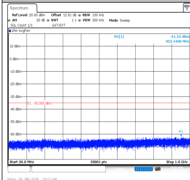
Band41-15MHz-16QAM-39725-1RB#0-30~1000-PASS
