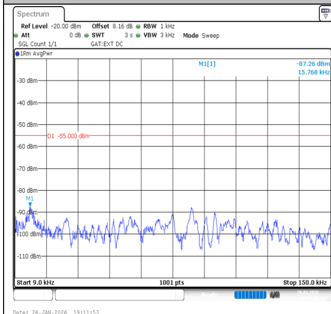
Band41-20MHz-QPSK-39750-1RB#0-0.009~0.15-PASS
