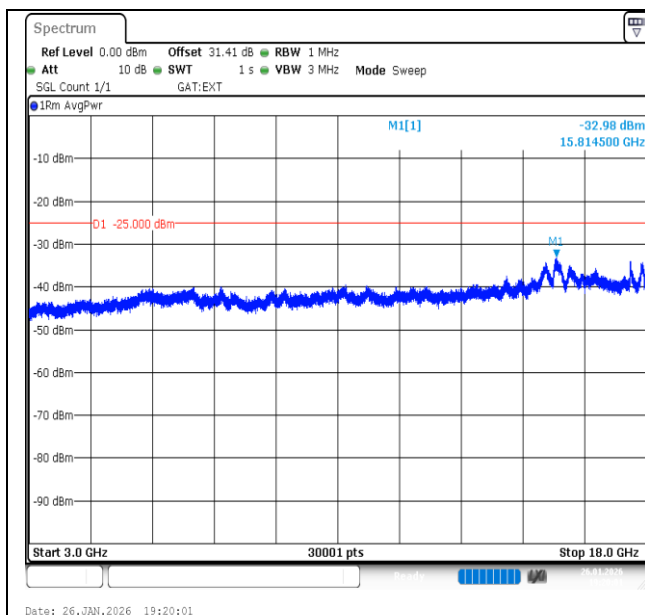
Band41-20MHz-QPSK-39750-1RB#99-3000~18000-PASS
