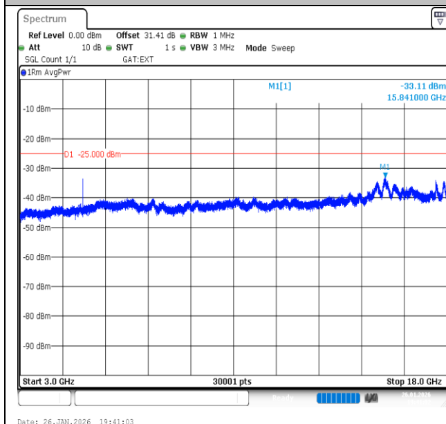
Band41-20MHz-QPSK-40620-1RB#99-3000~18000-PASS
