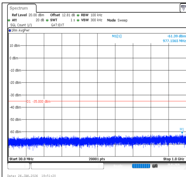
Band41-15MHz-QPSK-41515-1RB#0-30~1000-PASS
