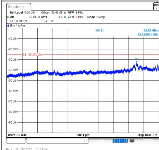
Band41-15MHz-16QAM-40620-1RB#0-3000~18000-PASS
