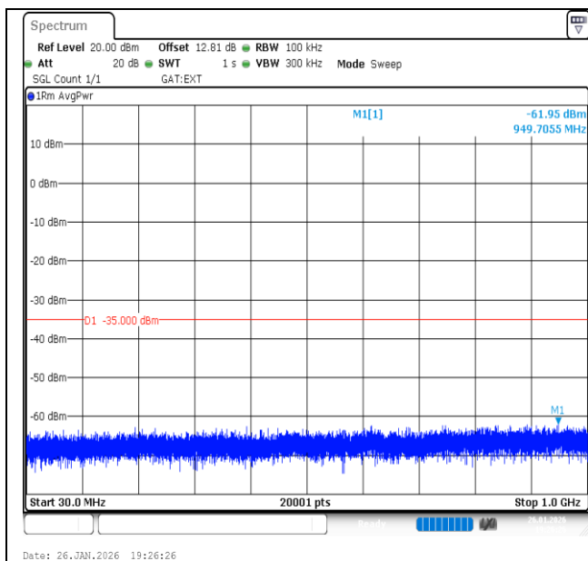
Band41-20MHz-QPSK-39750-100RB#0-30~1000-PASS
