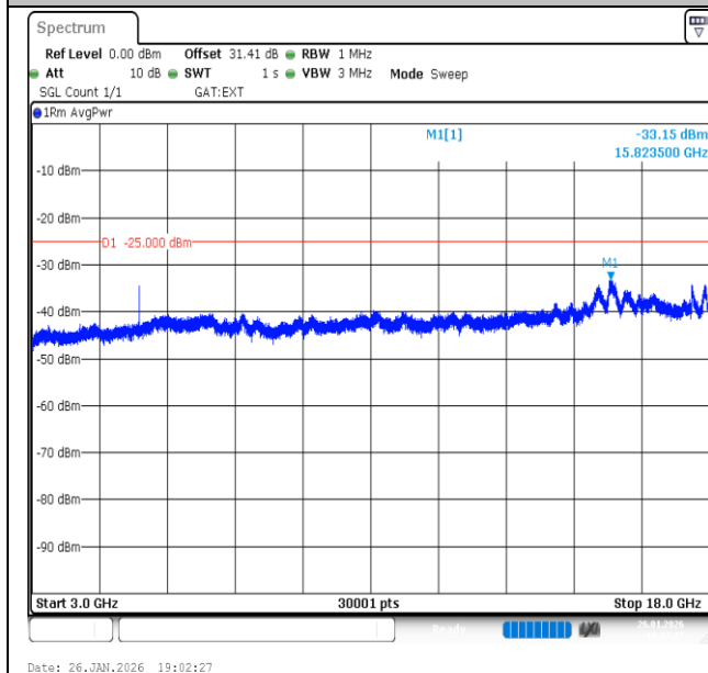
Band41-15MHz-16QAM-41515-1RB#74-3000~18000-PASS
