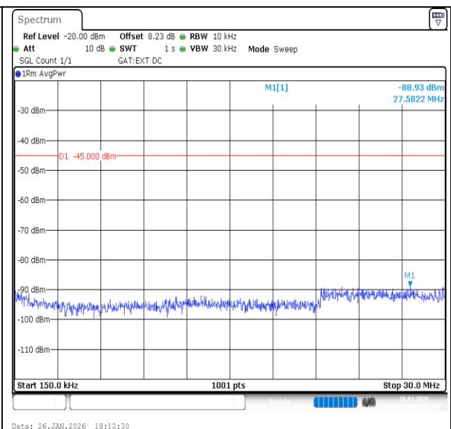
Band41-15MHz-16QAM-39725-1RB#0-0.15~30-PASS
