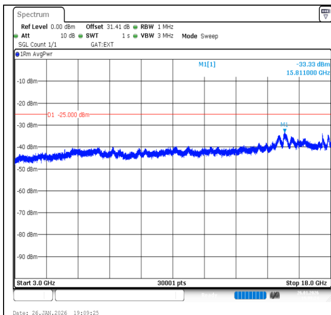
Band41-15MHz-16QAM-41515-75RB#0-3000~18000-PASS
