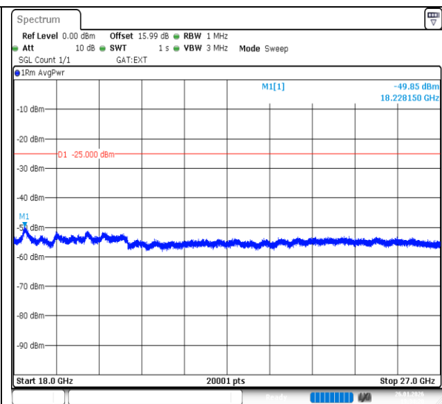
Band41-20MHz-QPSK-40620-1RB#0-18000~27000-PASS
