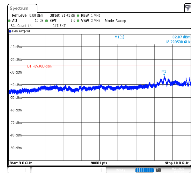
Band41-20MHz-QPSK-40620-1RB#0-3000~18000-PASS
