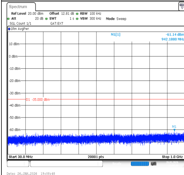
Band41-15MHz-16QAM-41515-75RB#0-30~1000-PASS
