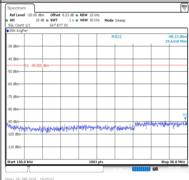
Band41-15MHz-QPSK-41515-75RB#0-0.15~30-PASS
