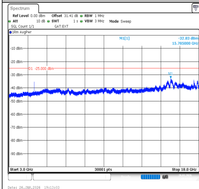
Band41-20MHz-QPSK-39750-1RB#0-3000~18000-PASS
