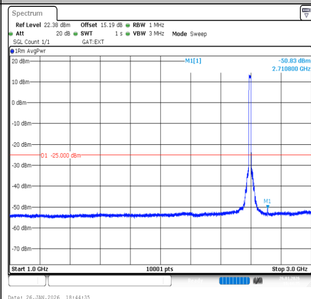
Band41-15MHz-QPSK-40620-75RB#0-1000~3000-PASS
