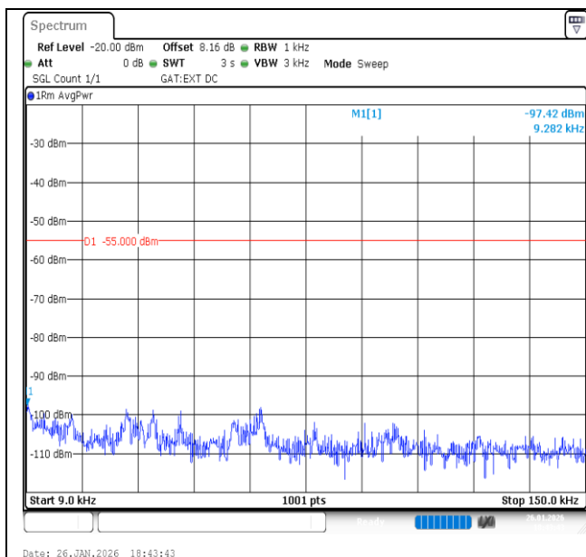
Band41-15MHz-QPSK-40620-75RB#0-0.009~0.15-PASS
