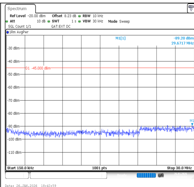
Band41-15MHz-QPSK-40620-75RB#0-0.15~30-PASS
