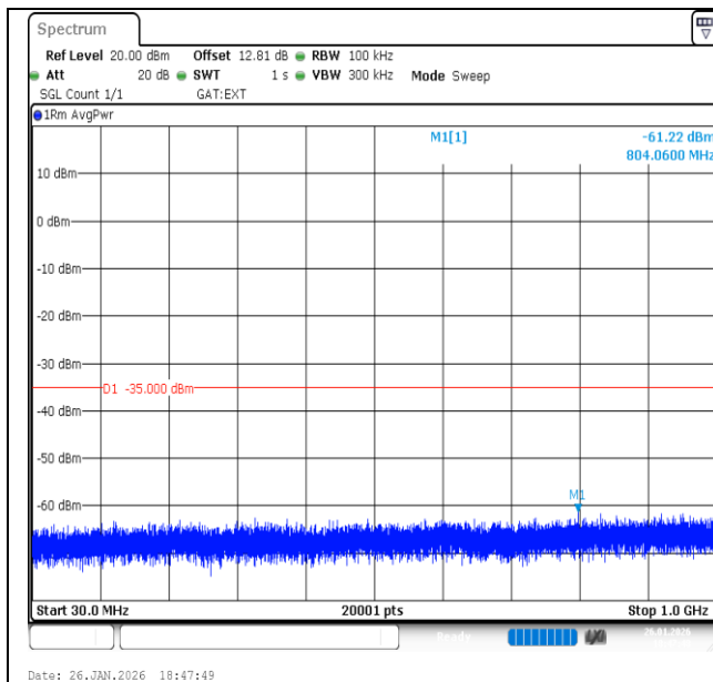
Band41-15MHz-16QAM-40620-75RB#0-30~1000-PASS
