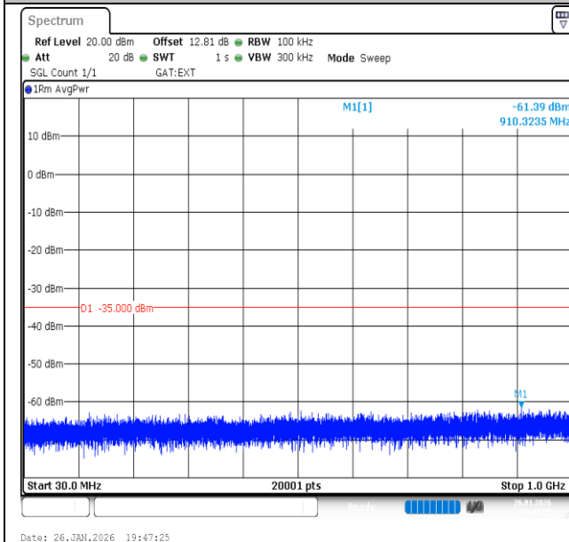
Band41-20MHz-QPSK-40620-100RB#0-30~1000-PASS
