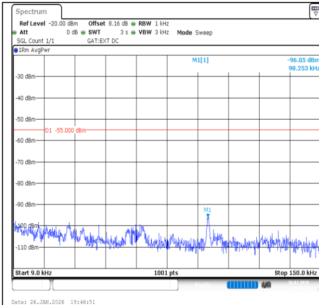
Band41-20MHz-QPSK-40620-100RB#0-0.009~0.15-PASS
