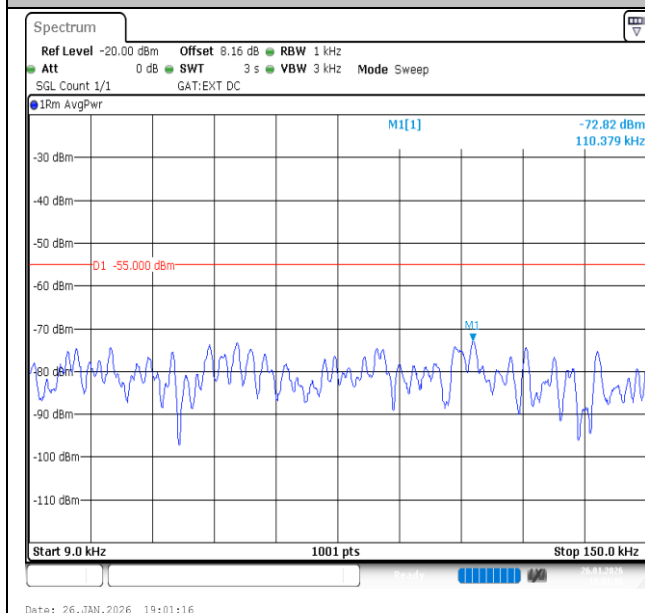
Band41-15MHz-16QAM-41515-1RB#74-0.009~0.15-PASS
