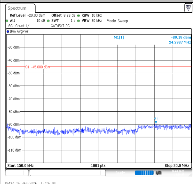
Band41-20MHz-QPSK-39750-100RB#0-0.15~30-PASS
