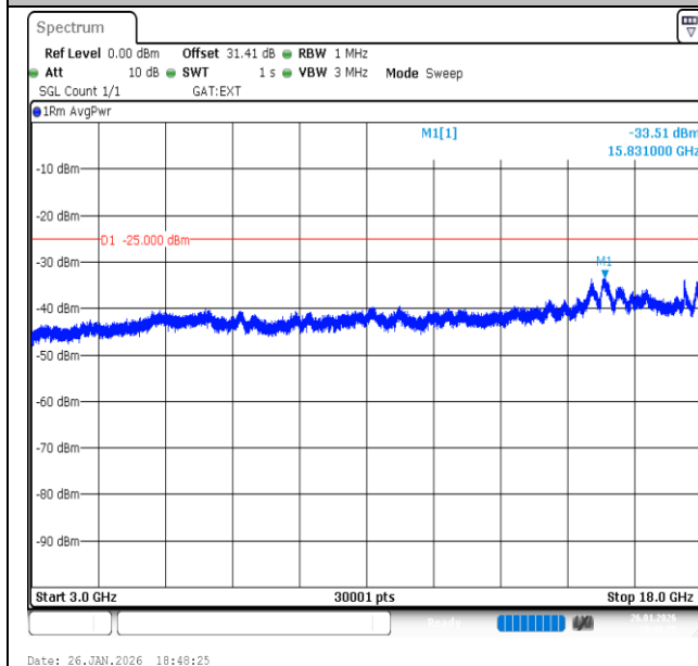
Band41-15MHz-16QAM-40620-75RB#0-3000~18000-PASS
