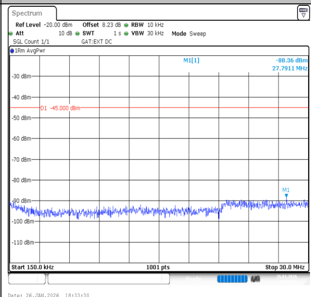
Band41-15MHz-16QAM-40620-1RB#0-0.15~30-PASS
