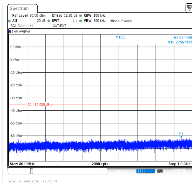
Band41-15MHz-16QAM-41515-1RB#74-30~1000-PASS
