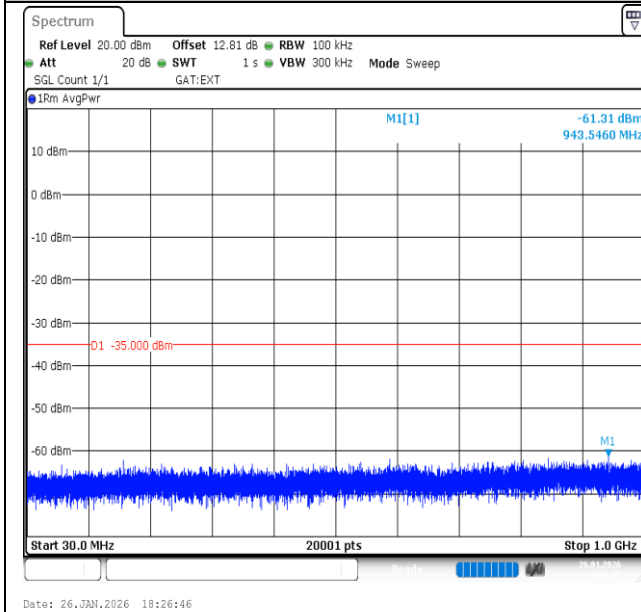
Band41-15MHz-16QAM-39725-75RB#0-30~1000-PASS
