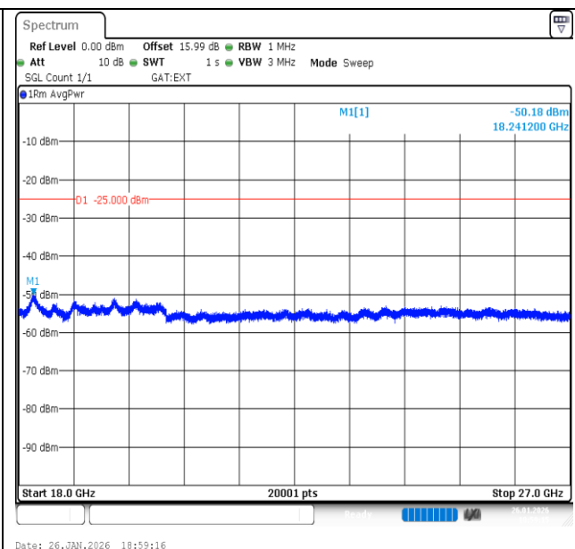
Band41-15MHz-QPSK-41515-1RB#74-18000~27000-PASS
