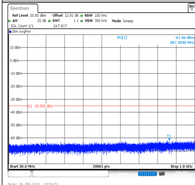
Band41-15MHz-16QAM-41515-1RB#0-30~1000-PASS
