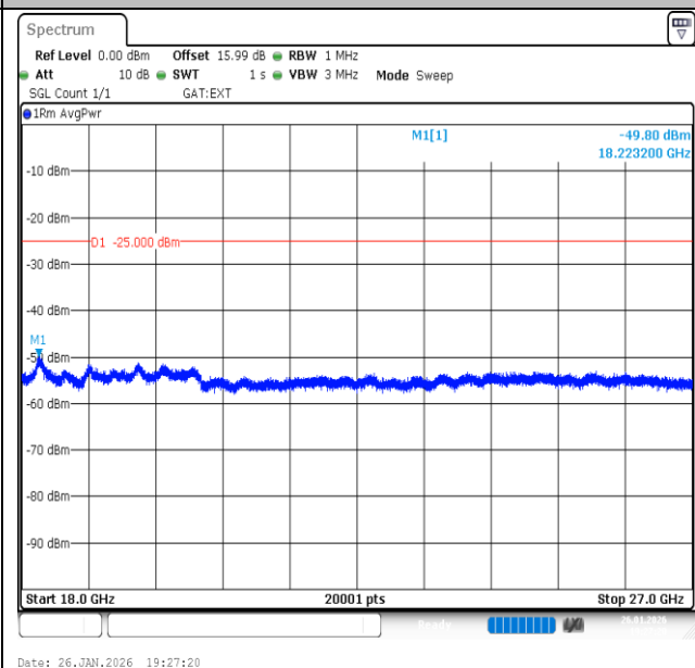
Band41-20MHz-QPSK-39750-100RB#0-18000~27000-PASS
