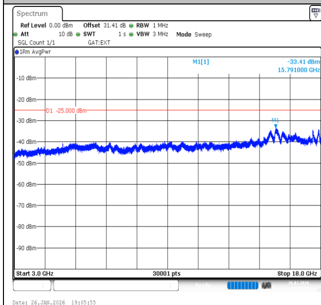
Band41-15MHz-QPSK-41515-75RB#0-3000~18000-PASS
