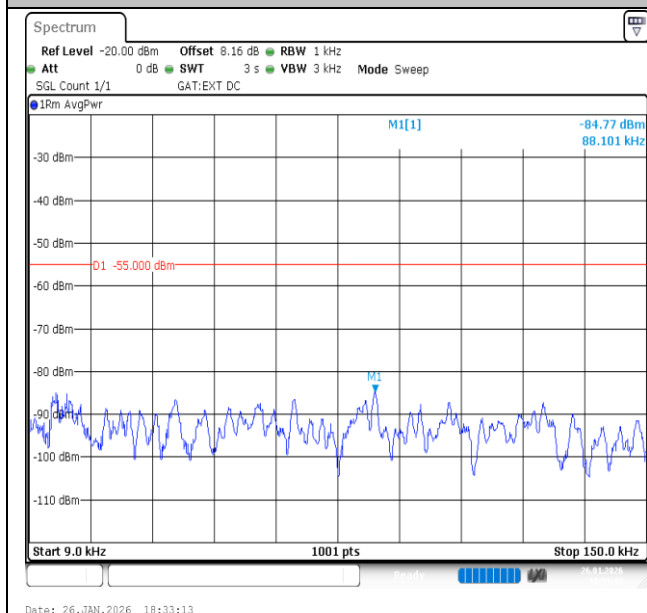
Band41-15MHz-16QAM-40620-1RB#0-0.009~0.15-PASS
