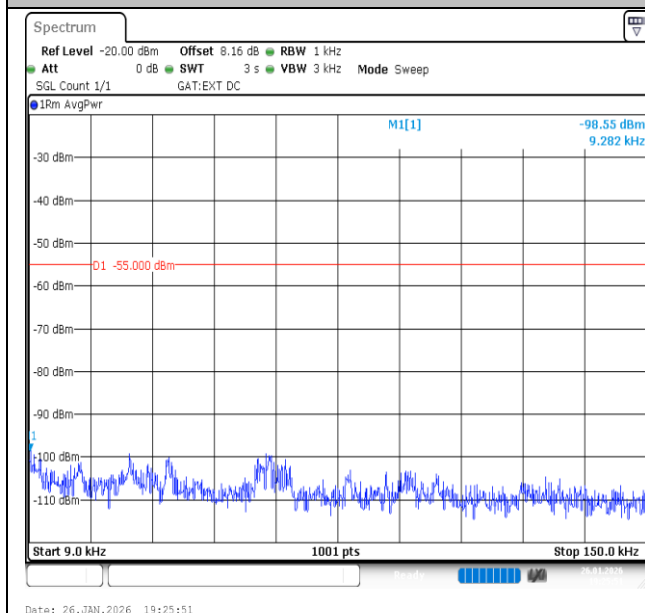
Band41-20MHz-QPSK-39750-100RB#0-0.009~0.15-PASS
