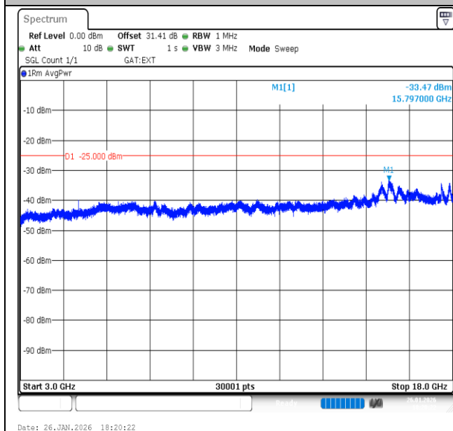
Band41-15MHz-16QAM-39725-1RB#74-3000~18000-PASS
