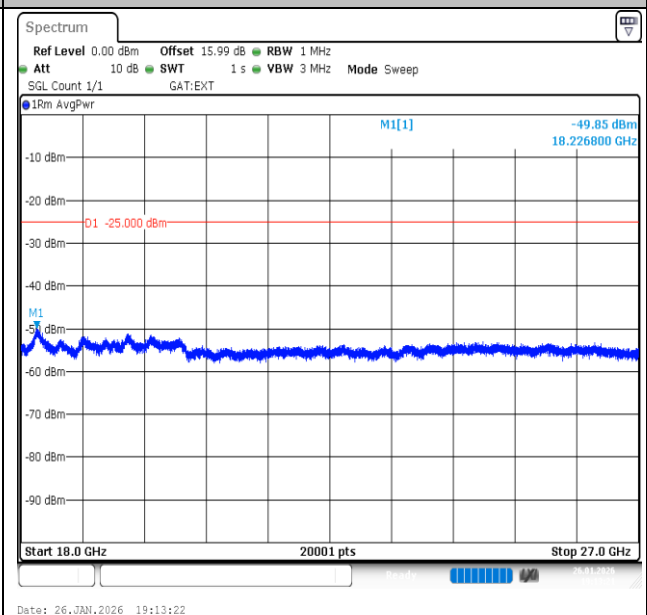
Band41-20MHz-QPSK-39750-1RB#0-18000~27000-PASS
