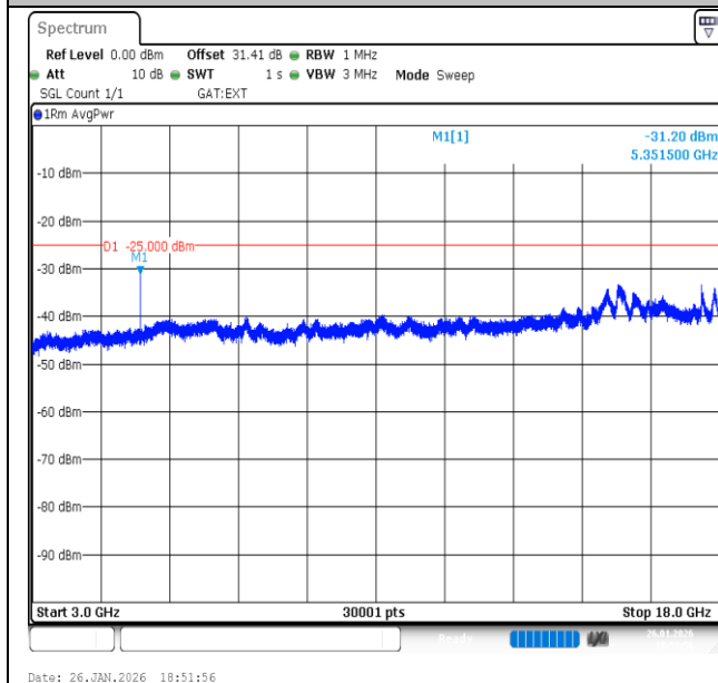
Band41-15MHz-QPSK-41515-1RB#0-3000~18000-PASS
