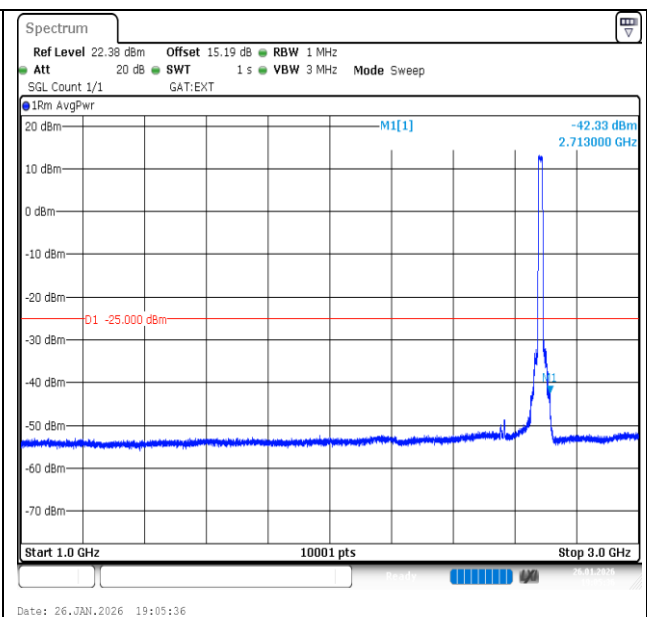
Band41-15MHz-QPSK-41515-75RB#0-1000~3000-PASS
