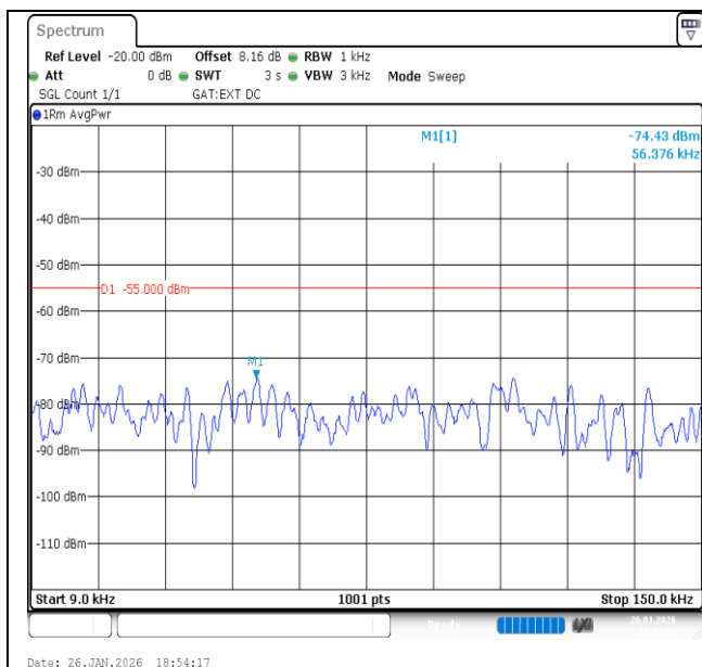
Band41-15MHz-16QAM-41515-1RB#0-0.009~0.15-PASS
