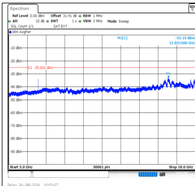
Band41-15MHz-16QAM-41515-1RB#0-3000~18000-PASS
