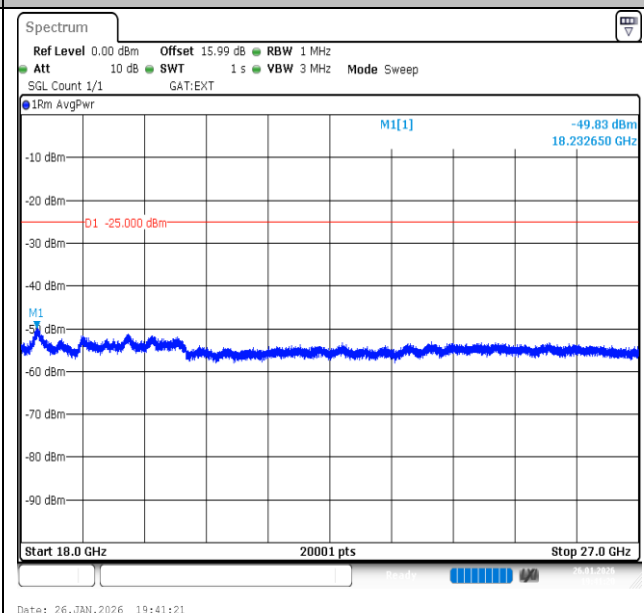
Band41-20MHz-QPSK-40620-1RB#99-18000~27000-PASS
