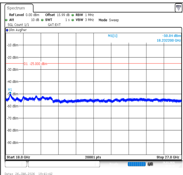
Band41-15MHz-16QAM-40620-1RB#74-18000~27000-PASS
