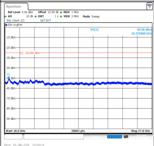
Band41-15MHz-QPSK-41515-75RB#0-18000~27000-PASS
