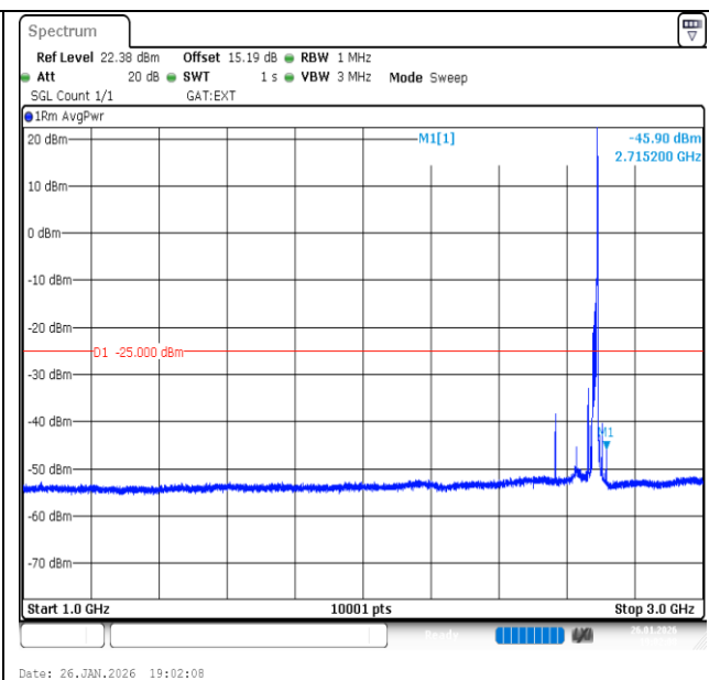
Band41-15MHz-16QAM-41515-1RB#74-1000~3000-PASS
