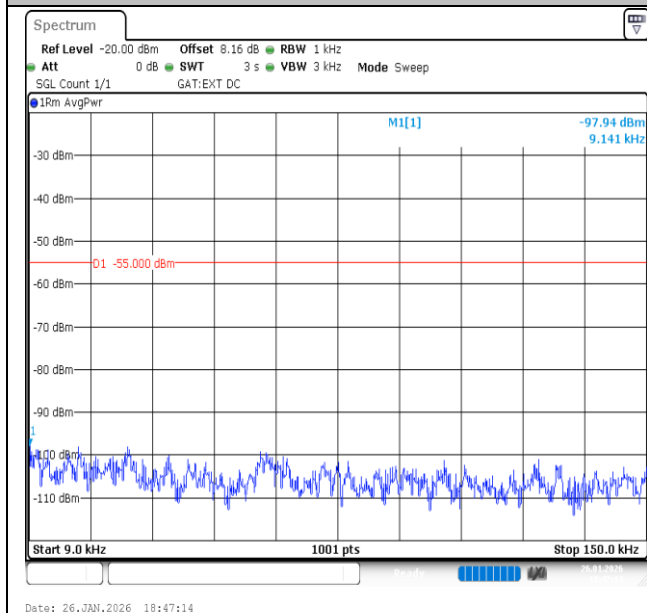
Band41-15MHz-16QAM-40620-75RB#0-0.009~0.15-PASS
