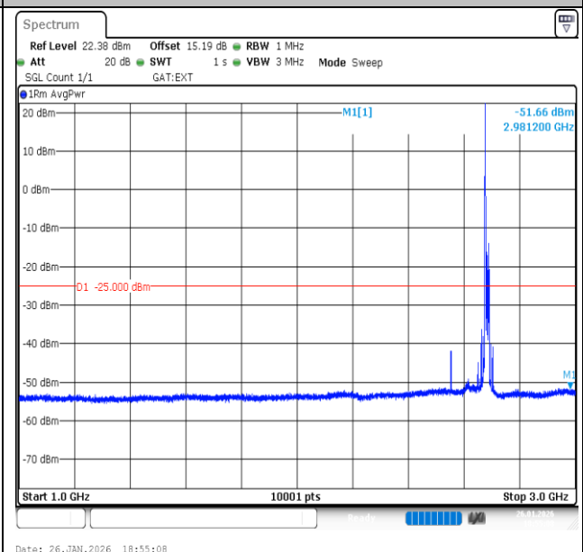
Band41-15MHz-16QAM-41515-1RB#0-1000~3000-PASS
