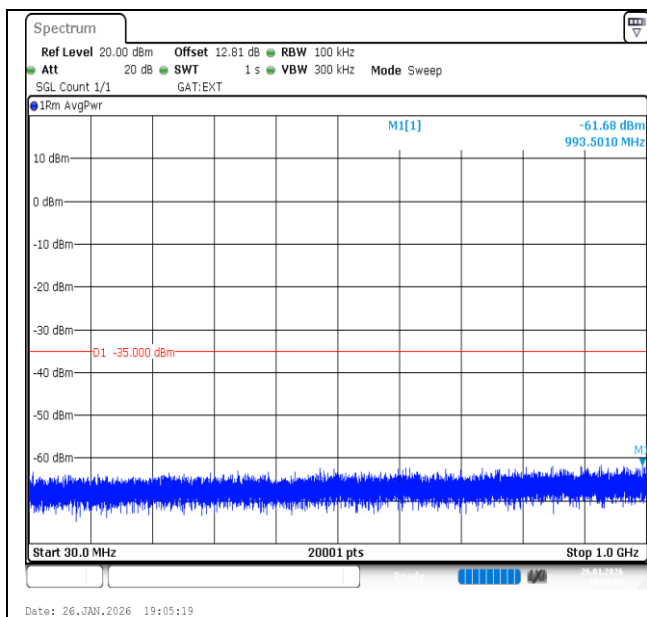
Band41-15MHz-QPSK-41515-75RB#0-30~1000-PASS
