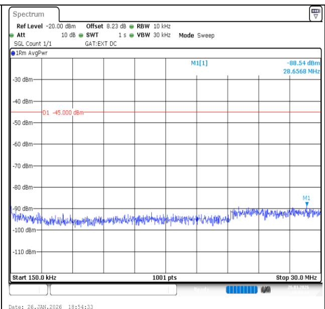
Band41-15MHz-16QAM-41515-1RB#0-0.15~30-PASS
