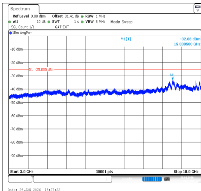
Band41-15MHz-16QAM-39725-75RB#0-3000~18000-PASS
