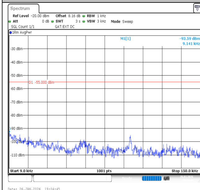
Band41-15MHz-QPSK-41515-75RB#0-0.009~0.15-PASS
