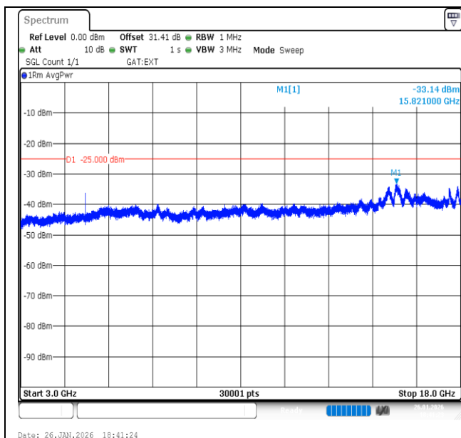
Band41-15MHz-16QAM-40620-1RB#74-3000~18000-PASS
