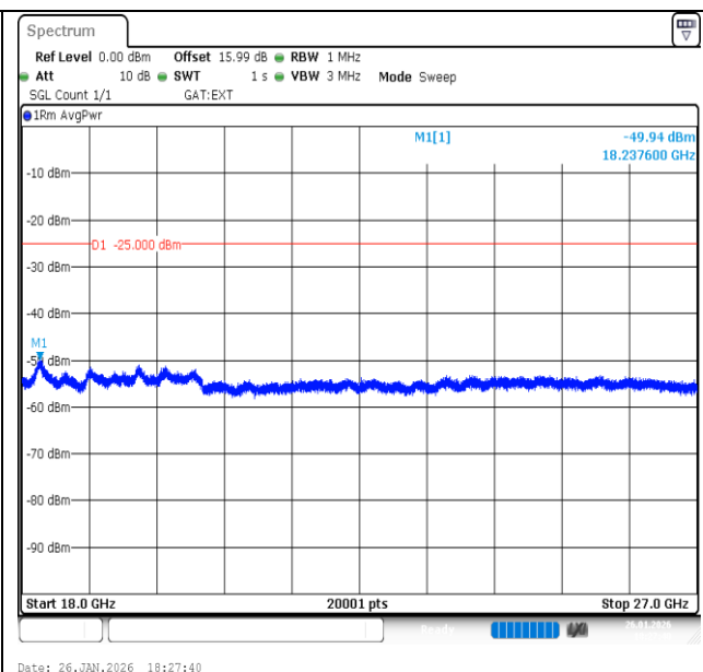
Band41-15MHz-16QAM-39725-75RB#0-18000~27000-PASS
