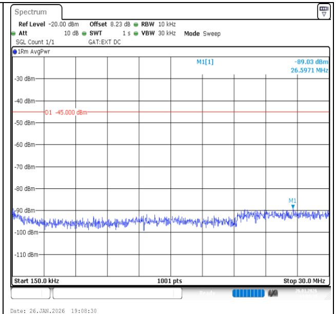
Band41-15MHz-16QAM-41515-75RB#0-0.15~30-PASS
