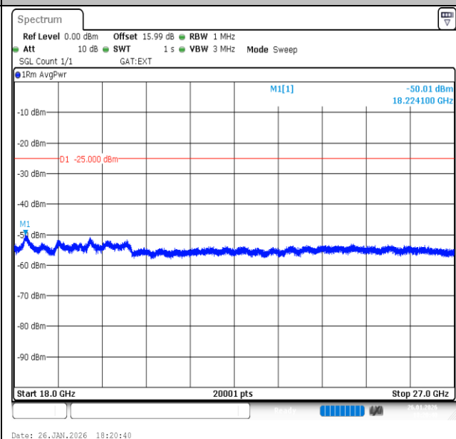
Band41-15MHz-16QAM-39725-1RB#74-18000~27000-PASS
