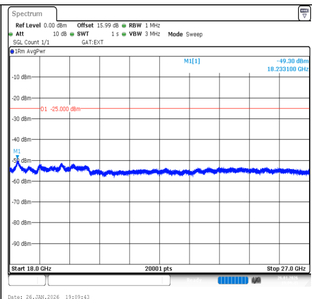
Band41-15MHz-16QAM-41515-75RB#0-18000~27000-PASS
