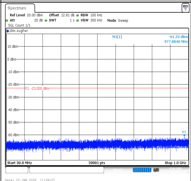
Band66-1.4MHz-QPSK-132322-1RB#0-30~1000-PASS
