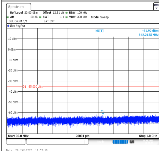
Band41-20MHz-16QAM-41490-1RB#0-30~1000-PASS
