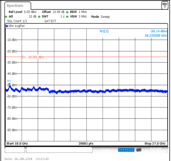
Band41-20MHz-16QAM-39750-1RB#99-18000~27000-PASS
