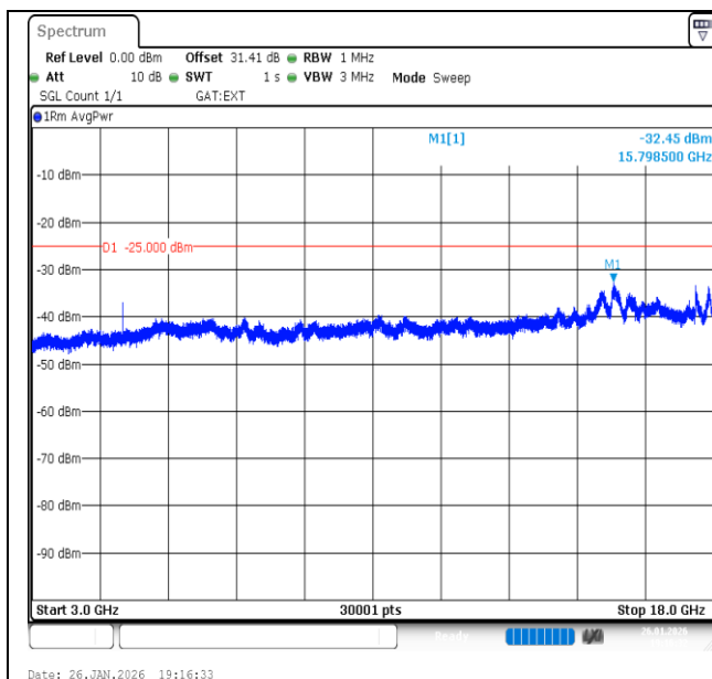
Band41-20MHz-16QAM-39750-1RB#0-3000~18000-PASS
