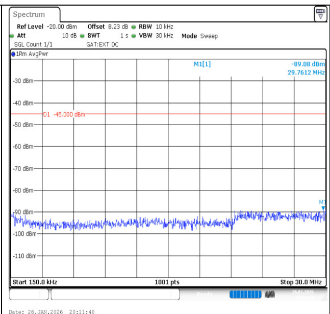
Band41-20MHz-16QAM-41490-100RB#0-0.15~30-PASS
