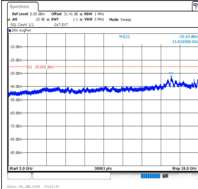
Band41-20MHz-16QAM-39750-1RB#99-3000~18000-PASS
