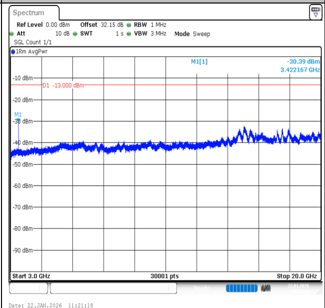
Band66-1.4MHz-QPSK-131979-1RB#5-3000~20000-PASS
