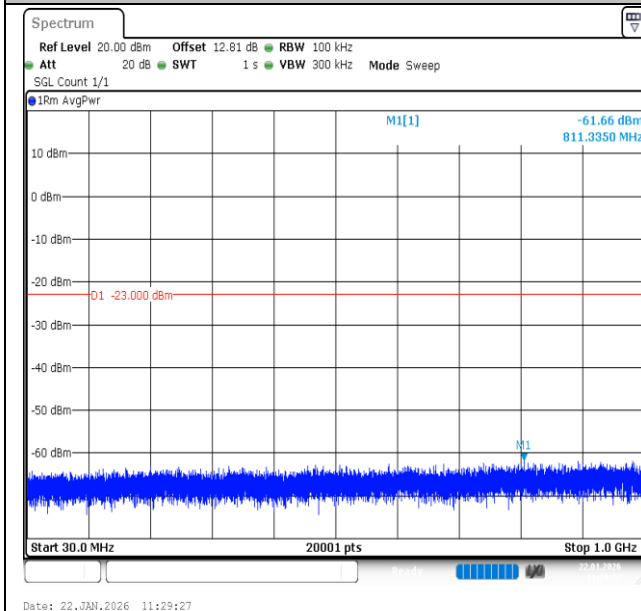
Band66-1.4MHz-QPSK-132665-1RB#0-30~1000-PASS
