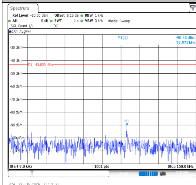
Band66-1.4MHz-QPSK-131979-1RB#0-0.009~0.15-PASS
