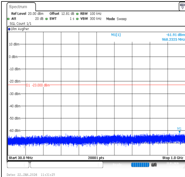
Band66-1.4MHz-QPSK-132665-6RB#0-30~1000-PASS
