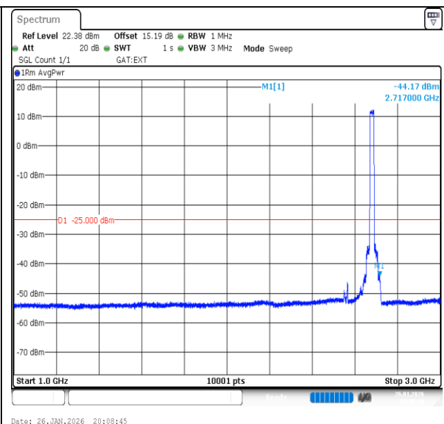
Band41-20MHz-QPSK-41490-100RB#0-1000~3000-PASS
