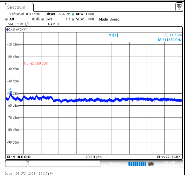
Band41-20MHz-16QAM-40620-1RB#0-18000~27000-PASS
