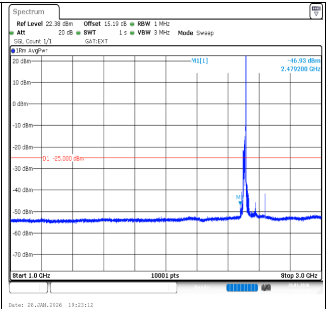
Band41-20MHz-16QAM-39750-1RB#99-1000~3000-PASS
