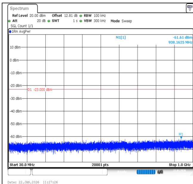
Band66-1.4MHz-QPSK-132322-1RB#5-30~1000-PASS
