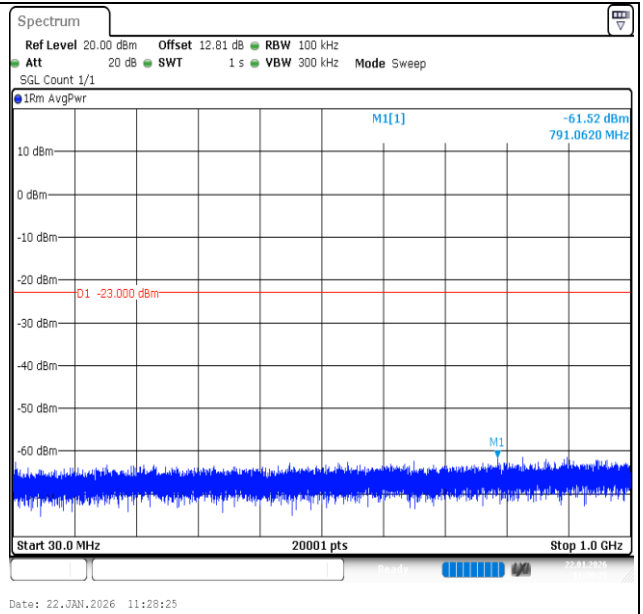
Band66-1.4MHz-QPSK-132322-6RB#0-30~1000-PASS
