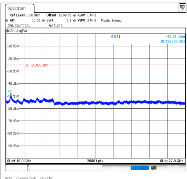
Band41-20MHz-16QAM-39750-1RB#0-18000~27000-PASS
