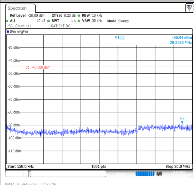
Band41-20MHz-16QAM-39750-1RB#99-0.15~30-PASS
