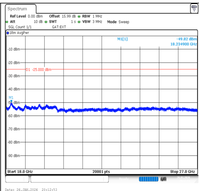
Band41-20MHz-16QAM-41490-100RB#0-18000~27000-PASS
