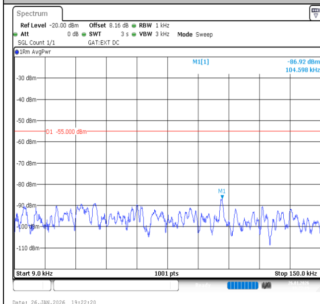
Band41-20MHz-16QAM-39750-1RB#99-0.009~0.15-PASS
