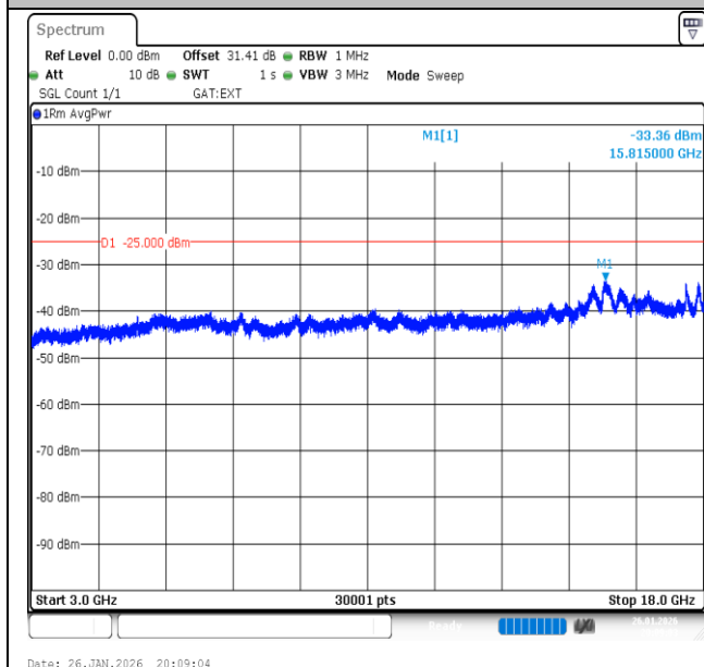
Band41-20MHz-QPSK-41490-100RB#0-3000~18000-PASS
