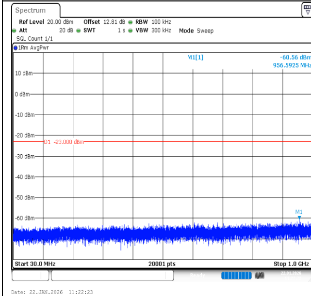
Band66-1.4MHz-QPSK-131979-6RB#0-30~1000-PASS
