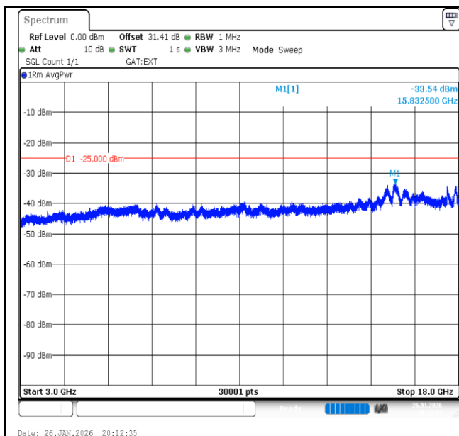
Band41-20MHz-16QAM-41490-100RB#0-3000~18000-PASS
