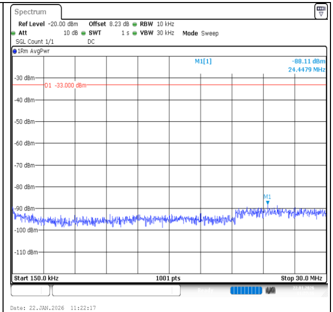
Band66-1.4MHz-QPSK-131979-6RB#0-0.15~30-PASS
