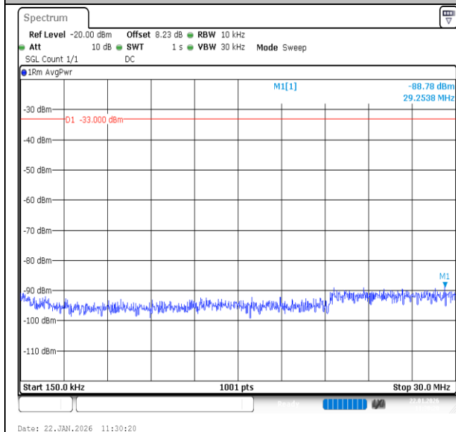
Band66-1.4MHz-QPSK-132665-1RB#5-0.15~30-PASS
