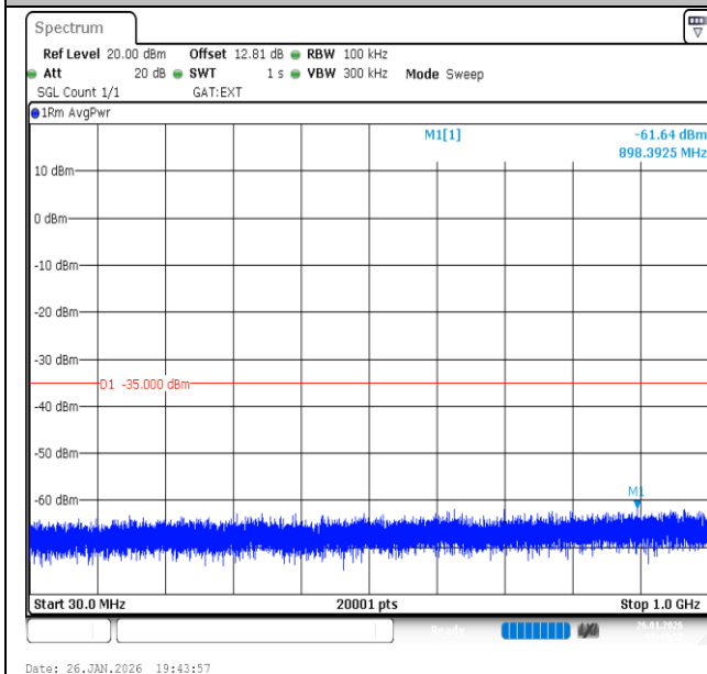
Band41-20MHz-16QAM-40620-1RB#99-30~1000-PASS
