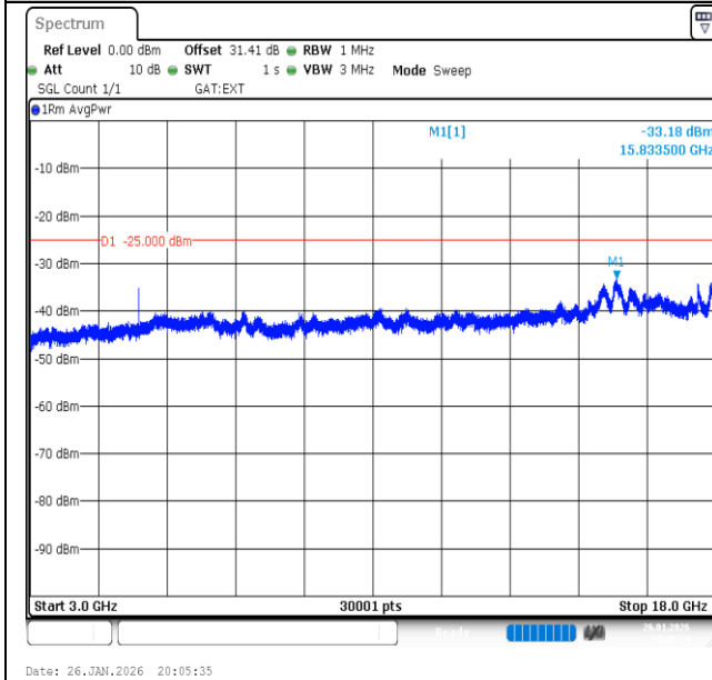
Band41-20MHz-16QAM-41490-1RB#99-3000~18000-PASS
