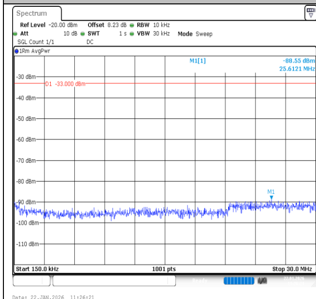
Band66-1.4MHz-QPSK-132322-1RB#0-0.15~30-PASS
