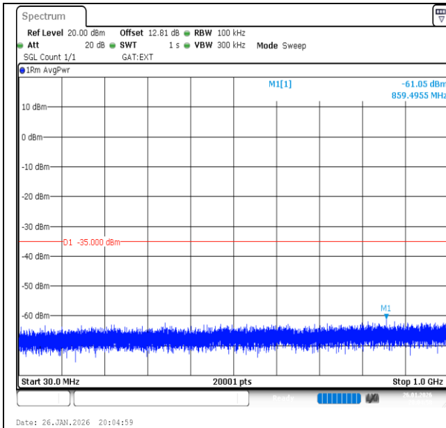
Band41-20MHz-16QAM-41490-1RB#99-30~1000-PASS
