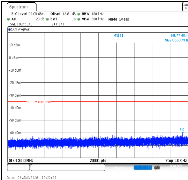
Band41-20MHz-16QAM-39750-1RB#99-30~1000-PASS
