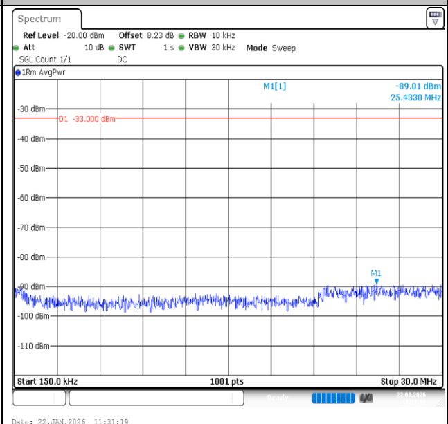
Band66-1.4MHz-QPSK-132665-6RB#0-0.15~30-PASS
