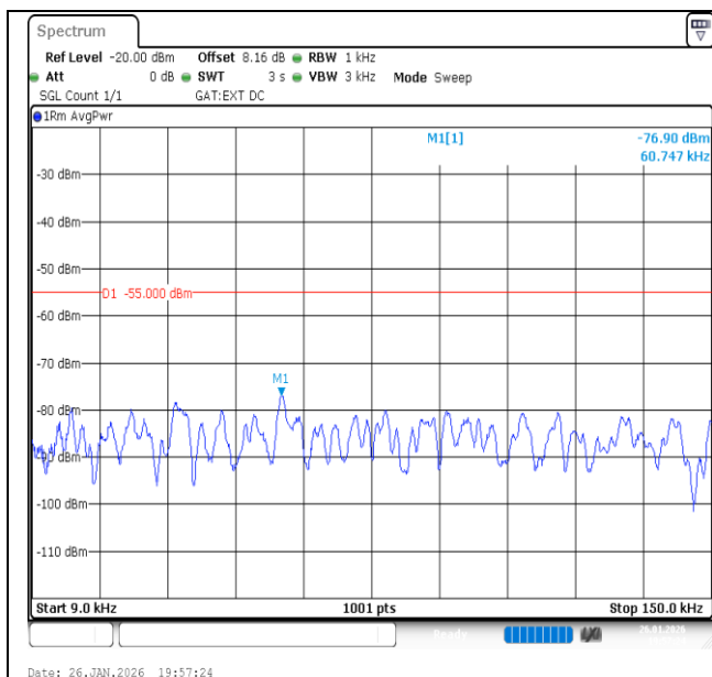
Band41-20MHz-16QAM-41490-1RB#0-0.009~0.15-PASS
