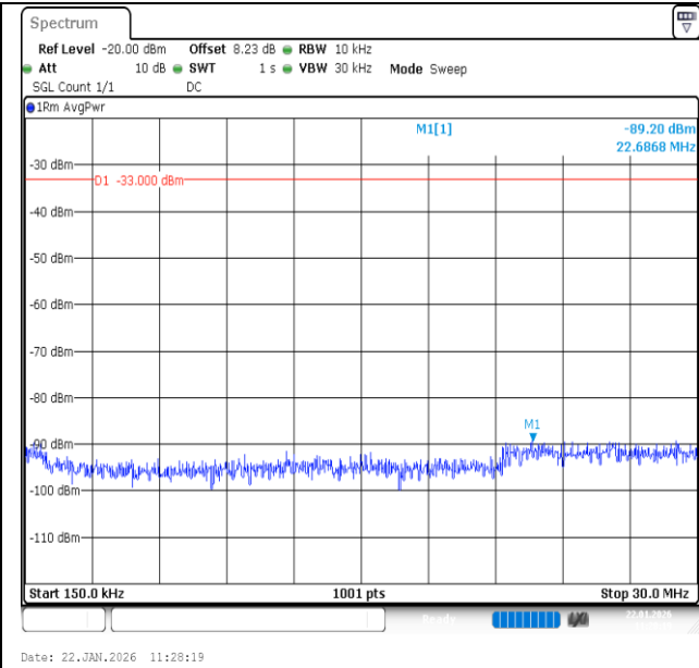
Band66-1.4MHz-QPSK-132322-6RB#0-0.15~30-PASS
