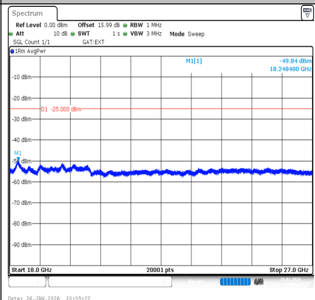
Band41-20MHz-QPSK-41490-100RB#0-18000~27000-PASS
