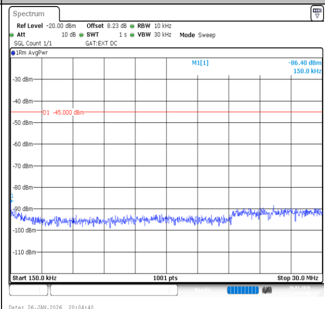
Band41-20MHz-16QAM-41490-1RB#99-0.15~30-PASS
