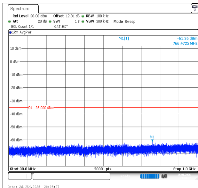
Band41-20MHz-QPSK-41490-100RB#0-30~1000-PASS
