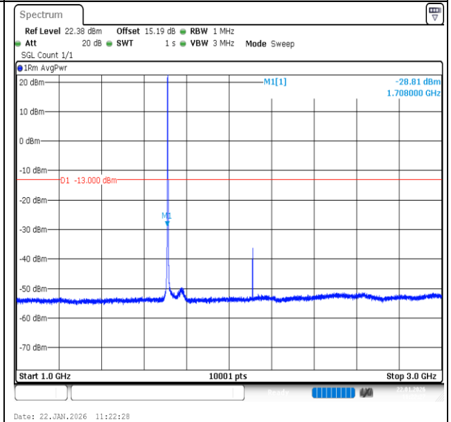
Band66-1.4MHz-QPSK-131979-6RB#0-1000~3000-PASS
