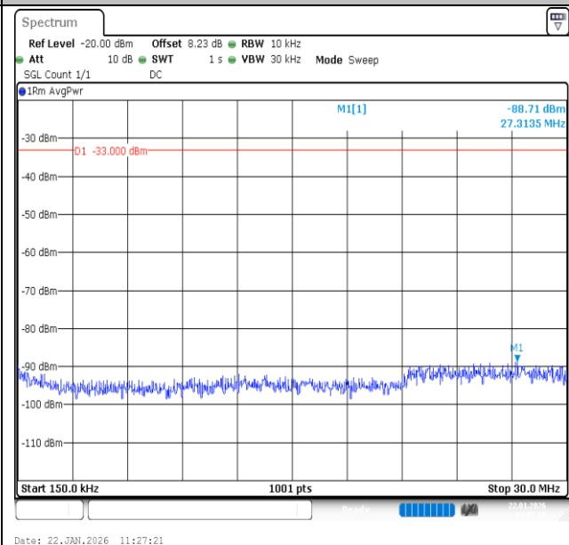
Band66-1.4MHz-QPSK-132322-1RB#5-0.15~30-PASS
