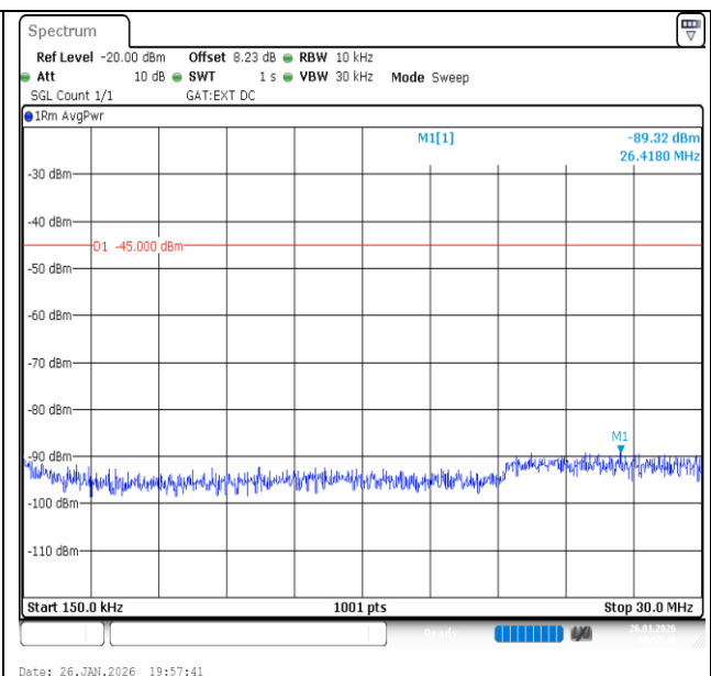
Band41-20MHz-16QAM-41490-1RB#0-0.15~30-PASS
