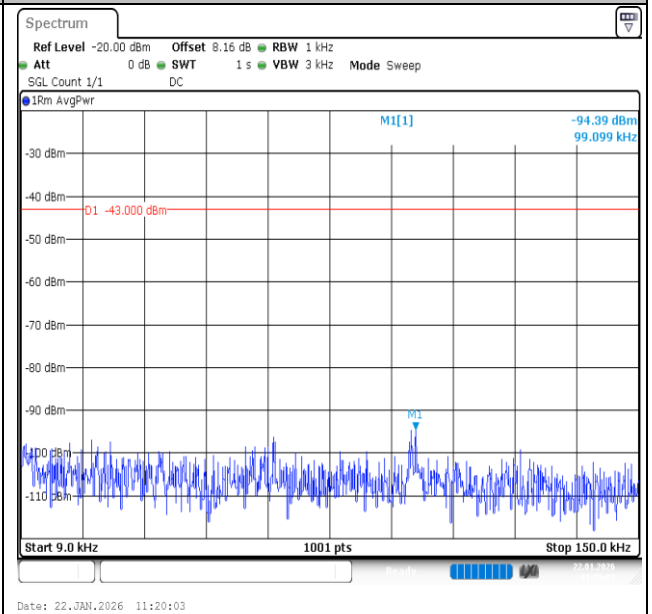
Band66-1.4MHz-16QAM-131979-1RB#0-0.009~0.15-PASS
