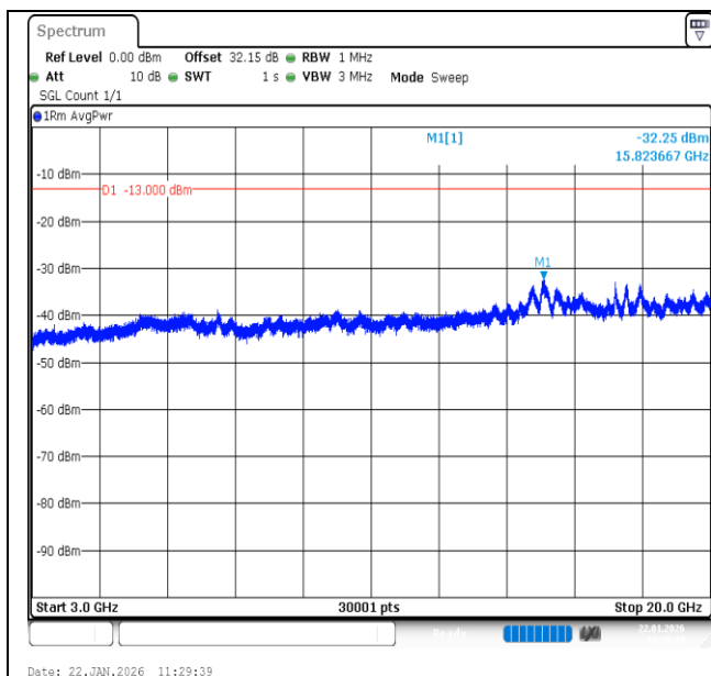
Band66-1.4MHz-QPSK-132665-1RB#0-3000~20000-PASS
