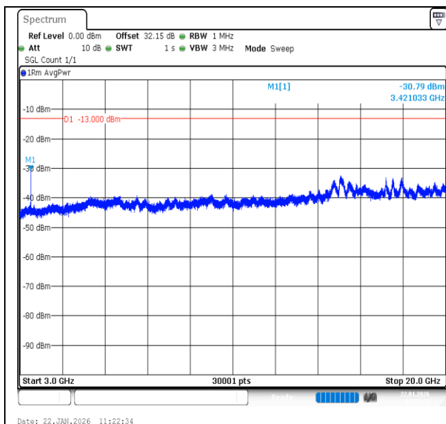
Band66-1.4MHz-QPSK-131979-6RB#0-3000~20000-PASS
