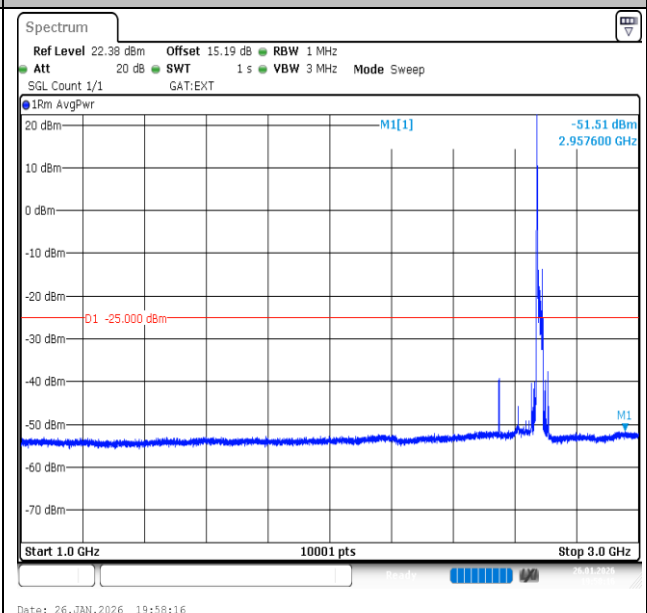
Band41-20MHz-16QAM-41490-1RB#0-1000~3000-PASS
