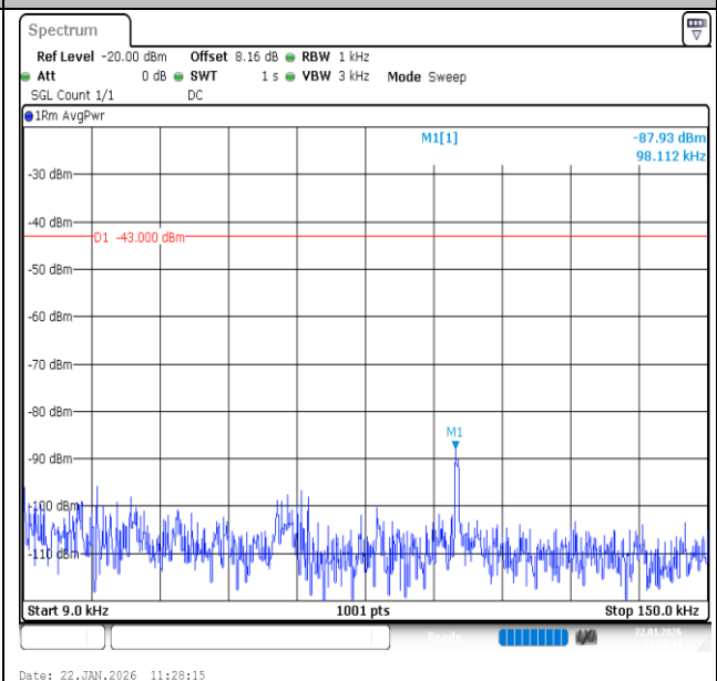
Band66-1.4MHz-QPSK-132322-6RB#0-0.009~0.15-PASS
