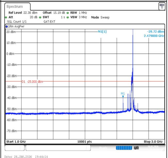
Band41-20MHz-16QAM-40620-1RB#99-1000~3000-PASS
