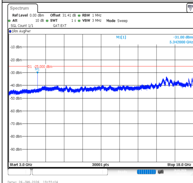
Band41-20MHz-QPSK-41490-1RB#0-3000~18000-PASS
