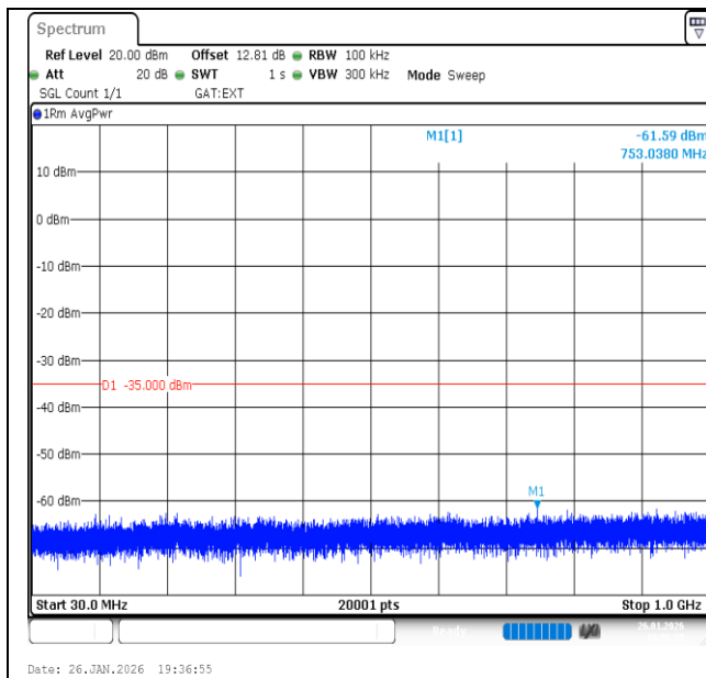
Band41-20MHz-16QAM-40620-1RB#0-30~1000-PASS
