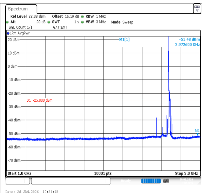
Band41-20MHz-QPSK-41490-1RB#0-1000~3000-PASS
