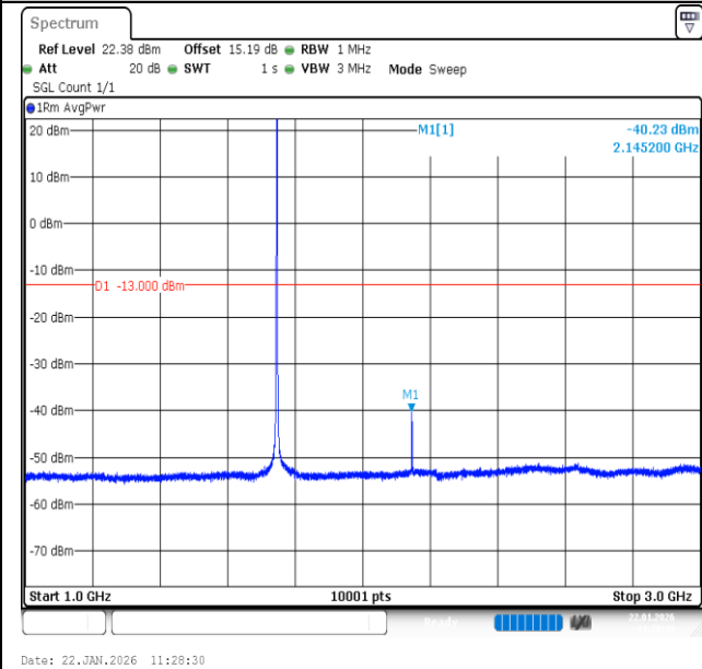
Band66-1.4MHz-QPSK-132322-6RB#0-1000~3000-PASS
