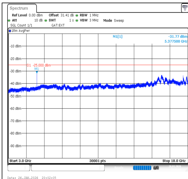
Band41-20MHz-QPSK-41490-1RB#99-3000~18000-PASS
