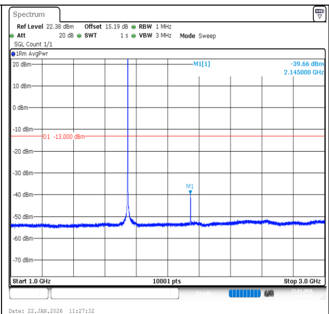
Band66-1.4MHz-QPSK-132322-1RB#5-1000~3000-PASS
