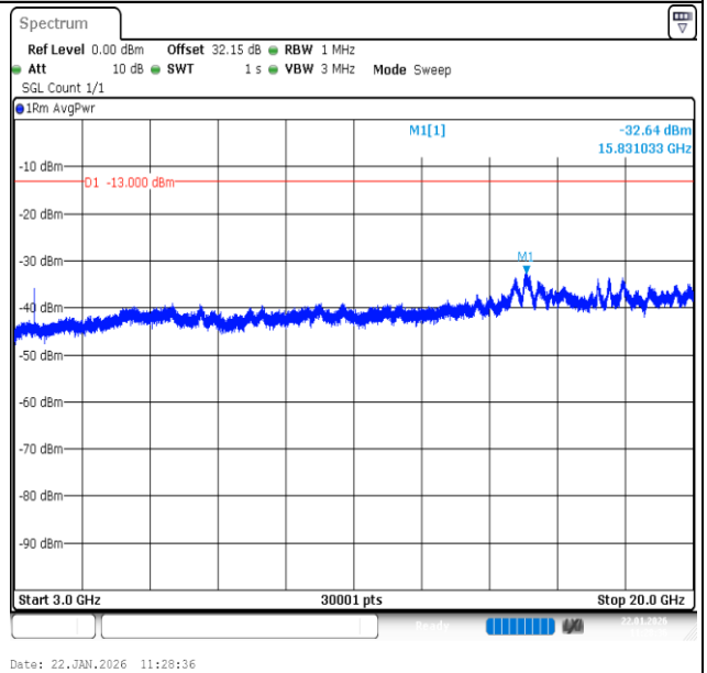
Band66-1.4MHz-QPSK-132322-6RB#0-3000~20000-PASS
