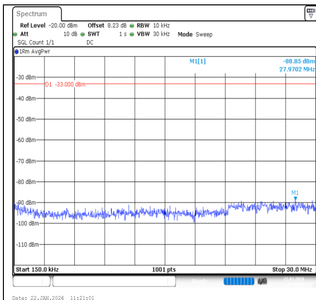
Band66-1.4MHz-QPSK-131979-1RB#5-0.15~30-PASS
