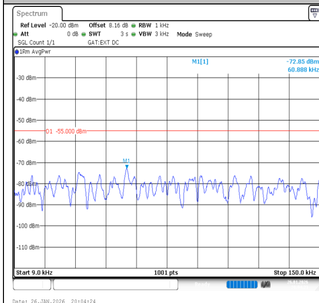
Band41-20MHz-16QAM-41490-1RB#99-0.009~0.15-PASS
