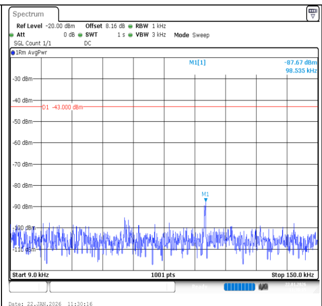
Band66-1.4MHz-QPSK-132665-1RB#5-0.009~0.15-PASS
