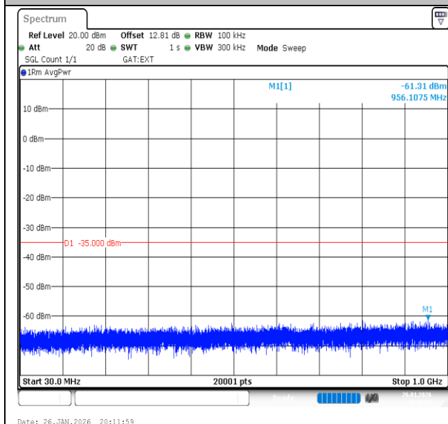
Band41-20MHz-16QAM-41490-100RB#0-30~1000-PASS
