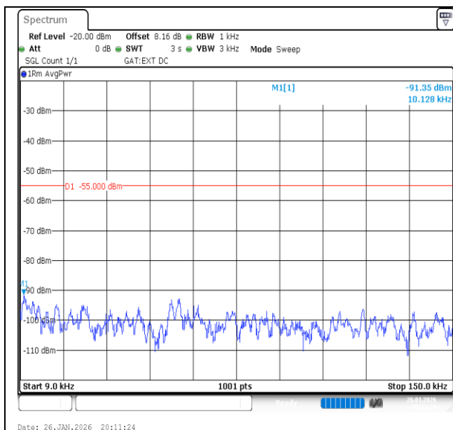
Band41-20MHz-16QAM-41490-100RB#0-0.009~0.15-PASS
