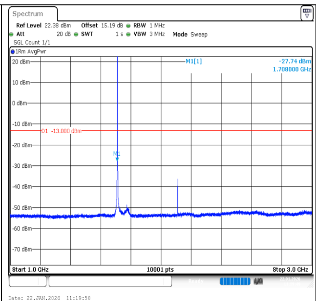
Band66-1.4MHz-QPSK-131979-1RB#0-1000~3000-PASS
