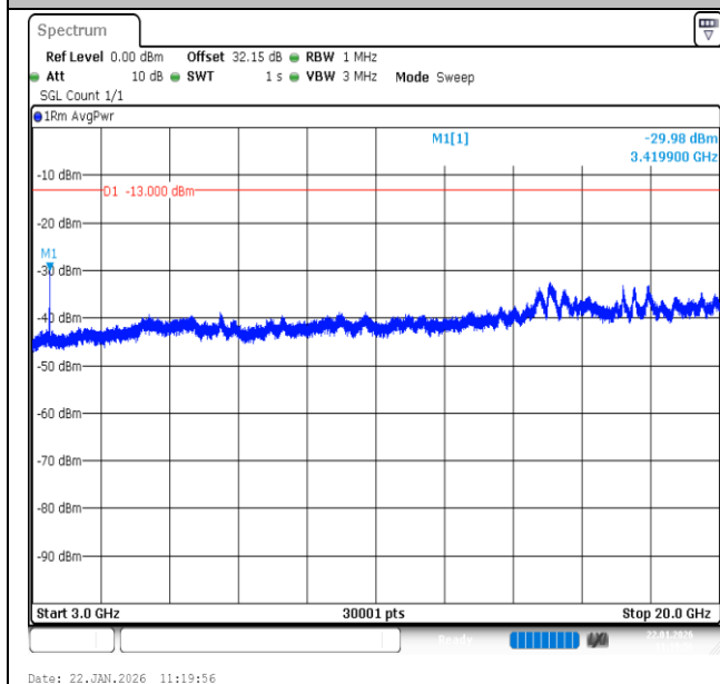
Band66-1.4MHz-QPSK-131979-1RB#0-3000~20000-PASS
