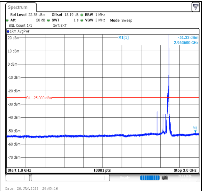
Band41-20MHz-16QAM-41490-1RB#99-1000~3000-PASS
