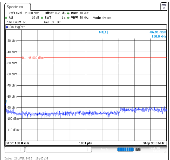
Band41-20MHz-16QAM-40620-1RB#99-0.15~30-PASS
