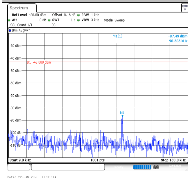
Band66-1.4MHz-QPSK-132665-6RB#0-0.009~0.15-PASS
