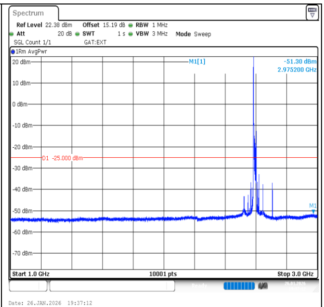
Band41-20MHz-16QAM-40620-1RB#0-1000~3000-PASS
