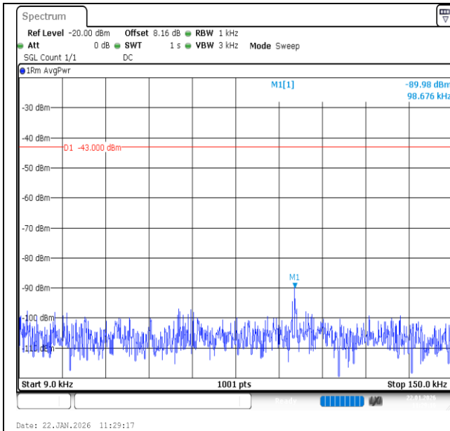
Band66-1.4MHz-QPSK-132665-1RB#0-0.009~0.15-PASS
