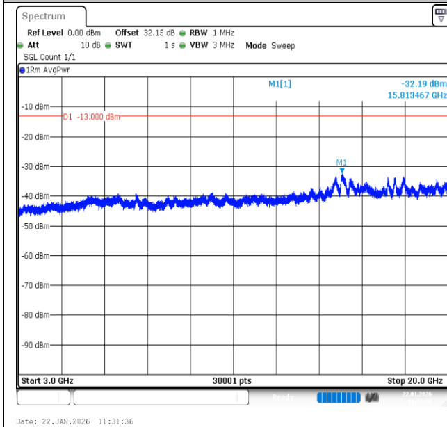
Band66-1.4MHz-QPSK-132665-6RB#0-3000~20000-PASS
