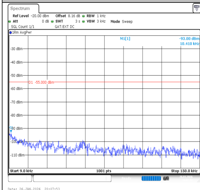
Band41-20MHz-QPSK-41490-100RB#0-0.009~0.15-PASS
