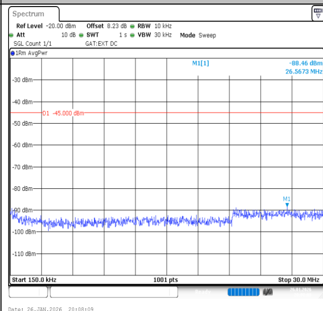
Band41-20MHz-QPSK-41490-100RB#0-0.15~30-PASS
