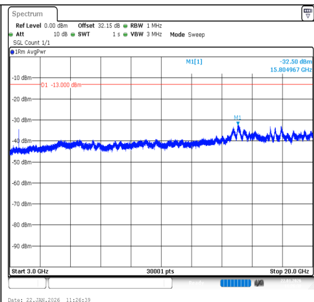
Band66-1.4MHz-QPSK-132322-1RB#0-3000-20000-PASS
