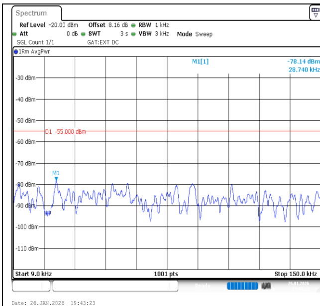
Band41-20MHz-16QAM-40620-1RB#99-0.009~0.15-PASS
