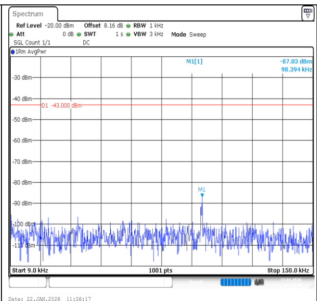
Band66-1.4MHz-QPSK-132322-1RB#0-0.009~0.15-PASS
