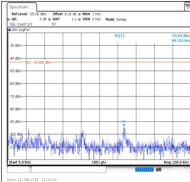
Band66-1.4MHz-QPSK-131979-6RB#0-0.009~0.15-PASS
