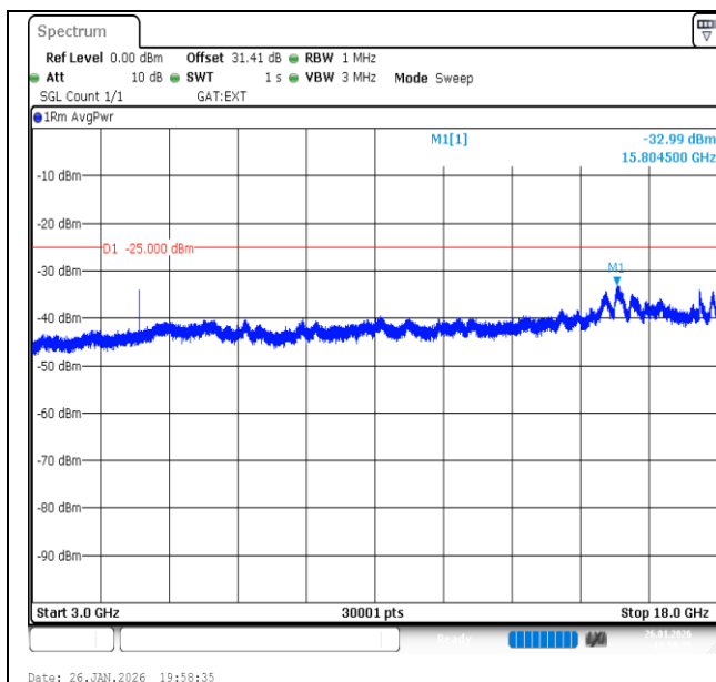
Band41-20MHz-16QAM-41490-1RB#0-3000~18000-PASS
