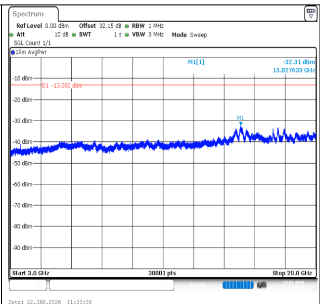
Band66-1.4MHz-QPSK-132665-1RB#5-3000~20000-PASS
