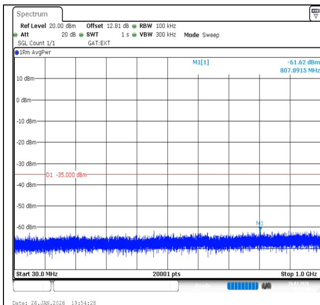
Band41-20MHz-QPSK-41490-1RB#0-30~1000-PASS
