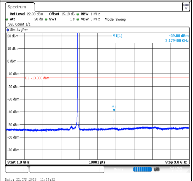
Band66-1.4MHz-QPSK-132665-1RB#0-1000~3000-PASS
