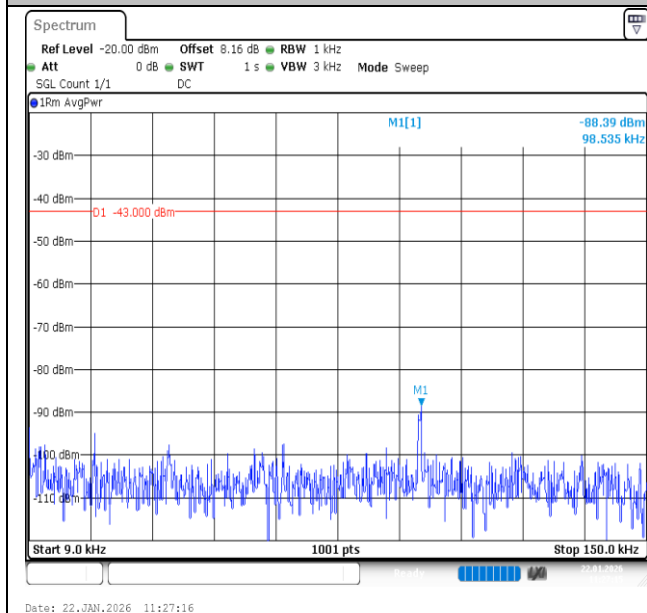
Band66-1.4MHz-QPSK-132322-1RB#5-0.009~0.15-PASS
