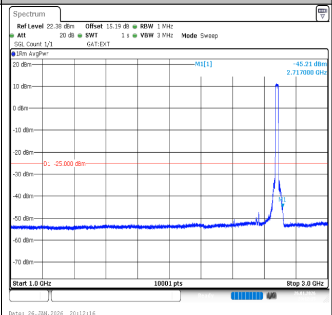
Band41-20MHz-16QAM-41490-100RB#0-1000~3000-PASS
