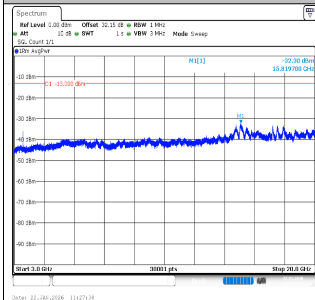
Band66-1.4MHz-QPSK-132322-1RB#5-3000~20000-PASS
