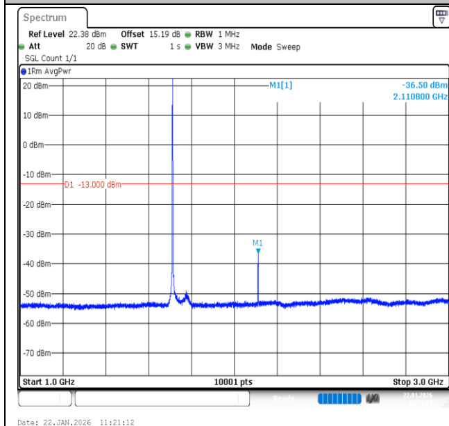
Band66-1.4MHz-QPSK-131979-1RB#5-1000~3000-PASS
