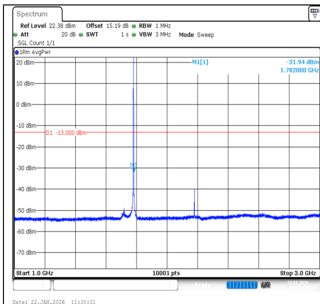
Band66-1.4MHz-QPSK-132665-1RB#5-1000~3000-PASS
