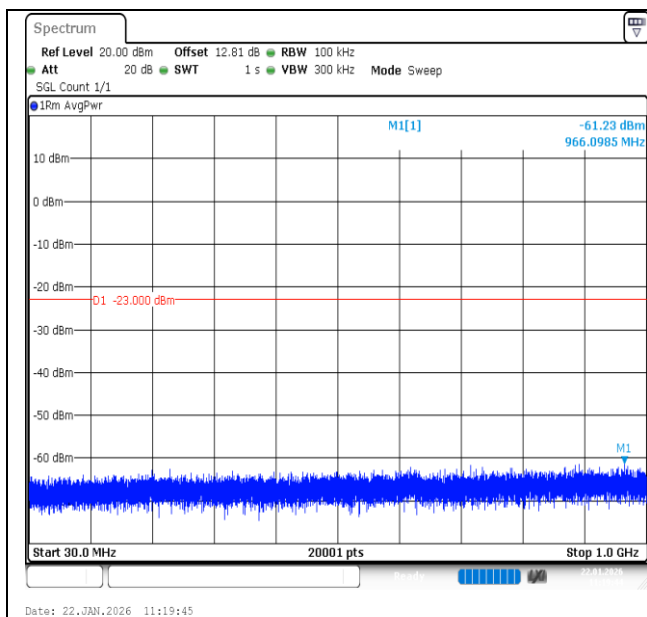
Band66-1.4MHz-QPSK-131979-1RB#0-30~1000-PASS
