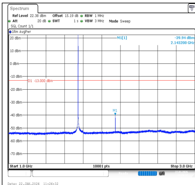
Band66-1.4MHz-QPSK-132322-1RB#0-1000-3000-PASS
