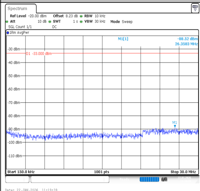
Band66-1.4MHz-QPSK-131979-1RB#0-0.15~30-PASS
