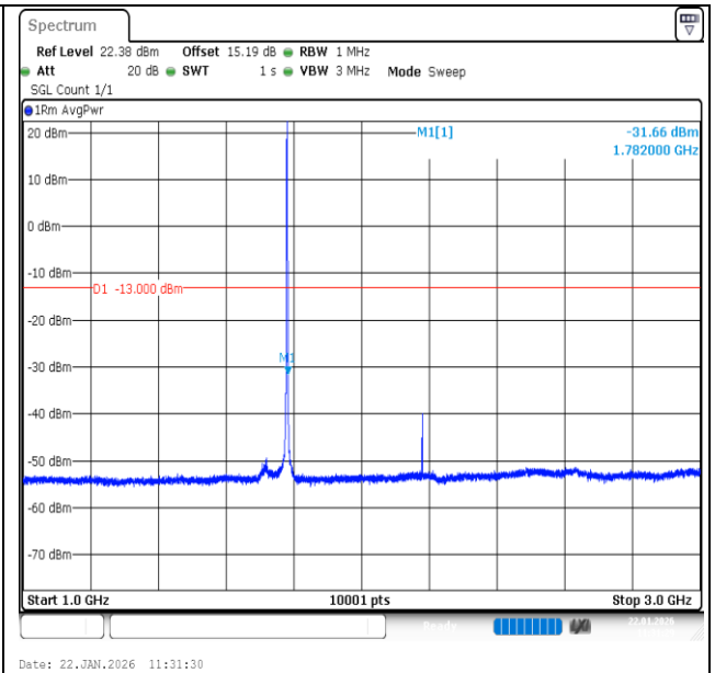
Band66-1.4MHz-QPSK-132665-6RB#0-1000~3000-PASS
