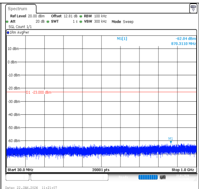
Band66-1.4MHz-QPSK-131979-1RB#5-30~1000-PASS
