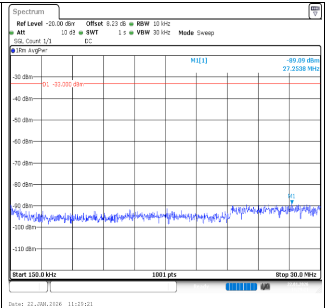
Band66-1.4MHz-QPSK-132665-1RB#0-0.15~30-PASS
