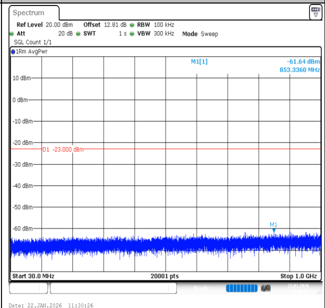
Band66-1.4MHz-QPSK-132665-1RB#5-30~1000-PASS
