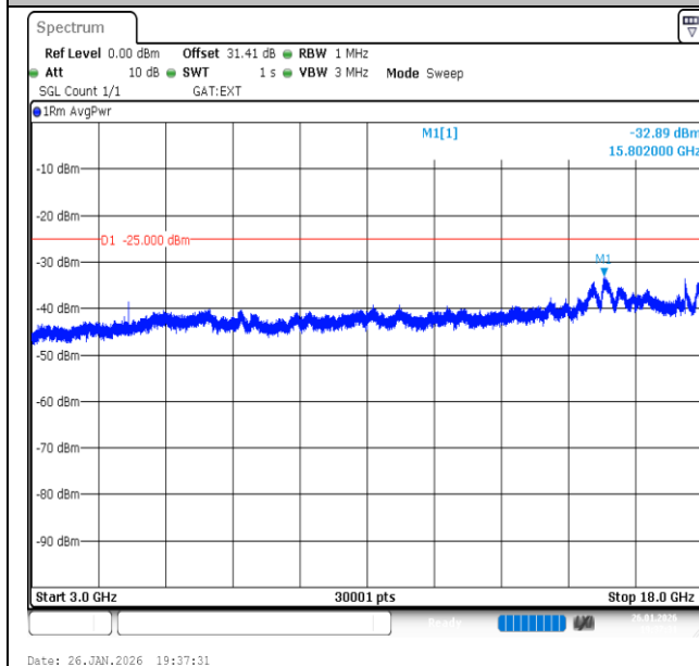
Band41-20MHz-16QAM-40620-1RB#0-3000~18000-PASS
