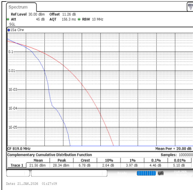
Band26(814-824)-10MHz-QPSK-26740-1RB#0-PASS
