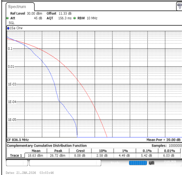
Band26(824-849)-15MHz-QPSK-26915-1RB#0-PASS
