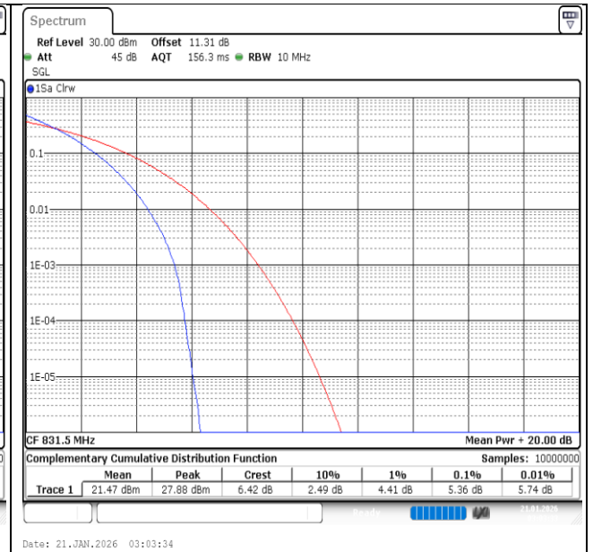
Band26(824-849)-15MHz-QPSK-26865-75RB#0-PASS
