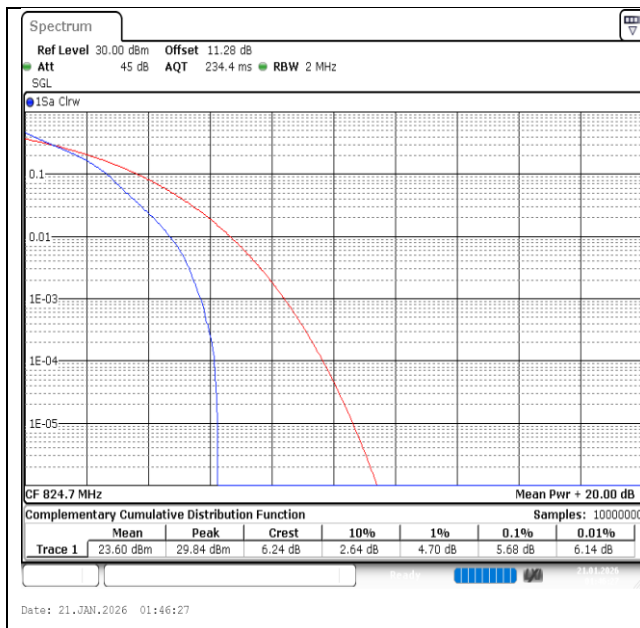
Band26(824-849)-1.4MHz-QPSK-26797-1RB#0-PASS
