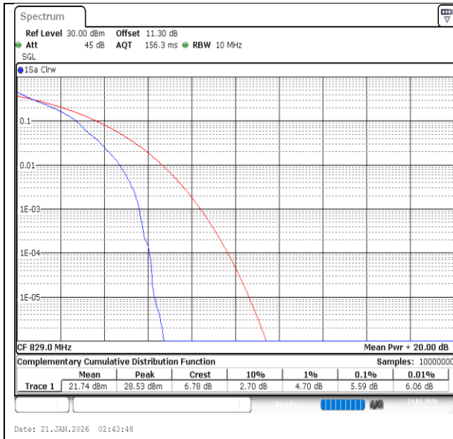
Band26(824-849)-10MHz-QPSK-26840-1RB#0-PASS
