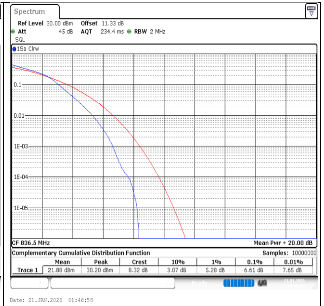
Band26(824-849)-1.4MHz-16QAM-26915-6RB#0-PASS
