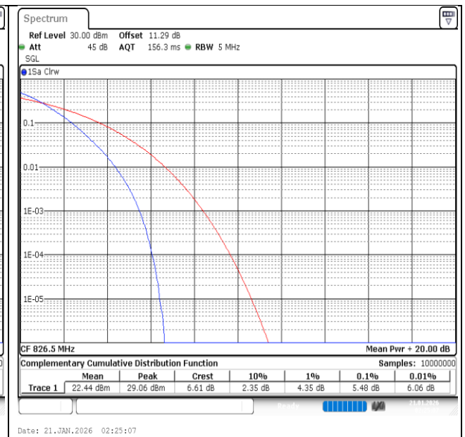
Band26(824-849)-5MHz-QPSK-26815-25RB#0-PASS
