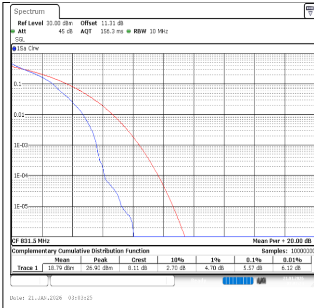
Band26(824-849)-15MHz-QPSK-26865-1RB#0-PASS
