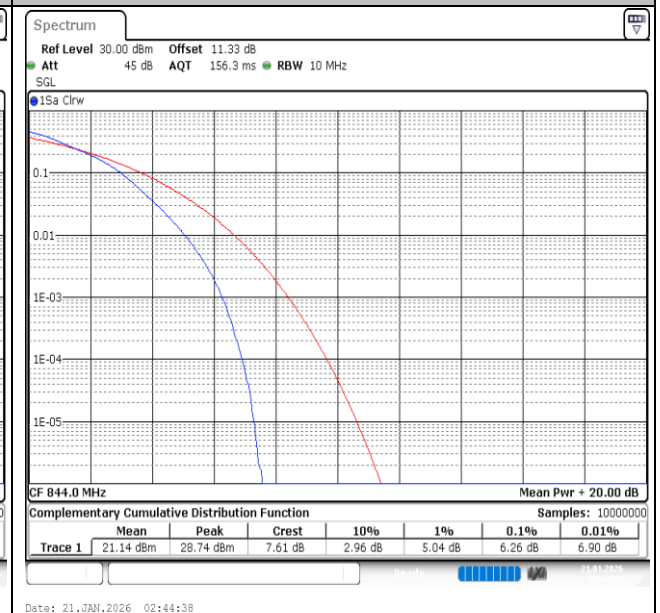
Band26(824-849)-10MHz-16QAM-26990-50RB#0-PASS
