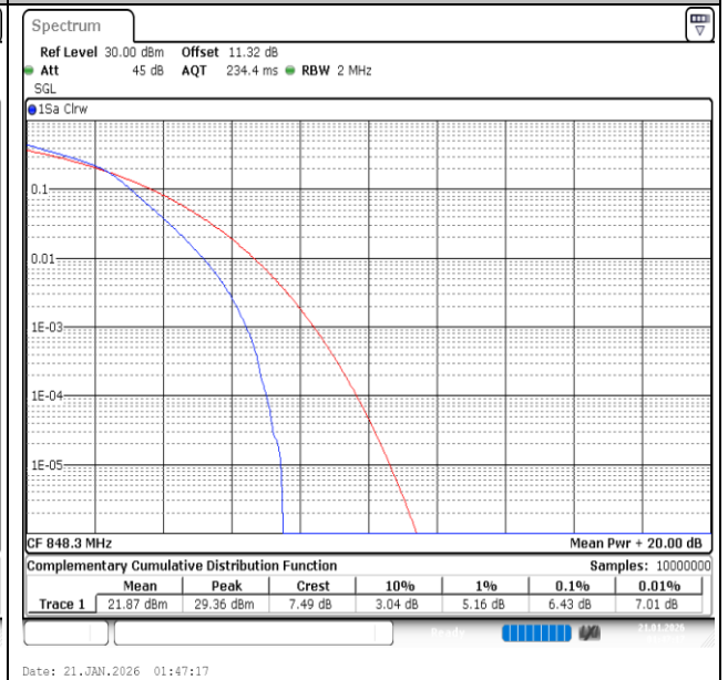
Band26(824-849)-1.4MHz-16QAM-27033-6RB#0-PASS
