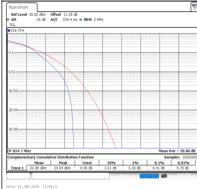
Band26(824-849)-1.4MHz-16QAM-26797-1RB#0-PASS
