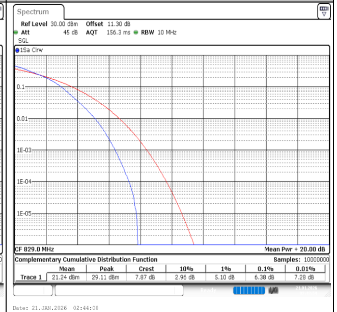
Band26(824-849)-10MHz-16QAM-26840-50RB#0-PASS
