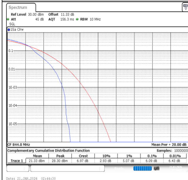
Band26(824-849)-10MHz-16QAM-26990-1RB#0-PASS
