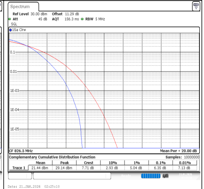
Band26(824-849)-5MHz-16QAM-26815-25RB#0-PASS
