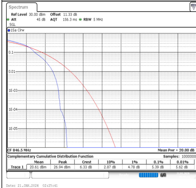
Band26(824-849)-5MHz-16QAM-27015-1RB#0-PASS
