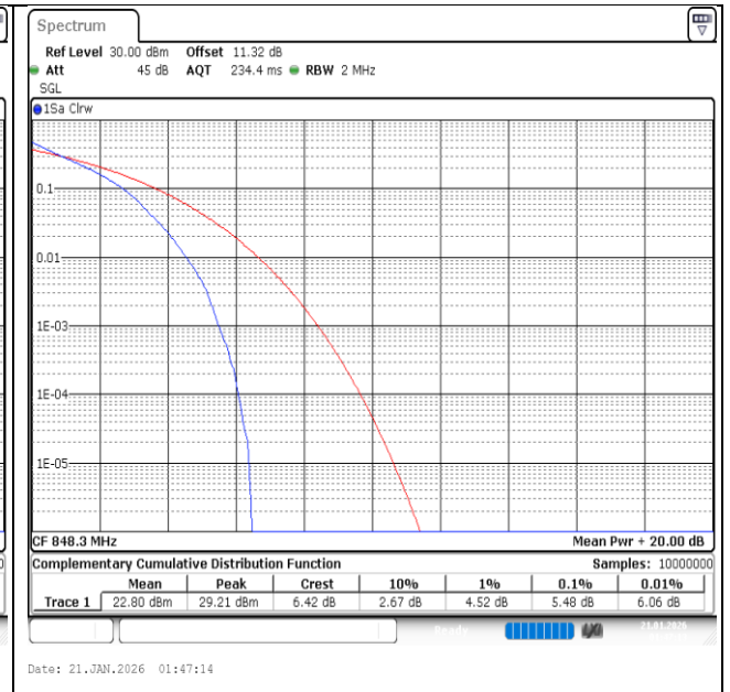
Band26(824-849)-1.4MHz-QPSK-27033-6RB#0-PASS
