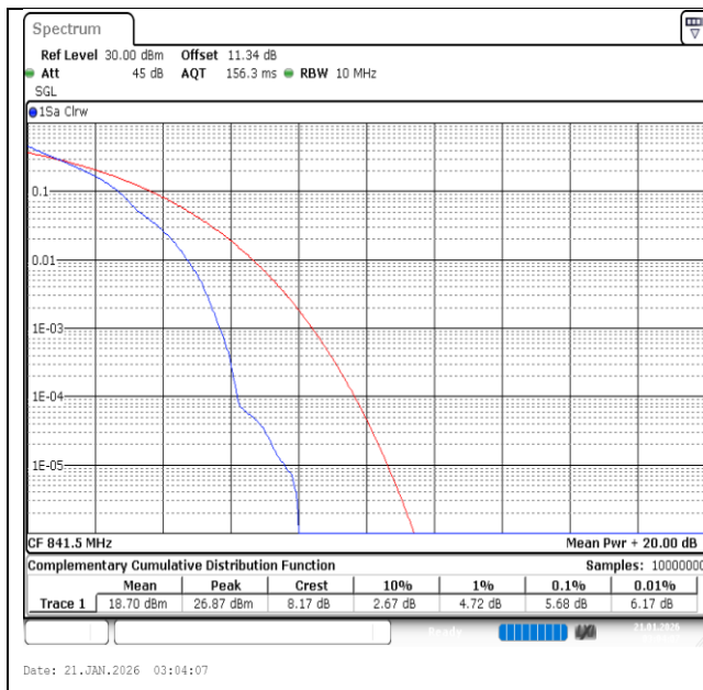
Band26(824-849)-15MHz-QPSK-26965-1RB#0-PASS
