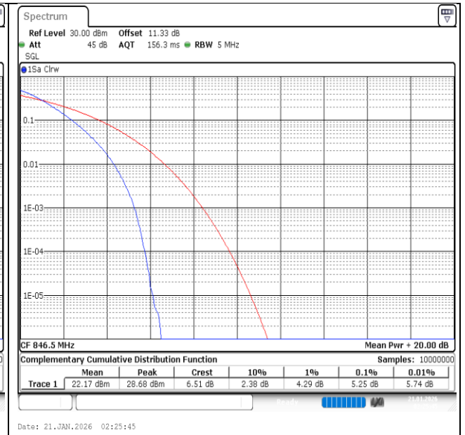
Band26(824-849)-5MHz-QPSK-27015-25RB#0-PASS
