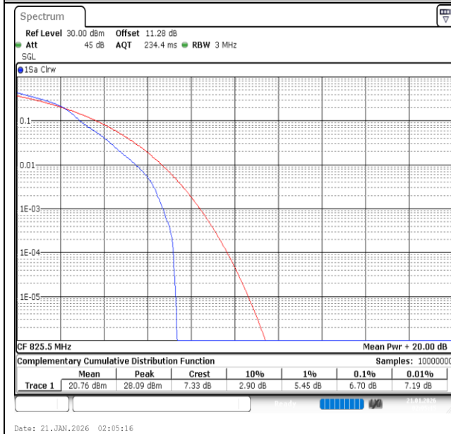
Band26(824-849)-3MHz-16QAM-26805-1RB#0-PASS
