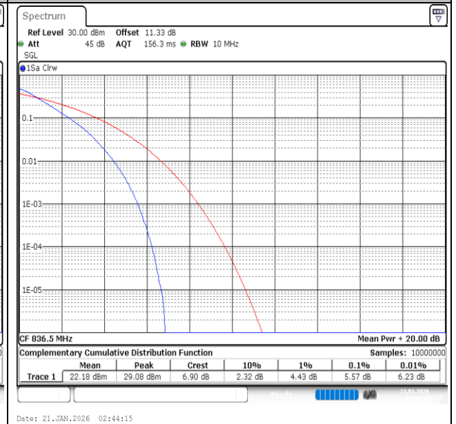
Band26(824-849)-10MHz-QPSK-26915-50RB#0-PASS
