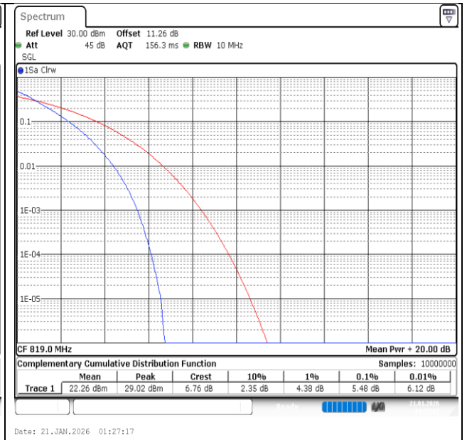
Band26(814-824)-10MHz-QPSK-26740-50RB#0-PASS
