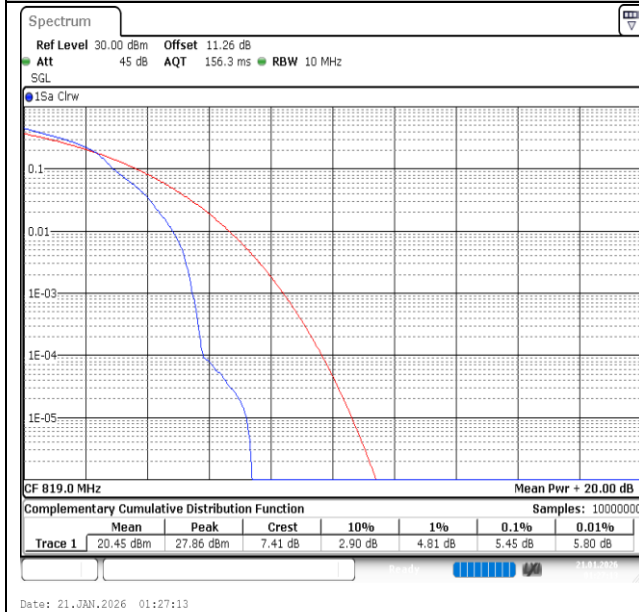
Band26(814-824)-10MHz-16QAM-26740-1RB#0-PASS
