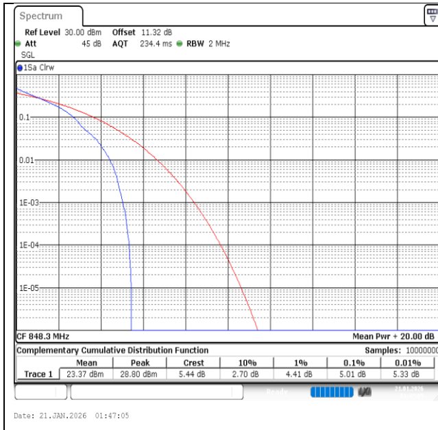
Band26(824-849)-1.4MHz-QPSK-27033-1RB#0-PASS
