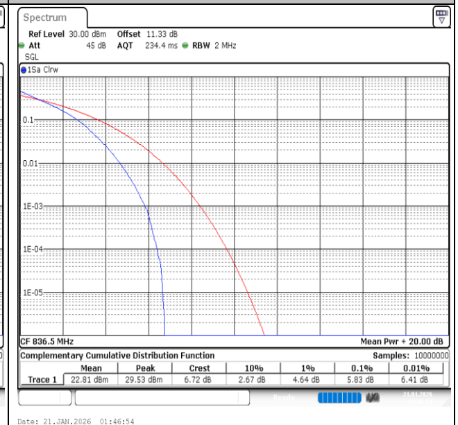
Band26(824-849)-1.4MHz-QPSK-26915-6RB#0-PASS
