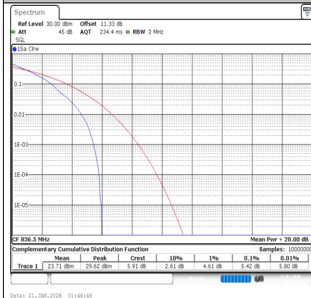
Band26(824-849)-1.4MHz-QPSK-26915-1RB#0-PASS
