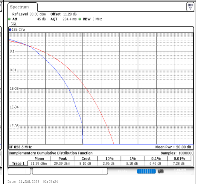
Band26(824-849)-3MHz-16QAM-26805-15RB#0-PASS
