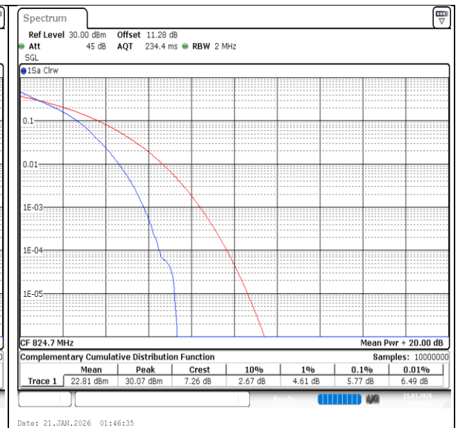
Band26(824-849)-1.4MHz-QPSK-26797-6RB#0-PASS
