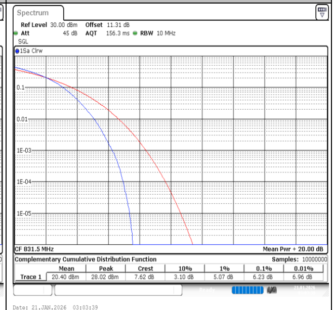
Band26(824-849)-15MHz-16QAM-26865-75RB#0-PASS
