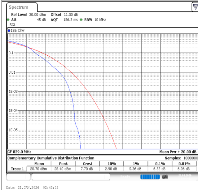
Band26(824-849)-10MHz-16QAM-26840-1RB#0-PASS
