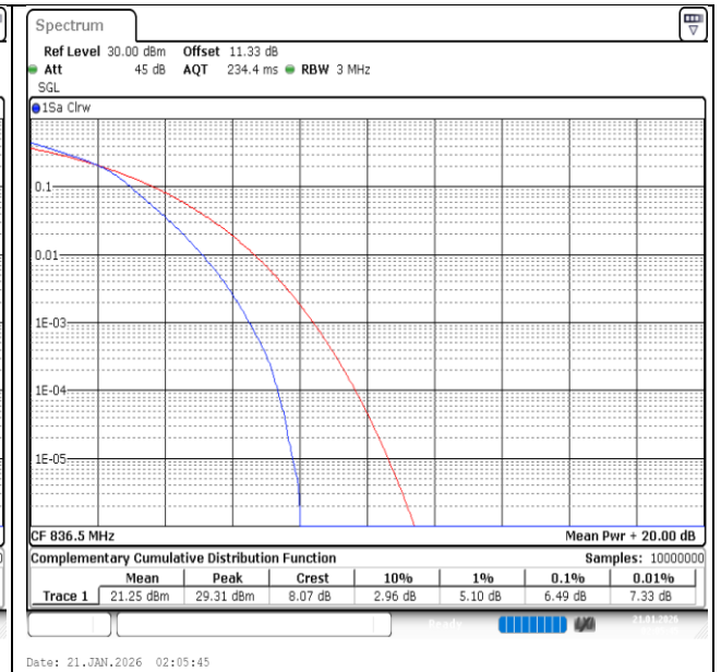
Band26(824-849)-3MHz-16QAM-26915-15RB#0-PASS
