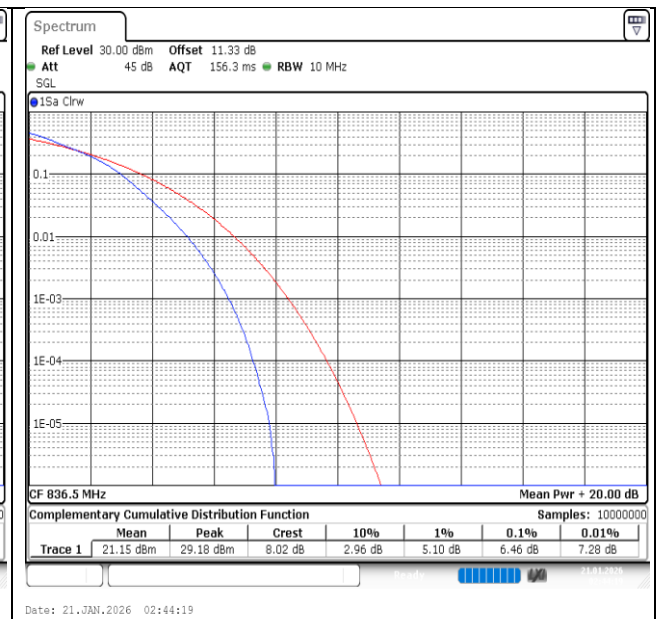
Band26(824-849)-10MHz-16QAM-26915-50RB#0-PASS
