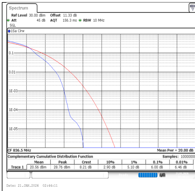
Band26(824-849)-10MHz-16QAM-26915-1RB#0-PASS
