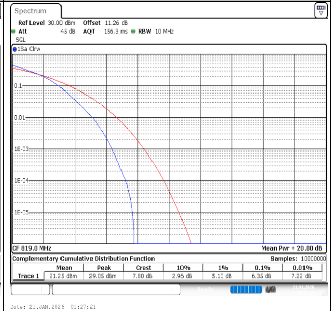
Band26(814-824)-10MHz-16QAM-26740-50RB#0-PASS
