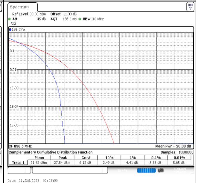
Band26(824-849)-15MHz-QPSK-26915-75RB#0-PASS
