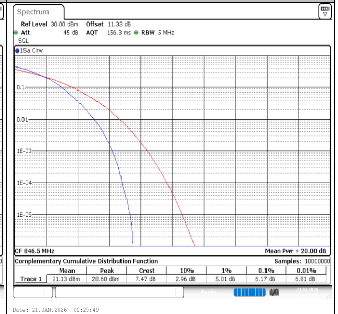
Band26(824-849)-5MHz-16QAM-27015-25RB#0-PASS
