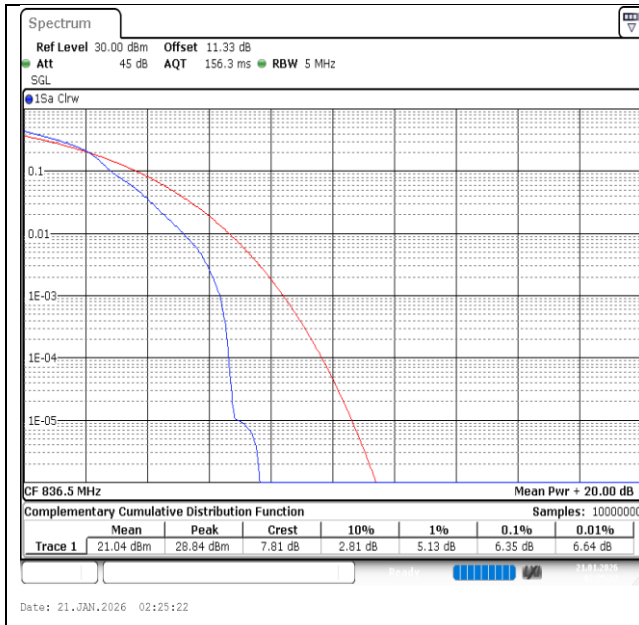
Band26(824-849)-5MHz-16QAM-26915-1RB#0-PASS
