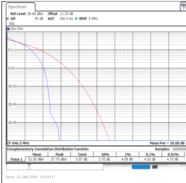
Band26(824-849)-5MHz-QPSK-27015-1RB#0-PASS
