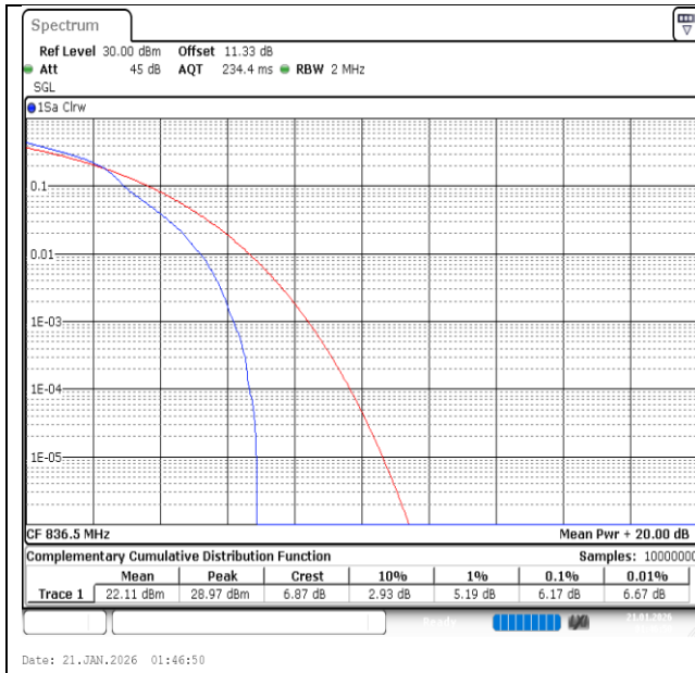
Band26(824-849)-1.4MHz-16QAM-26915-1RB#0-PASS
