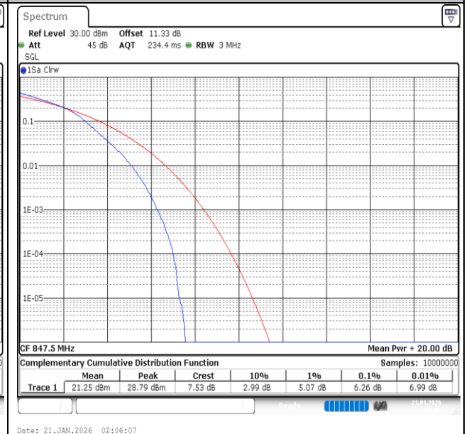
Band26(824-849)-3MHz-16QAM-27025-15RB#0-PASS
