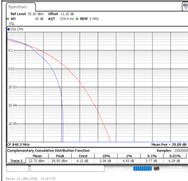
Band26(824-849)-1.4MHz-16QAM-27033-1RB#0-PASS
