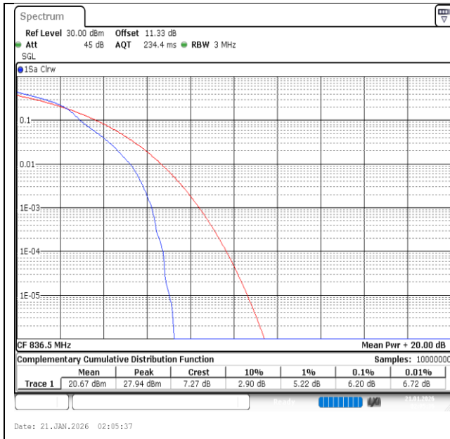
Band26(824-849)-3MHz-16QAM-26915-1RB#0-PASS
