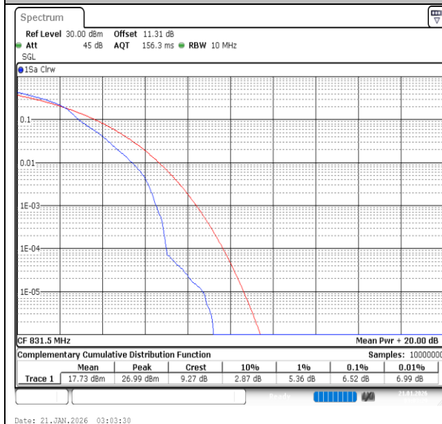
Band26(824-849)-15MHz-16QAM-26865-1RB#0-PASS
