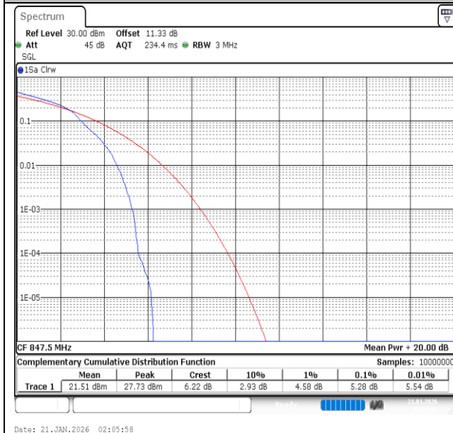
Band26(824-849)-3MHz-16QAM-27025-1RB#0-PASS
