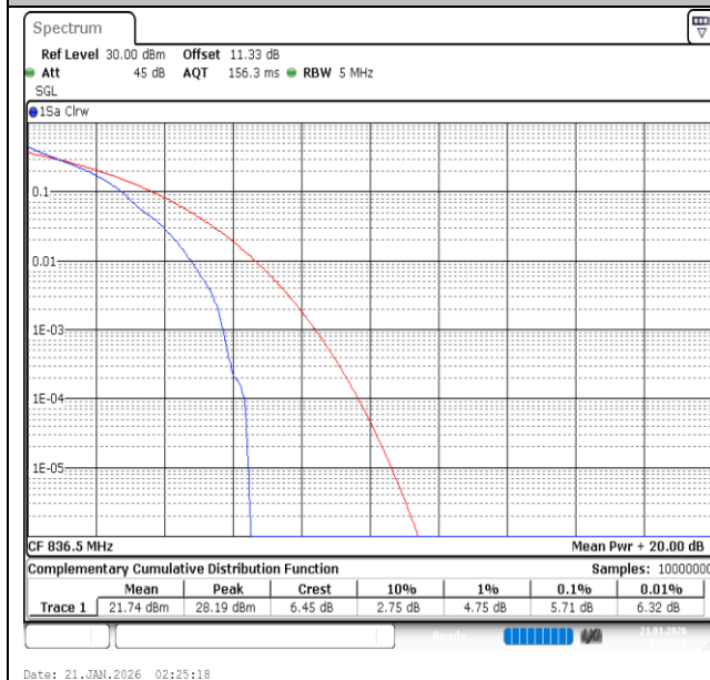
Band26(824-849)-5MHz-QPSK-26915-1RB#0-PASS
