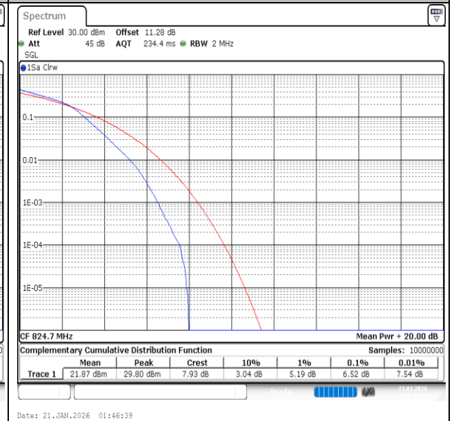
Band26(824-849)-1.4MHz-16QAM-26797-6RB#0-PASS
