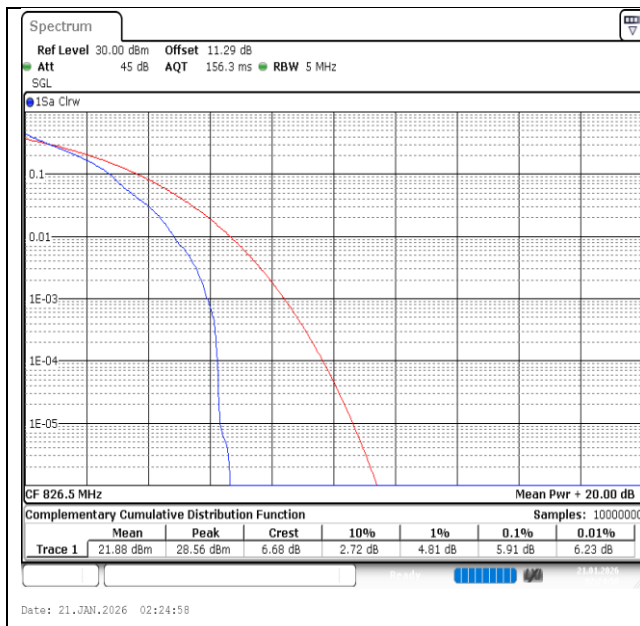
Band26(824-849)-5MHz-QPSK-26815-1RB#0-PASS
