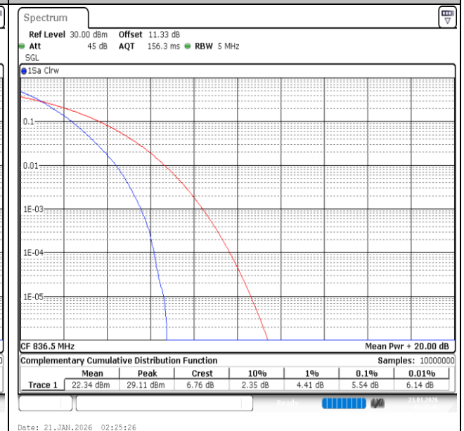
Band26(824-849)-5MHz-QPSK-26915-25RB#0-PASS
