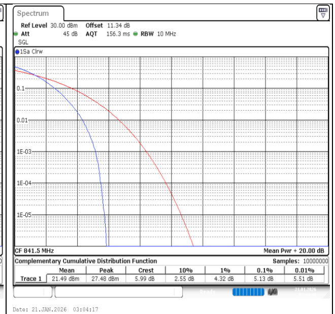
Band26(824-849)-15MHz-QPSK-26965-75RB#0-PASS
