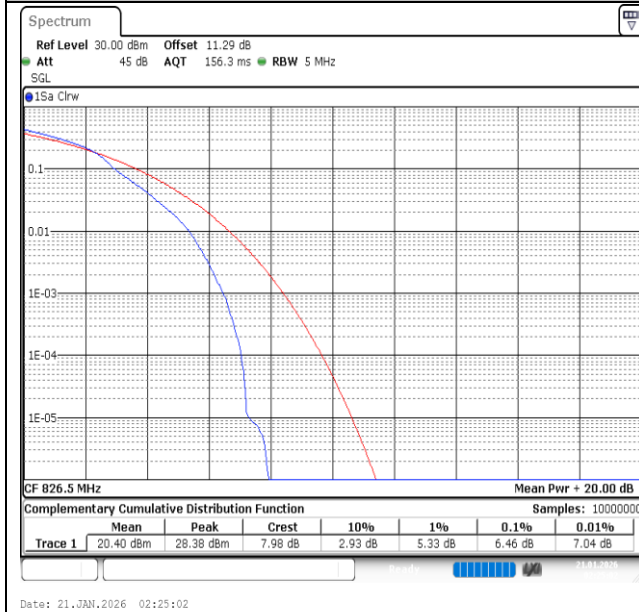
Band26(824-849)-5MHz-16QAM-26815-1RB#0-PASS
