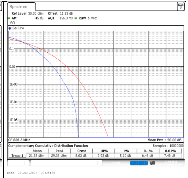
Band26(824-849)-5MHz-16QAM-26915-25RB#0-PASS
