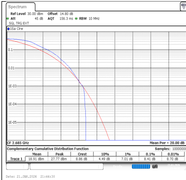
Band41-10MHz-QPSK-41540-1RB#0-PASS
