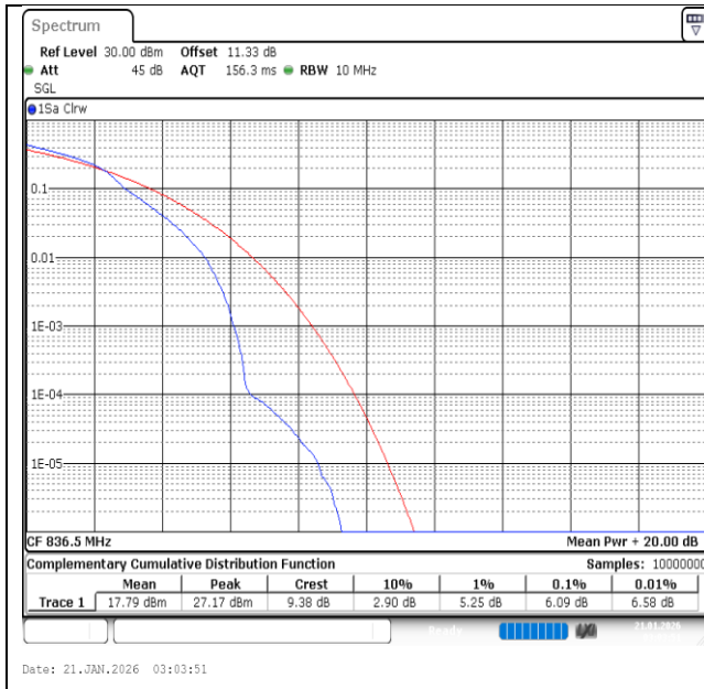
Band26(824-849)-15MHz-16QAM-26915-1RB#0-PASS
