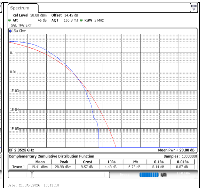
Band40(2350-2360)-5MHz-QPSK-39175-25RB#0-PASS
