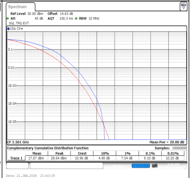
Band41-10MHz-16QAM-39700-50RB#0-PASS
