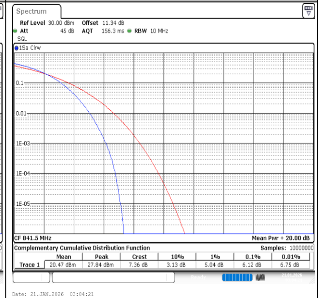
Band26(824-849)-15MHz-16QAM-26965-75RB#0-PASS
