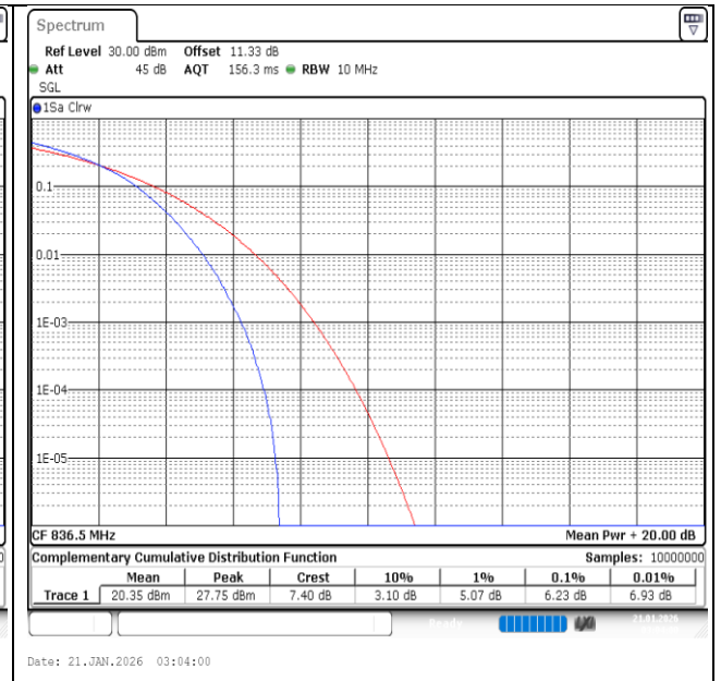
Band26(824-849)-15MHz-16QAM-26915-75RB#0-PASS
