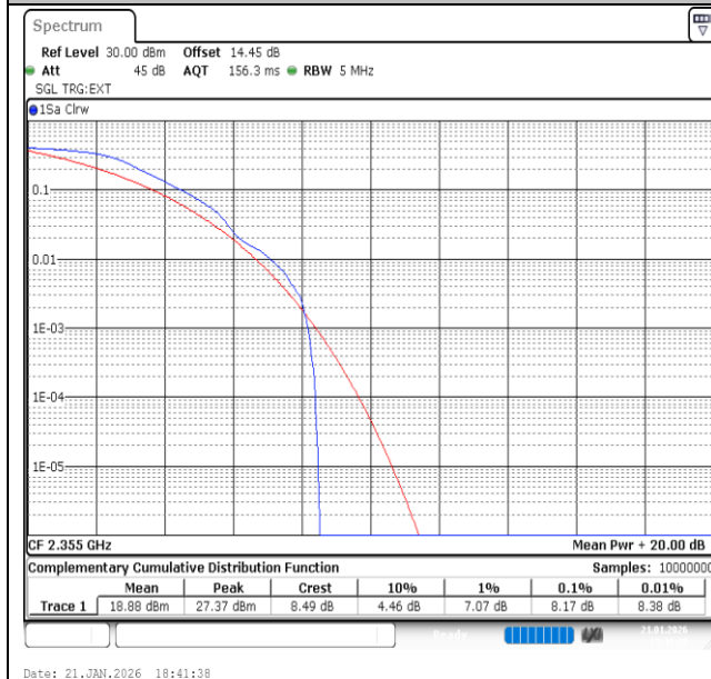
Band40(2350-2360)-5MHz-QPSK-39200-1RB#0-PASS
