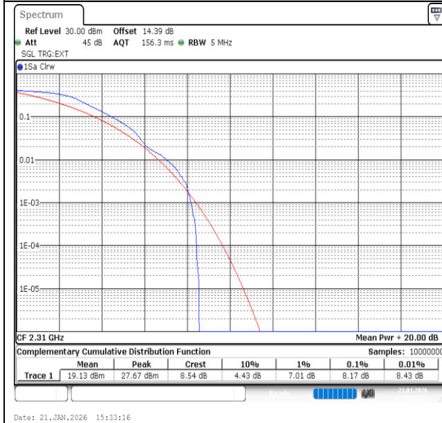
Band40(2305-2315)-5MHz-QPSK-38750-1RB#0-PASS
