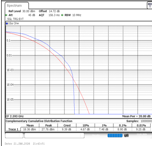
Band41-10MHz-QPSK-40620-1RB#0-PASS
