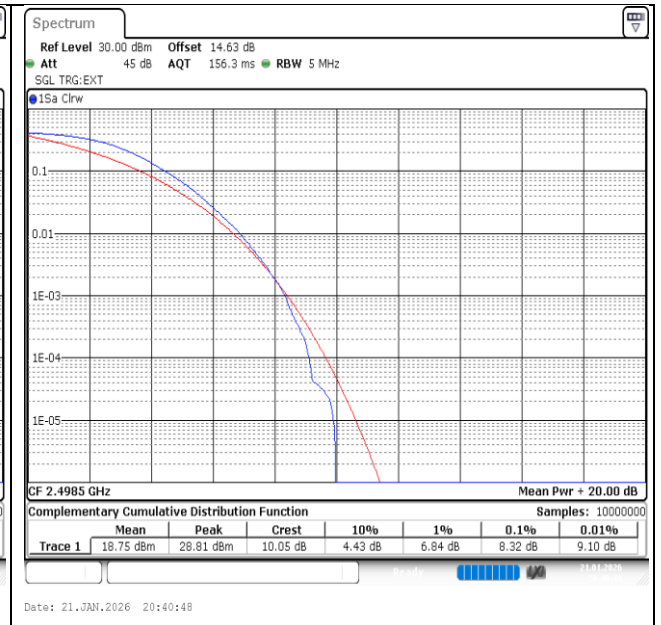
Band41-5MHz-QPSK-39675-25RB#0-PASS
