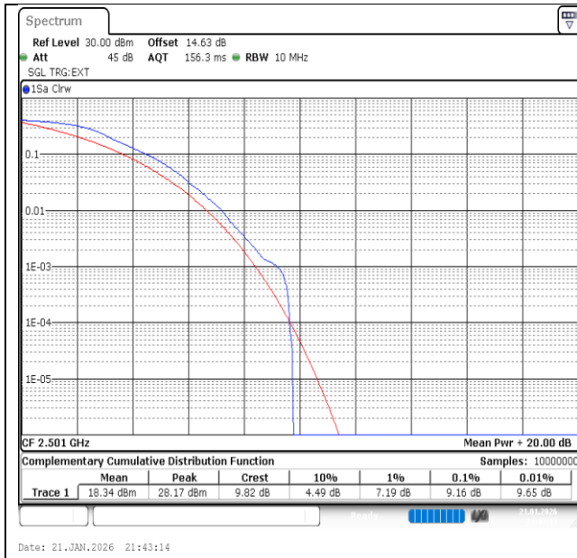
Band41-10MHz-QPSK-39700-1RB#0-PASS
