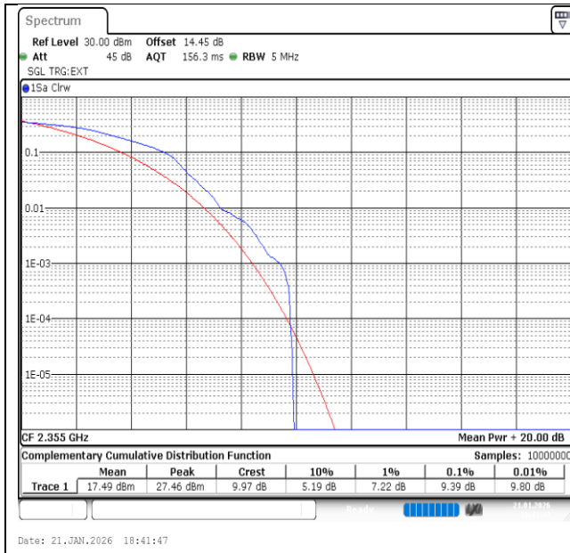
Band40(2350-2360)-5MHz-16QAM-39200-1RB#0-PASS
