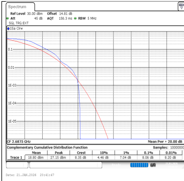
Band41-5MHz-QPSK-41565-1RB#0-PASS
