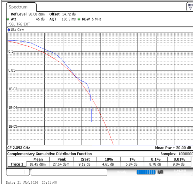
Band41-5MHz-QPSK-40620-1RB#0-PASS
