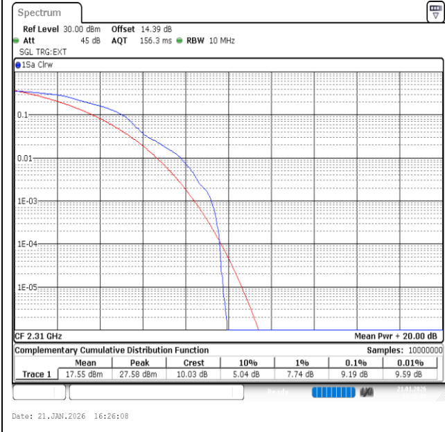
Band40(2305-2315)-10MHz-16QAM-38750-1RB#0-PASS
