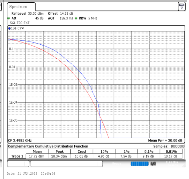
Band41-5MHz-16QAM-39675-25RB#0-PASS
