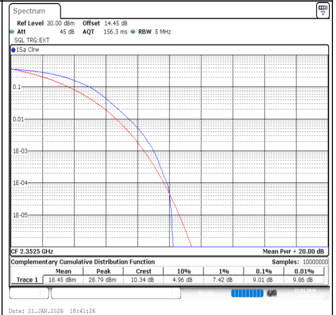
Band40(2350-2360)-5MHz-16QAM-39175-25RB#0-PASS
