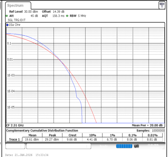
Band40(2305-2315)-5MHz-QPSK-38750-25RB#0-PASS
