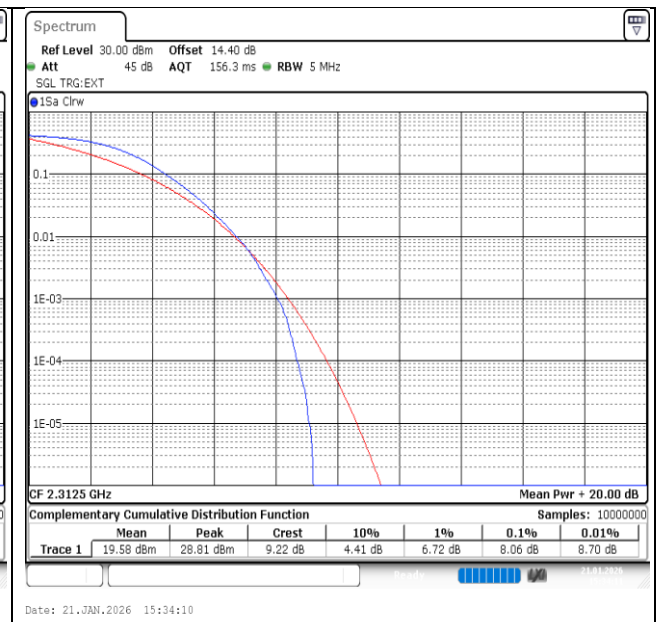
Band40(2305-2315)-5MHz-QPSK-38775-25RB#0-PASS
