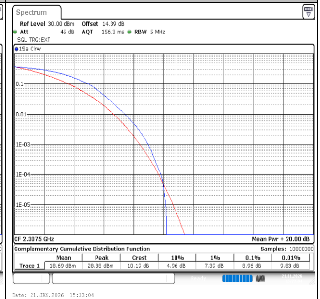
Band40(2305-2315)-5MHz-16QAM-38725-25RB#0-PASS
