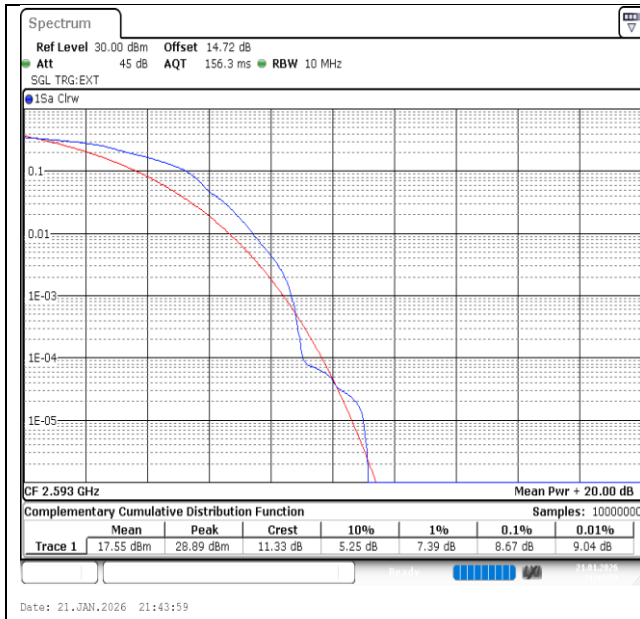
Band41-10MHz-16QAM-40620-1RB#0-PASS
