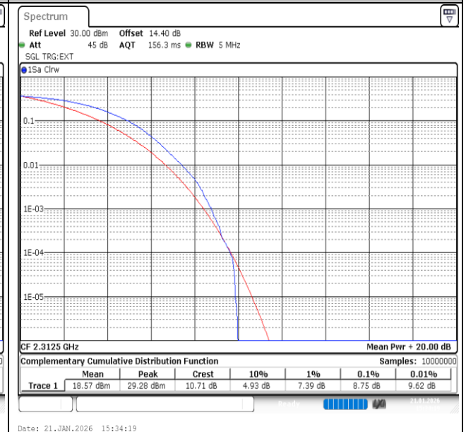
Band40(2305-2315)-5MHz-16QAM-38775-25RB#0-PASS
