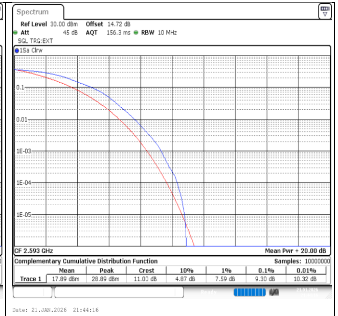
Band41-10MHz-16QAM-40620-50RB#0-PASS
