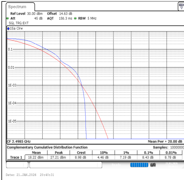
Band41-5MHz-QPSK-39675-1RB#0-PASS
