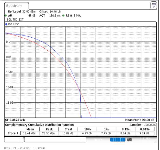
Band40(2350-2360)-5MHz-16QAM-39225-25RB#0-PASS
