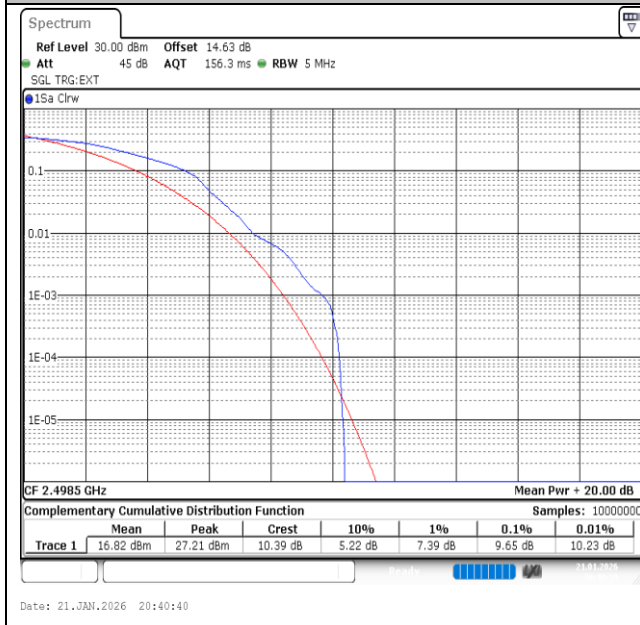
Band41-5MHz-16QAM-39675-1RB#0-PASS
