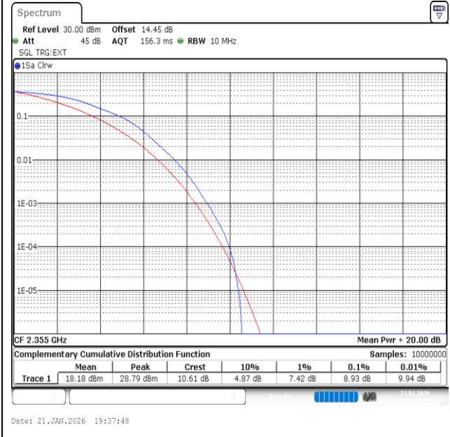
Band40(2350-2360)-10MHz-16QAM-39200-50RB#0-PAS
