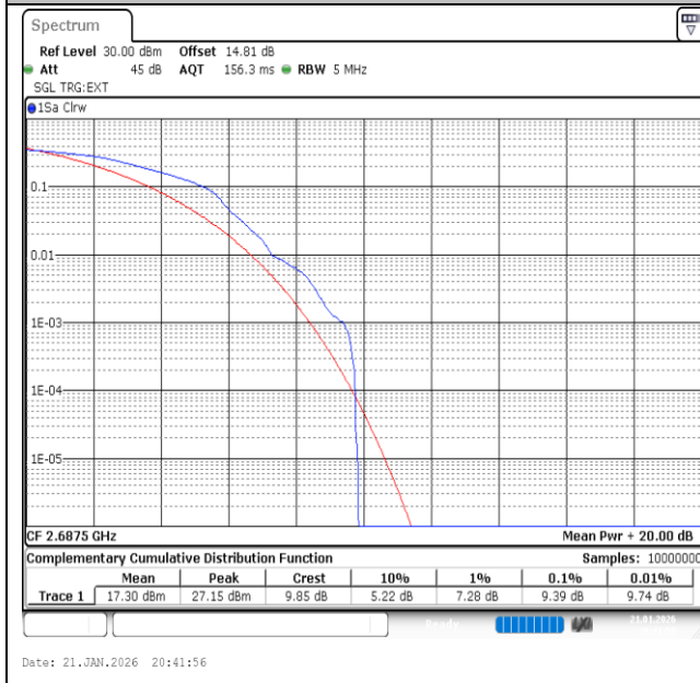
Band41-5MHz-16QAM-41565-1RB#0-PASS
