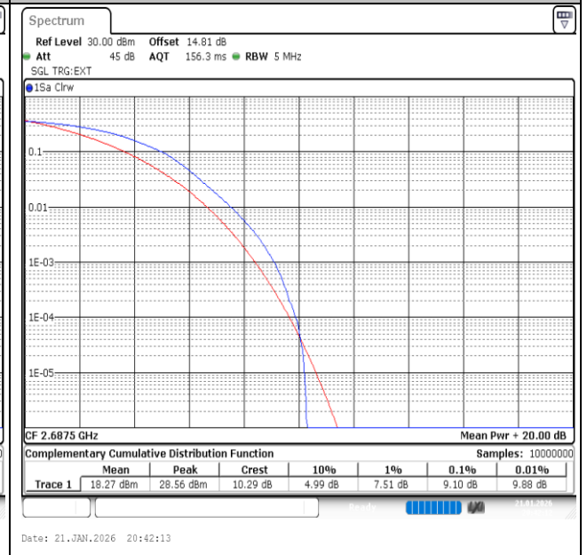
Band41-5MHz-16QAM-41565-25RB#0-PASS
