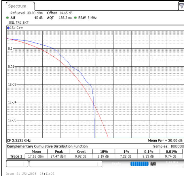
Band40(2350-2360)-5MHz-16QAM-39175-1RB#0-PASS
