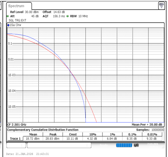
Band41-10MHz-QPSK-39700-50RB#0-PASS
