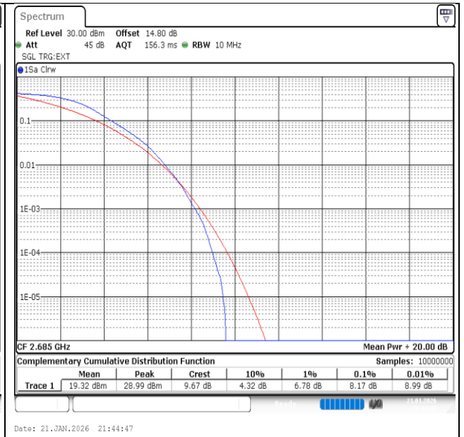
Band41-10MHz-QPSK-41540-50RB#0-PASS
