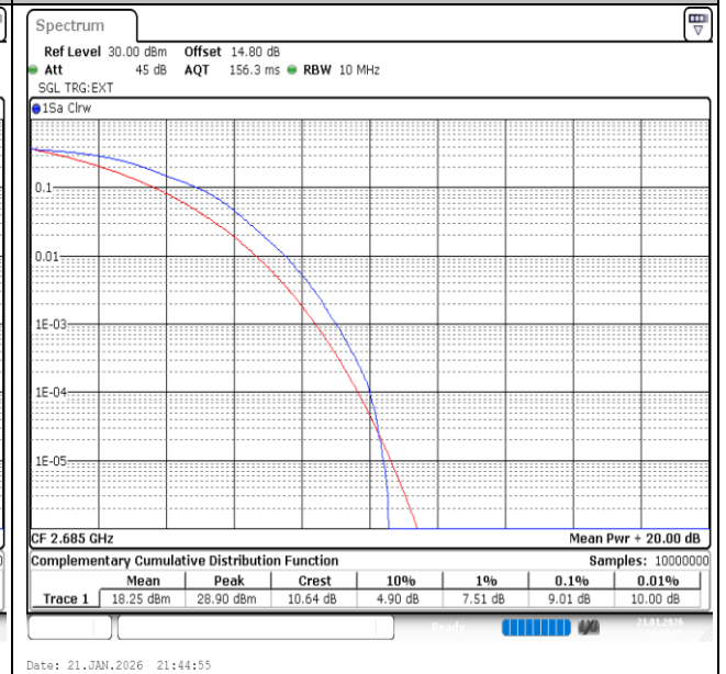
Band41-10MHz-16QAM-41540-50RB#0-PASS
