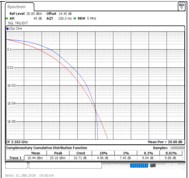
Band40(2350-2360)-5MHz-16QAM-39200-25RB#0-PASS
