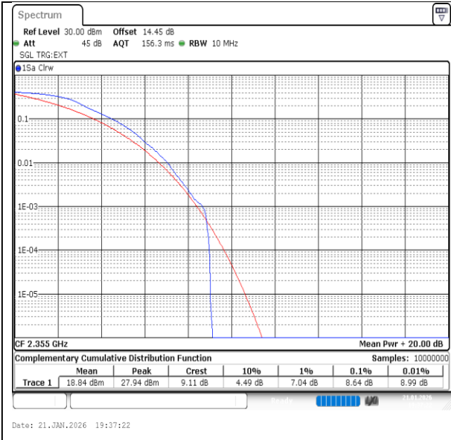
Band40(2350-2360)-10MHz-QPSK-39200-1RB#0-PASS
