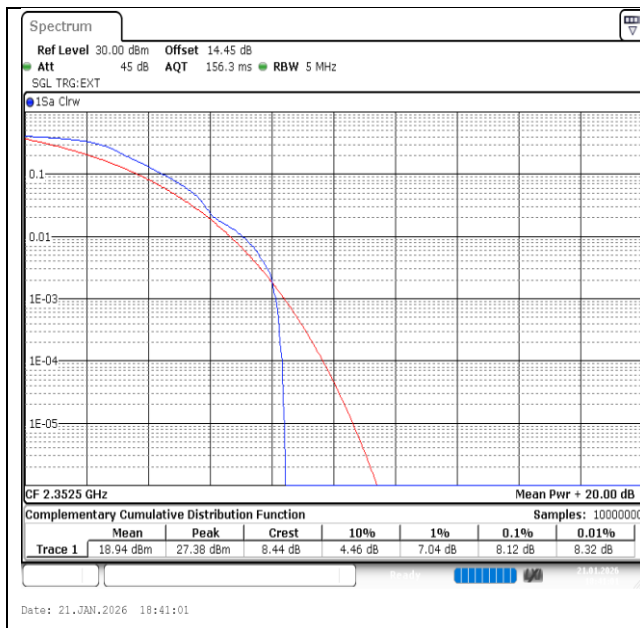
Band40(2350-2360)-5MHz-QPSK-39175-1RB#0-PASS
