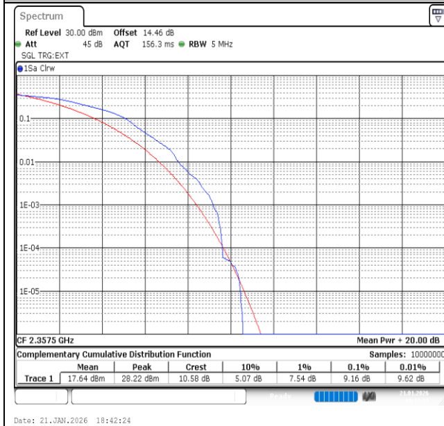
Band40(2350-2360)-5MHz-16QAM-39225-1RB#0-PASS
