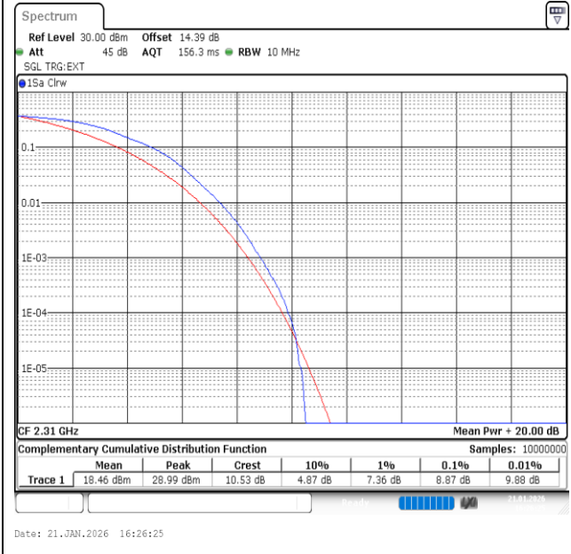
Band40(2305-2315)-10MHz-16QAM-38750-50RB#0-PAS
