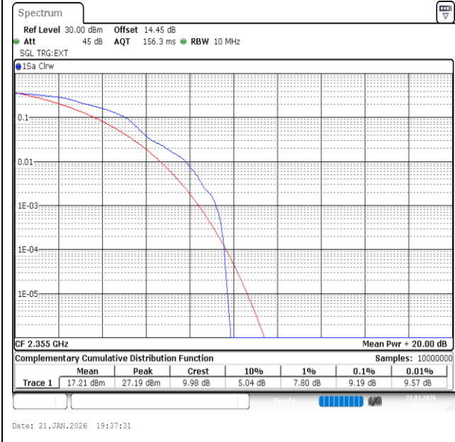
Band40(2350-2360)-10MHz-16QAM-39200-1RB#0-PASS
