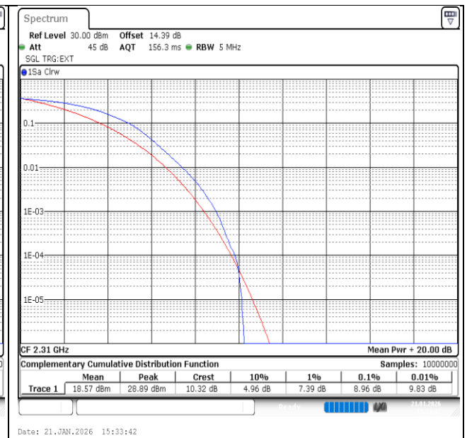
Band40(2305-2315)-5MHz-16QAM-38750-25RB#0-PASS
