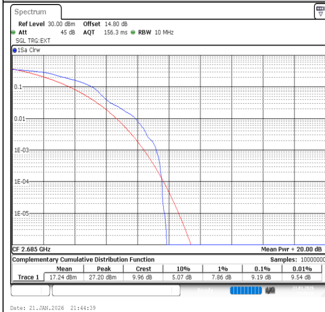
Band41-10MHz-16QAM-41540-1RB#0-PASS
