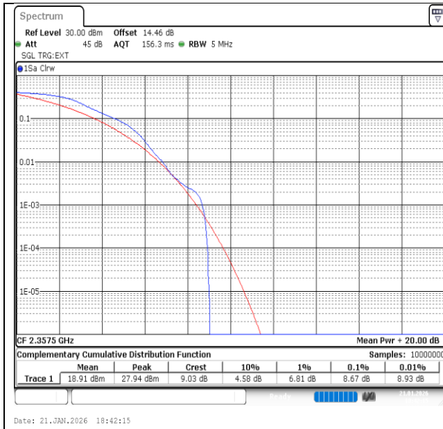
Band40(2350-2360)-5MHz-QPSK-39225-1RB#0-PASS
