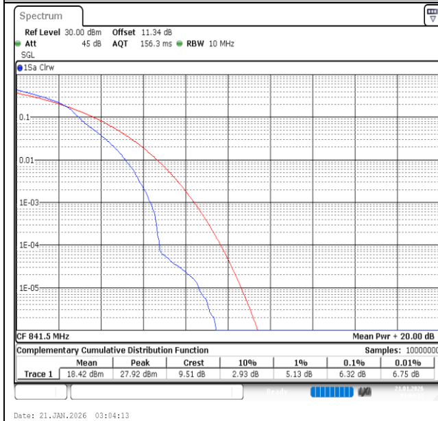
Band26(824-849)-15MHz-16QAM-26965-1RB#0-PASS
