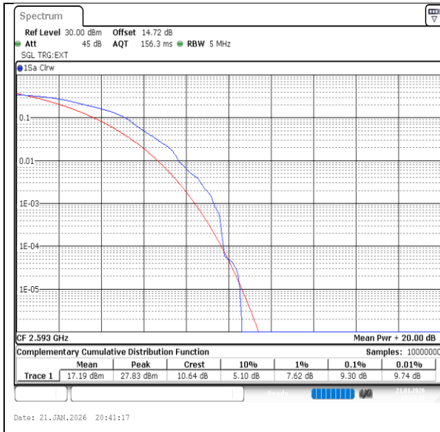
Band41-5MHz-16QAM-40620-1RB#0-PASS
