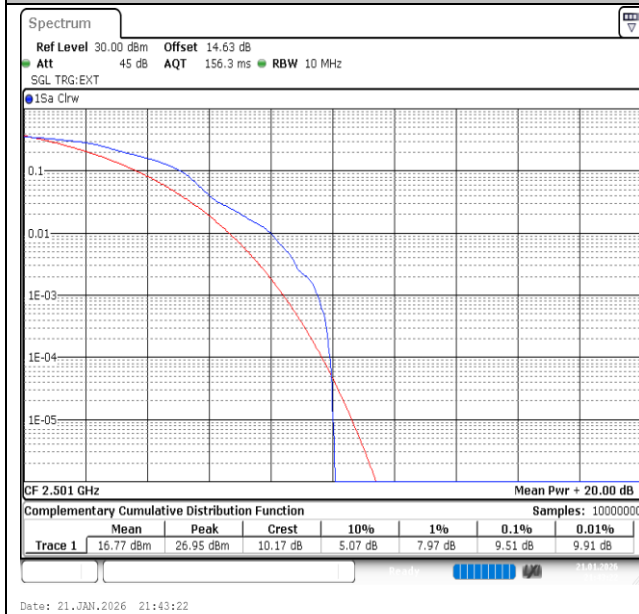
Band41-10MHz-16QAM-39700-1RB#0-PASS
