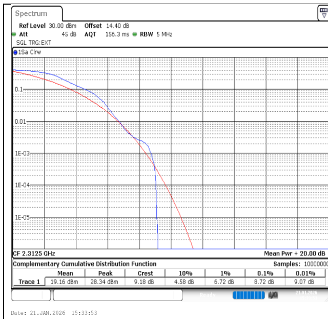
Band40(2305-2315)-5MHz-QPSK-38775-1RB#0-PASS
