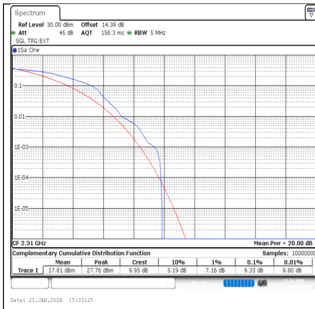
Band40(2305-2315)-5MHz-16QAM-38750-1RB#0-PASS
