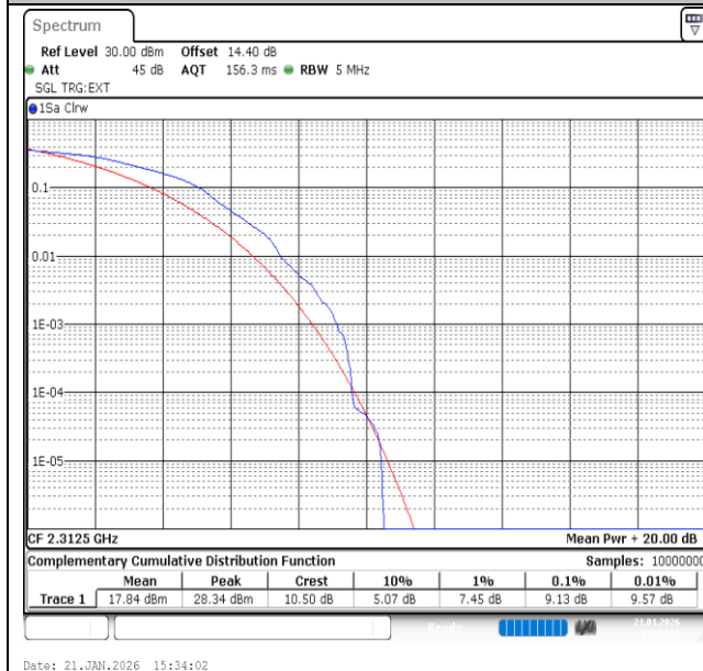
Band40(2305-2315)-5MHz-16QAM-38775-1RB#0-PASS
