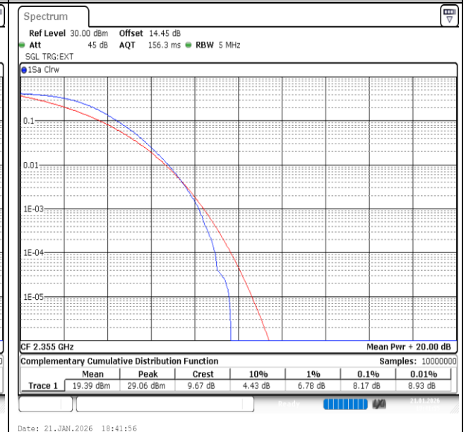
Band40(2350-2360)-5MHz-QPSK-39200-25RB#0-PASS
