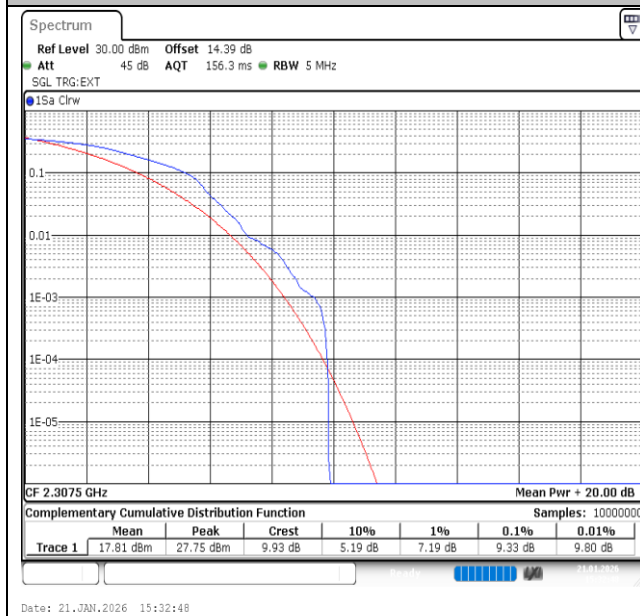
Band40(2305-2315)-5MHz-16QAM-38725-1RB#0-PASS
