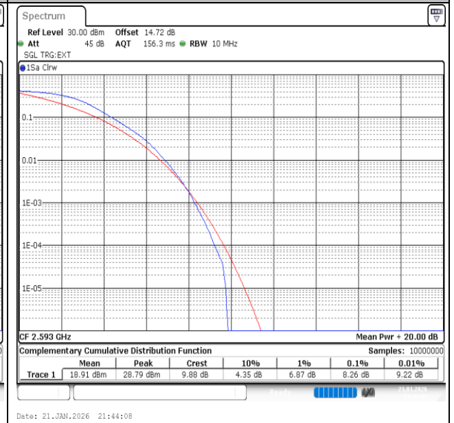
Band41-10MHz-QPSK-40620-50RB#0-PASS
