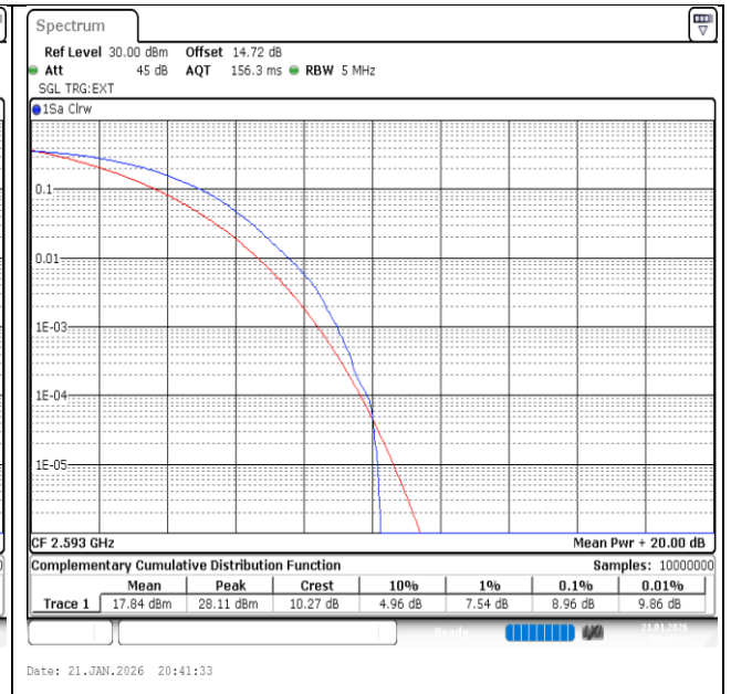
Band41-5MHz-16QAM-40620-25RB#0-PASS
