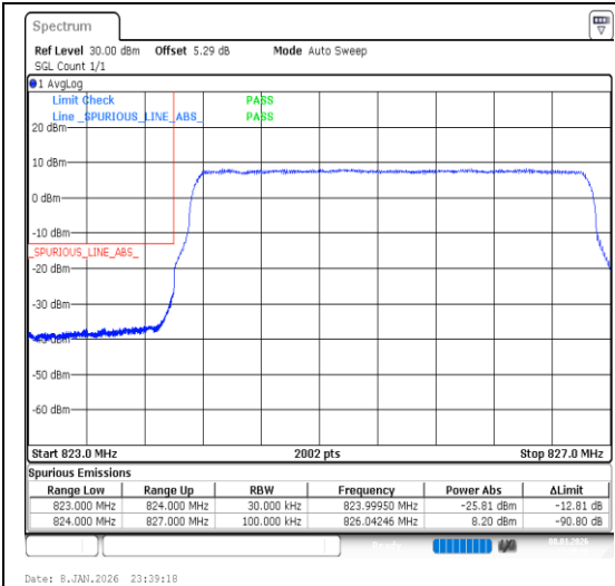
Band26(824-849)-3MHz-16QAM-26805-15RB#0-P ASS
