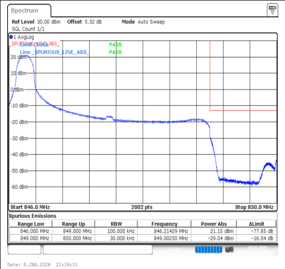
Band26(824-849)-3MHz-QPSK-27025-1RB#0-PA SS
