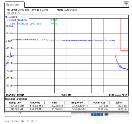
Band26(824-849)-15MHz-QPSK-26965-75RB#0-P ASS
