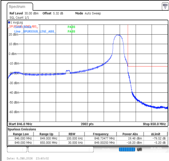
Band26(824-849)-3MHz-16QAM-27025-1RB#14-P ASS
