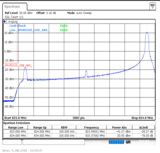
Band26(824-849)-10MHz-QPSK-26840-1RB#49-P
