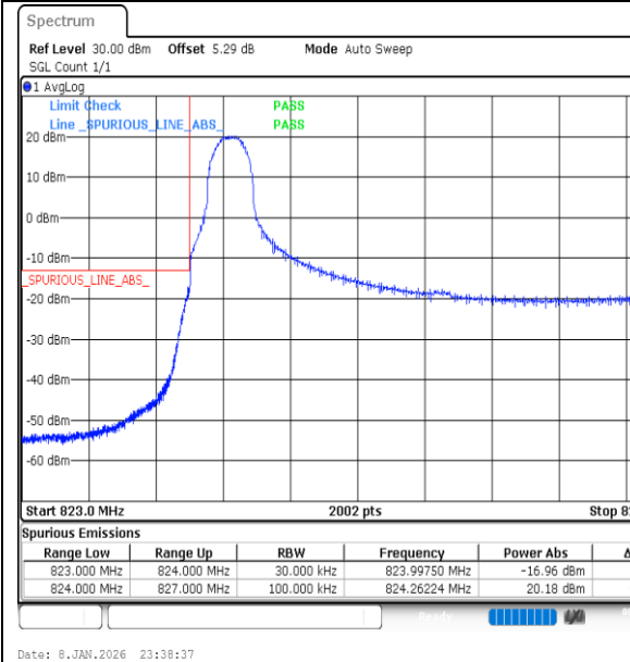
Band26(824-849)-3MHz-16QAM-26805-1RB#0-PA SS
