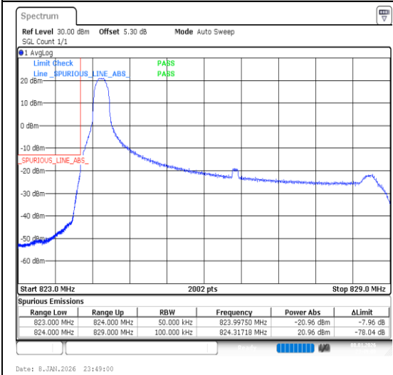
Band26(824-849)-5MHz-QPSK-26815-1RB#0-PA SS
