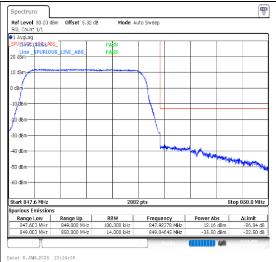
Band26(824-849)-1.4MHz-16QAM-27033-6RB#0 -PASS
