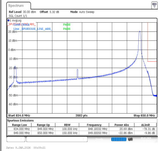
Band26(824-849)-15MHz-QPSK-26965-1RB#74-P ASS
