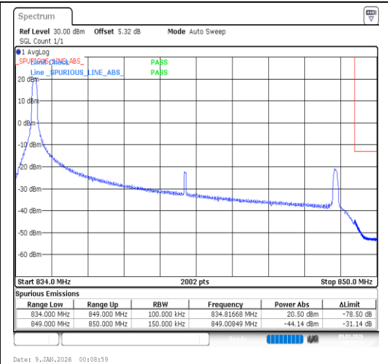
Band26(824-849)-15MHz-QPSK-26965-1RB#0-P ASS
