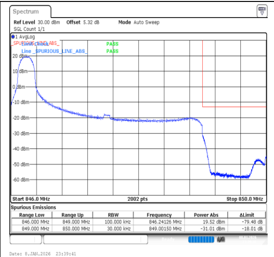
Band26(824-849)-3MHz-16QAM-27025-1RB#0-P ASS
