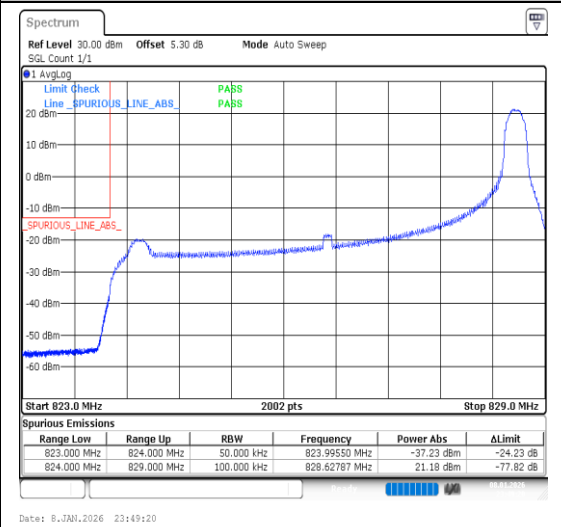
Band26(824-849)-5MHz-QPSK-26815-1RB#24-P ASS
