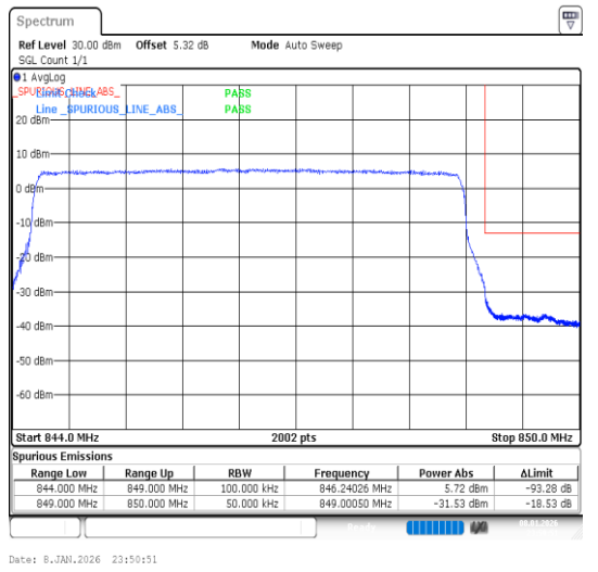
Band26(824-849)-5MHz-16QAM-27015-25RB#0-P
