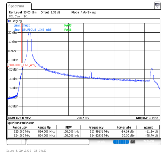
Band26(824-849)-10MHz-16QAM-26840-1RB#0-P ASS
