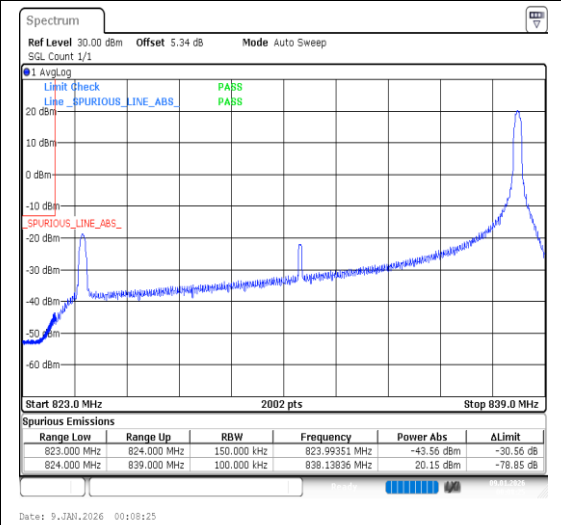
Band26(824-849)-15MHz-16QAM-26865-1RB#74-P PASS
