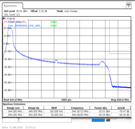
Band26(824-849)-5MHz-16QAM-27015-1RB#0-P
