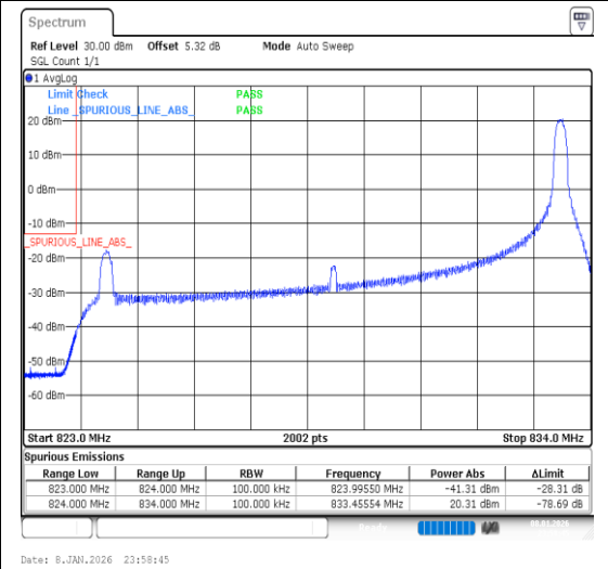
Band26(824-849)-10MHz-16QAM-26840-1RB#49-P PASS
