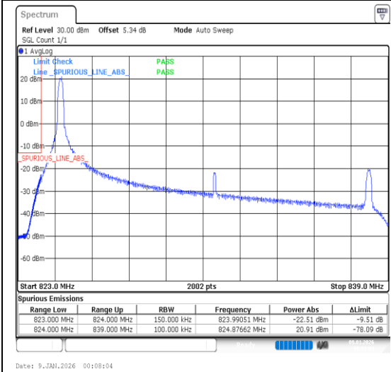
Band26(824-849)-15MHz-16QAM-26865-1RB#0-P ASS
