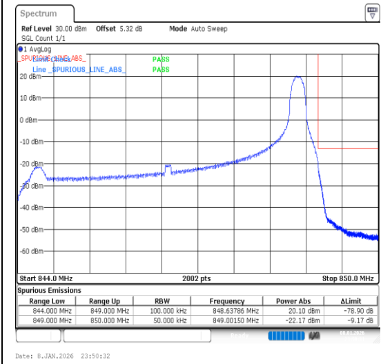
Band26(824-849)-5MHz-16QAM-27015-1RB#24-P
