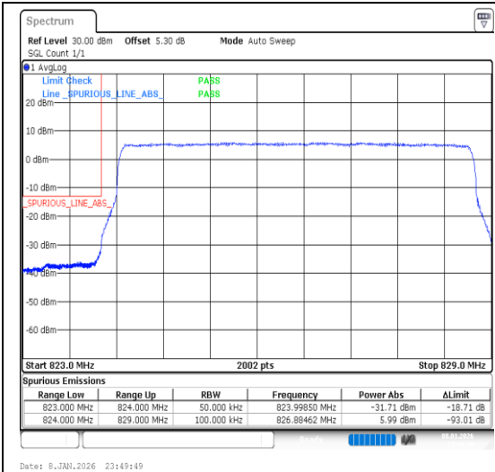
Band26(824-849)-5MHz-16QAM-26815-25RB#0-P
