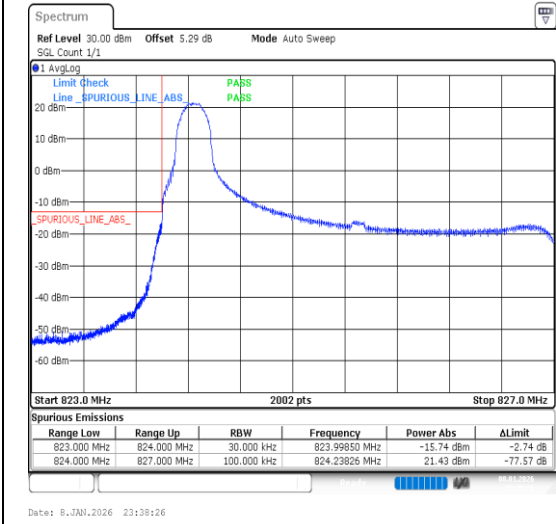
Band26(824-849)-3MHz-QPSK-26805-1RB#0-PAS S
