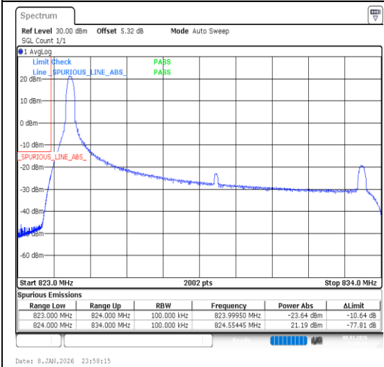
Band26(824-849)-10MHz-QPSK-26840-1RB#0-P
