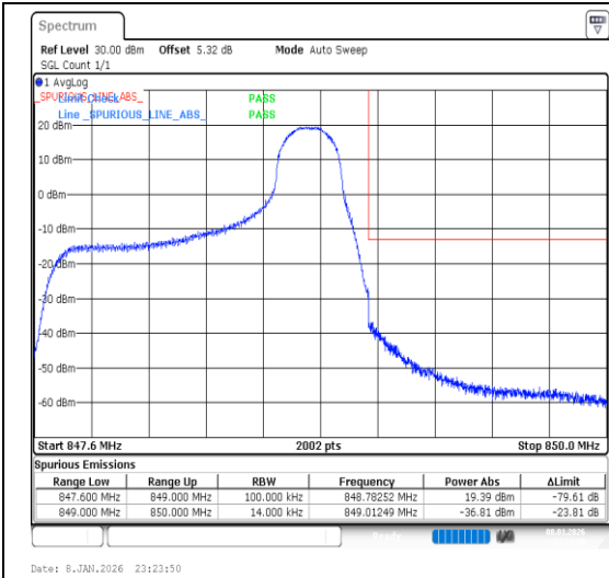
Band26(824-849)-1.4MHz-16QAM-27033-1RB#5-P ASS
