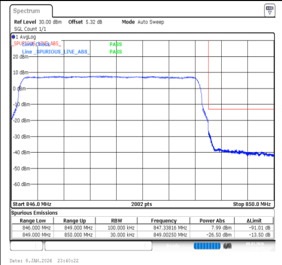
Band26(824-849)-3MHz-16QAM-27025-15RB#0-P ASS
