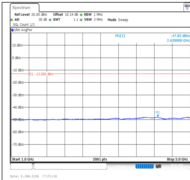
Band12-5MHz-16QAM-23035-25RB#0-1000~3000-PASS
