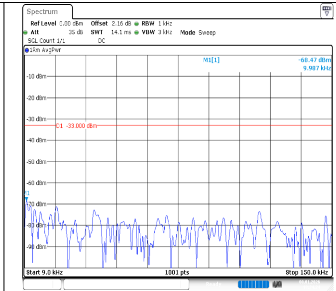
Band12-10MHz-QPSK-23095-50RB#0-0.009~0.15-PASS
