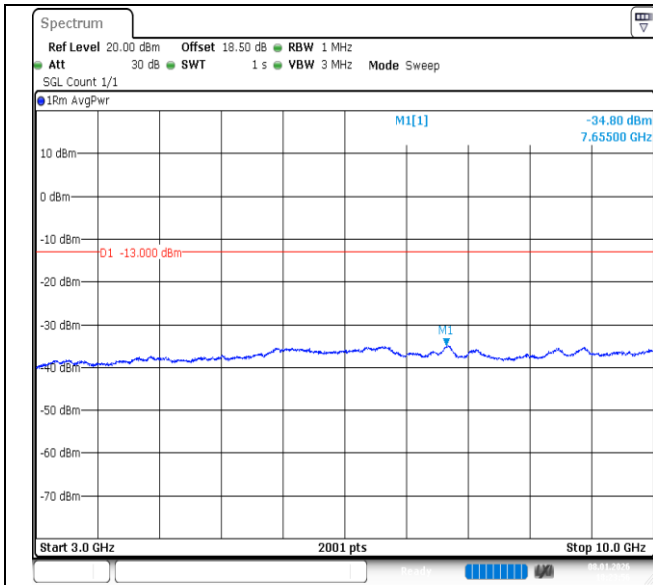
Band12-10MHz-QPSK-23095-1RB#49-3000~10000-PASS
