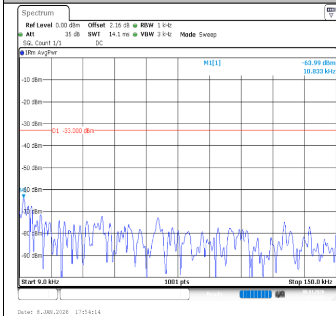
Band12-5MHz-16QAM-23095-1RB#0-0.009~0.15-PASS
