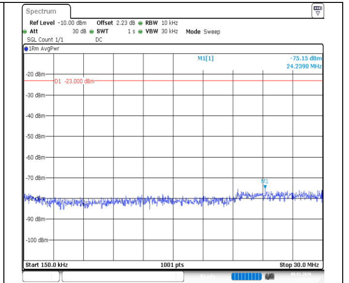
Band12-10MHz-QPSK-23095-1RB#49-0.15~30-PASS
