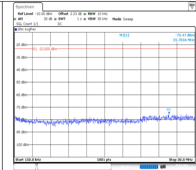
Band12-5MHz-16QAM-23095-25RB#0-0.15~30-PASS
