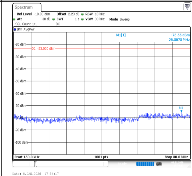
Band12-5MHz-16QAM-23095-1RB#0-0.15~30-PASS
