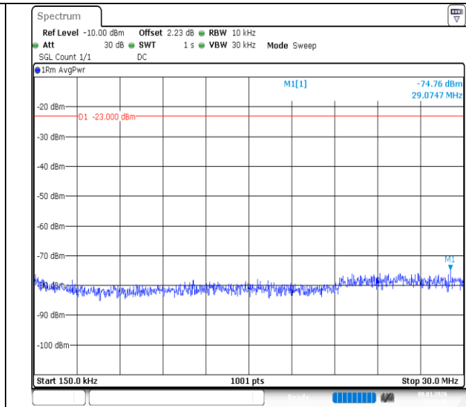
Band12-10MHz-QPSK-23060-1RB#0-0.15~30-PASS
