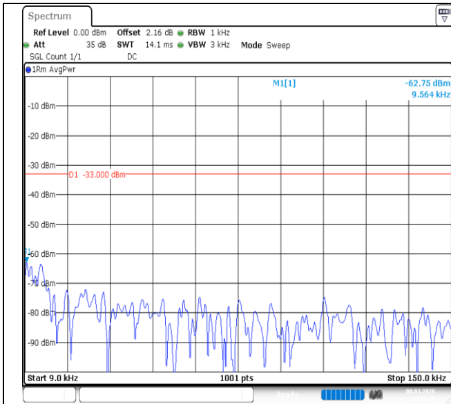
Band12-5MHz-16QAM-23035-1RB#24-0.009~0.15-PASS
