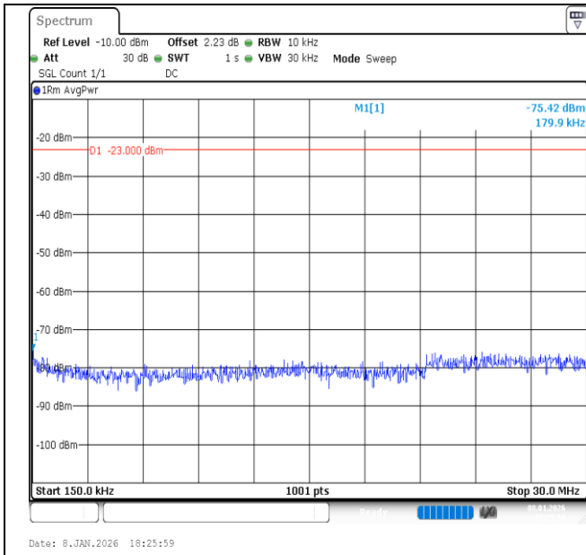
Band12-10MHz-QPSK-23130-1RB#49-0.15~30-PASS
