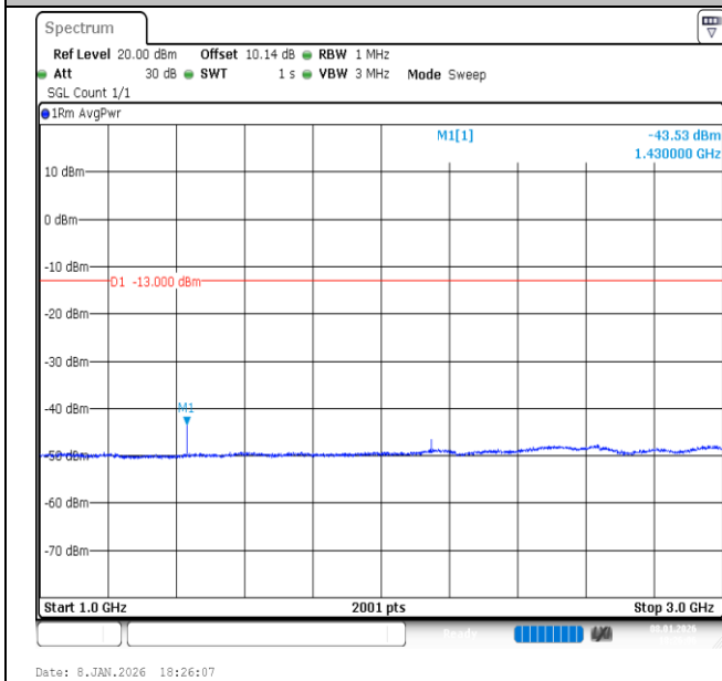
Band12-10MHz-QPSK-23130-1RB#49-1000~3000-PASS
