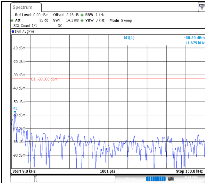
Band12-10MHz-QPSK-23095-1RB#49-0.009~0.15-PASS
