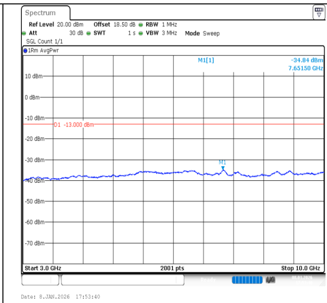
Band12-5MHz-16QAM-23035-25RB#0-3000~10000-PASS
