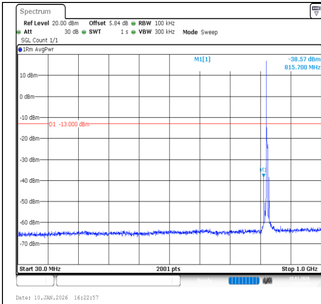
Band26 (824-849)-5MHz-QPSK-26815-1RB#0-30~1000-PASS
