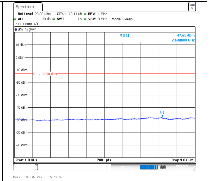
Band26 (824-849)-5MHz-QPSK-27015-25RB#0-1000~3000-PASS
