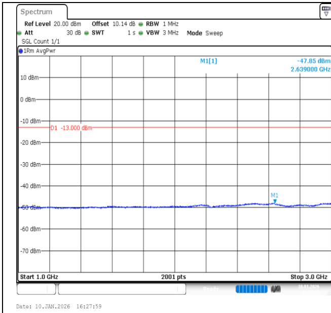
Band26 (824-849)-5MHz-16QAM-27015-1RB#0-1000-3000-PASS
