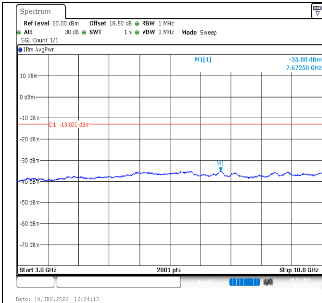
Band26 (824-849)-5MHz-16QAM-26815-1RB#24-3000~10000-PASS
