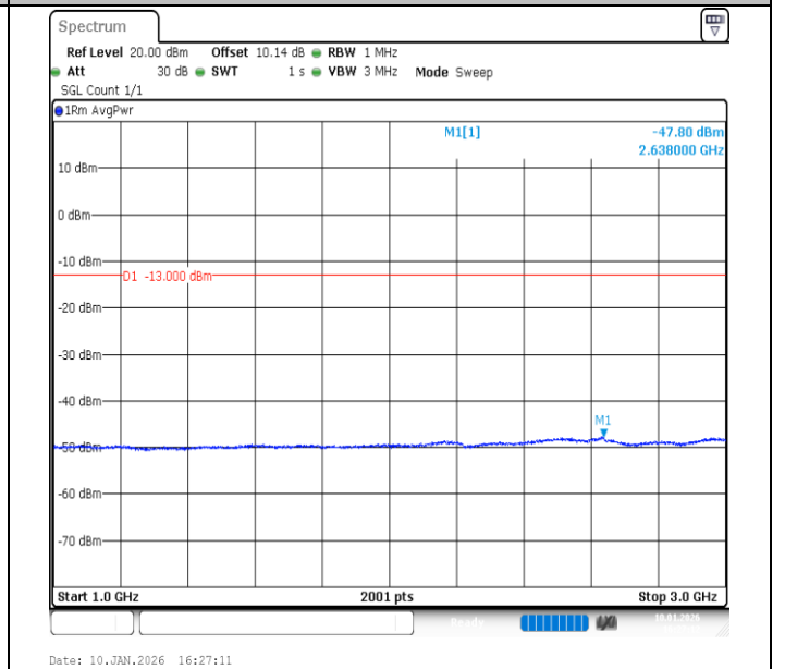
Band26 (824-849)-5MHz-16QAM-26915-25RB#0-1000~3000-PASS
