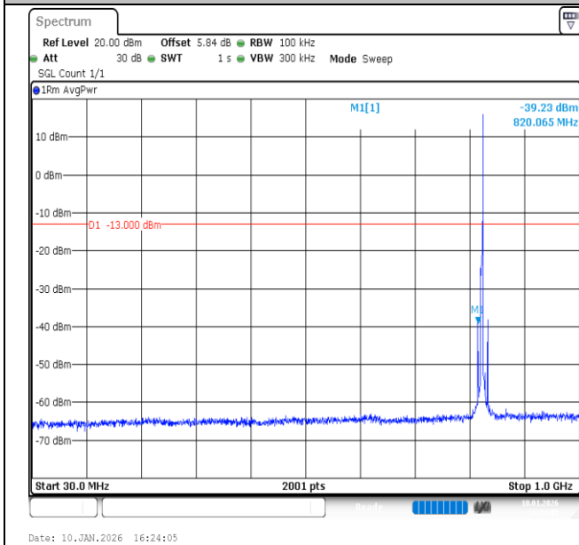
Band26 (824-849)-5MHz-16QAM-26815-1RB#24-30~1000-PASS
