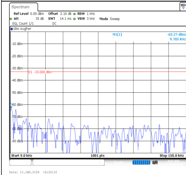
Band26 (824-849)-5MHz-16QAM-27015-1RB#24-0.009-0.15-PASS
