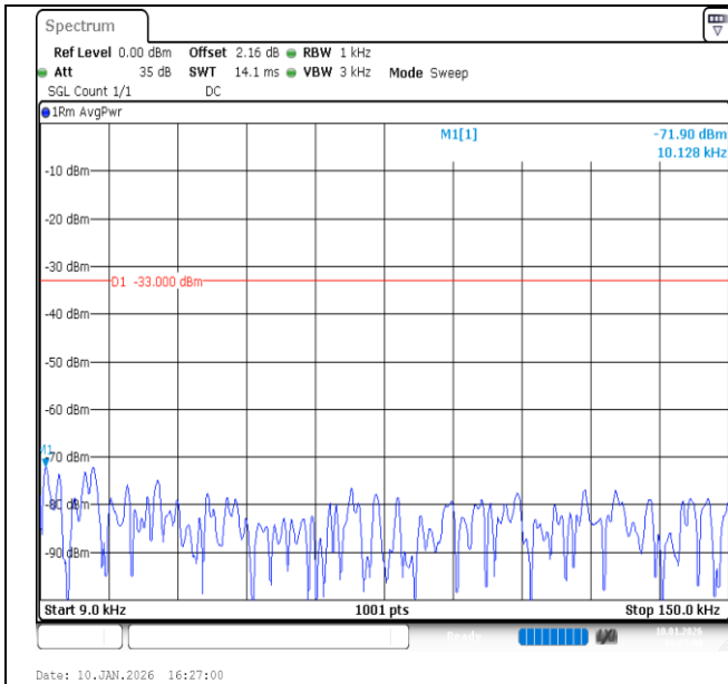
Band26 (824-849)-5MHz-16QAM-26915-25RB#0-0.009~0.15-PASS
