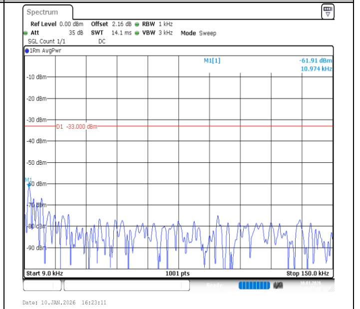
Band26 (824-849)-5MHz-16QAM-26815-1RB#0-0.009~0.15-PASS
