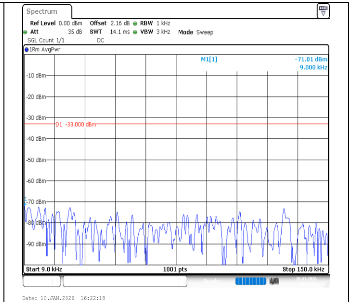
Band26 (824-849)-3MHz-16QAM-27025-15RB#0-0.009~0.15-PASS
