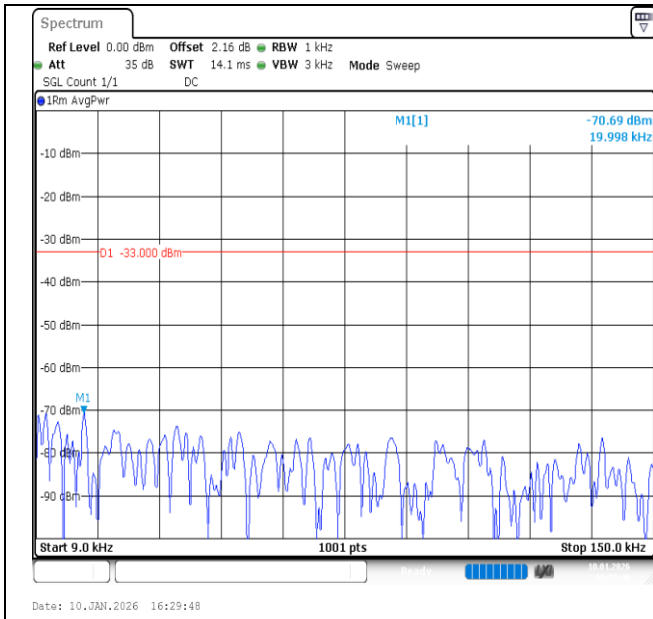
Band26 (824-849)-10MHz-QPSK-26840-1RB#0-0.009~0.15-PASS
