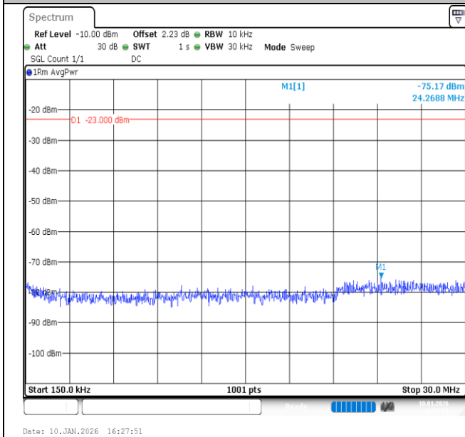
Band26 (824-849)-5MHz-16QAM-27015-1RB#0-0.15~30-PASS
