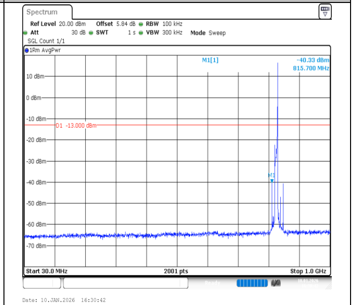
Band26 (824-849)-10MHz-QPSK-26840-1RB#49-30~1000-PASS
