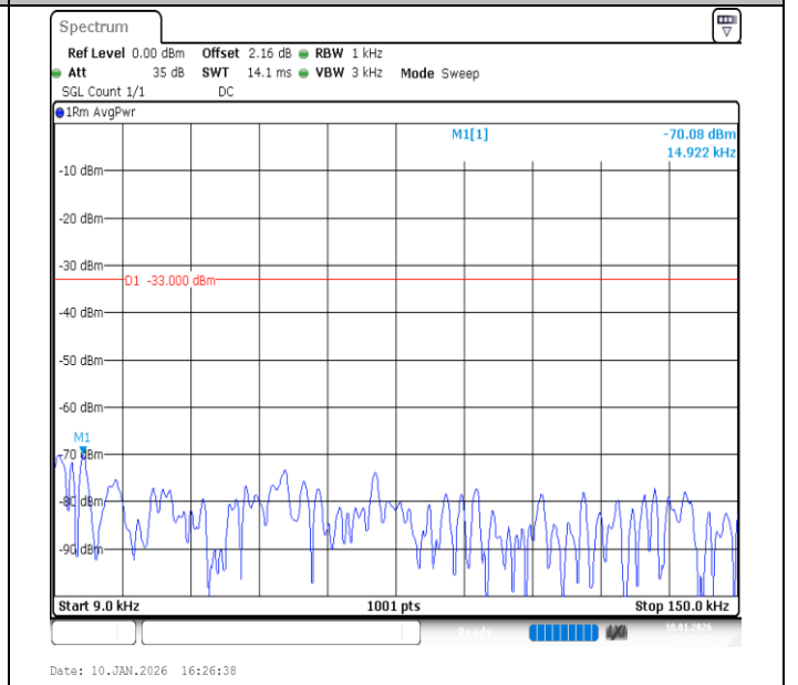
Band26 (824-849)-5MHz-QPSK-26915-25RB#0-0.009~0.15-PASS
