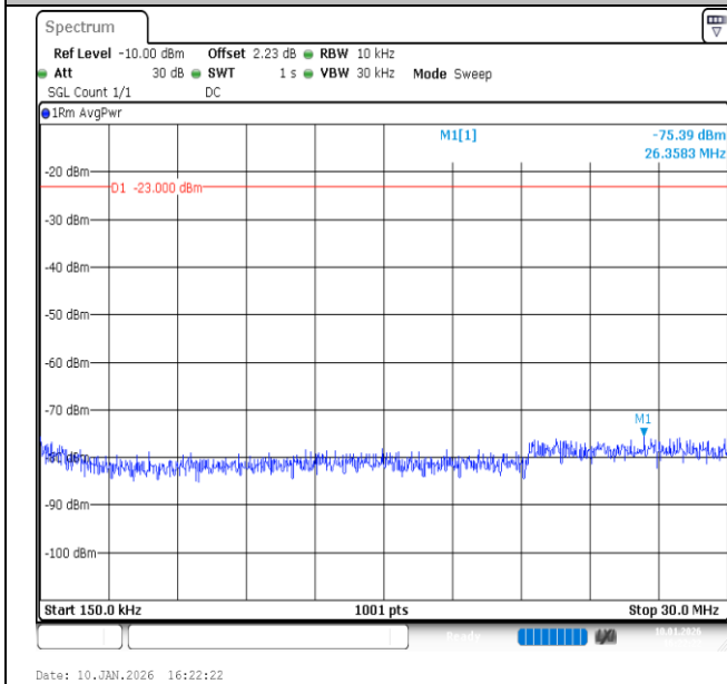
Band26 (824-849)-3MHz-16QAM-27025-15RB#0-0.15~30-PASS
