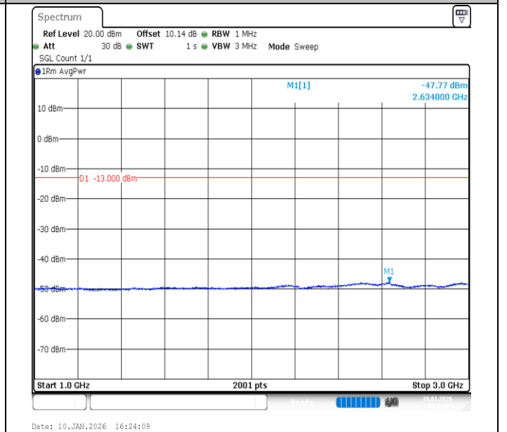
Band26 (824-849)-5MHz-16QAM-26815-1RB#24-1000~3000-PASS
