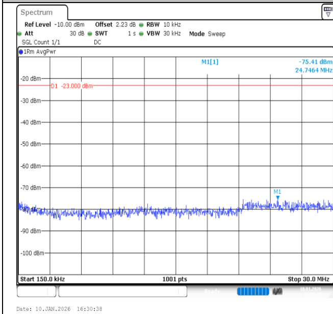
Band26 (824-849)-10MHz-QPSK-26840-1RB#49-0.15~30-PASS
