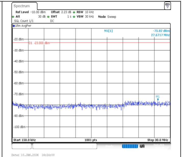
Band26 (824-849)-5MHz-16QAM-26815-1RB#24-0.15~30-PASS
