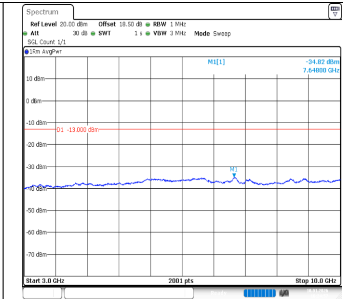
Band26 (824-849)-5MHz-16QAM-26815-25RB#0-3000~10000-PASS
