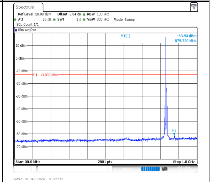
Band26 (824-849)-5MHz-QPSK-26915-1RB#0-30~1000-PASS
