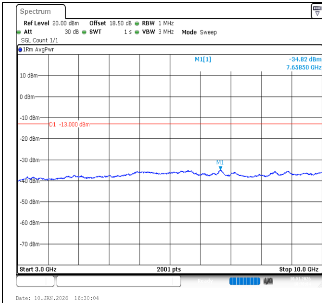
Band26 (824-849)-10MHz-QPSK-26840-1RB#0-3000~10000-PASS
