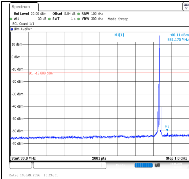
Band26 (824-849)-5MHz-QPSK-26915-1RB#24-30~1000-PASS
