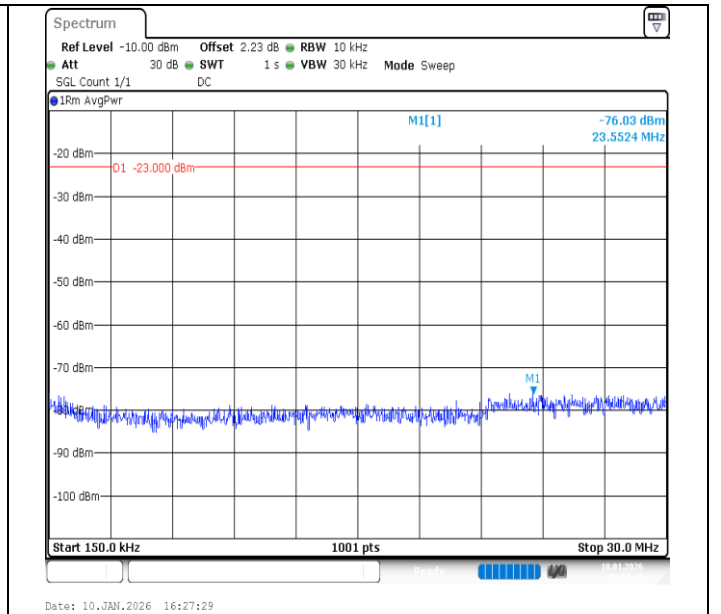
Band26 (824-849)-5MHz-QPSK-27015-1RB#0-0.15~30-PASS
