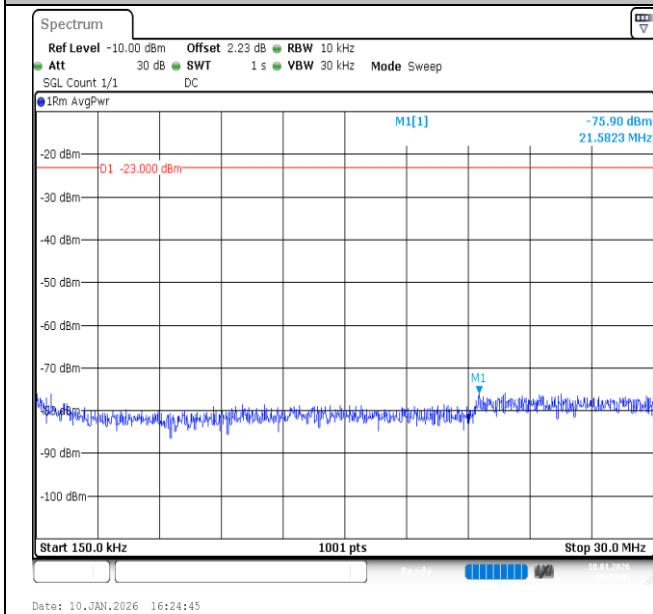
Band26 (824-849)-5MHz-16QAM-26815-25RB#0-0.15~30-PASS
