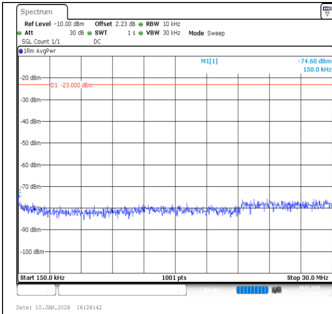
Band26 (824-849)-5MHz-QPSK-26915-25RB#0-0.15~30-PASS
