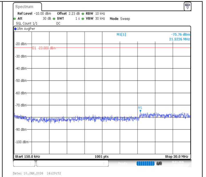
Band26 (824-849)-10MHz-QPSK-26840-1RB#0-0.15~30-PASS
