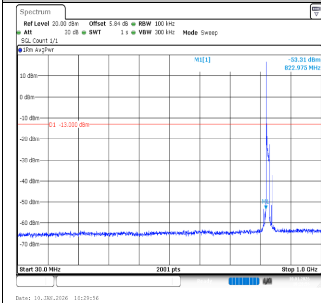
Band26 (824-849)-10MHz-QPSK-26840-1RB#0-30~1000-PASS
