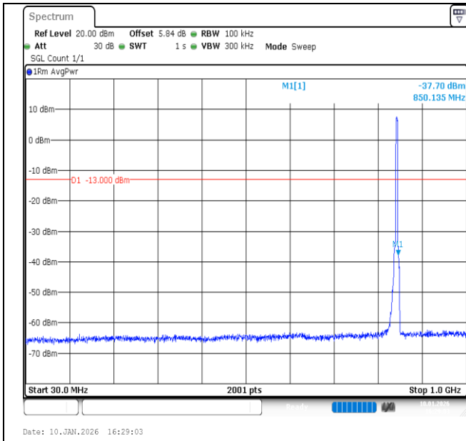
Band26 (824-849)-5MHz-QPSK-27015-25RB#0-30~1000-PASS
