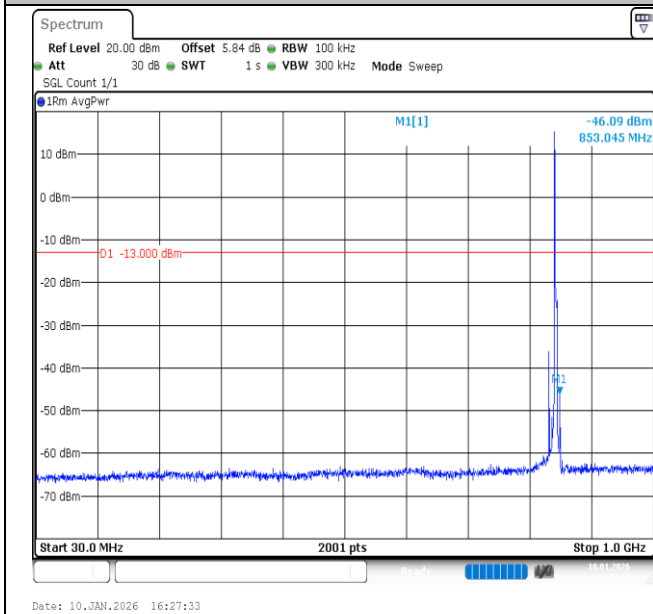
Band26 (824-849)-5MHz-QPSK-27015-1RB#0-30~1000-PASS
