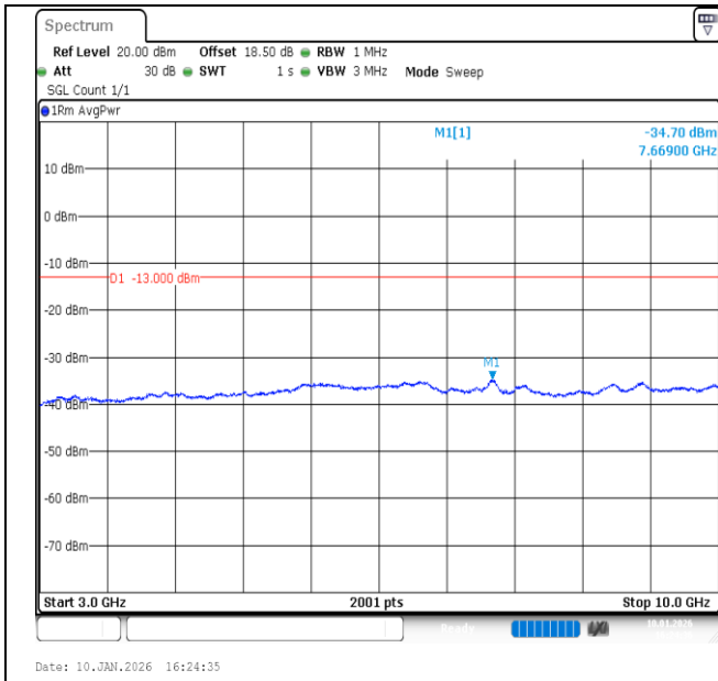
Band26 (824-849)-5MHz-QPSK-26815-25RB#0-3000~10000-PASS
