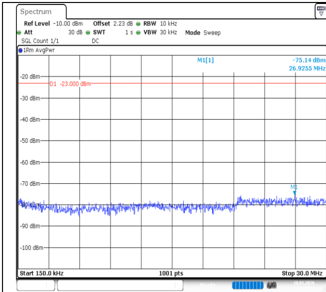
Band26 (824-849)-3MHz-16QAM-27025-1RB#0-0.15~30-PASS
