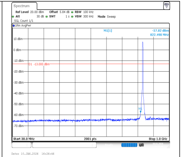
Band26 (824-849)-5MHz-QPSK-26915-25RB#0-30~1000-PASS
