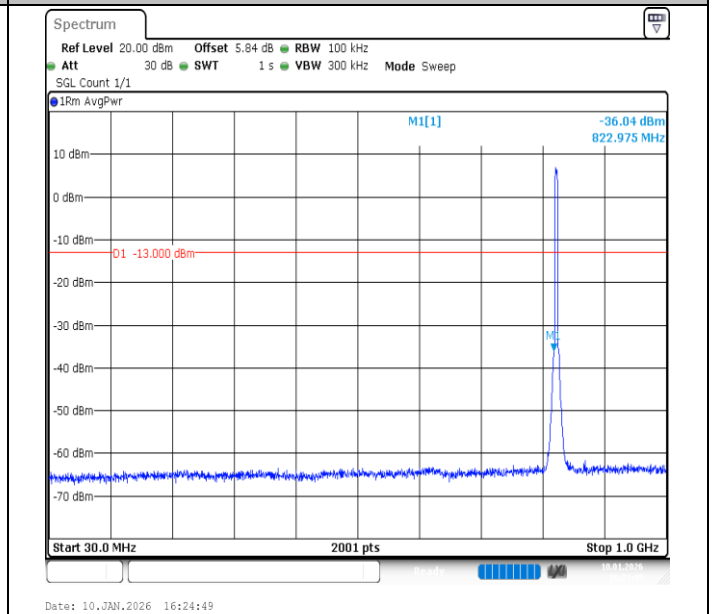
Band26 (824-849)-5MHz-16QAM-26815-25RB#0-30~1000-PASS
