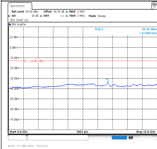
Band26 (824-849)-5MHz-QPSK-27015-25RB#0-3000~10000-PASS
