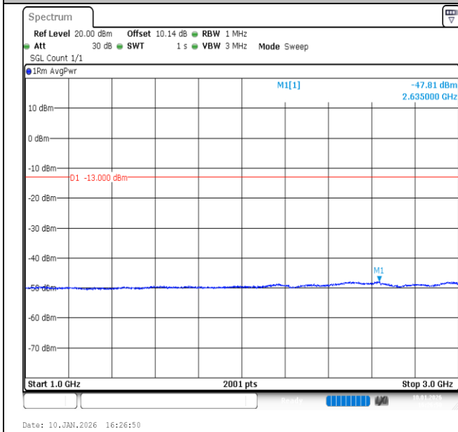
Band26 (824-849)-5MHz-QPSK-26915-25RB#0-1000~3000-PASS
