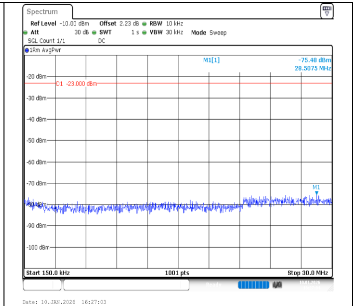
Band26 (824-849)-5MHz-16QAM-26915-25RB#0-0.15~30-PASS
