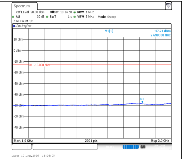
Band26 (824-849)-5MHz-QPSK-26915-1RB#24-1000~3000-PASS
