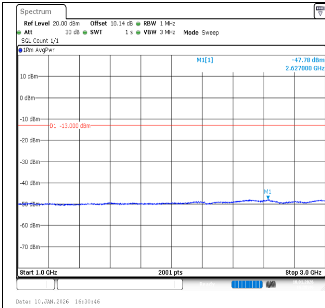
Band26 (824-849)-10MHz-QPSK-26840-1RB#49-1000~3000-PASS
