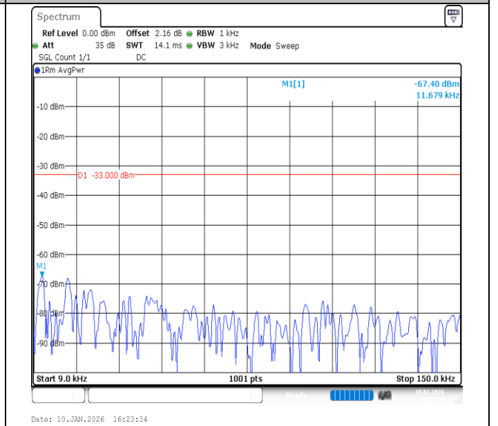
Band26 (824-849)-5MHz-QPSK-26815-1RB#24-0.009~0.15-PASS
