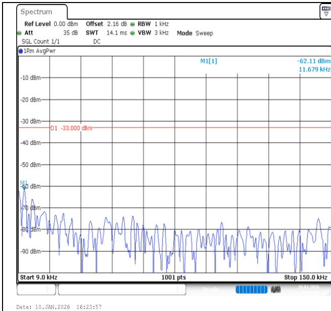
Band26 (824-849)-5MHz-16QAM-26815-1RB#24-0.009~0.15-PASS
