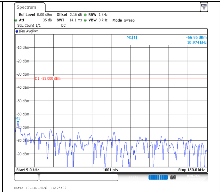
Band26 (824-849)-5MHz-QPSK-26915-1RB#0-0.009~0.15-PASS
