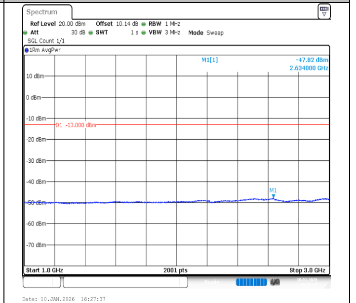
Band26 (824-849)-5MHz-QPSK-27015-1RB#0-1000~3000-PASS
