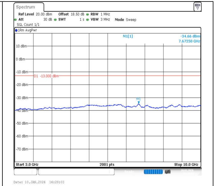
Band26 (824-849)-5MHz-16QAM-27015-1RB#0-3000-10000-PASS
