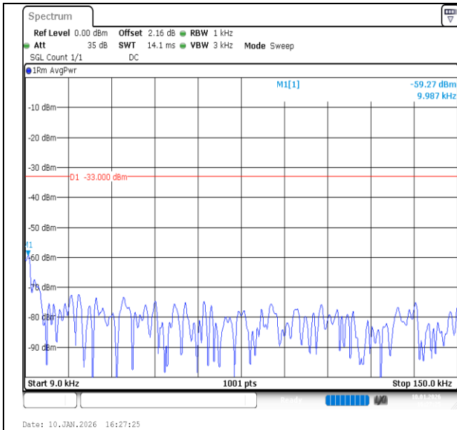
Band26 (824-849)-5MHz-QPSK-27015-1RB#0-0.009~0.15-PASS
