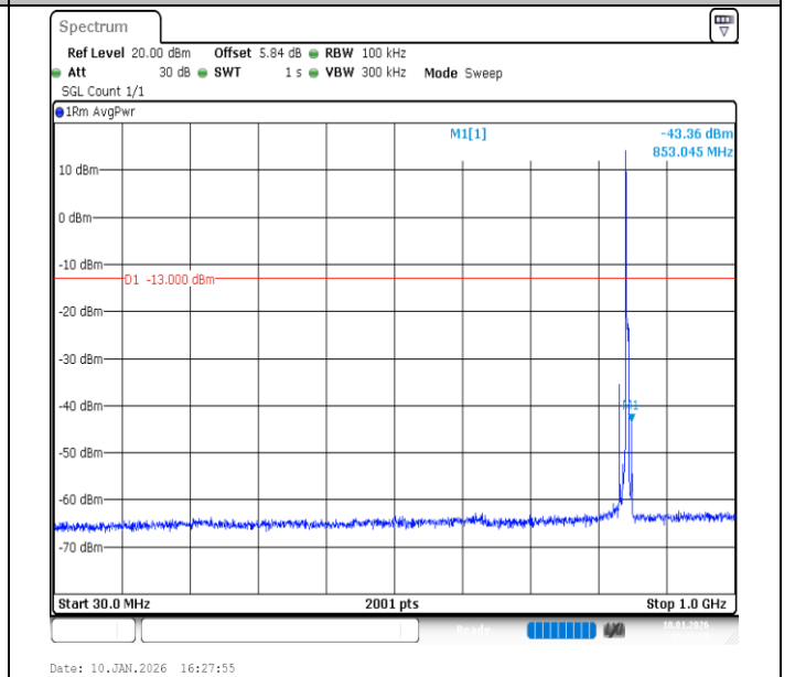
Band26 (824-849)-5MHz-16QAM-27015-1RB#0-30~1000-PASS
