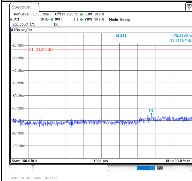
Band26 (824-849)-5MHz-QPSK-26915-1RB#0-0.15~30-PASS
