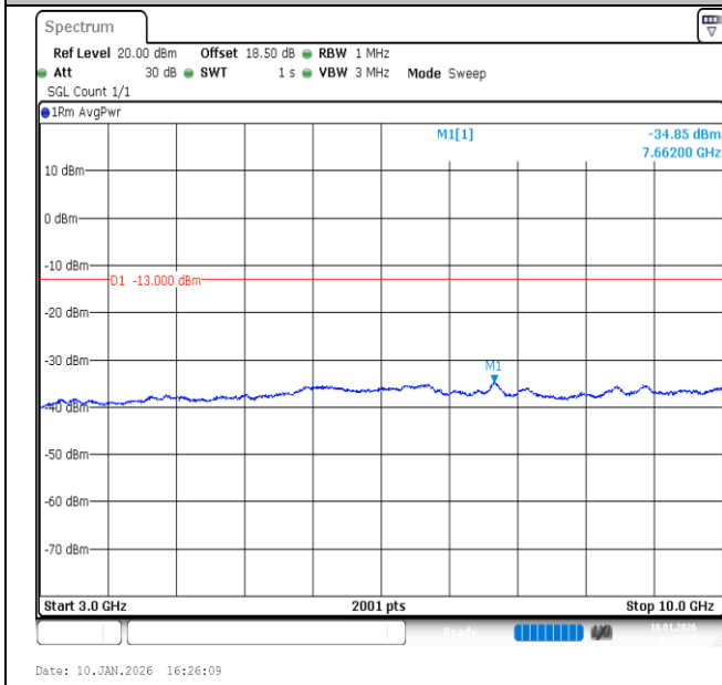
Band26 (824-849)-5MHz-QPSK-26915-1RB#24-3000~10000-PASS
