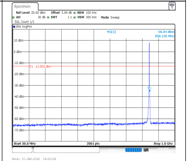
Band26 (824-849)-3MHz-16QAM-27025-15RB#0-30~1000-PASS
