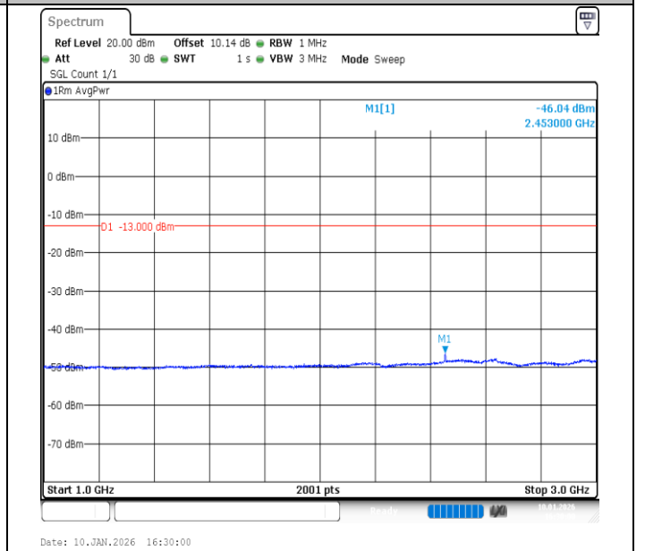
Band26 (824-849)-10MHz-QPSK-26840-1RB#0-1000~3000-PASS
