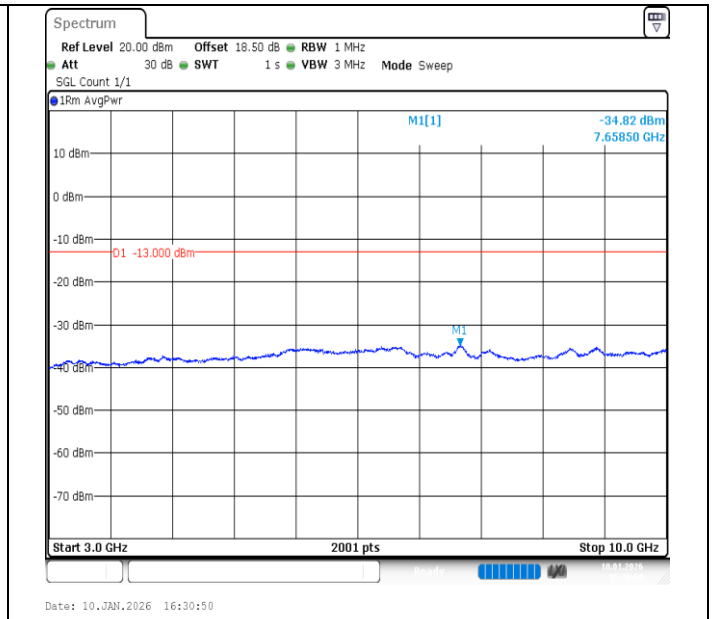
Band26 (824-849)-10MHz-QPSK-26840-1RB#49-3000~10000-PASS
