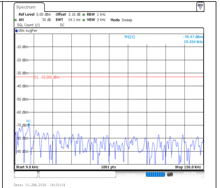
Band26 (824-849)-10MHz-QPSK-26840-1RB#49-0.009~0.15-PASS
