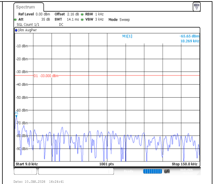
Band26 (824-849)-5MHz-16QAM-26815-25RB#0-0.009~0.15-PASS
