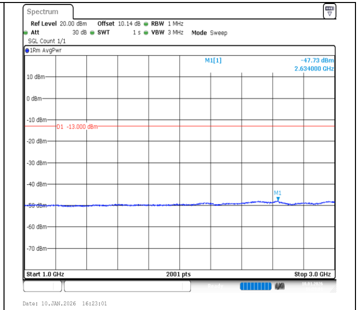
Band26 (824-849)-5MHz-QPSK-26815-1RB#0-1000~3000-PASS
