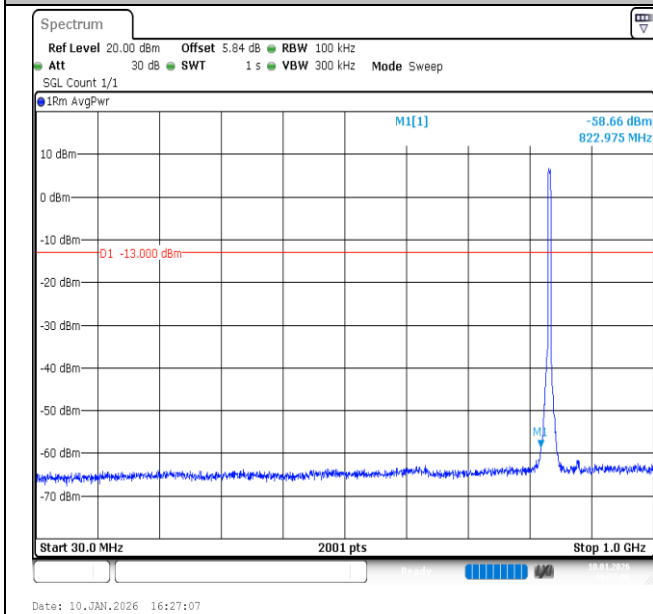
Band26 (824-849)-5MHz-16QAM-26915-25RB#0-30~1000-PASS
