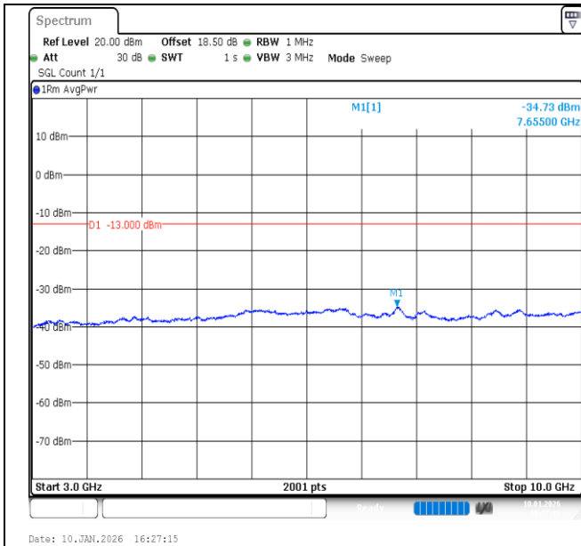
Band26 (824-849)-5MHz-16QAM-26915-25RB#0-3000~10000-PASS
