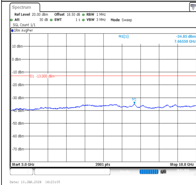
Band26 (824-849)-5MHz-QPSK-26815-1RB#0-3000~10000-PASS
