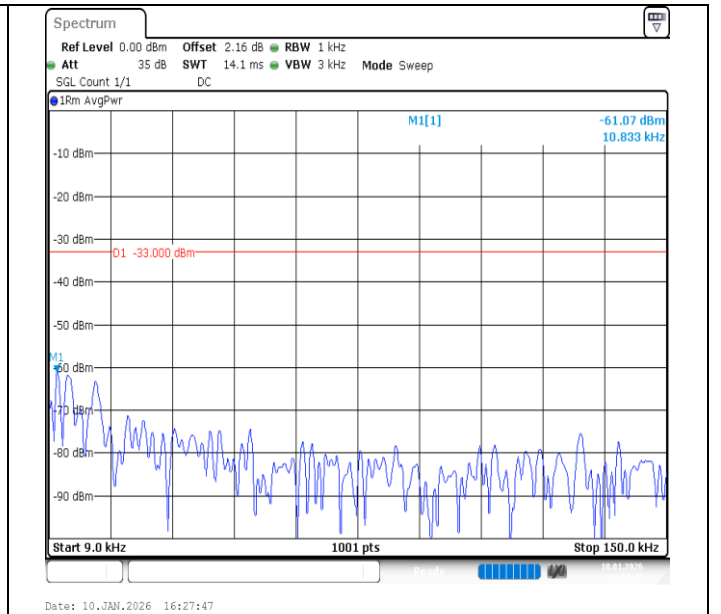
Band26 (824-849)-5MHz-16QAM-27015-1RB#0-0.009~0.15-PASS
