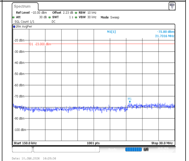
Band26 (824-849)-5MHz-16QAM-27015-1RB#24-0.15-30-PASS
