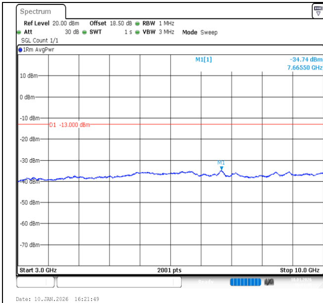
Band26 (824-849)-3MHz-16QAM-27025-1RB#14-3000~10000-PASS
