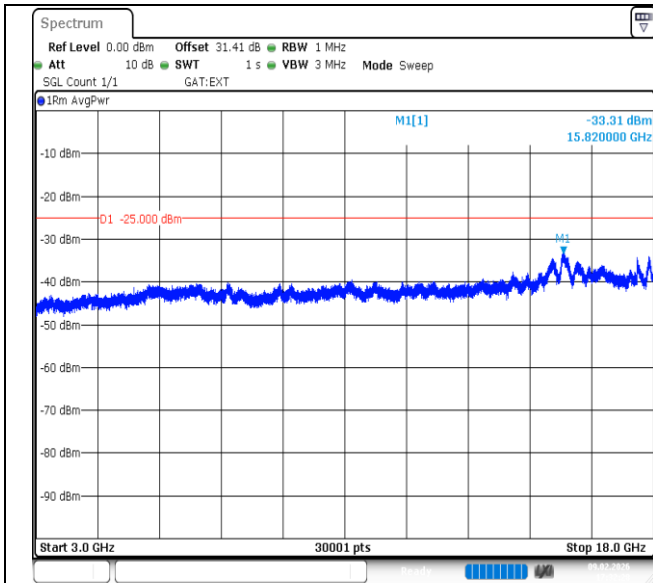
Band41-10MHz-16QAM-41540-1RB#49-3000~18000-PASS
