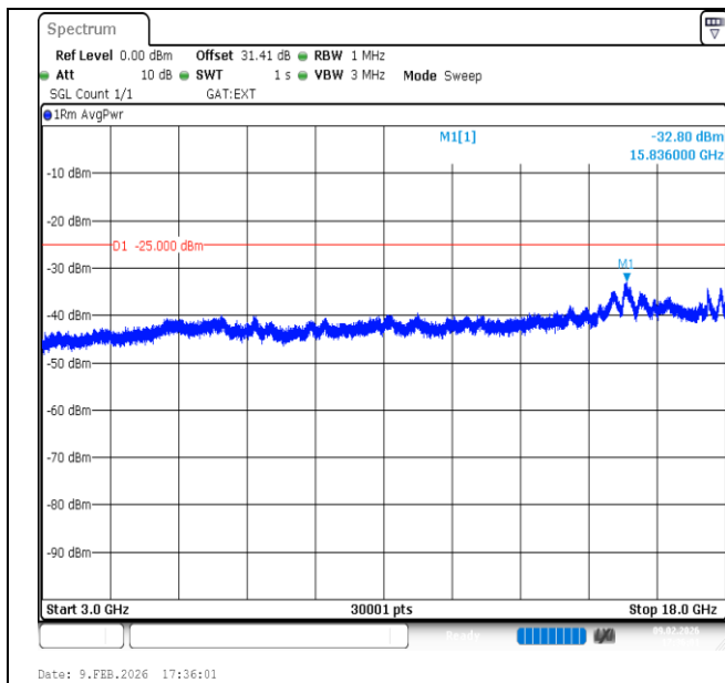
Band41-10MHz-QPSK-41540-50RB#0-3000~18000-PASS
