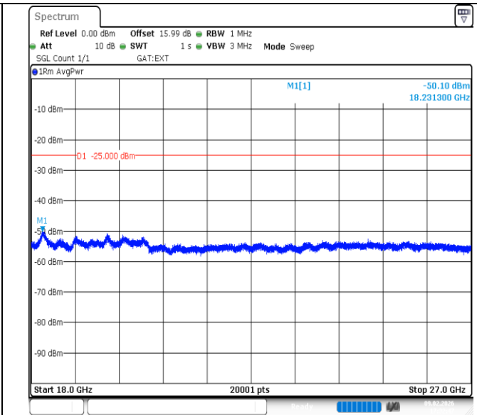
Band41-10MHz-16QAM-41540-1RB#49-18000~27000-PASS
