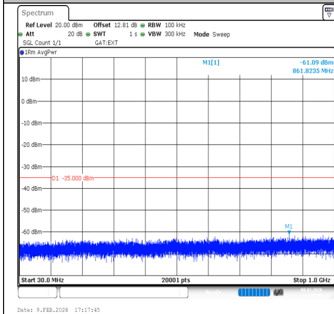
Band41-10MHz-16QAM-40620-50RB#0-30~1000-PASS
