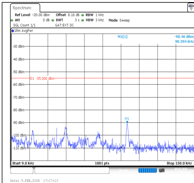
Band41-10MHz-16QAM-40620-50RB#0-0.009~0.15-PASS
