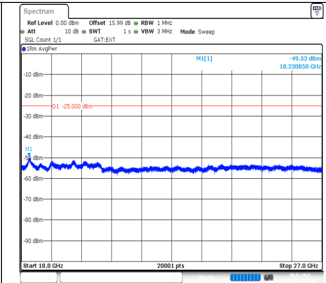
Band41-10MHz-16QAM-40620-50RB#0-18000~27000-PASS
