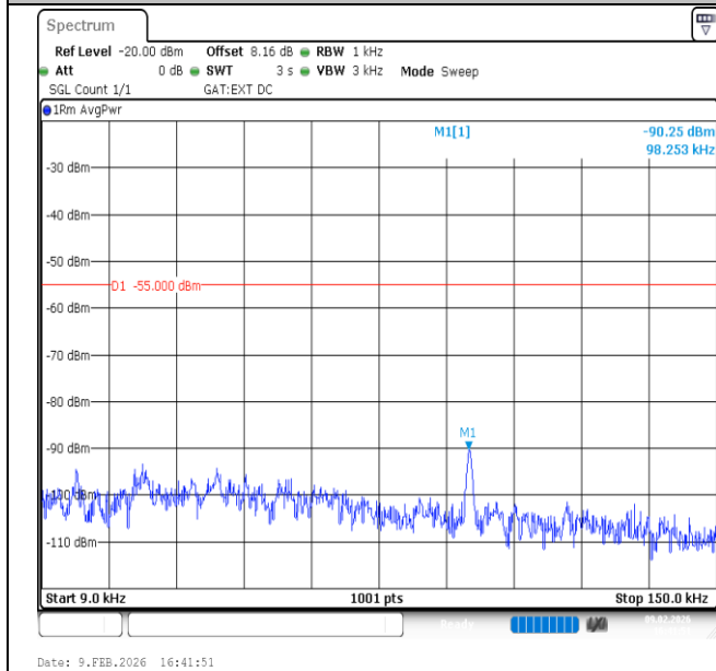
Band41-10MHz-16QAM-39700-1RB#0-0.009~0.15-PASS
