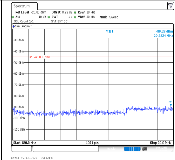
Band41-10MHz-16QAM-39700-1RB#0-0.15~30-PASS
