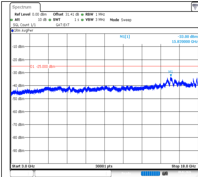
Band41-10MHz-16QAM-40620-50RB#0-3000~18000-PASS
