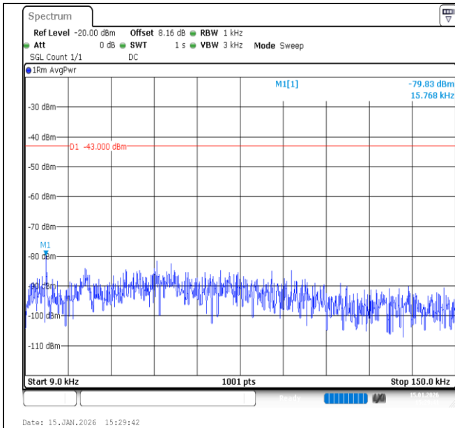
Band66-10MHz-16QAM-132022-1RB#49-0.009~0.15-PASS
