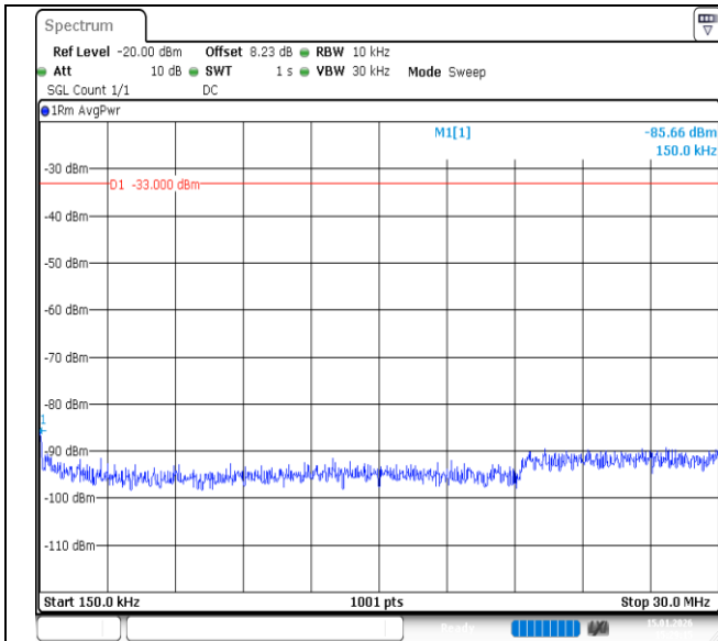
Band66-10MHz-QPSK-132022-1RB#49-0.15~30-PASS
