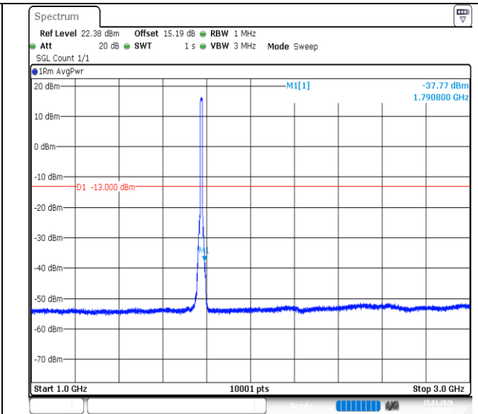
Band66-10MHz-QPSK-132622-50RB#0-1000~3000-PASS
