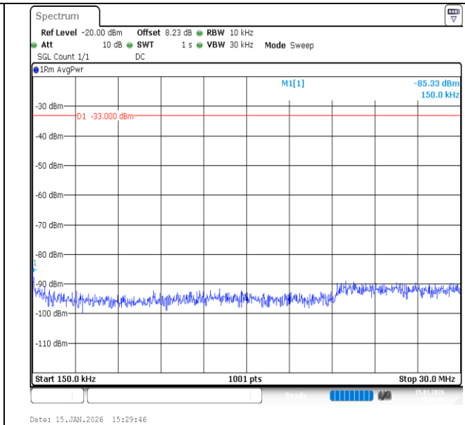
Band66-10MHz-16QAM-132022-1RB#49-0.15~30-PASS
