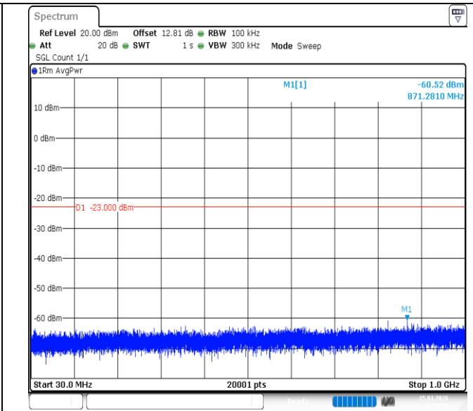
Band66-10MHz-16QAM-132022-1RB#0-30~1000-PASS
