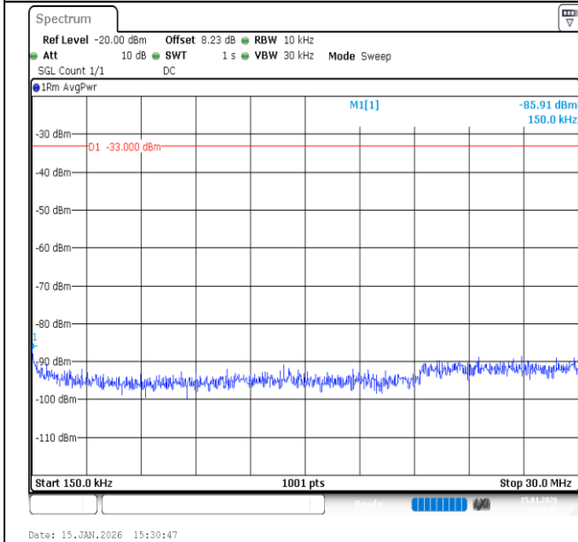
Band66-10MHz-16QAM-132022-50RB#0-0.15~30-PASS
