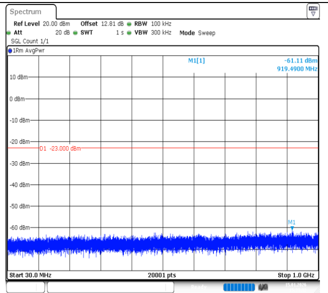
Band66-10MHz-QPSK-132322-50RB#0-30~1000-PASS
