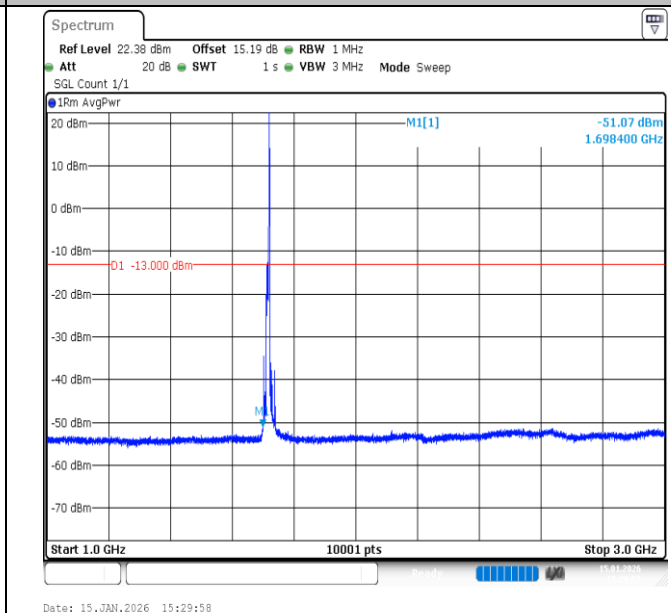
Band66-10MHz-16QAM-132022-1RB#49-1000~3000-PASS
