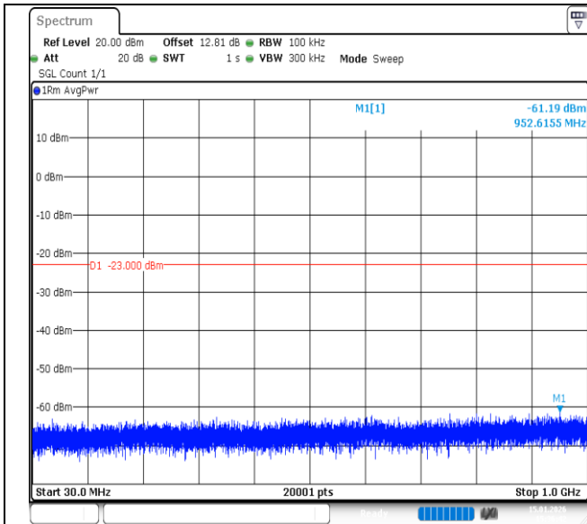
Band66-10MHz-QPSK-132622-50RB#0-30~1000-PASS
