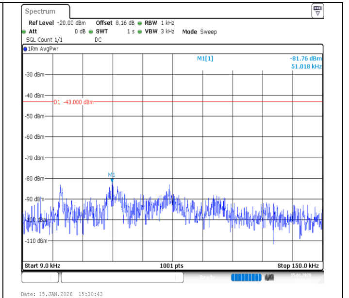
Band66-10MHz-16QAM-132022-50RB#0-0.009~0.15-PASS
