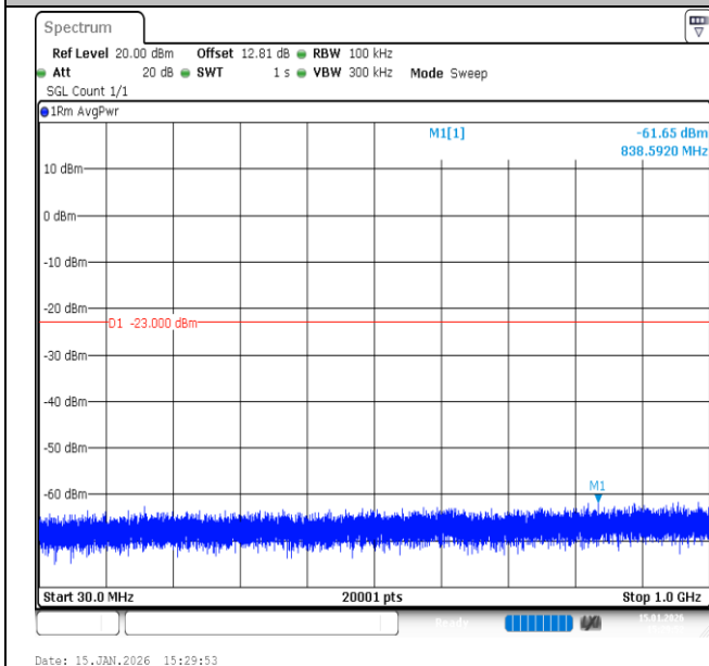
Band66-10MHz-16QAM-132022-1RB#49-30~1000-PASS
