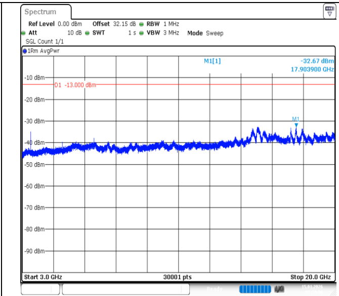
Band66-15MHz-QPSK-132047-1RB#74-3000-20000-PASS
