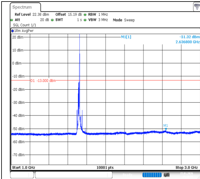
Band66-15MHz-QPSK-132047-1RB#74-1000-3000-PASS
