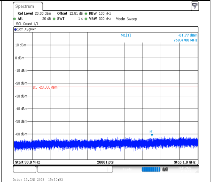
Band66-10MHz-16QAM-132022-50RB#0-30~1000-PASS
