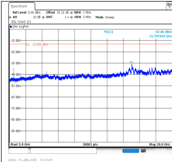
Band66-10MHz-16QAM-132022-1RB#49-3000~20000-PASS
