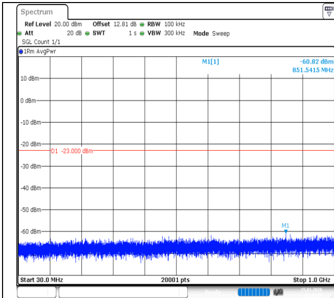
Band66-15MHz-16QAM-132322-75RB#0-30~1000-PASS
