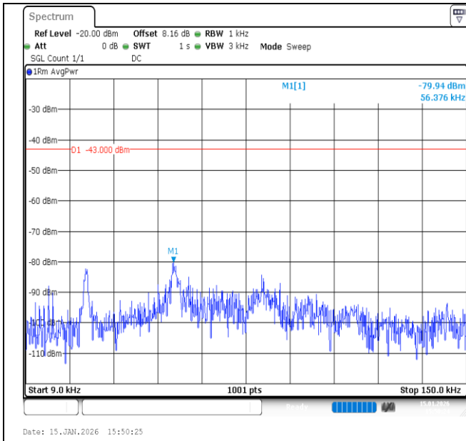
Band66-20MHz-QPSK-132072-100RB#0-0.009~0.15-PASS
