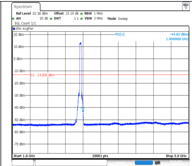
Band66-20MHz-QPSK-132572-100RB#0-1000~3000-PASS
