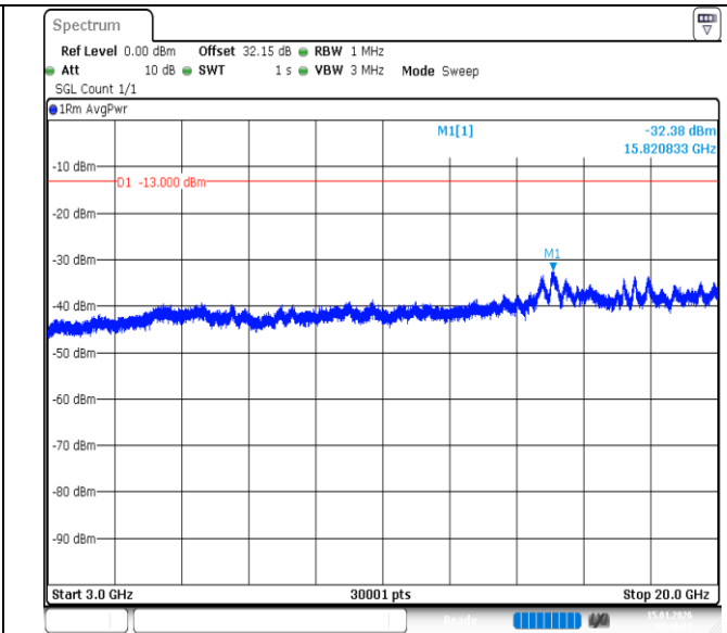
Band66-15MHz-16QAM-132597-75RB#0-3000~20000-PASS
