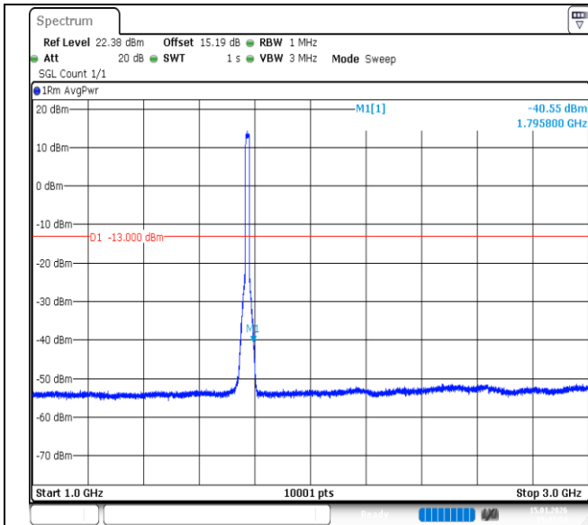
Band66-15MHz-16QAM-132597-75RB#0-1000~3000-PASS
