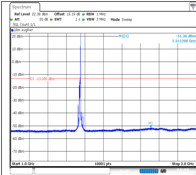
Band66-15MHz-16QAM-132322-1RB#74-1000~3000-PASS
