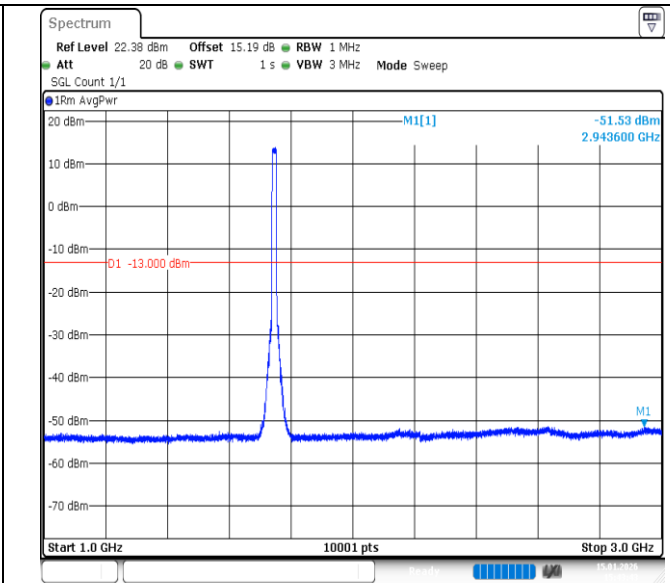
Band66-15MHz-16QAM-132322-75RB#0-1000~3000-PASS
