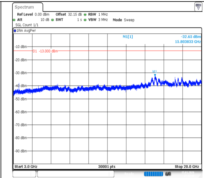
Band66-15MHz-16QAM-132322-1RB#74-3000~20000-PASS
