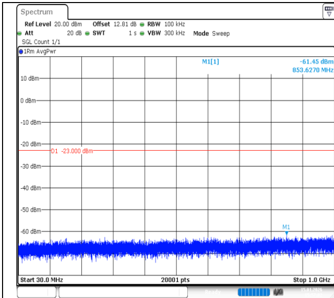
Band66-20MHz-QPSK-132572-100RB#0-30~1000-PASS
