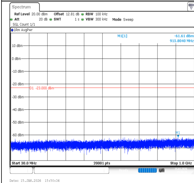
Band66-20MHz-QPSK-132072-100RB#0-30~1000-PASS
