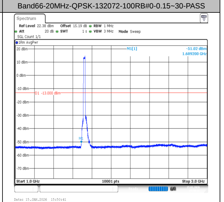
Band66-20MHz-QPSK-132072-100RB#0-1000~3000-PASS
