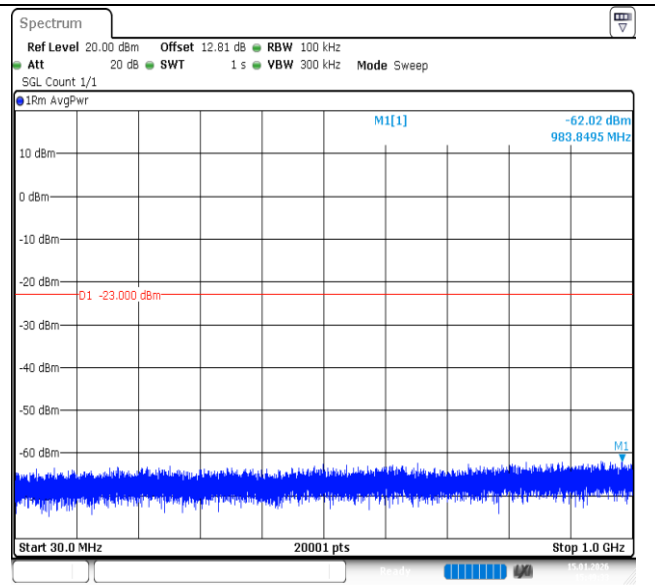
Band66-20MHz-QPSK-132072-1RB#99-30~1000-PASS
